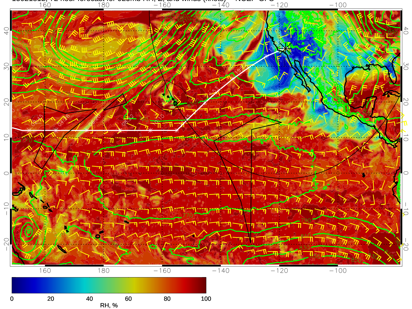
15021812, 72 hour forecast for 925mb RH, Z, and winds (knots) -- NCEP GFS
