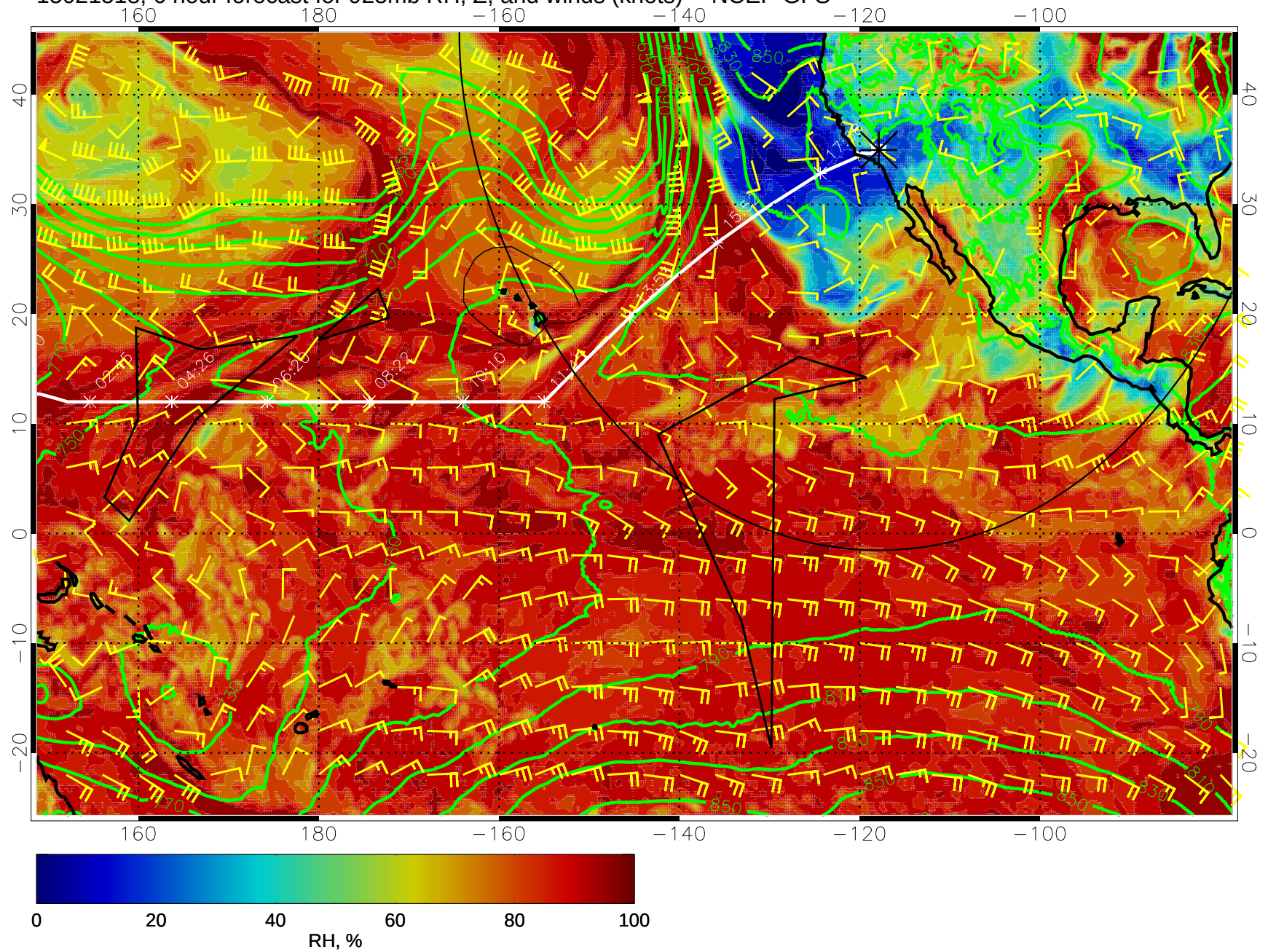
15021518, 6 hour forecast for 925mb RH, Z, and winds (knots) -- NCEP GFS
