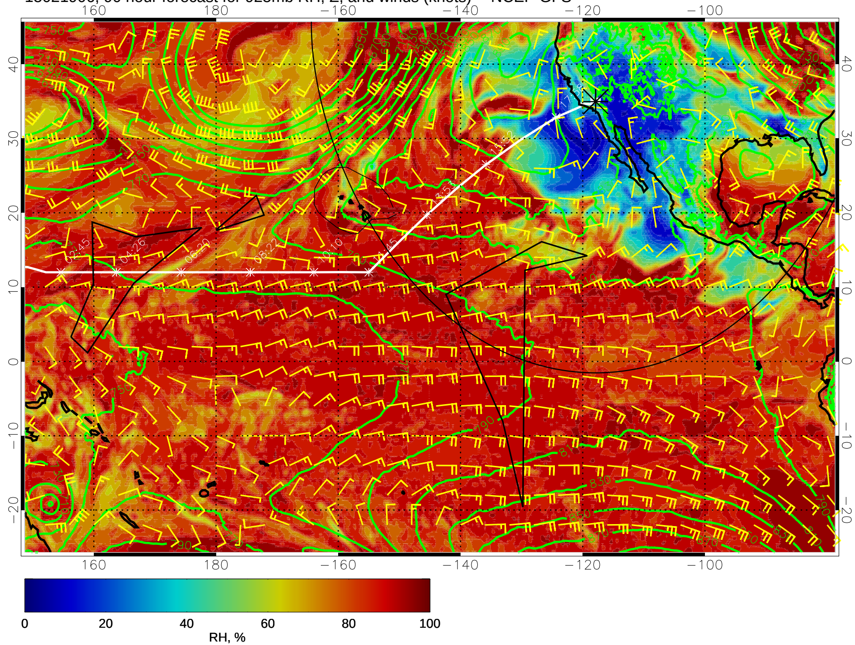
15021906, 90 hour forecast for 925mb RH, Z, and winds (knots) -- NCEP GFS
