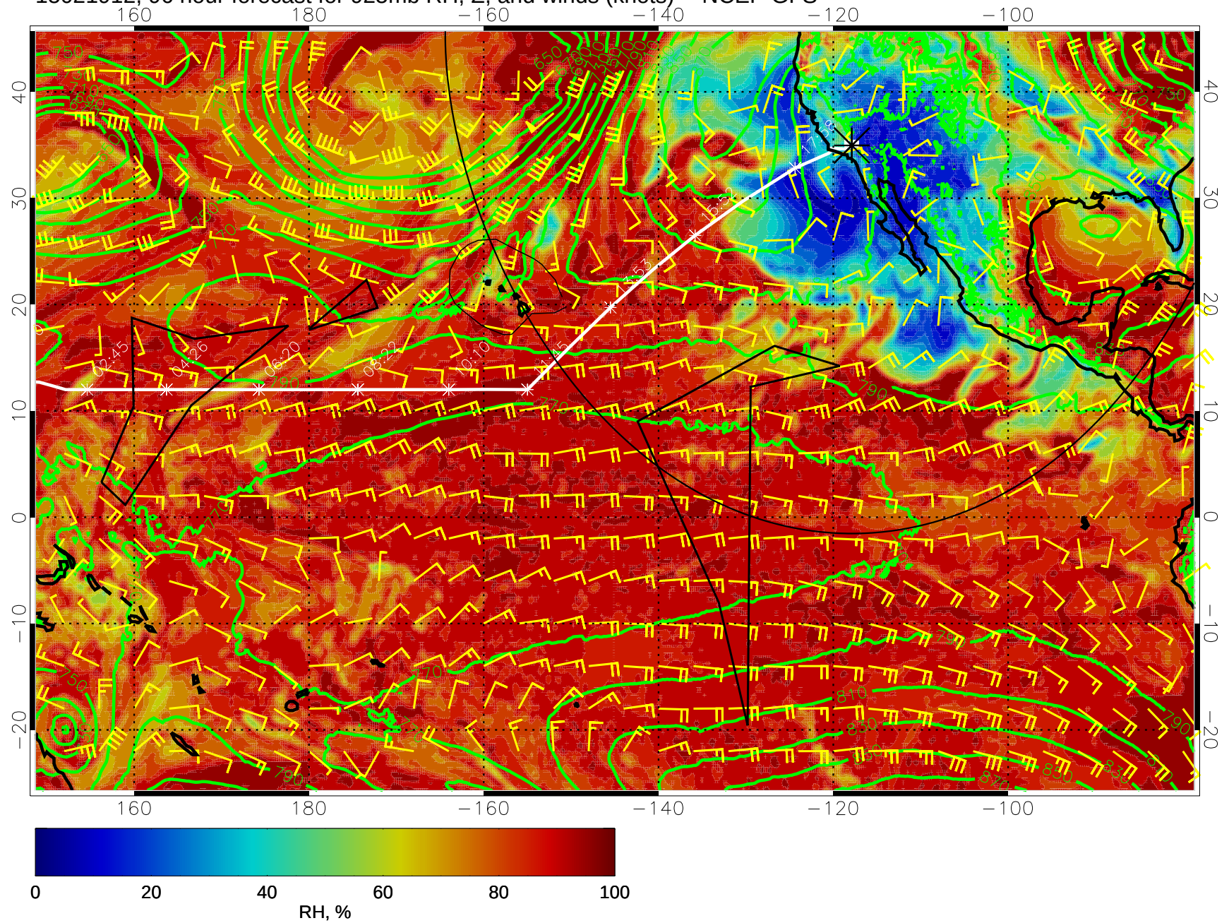
15021912, 96 hour forecast for 925mb RH, Z, and winds (knots) -- NCEP GFS
