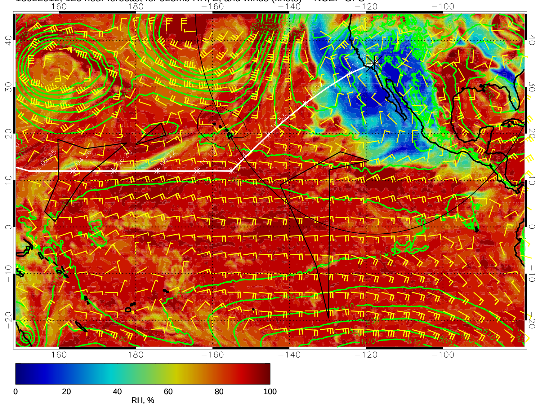
15022012, 120 hour forecast for 925mb RH, Z, and winds (knots) -- NCEP GFS
