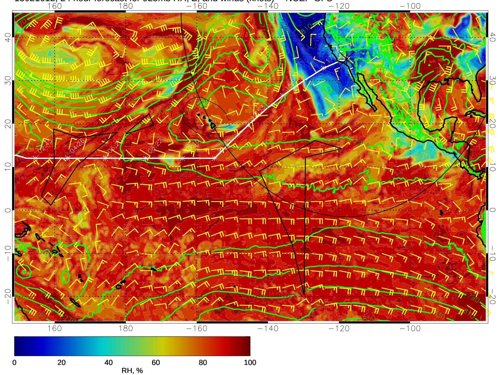
15021612, 24 hour forecast for 925mb RH, Z, and winds (knots) -- NCEP GFS
