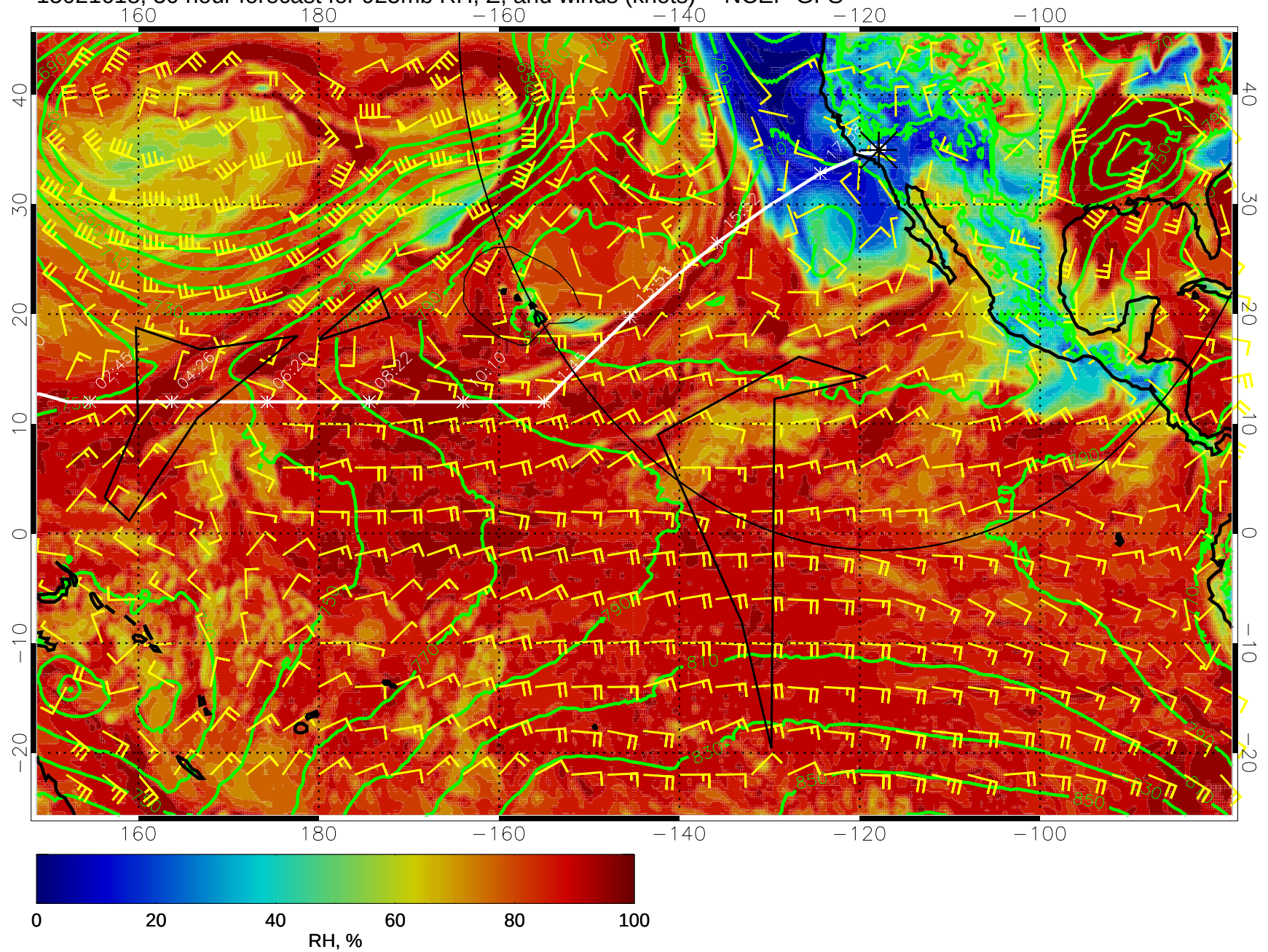
15021618, 30 hour forecast for 925mb RH, Z, and winds (knots) -- NCEP GFS
