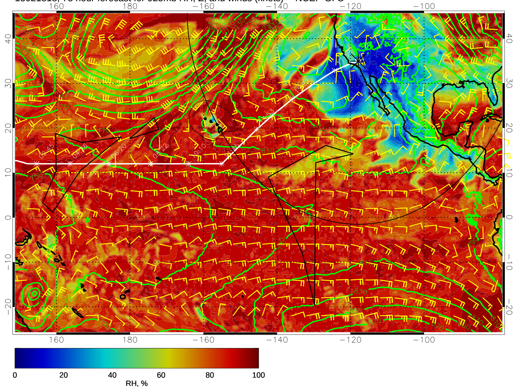
15021818, 78 hour forecast for 925mb RH, Z, and winds (knots) -- NCEP GFS
