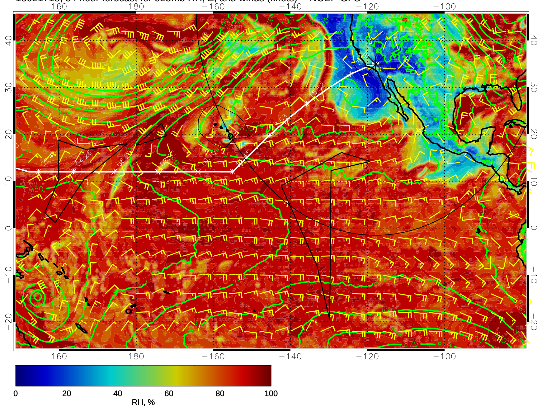
15021718, 54 hour forecast for 925mb RH, Z, and winds (knots) -- NCEP GFS
