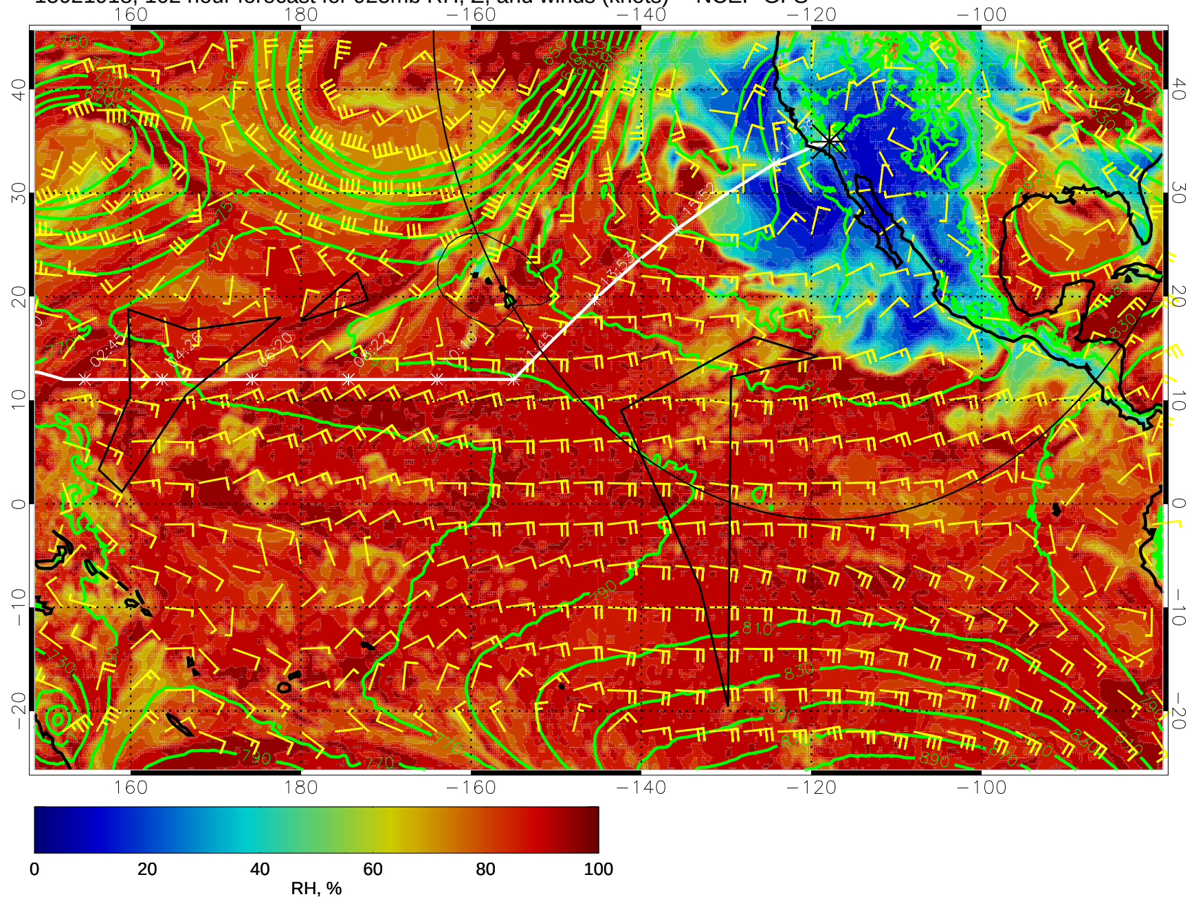
15021918, 102 hour forecast for 925mb RH, Z, and winds (knots) -- NCEP GFS
