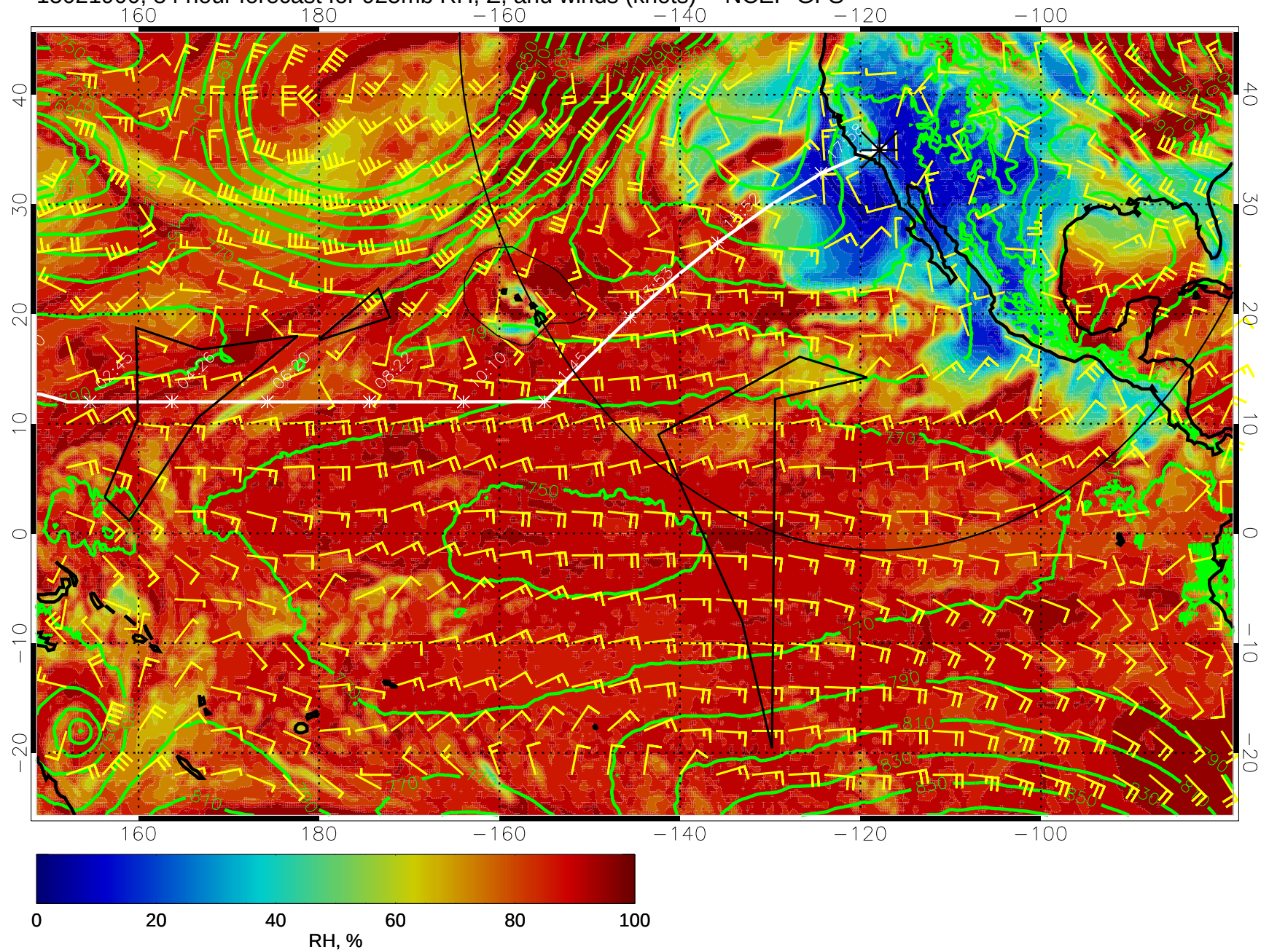
15021900, 84 hour forecast for 925mb RH, Z, and winds (knots) -- NCEP GFS
