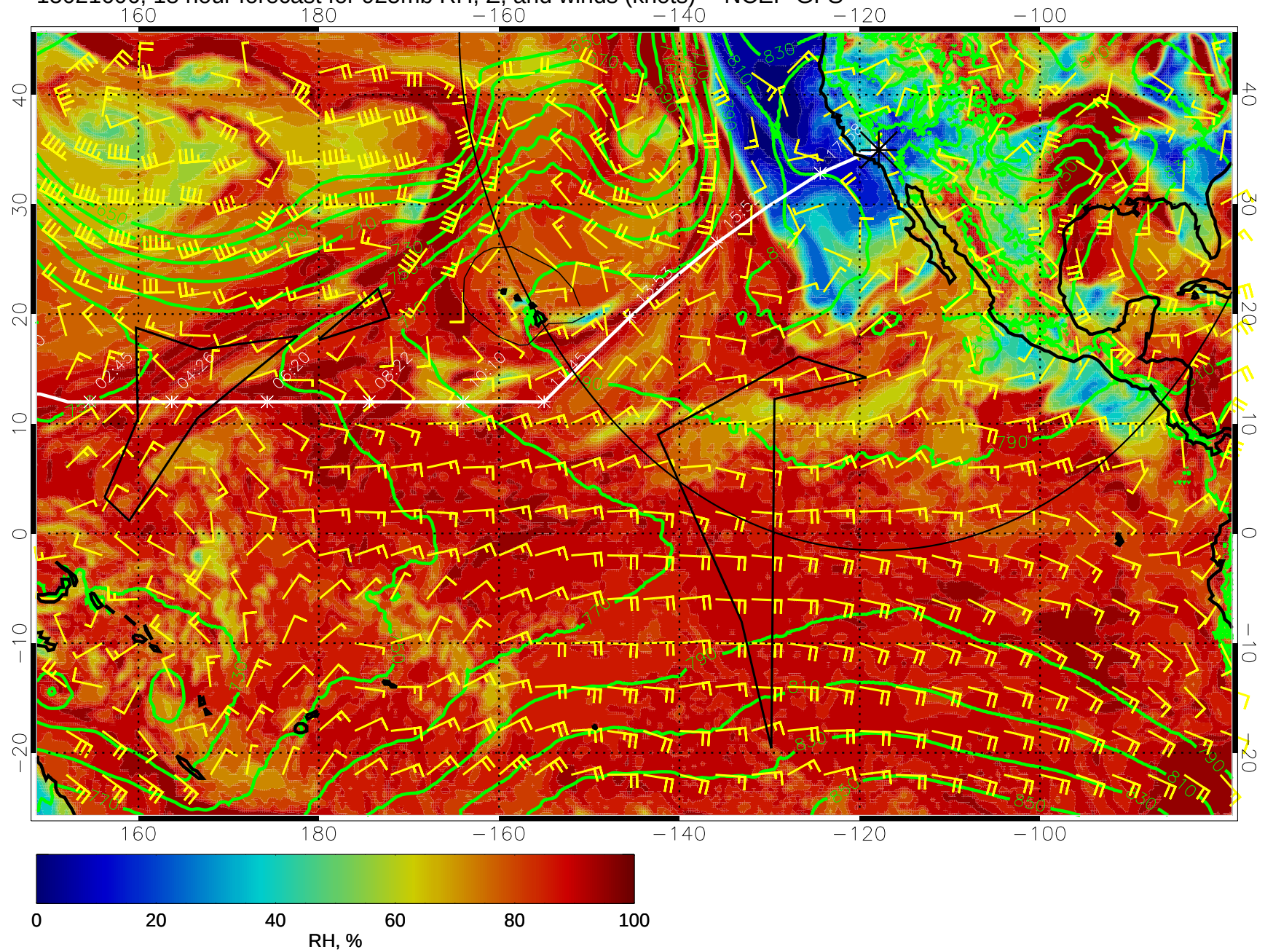
15021606, 18 hour forecast for 925mb RH, Z, and winds (knots) -- NCEP GFS
