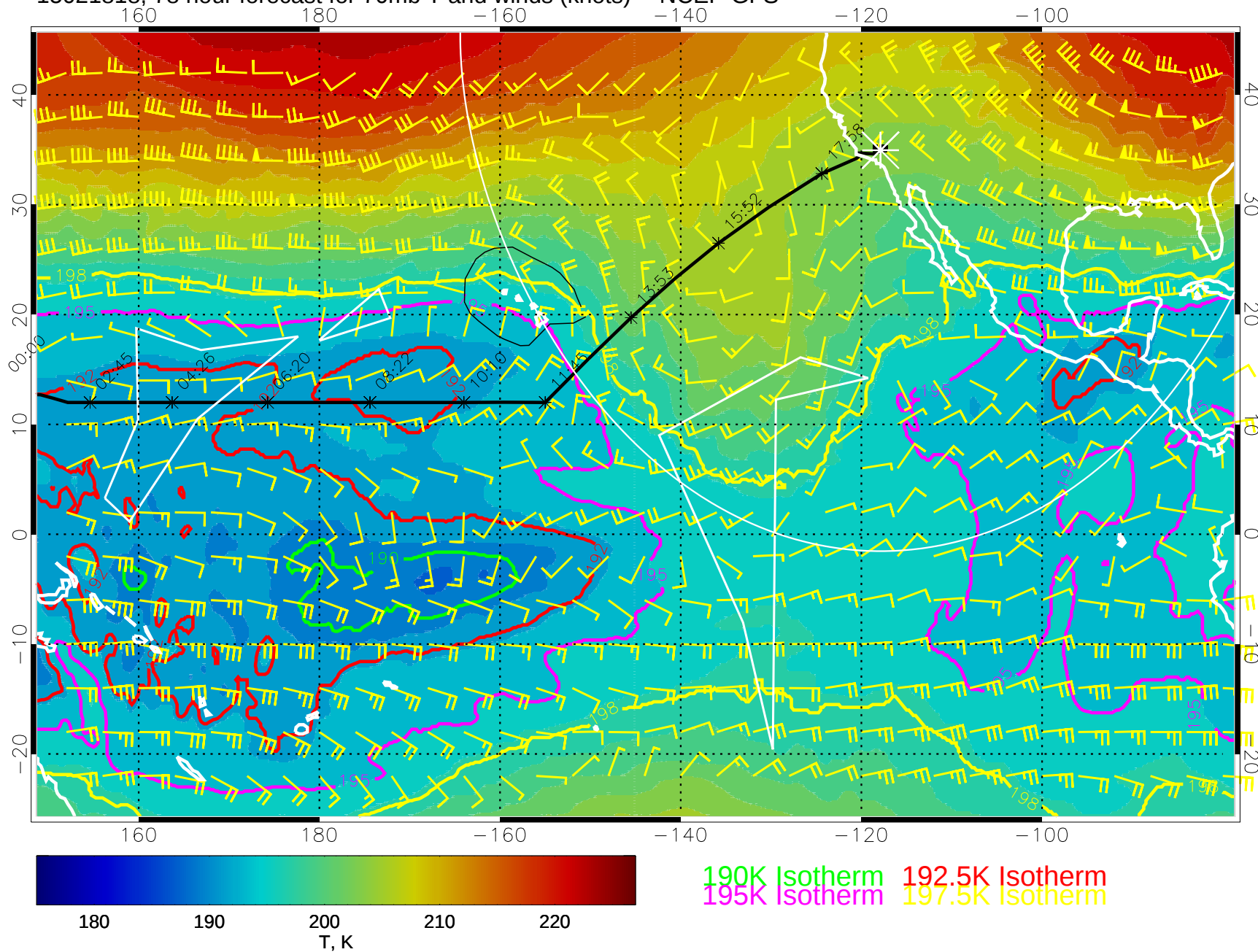
15021818, 78 hour forecast for 70mb T and winds (knots) -- NCEP GFS
