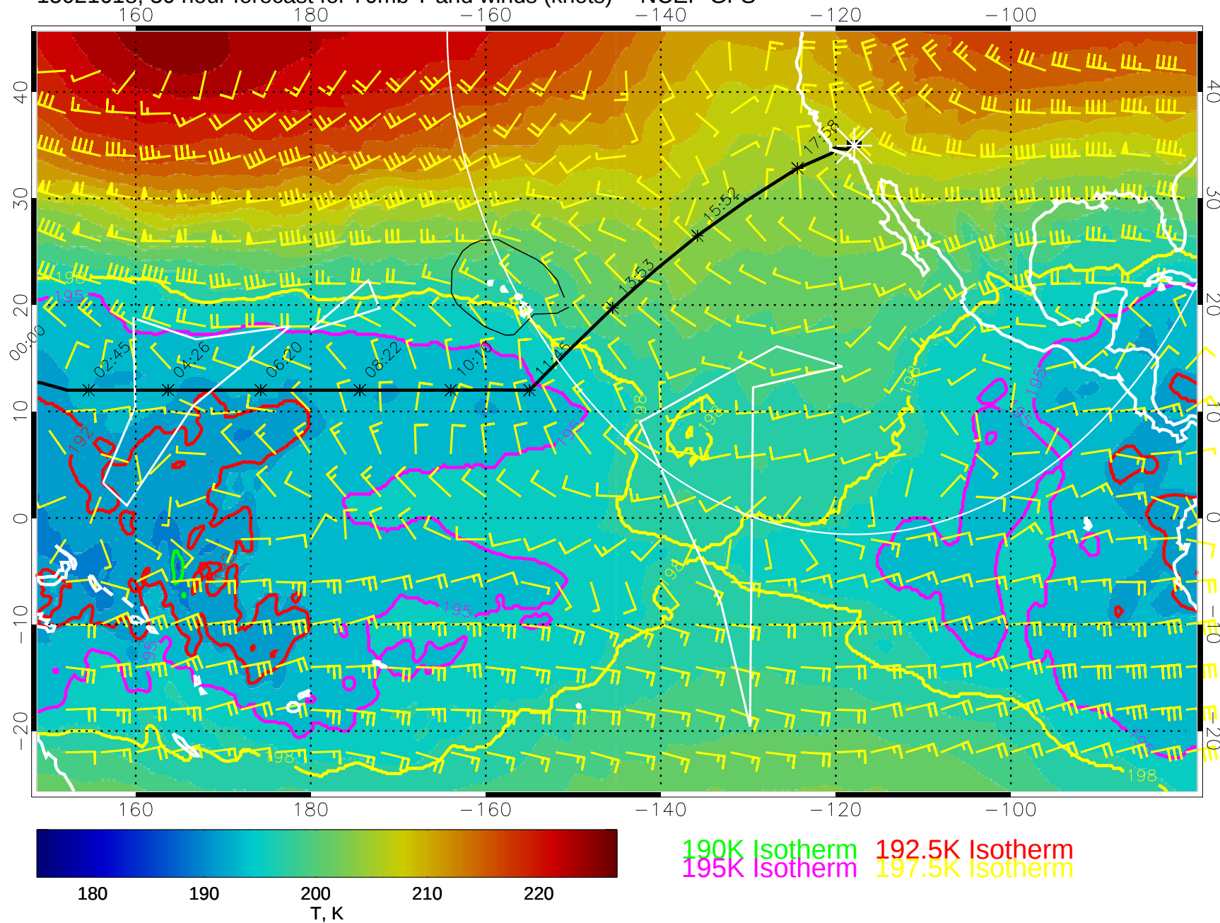
15021618, 30 hour forecast for 70mb T and winds (knots) -- NCEP GFS
