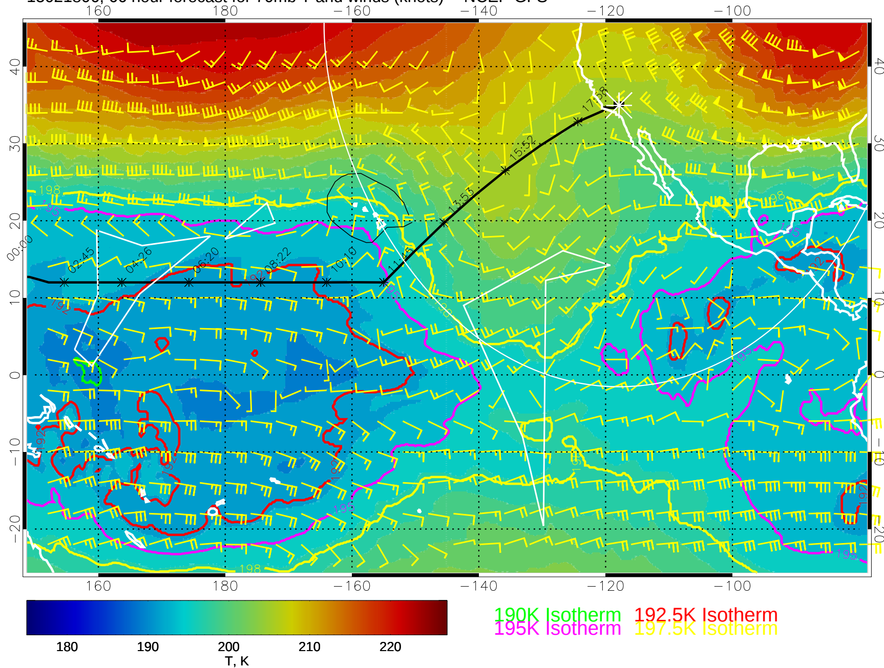
15021806, 66 hour forecast for 70mb T and winds (knots) -- NCEP GFS
