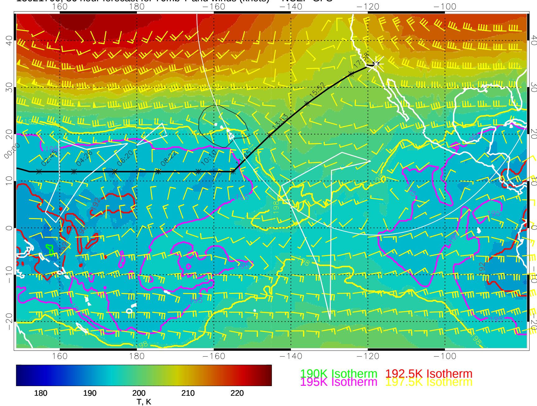
15021700, 36 hour forecast for 70mb T and winds (knots) -- NCEP GFS
