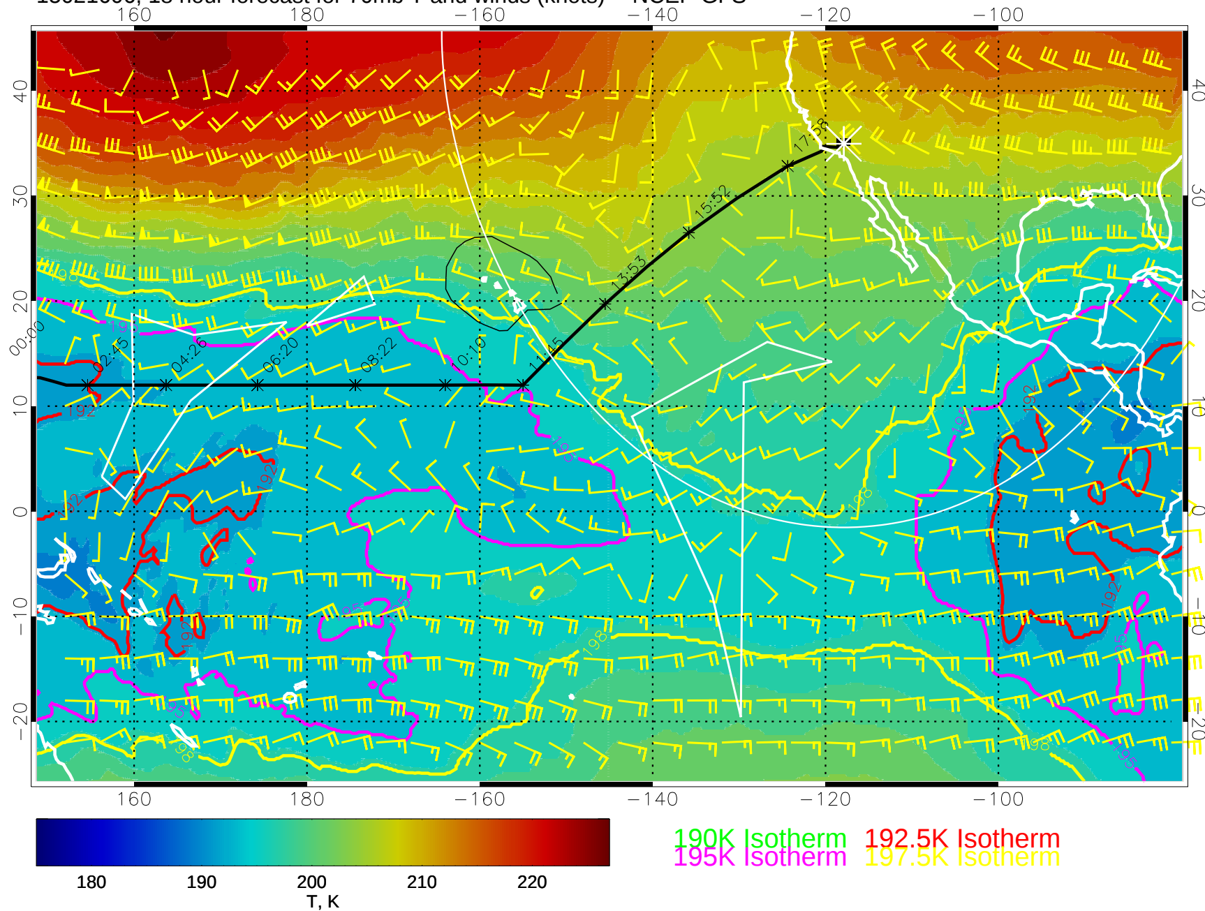
15021606, 18 hour forecast for 70mb T and winds (knots) -- NCEP GFS
