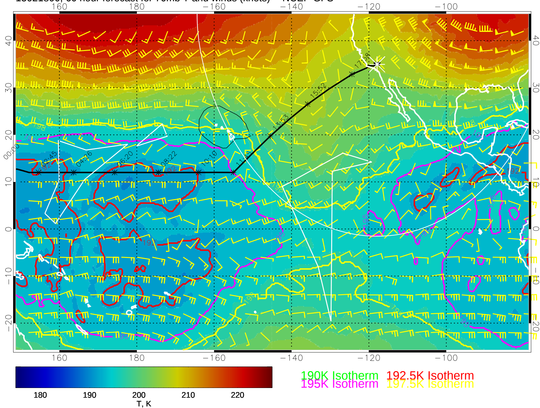
15021800, 60 hour forecast for 70mb T and winds (knots) -- NCEP GFS
