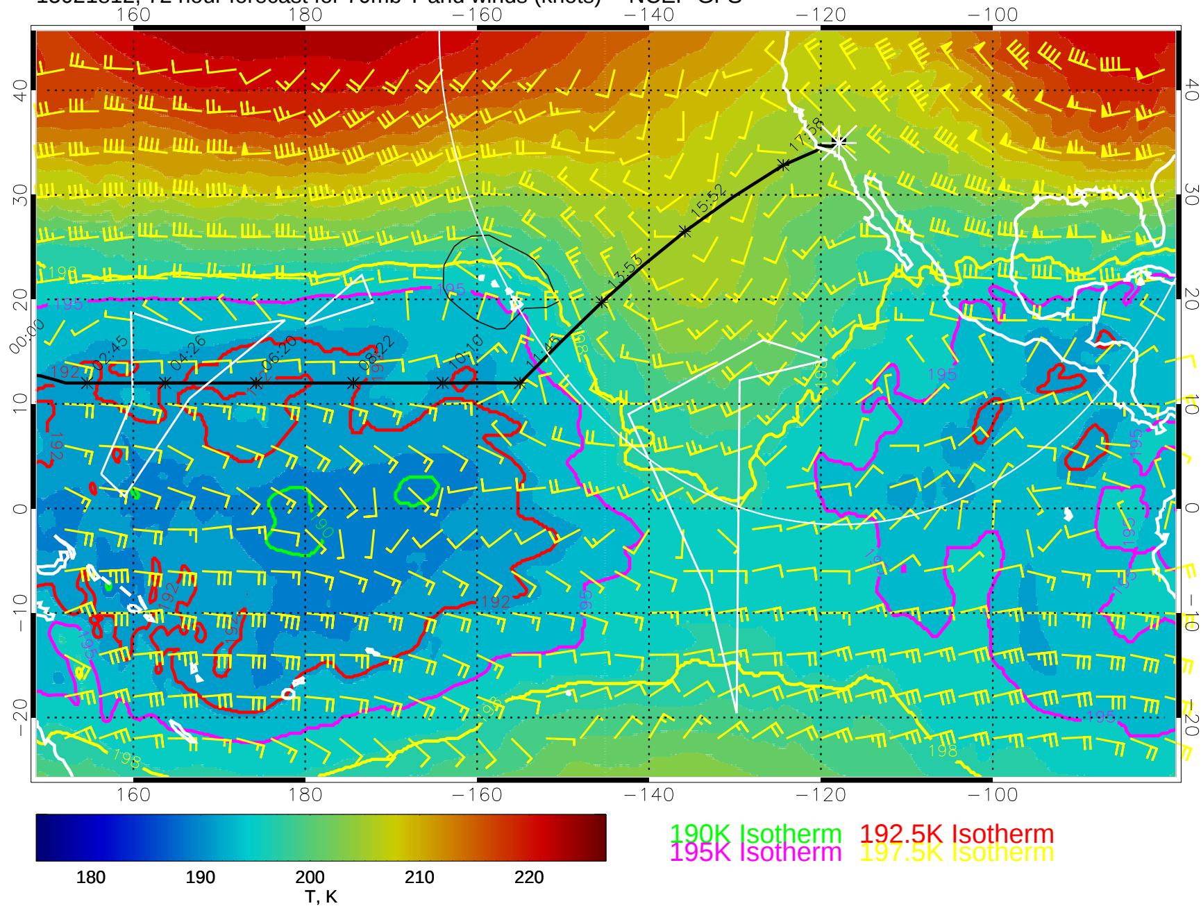
15021812, 72 hour forecast for 70mb T and winds (knots) -- NCEP GFS
