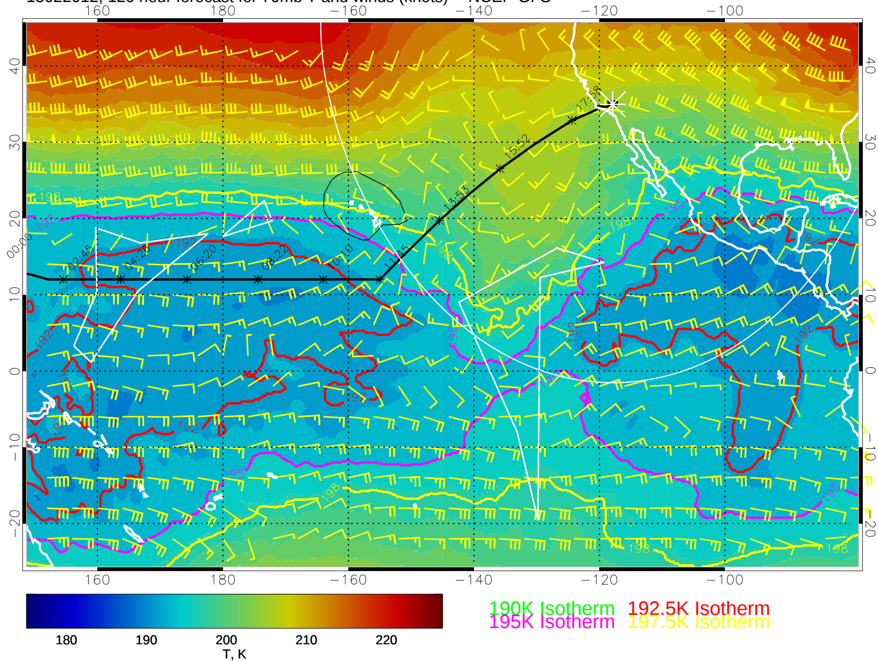
15022012, 120 hour forecast for 70mb T and winds (knots) -- NCEP GFS
