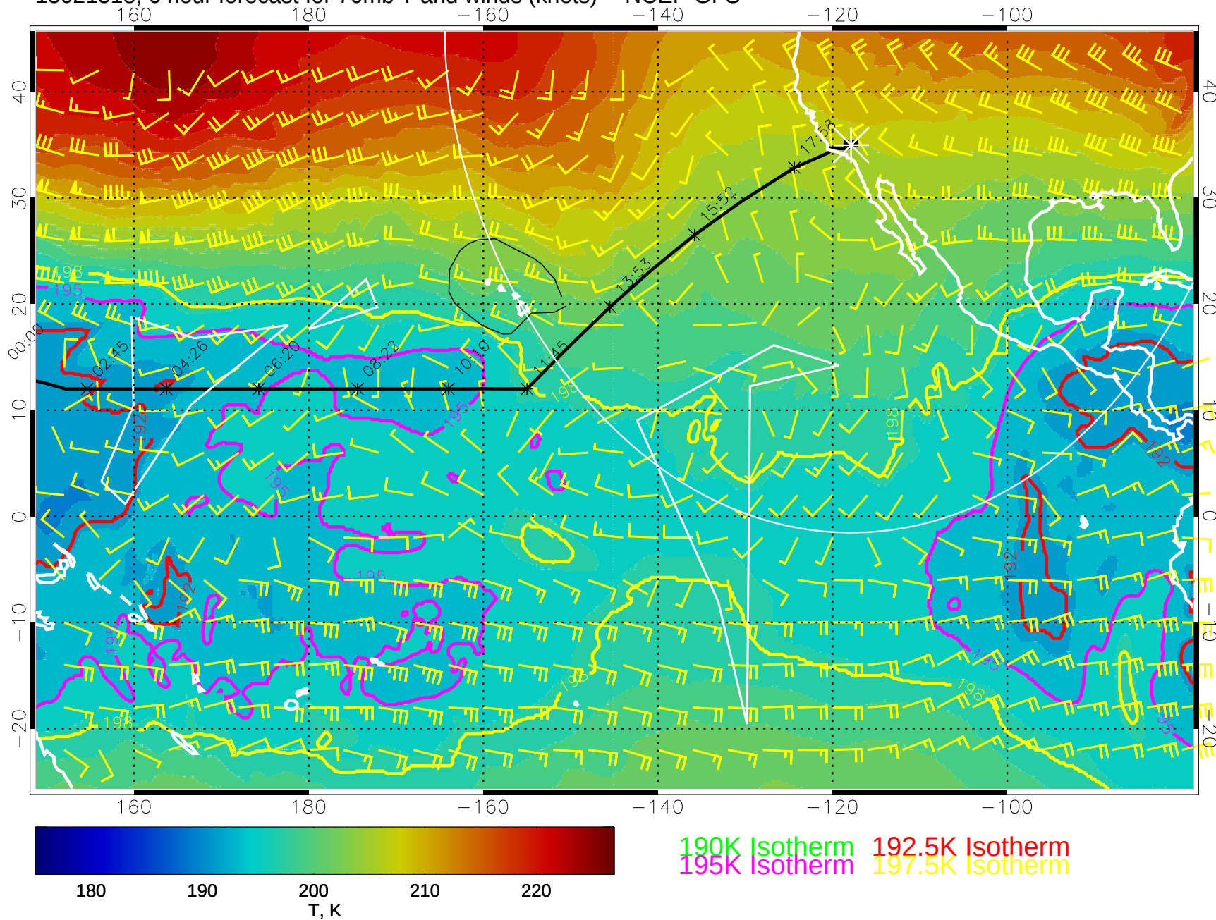
15021518, 6 hour forecast for 70mb T and winds (knots) -- NCEP GFS
