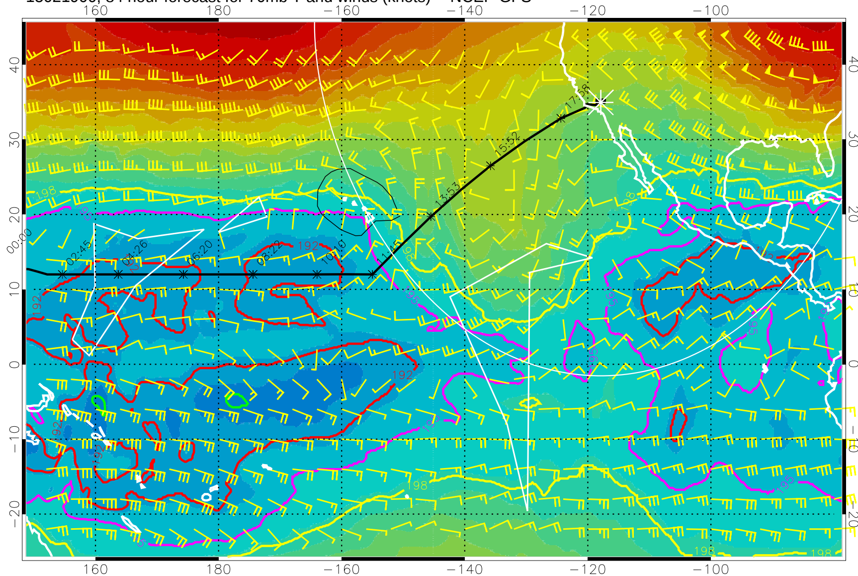
15021900, 84 hour forecast for 70mb T and winds (knots) -- NCEP GFS
