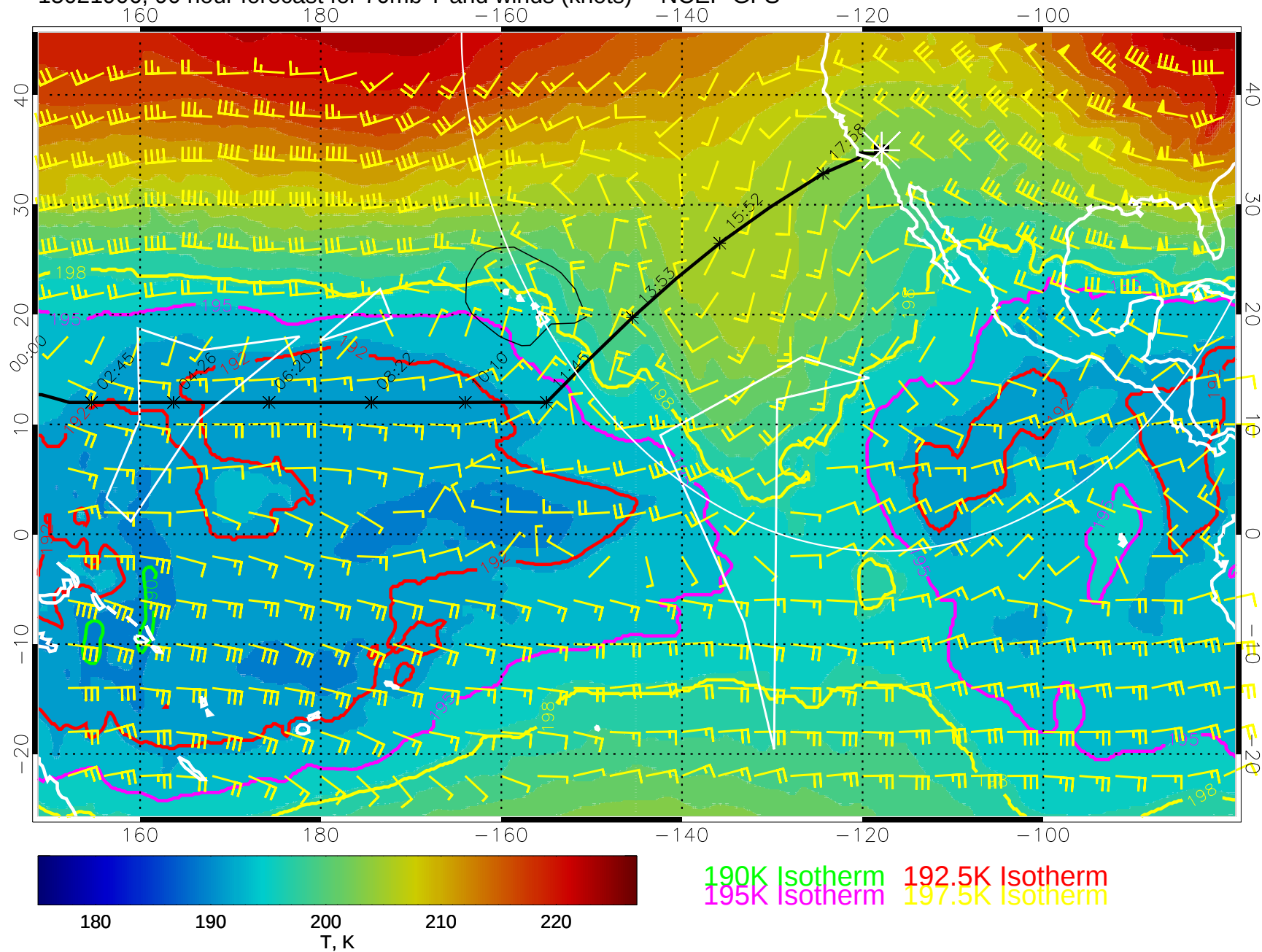
15021906, 90 hour forecast for 70mb T and winds (knots) -- NCEP GFS
