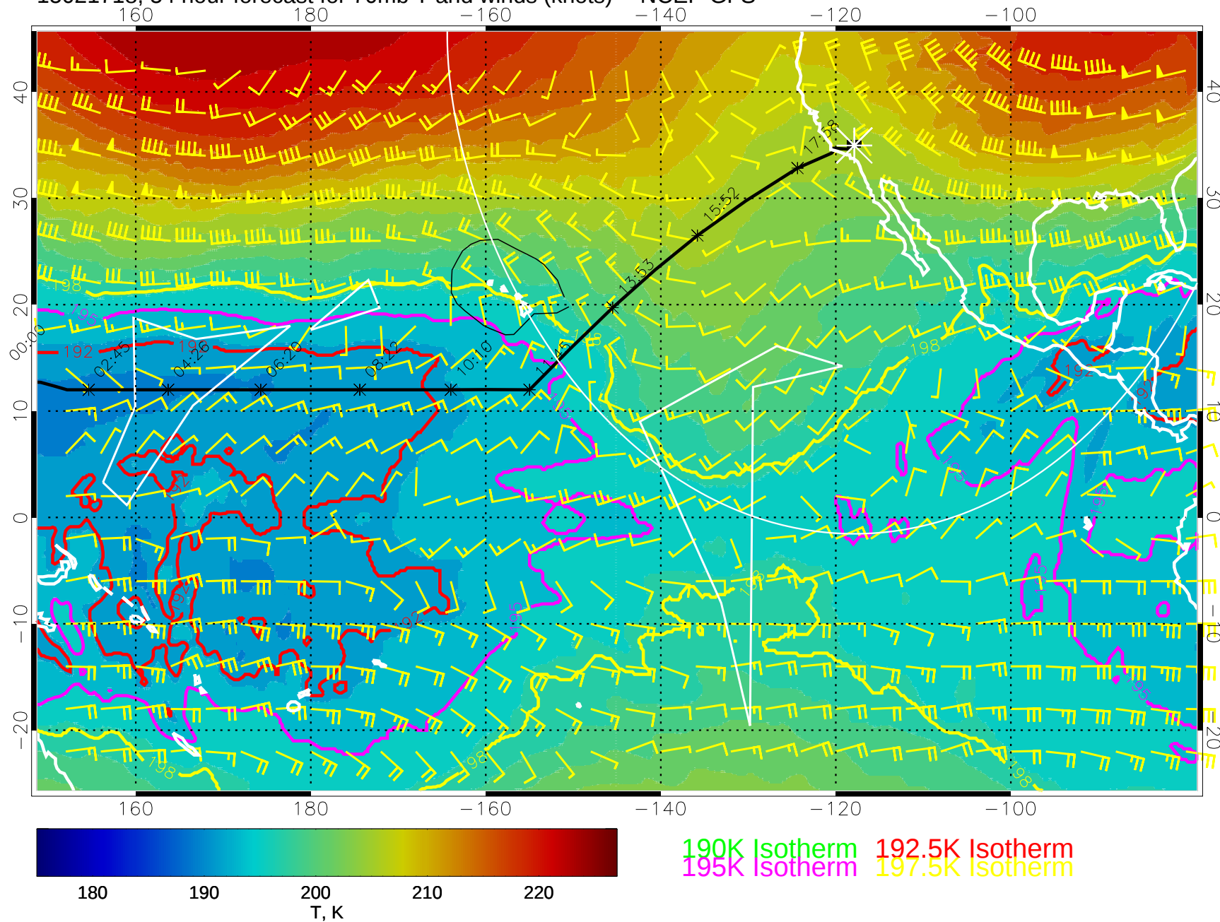
15021718, 54 hour forecast for 70mb T and winds (knots) -- NCEP GFS
