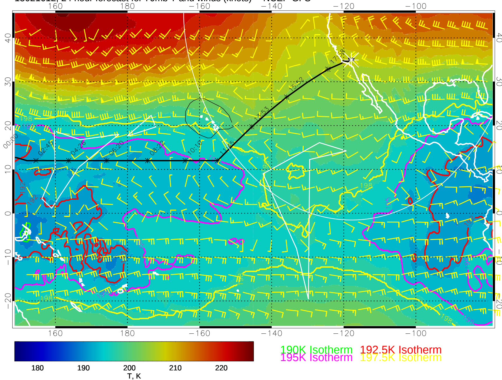
15021612, 24 hour forecast for 70mb T and winds (knots) -- NCEP GFS
