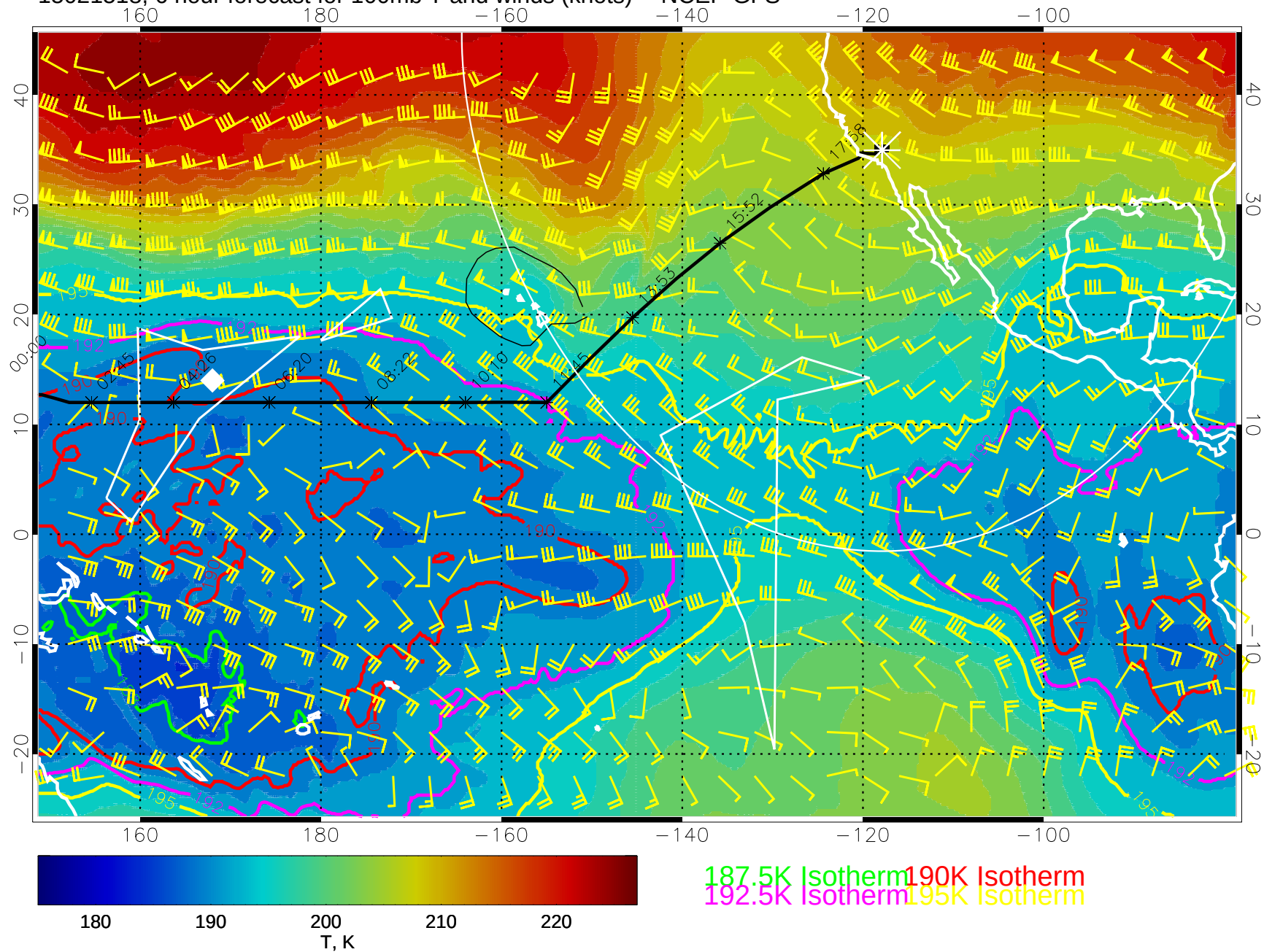
15021518, 6 hour forecast for 100mb T and winds (knots) -- NCEP GFS
