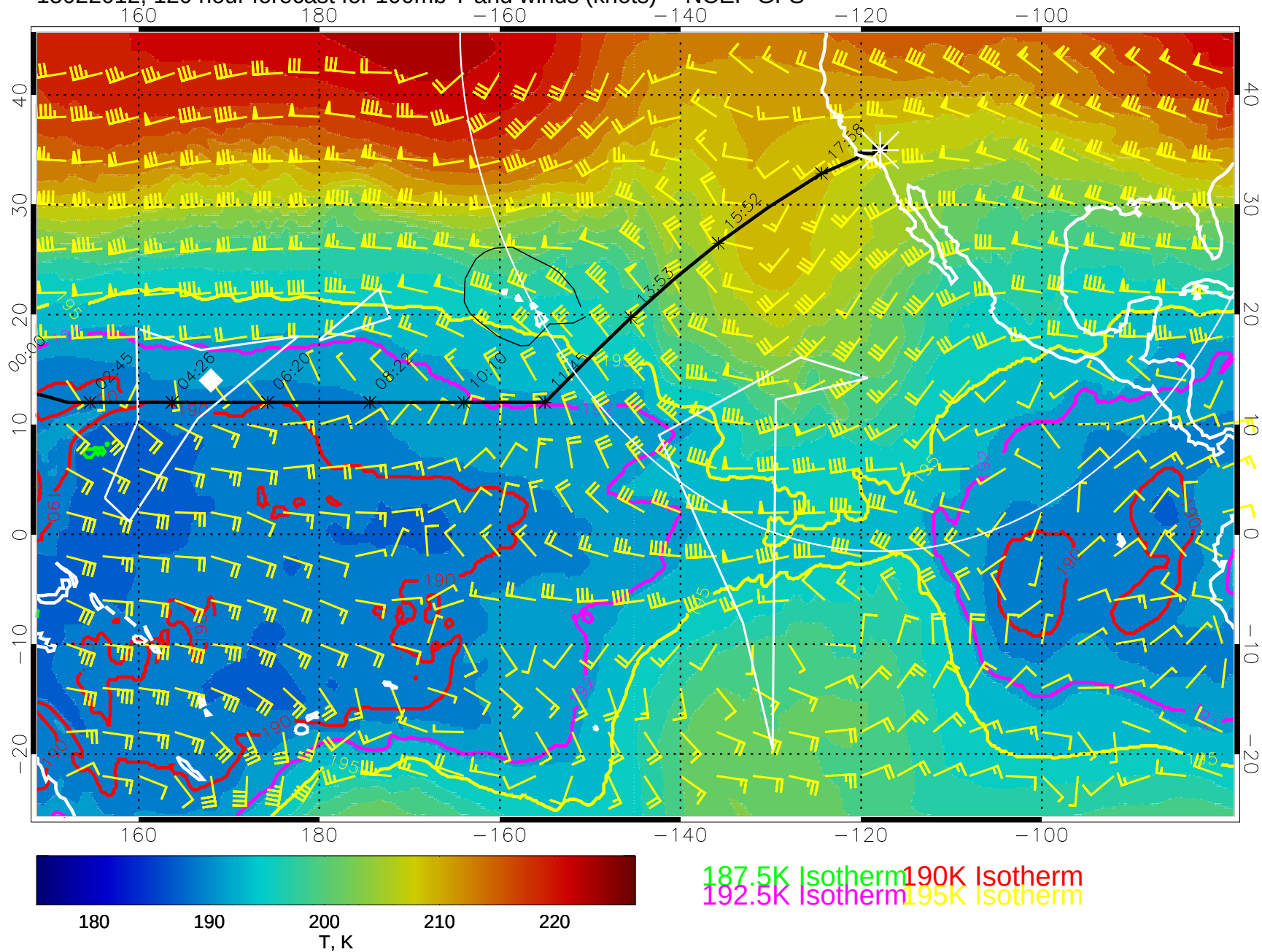
15022012, 120 hour forecast for 100mb T and winds (knots) -- NCEP GFS
