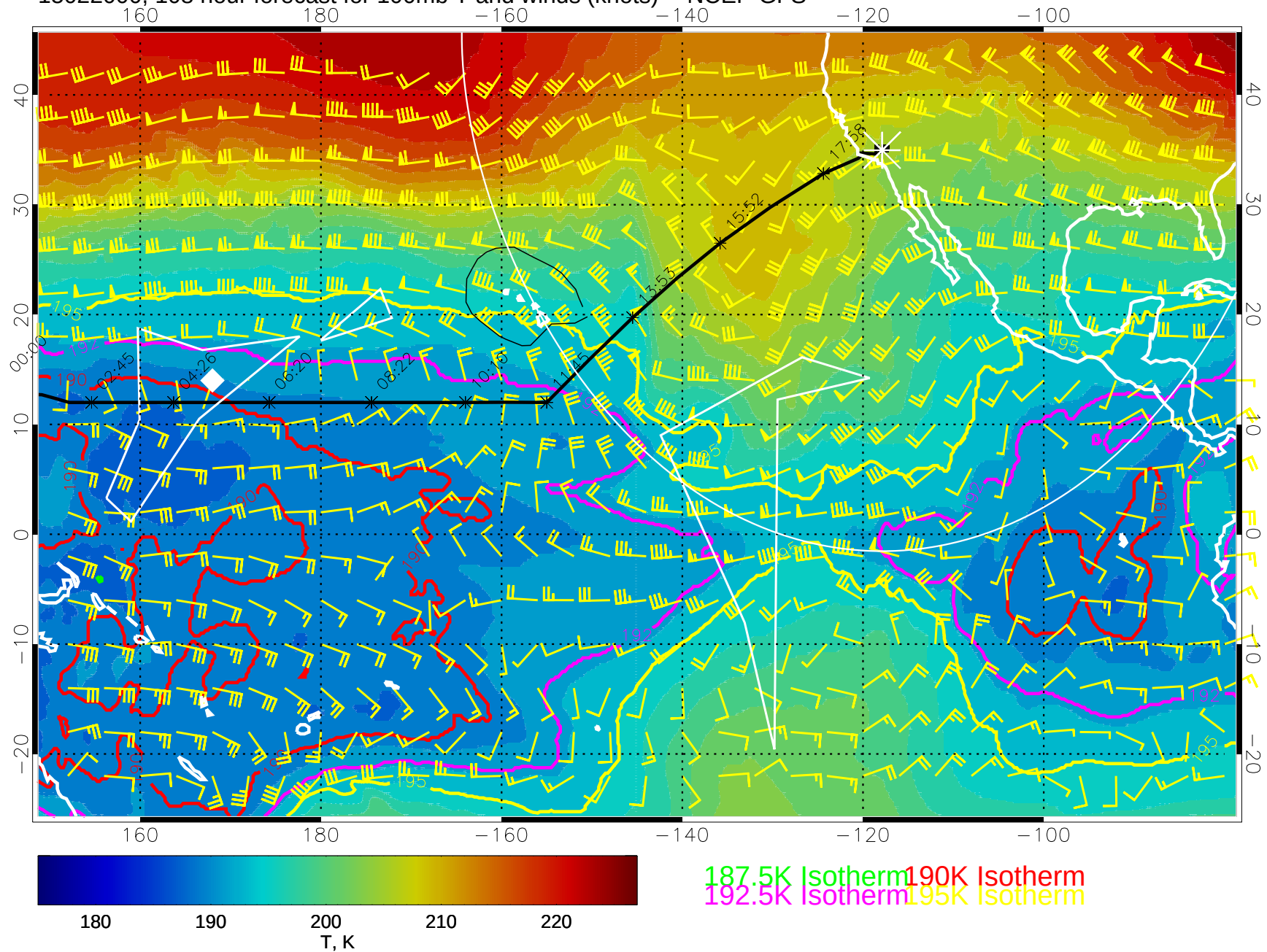
15022000, 108 hour forecast for 100mb T and winds (knots) -- NCEP GFS
