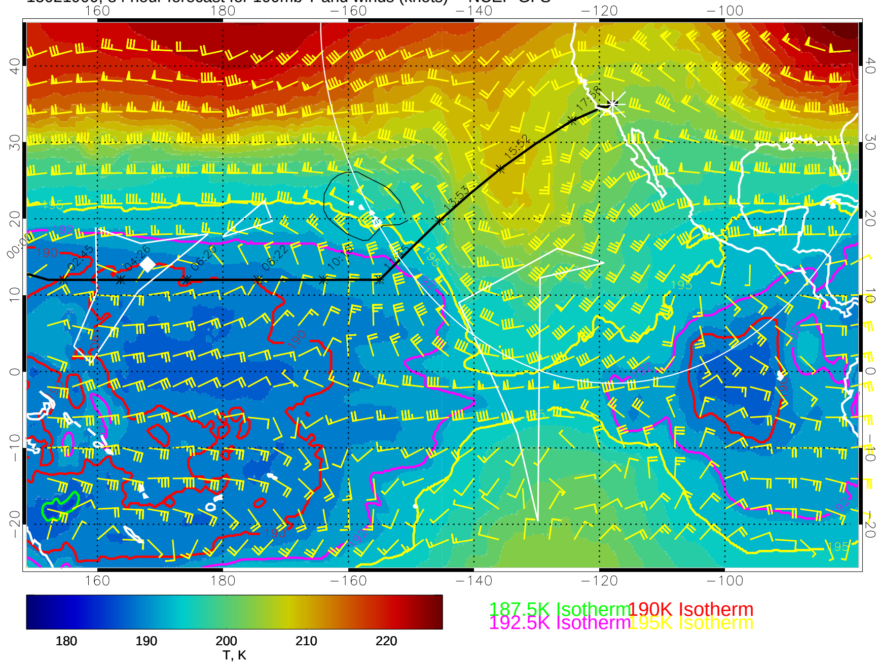
15021900, 84 hour forecast for 100mb T and winds (knots) -- NCEP GFS
