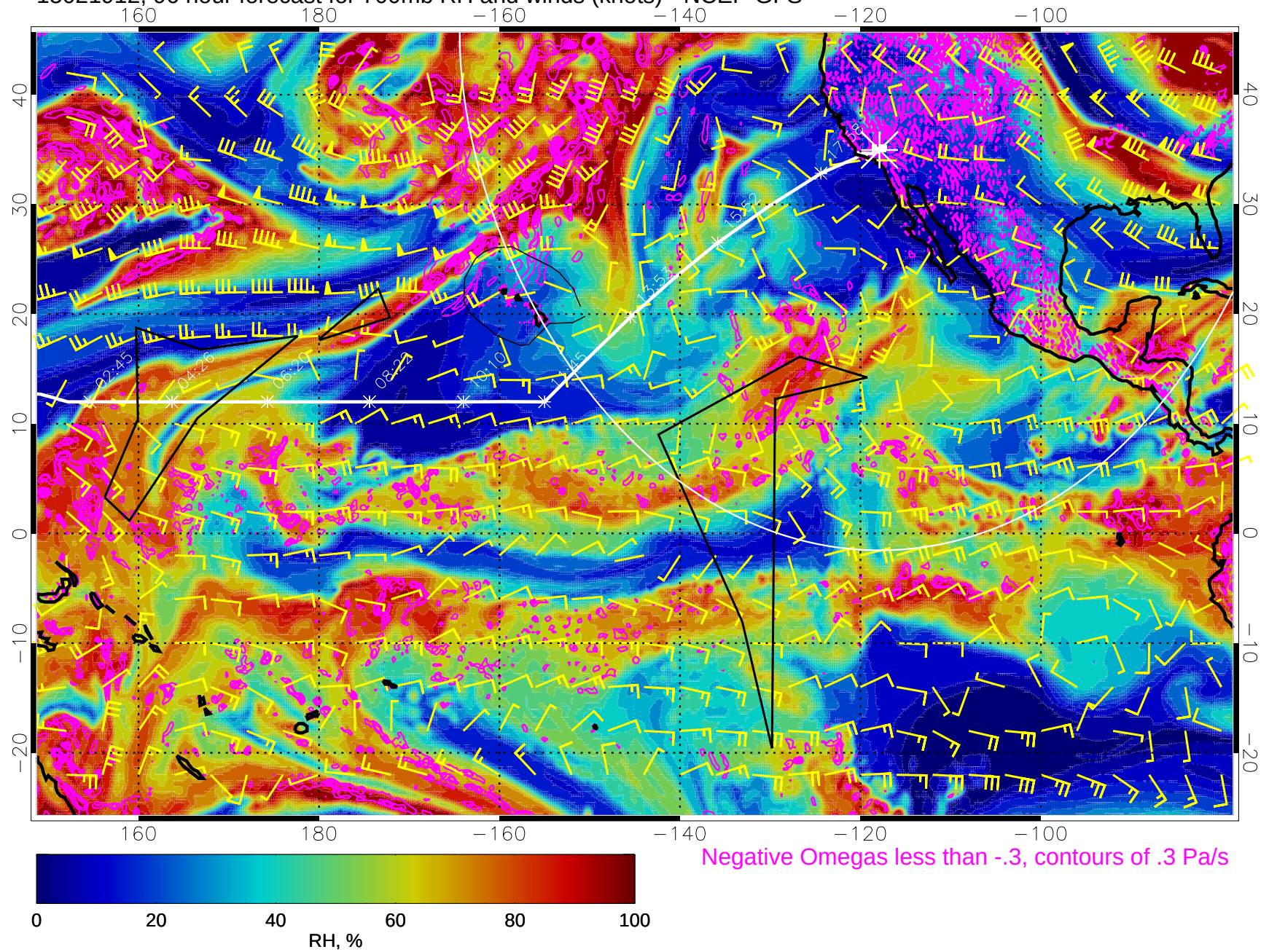
15021912, 96 hour forecast for 700mb RH and winds (knots) - NCEP GFS
