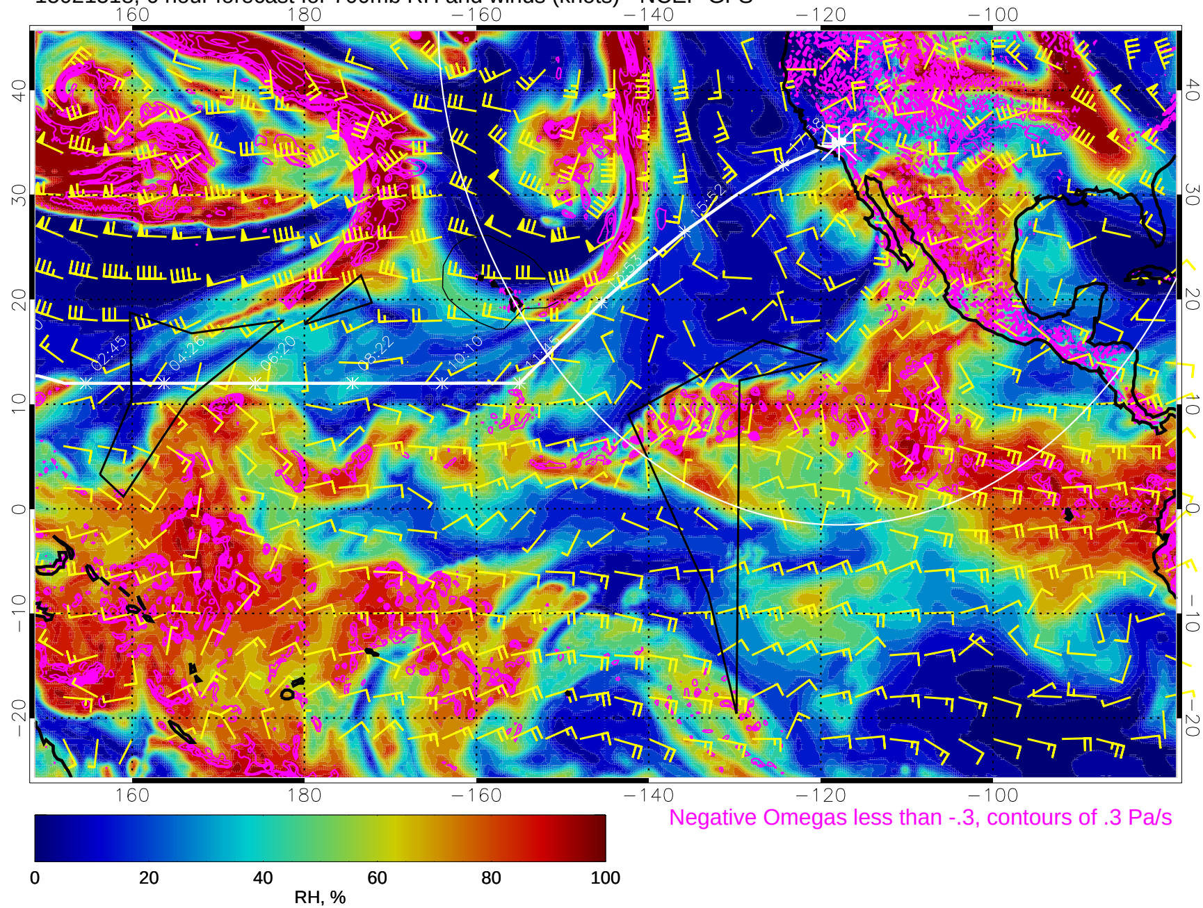
15021518, 6 hour forecast for 700mb RH and winds (knots) - NCEP GFS
