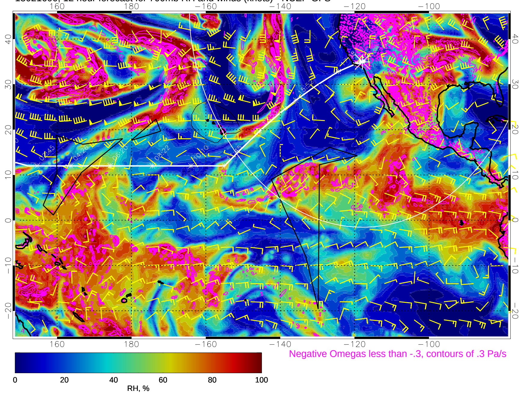
15021600, 12 hour forecast for 700mb RH and winds (knots) - NCEP GFS
