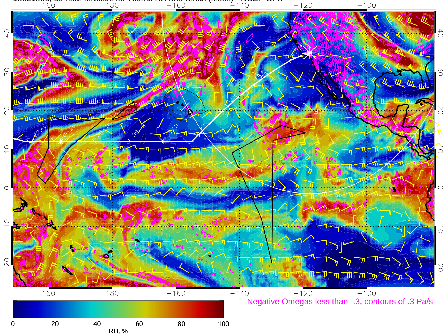
15021906, 90 hour forecast for 700mb RH and winds (knots) - NCEP GFS
