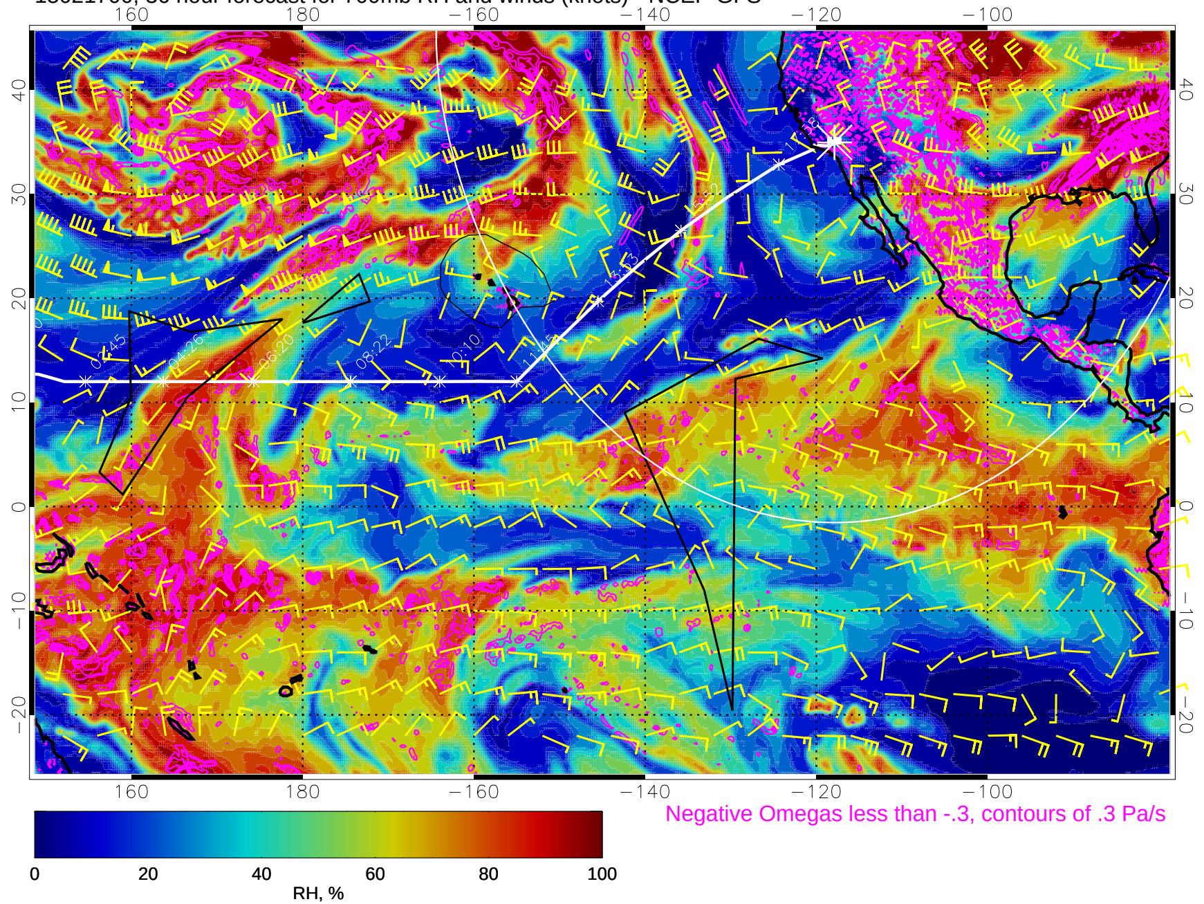
15021700, 36 hour forecast for 700mb RH and winds (knots) - NCEP GFS
