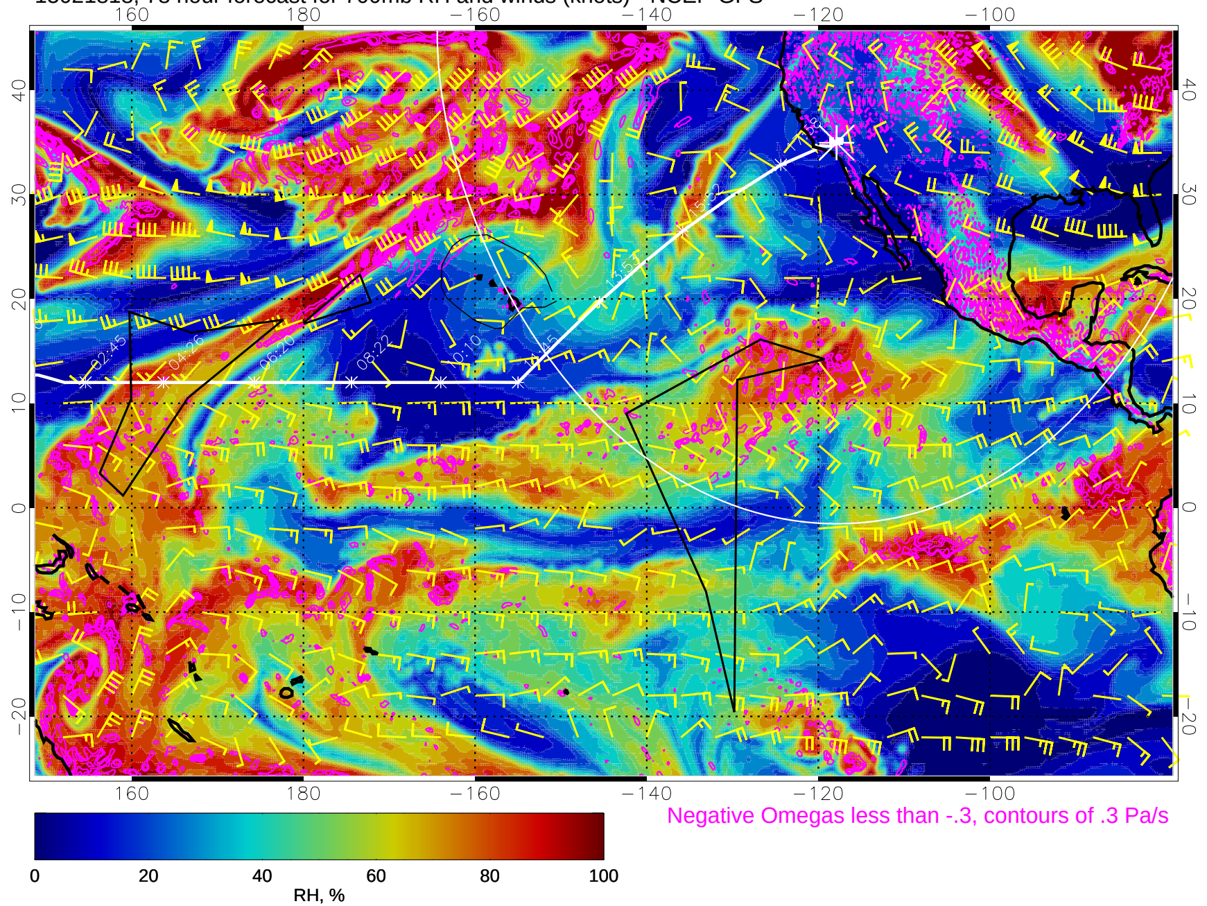
15021818, 78 hour forecast for 700mb RH and winds (knots) - NCEP GFS
