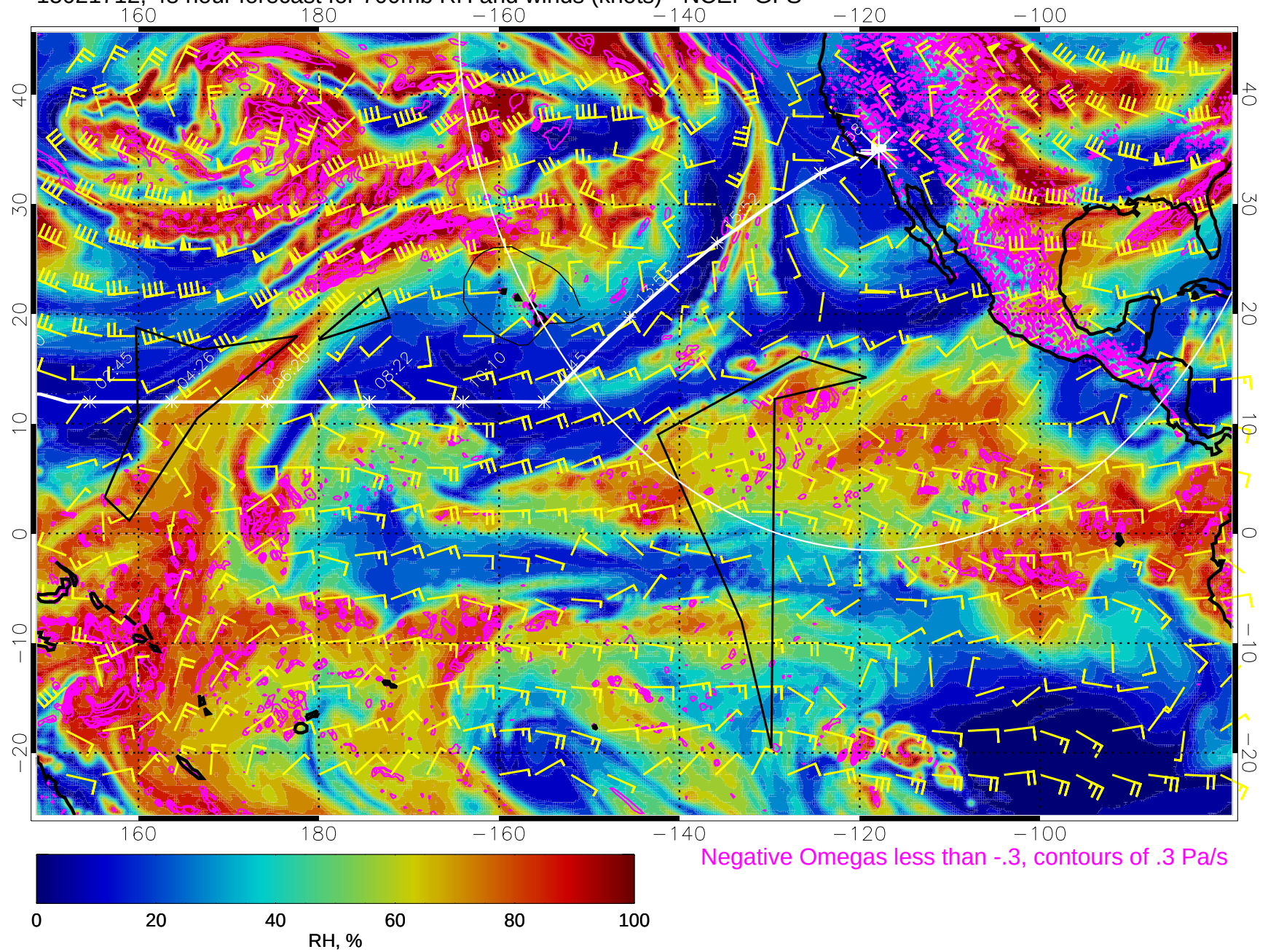
15021712, 48 hour forecast for 700mb RH and winds (knots) - NCEP GFS
