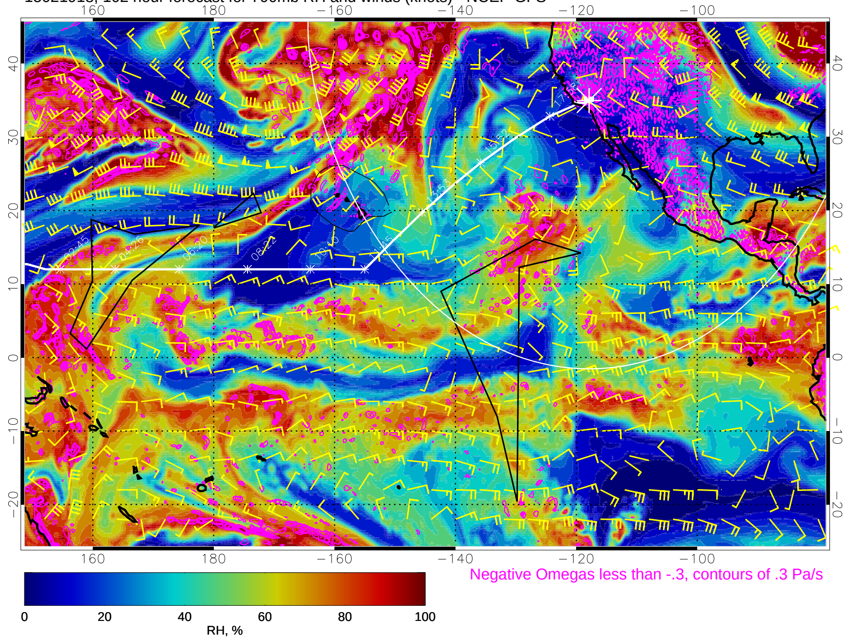
15021918, 102 hour forecast for 700mb RH and winds (knots) - NCEP GFS
