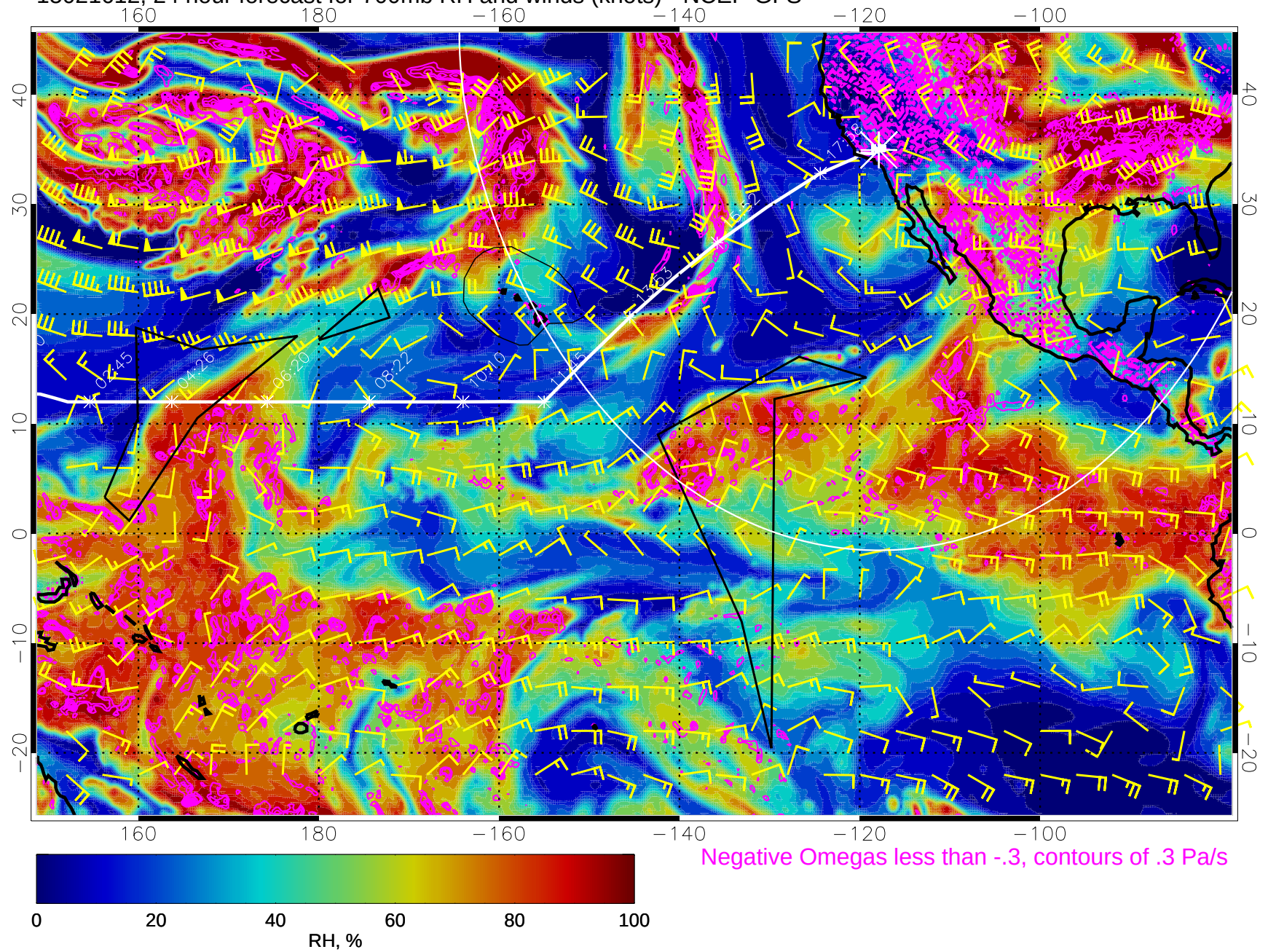
15021612, 24 hour forecast for 700mb RH and winds (knots) - NCEP GFS
