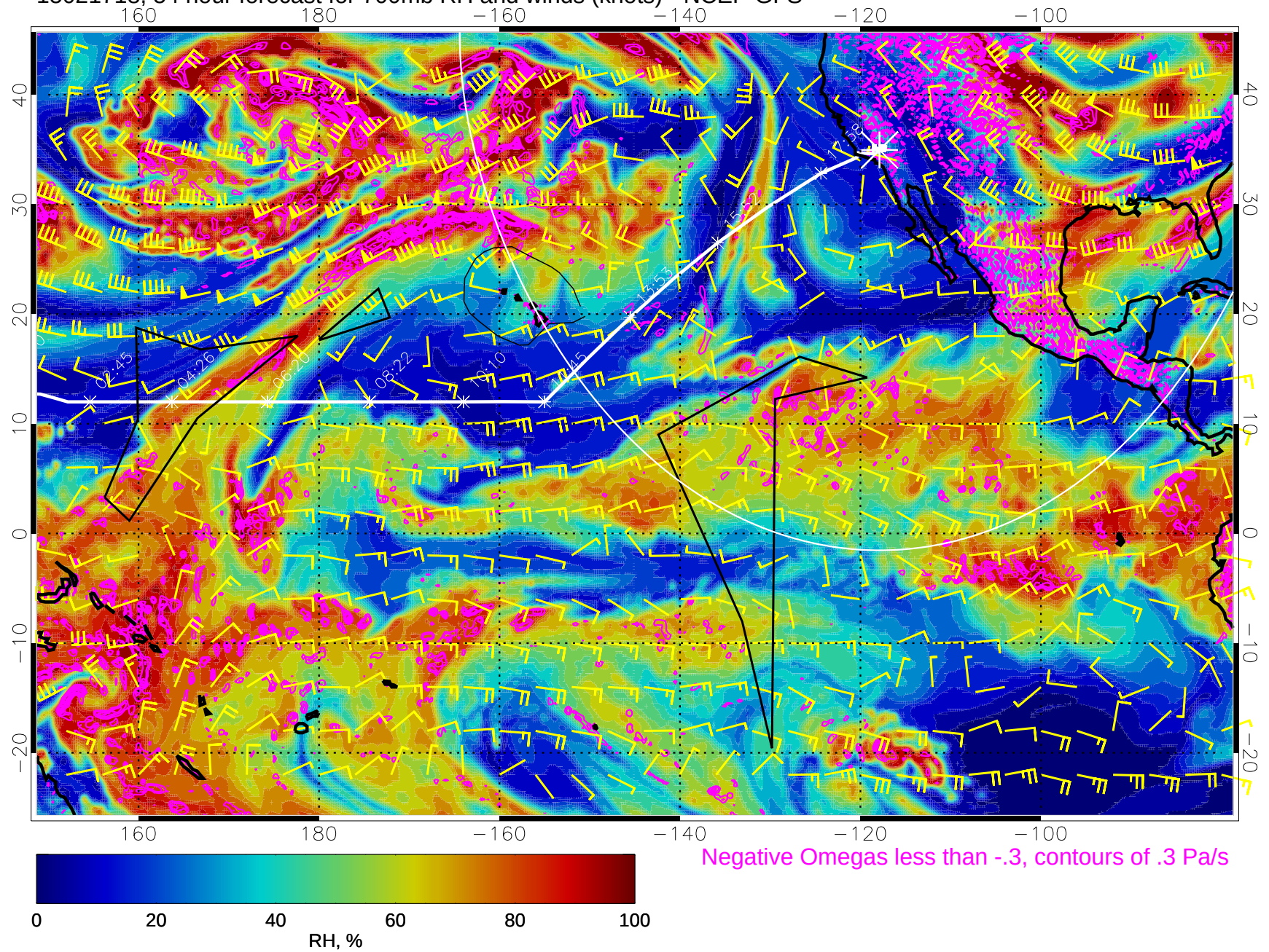
15021718, 54 hour forecast for 700mb RH and winds (knots) - NCEP GFS
