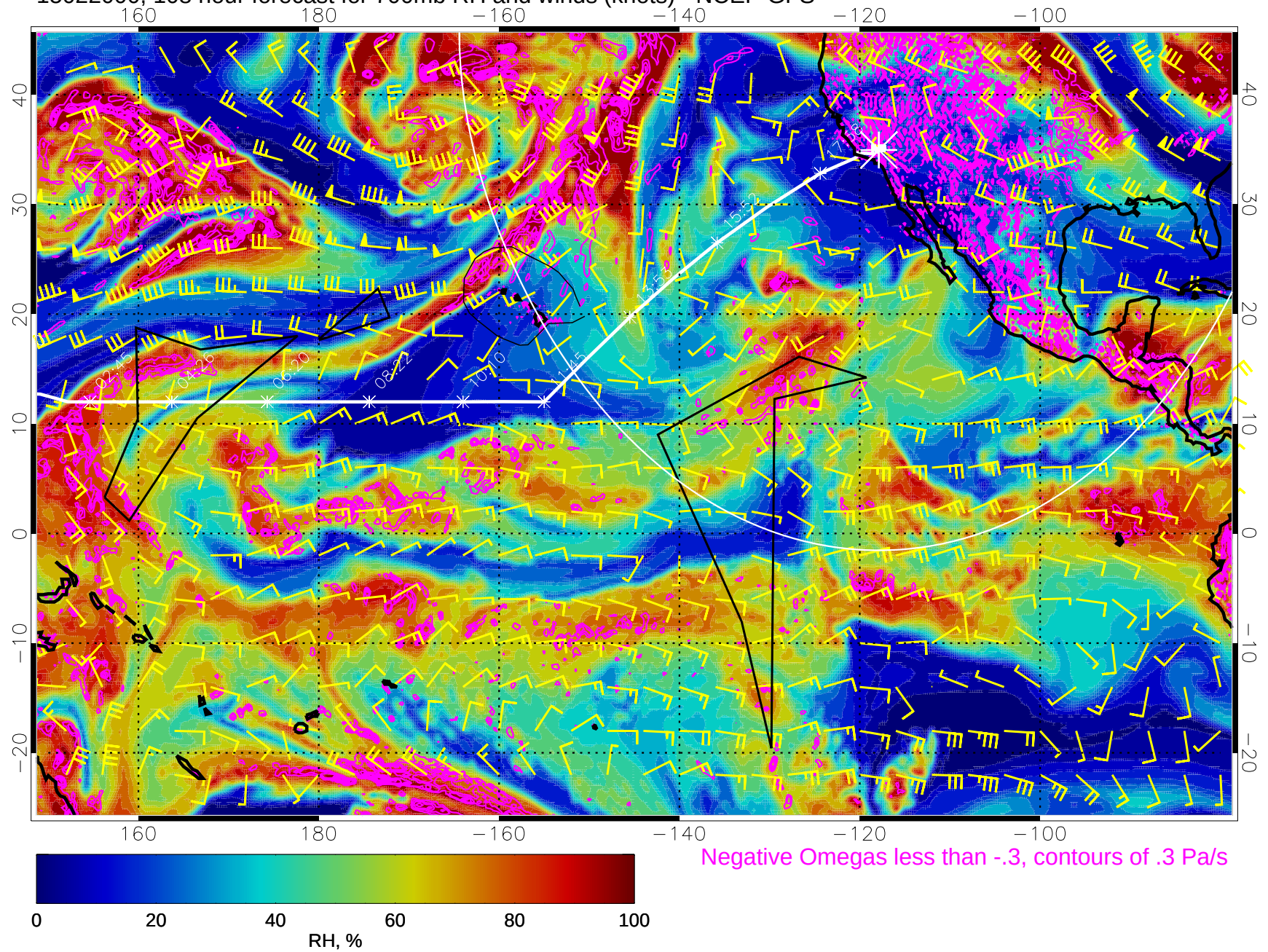
15022000, 108 hour forecast for 700mb RH and winds (knots) - NCEP GFS
