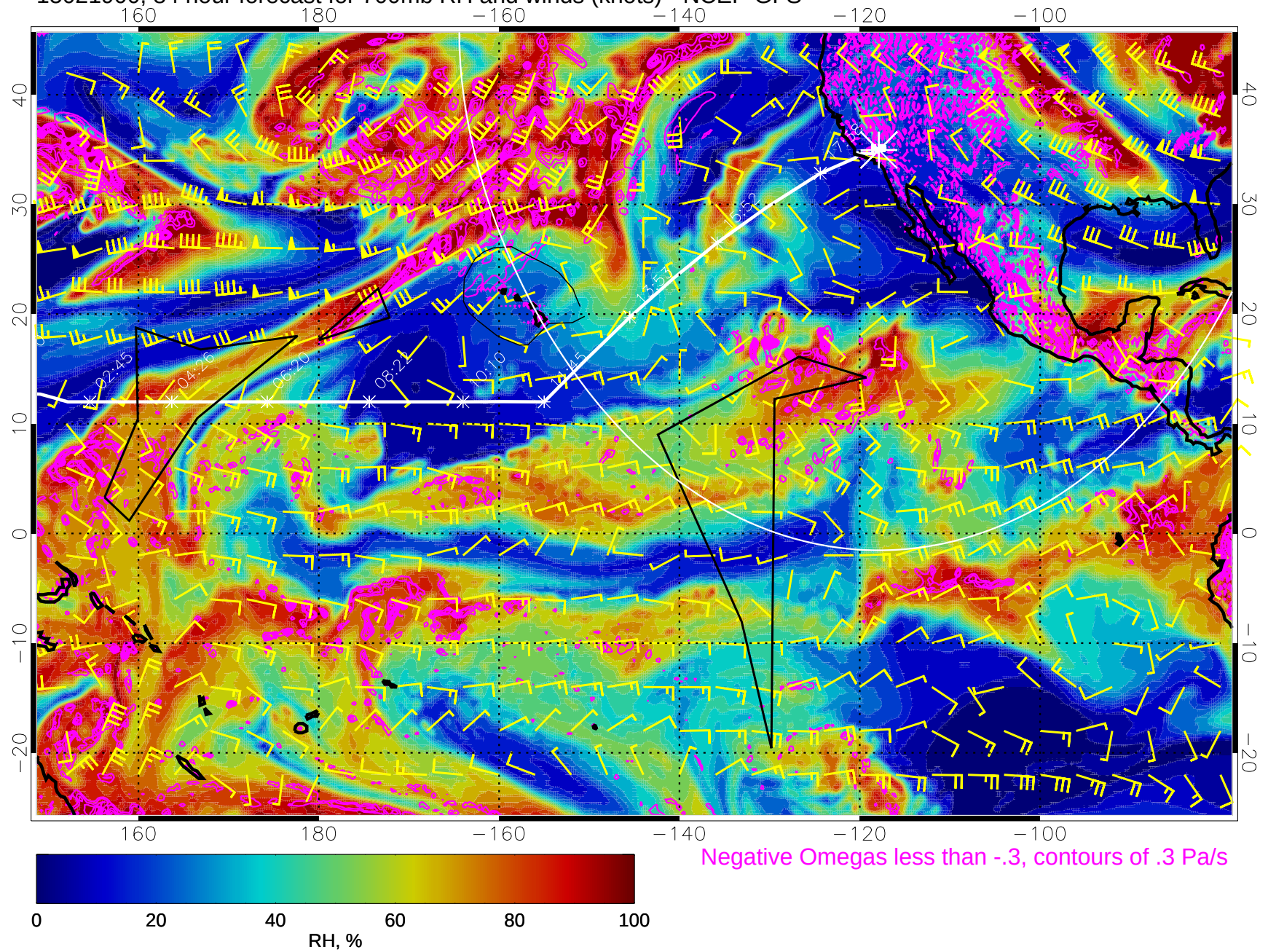
15021900, 84 hour forecast for 700mb RH and winds (knots) - NCEP GFS
