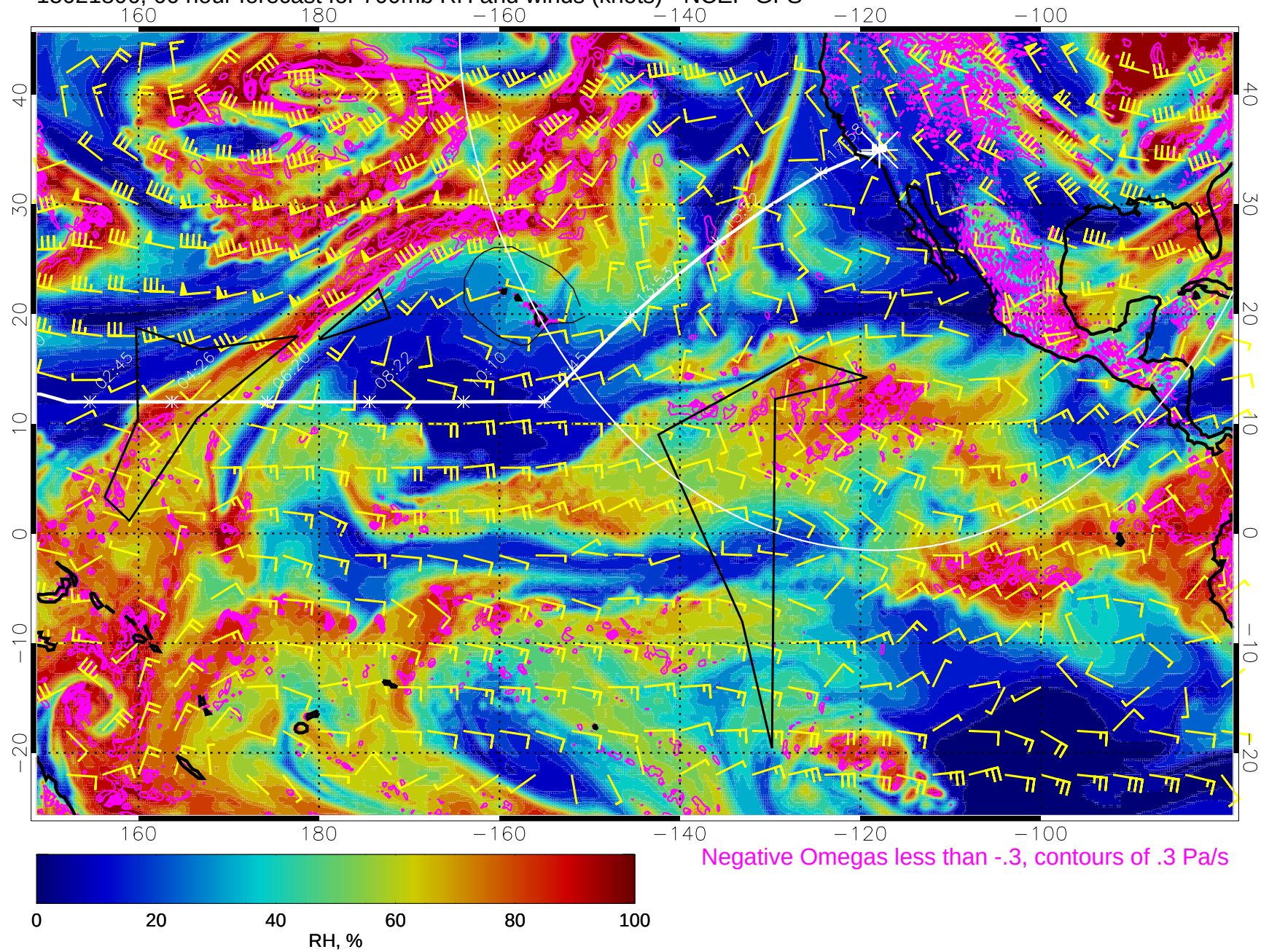
15021806, 66 hour forecast for 700mb RH and winds (knots) - NCEP GFS
