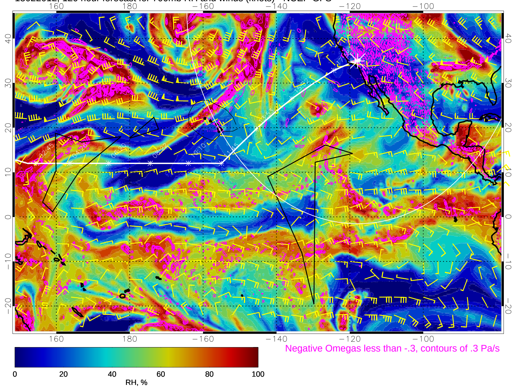
15022012, 120 hour forecast for 700mb RH and winds (knots) - NCEP GFS
