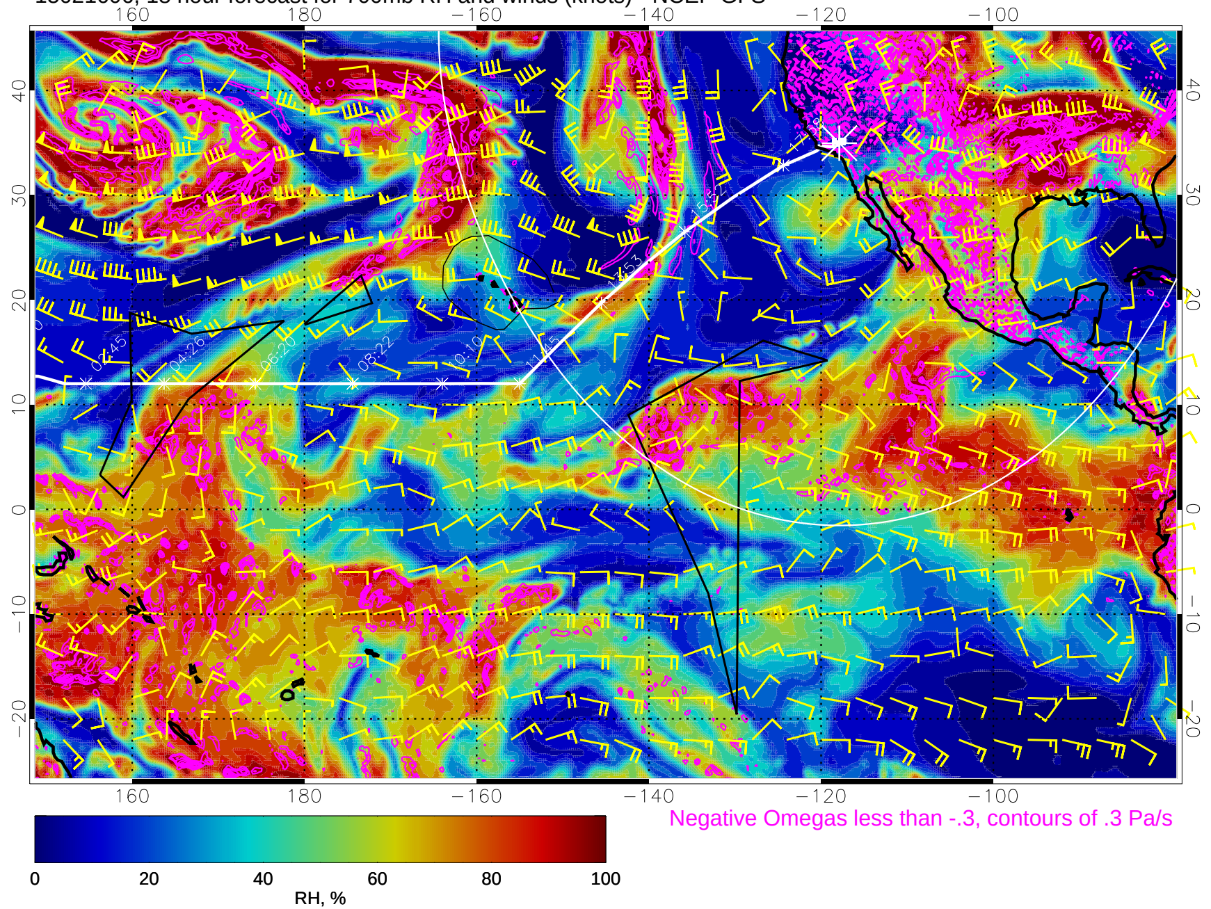
15021606, 18 hour forecast for 700mb RH and winds (knots) - NCEP GFS
