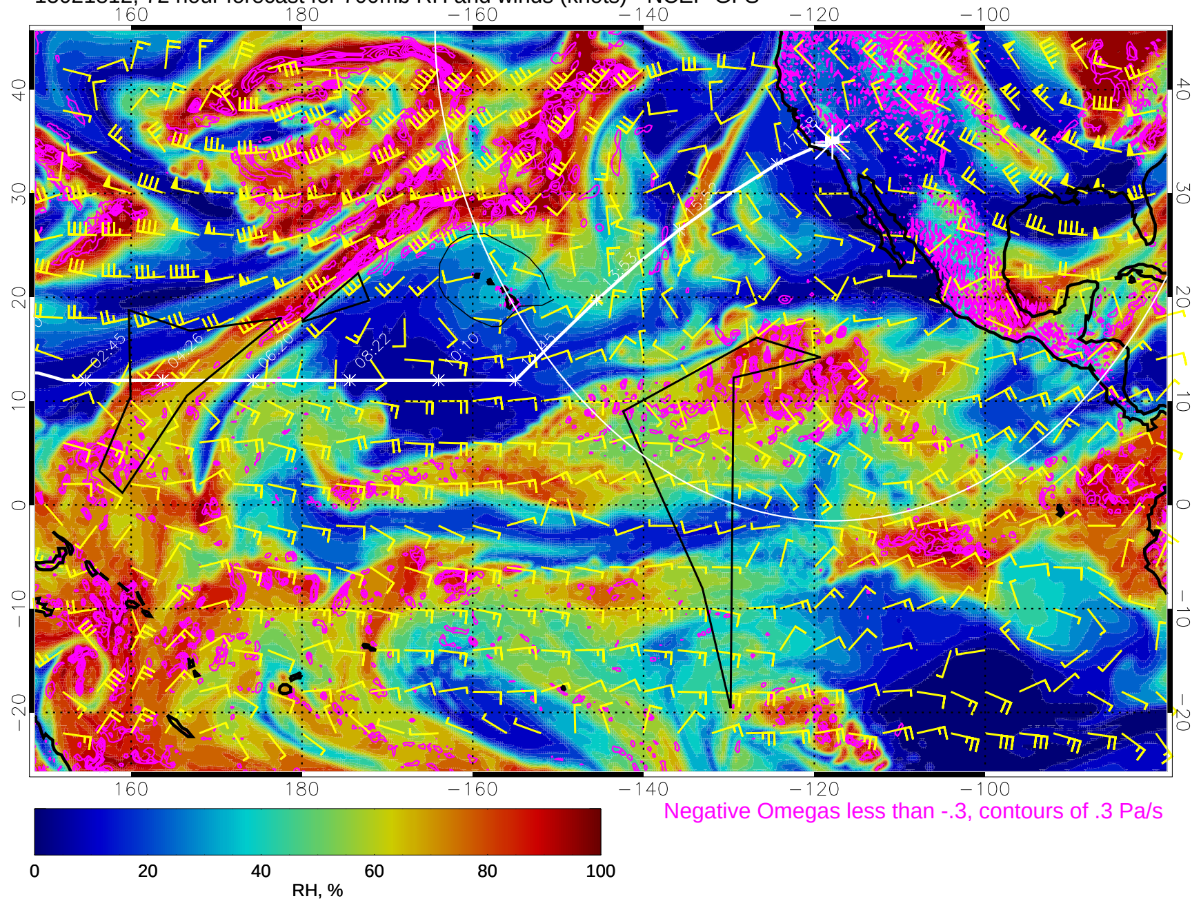
15021812, 72 hour forecast for 700mb RH and winds (knots) - NCEP GFS
