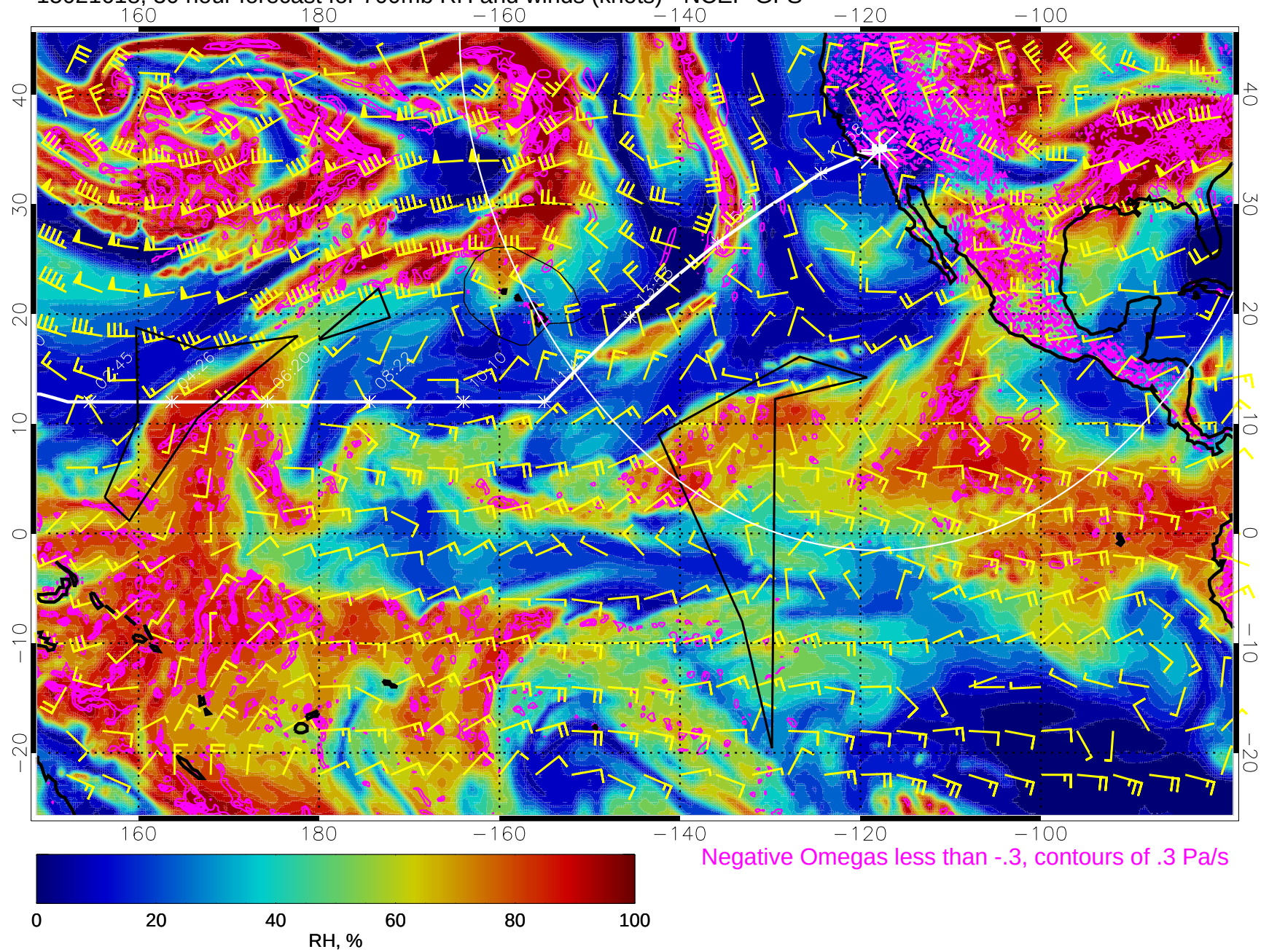
15021618, 30 hour forecast for 700mb RH and winds (knots) - NCEP GFS
