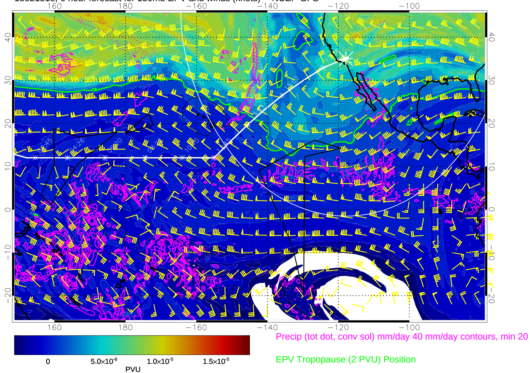
15021518, 6 hour forecast for 150mb EPV and winds (knots) -- NCEP GFS
