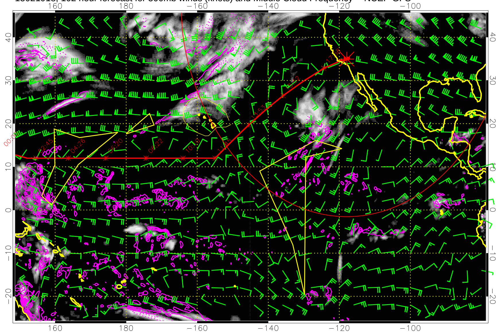
15021918, 102 hour forecast for 500mb winds (knots) and Middle Cloud Frequency -- NCEP GFS
