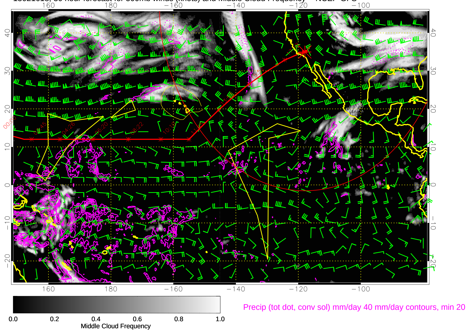
15021618, 30 hour forecast for 500mb winds (knots) and Middle Cloud Frequency -- NCEP GFS
