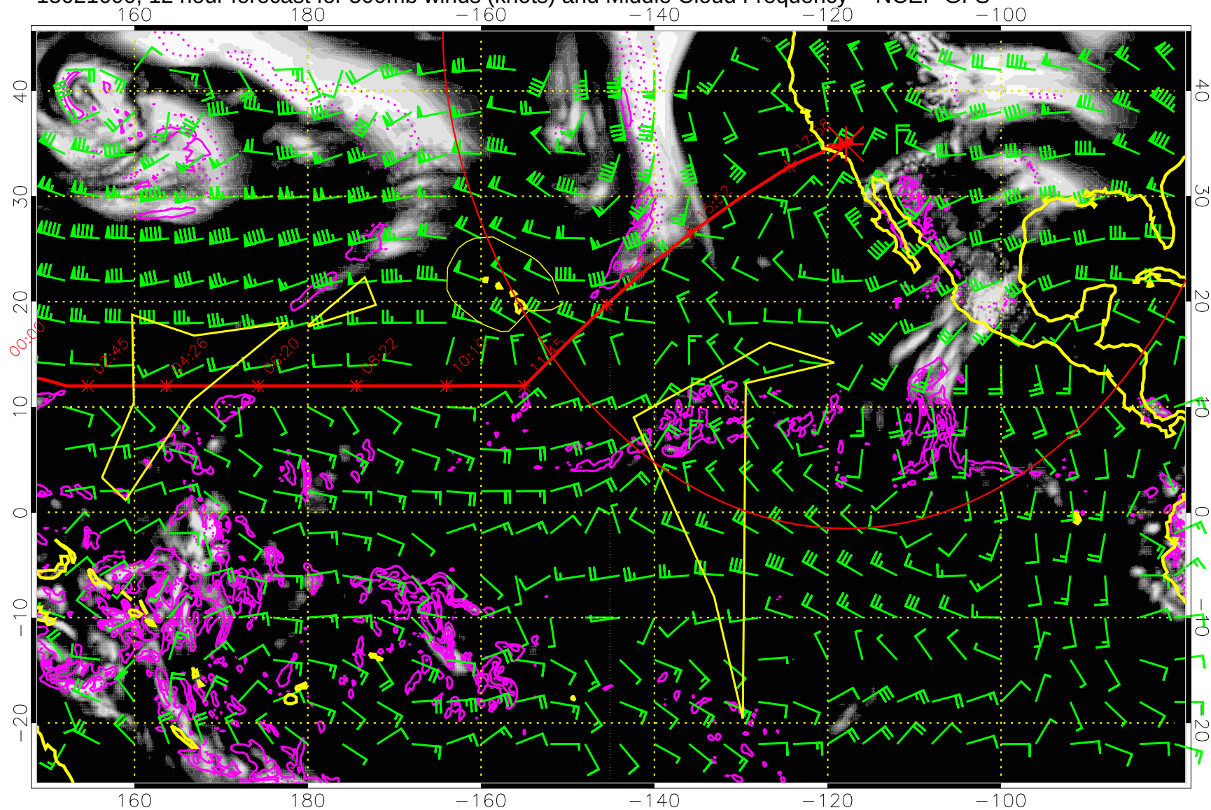
15021600, 12 hour forecast for 500mb winds (knots) and Middle Cloud Frequency -- NCEP GFS
