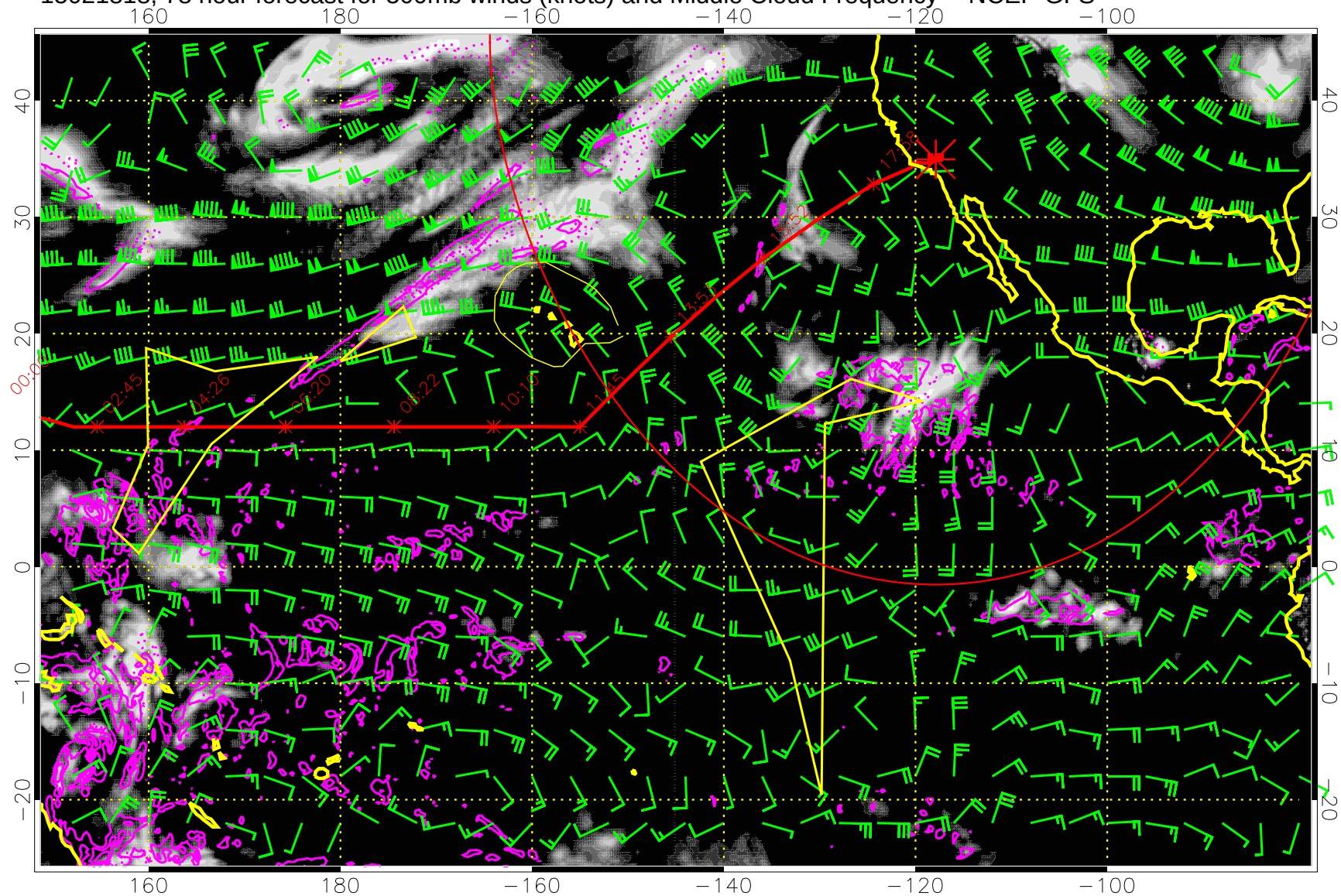
15021818, 78 hour forecast for 500mb winds (knots) and Middle Cloud Frequency -- NCEP GFS
