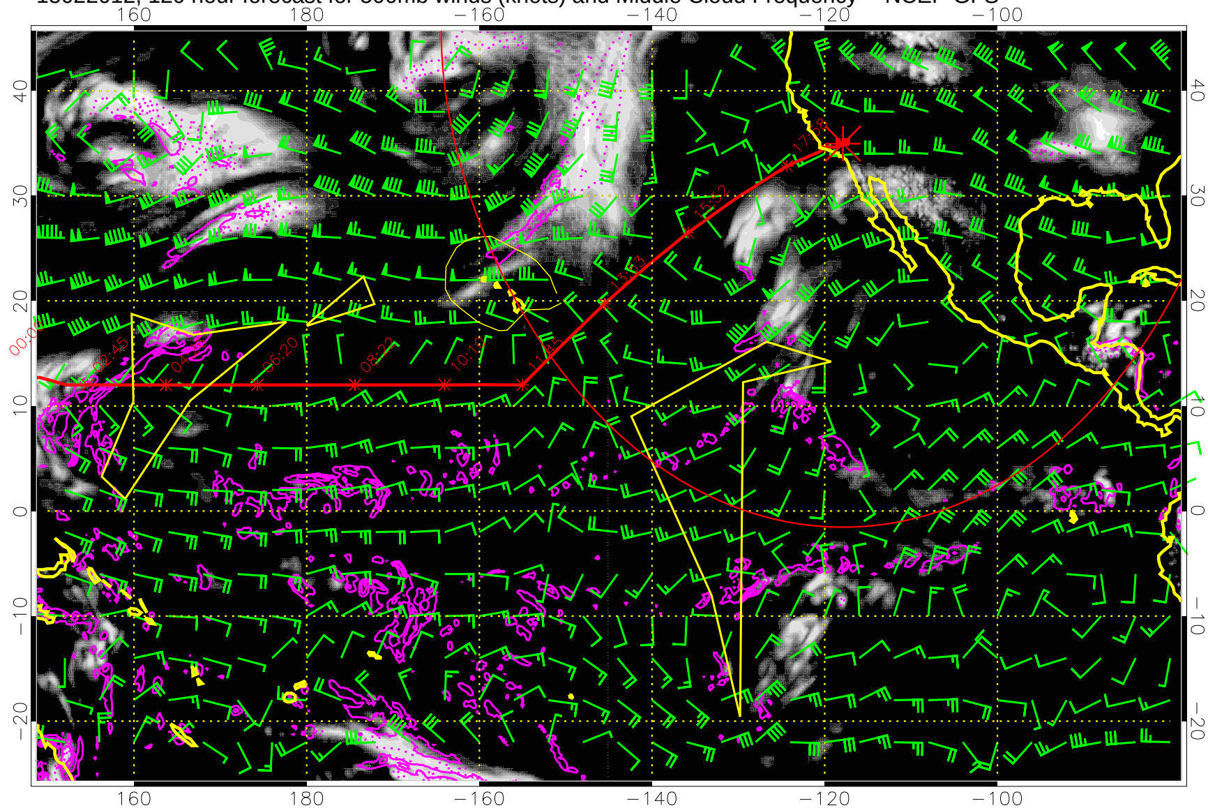
15022012, 120 hour forecast for 500mb winds (knots) and Middle Cloud Frequency -- NCEP GFS
