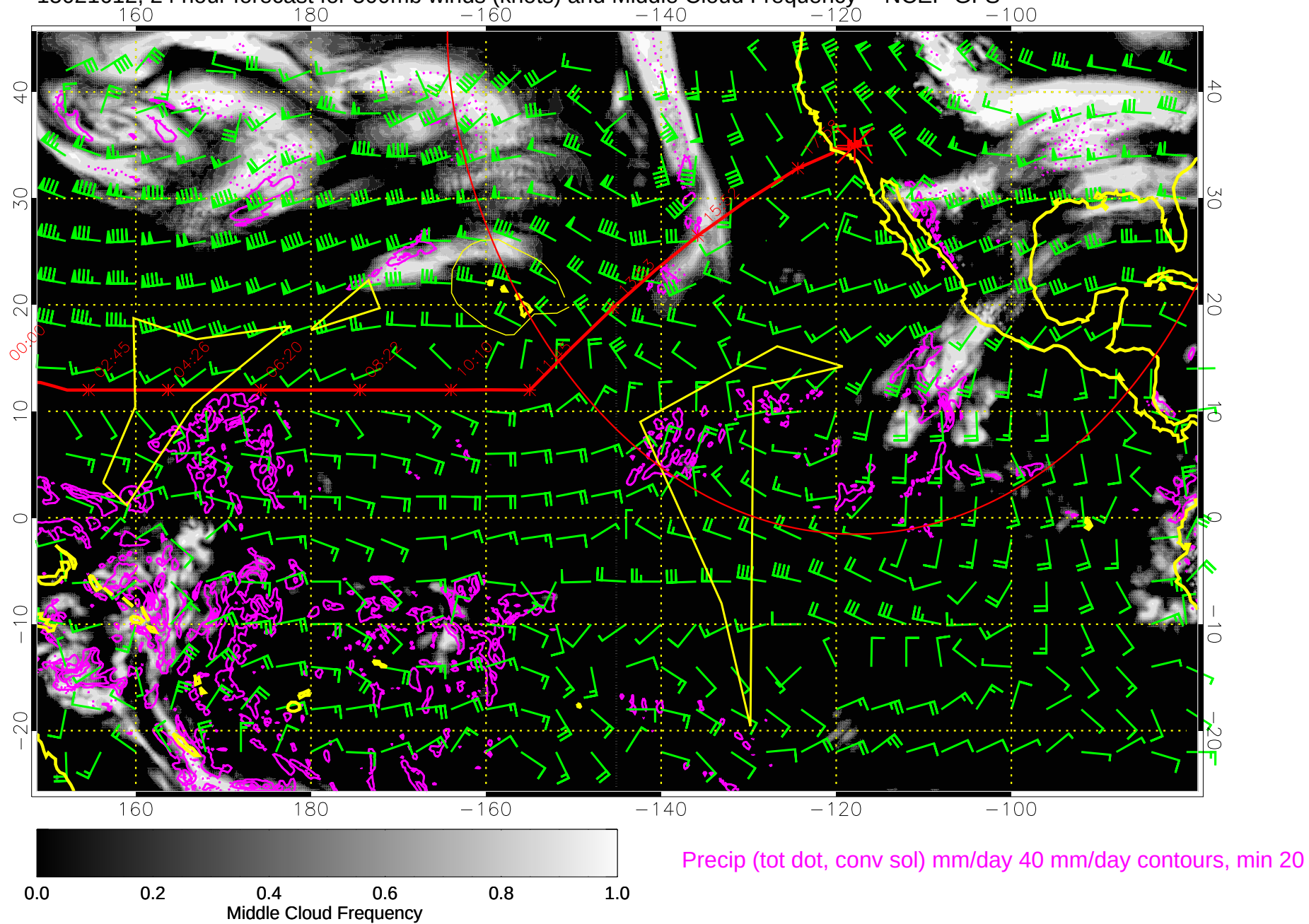
15021612, 24 hour forecast for 500mb winds (knots) and Middle Cloud Frequency -- NCEP GFS
