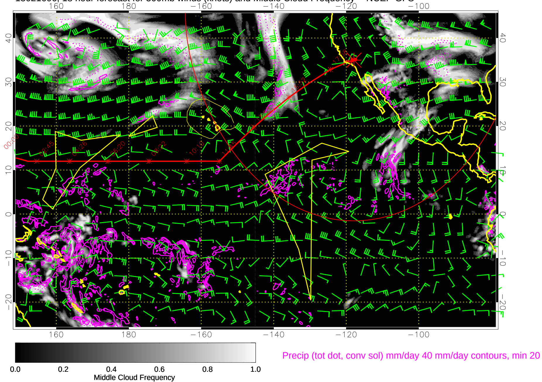
15021606, 18 hour forecast for 500mb winds (knots) and Middle Cloud Frequency -- NCEP GFS
