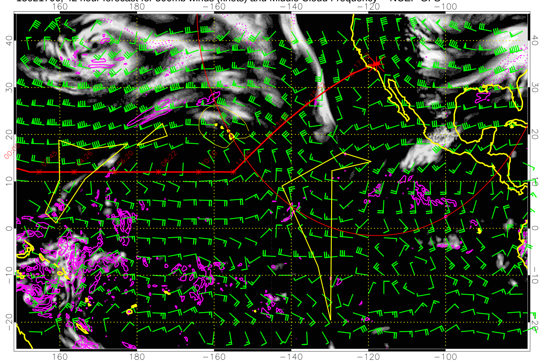
15021706, 42 hour forecast for 500mb winds (knots) and Middle Cloud Frequency -- NCEP GFS
