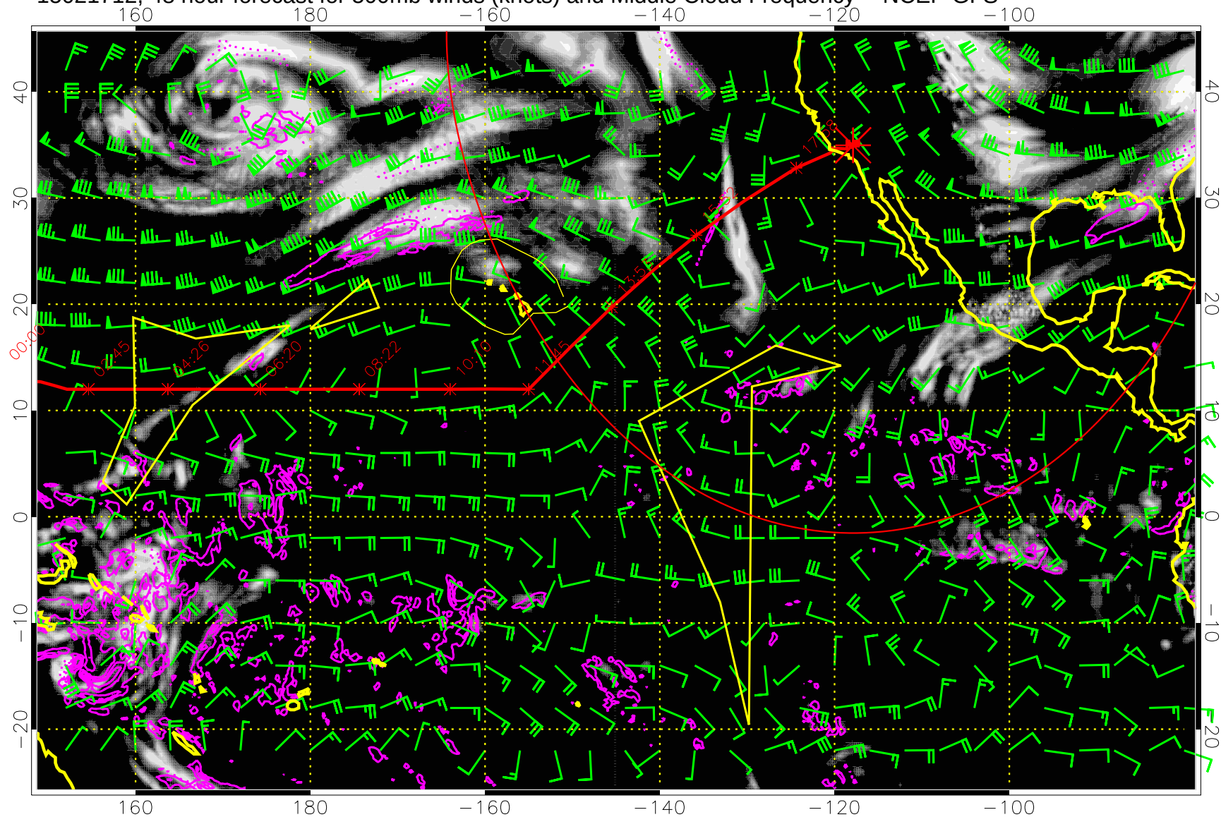
15021712, 48 hour forecast for 500mb winds (knots) and Middle Cloud Frequency -- NCEP GFS
