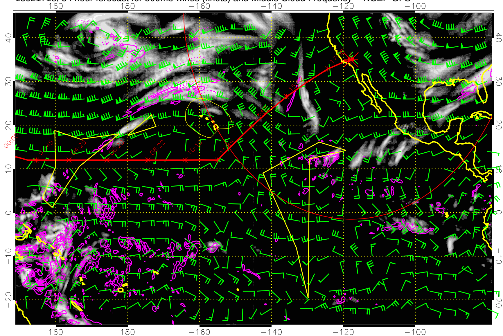
15021718, 54 hour forecast for 500mb winds (knots) and Middle Cloud Frequency -- NCEP GFS
