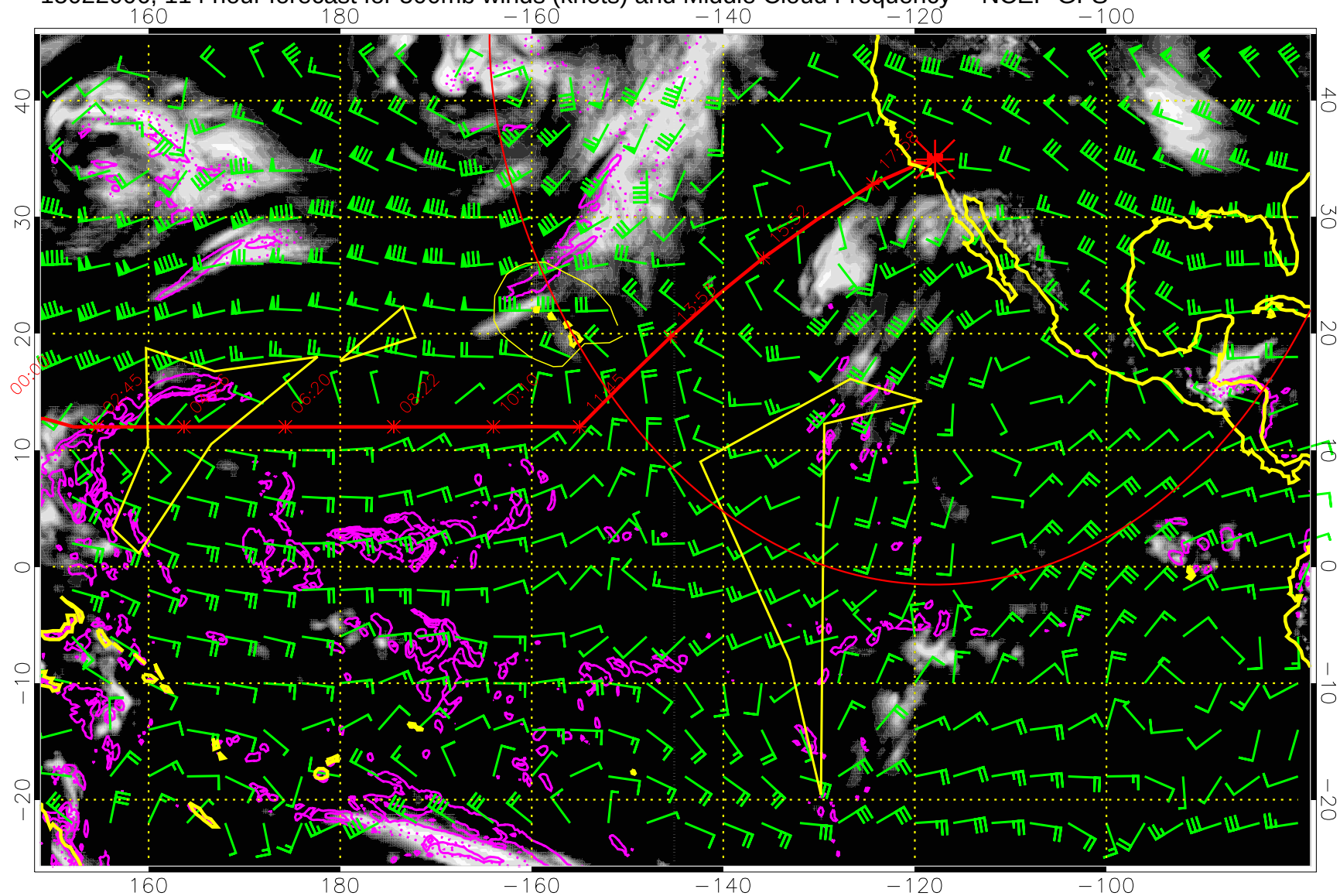
15022006, 114 hour forecast for 500mb winds (knots) and Middle Cloud Frequency -- NCEP GFS
