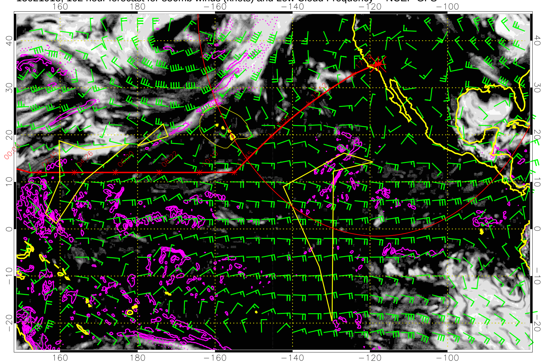
15021918, 102 hour forecast for 850mb winds (knots) and Low Cloud Frequency -- NCEP GFS
