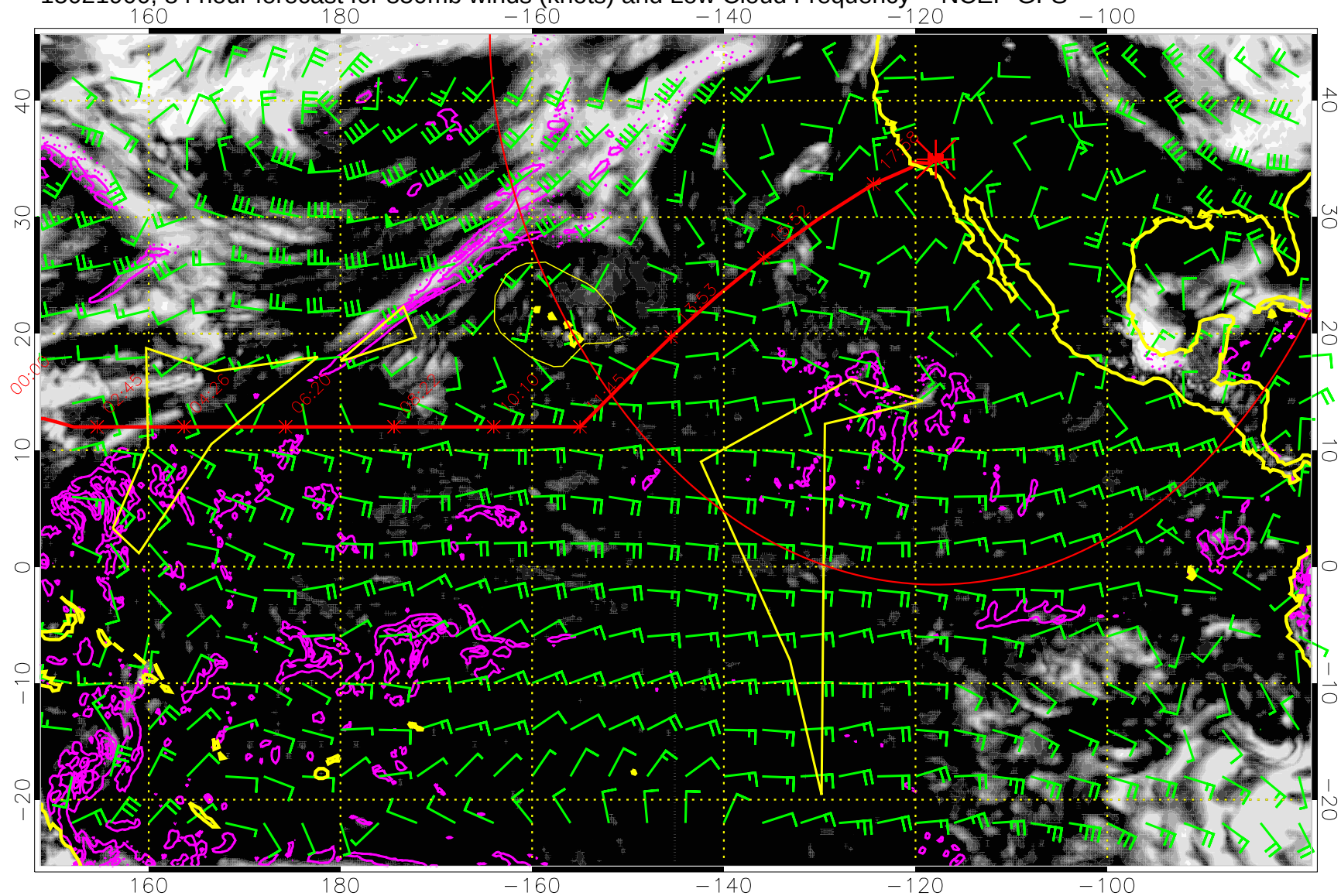
15021900, 84 hour forecast for 850mb winds (knots) and Low Cloud Frequency -- NCEP GFS
