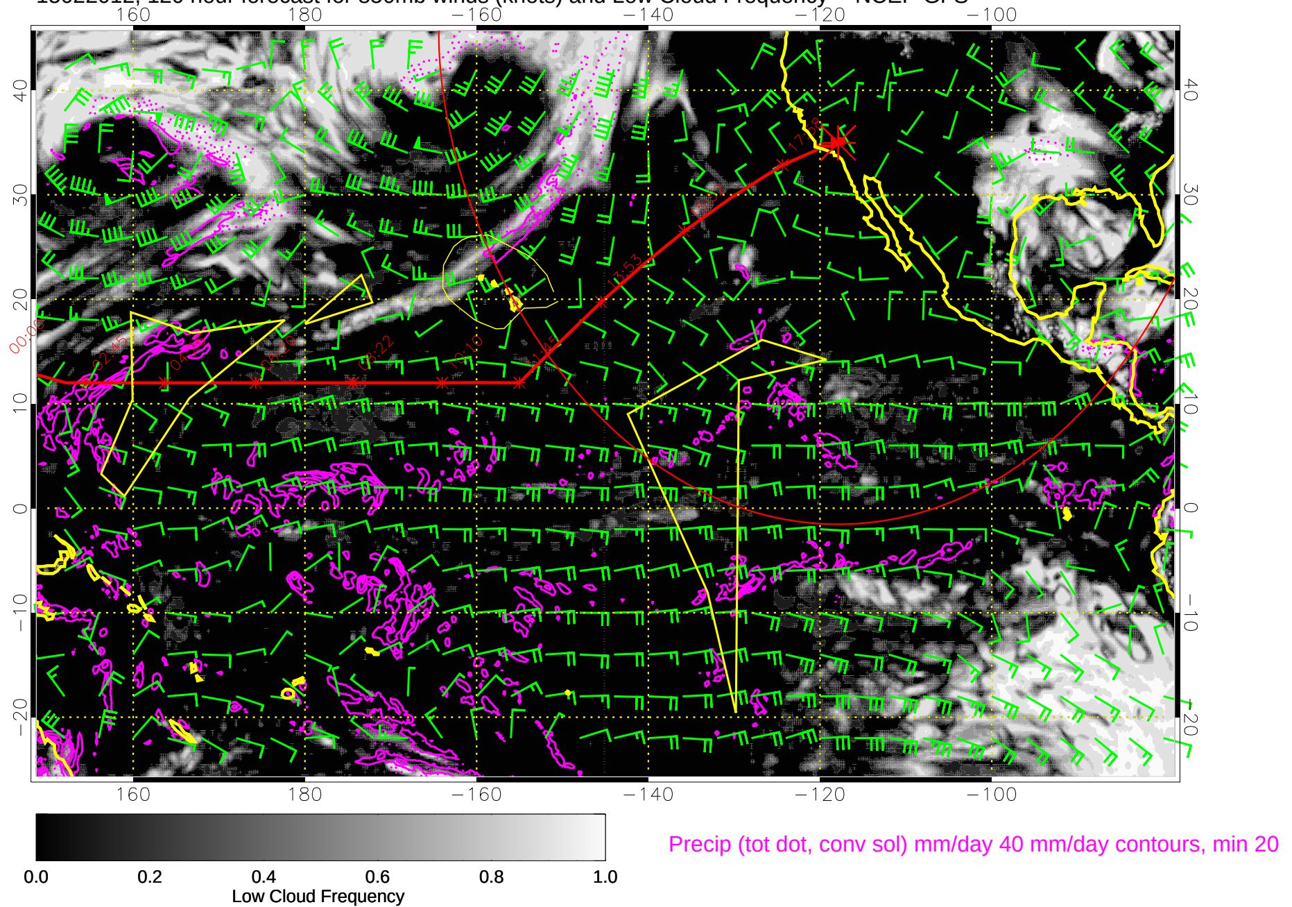
15022012, 120 hour forecast for 850mb winds (knots) and Low Cloud Frequency -- NCEP GFS
