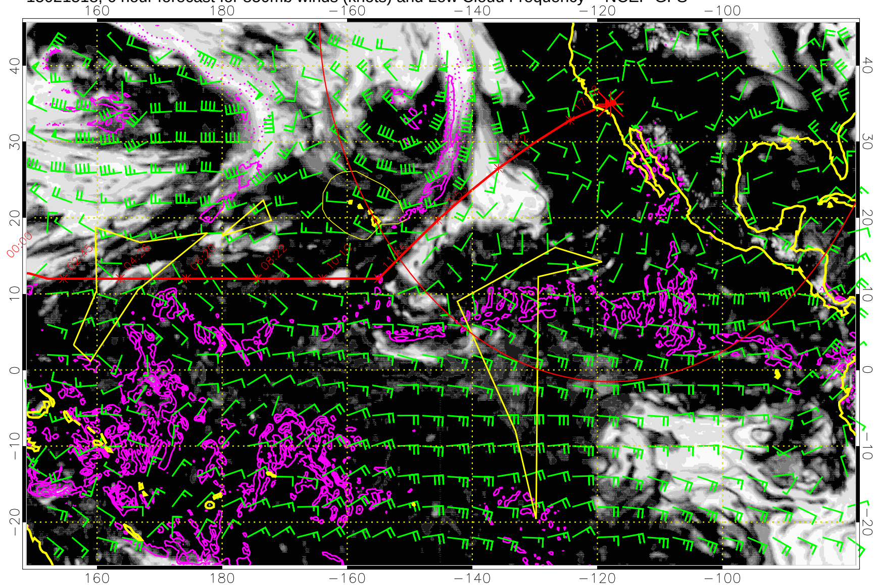
15021518, 6 hour forecast for 850mb winds (knots) and Low Cloud Frequency -- NCEP GFS
