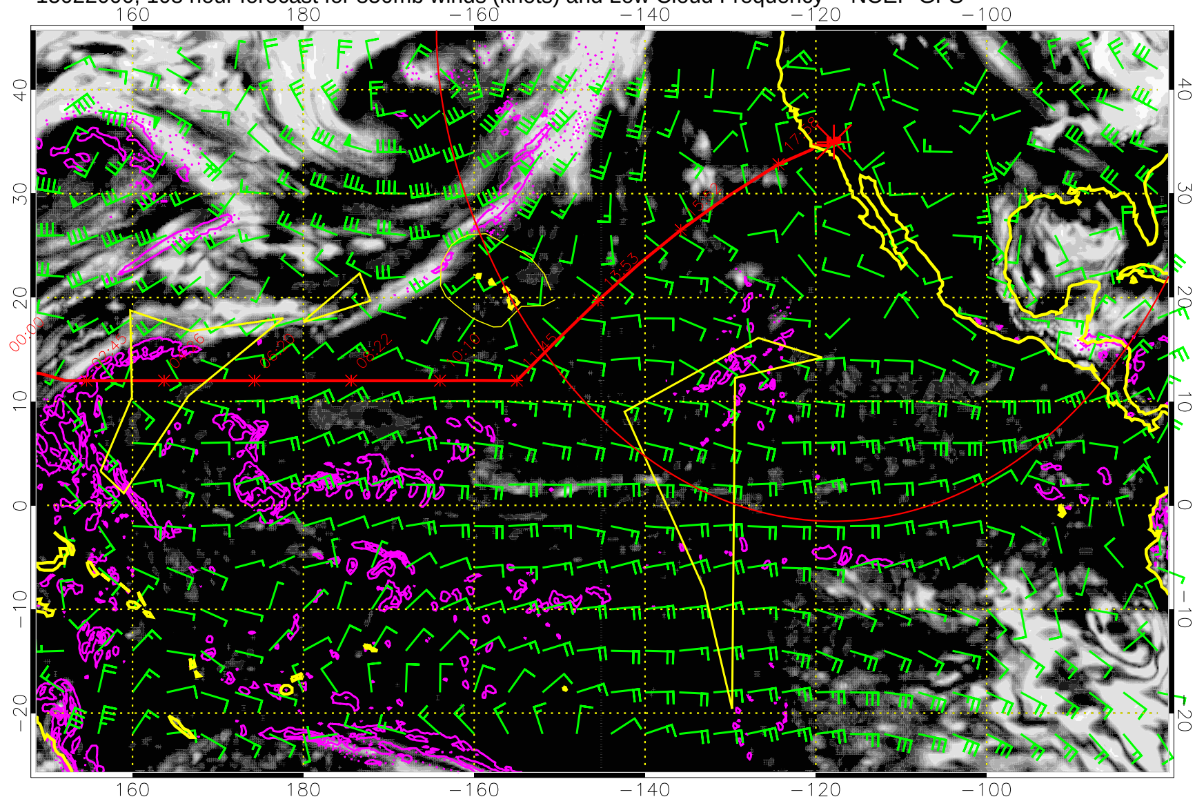
15022000, 108 hour forecast for 850mb winds (knots) and Low Cloud Frequency -- NCEP GFS
