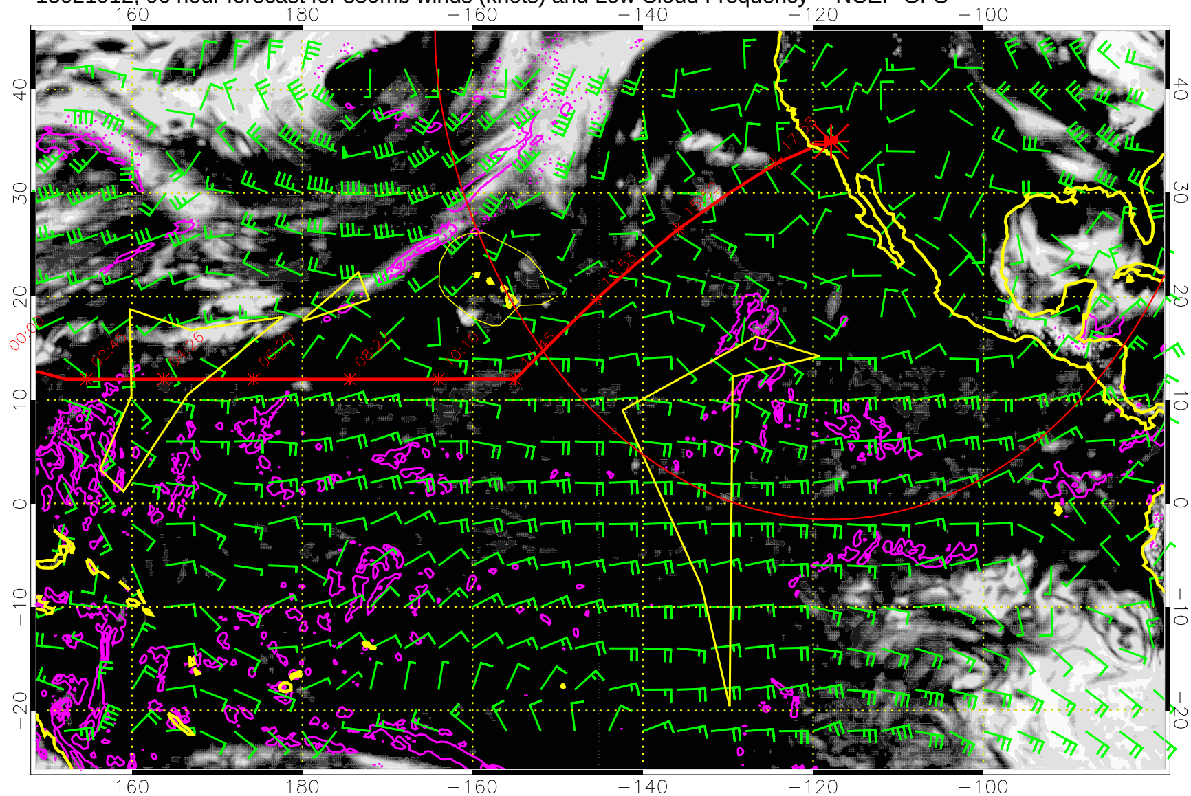
15021912, 96 hour forecast for 850mb winds (knots) and Low Cloud Frequency -- NCEP GFS
