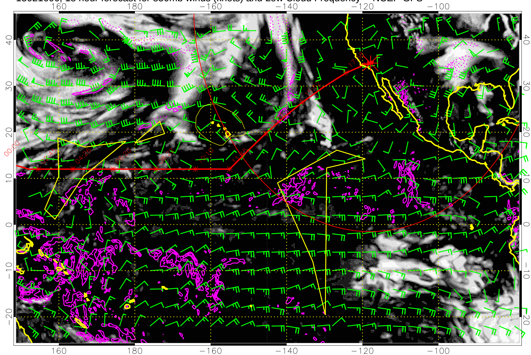
15021606, 18 hour forecast for 850mb winds (knots) and Low Cloud Frequency -- NCEP GFS
