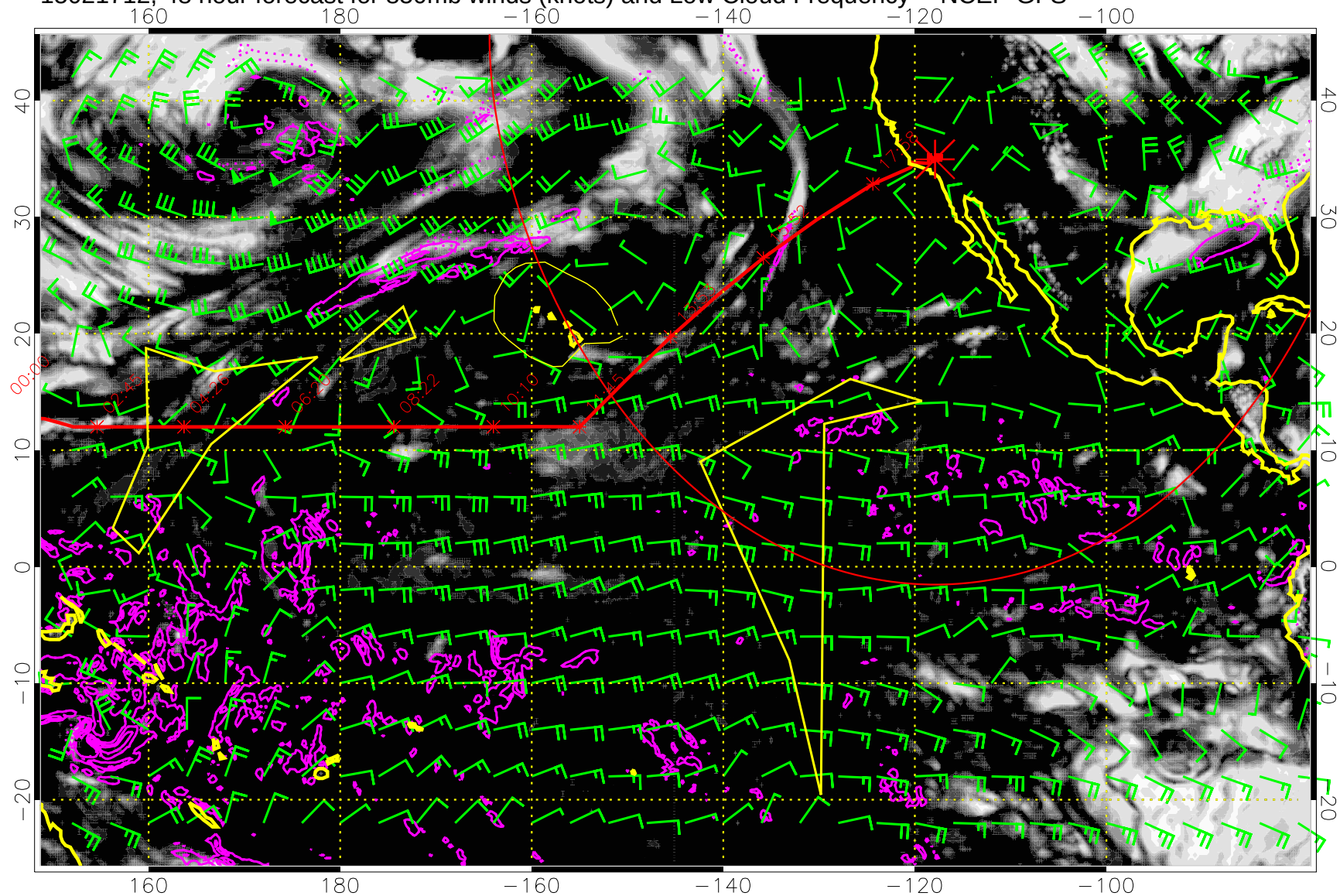
15021712, 48 hour forecast for 850mb winds (knots) and Low Cloud Frequency -- NCEP GFS
