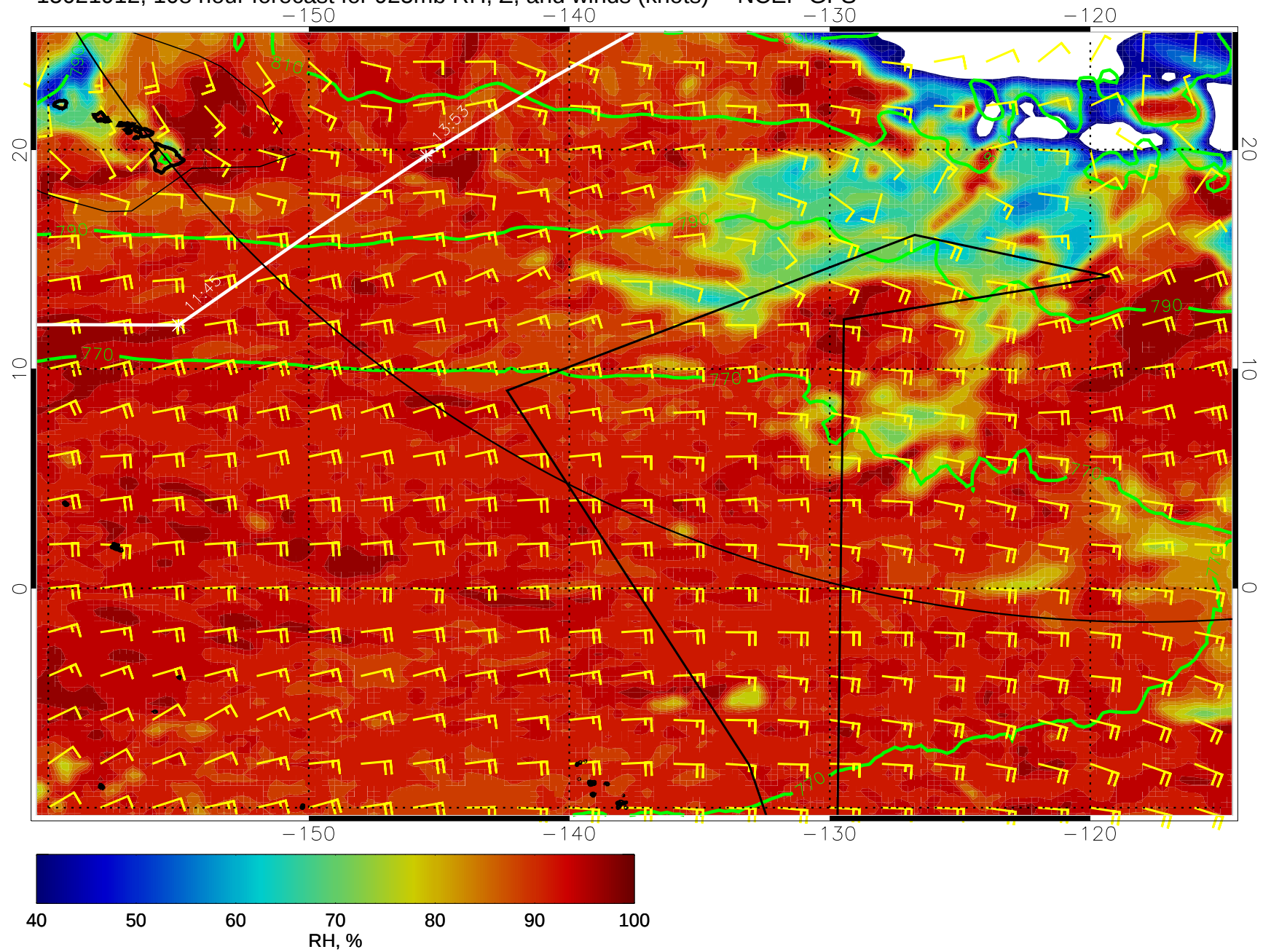
15021912, 108 hour forecast for 925mb RH, Z, and winds (knots) -- NCEP GFS
