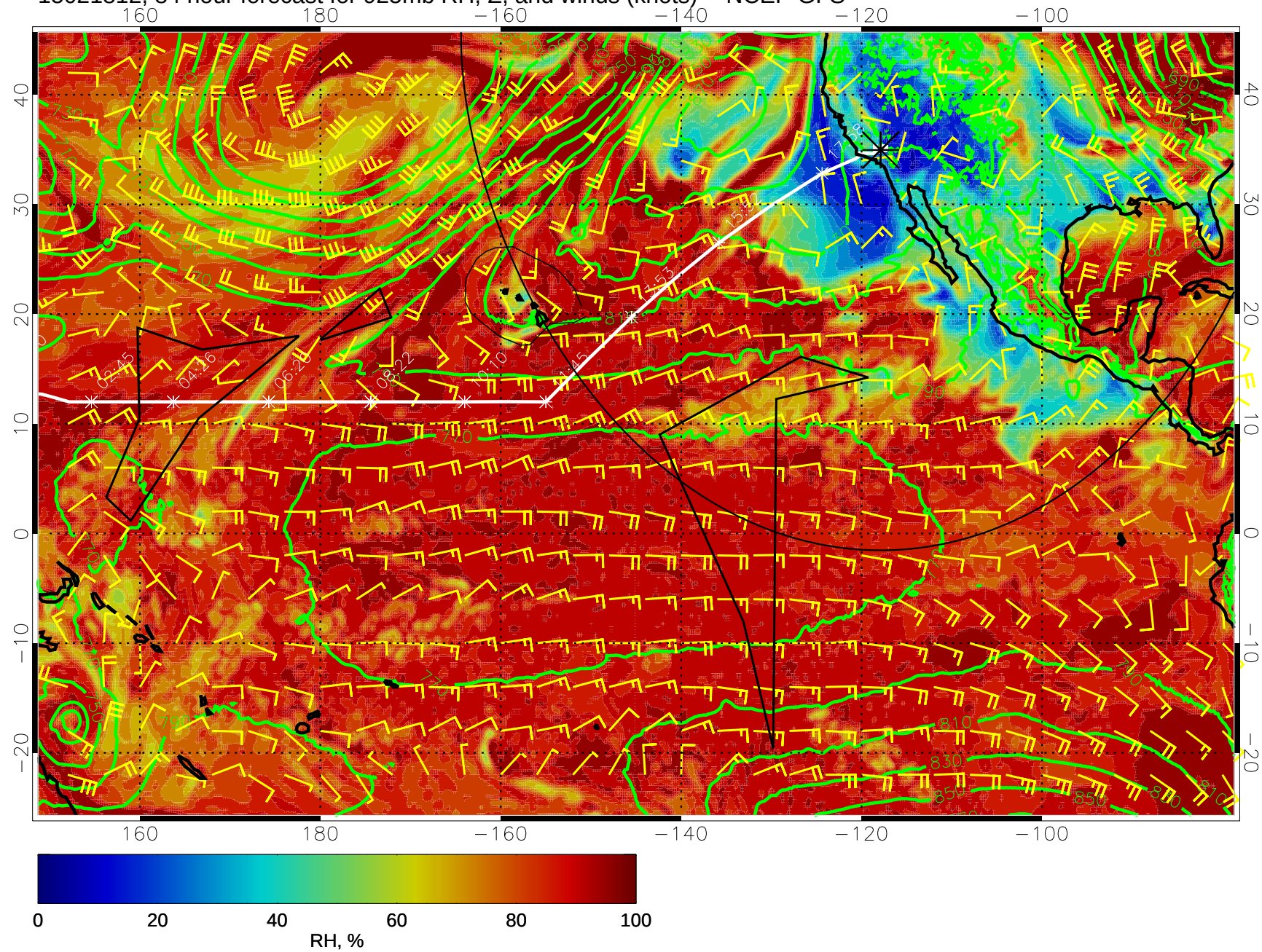
15021812, 84 hour forecast for 925mb RH, Z, and winds (knots) -- NCEP GFS
