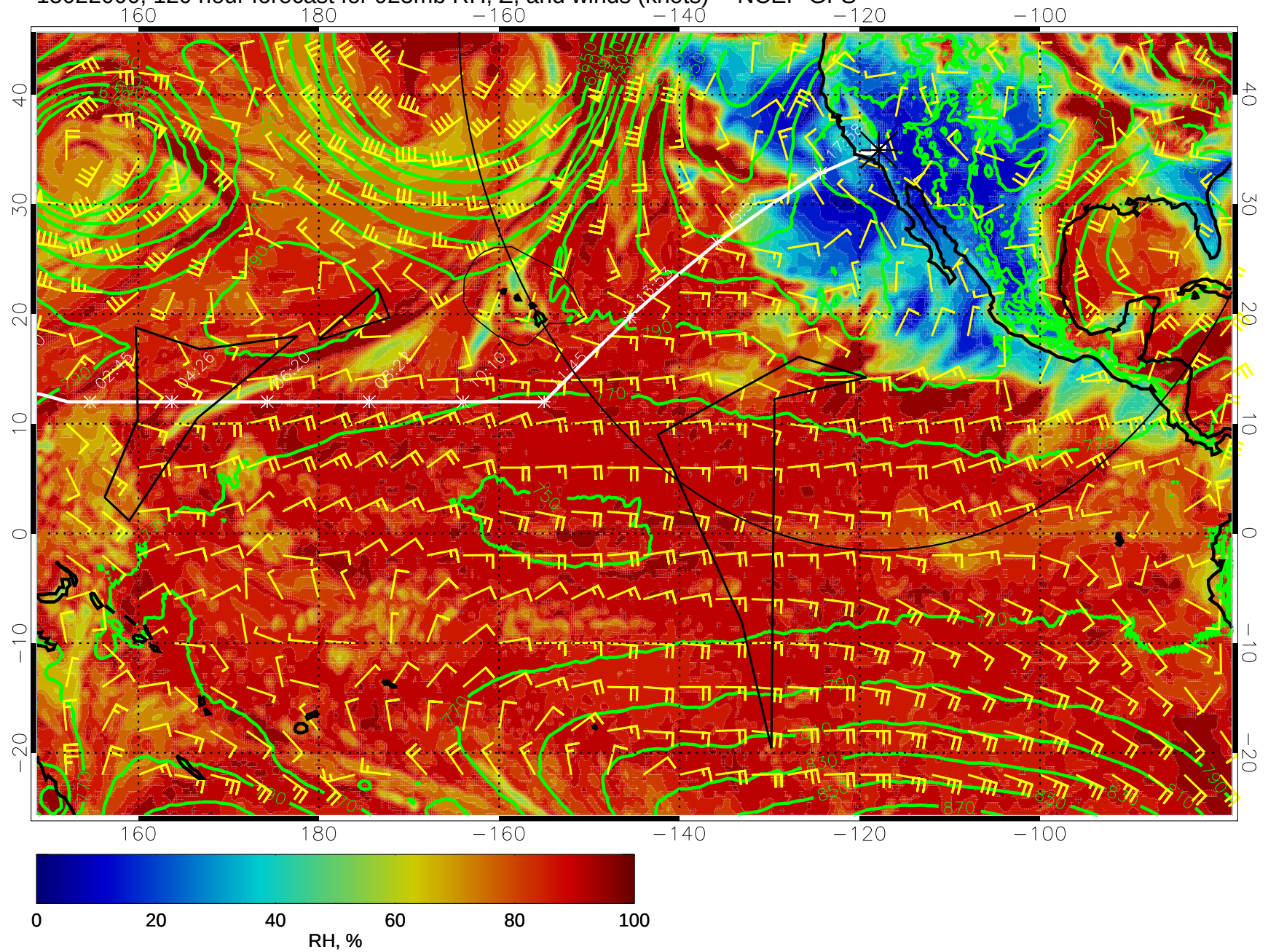
15022000, 120 hour forecast for 925mb RH, Z, and winds (knots) -- NCEP GFS
