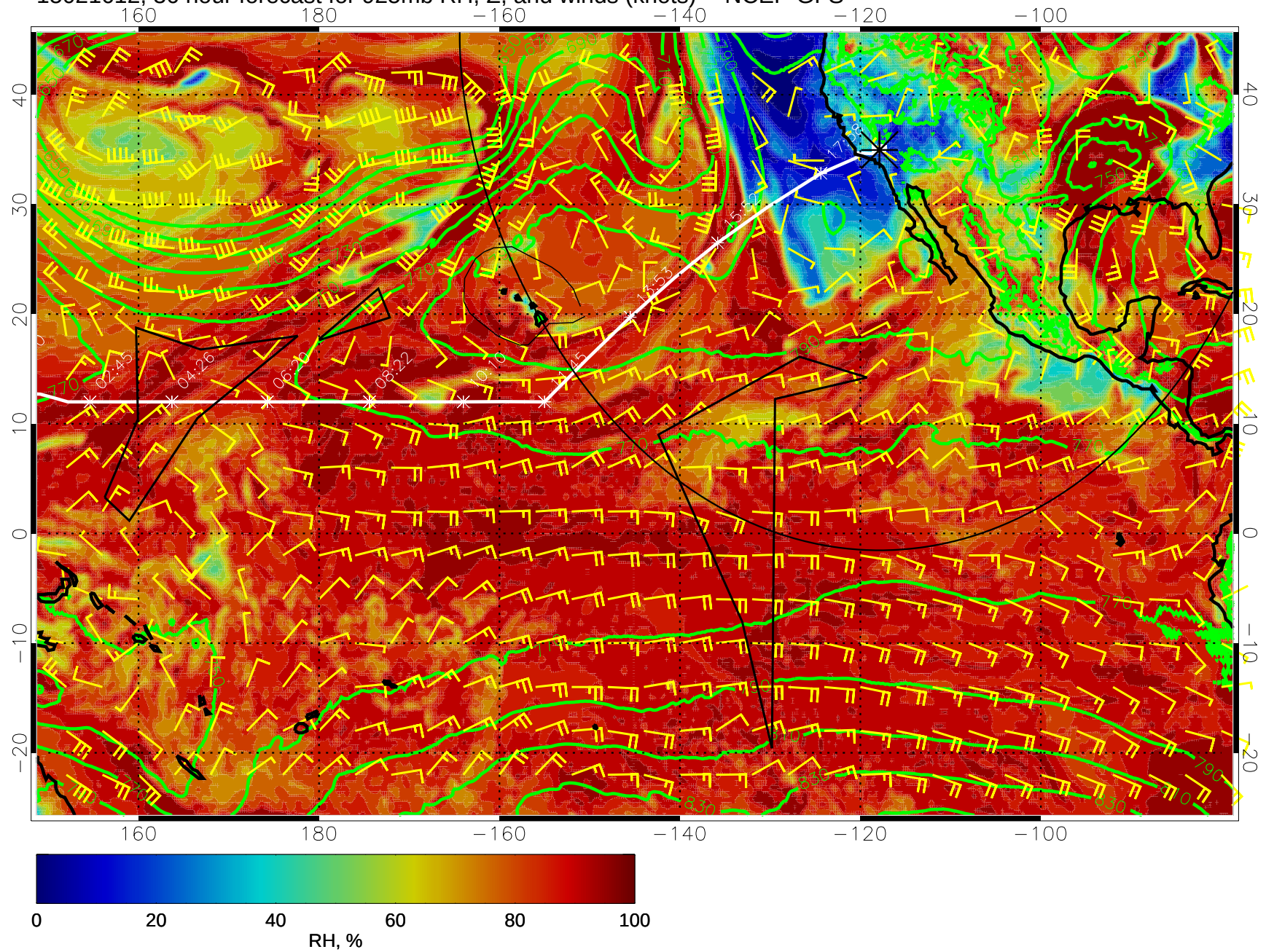
15021612, 36 hour forecast for 925mb RH, Z, and winds (knots) -- NCEP GFS
