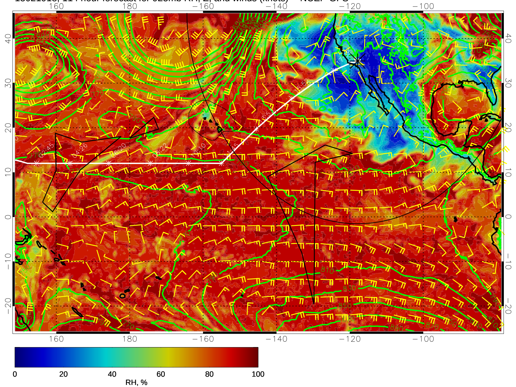
15021918, 114 hour forecast for 925mb RH, Z, and winds (knots) -- NCEP GFS
