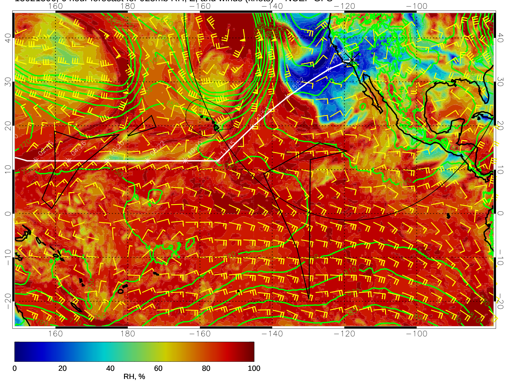
15021506, 6 hour forecast for 925mb RH, Z, and winds (knots) -- NCEP GFS
