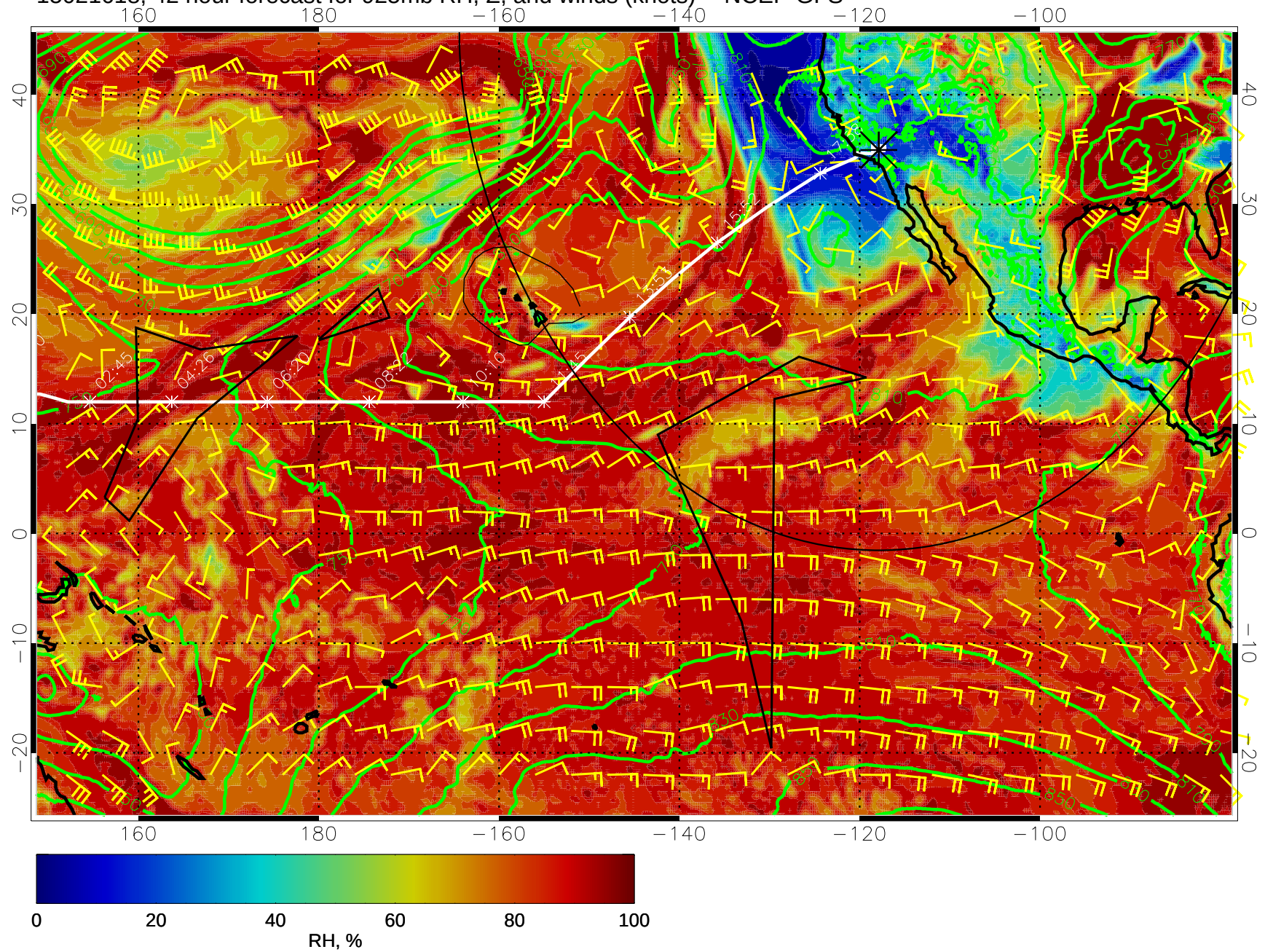
15021618, 42 hour forecast for 925mb RH, Z, and winds (knots) -- NCEP GFS
