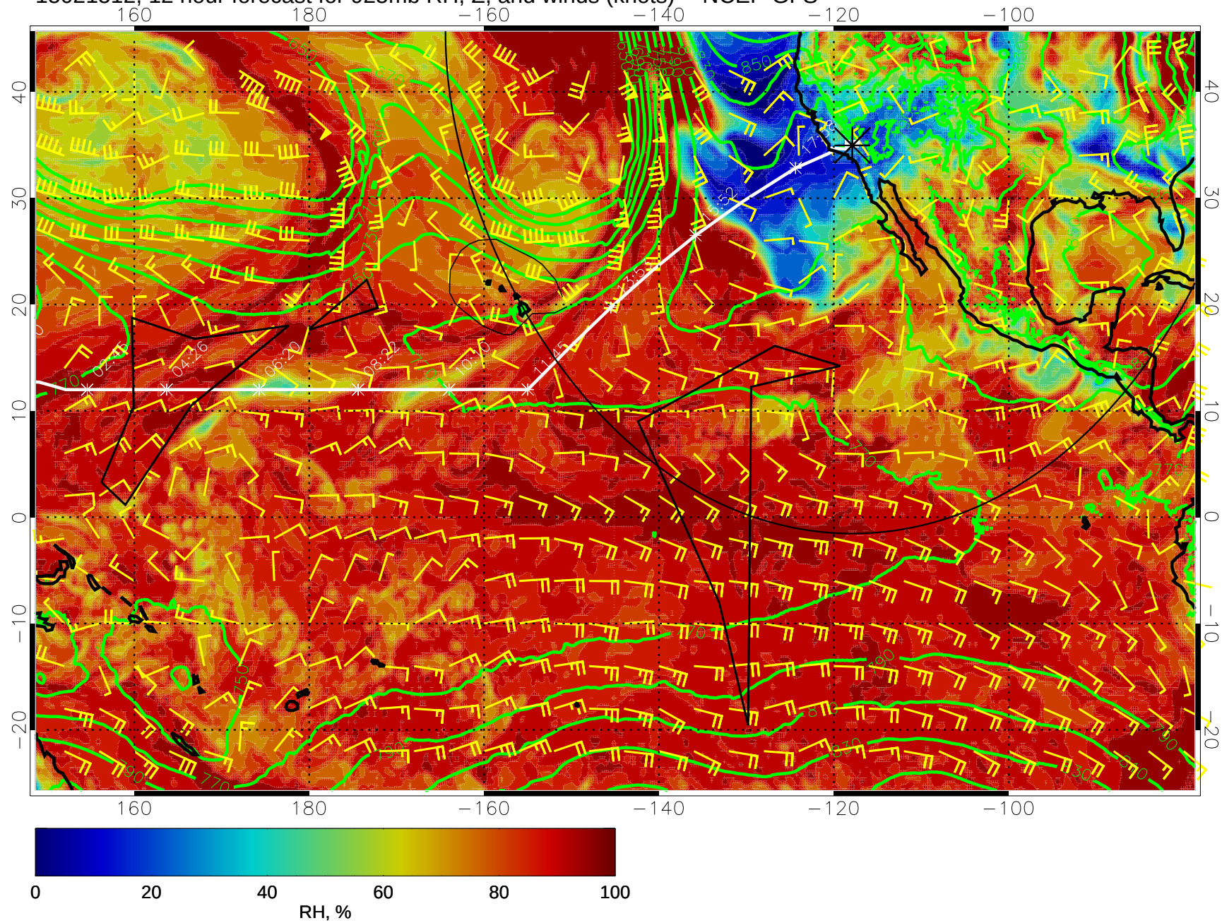
15021512, 12 hour forecast for 925mb RH, Z, and winds (knots) -- NCEP GFS
