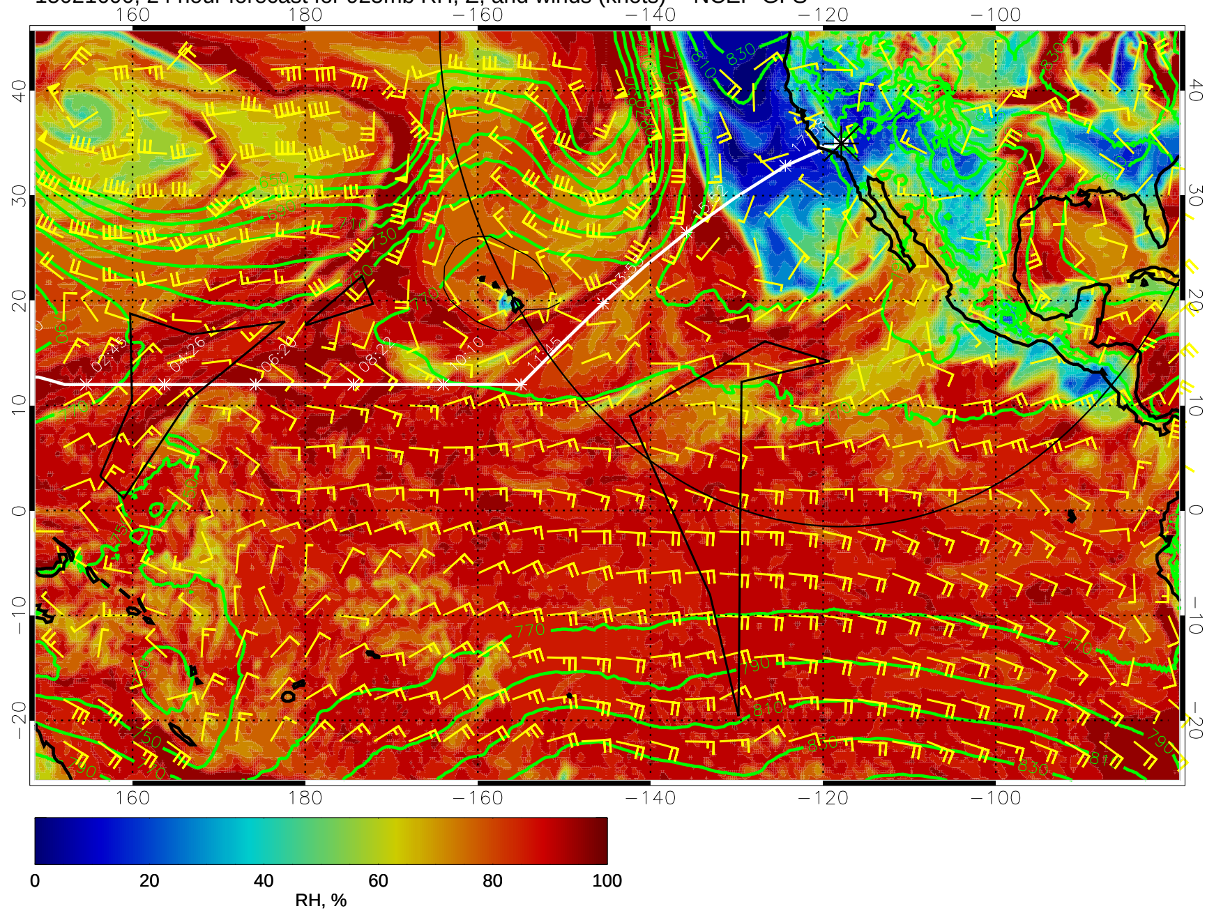
15021600, 24 hour forecast for 925mb RH, Z, and winds (knots) -- NCEP GFS
