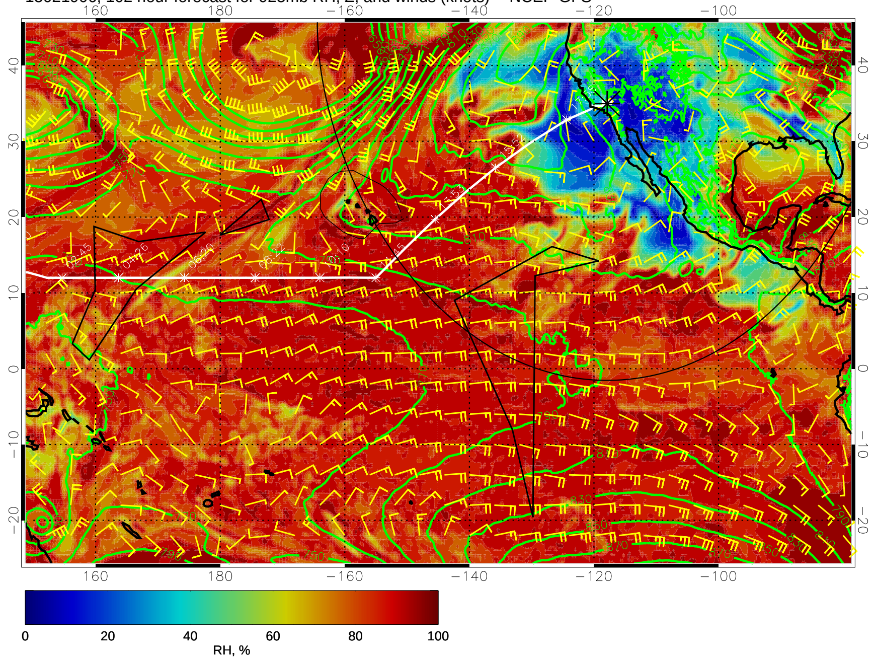
15021906, 102 hour forecast for 925mb RH, Z, and winds (knots) -- NCEP GFS
