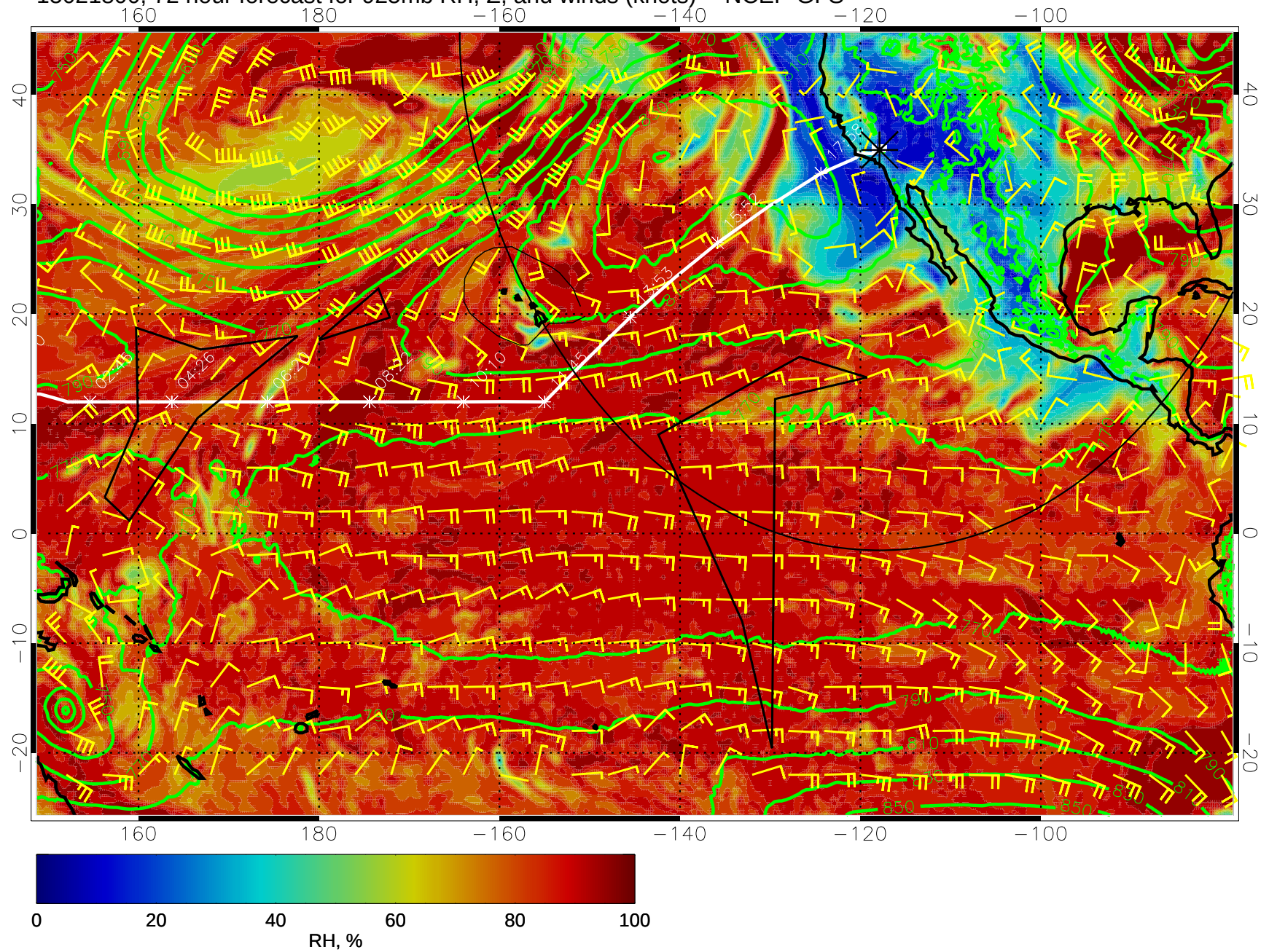
15021800, 72 hour forecast for 925mb RH, Z, and winds (knots) -- NCEP GFS
