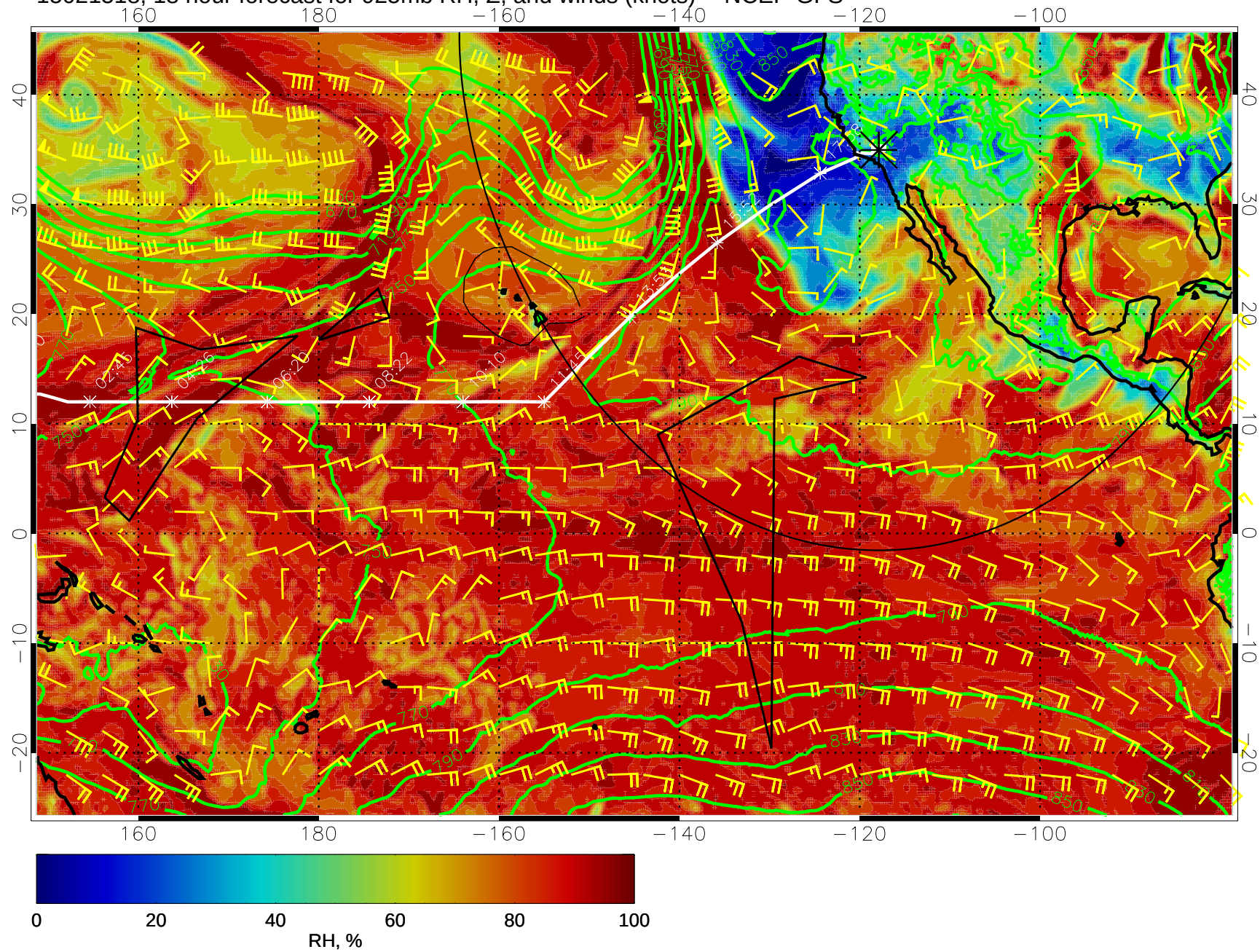
15021518, 18 hour forecast for 925mb RH, Z, and winds (knots) -- NCEP GFS
