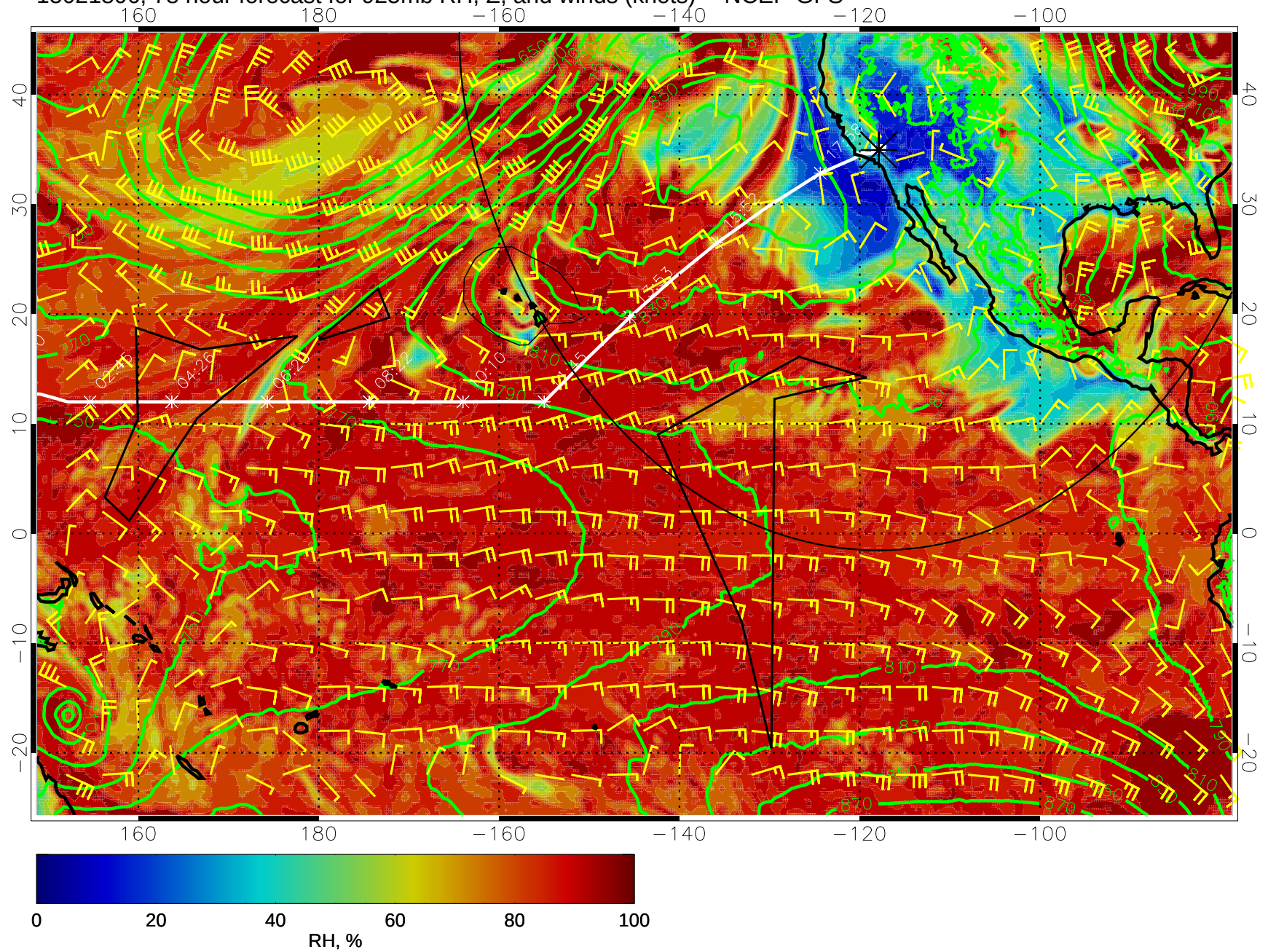
15021806, 78 hour forecast for 925mb RH, Z, and winds (knots) -- NCEP GFS
