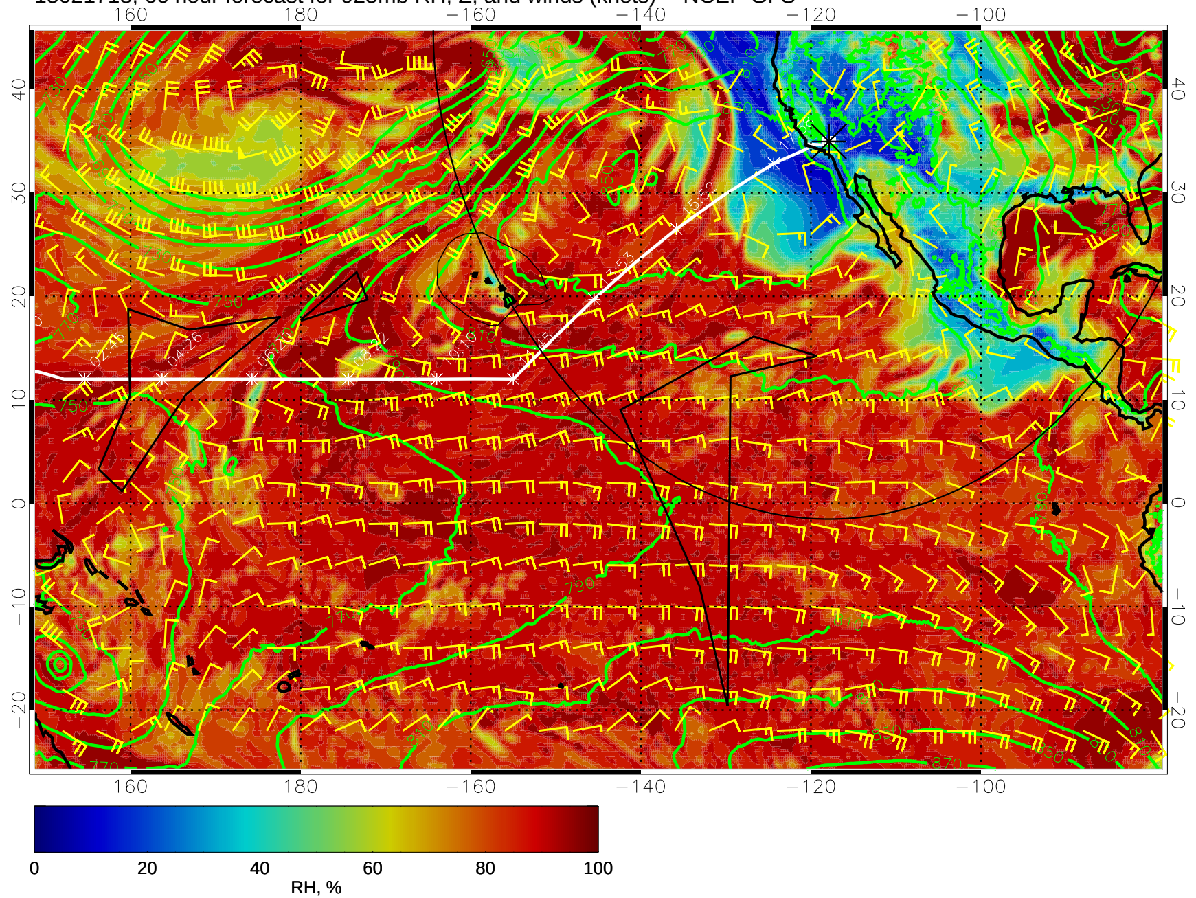
15021718, 66 hour forecast for 925mb RH, Z, and winds (knots) -- NCEP GFS
