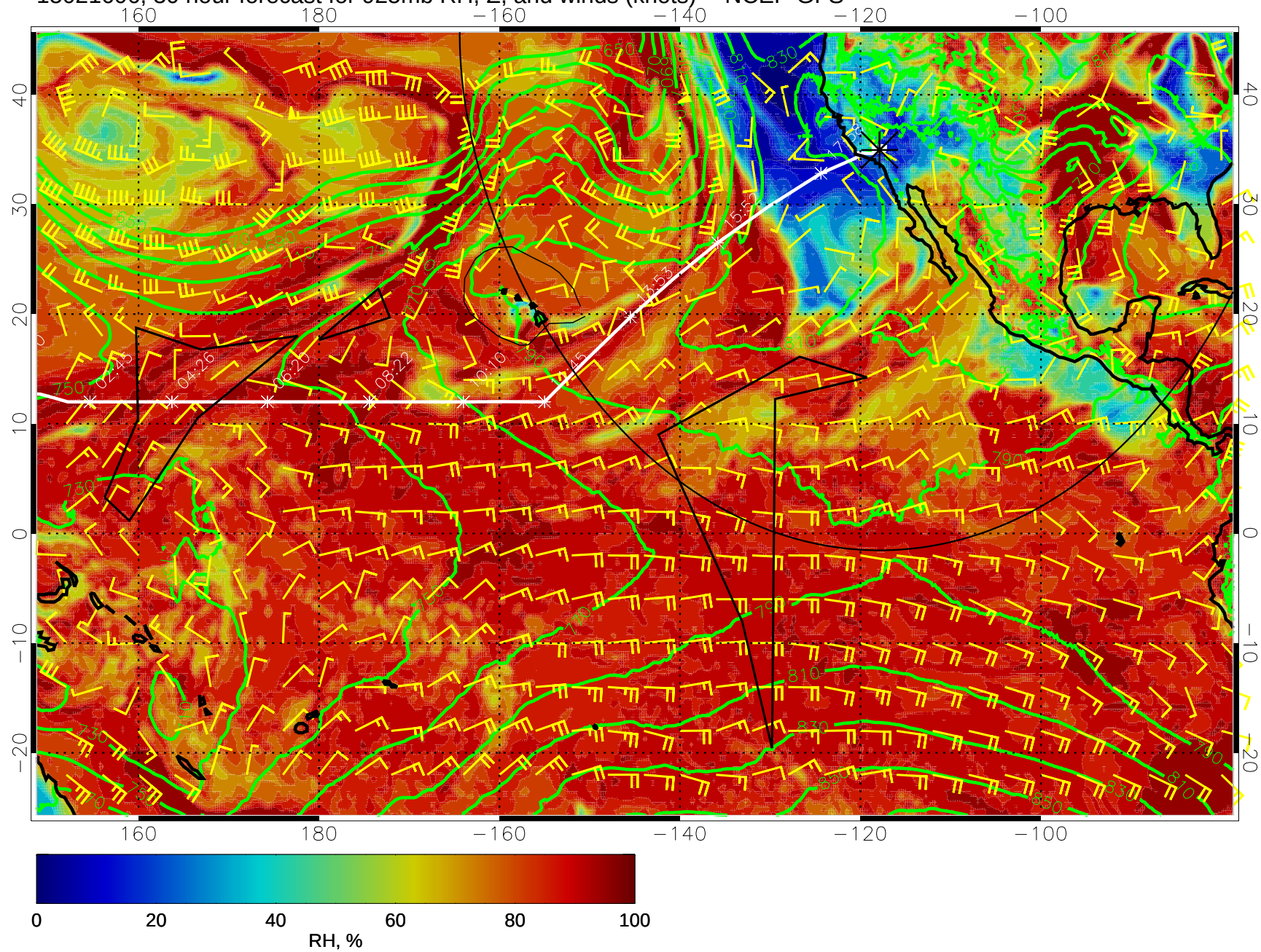
15021606, 30 hour forecast for 925mb RH, Z, and winds (knots) -- NCEP GFS
