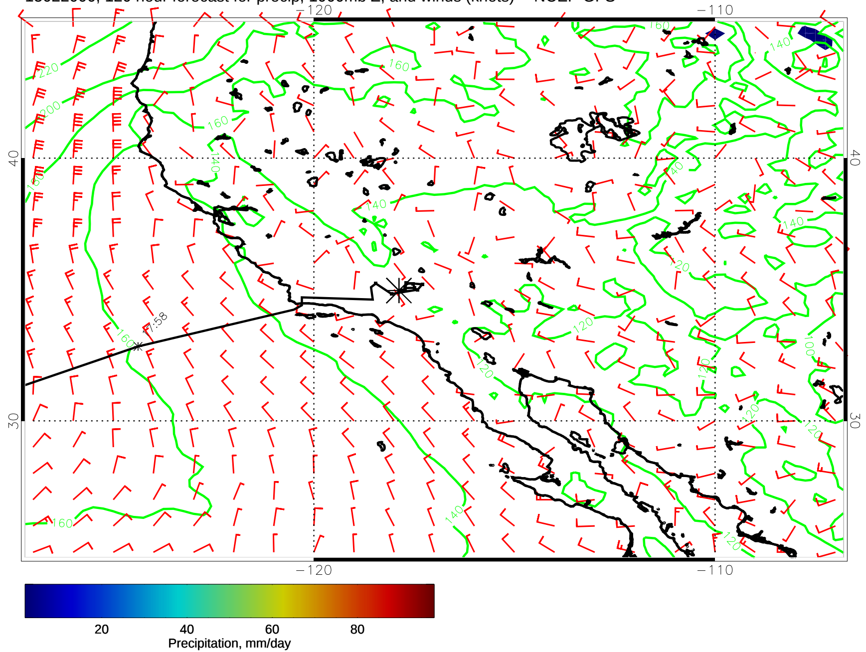
15022000, 120 hour forecast for precip, 1000mb Z, and winds (knots) -- NCEP GFS
