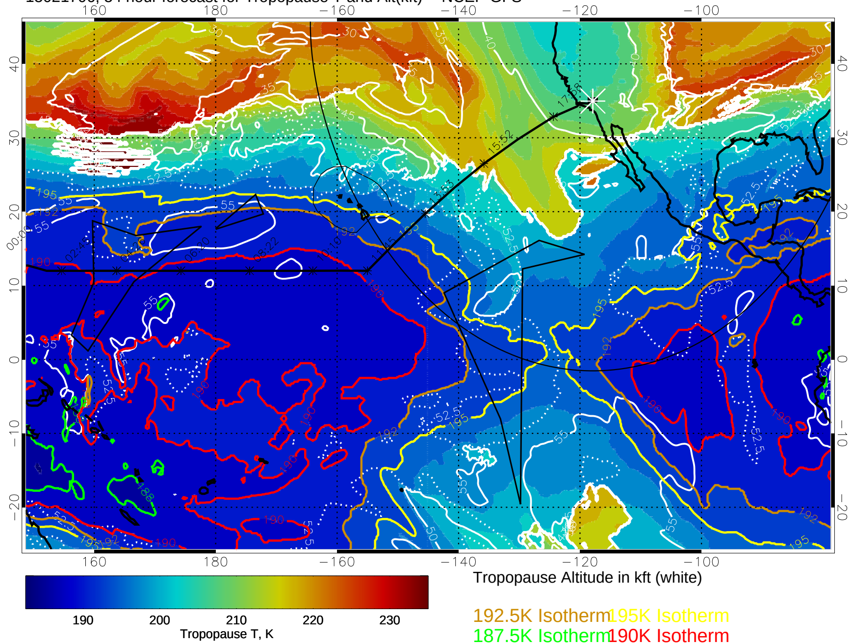
15021706, 54 hour forecast for Tropopause T and Alt(kft) -- NCEP GFS
