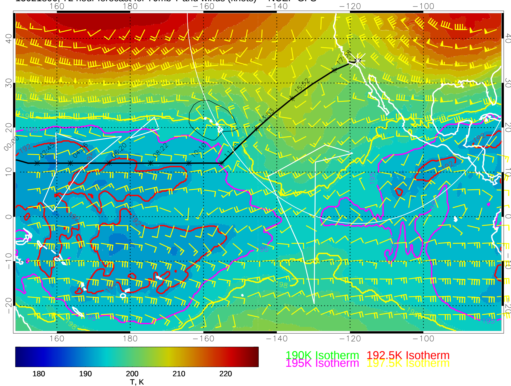
15021800, 72 hour forecast for 70mb T and winds (knots) -- NCEP GFS
