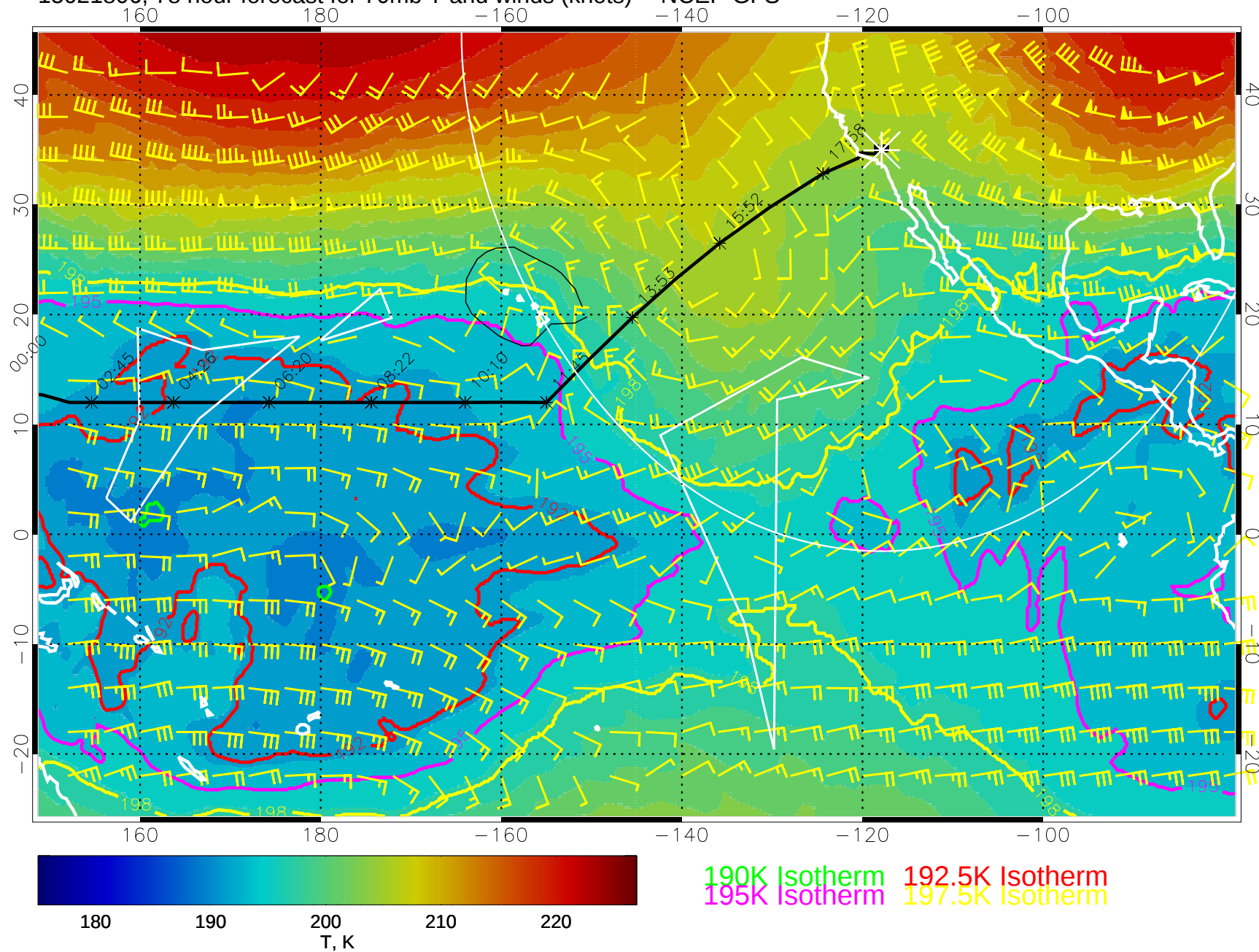
15021806, 78 hour forecast for 70mb T and winds (knots) -- NCEP GFS
