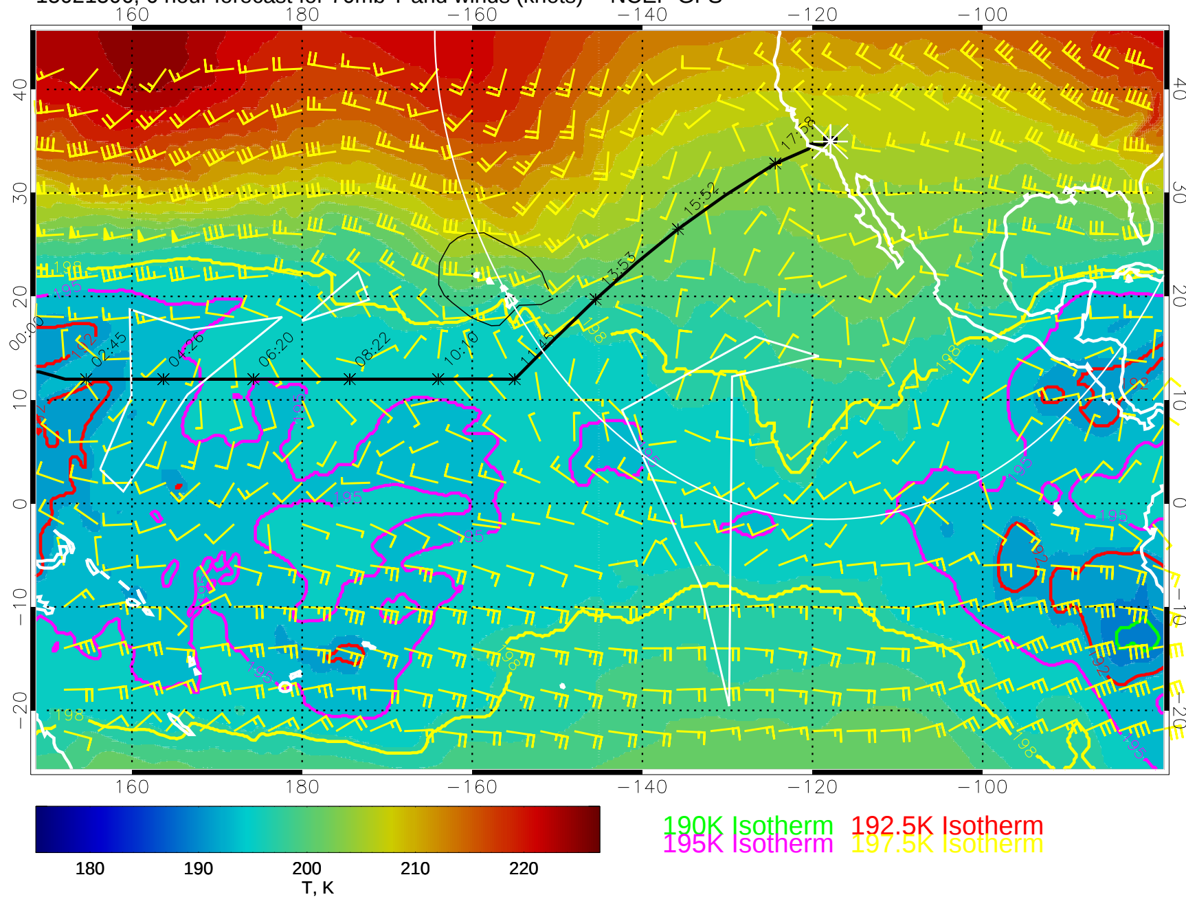
15021506, 6 hour forecast for 70mb T and winds (knots) -- NCEP GFS
