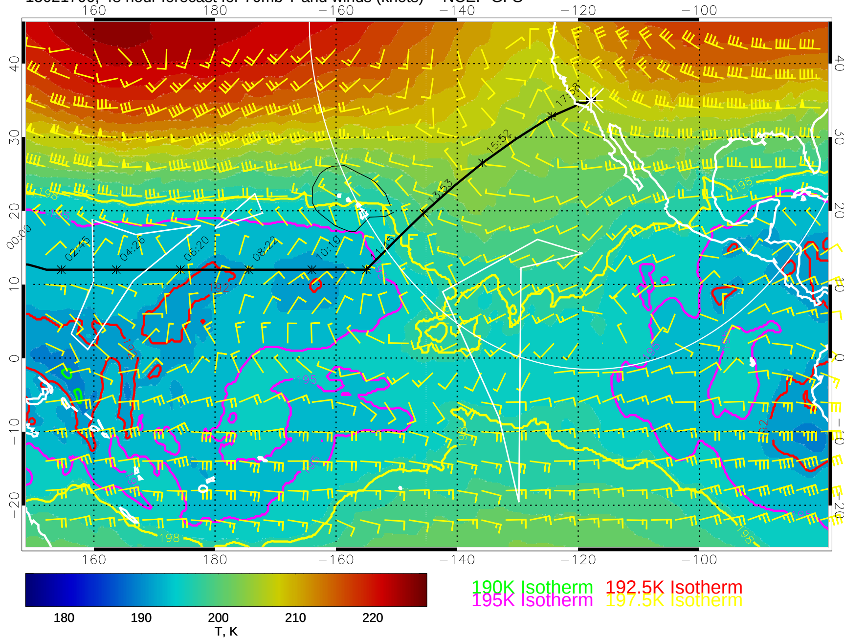
15021700, 48 hour forecast for 70mb T and winds (knots) -- NCEP GFS
