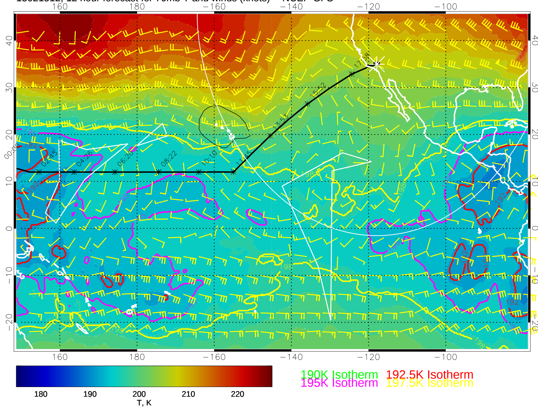
15021512, 12 hour forecast for 70mb T and winds (knots) -- NCEP GFS
