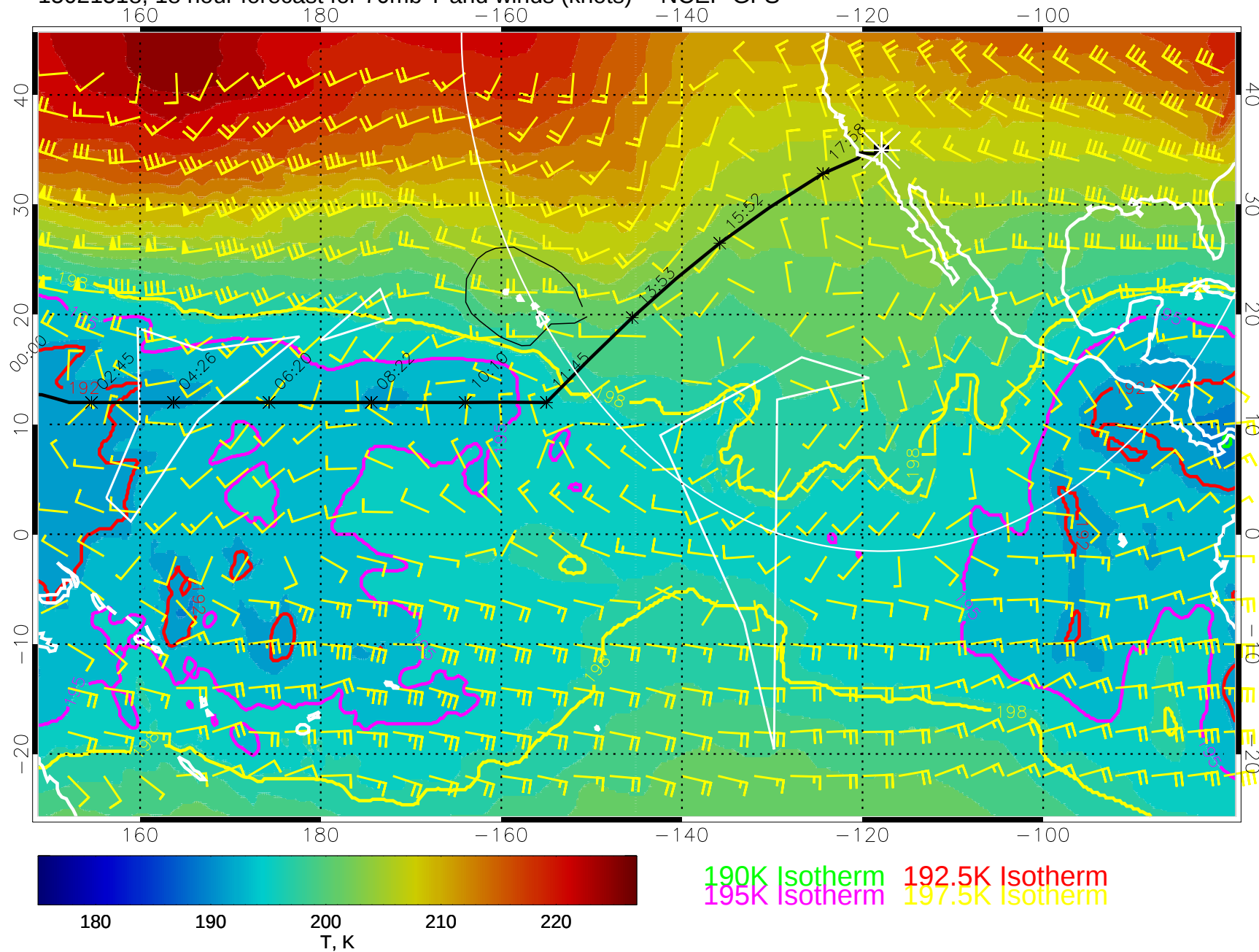
15021518, 18 hour forecast for 70mb T and winds (knots) -- NCEP GFS
