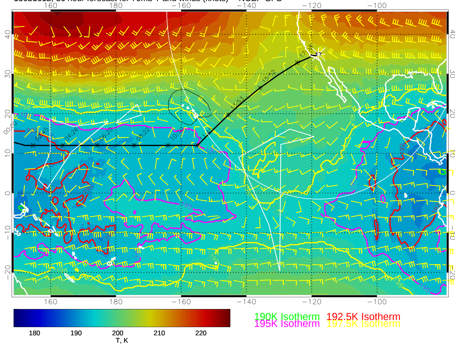
15021612, 36 hour forecast for 70mb T and winds (knots) -- NCEP GFS
