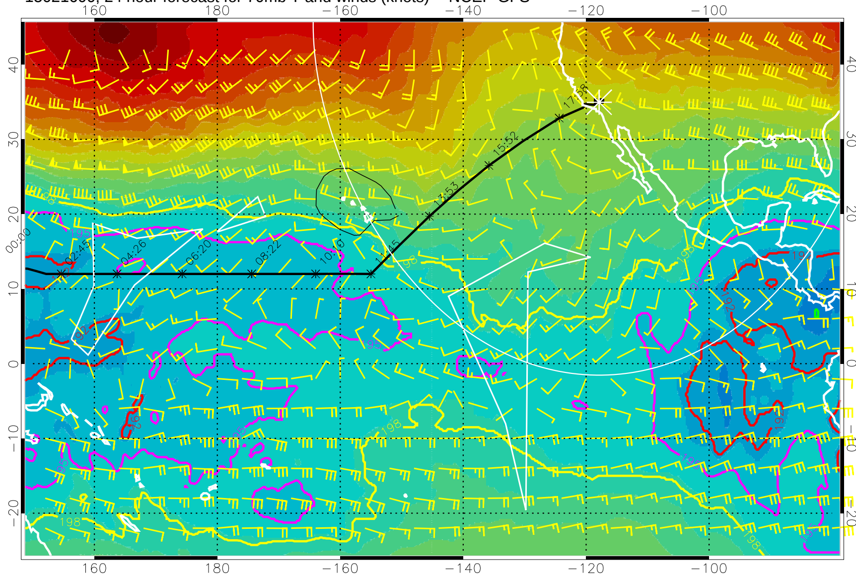
15021600, 24 hour forecast for 70mb T and winds (knots) -- NCEP GFS
