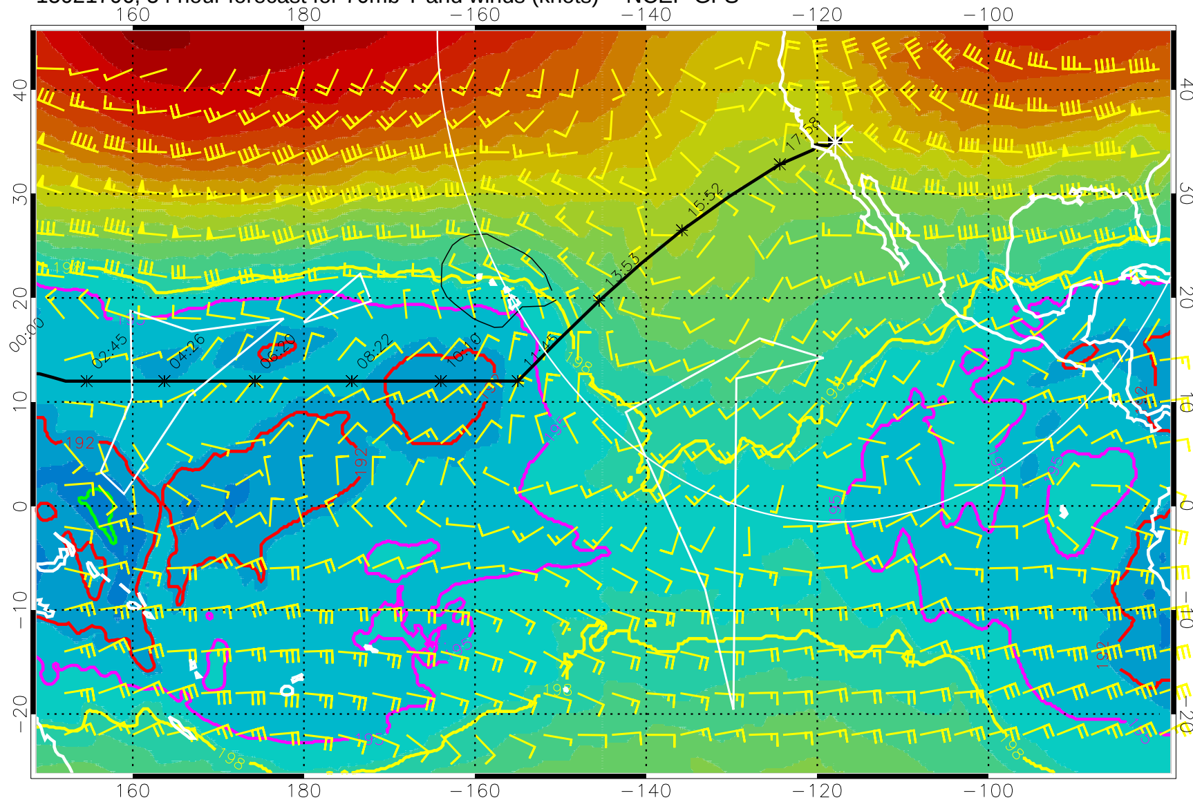
15021706, 54 hour forecast for 70mb T and winds (knots) -- NCEP GFS
