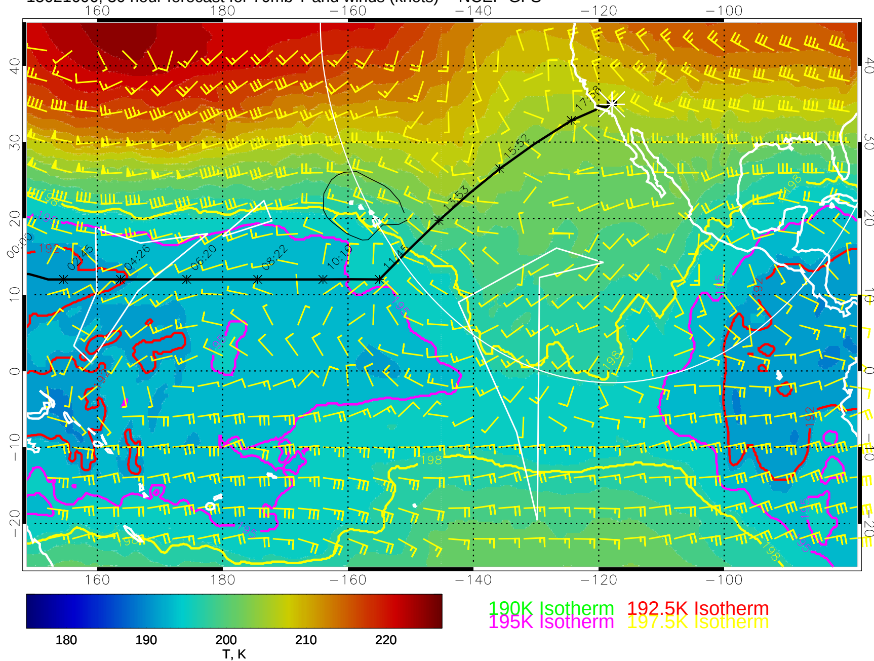
15021606, 30 hour forecast for 70mb T and winds (knots) -- NCEP GFS
