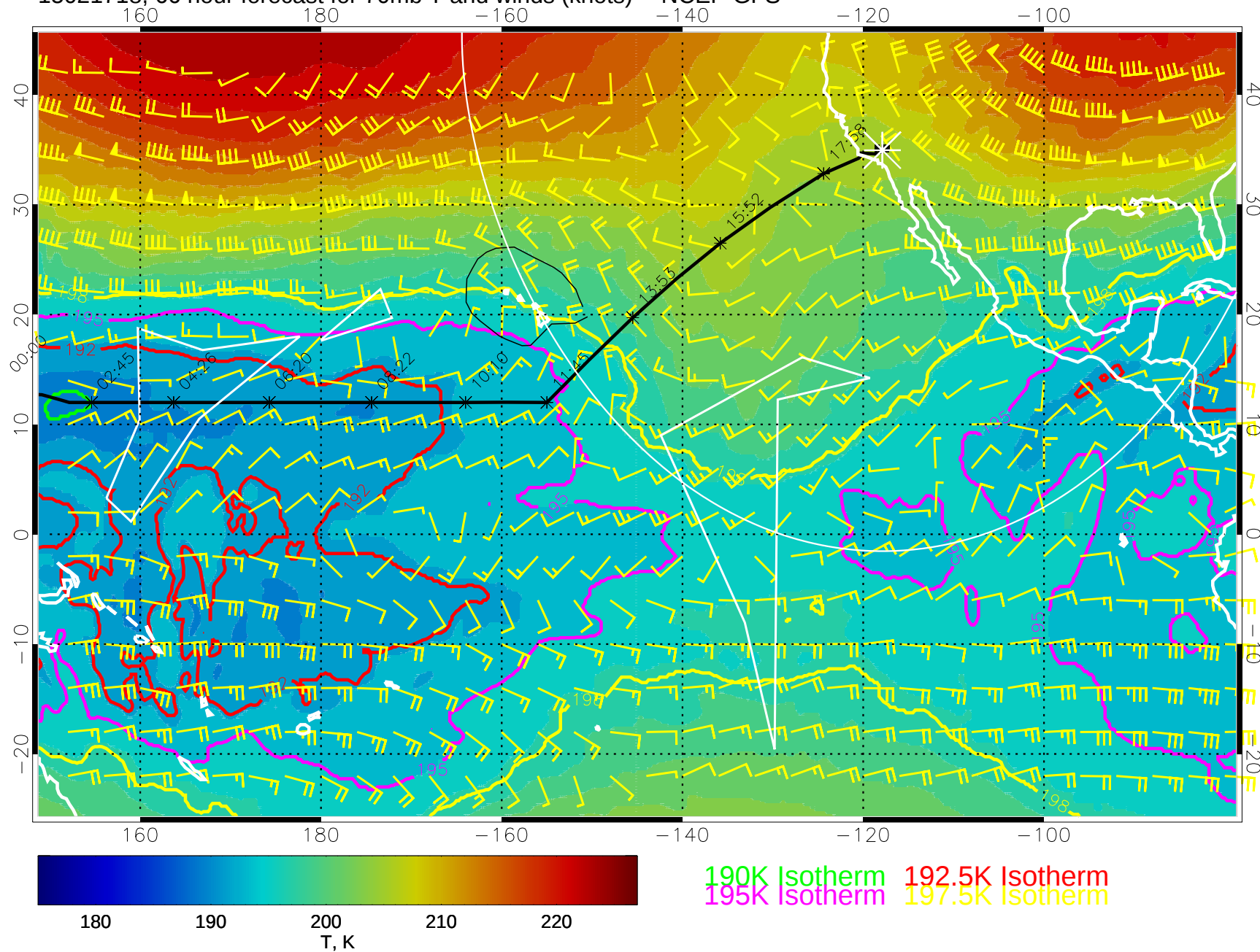
15021718, 66 hour forecast for 70mb T and winds (knots) -- NCEP GFS
