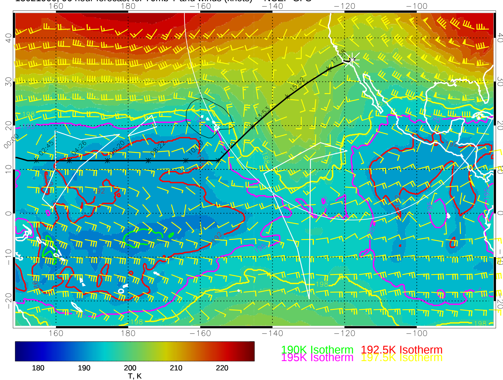
15021900, 96 hour forecast for 70mb T and winds (knots) -- NCEP GFS
