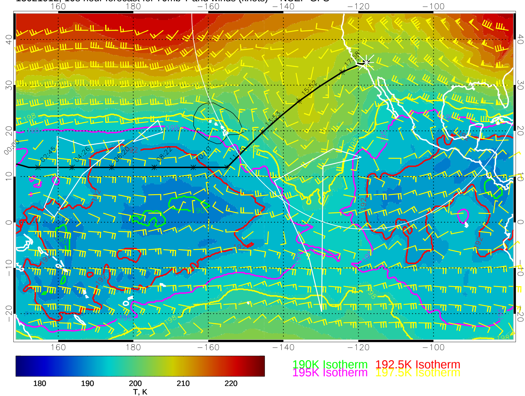
15021912, 108 hour forecast for 70mb T and winds (knots) -- NCEP GFS
