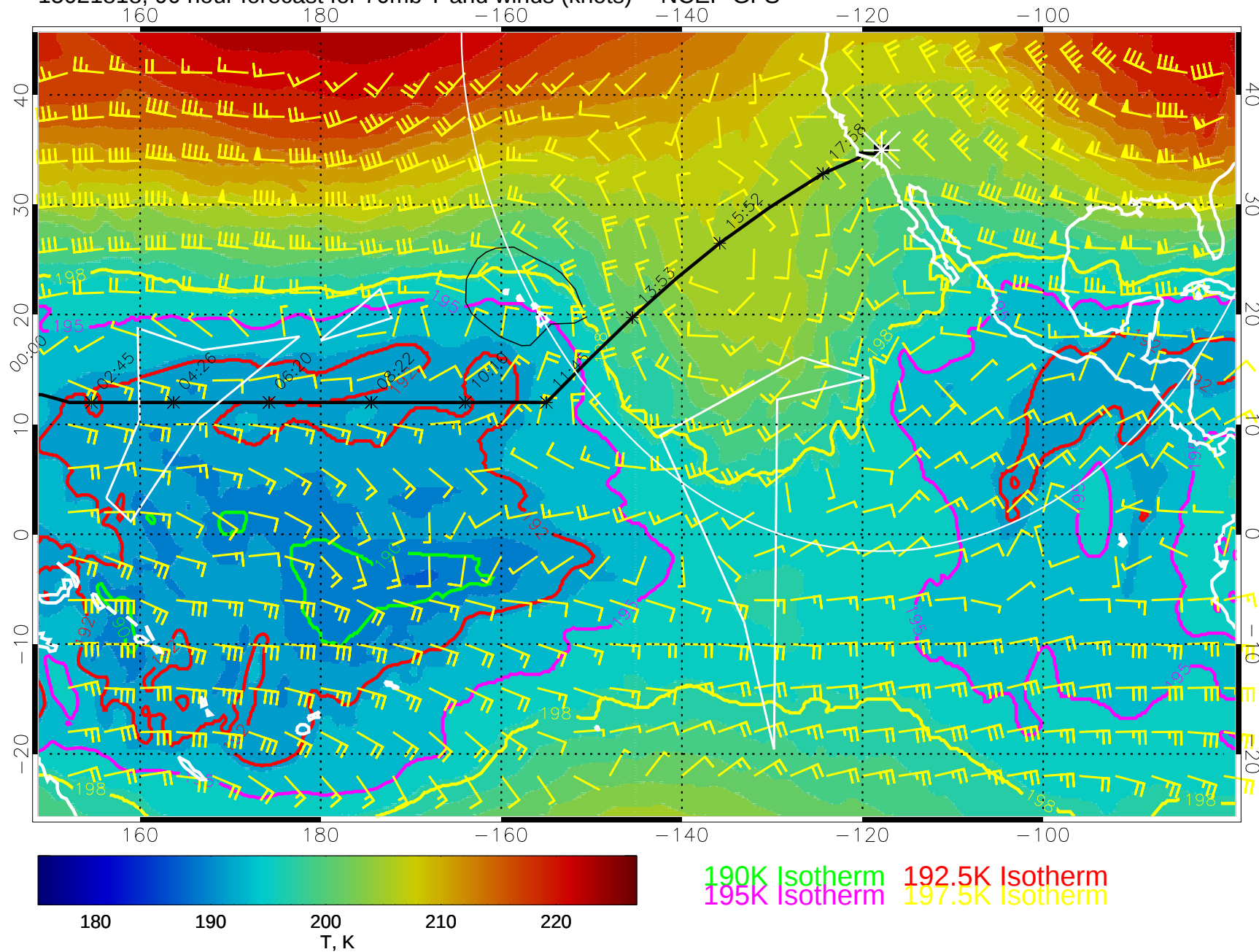
15021818, 90 hour forecast for 70mb T and winds (knots) -- NCEP GFS
