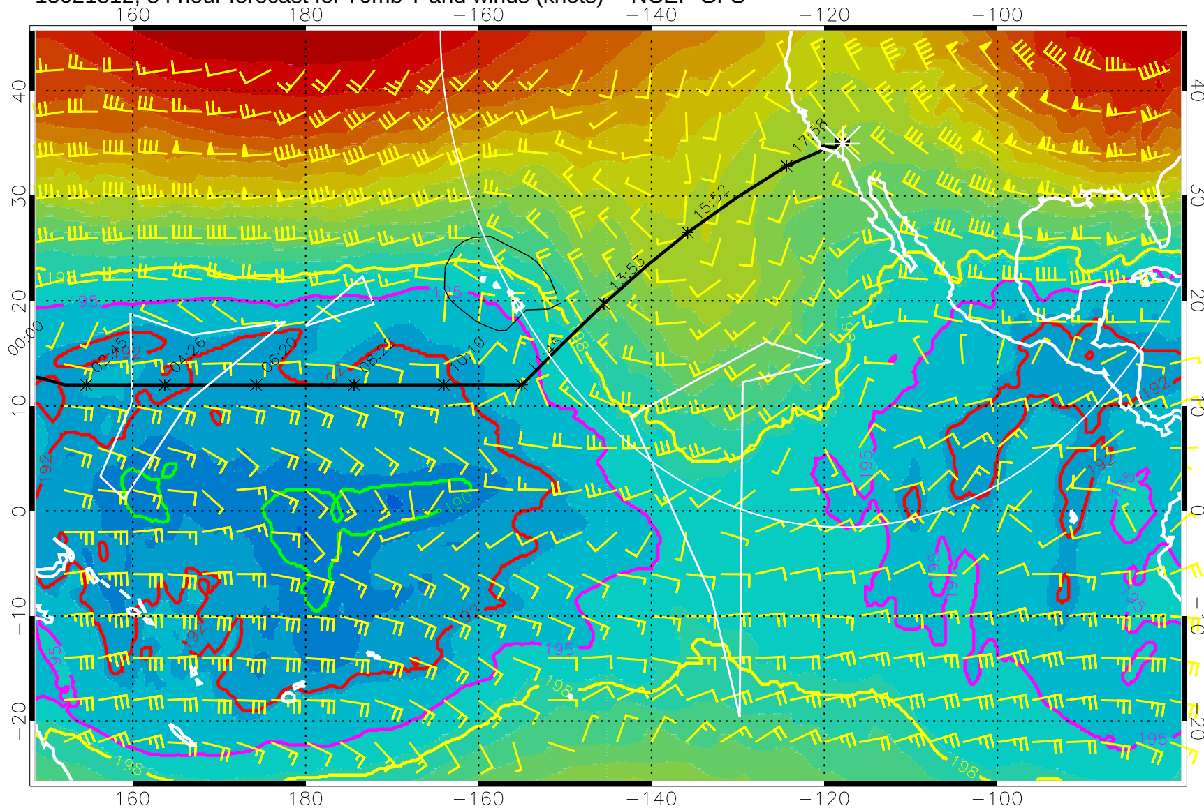
15021812, 84 hour forecast for 70mb T and winds (knots) -- NCEP GFS
