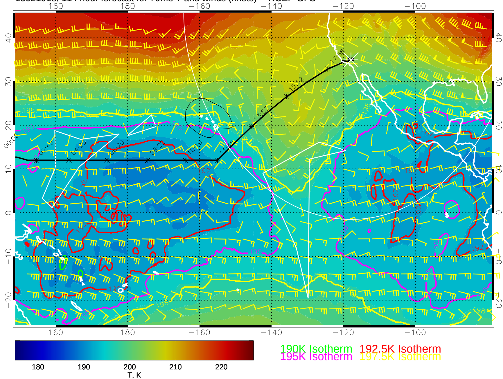
15021918, 114 hour forecast for 70mb T and winds (knots) -- NCEP GFS
