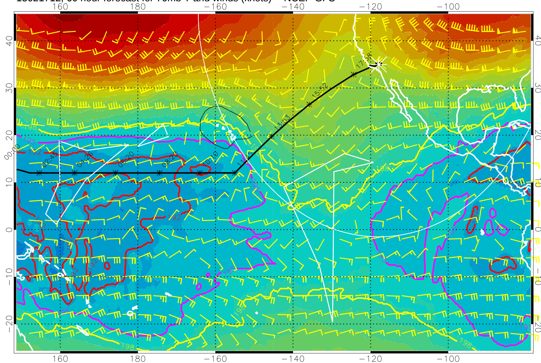
15021712, 60 hour forecast for 70mb T and winds (knots) -- NCEP GFS
