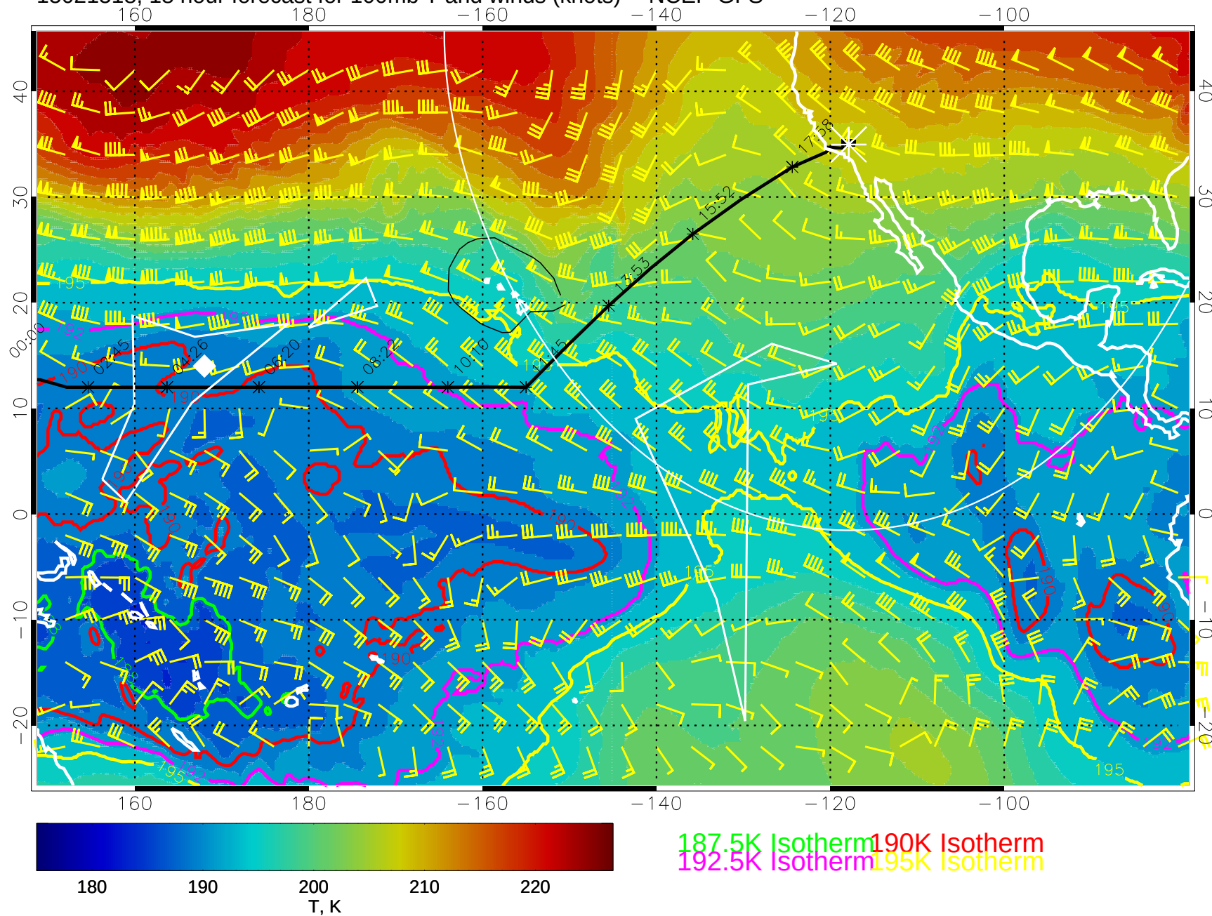
15021518, 18 hour forecast for 100mb T and winds (knots) -- NCEP GFS
