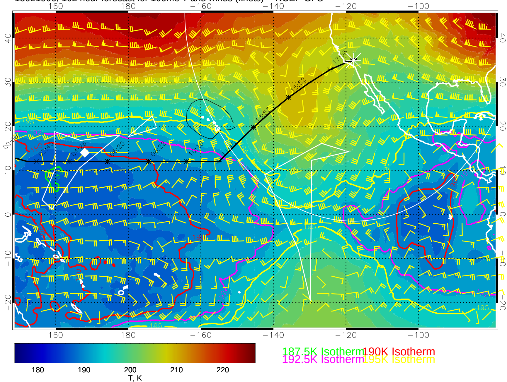
15021906, 102 hour forecast for 100mb T and winds (knots) -- NCEP GFS
