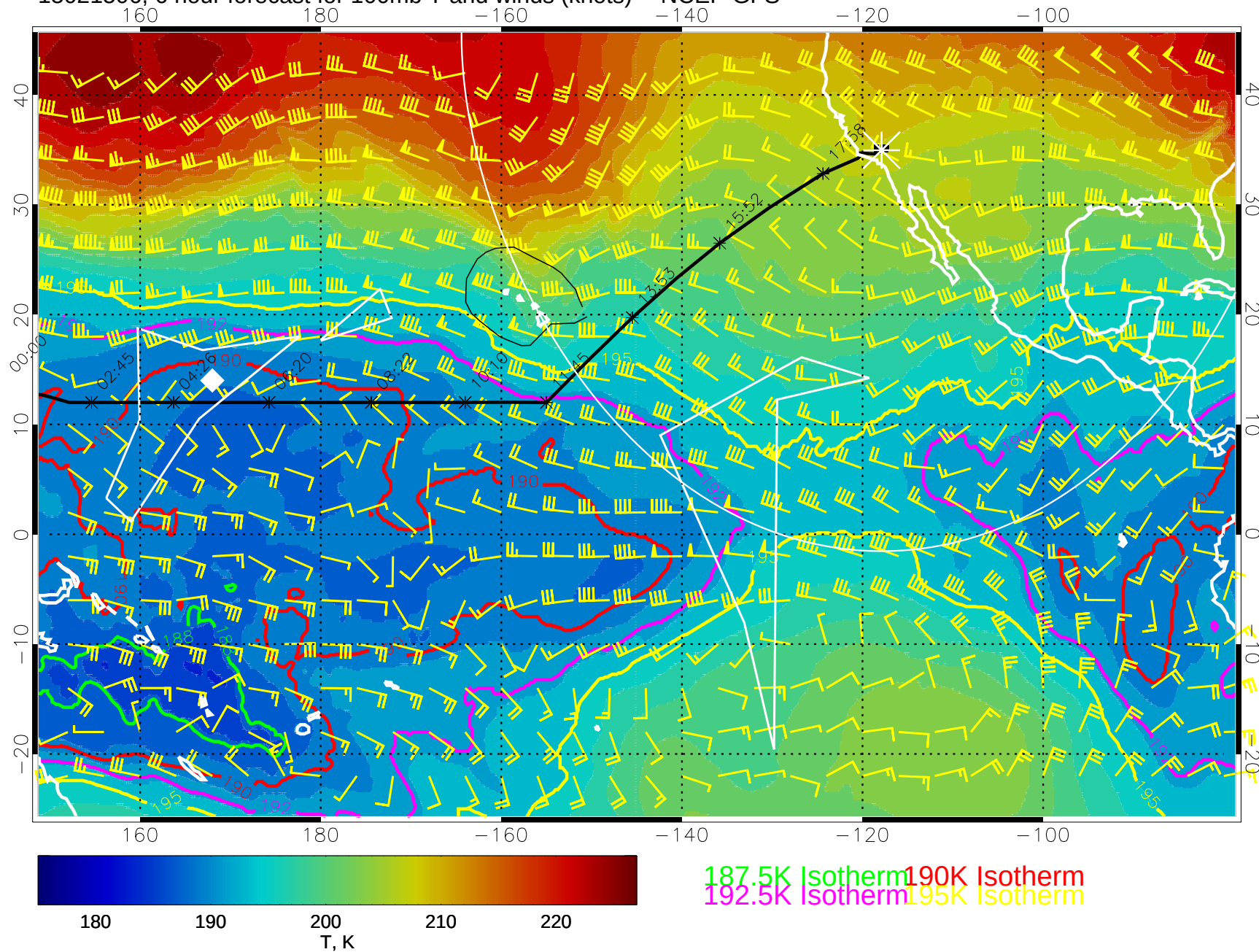
15021506, 6 hour forecast for 100mb T and winds (knots) -- NCEP GFS
