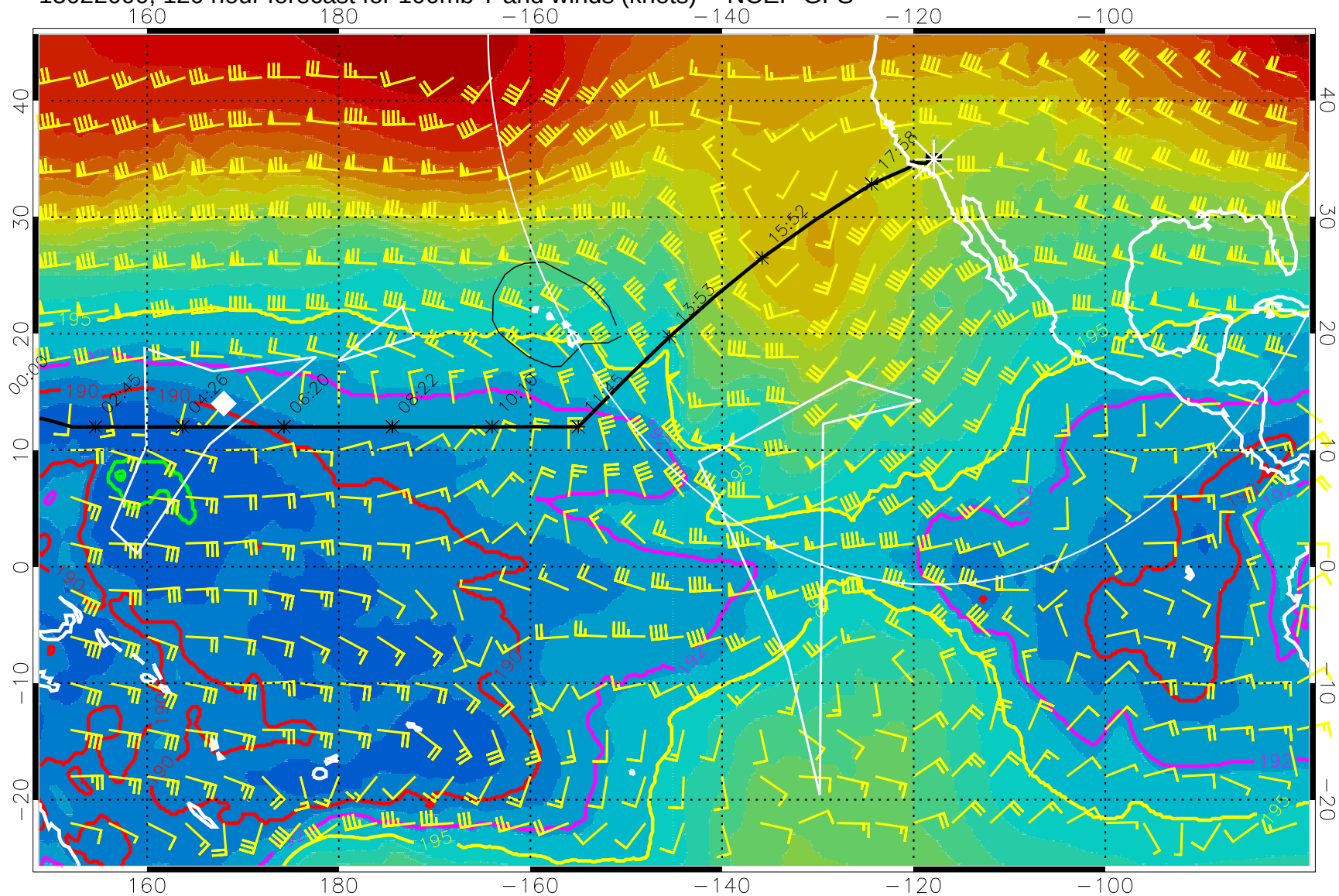
15022000, 120 hour forecast for 100mb T and winds (knots) -- NCEP GFS
