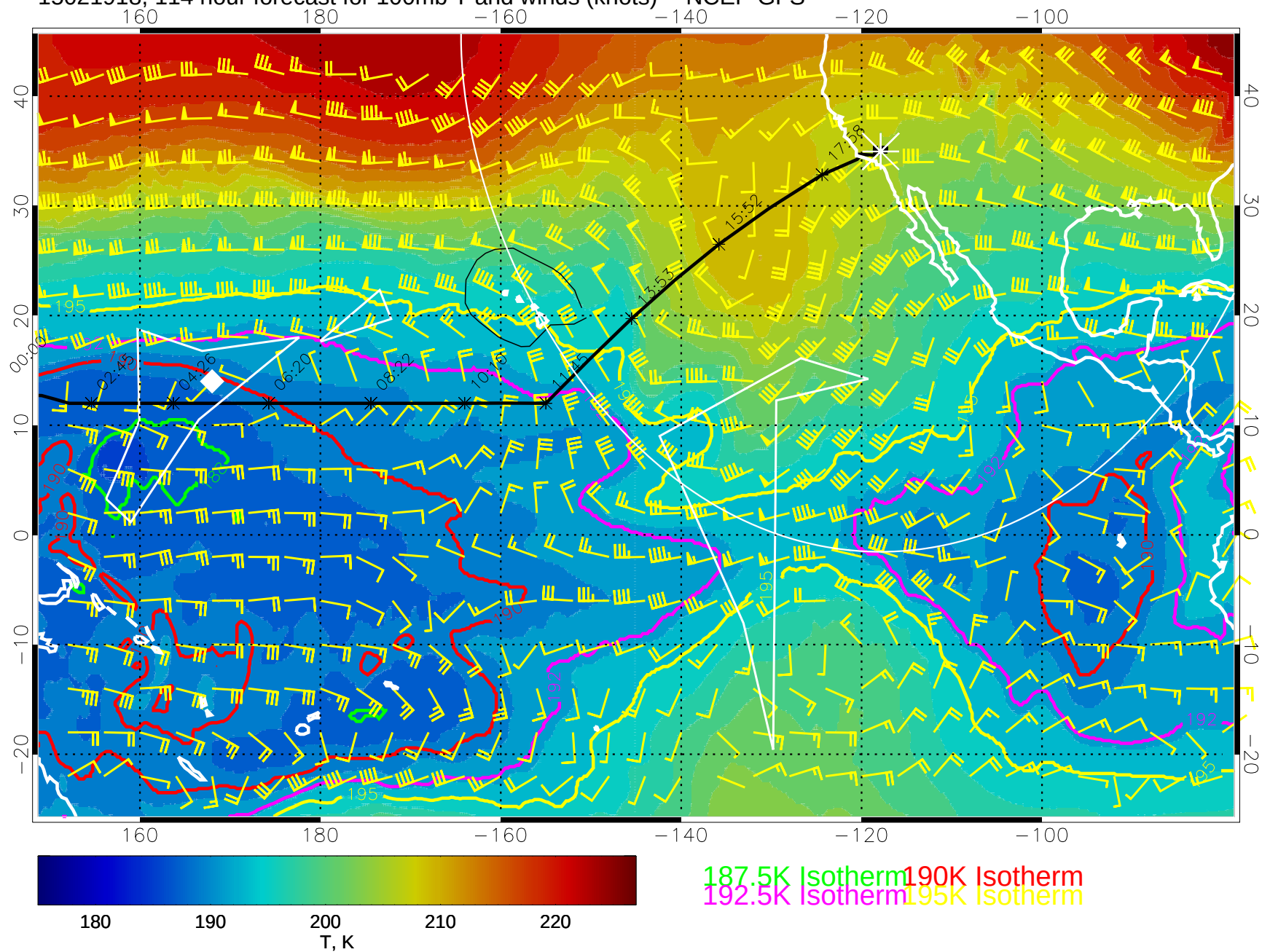
15021918, 114 hour forecast for 100mb T and winds (knots) -- NCEP GFS
