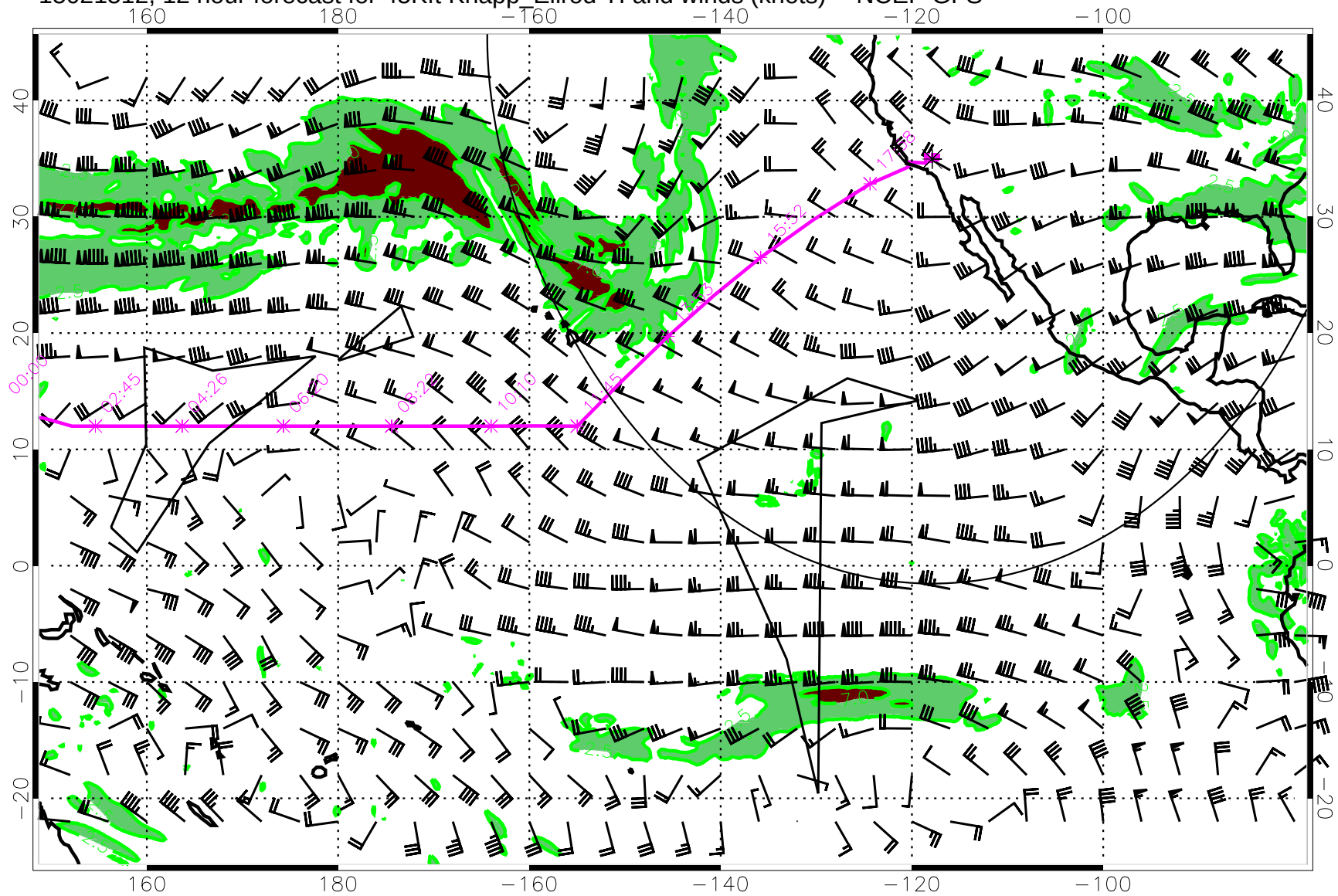
15021512, 12 hour forecast for 45Kft Knapp_Ellrod TI and winds (knots) -- NCEP GFS
