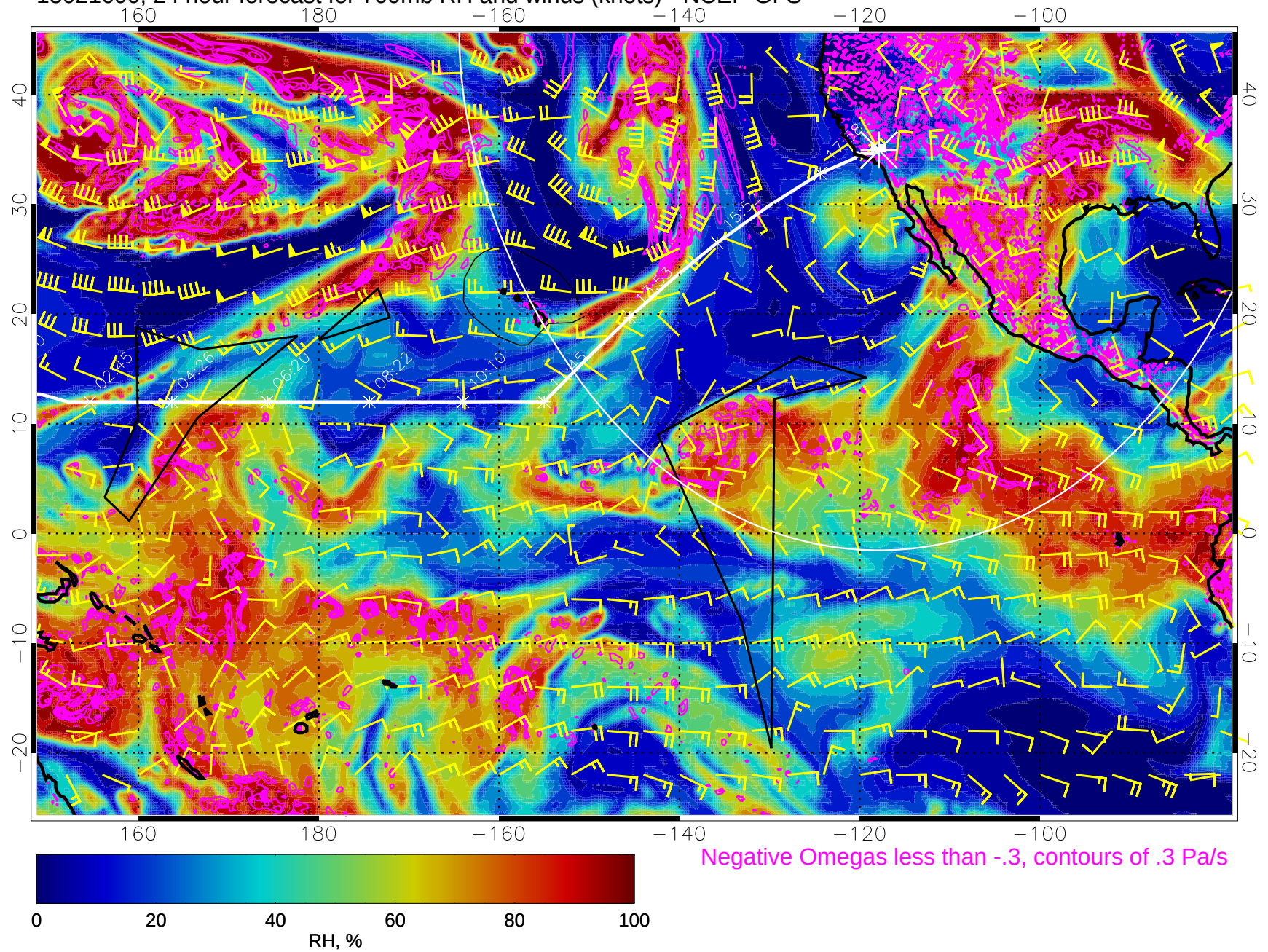
15021600, 24 hour forecast for 700mb RH and winds (knots) - NCEP GFS
