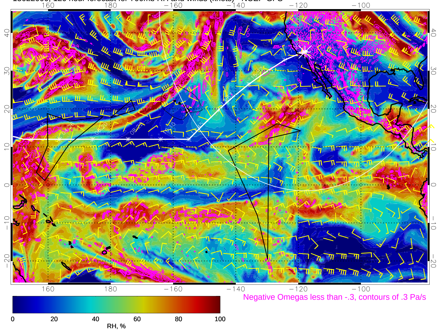
15022000, 120 hour forecast for 700mb RH and winds (knots) - NCEP GFS
