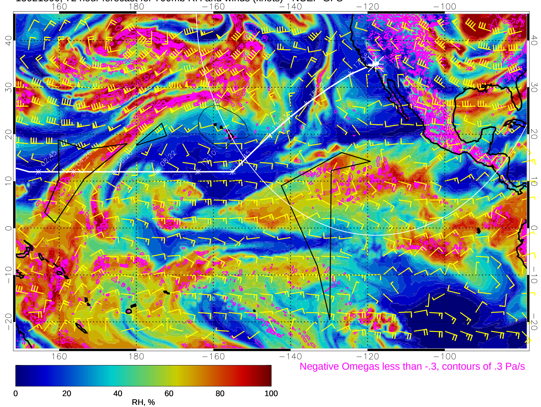
15021800, 72 hour forecast for 700mb RH and winds (knots) - NCEP GFS
