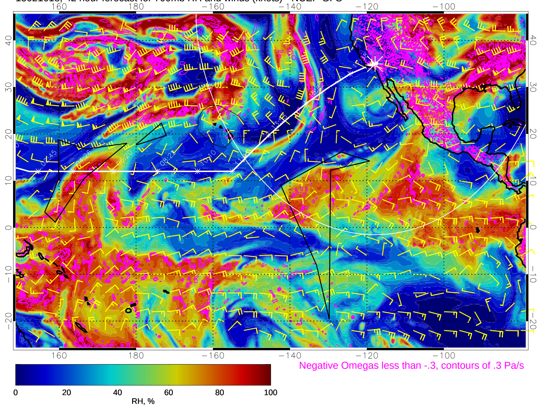
15021618, 42 hour forecast for 700mb RH and winds (knots) - NCEP GFS
