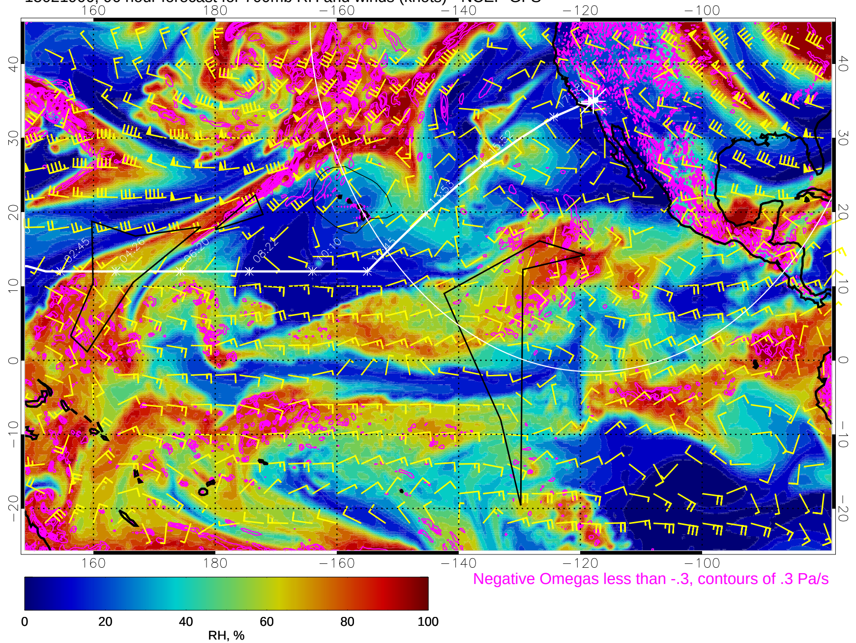
15021900, 96 hour forecast for 700mb RH and winds (knots) - NCEP GFS
