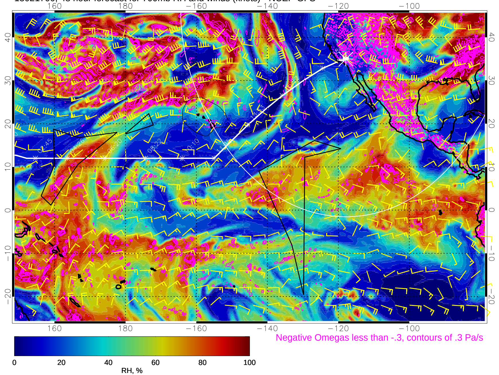
15021700, 48 hour forecast for 700mb RH and winds (knots) - NCEP GFS
