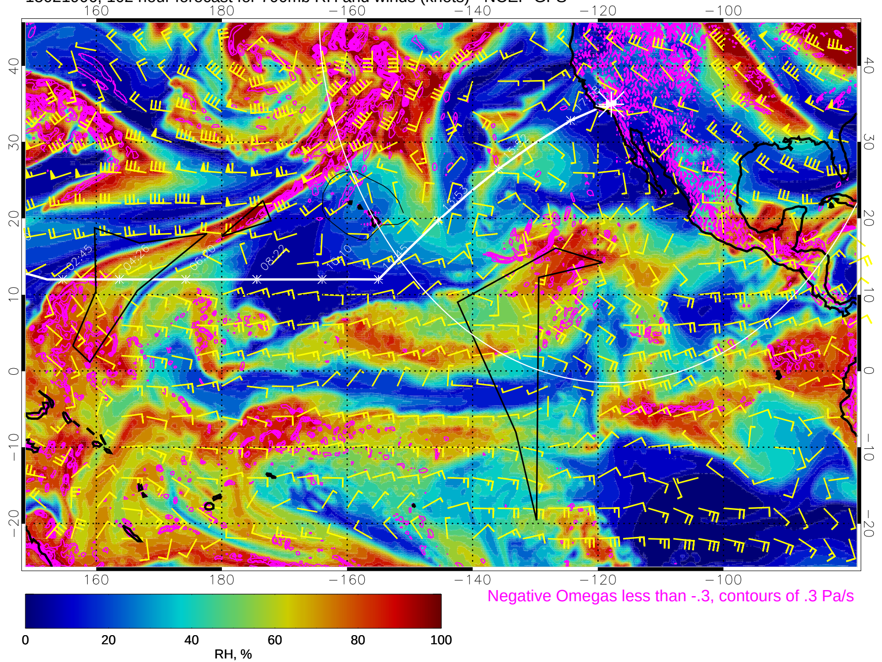
15021906, 102 hour forecast for 700mb RH and winds (knots) - NCEP GFS
