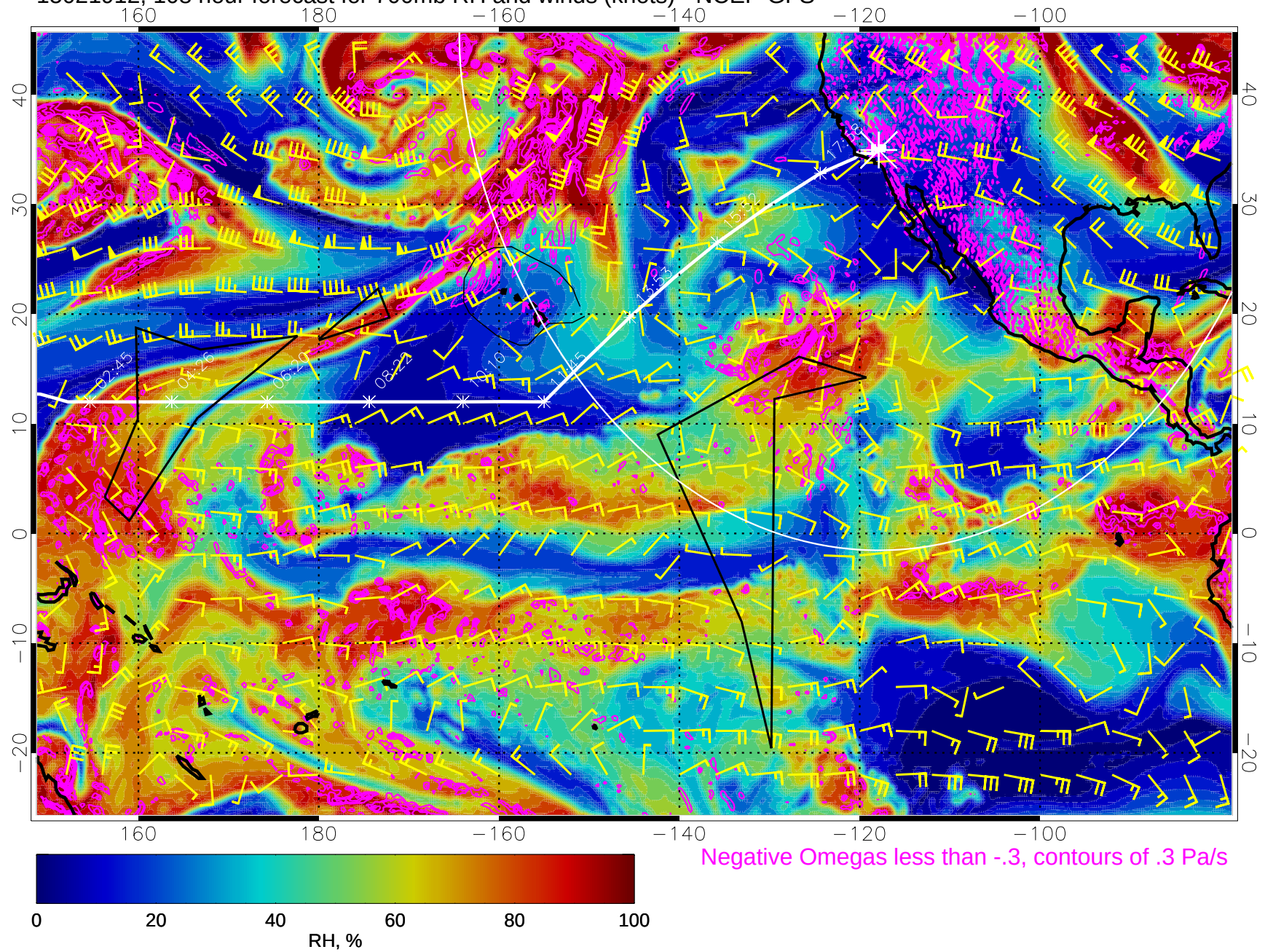
15021912, 108 hour forecast for 700mb RH and winds (knots) - NCEP GFS
