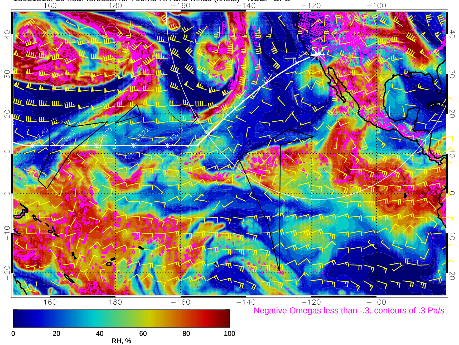
15021518, 18 hour forecast for 700mb RH and winds (knots) - NCEP GFS
