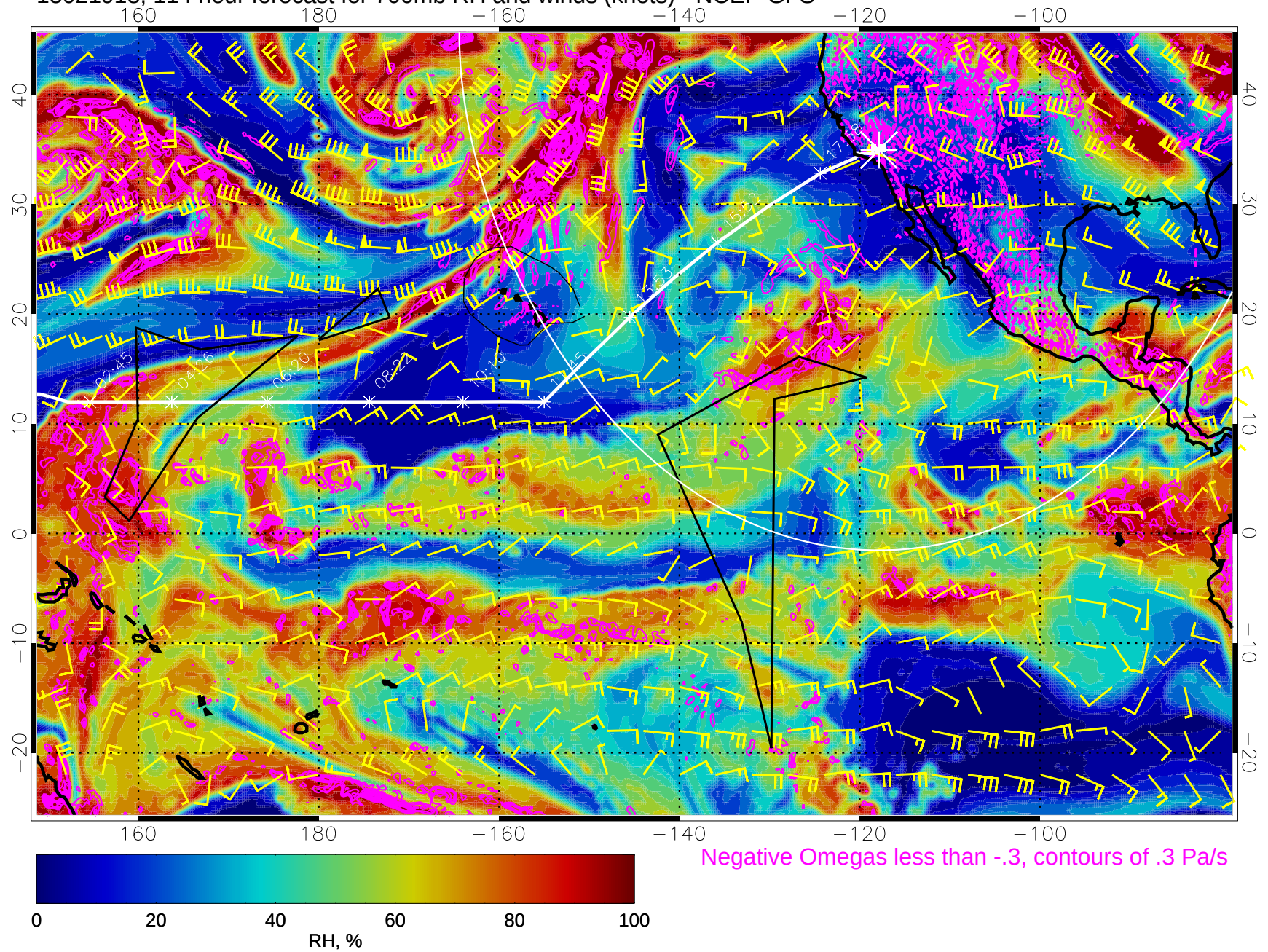
15021918, 114 hour forecast for 700mb RH and winds (knots) - NCEP GFS
