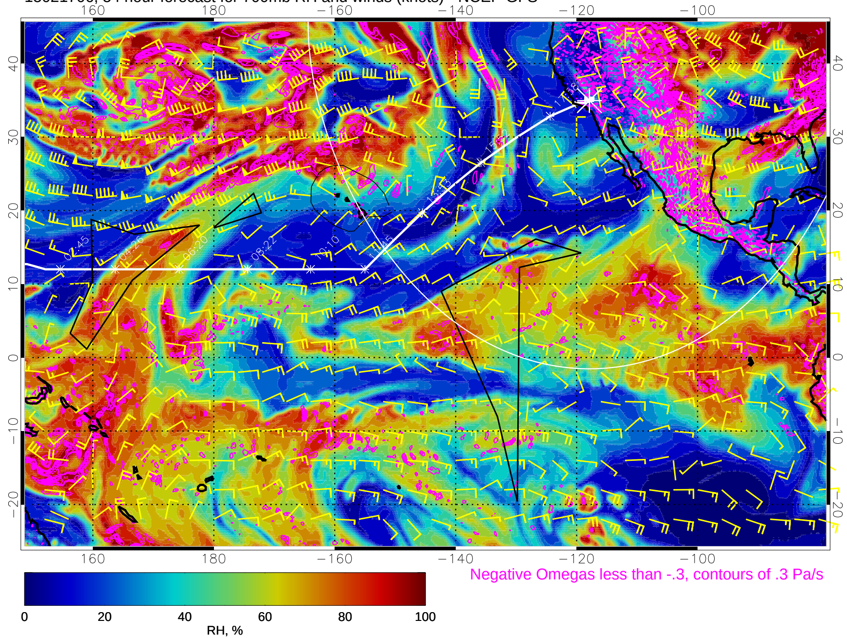
15021706, 54 hour forecast for 700mb RH and winds (knots) - NCEP GFS
