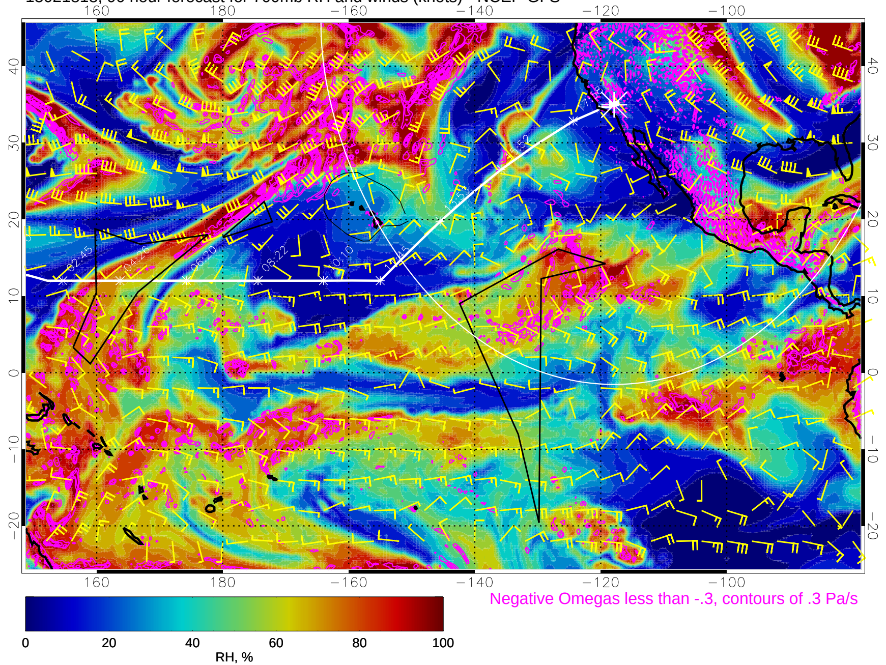
15021818, 90 hour forecast for 700mb RH and winds (knots) - NCEP GFS
