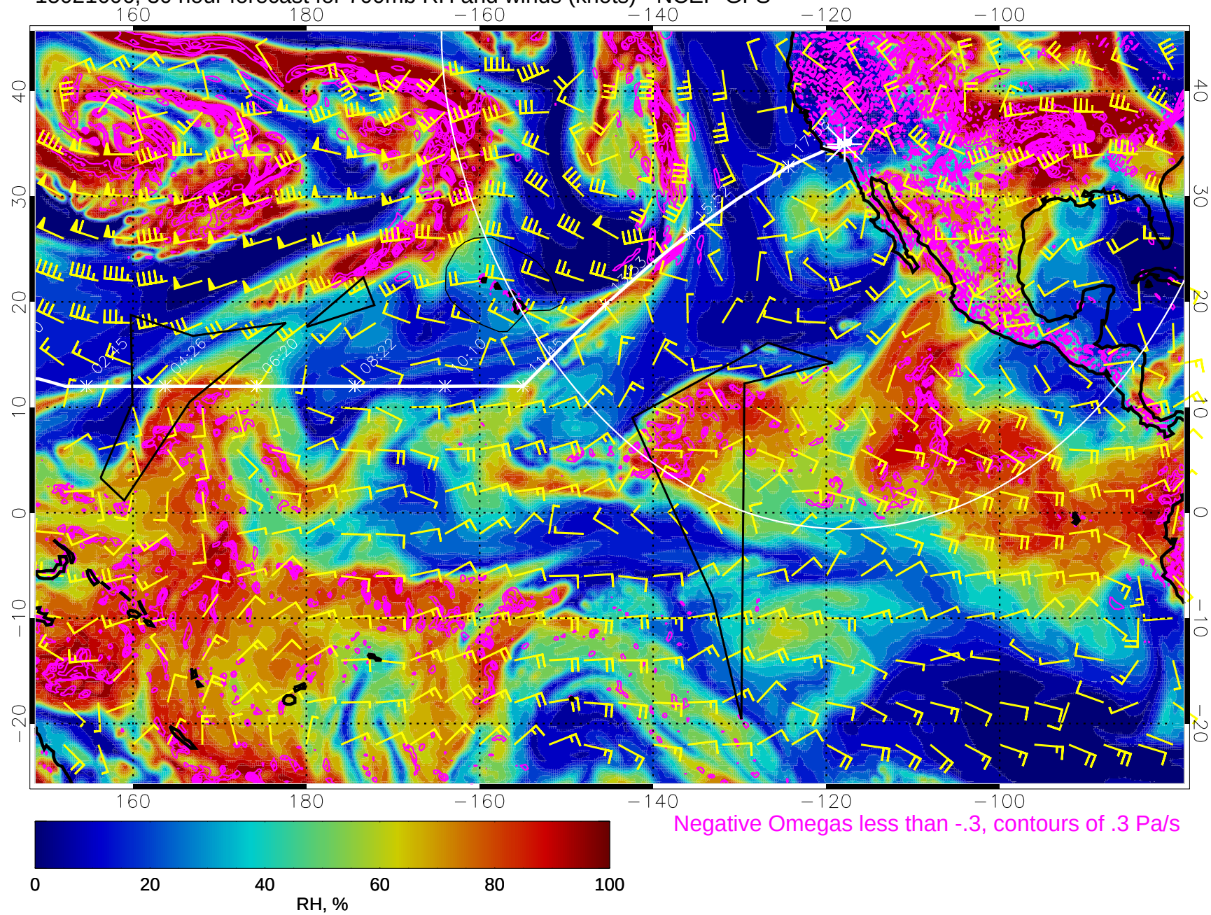
15021606, 30 hour forecast for 700mb RH and winds (knots) - NCEP GFS
