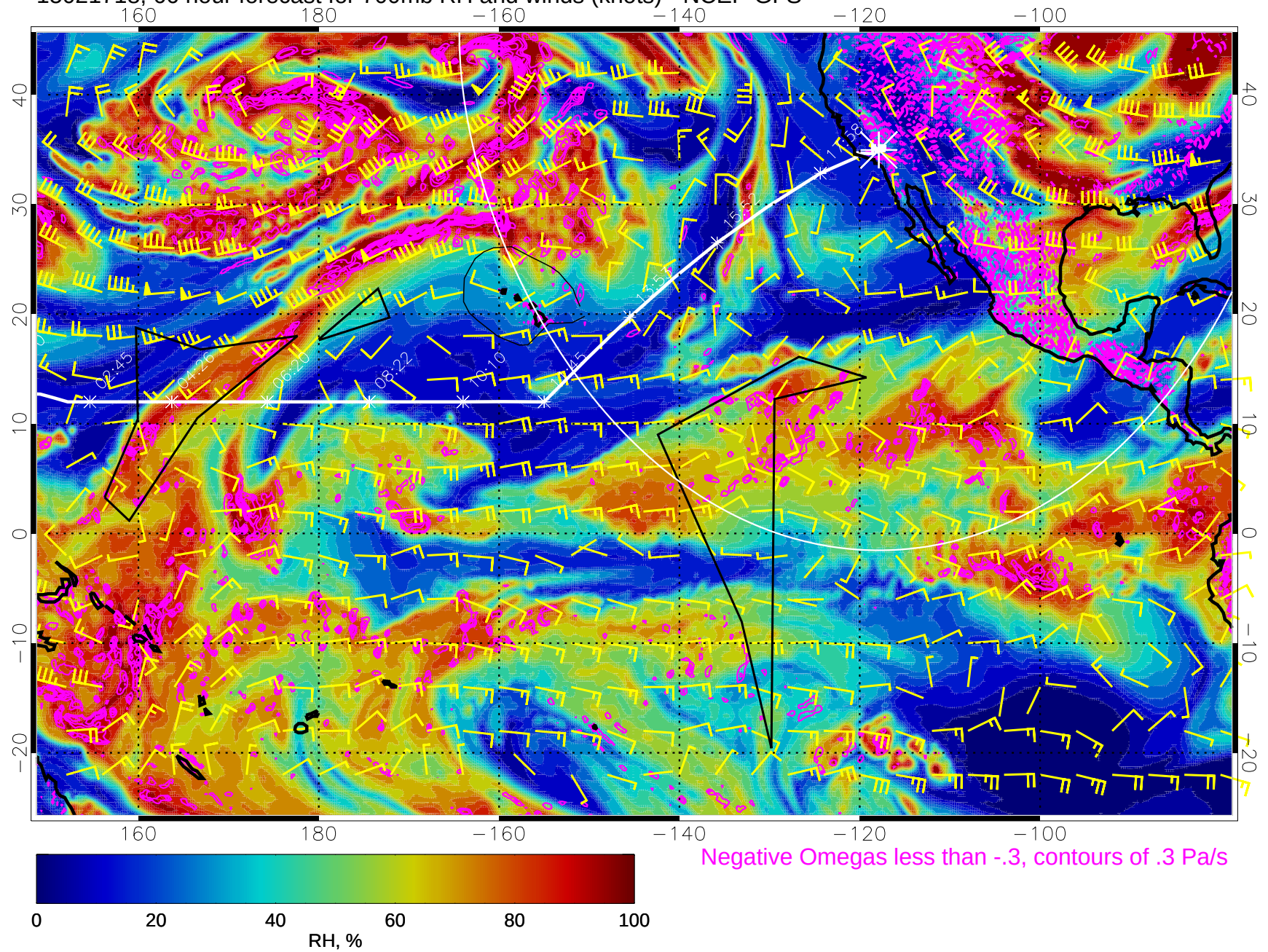
15021718, 66 hour forecast for 700mb RH and winds (knots) - NCEP GFS
