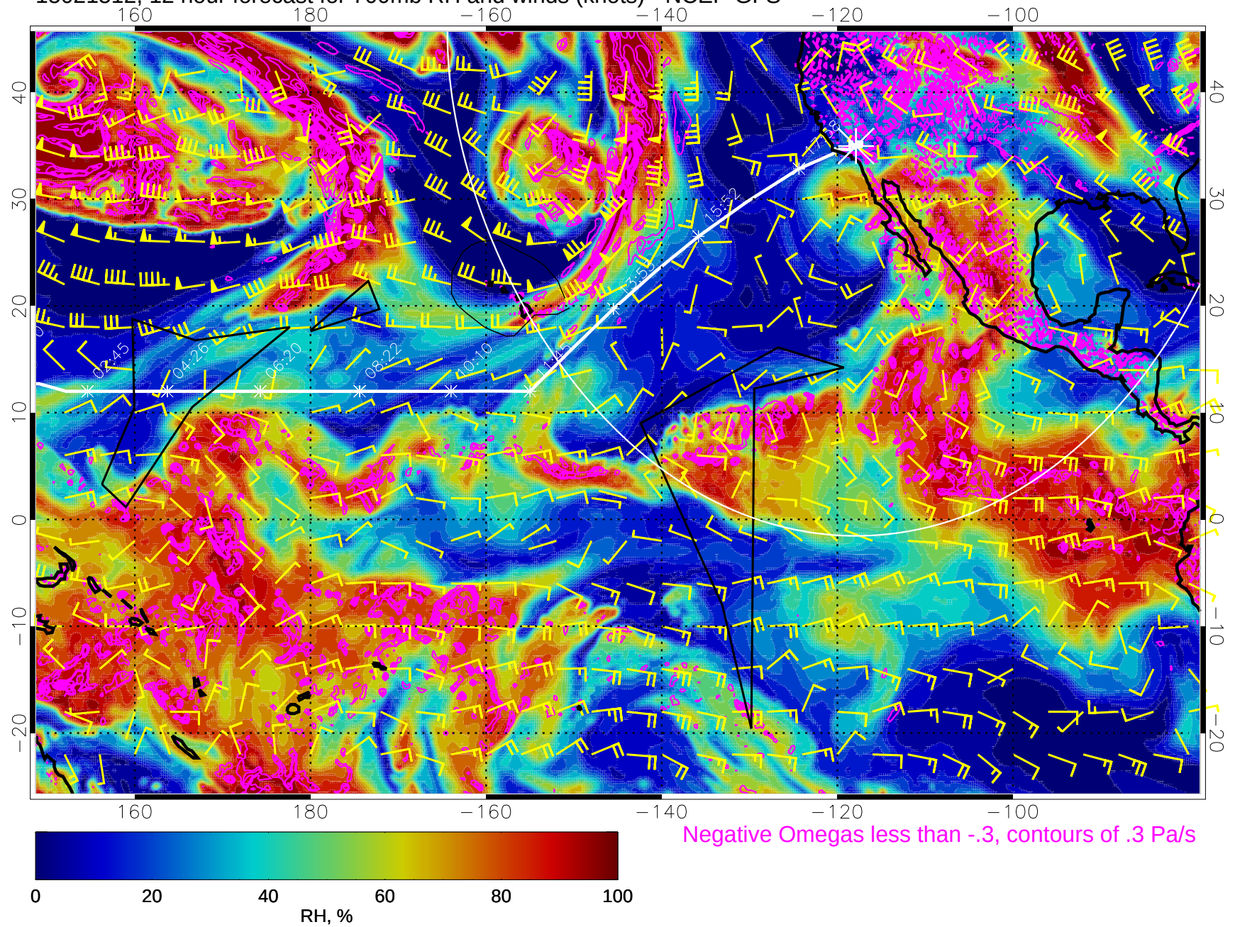
15021512, 12 hour forecast for 700mb RH and winds (knots) - NCEP GFS
