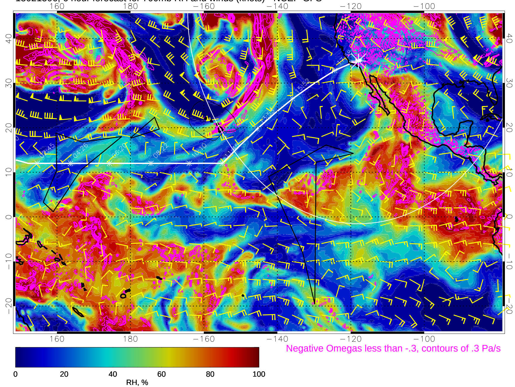
15021506, 6 hour forecast for 700mb RH and winds (knots) - NCEP GFS
