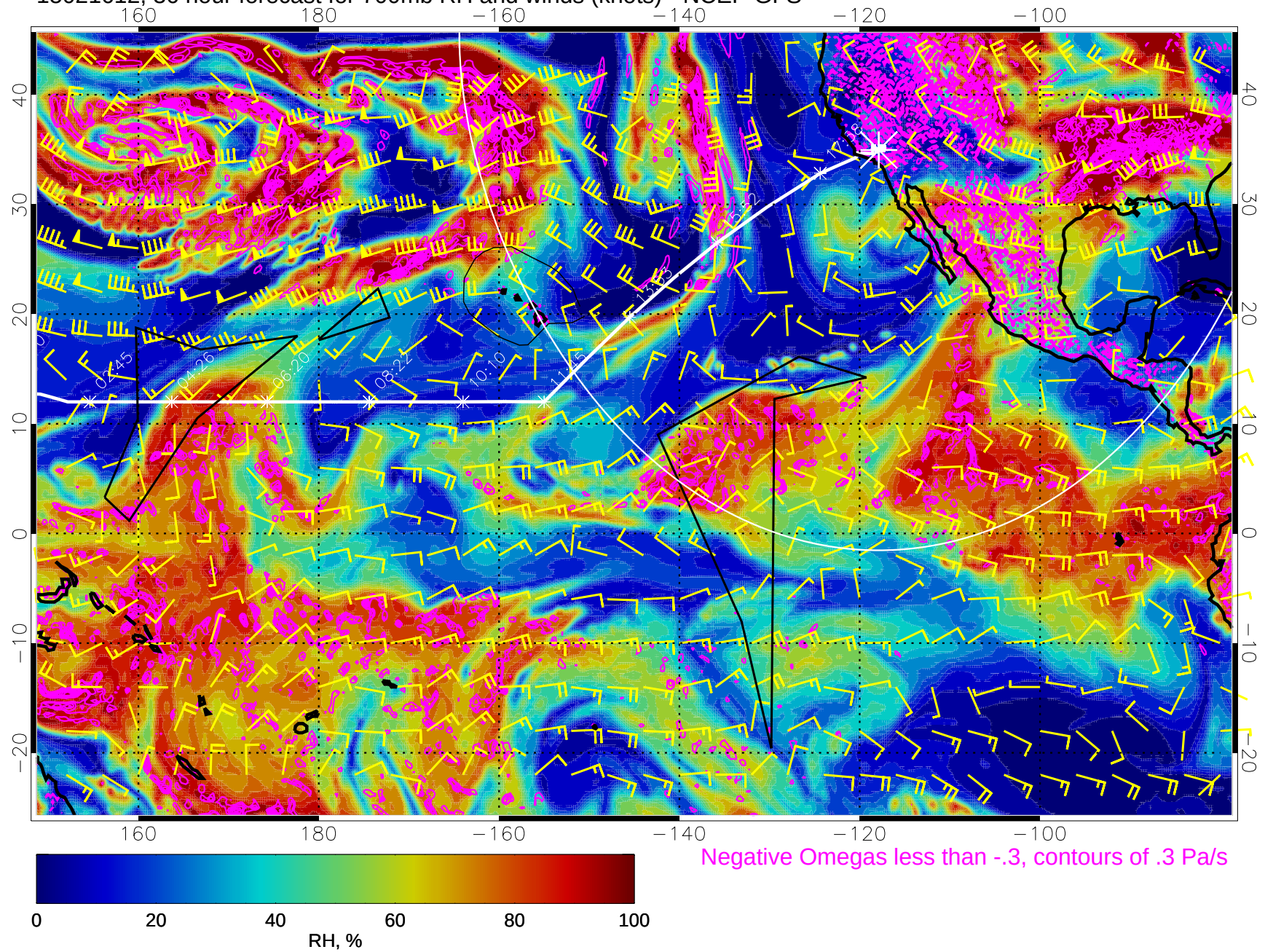
15021612, 36 hour forecast for 700mb RH and winds (knots) - NCEP GFS
