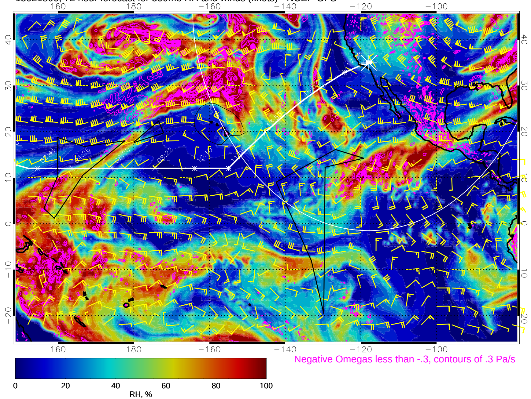
15021800, 72 hour forecast for 500mb RH and winds (knots) - NCEP GFS
