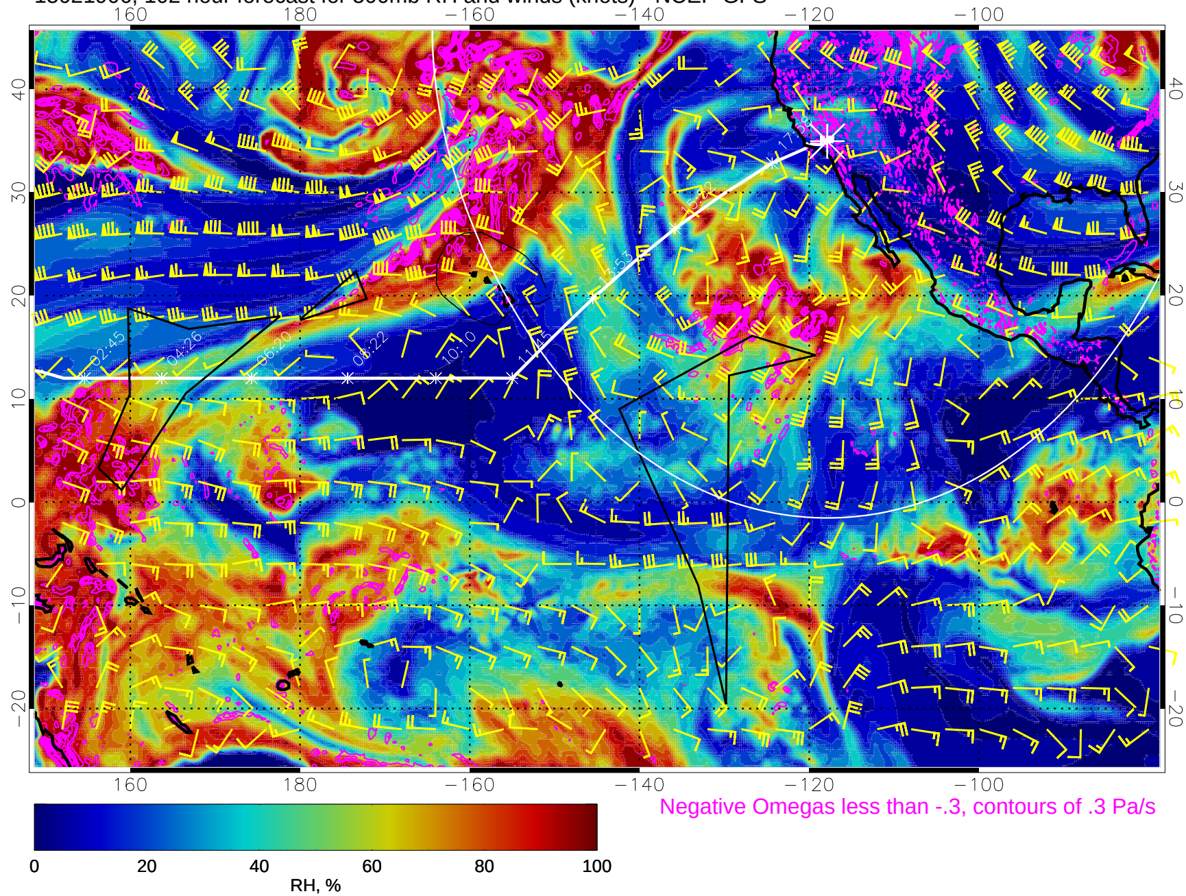
15021906, 102 hour forecast for 500mb RH and winds (knots) - NCEP GFS
