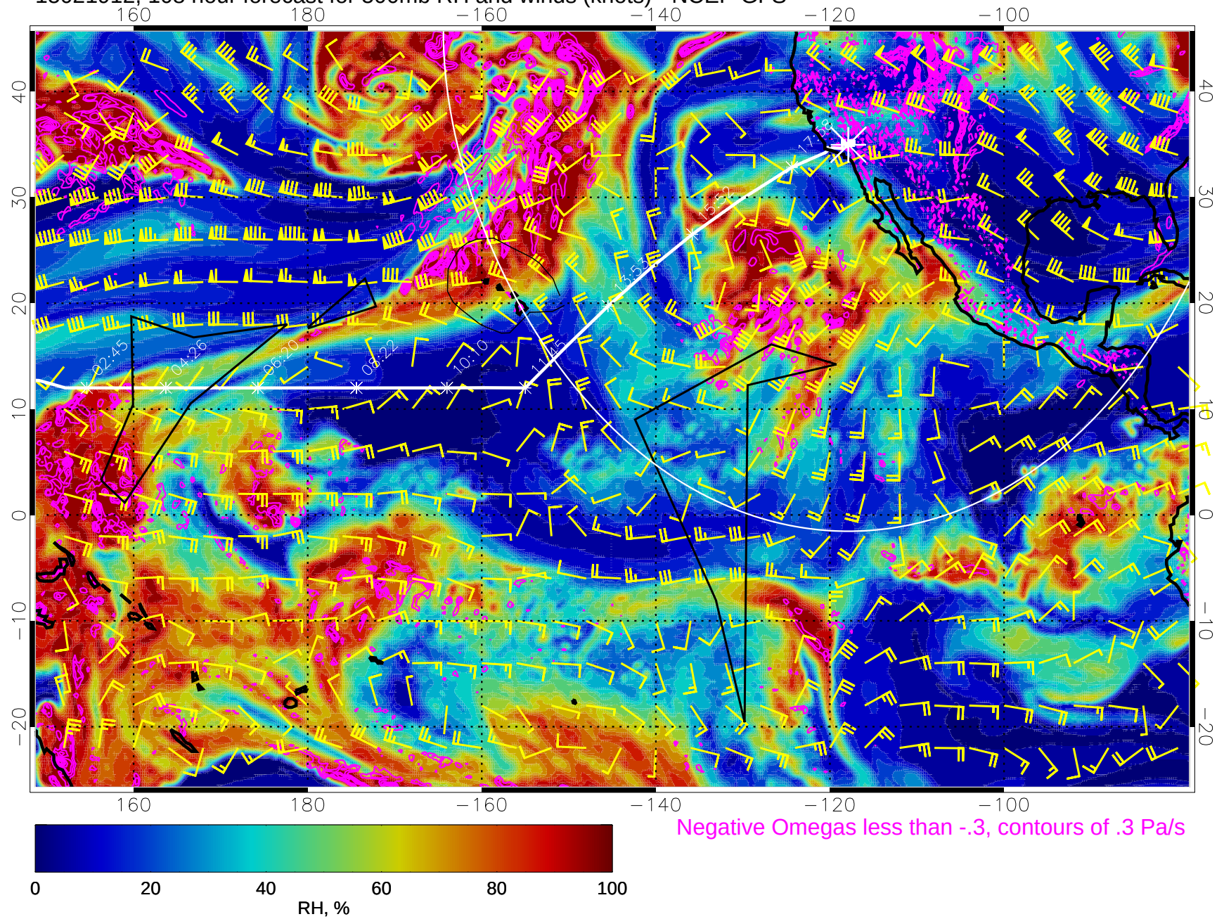
15021912, 108 hour forecast for 500mb RH and winds (knots) - NCEP GFS
