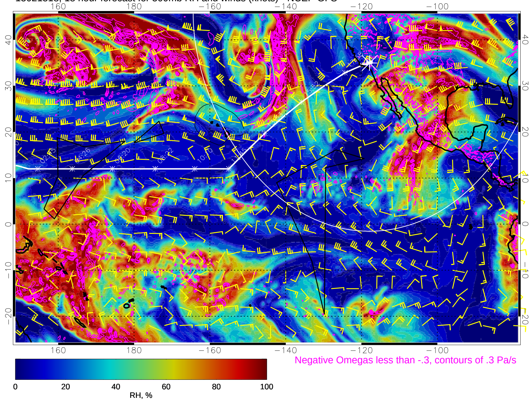
15021518, 18 hour forecast for 500mb RH and winds (knots) - NCEP GFS
