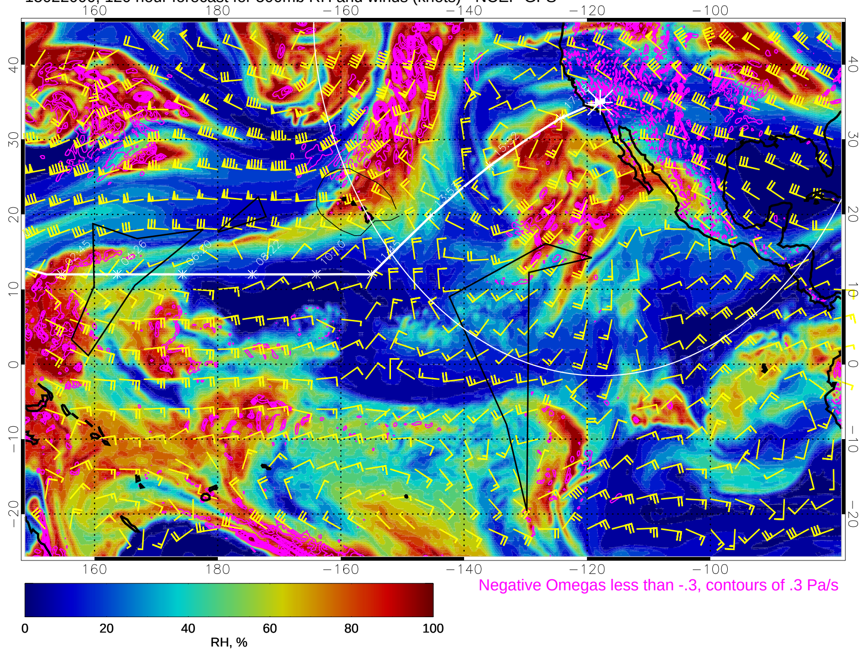
15022000, 120 hour forecast for 500mb RH and winds (knots) - NCEP GFS
