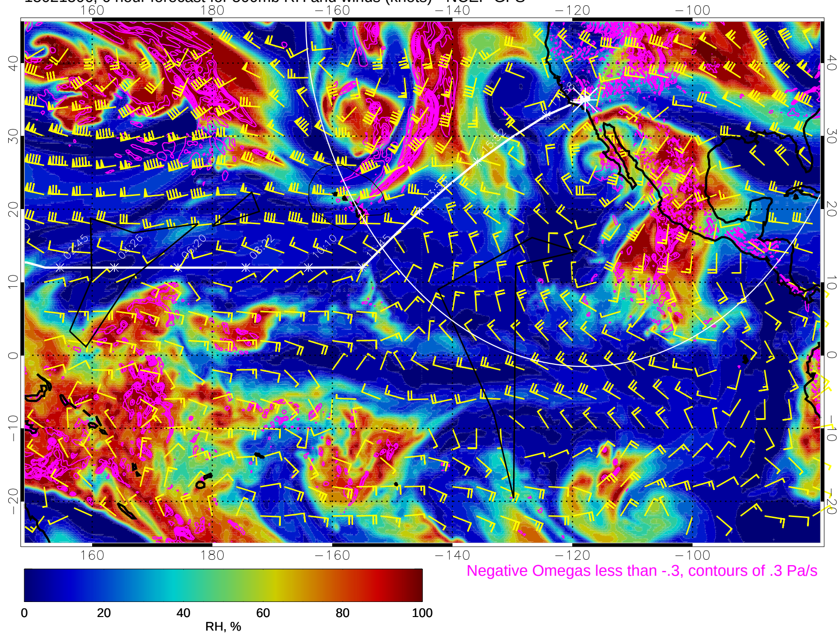
15021506, 6 hour forecast for 500mb RH and winds (knots) - NCEP GFS
