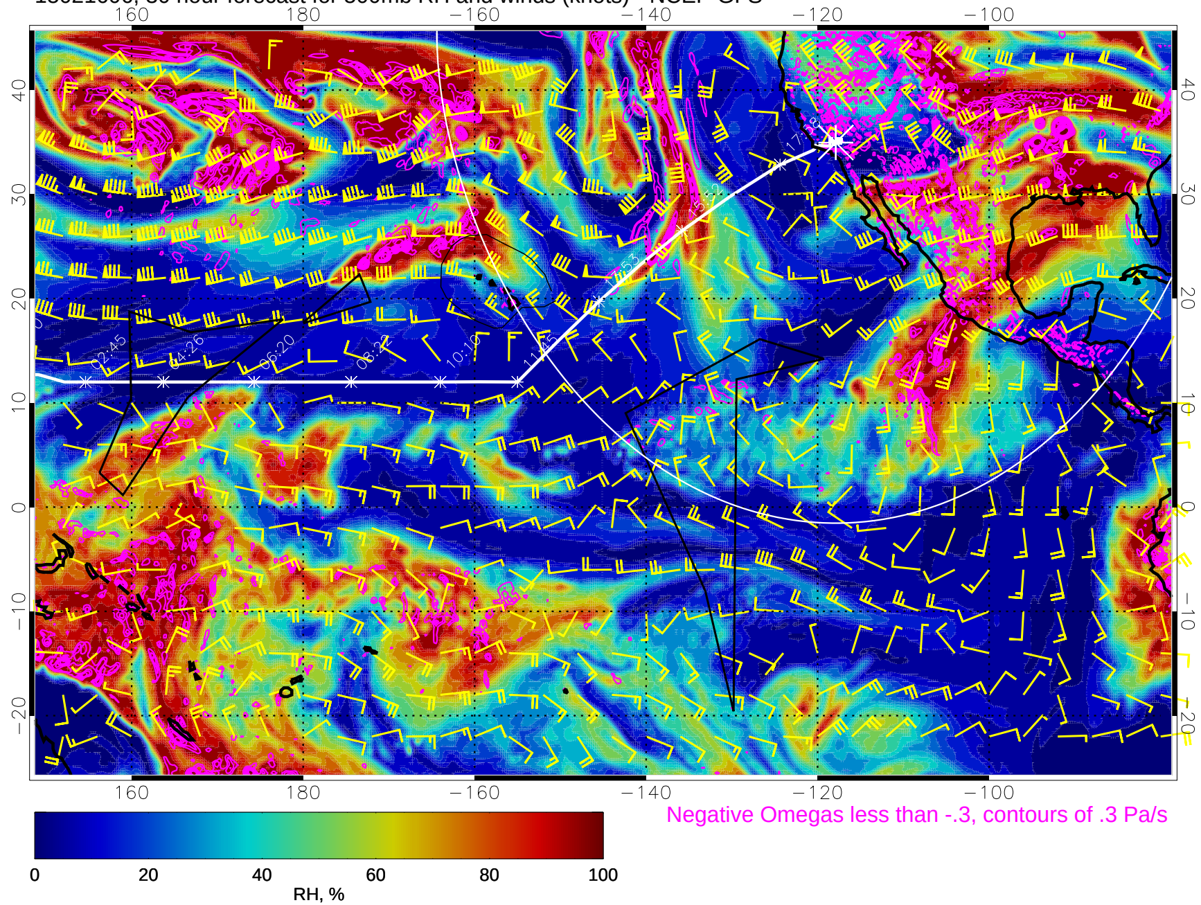
15021606, 30 hour forecast for 500mb RH and winds (knots) - NCEP GFS
