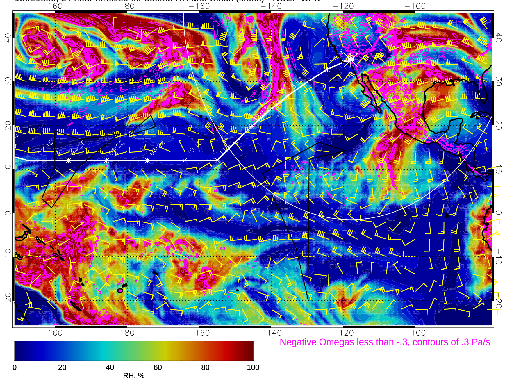
15021600, 24 hour forecast for 500mb RH and winds (knots) - NCEP GFS
