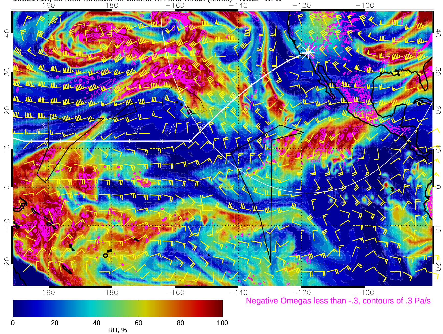
15021718, 66 hour forecast for 500mb RH and winds (knots) - NCEP GFS
