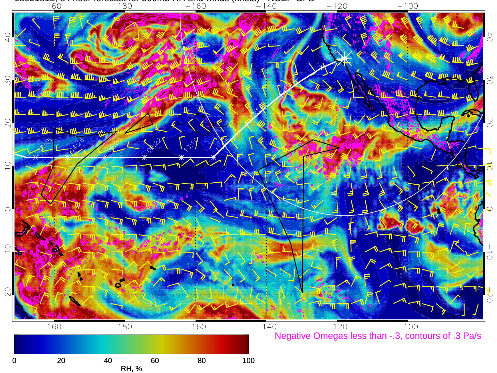
15021812, 84 hour forecast for 500mb RH and winds (knots) - NCEP GFS
