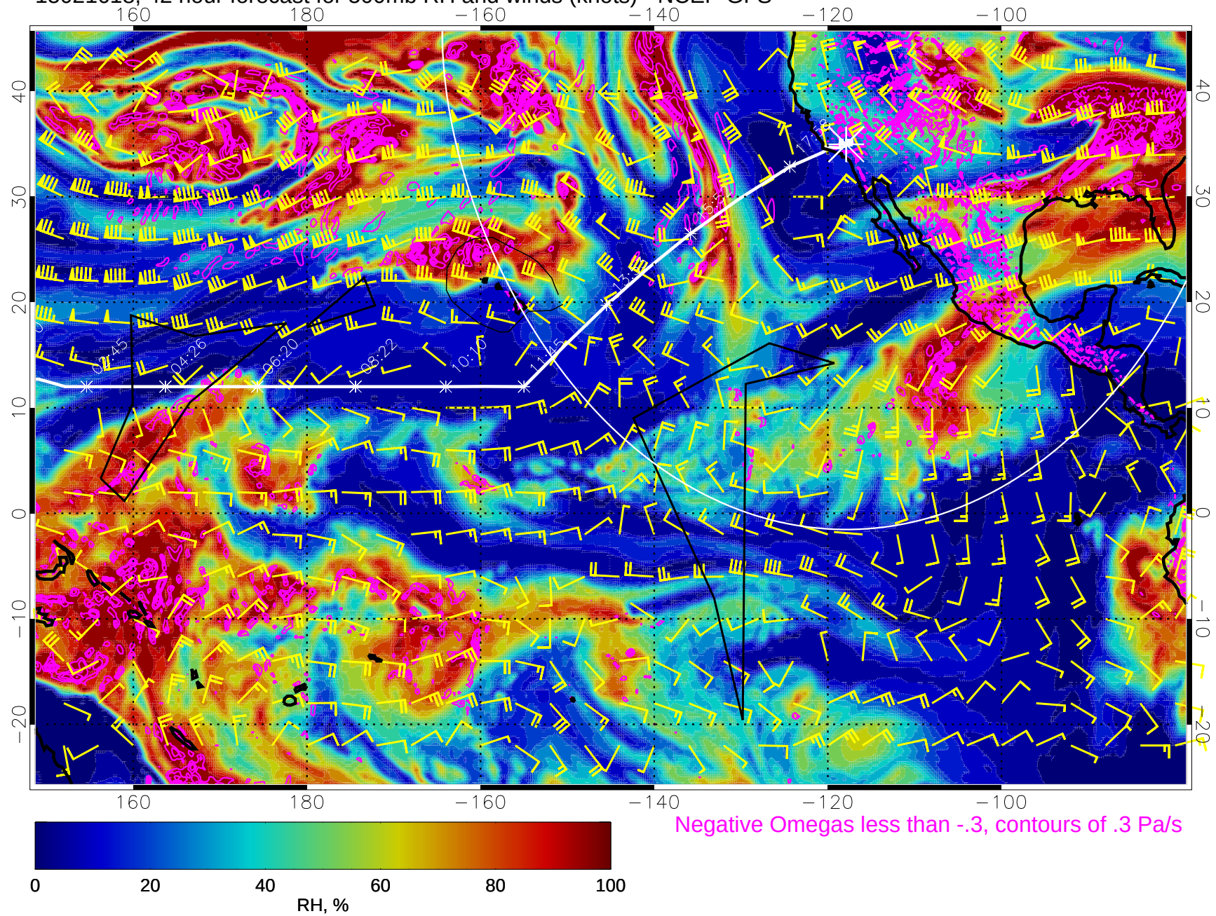
15021618, 42 hour forecast for 500mb RH and winds (knots) - NCEP GFS
