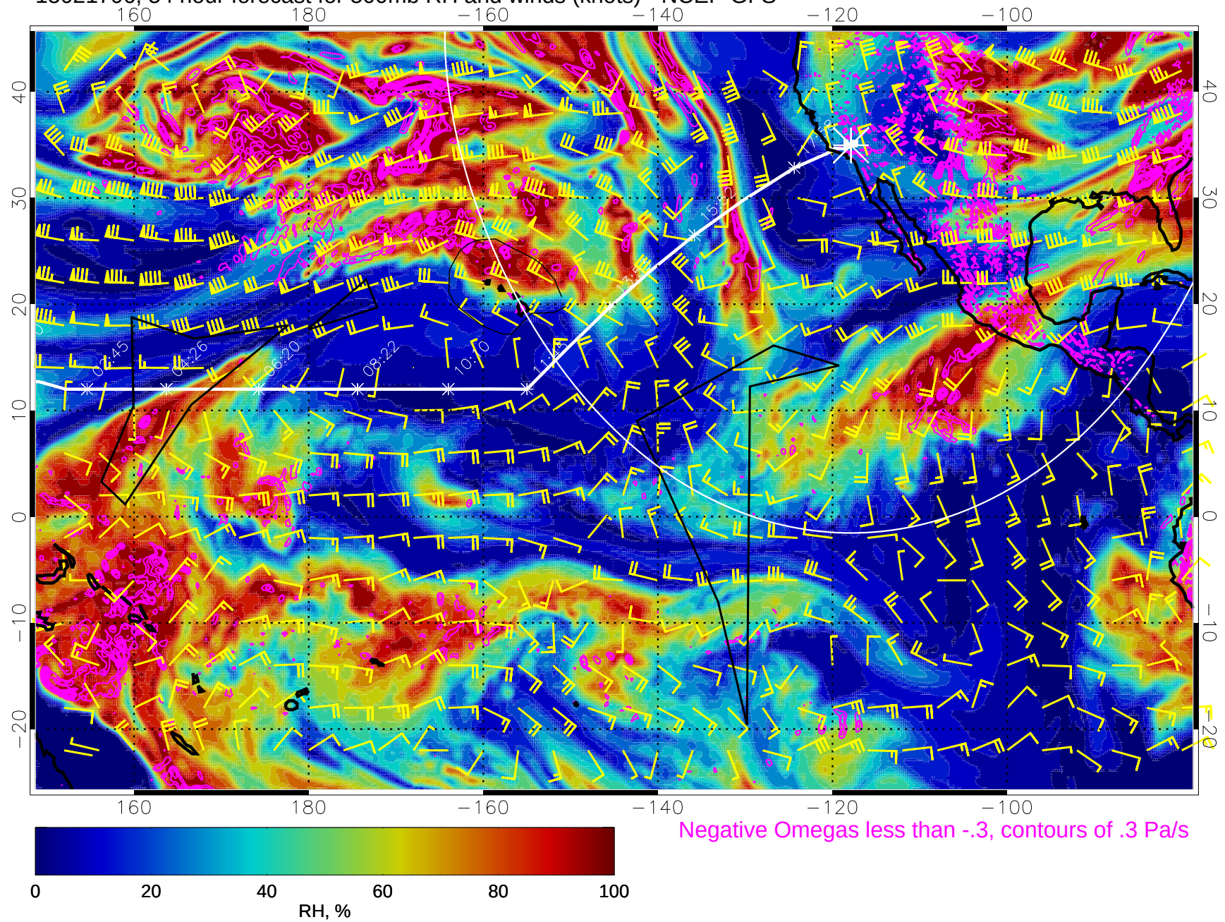
15021706, 54 hour forecast for 500mb RH and winds (knots) - NCEP GFS
