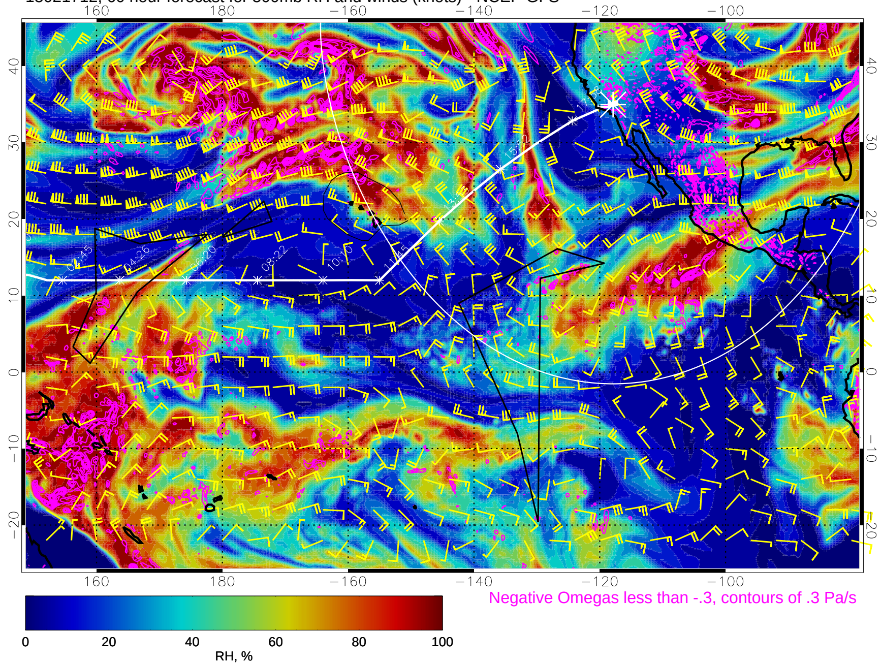
15021712, 60 hour forecast for 500mb RH and winds (knots) - NCEP GFS
