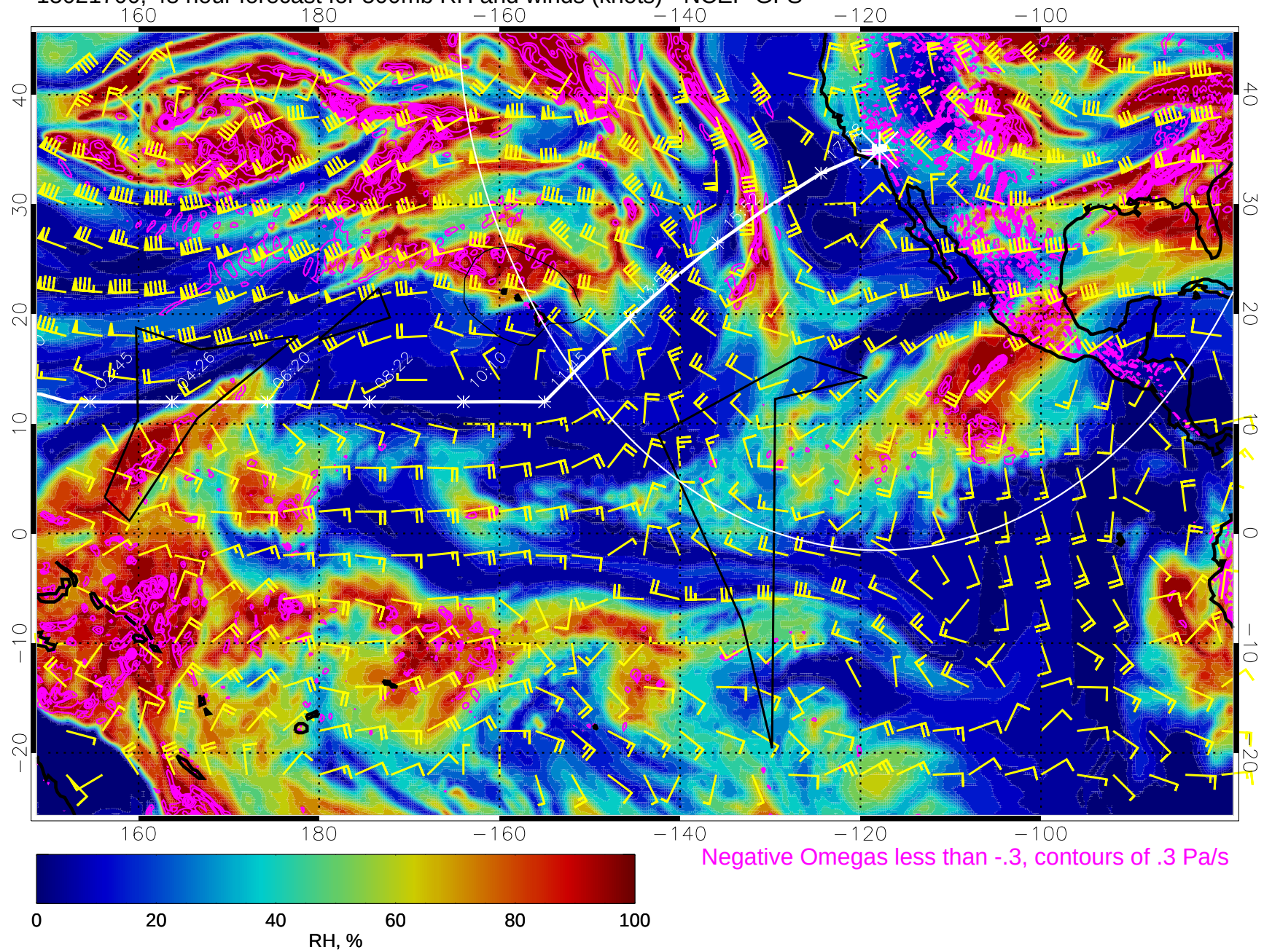
15021700, 48 hour forecast for 500mb RH and winds (knots) - NCEP GFS
