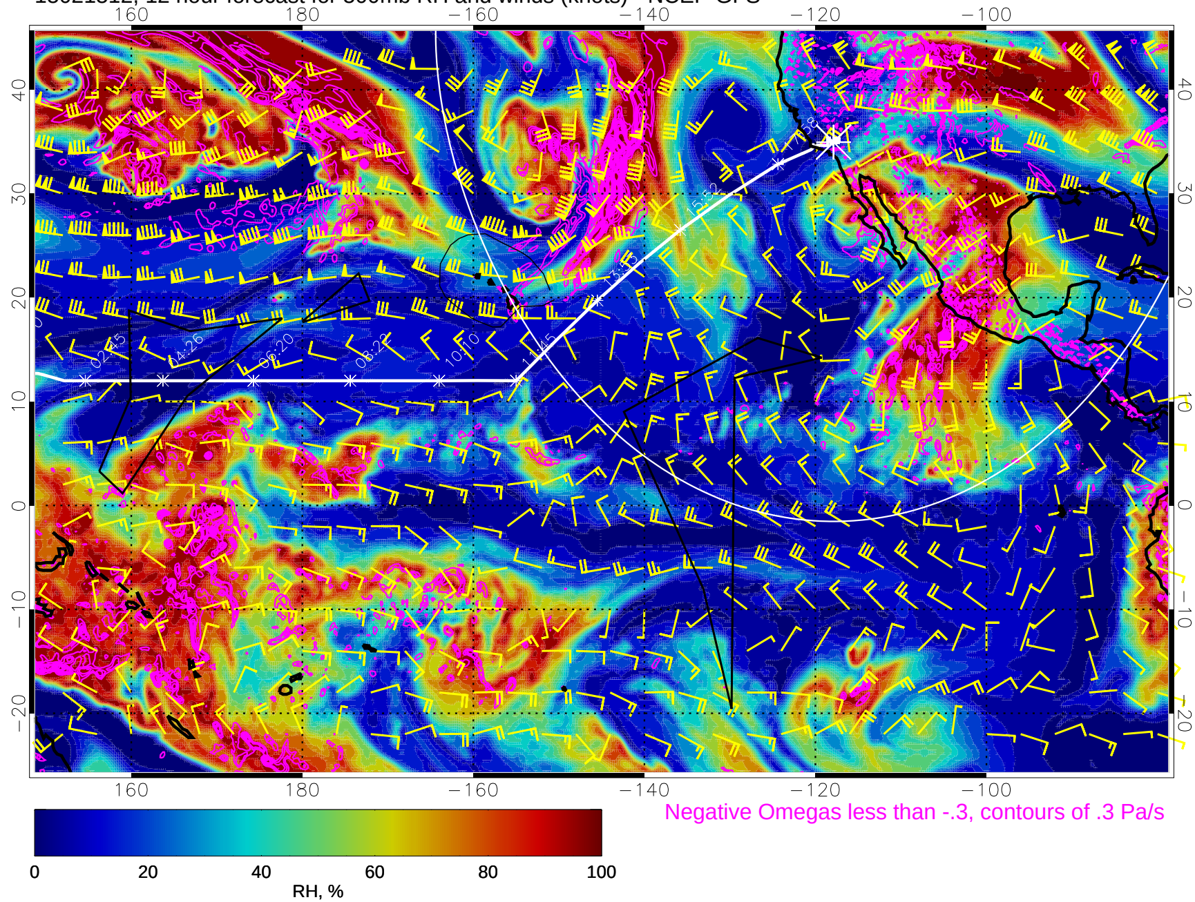
15021512, 12 hour forecast for 500mb RH and winds (knots) - NCEP GFS
