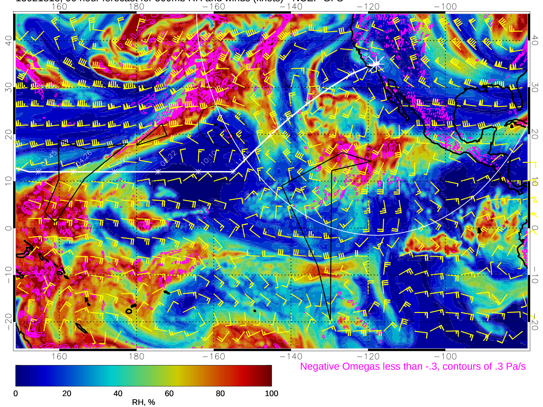
15021818, 90 hour forecast for 500mb RH and winds (knots) - NCEP GFS
