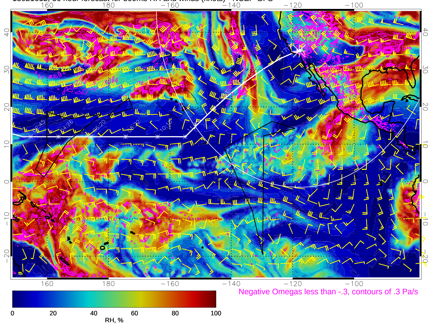
15021612, 36 hour forecast for 500mb RH and winds (knots) - NCEP GFS
