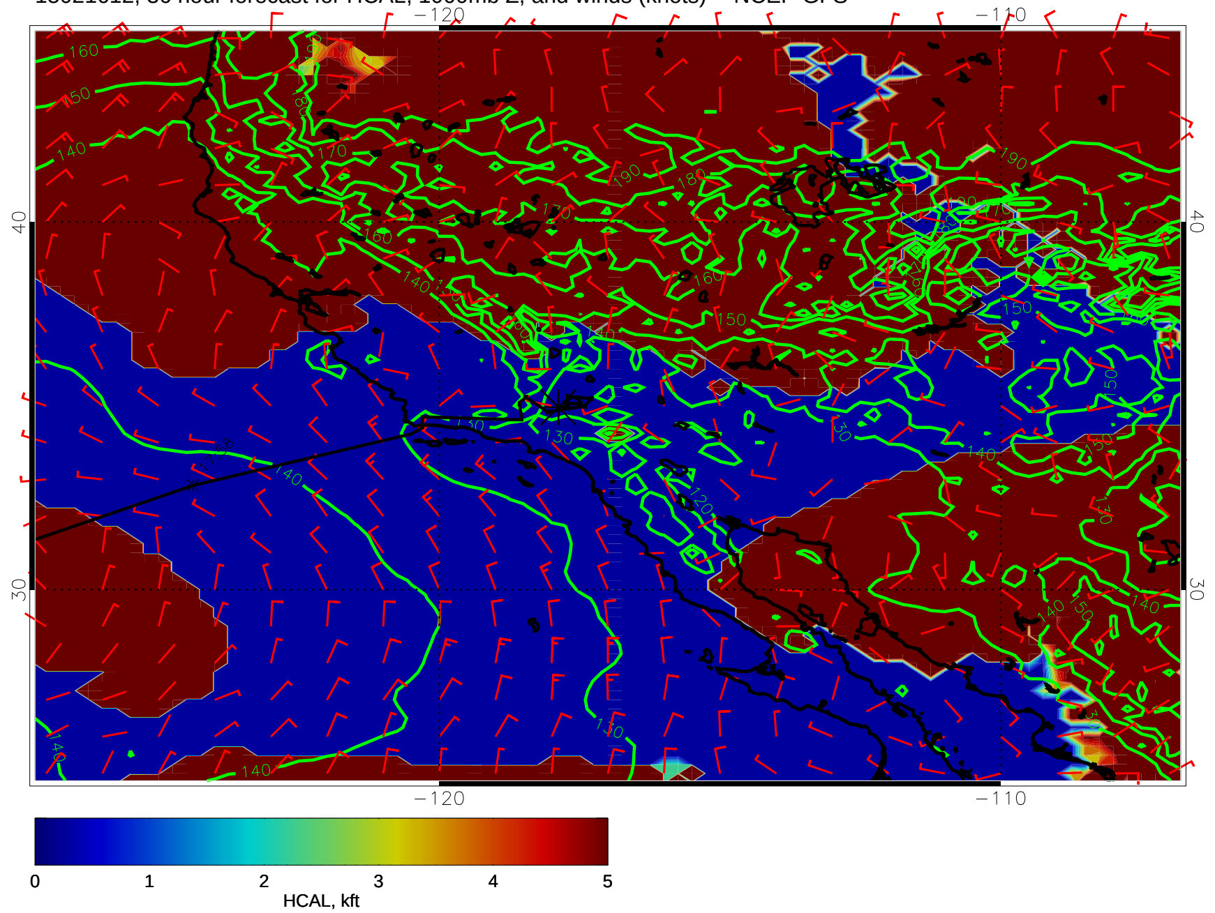
15021612, 36 hour forecast for HCAL, 1000mb Z, and winds (knots) -- NCEP GFS
