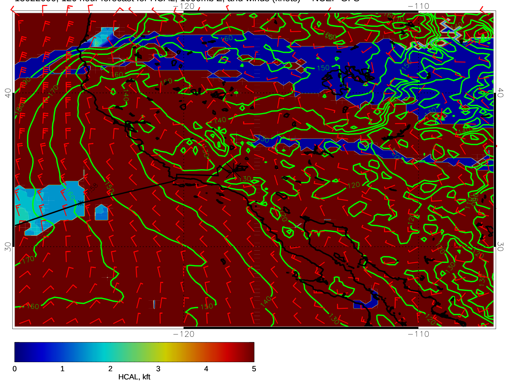
15022000, 120 hour forecast for HCAL, 1000mb Z, and winds (knots) -- NCEP GFS
