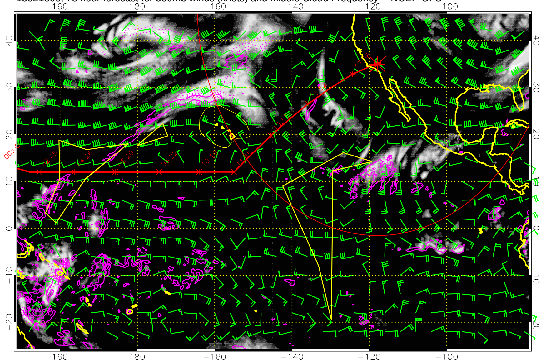
15021806, 78 hour forecast for 500mb winds (knots) and Middle Cloud Frequency -- NCEP GFS
