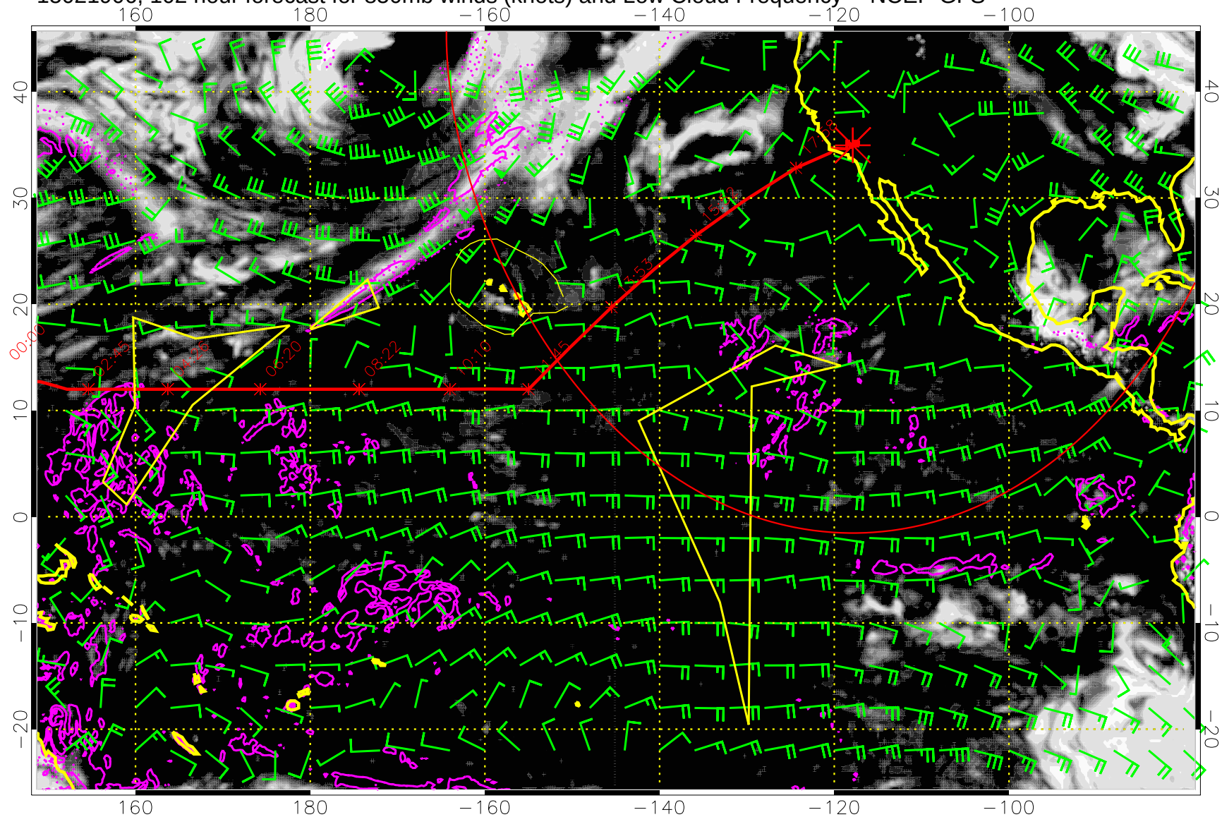
15021906, 102 hour forecast for 850mb winds (knots) and Low Cloud Frequency -- NCEP GFS
