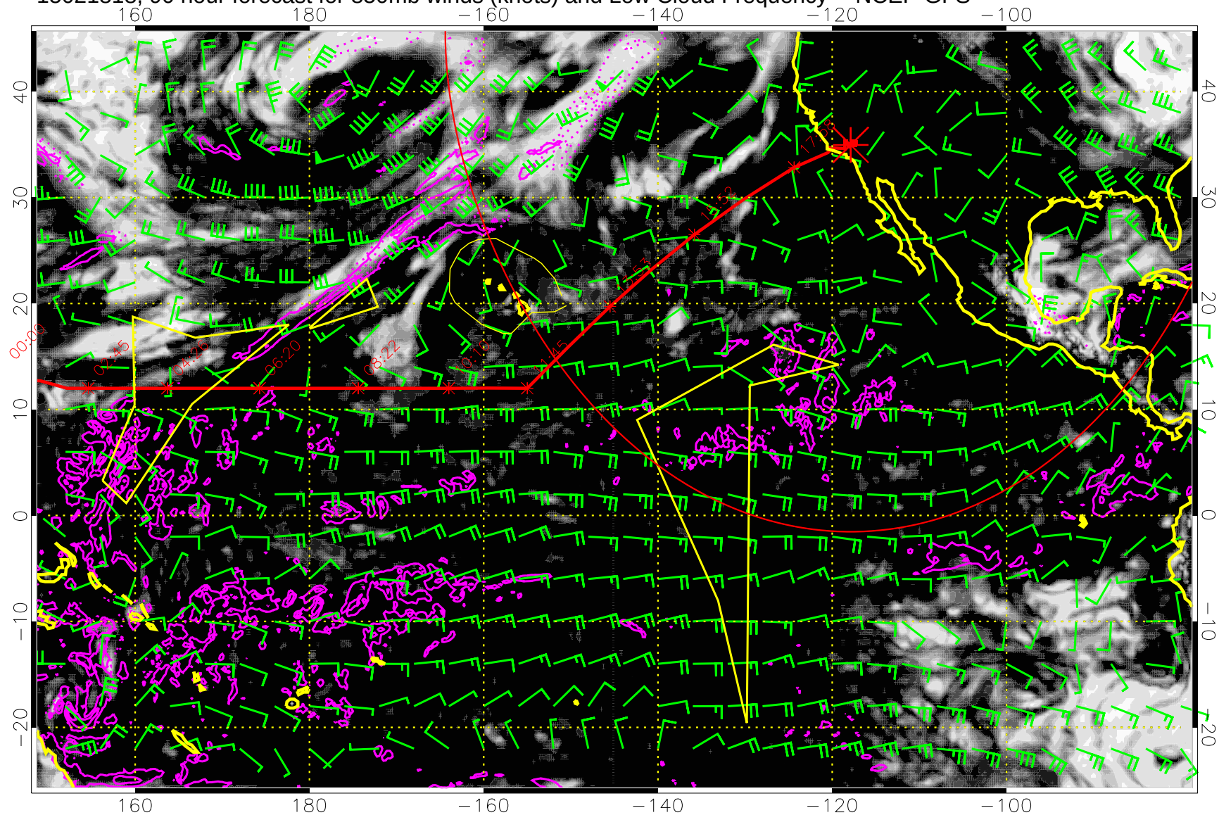
15021818, 90 hour forecast for 850mb winds (knots) and Low Cloud Frequency -- NCEP GFS
