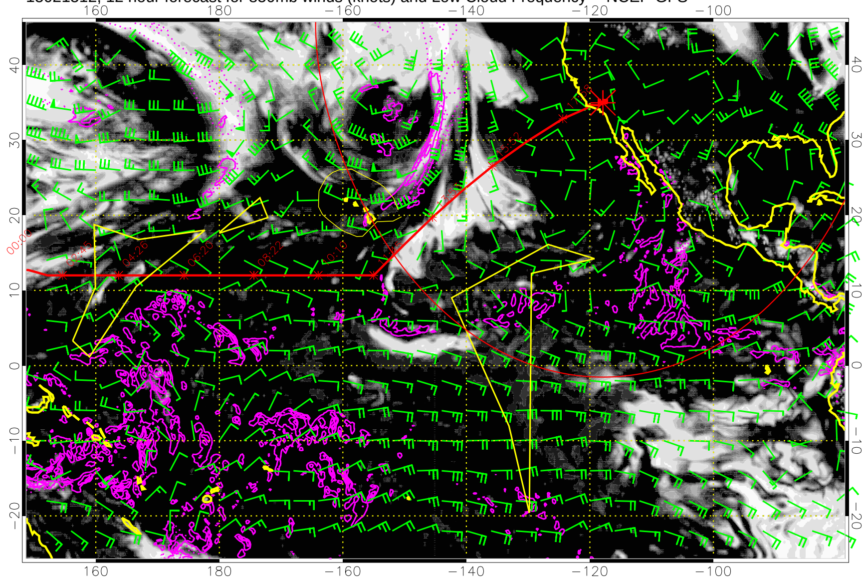
15021512, 12 hour forecast for 850mb winds (knots) and Low Cloud Frequency -- NCEP GFS
