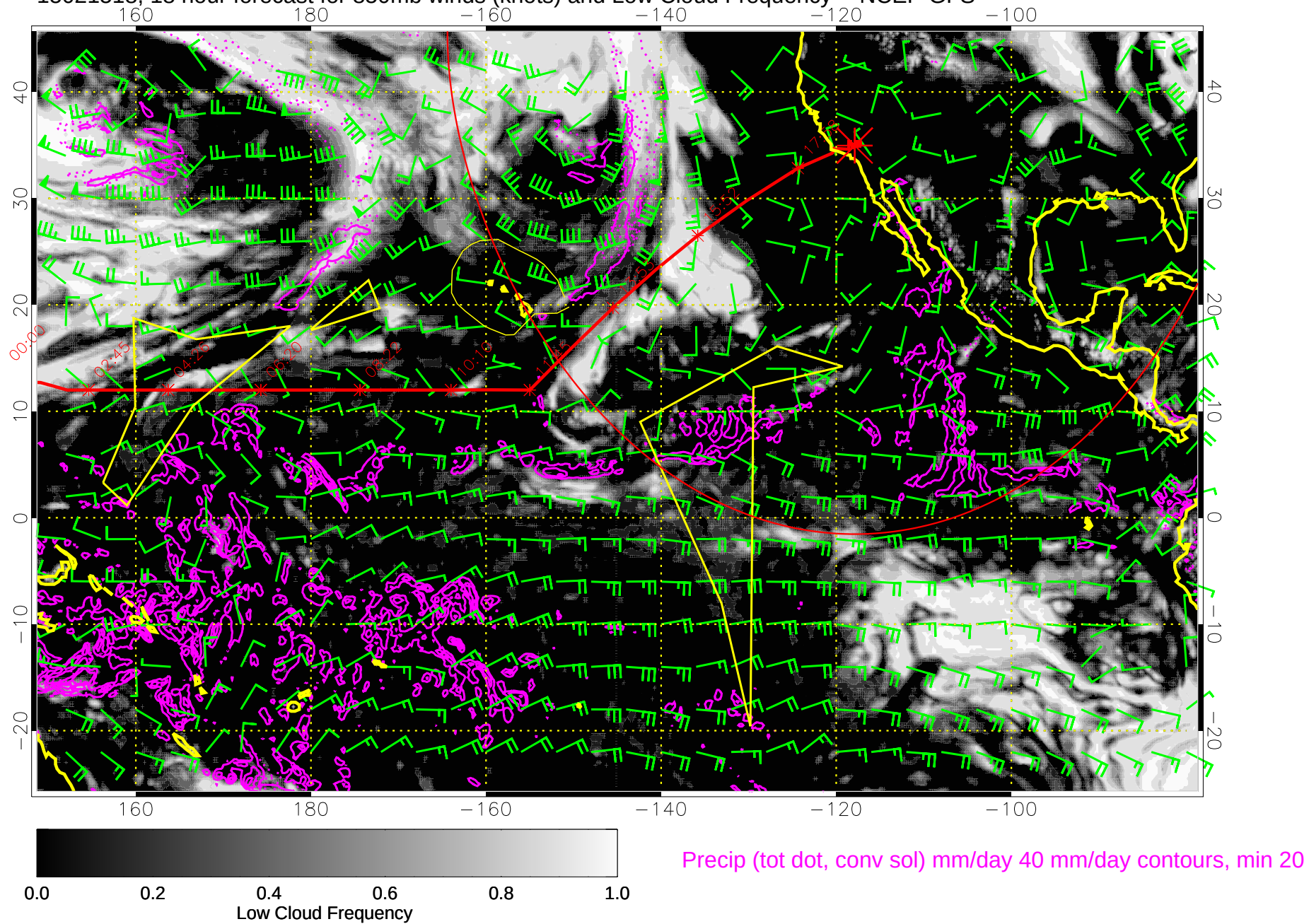
15021518, 18 hour forecast for 850mb winds (knots) and Low Cloud Frequency -- NCEP GFS
