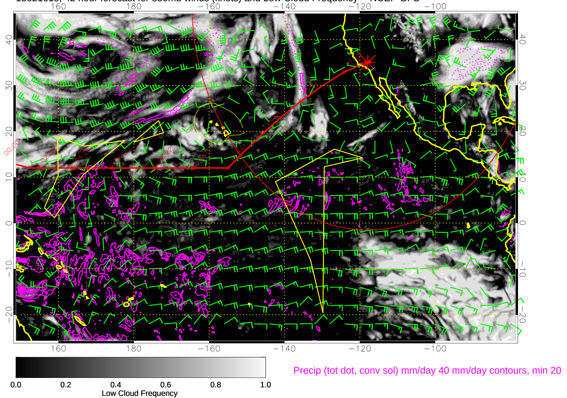
15021618, 42 hour forecast for 850mb winds (knots) and Low Cloud Frequency -- NCEP GFS
