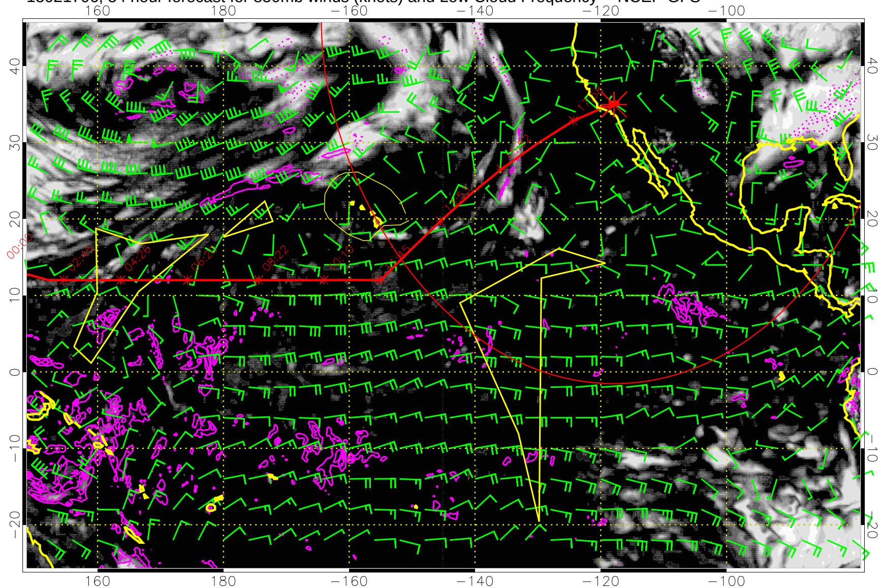
15021706, 54 hour forecast for 850mb winds (knots) and Low Cloud Frequency -- NCEP GFS
