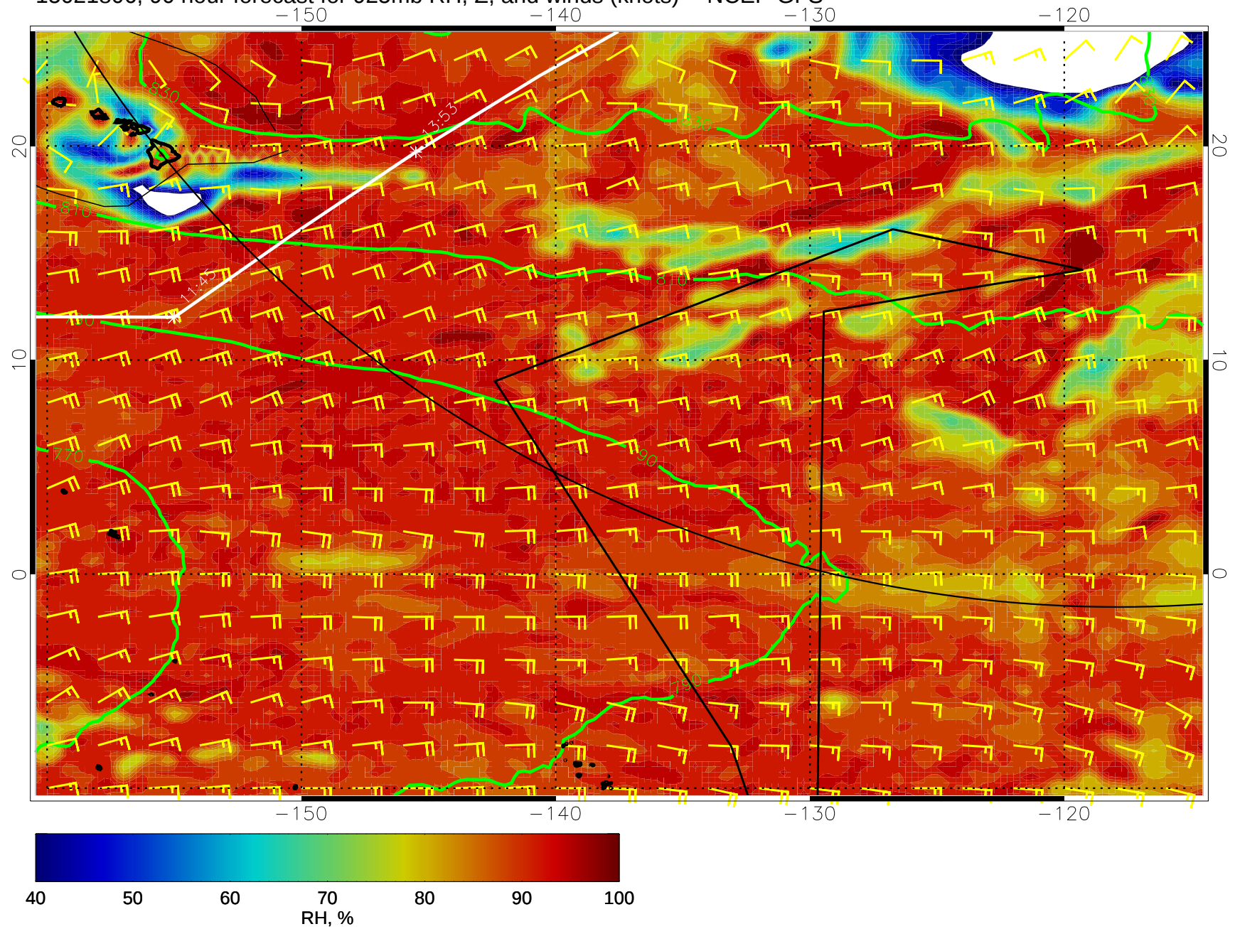
15021806, 90 hour forecast for 925mb RH, Z, and winds (knots) -- NCEP GFS
