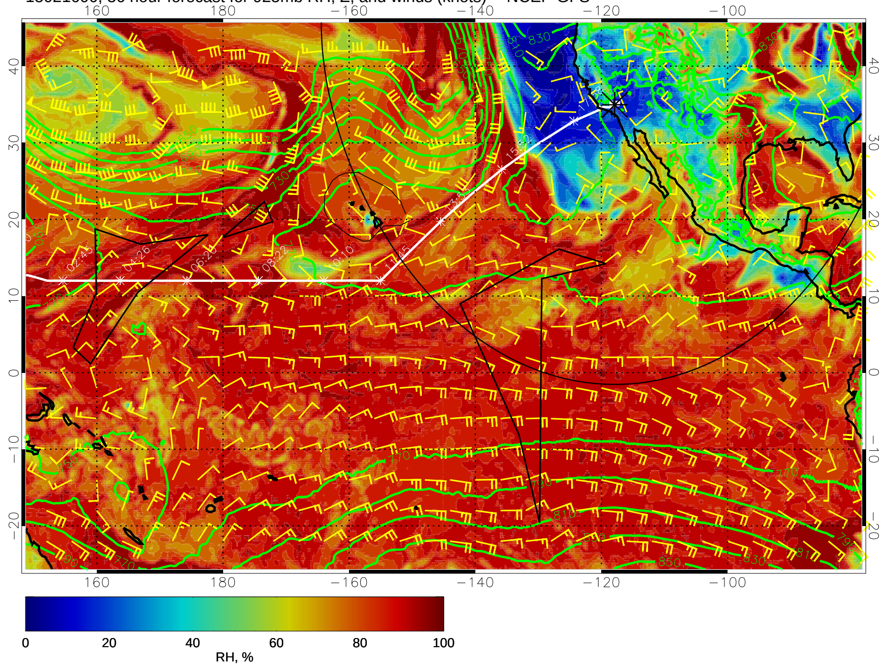
15021600, 36 hour forecast for 925mb RH, Z, and winds (knots) -- NCEP GFS
