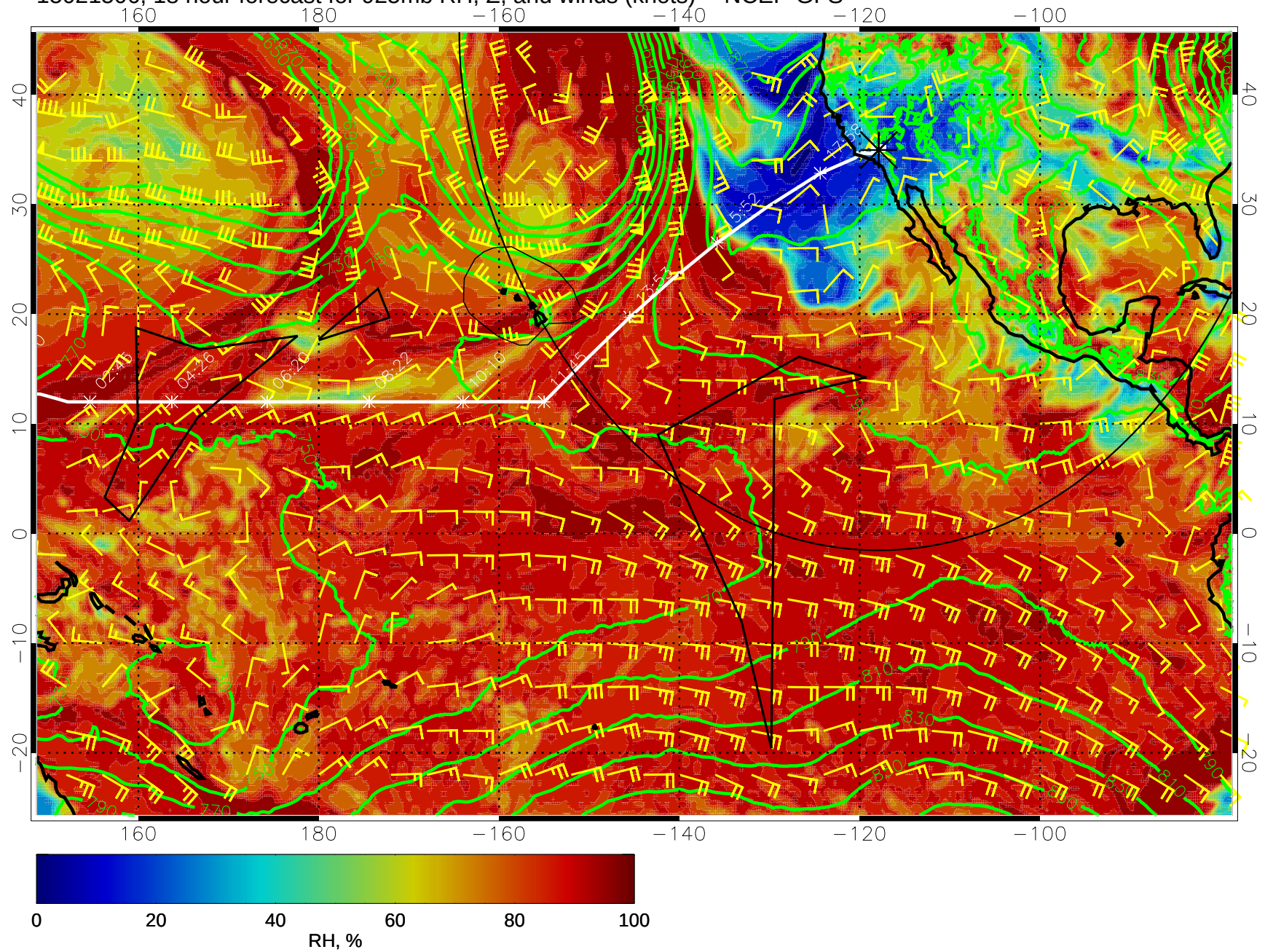
15021506, 18 hour forecast for 925mb RH, Z, and winds (knots) -- NCEP GFS
