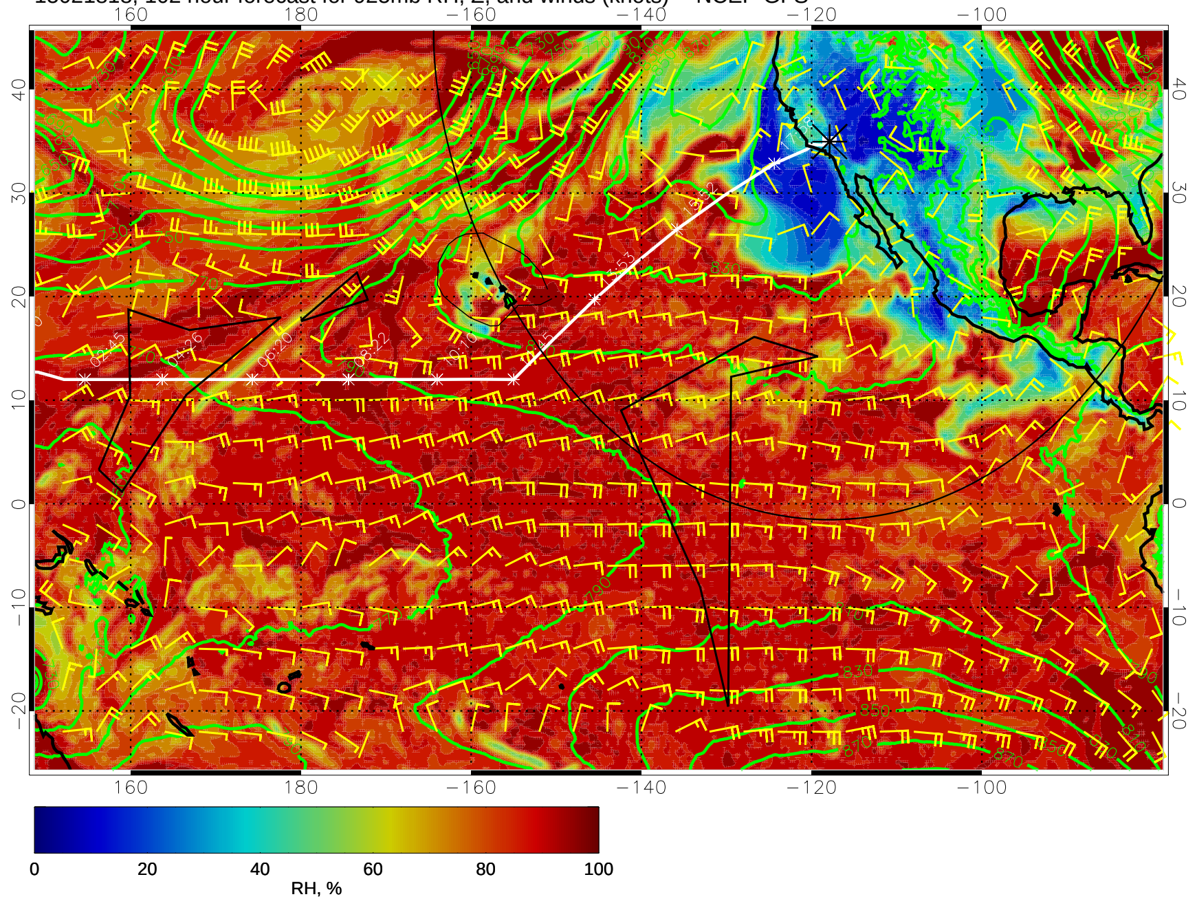
15021818, 102 hour forecast for 925mb RH, Z, and winds (knots) -- NCEP GFS
