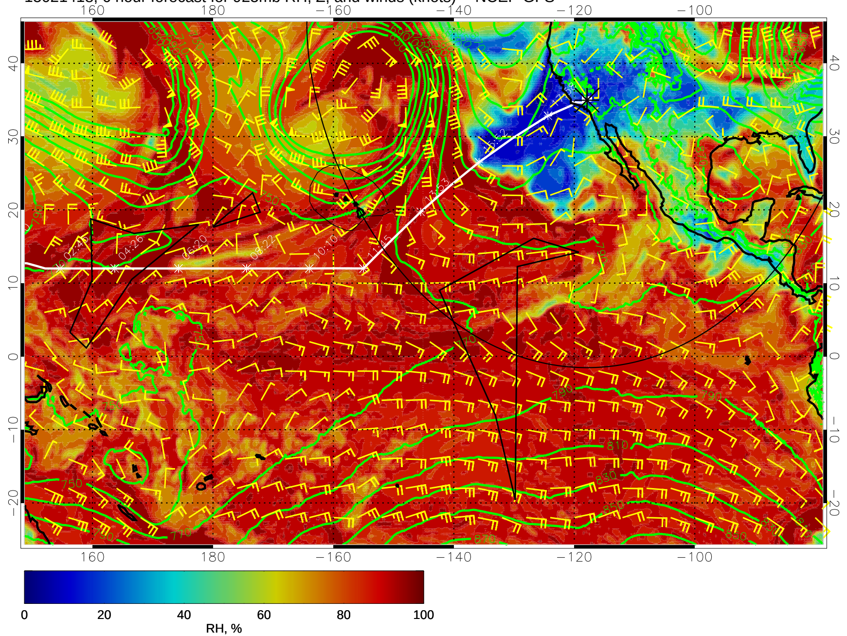
15021418, 6 hour forecast for 925mb RH, Z, and winds (knots) -- NCEP GFS
