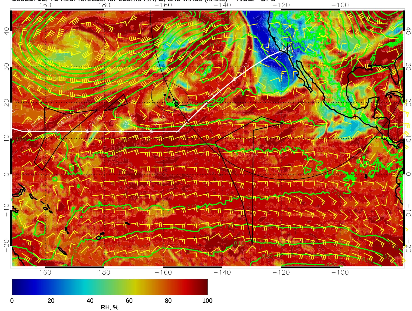
15021712, 72 hour forecast for 925mb RH, Z, and winds (knots) -- NCEP GFS
