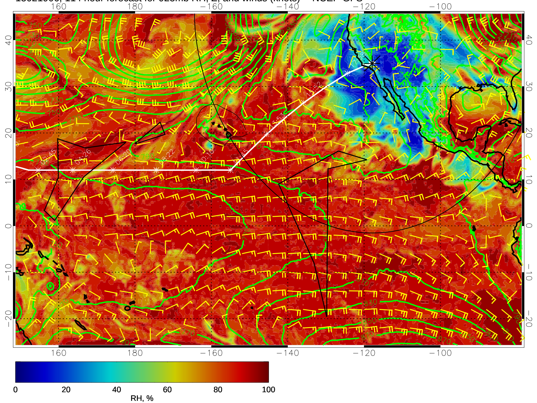
15021906, 114 hour forecast for 925mb RH, Z, and winds (knots) -- NCEP GFS
