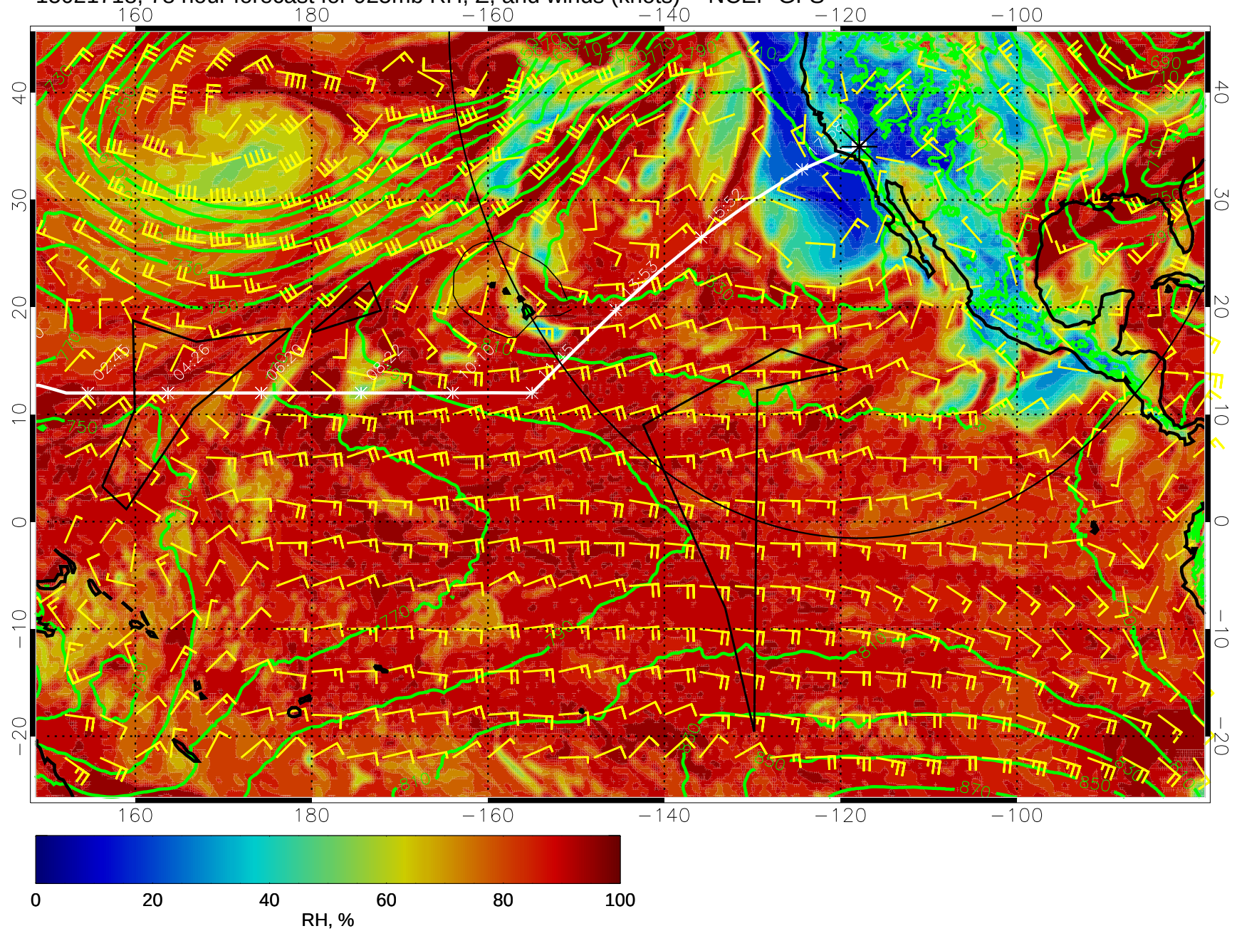
15021718, 78 hour forecast for 925mb RH, Z, and winds (knots) -- NCEP GFS
