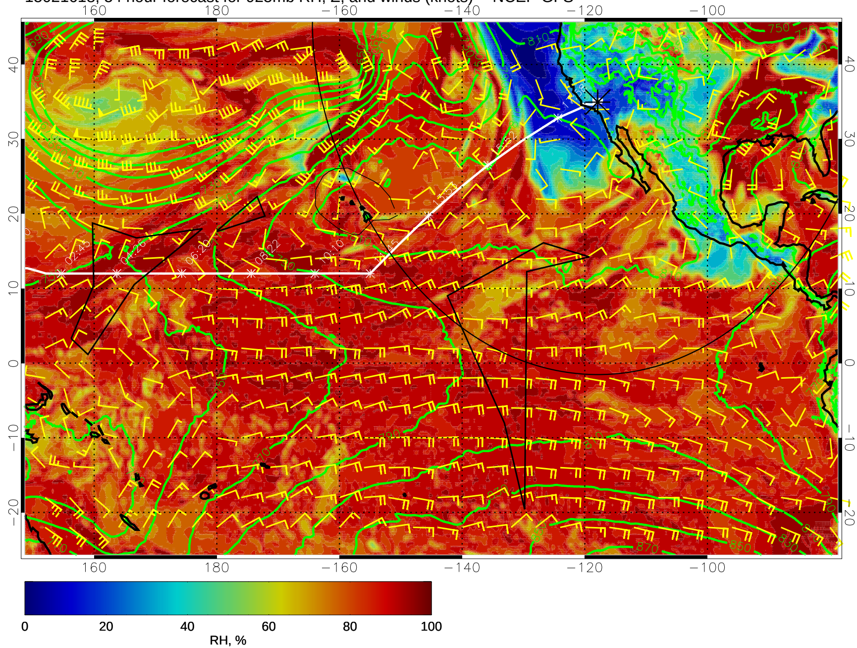
15021618, 54 hour forecast for 925mb RH, Z, and winds (knots) -- NCEP GFS
