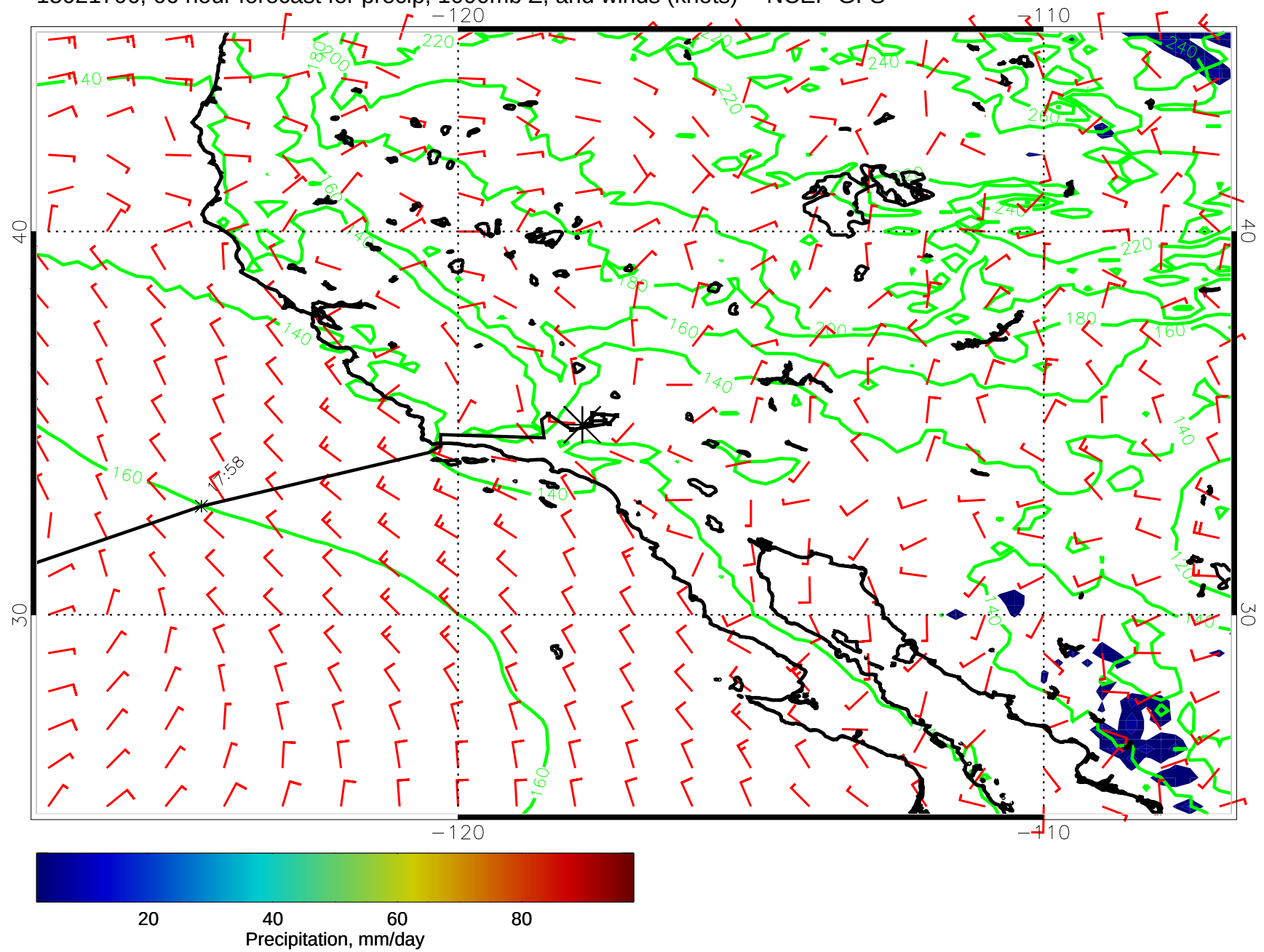
15021706, 66 hour forecast for precip, 1000mb Z, and winds (knots) -- NCEP GFS
