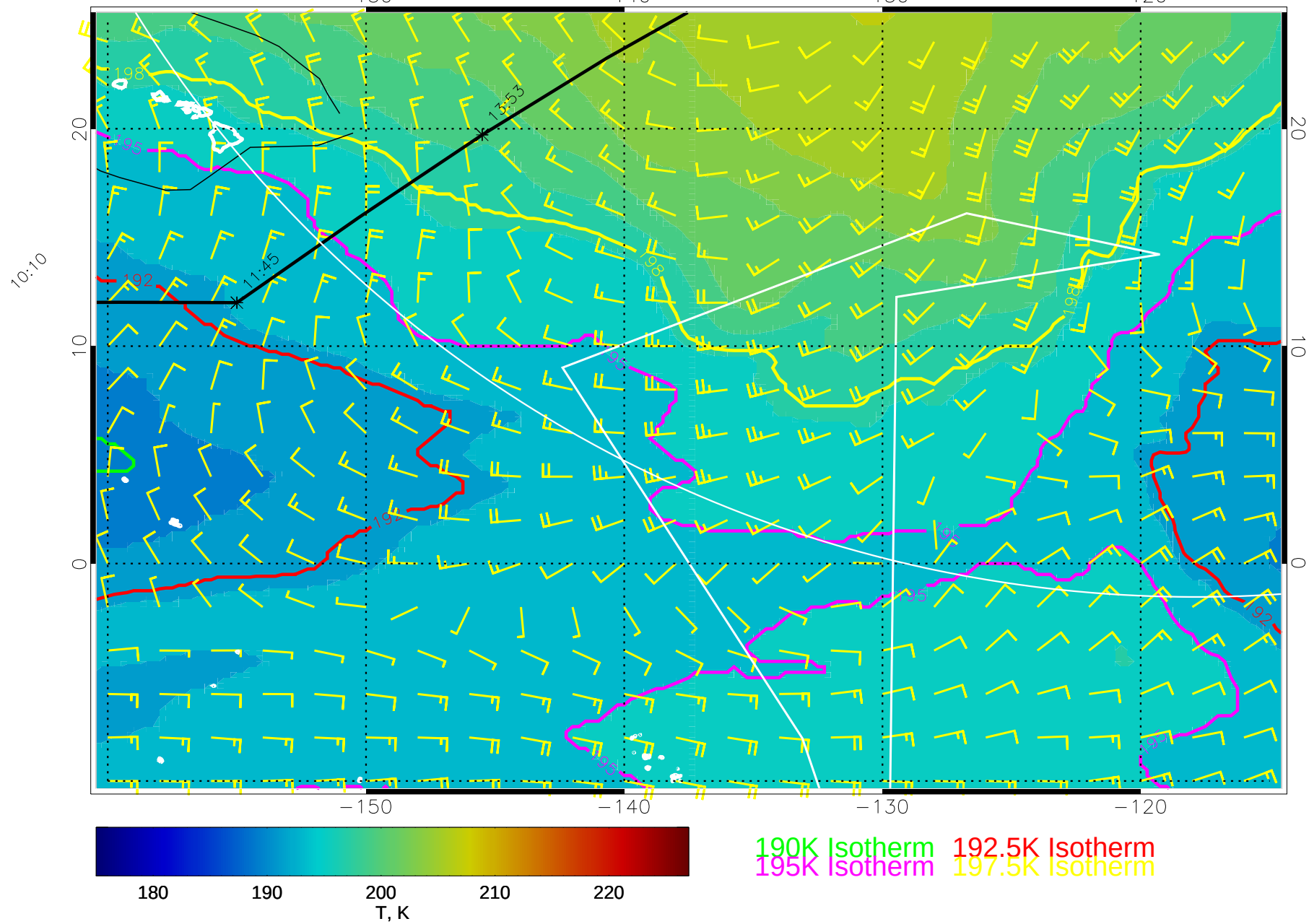
15021912, 120 hour forecast for 70mb T and winds (knots) -- NCEP GFS
