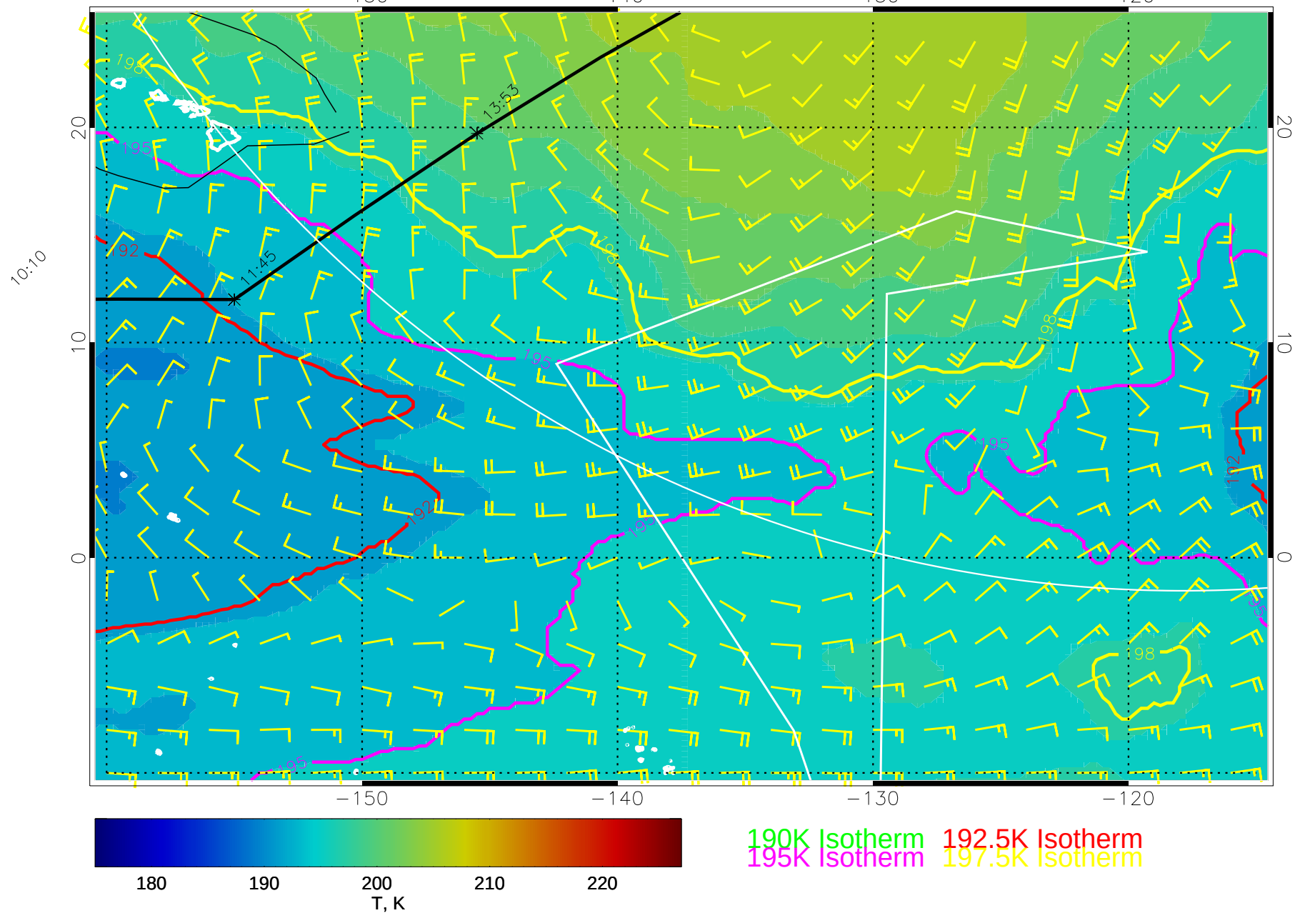
15021906, 114 hour forecast for 70mb T and winds (knots) -- NCEP GFS
