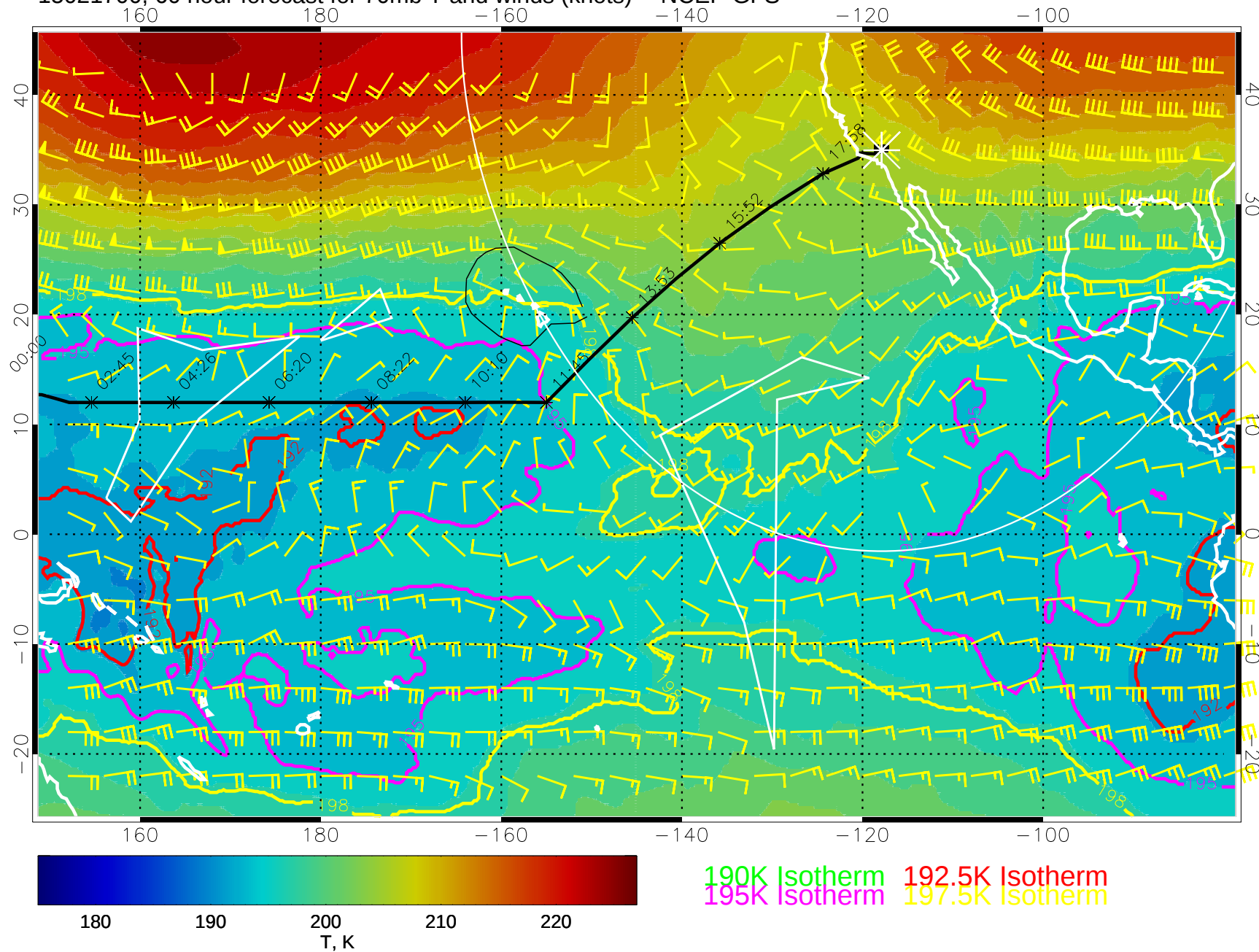
15021700, 60 hour forecast for 70mb T and winds (knots) -- NCEP GFS
