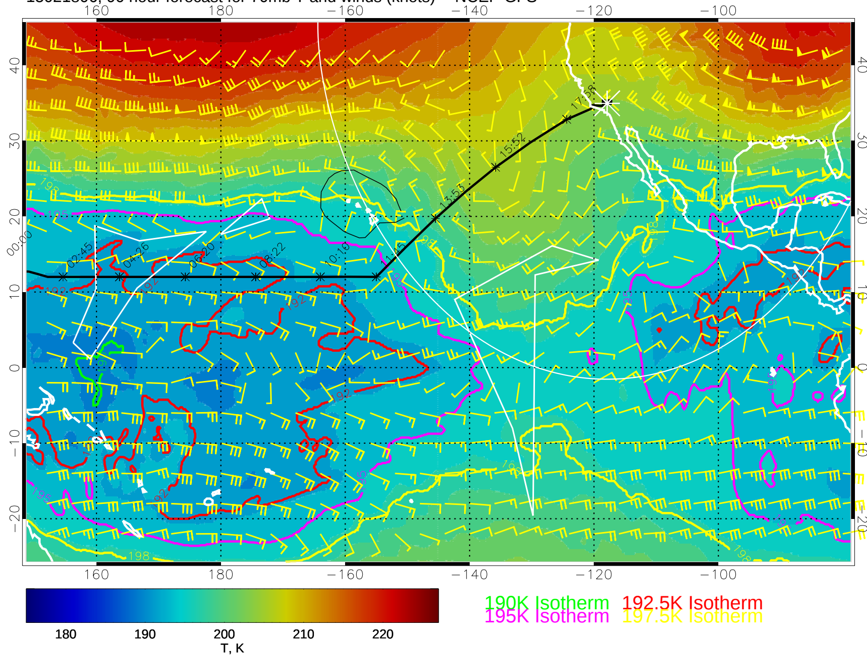
15021806, 90 hour forecast for 70mb T and winds (knots) -- NCEP GFS
