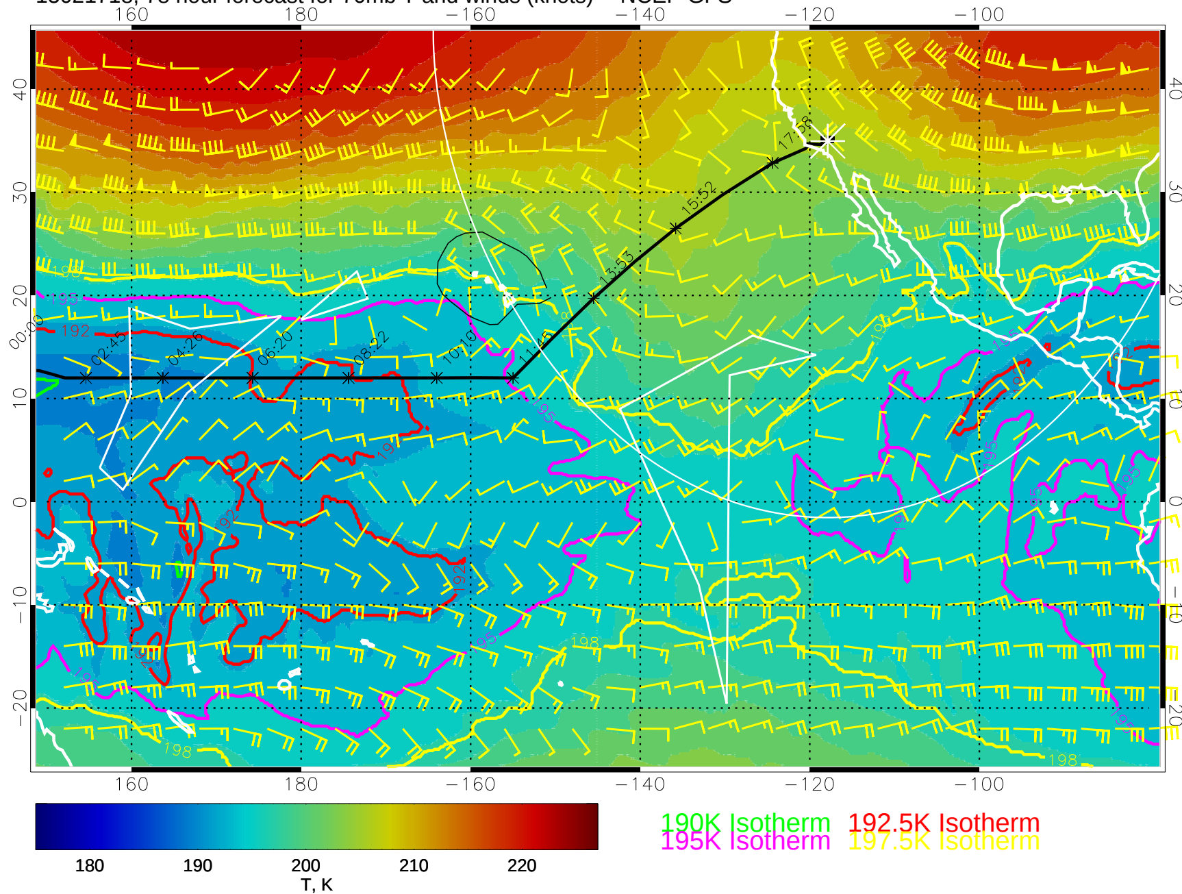
15021718, 78 hour forecast for 70mb T and winds (knots) -- NCEP GFS
