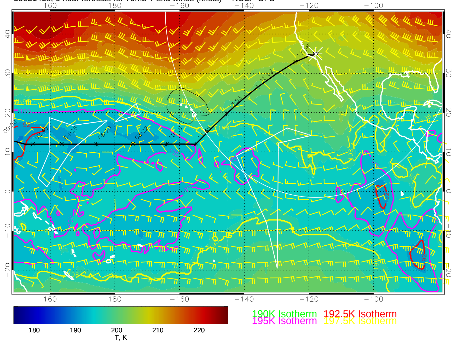
15021418, 6 hour forecast for 70mb T and winds (knots) -- NCEP GFS
