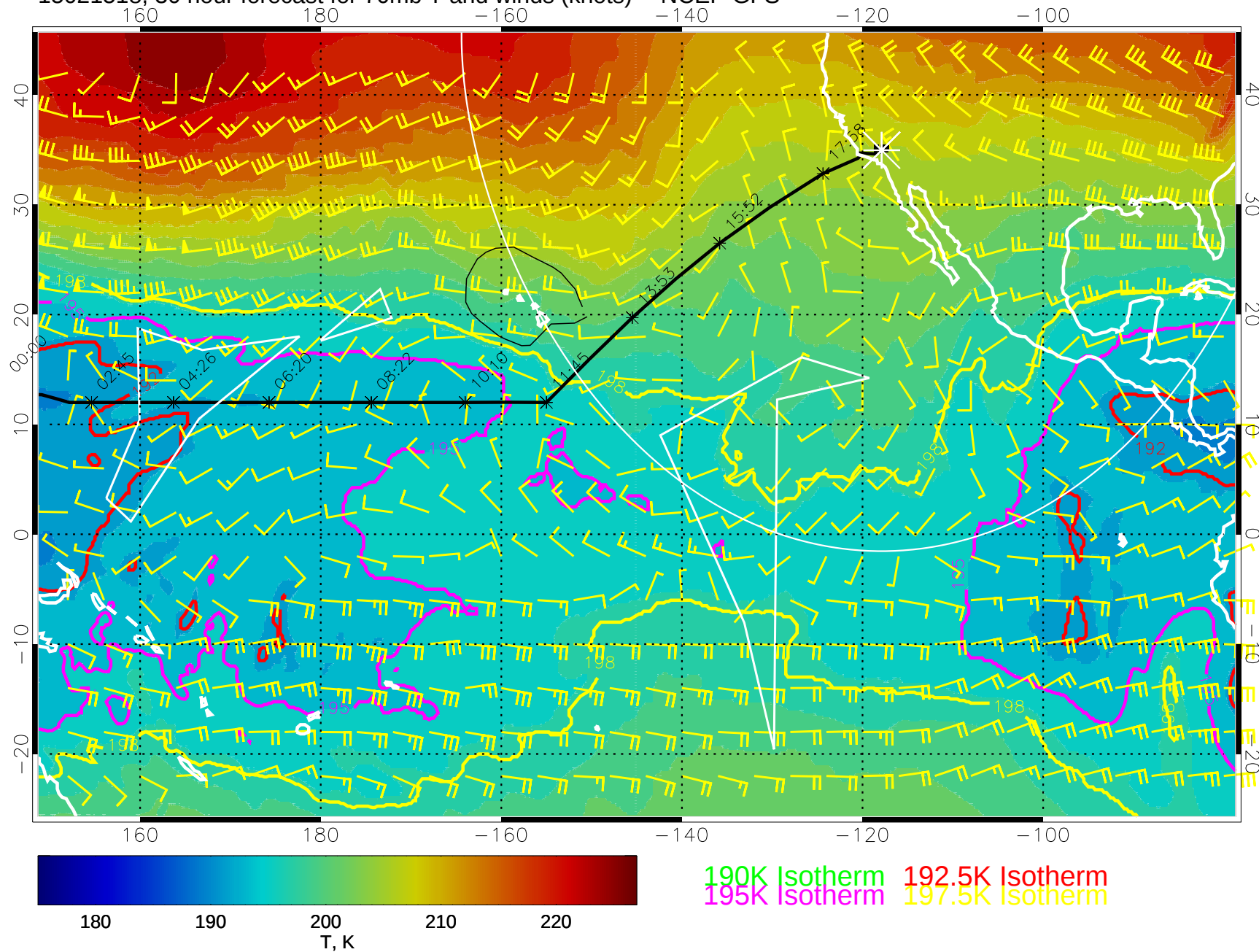
15021518, 30 hour forecast for 70mb T and winds (knots) -- NCEP GFS
