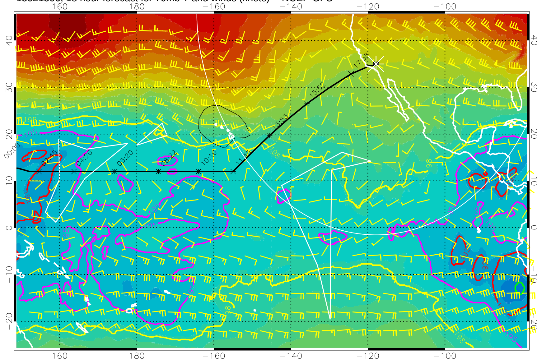
15021506, 18 hour forecast for 70mb T and winds (knots) -- NCEP GFS
