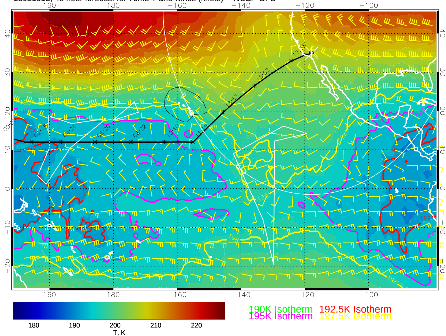
15021612, 48 hour forecast for 70mb T and winds (knots) -- NCEP GFS
