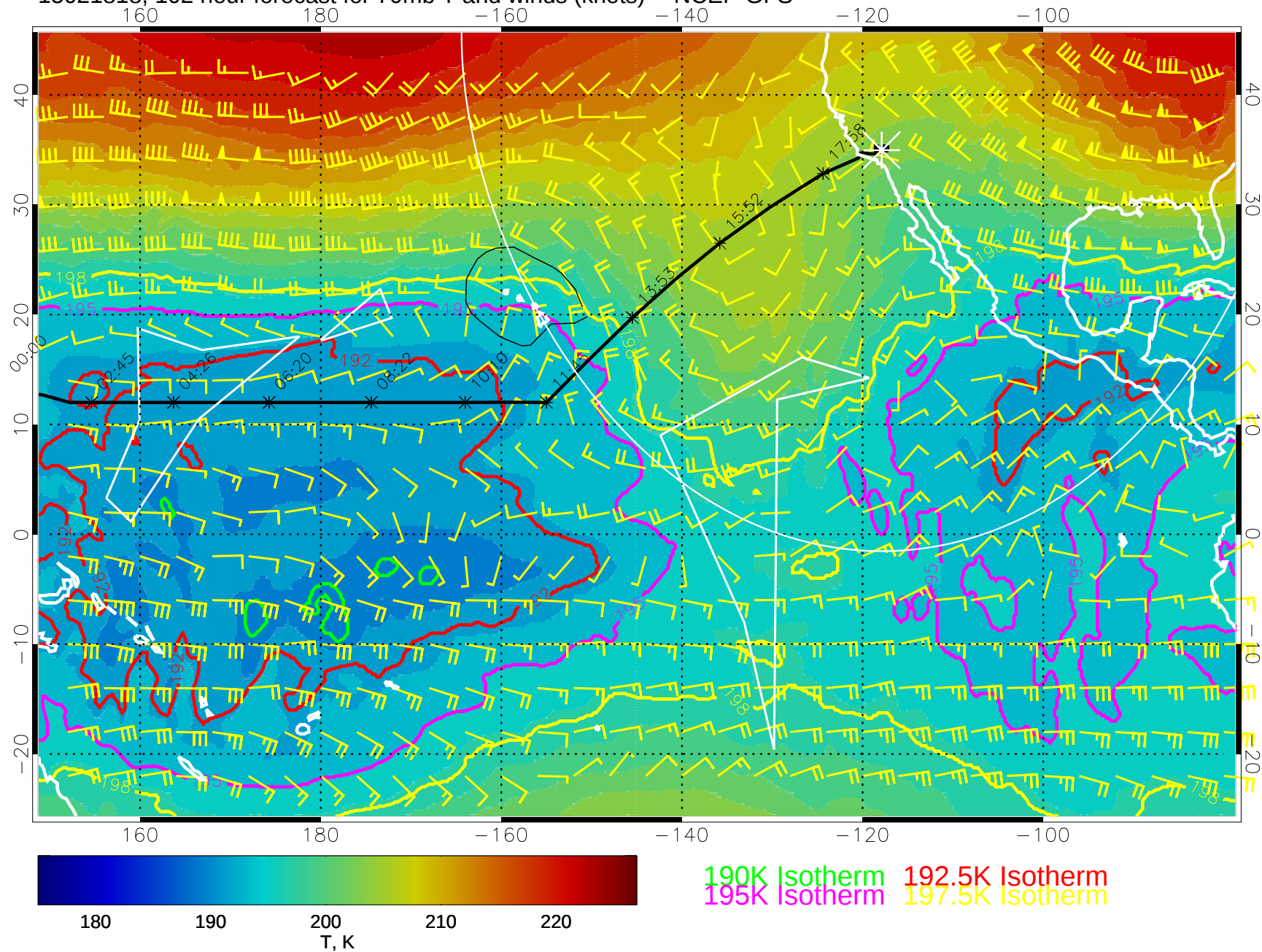
15021818, 102 hour forecast for 70mb T and winds (knots) -- NCEP GFS
