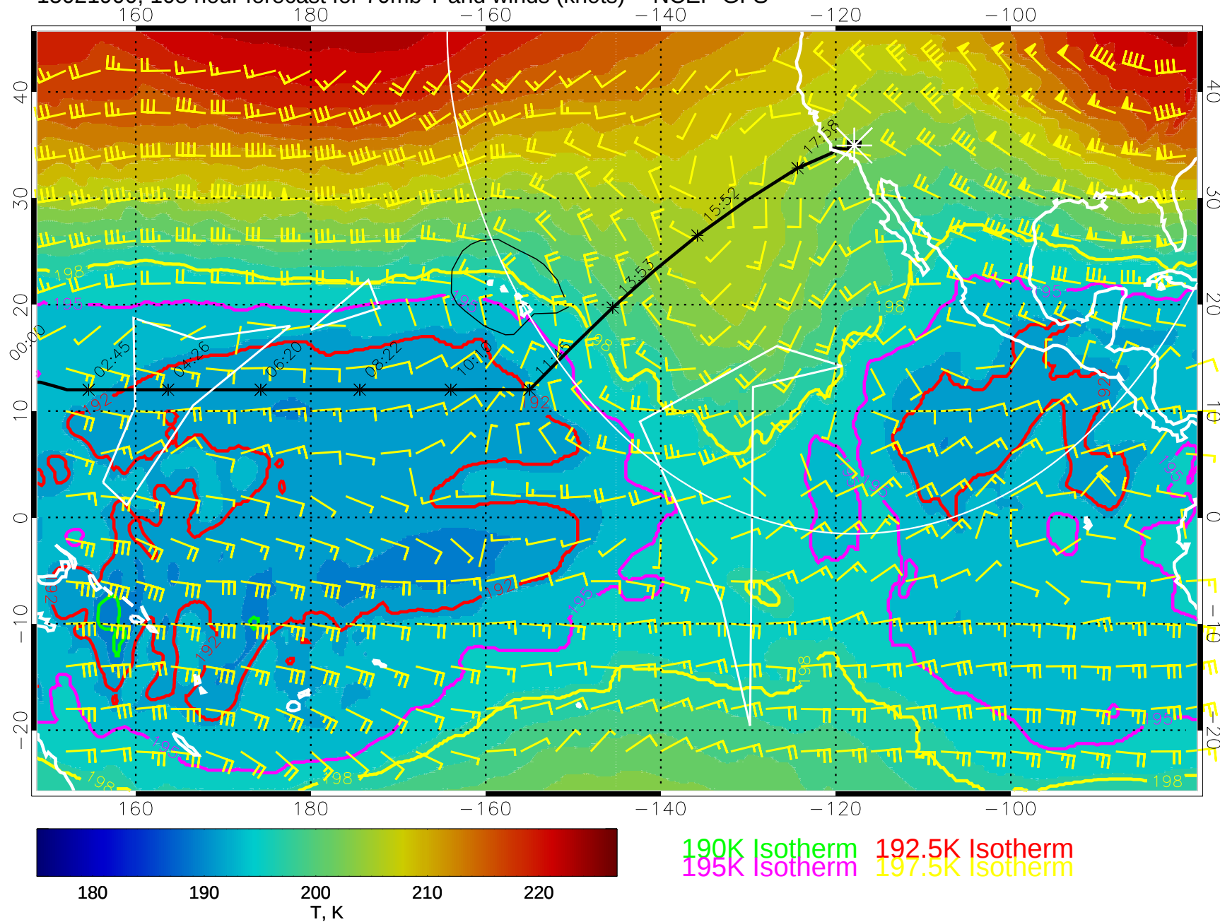
15021900, 108 hour forecast for 70mb T and winds (knots) -- NCEP GFS
