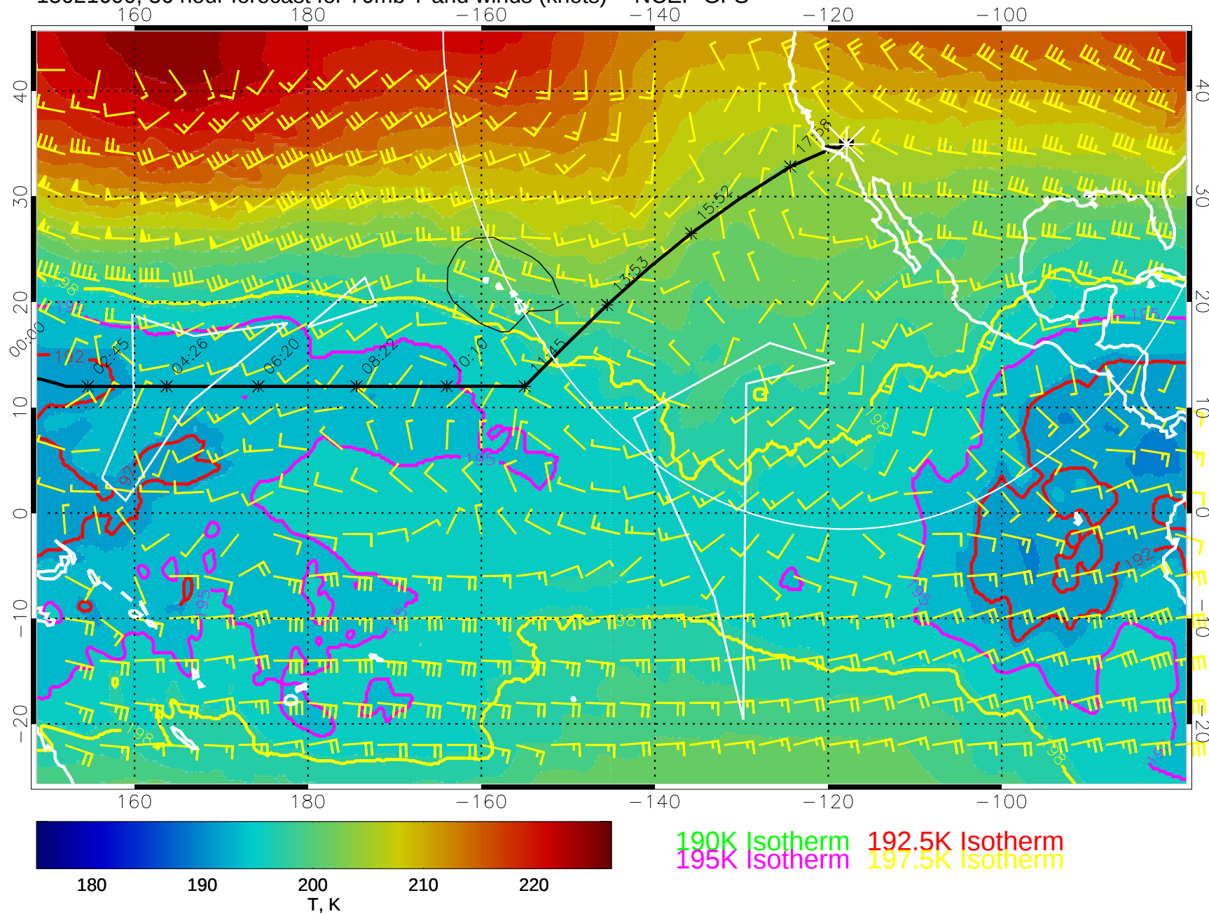
15021600, 36 hour forecast for 70mb T and winds (knots) -- NCEP GFS
