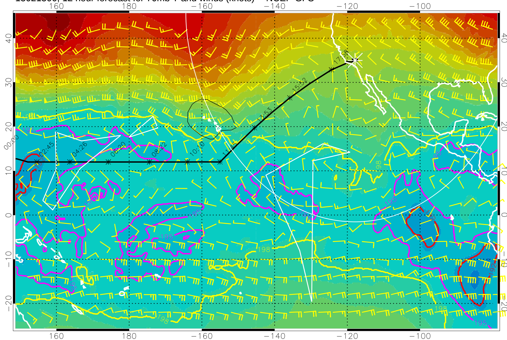
15021500, 12 hour forecast for 70mb T and winds (knots) -- NCEP GFS
