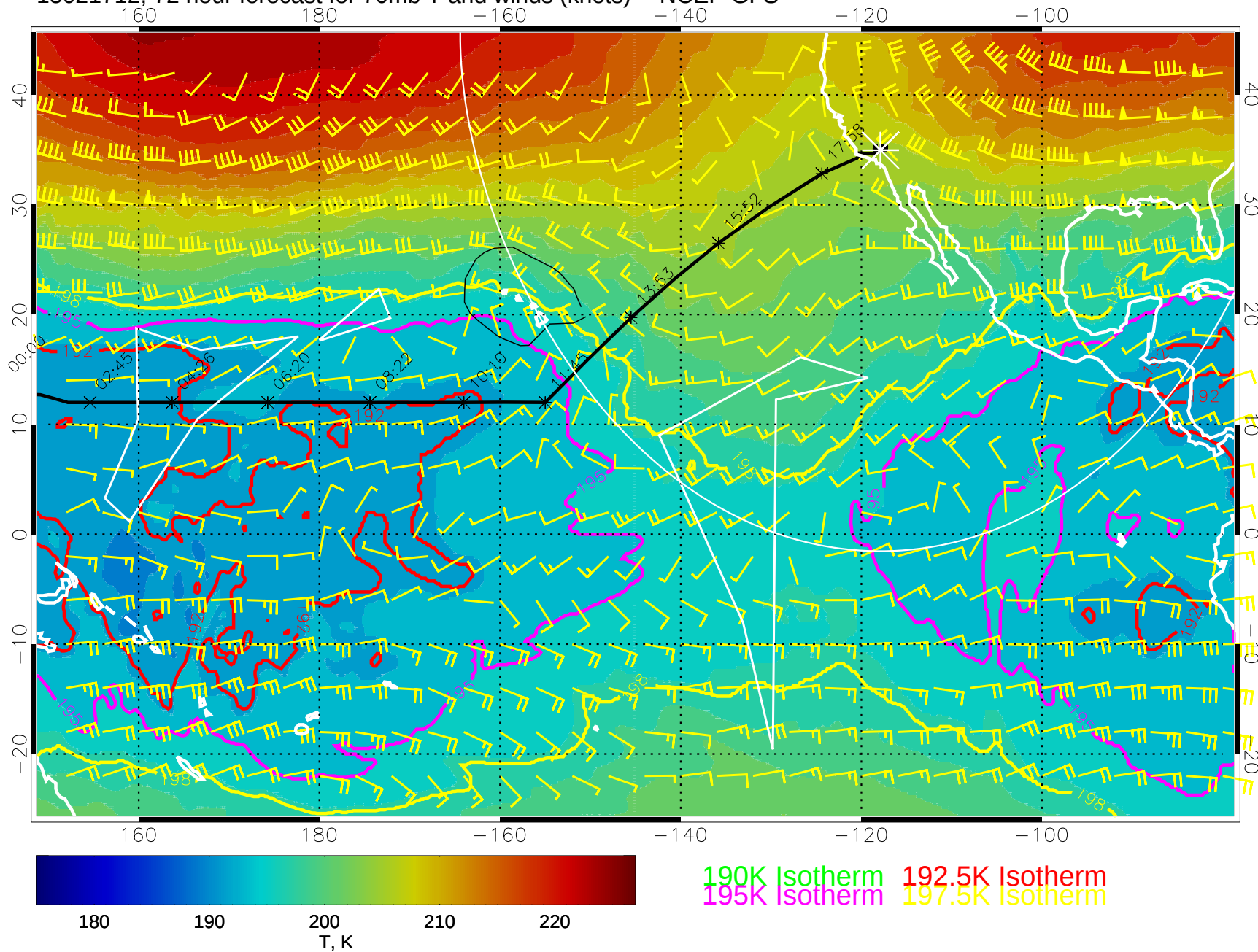
15021712, 72 hour forecast for 70mb T and winds (knots) -- NCEP GFS
