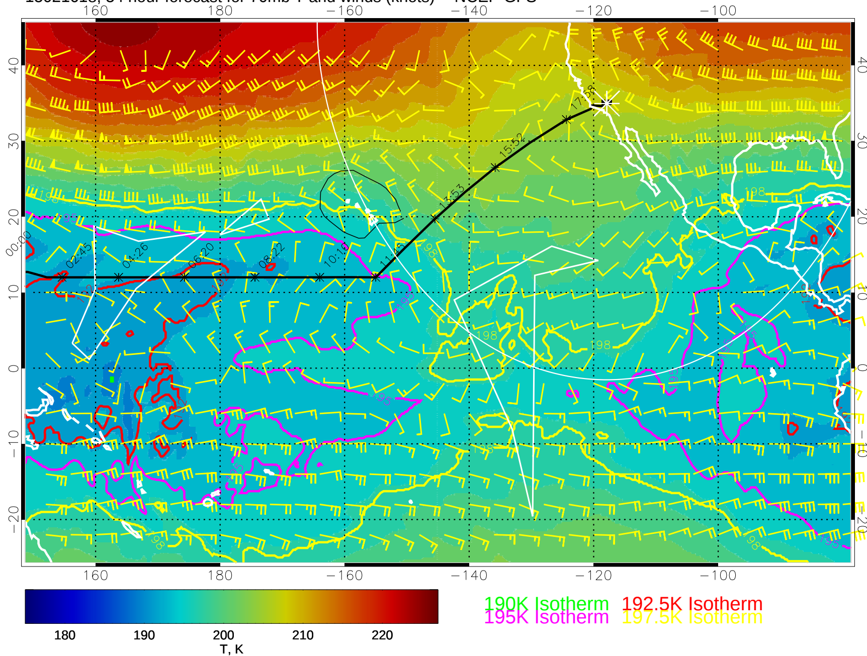
15021618, 54 hour forecast for 70mb T and winds (knots) -- NCEP GFS
