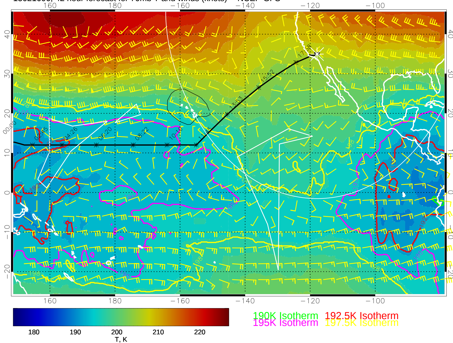
15021606, 42 hour forecast for 70mb T and winds (knots) -- NCEP GFS
