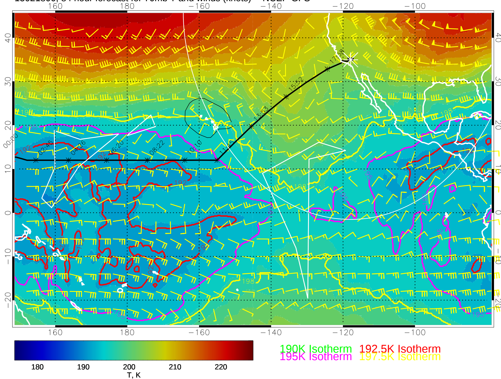
15021800, 84 hour forecast for 70mb T and winds (knots) -- NCEP GFS
