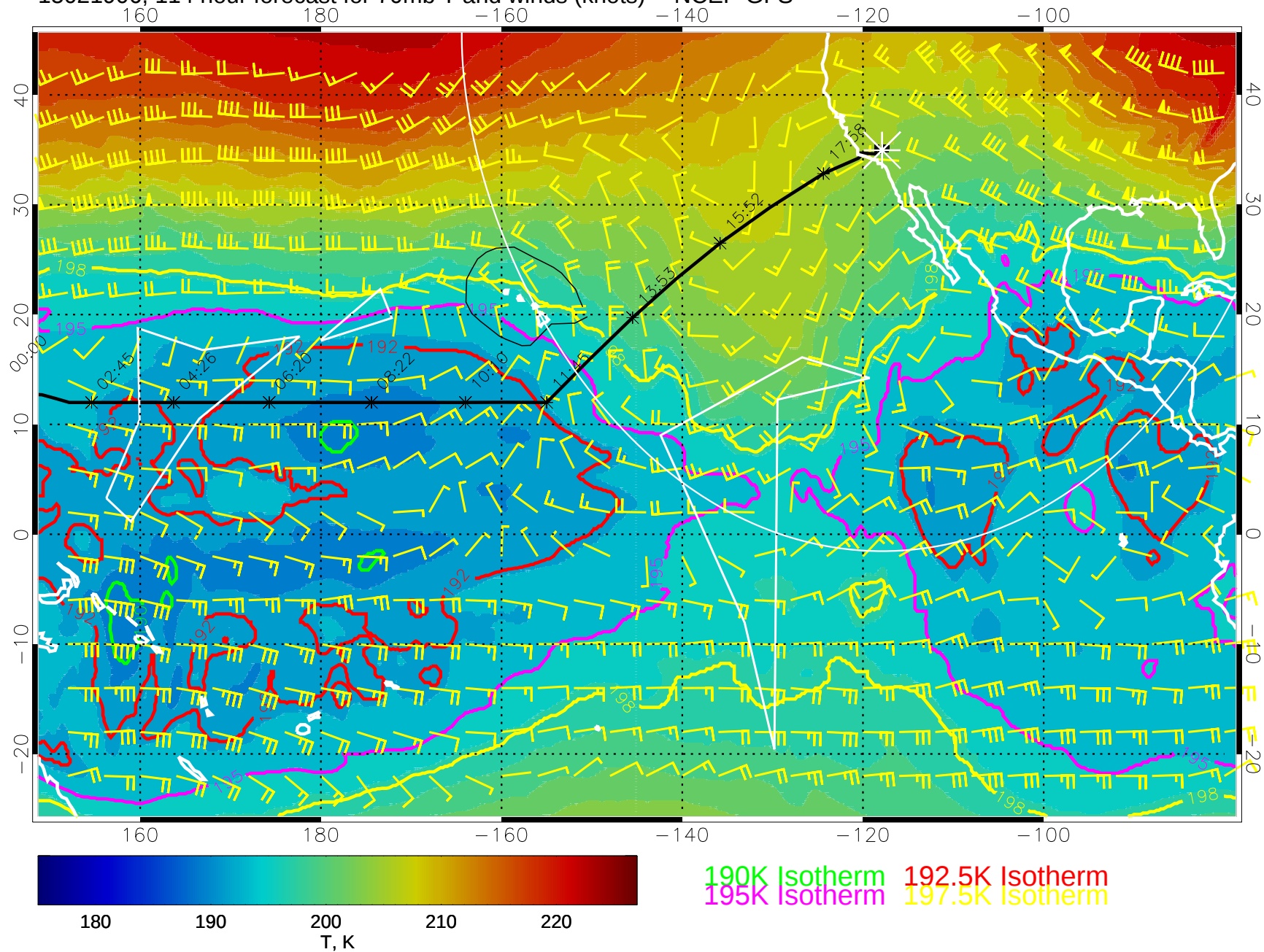
15021906, 114 hour forecast for 70mb T and winds (knots) -- NCEP GFS
