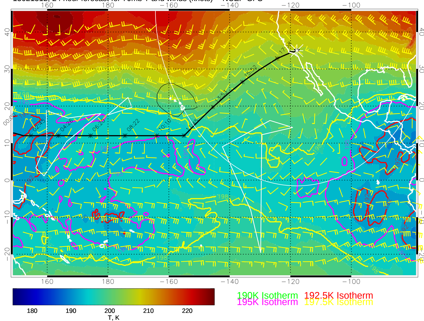
15021512, 24 hour forecast for 70mb T and winds (knots) -- NCEP GFS
