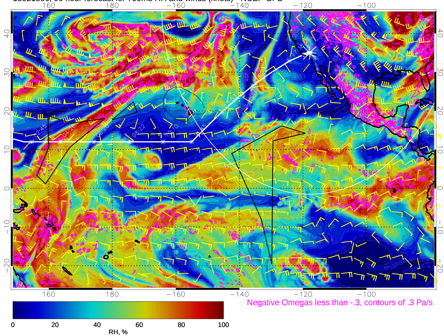
15021806, 90 hour forecast for 700mb RH and winds (knots) - NCEP GFS
