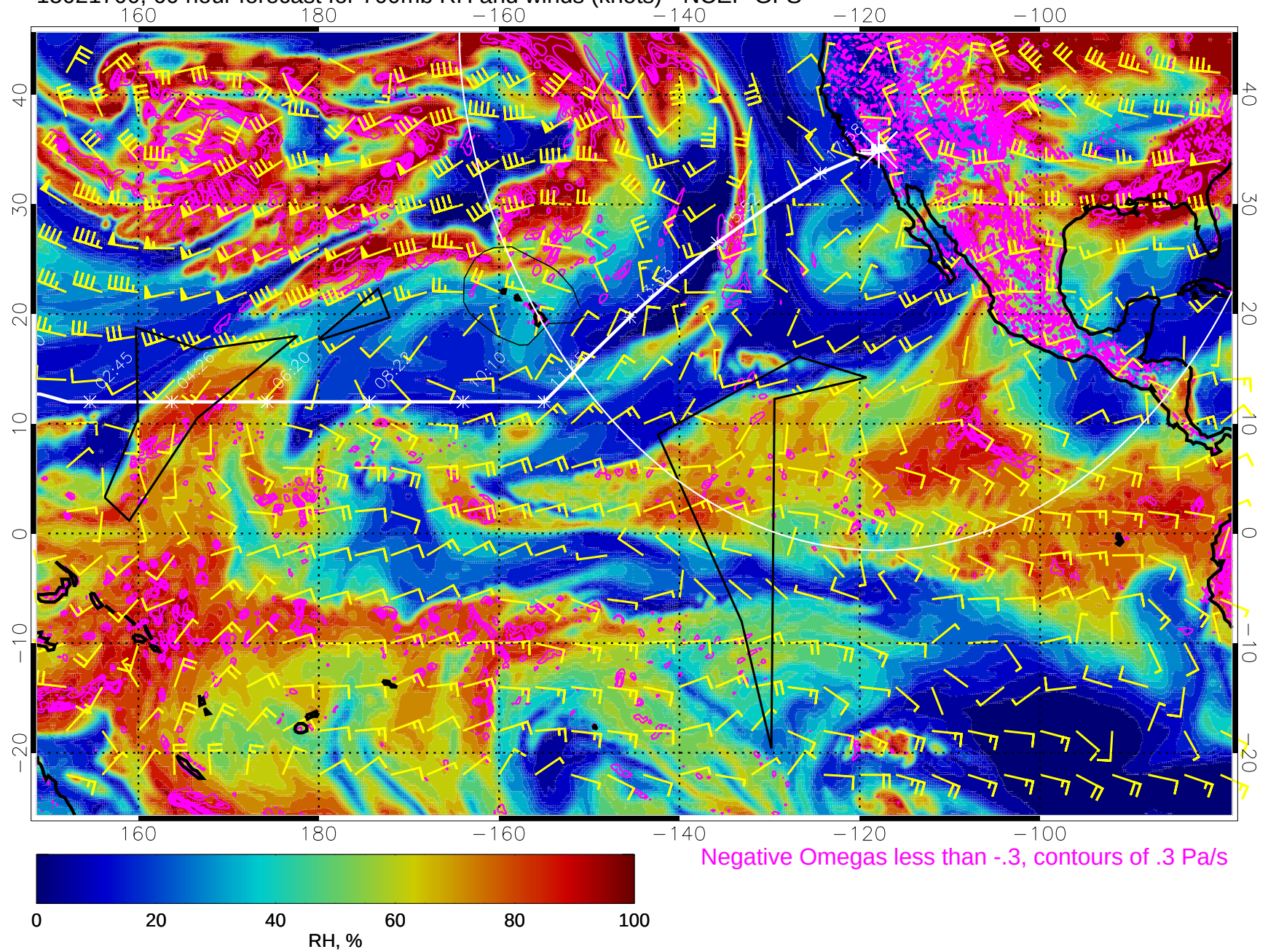
15021700, 60 hour forecast for 700mb RH and winds (knots) - NCEP GFS
