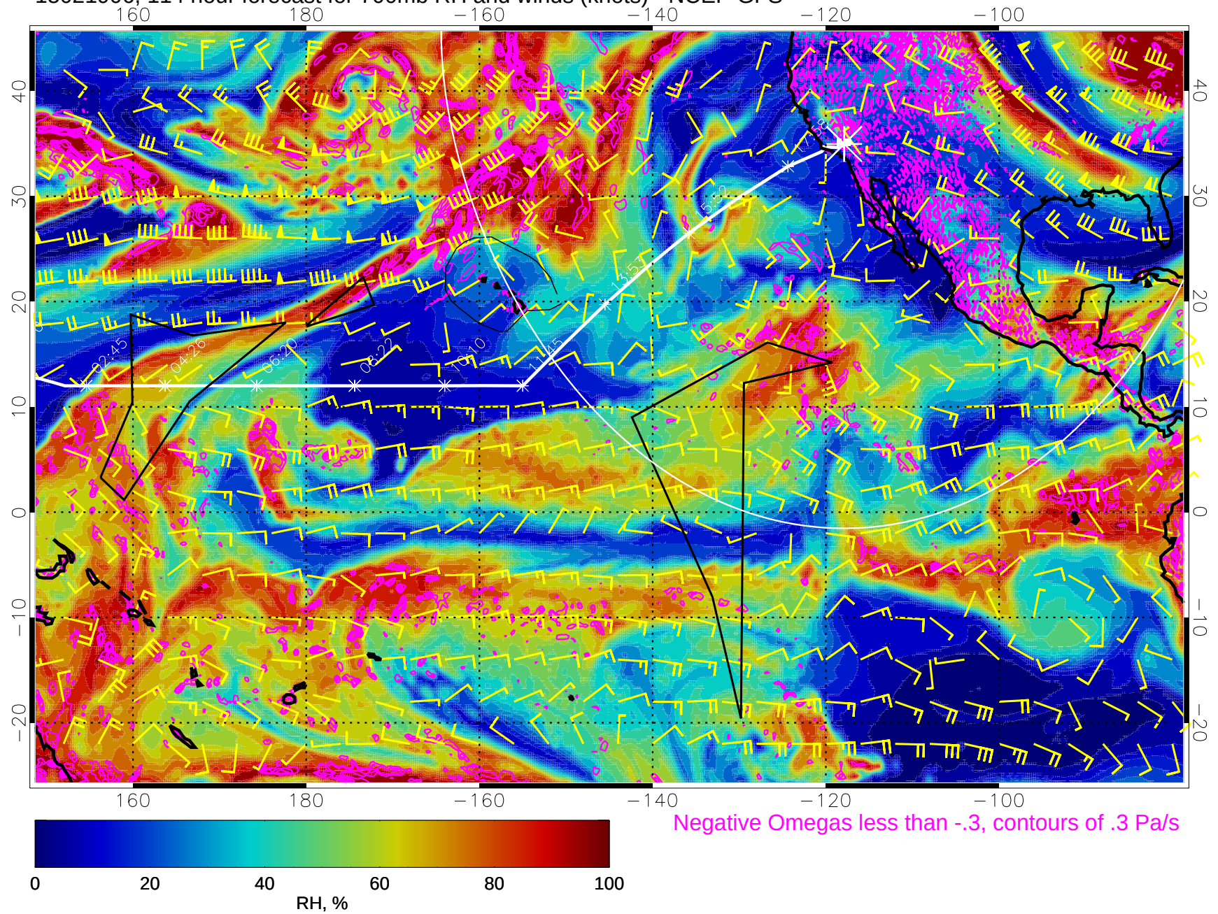
15021906, 114 hour forecast for 700mb RH and winds (knots) - NCEP GFS
