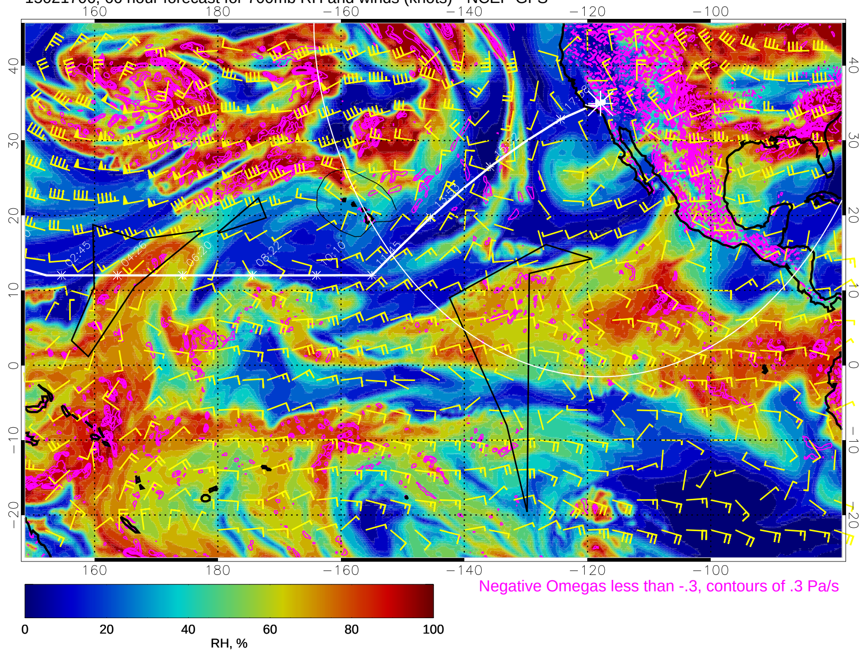
15021706, 66 hour forecast for 700mb RH and winds (knots) - NCEP GFS
