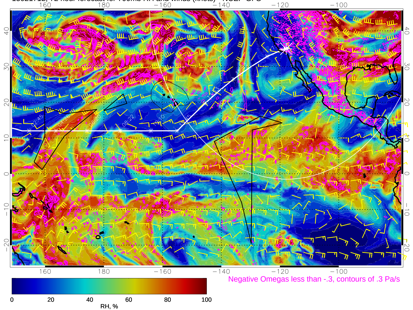
15021712, 72 hour forecast for 700mb RH and winds (knots) - NCEP GFS
