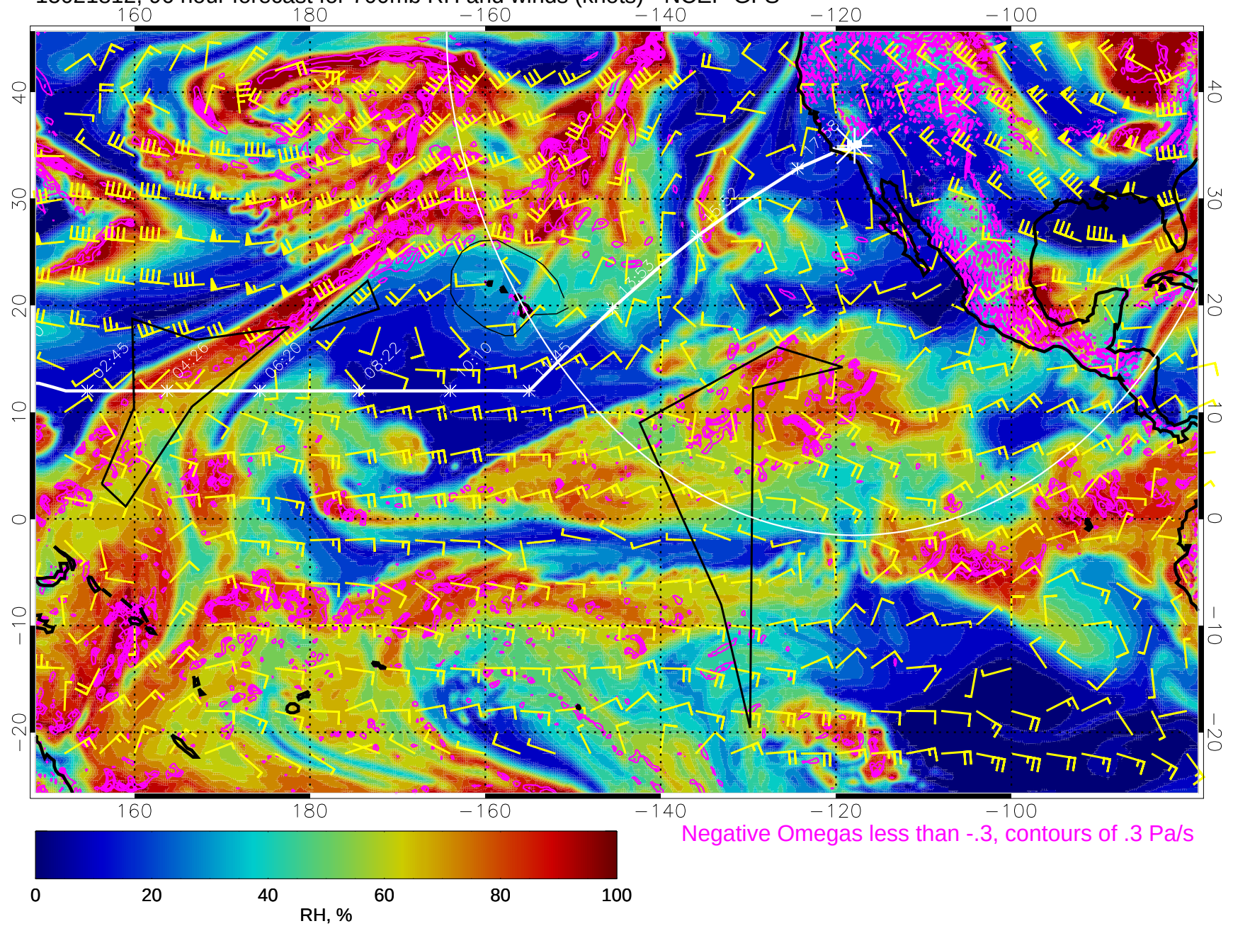
15021812, 96 hour forecast for 700mb RH and winds (knots) - NCEP GFS
