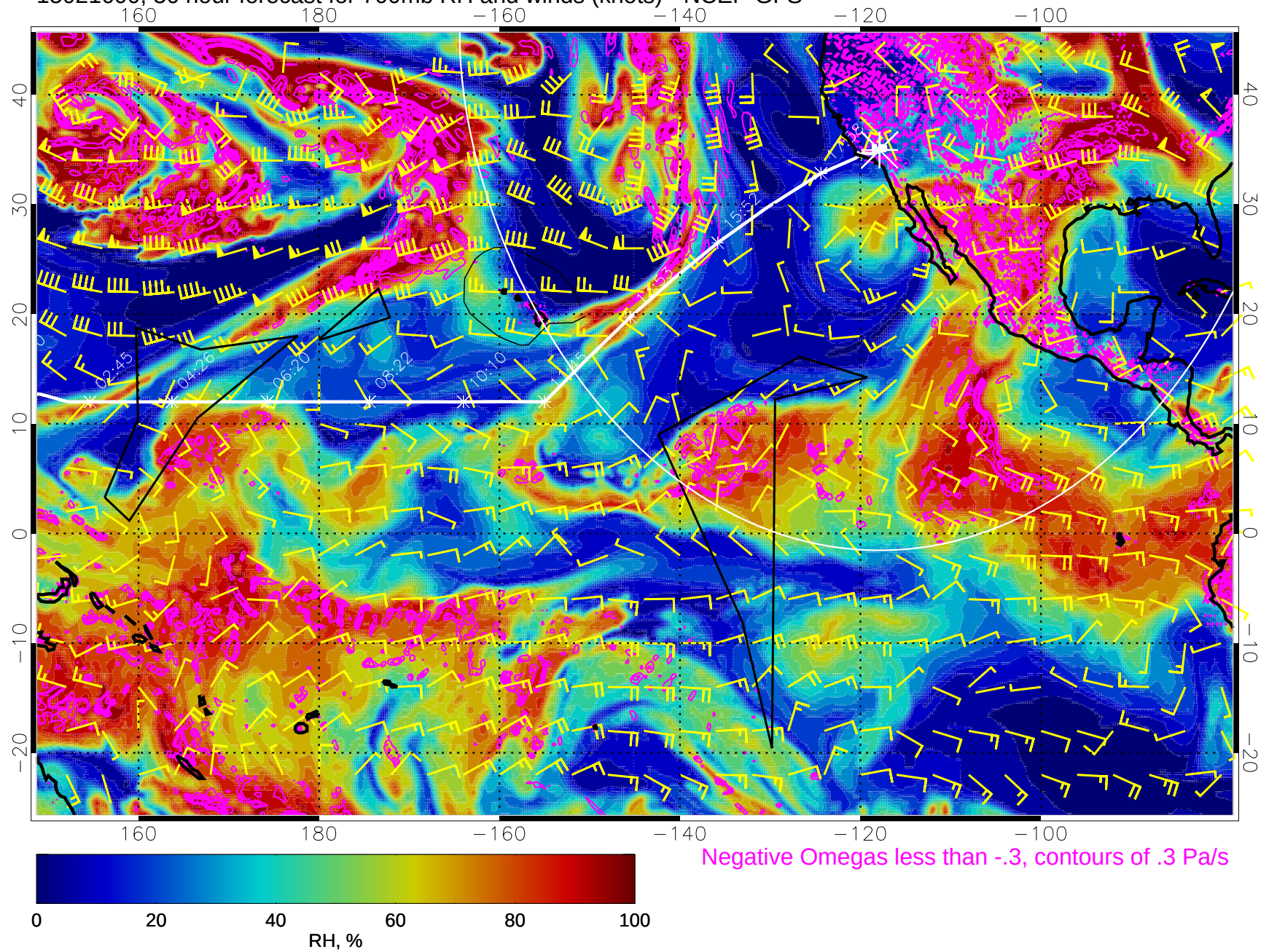
15021600, 36 hour forecast for 700mb RH and winds (knots) - NCEP GFS
