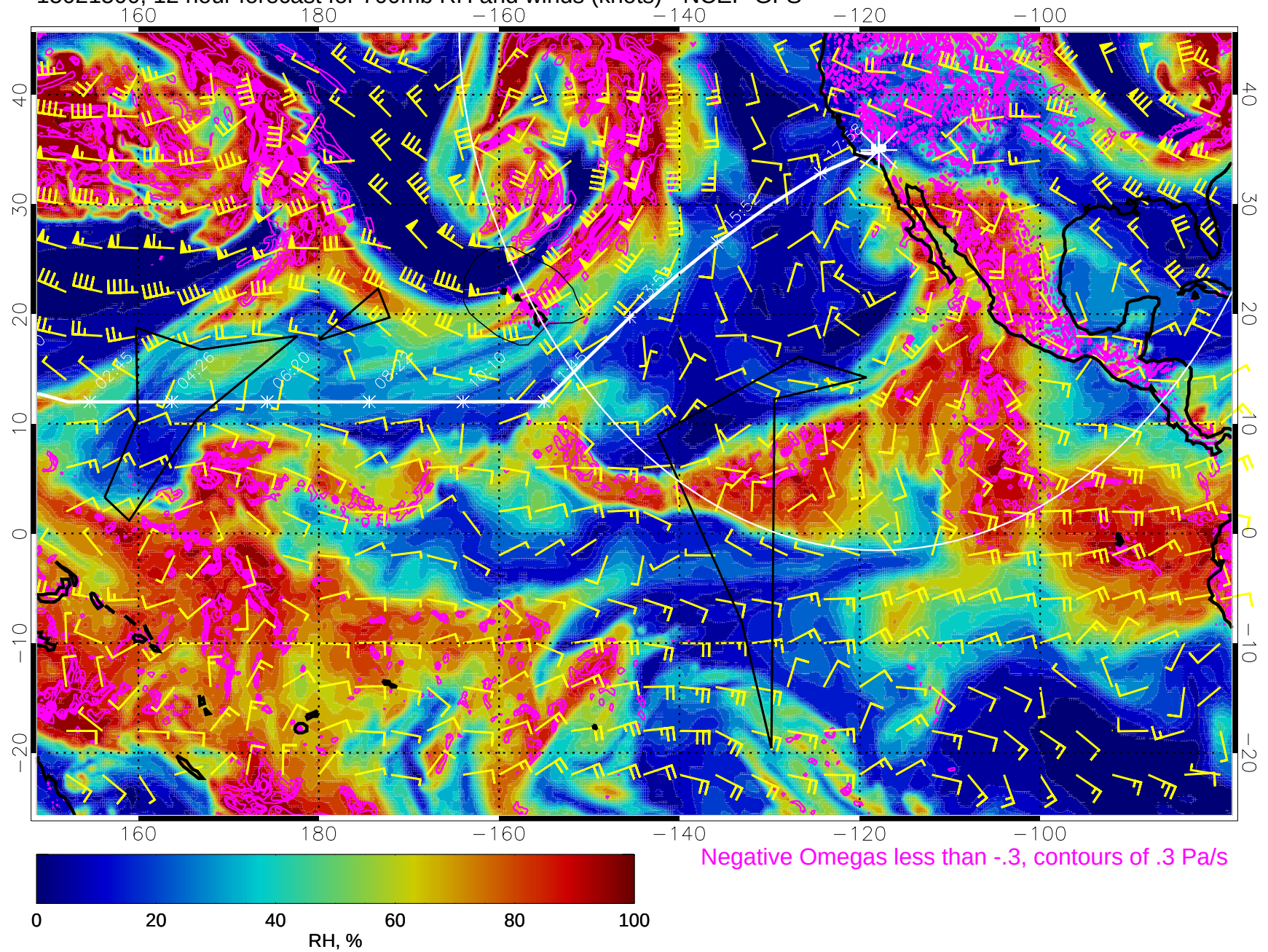
15021500, 12 hour forecast for 700mb RH and winds (knots) - NCEP GFS
