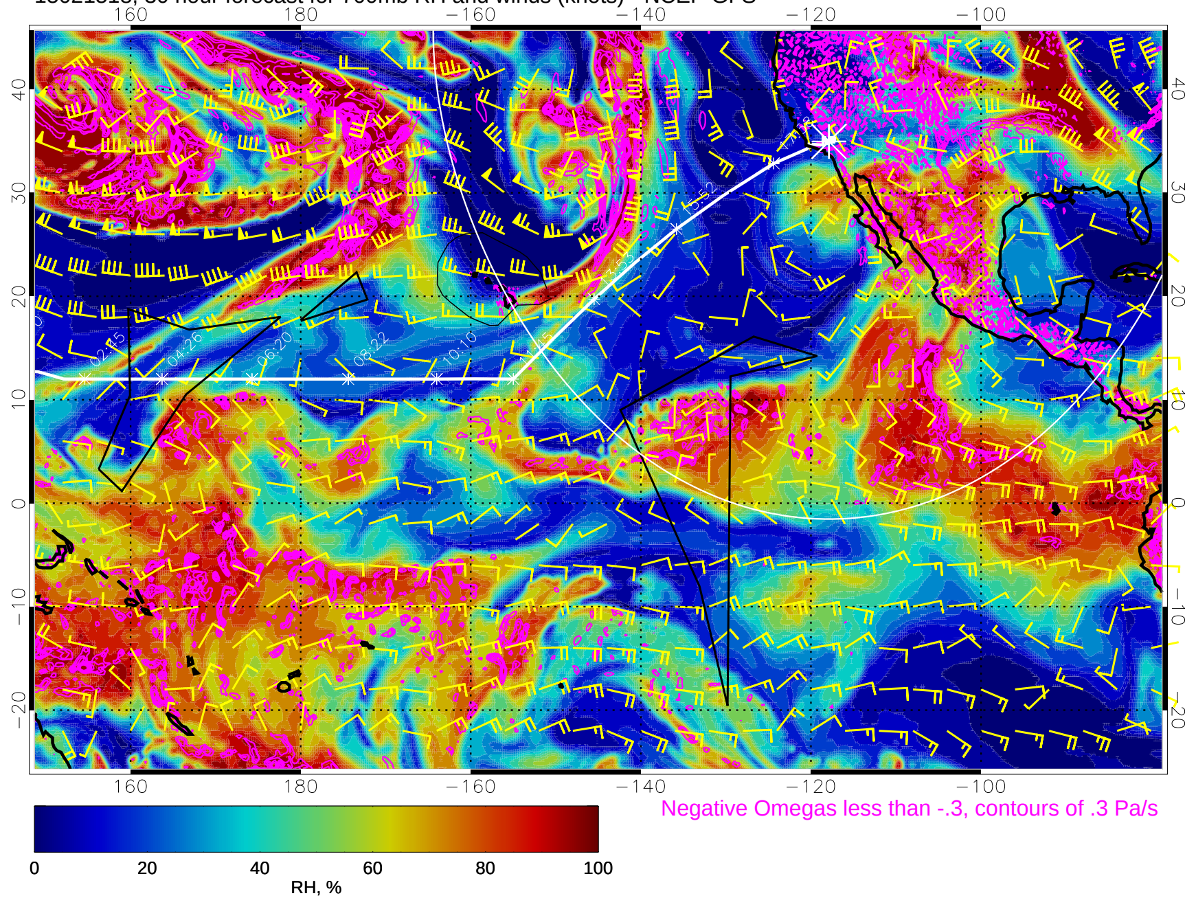
15021518, 30 hour forecast for 700mb RH and winds (knots) - NCEP GFS
