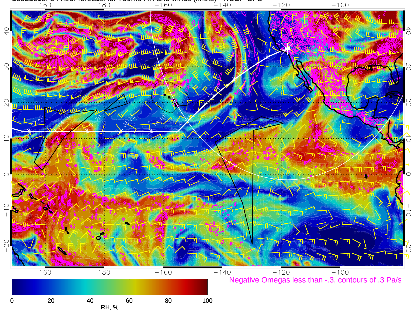
15021618, 54 hour forecast for 700mb RH and winds (knots) - NCEP GFS
