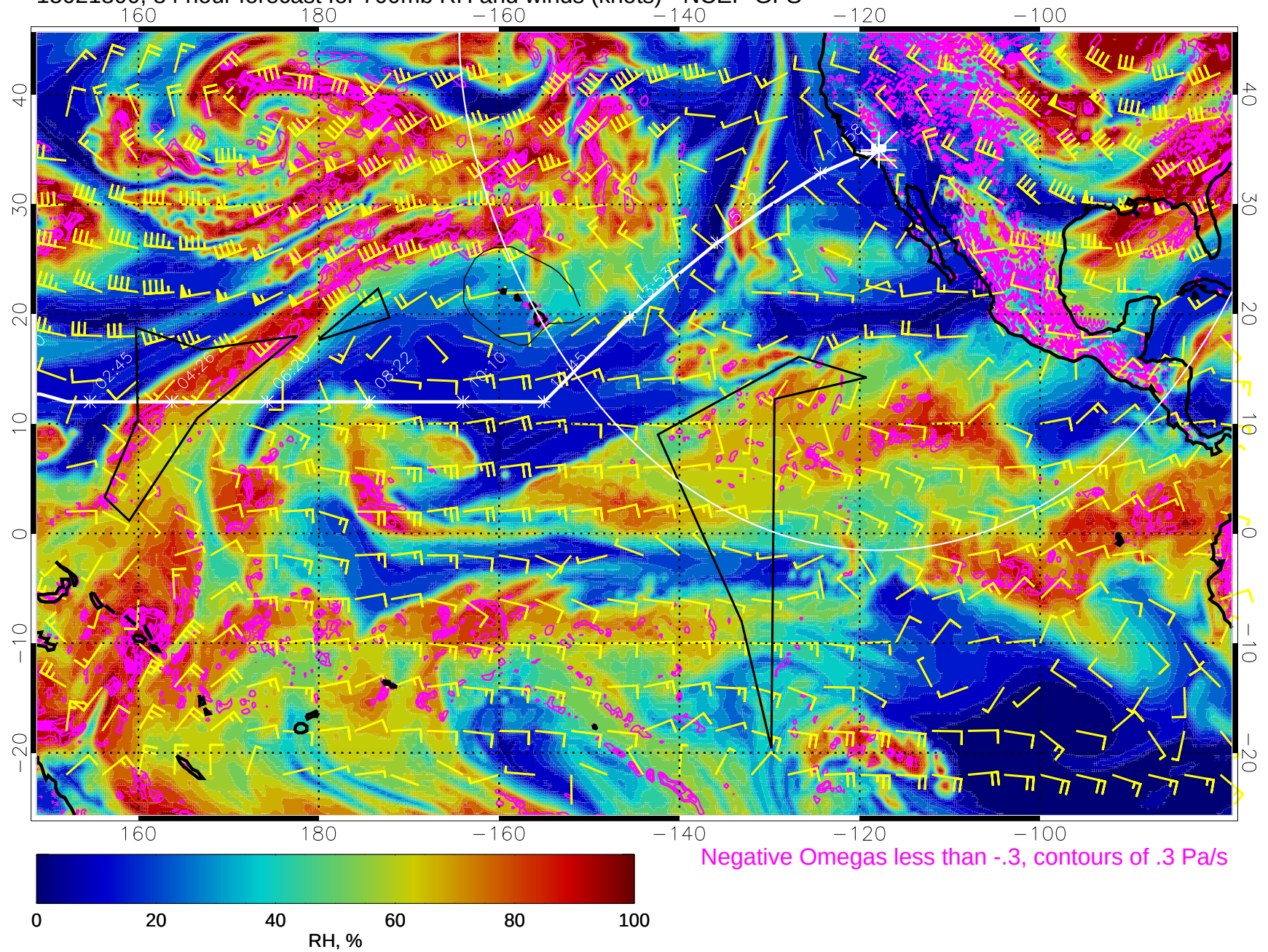
15021800, 84 hour forecast for 700mb RH and winds (knots) - NCEP GFS
