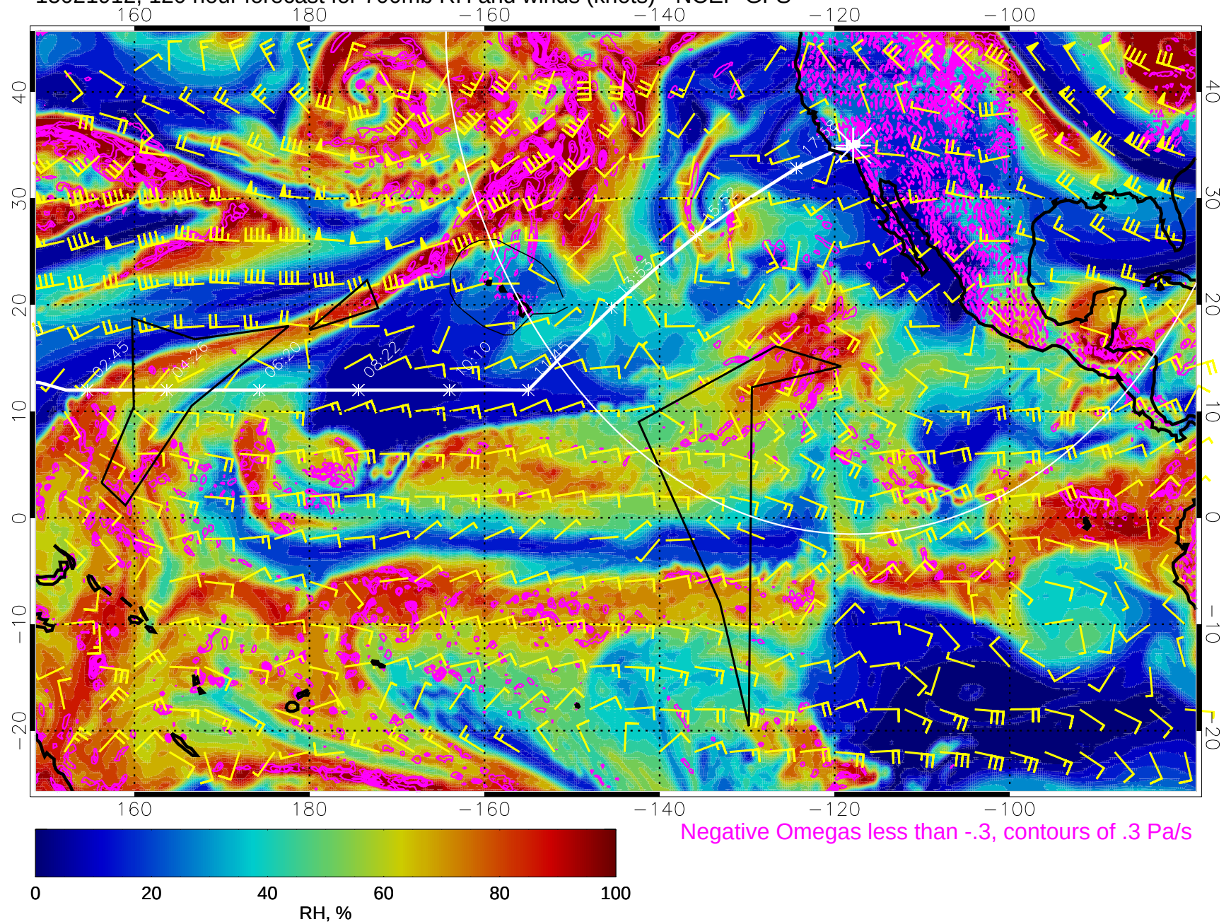
15021912, 120 hour forecast for 700mb RH and winds (knots) - NCEP GFS
