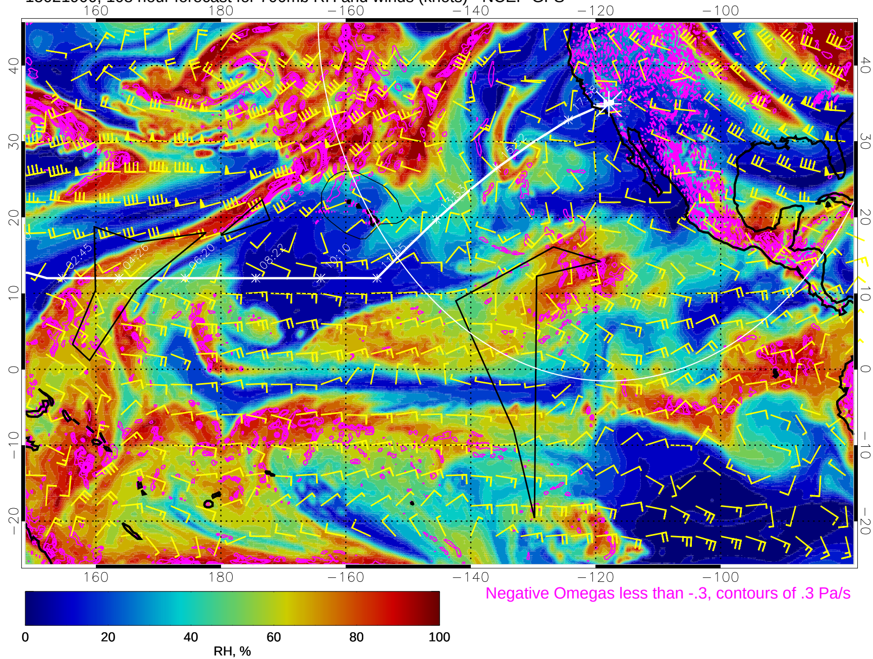
15021900, 108 hour forecast for 700mb RH and winds (knots) - NCEP GFS
