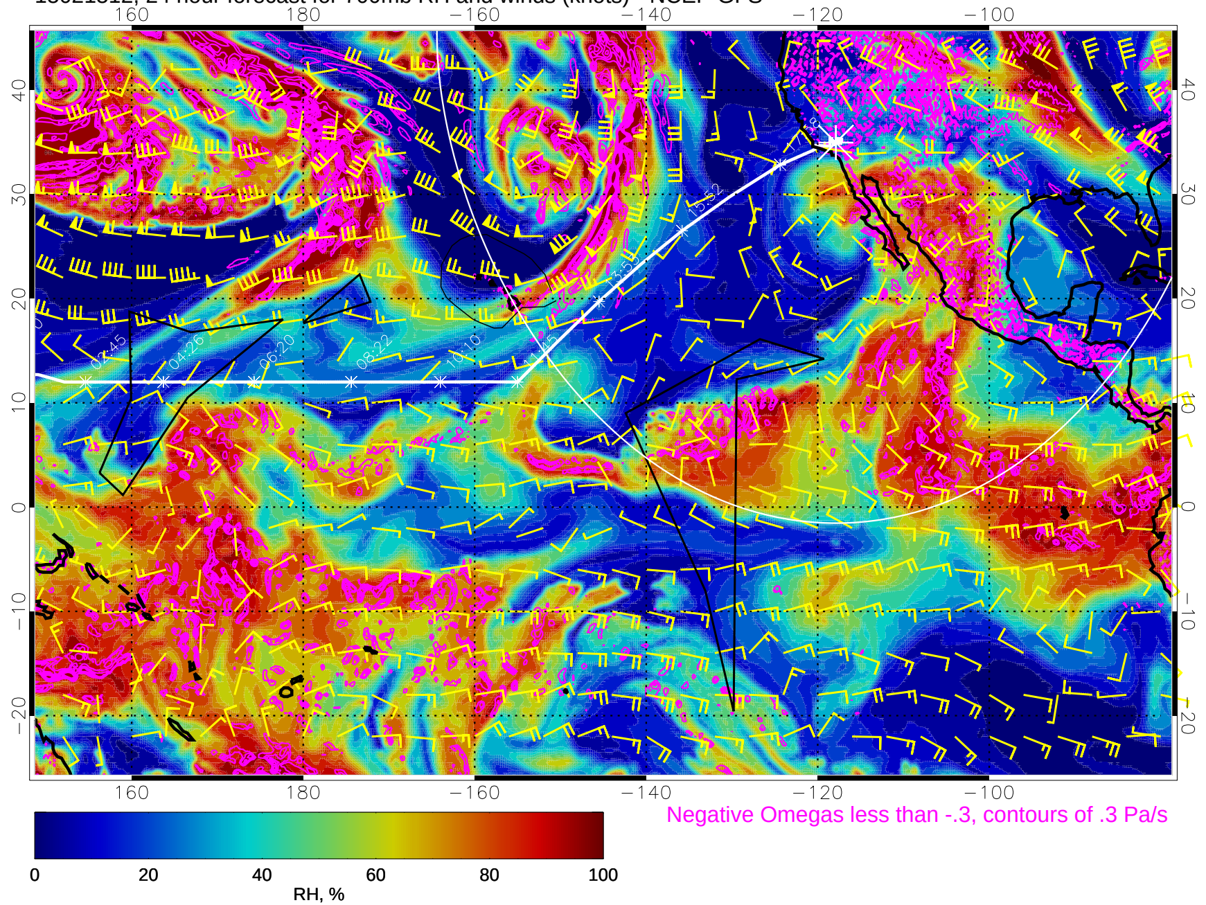
15021512, 24 hour forecast for 700mb RH and winds (knots) - NCEP GFS
