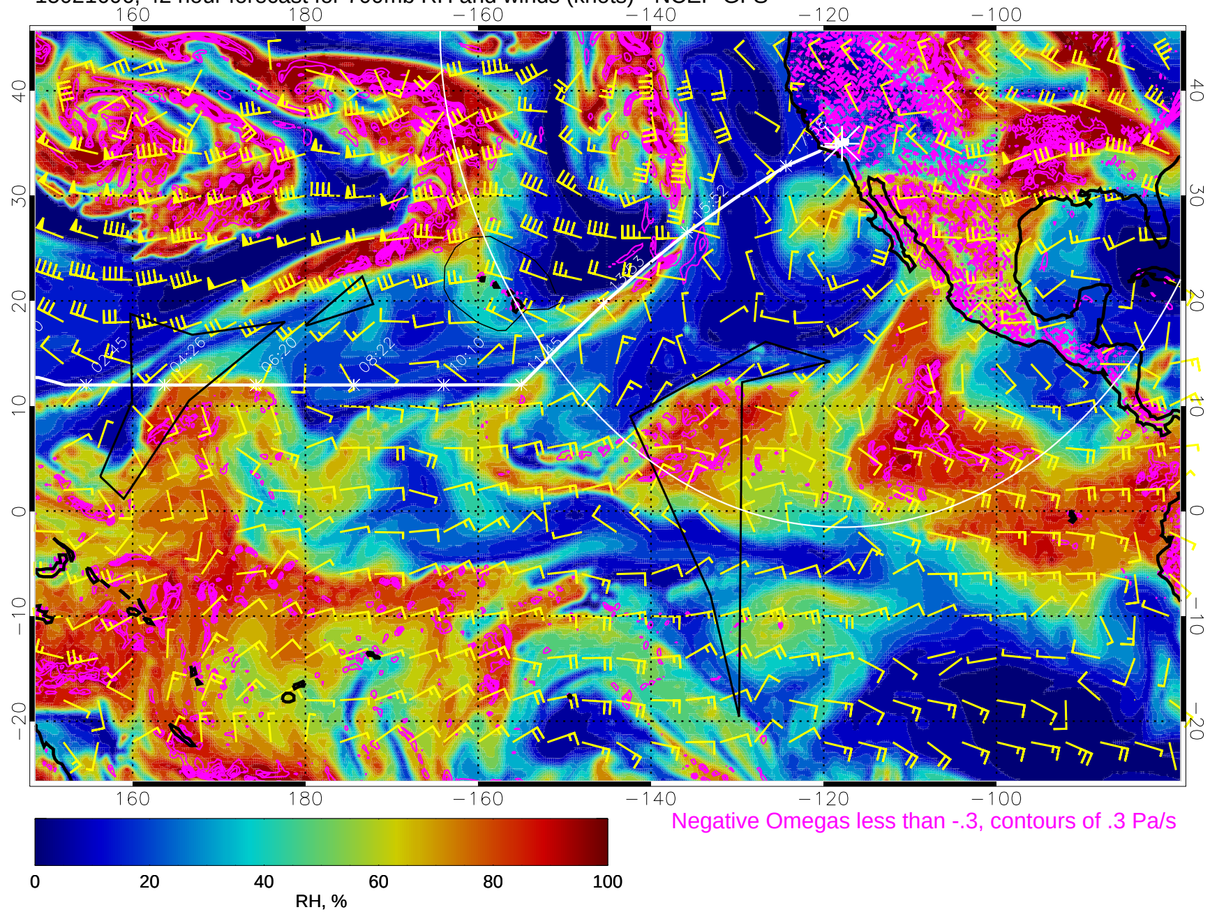
15021606, 42 hour forecast for 700mb RH and winds (knots) - NCEP GFS
