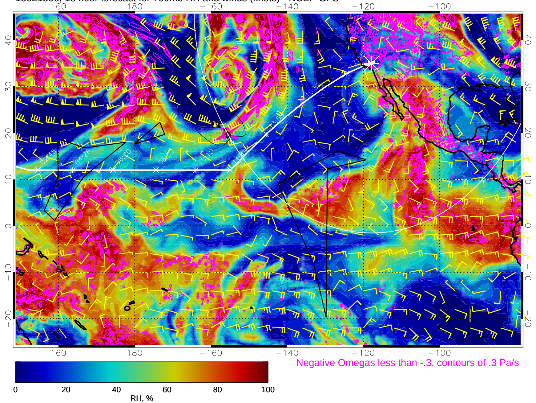
15021506, 18 hour forecast for 700mb RH and winds (knots) - NCEP GFS
