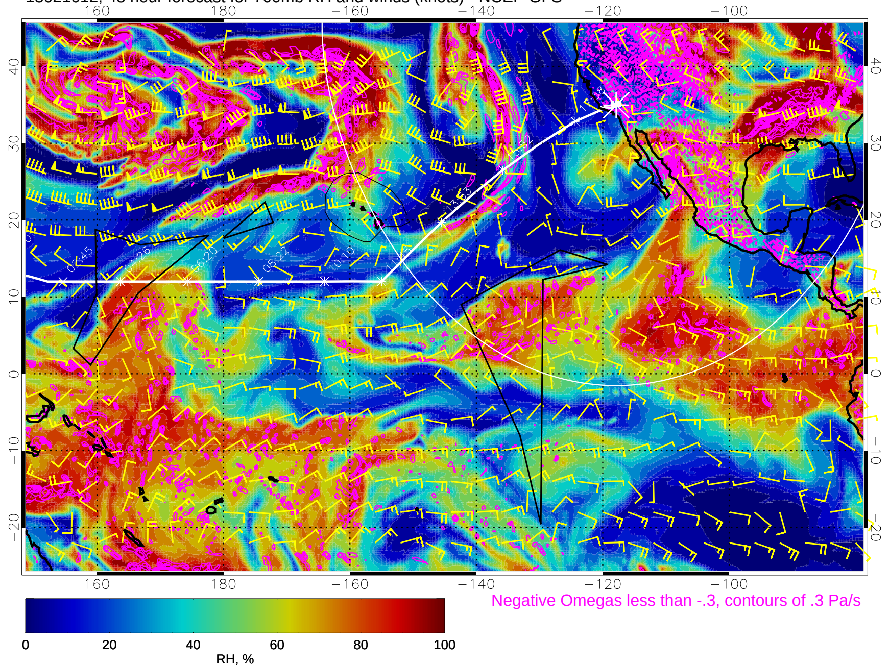
15021612, 48 hour forecast for 700mb RH and winds (knots) - NCEP GFS
