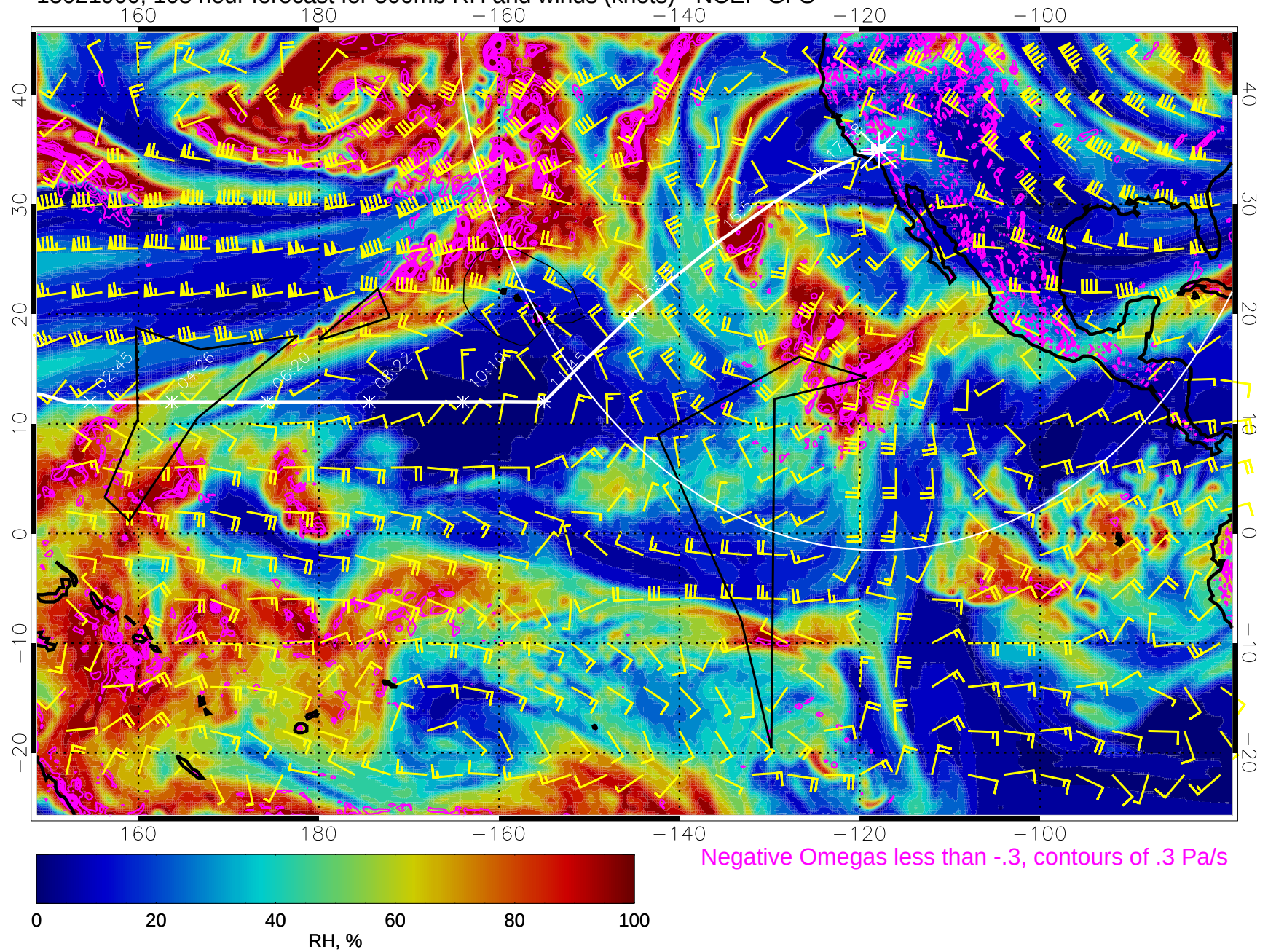
15021900, 108 hour forecast for 500mb RH and winds (knots) - NCEP GFS
