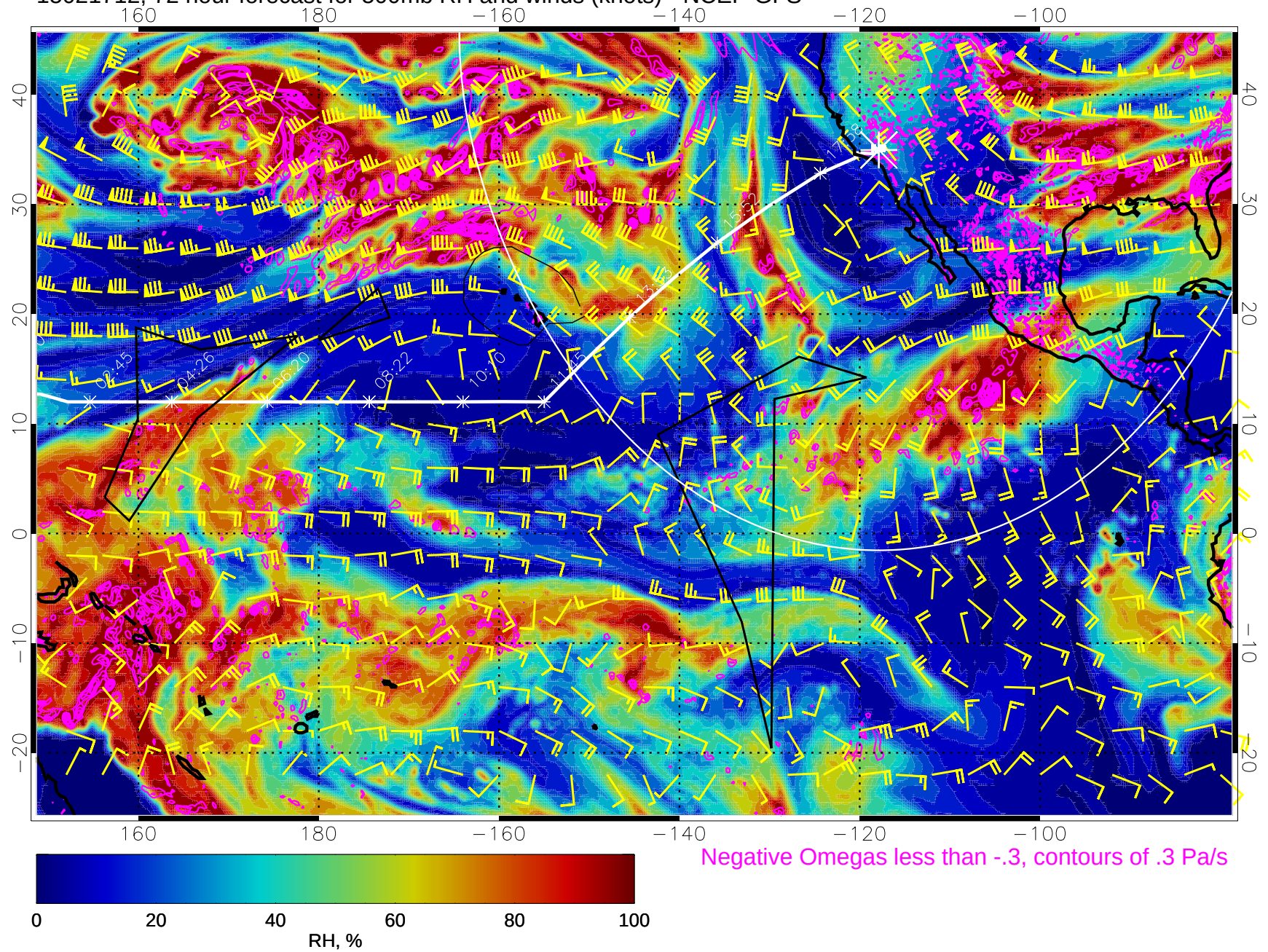
15021712, 72 hour forecast for 500mb RH and winds (knots) - NCEP GFS
