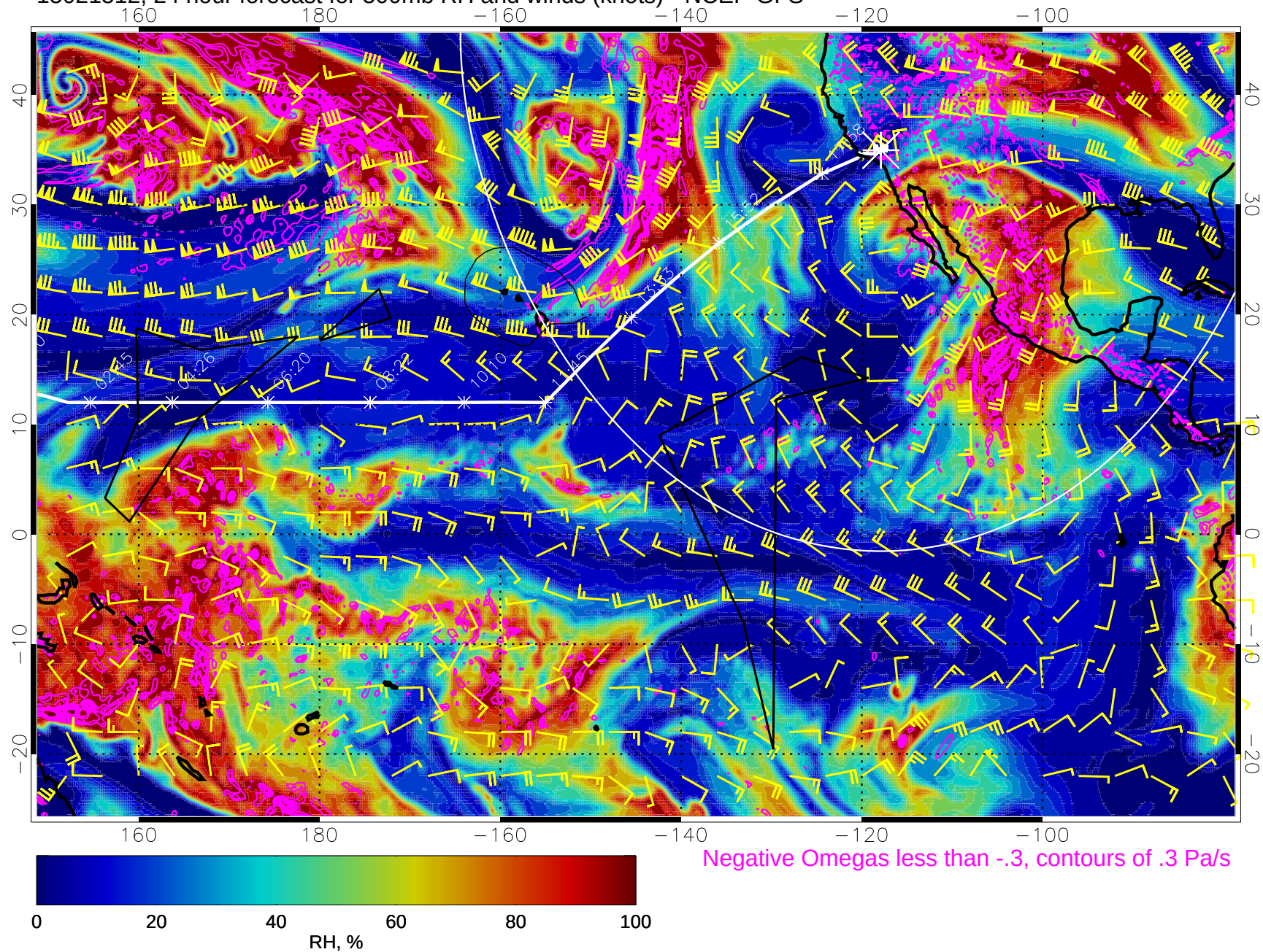
15021512, 24 hour forecast for 500mb RH and winds (knots) - NCEP GFS
