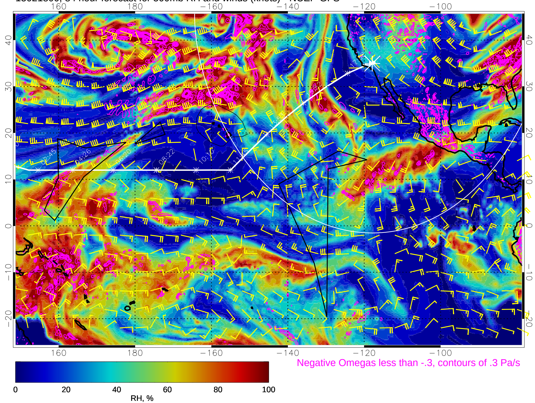
15021800, 84 hour forecast for 500mb RH and winds (knots) - NCEP GFS
