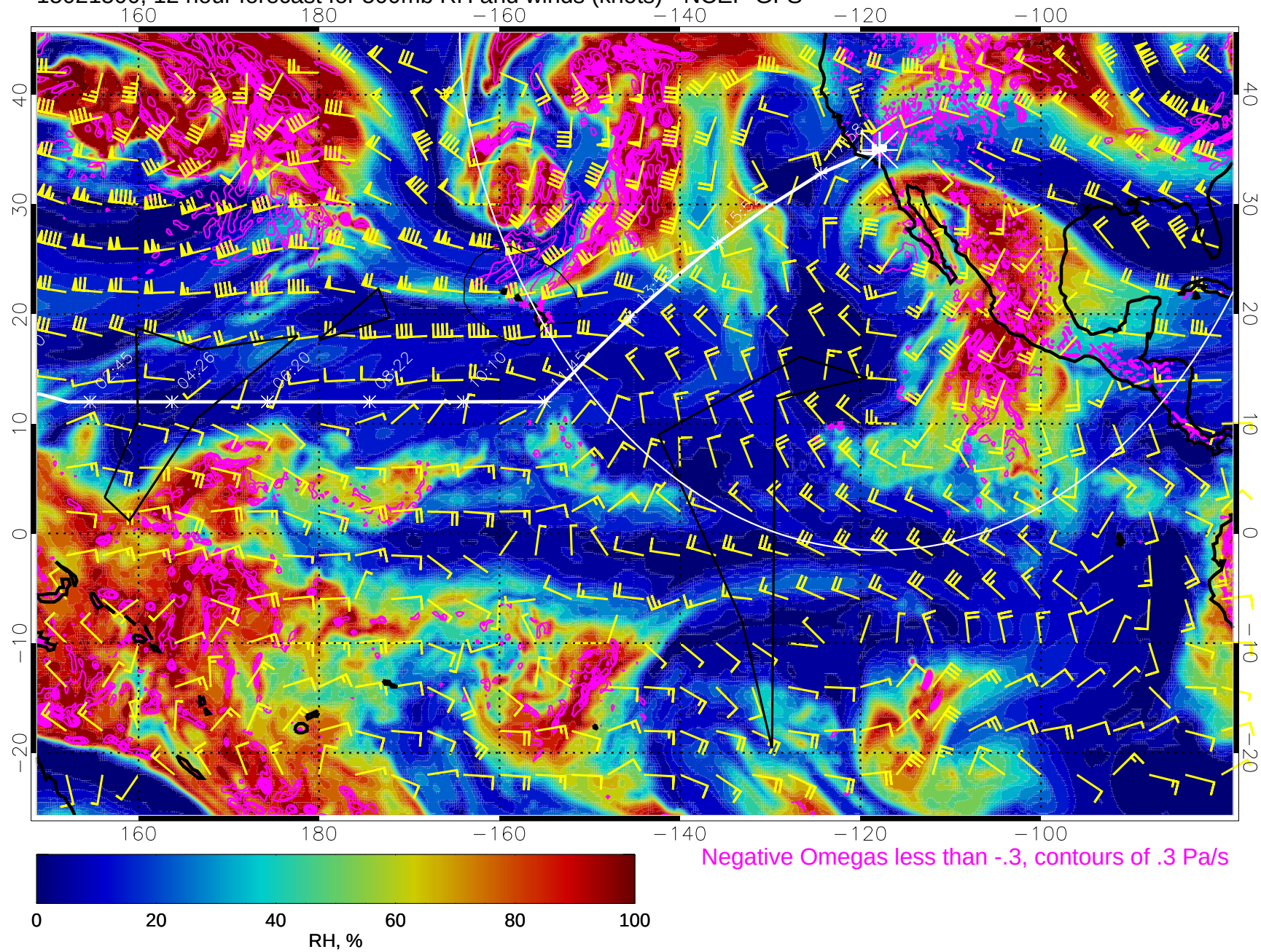
15021500, 12 hour forecast for 500mb RH and winds (knots) - NCEP GFS
