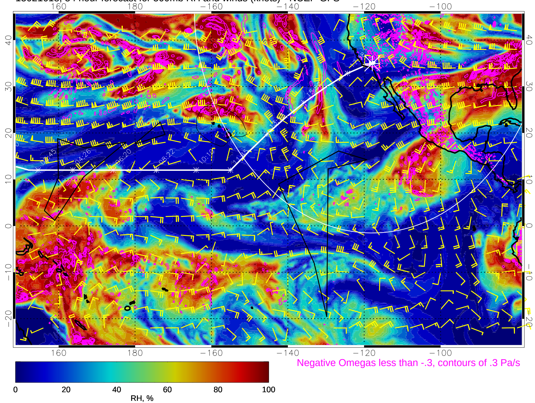
15021618, 54 hour forecast for 500mb RH and winds (knots) - NCEP GFS
