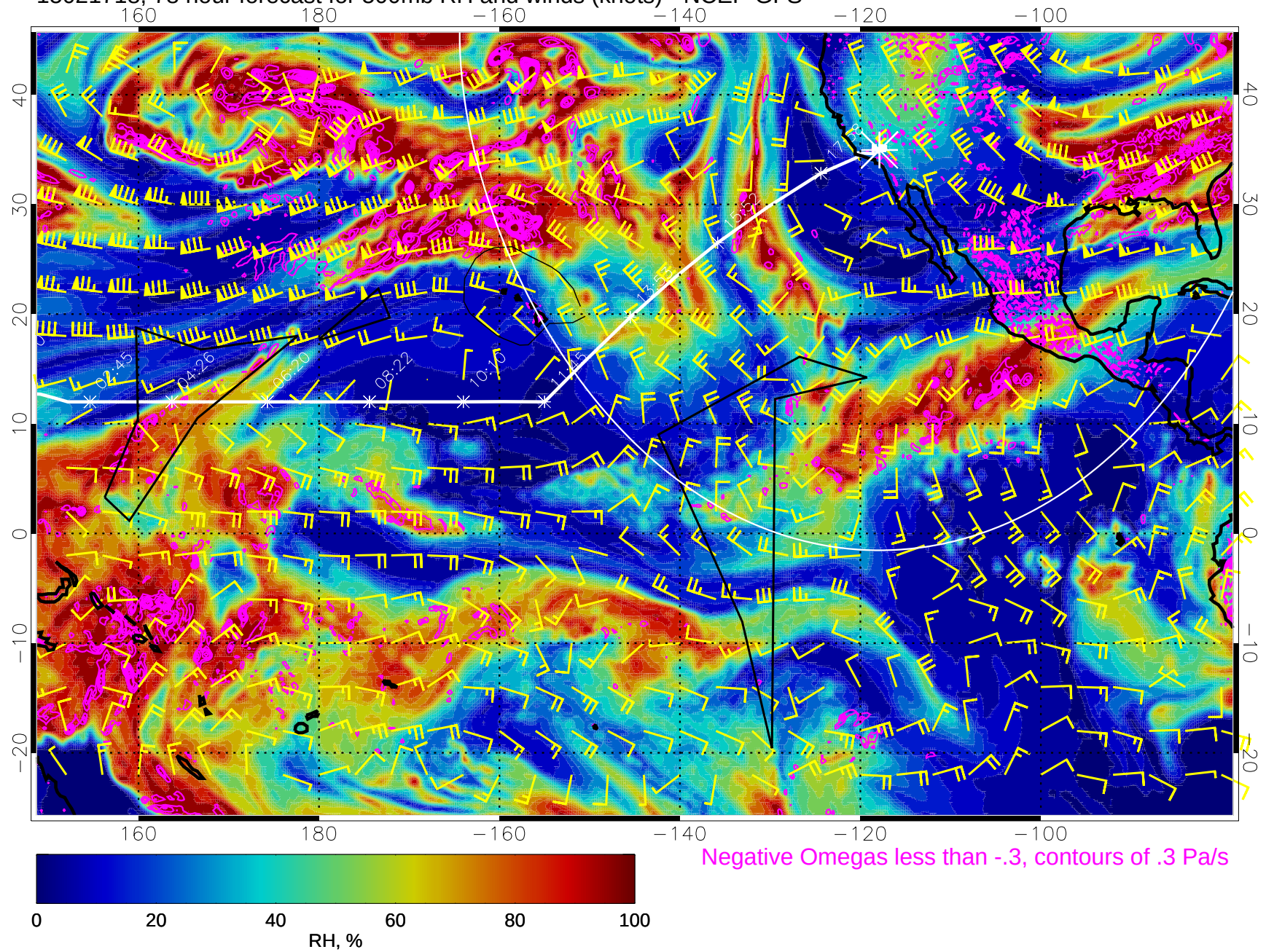
15021718, 78 hour forecast for 500mb RH and winds (knots) - NCEP GFS
