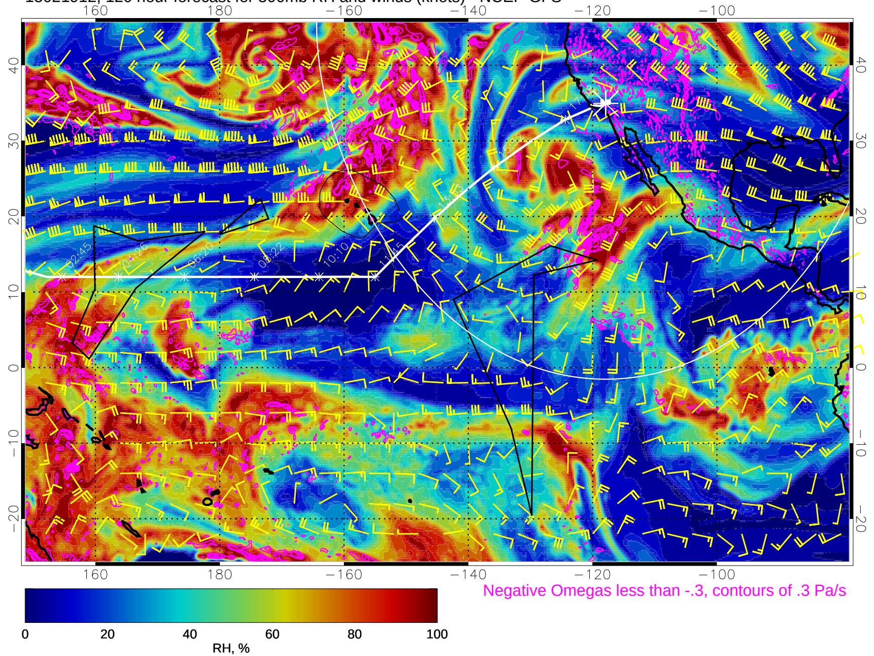
15021912, 120 hour forecast for 500mb RH and winds (knots) - NCEP GFS
