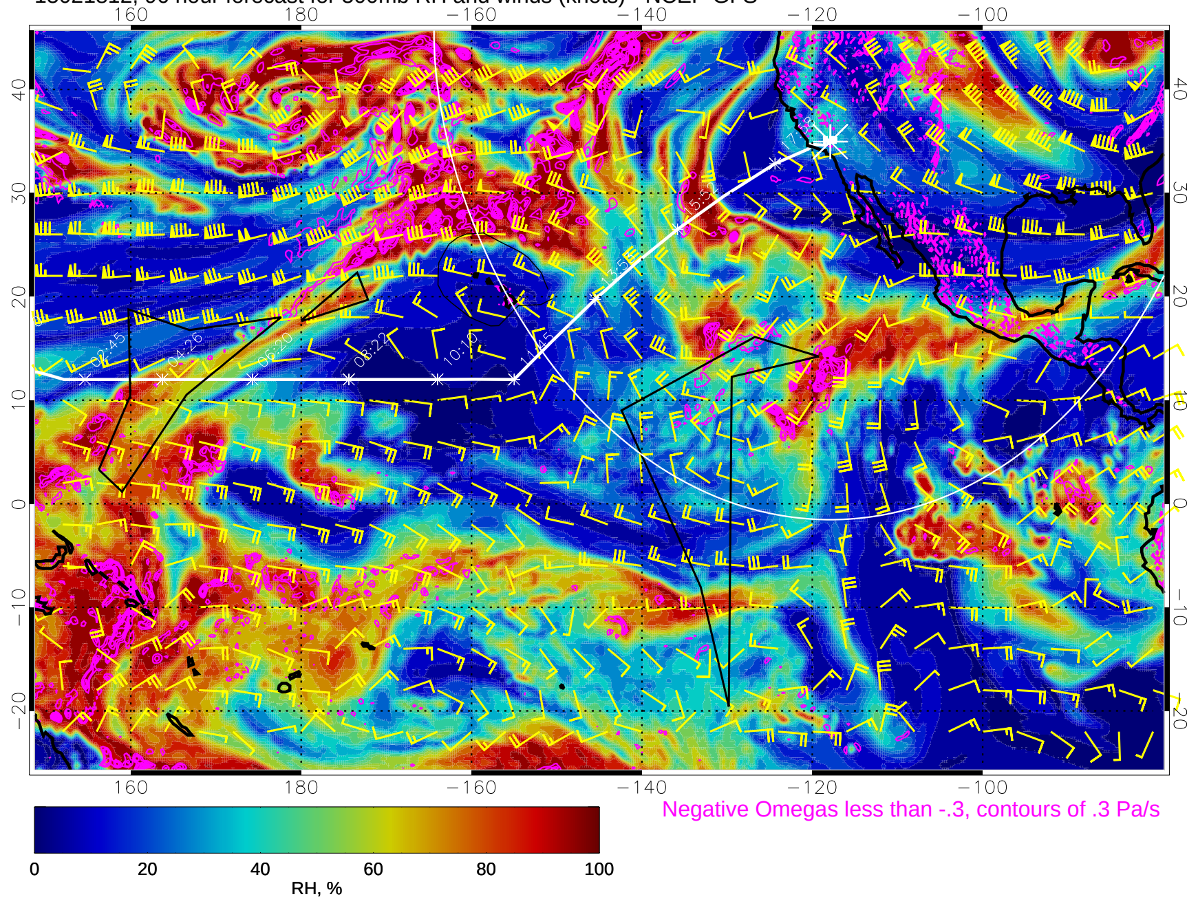
15021812, 96 hour forecast for 500mb RH and winds (knots) - NCEP GFS
