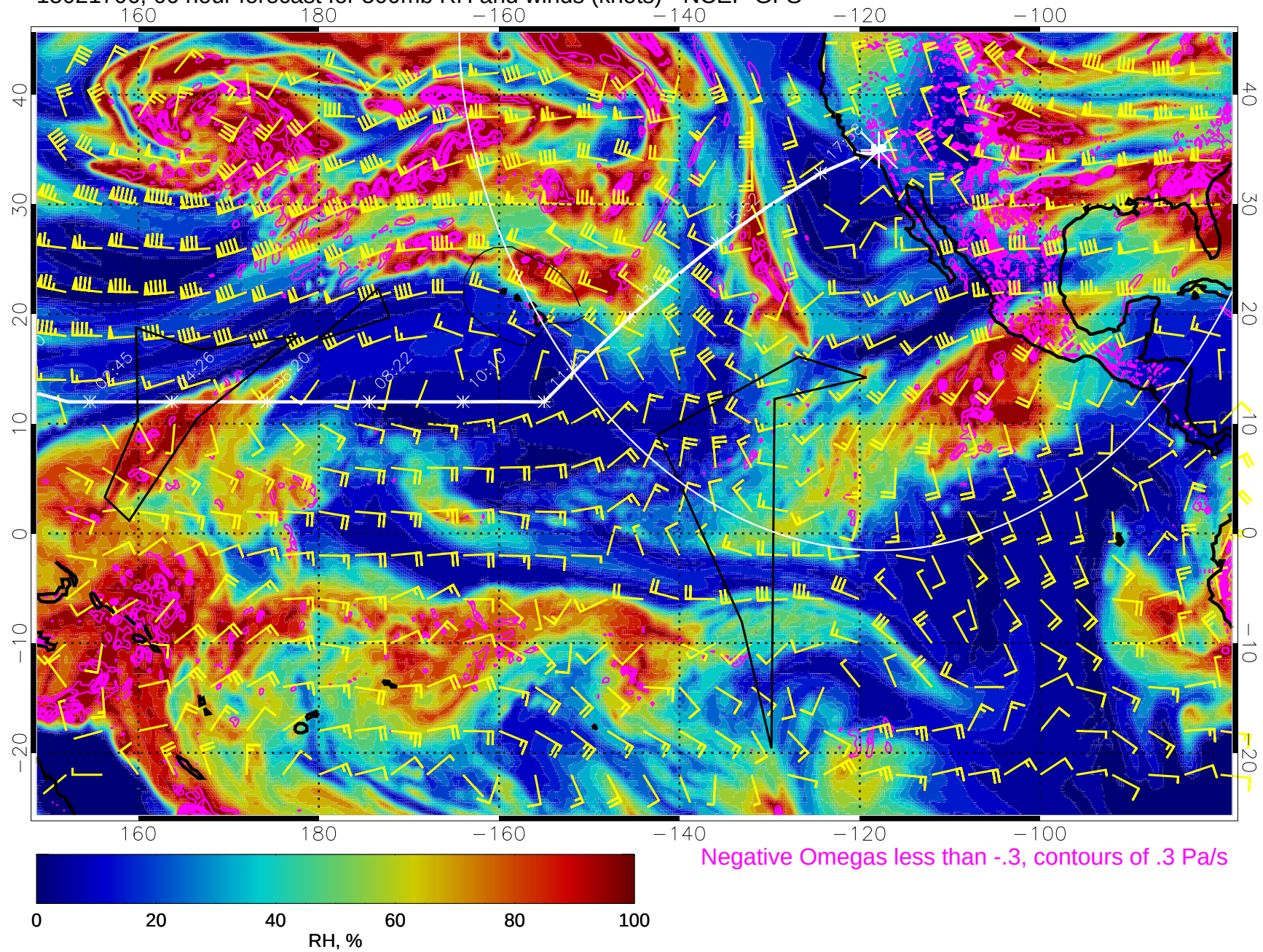
15021706, 66 hour forecast for 500mb RH and winds (knots) - NCEP GFS
