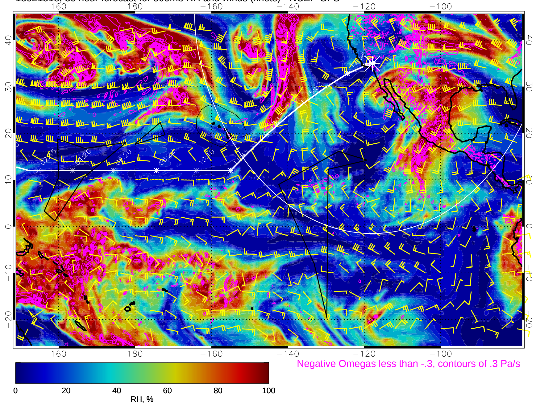
15021518, 30 hour forecast for 500mb RH and winds (knots) - NCEP GFS
