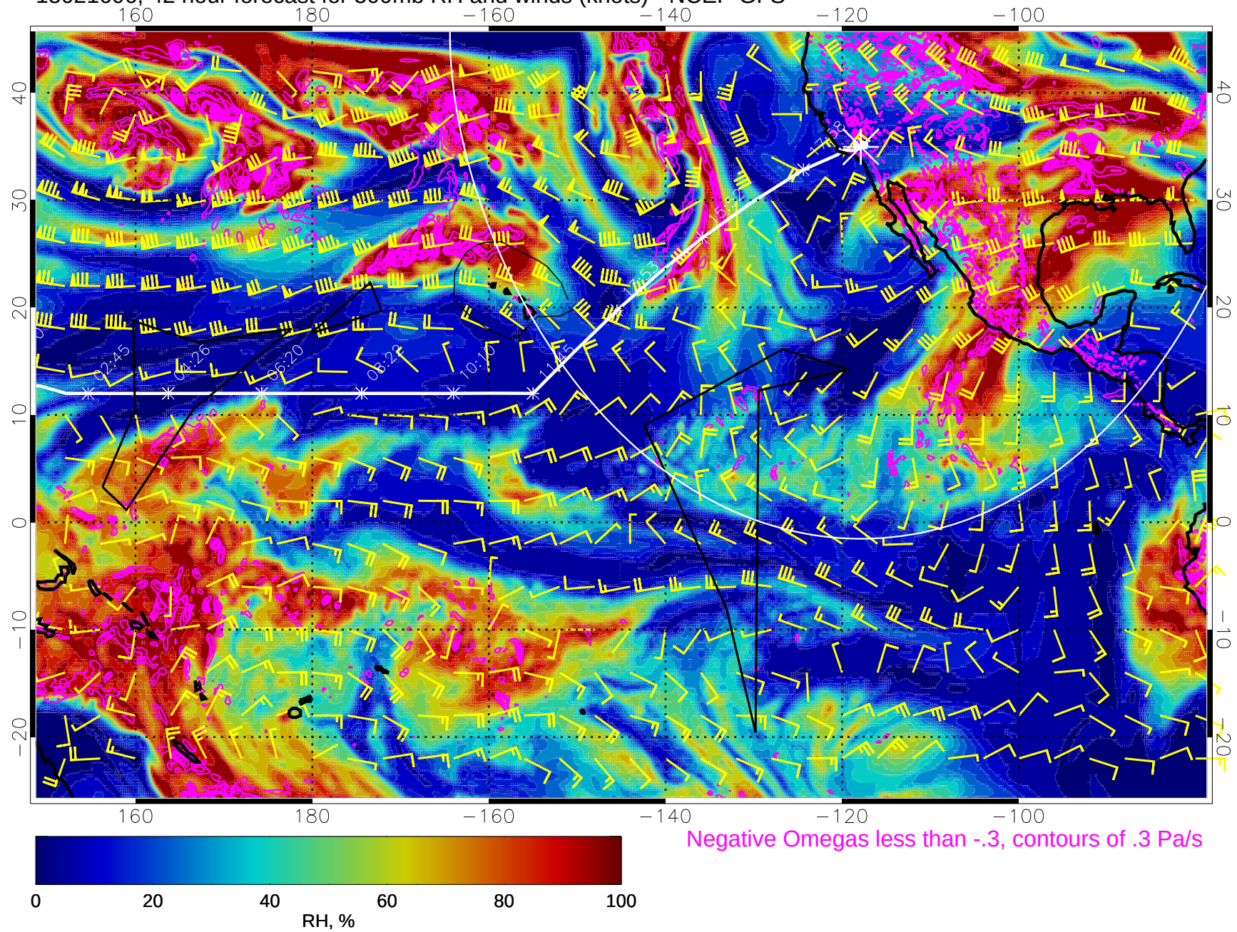
15021606, 42 hour forecast for 500mb RH and winds (knots) - NCEP GFS
