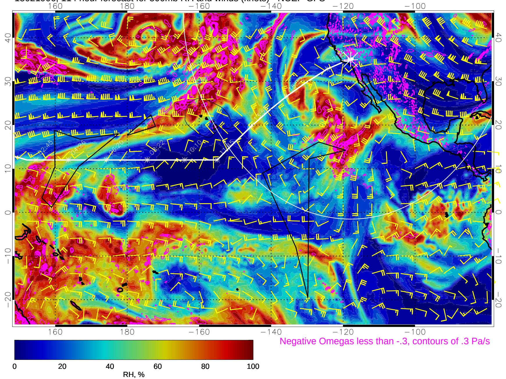
15021906, 114 hour forecast for 500mb RH and winds (knots) - NCEP GFS
