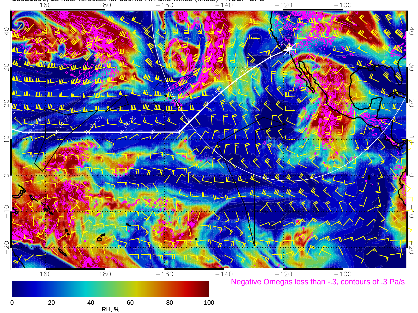
15021506, 18 hour forecast for 500mb RH and winds (knots) - NCEP GFS
