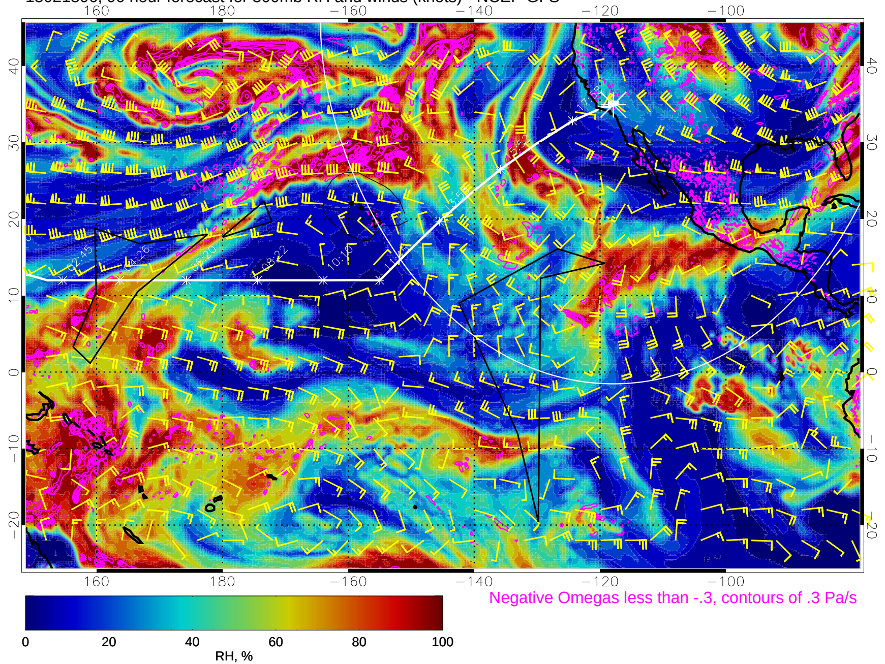
15021806, 90 hour forecast for 500mb RH and winds (knots) - NCEP GFS
