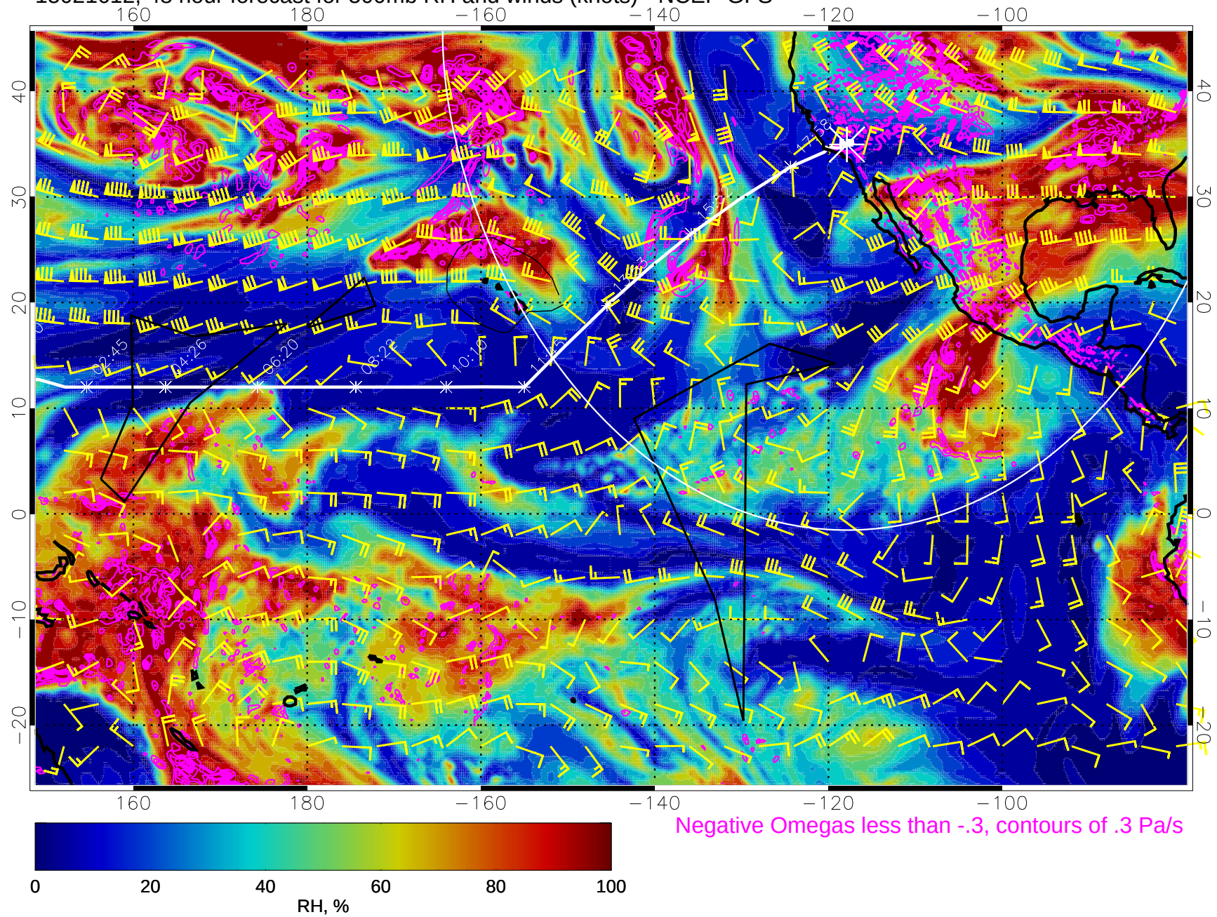
15021612, 48 hour forecast for 500mb RH and winds (knots) - NCEP GFS
