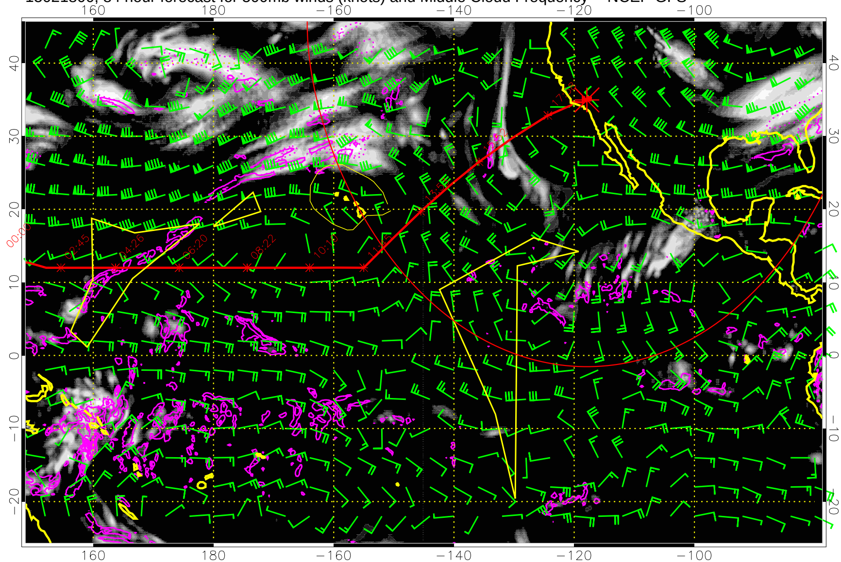
15021800, 84 hour forecast for 500mb winds (knots) and Middle Cloud Frequency -- NCEP GFS
