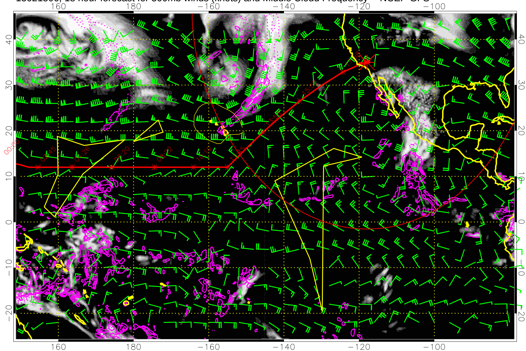
15021506, 18 hour forecast for 500mb winds (knots) and Middle Cloud Frequency -- NCEP GFS
