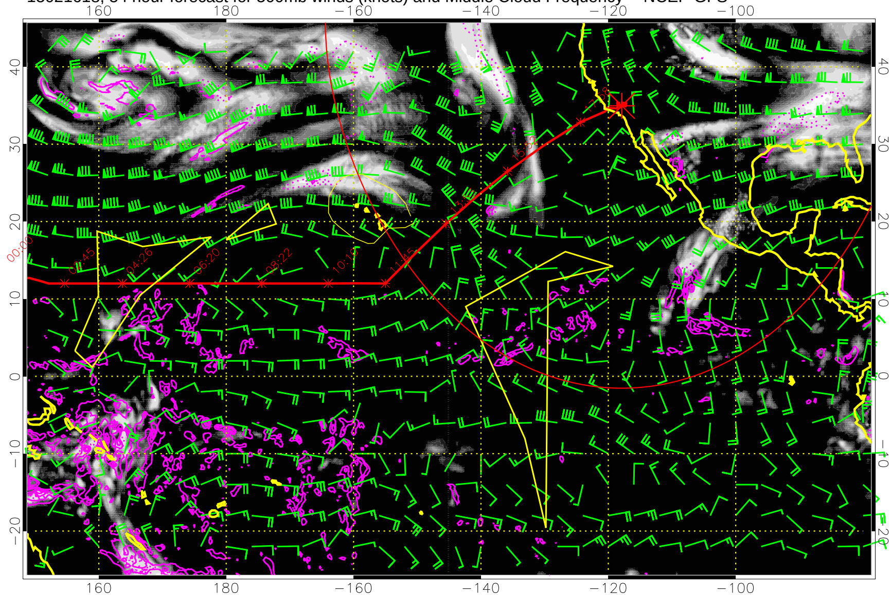
15021618, 54 hour forecast for 500mb winds (knots) and Middle Cloud Frequency -- NCEP GFS
