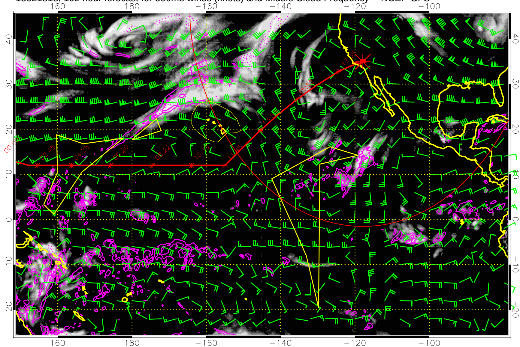
15021818, 102 hour forecast for 500mb winds (knots) and Middle Cloud Frequency -- NCEP GFS
