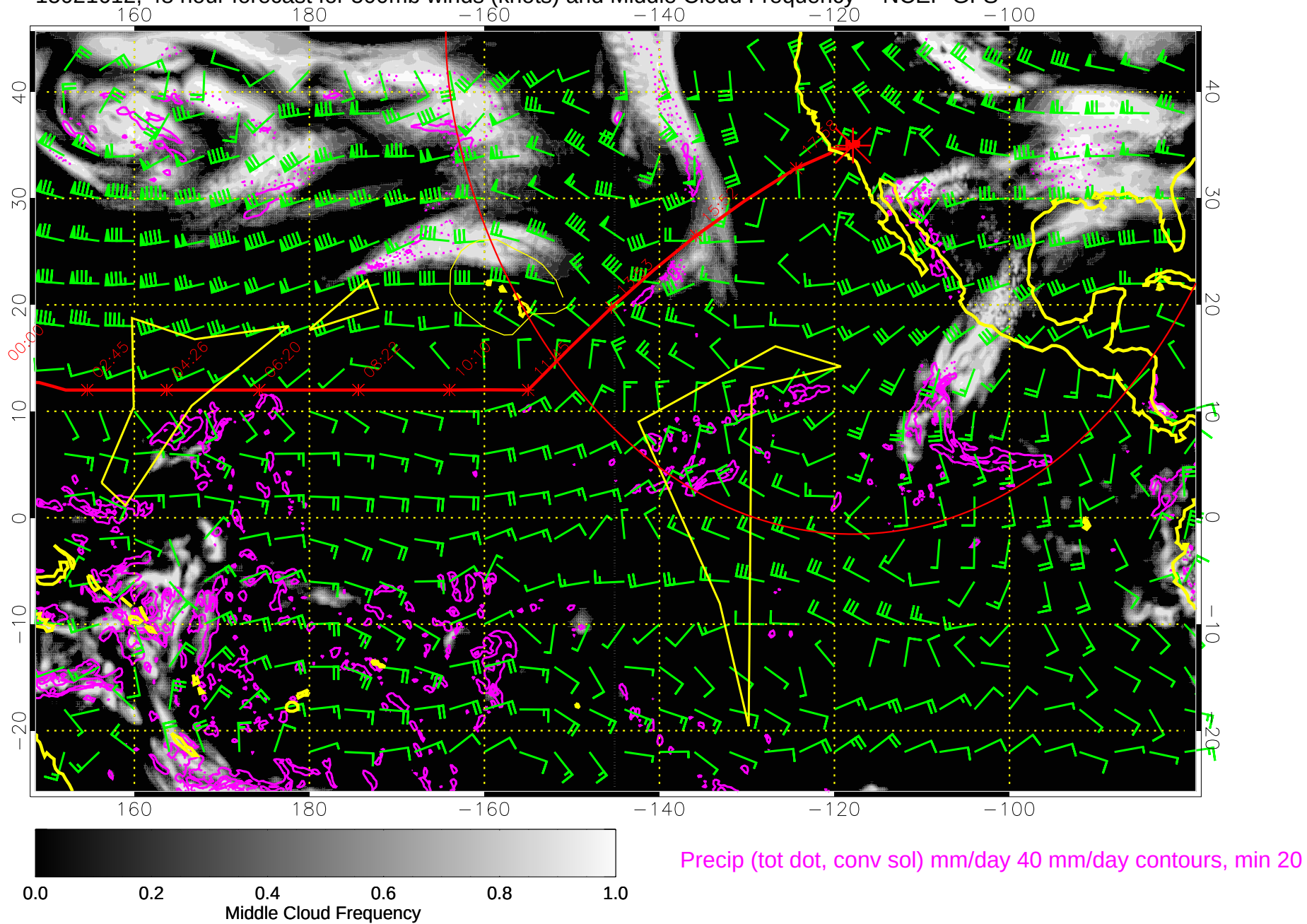
15021612, 48 hour forecast for 500mb winds (knots) and Middle Cloud Frequency -- NCEP GFS
