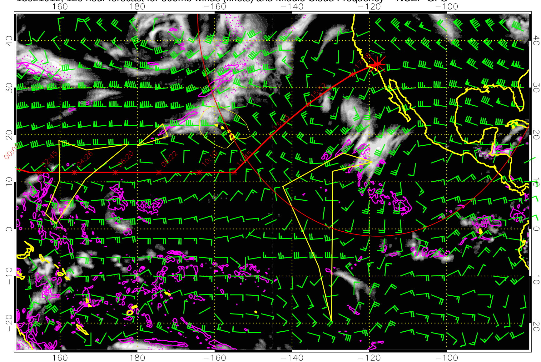
15021912, 120 hour forecast for 500mb winds (knots) and Middle Cloud Frequency -- NCEP GFS
