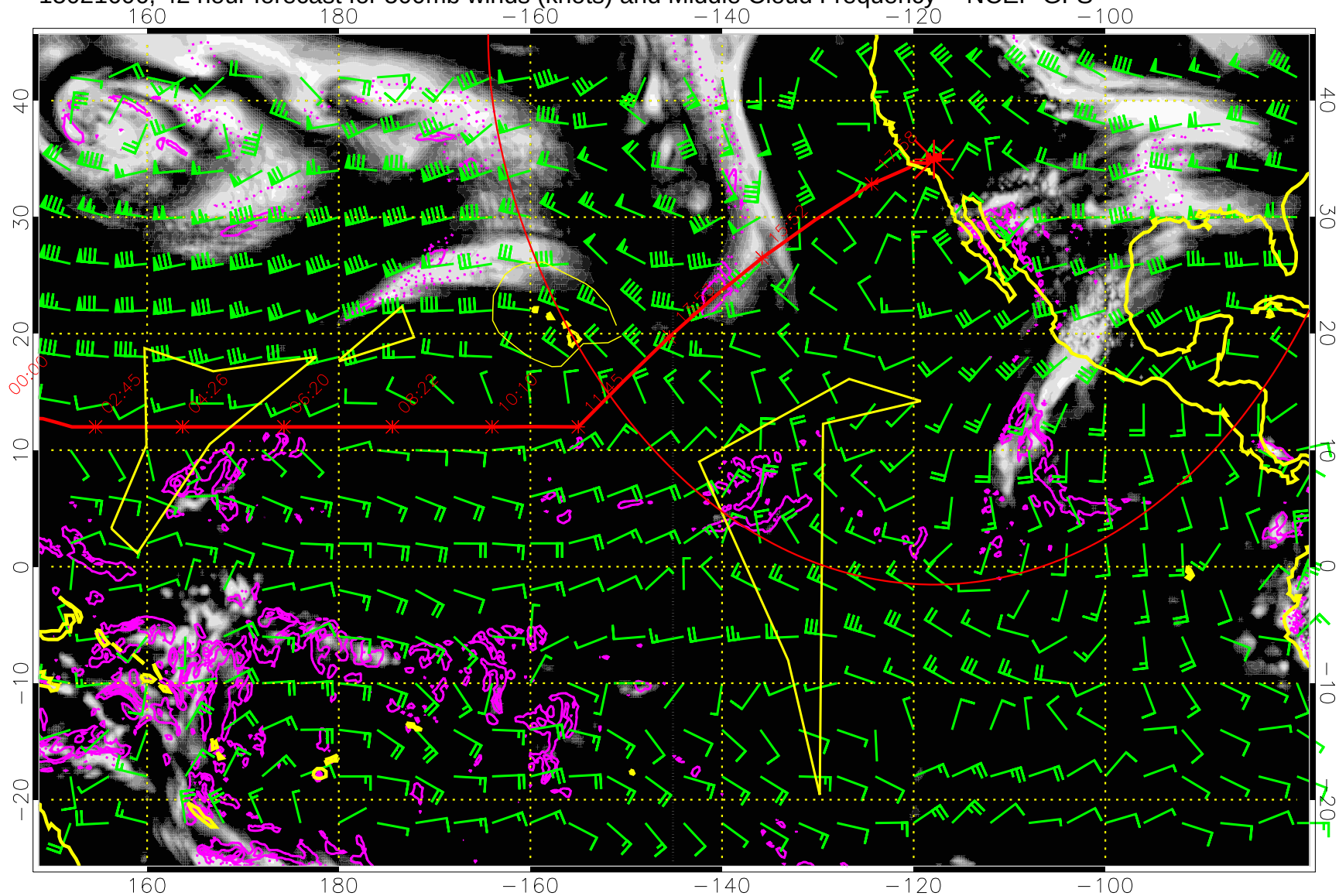
15021606, 42 hour forecast for 500mb winds (knots) and Middle Cloud Frequency -- NCEP GFS
