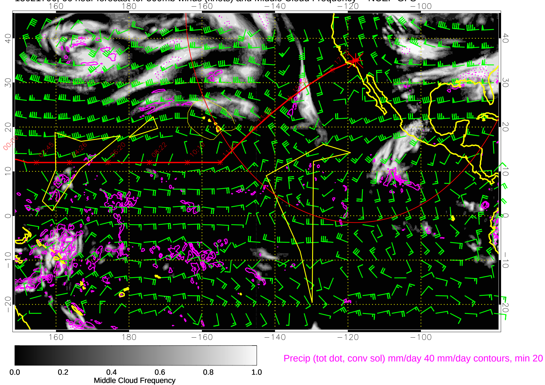
15021706, 66 hour forecast for 500mb winds (knots) and Middle Cloud Frequency -- NCEP GFS
