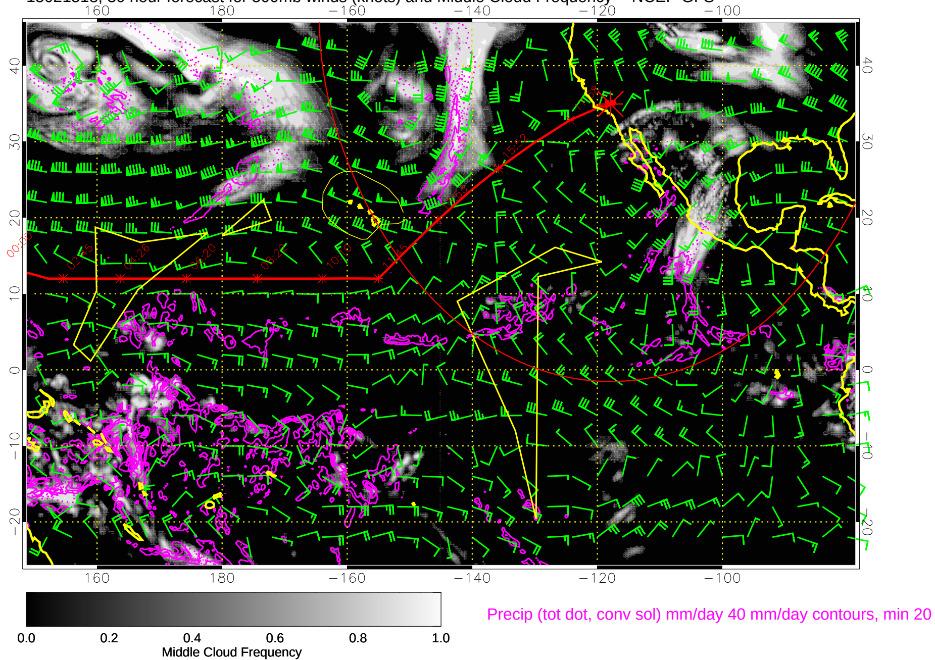
15021518, 30 hour forecast for 500mb winds (knots) and Middle Cloud Frequency -- NCEP GFS
