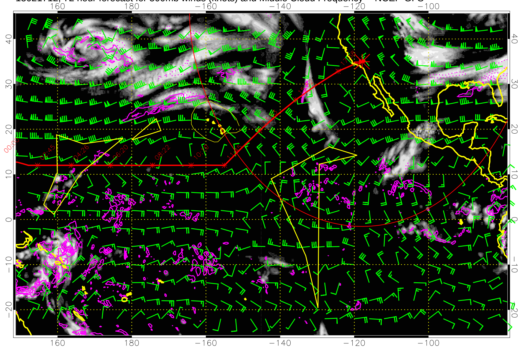
15021712, 72 hour forecast for 500mb winds (knots) and Middle Cloud Frequency -- NCEP GFS
