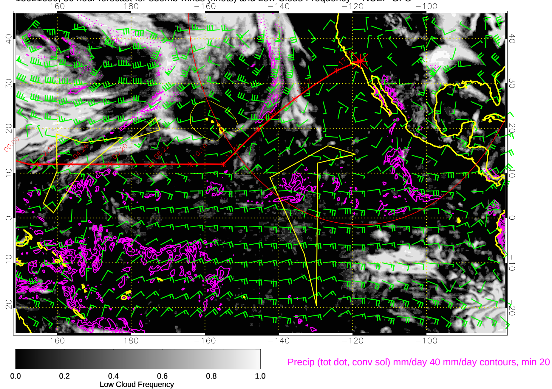
15021600, 36 hour forecast for 850mb winds (knots) and Low Cloud Frequency -- NCEP GFS
