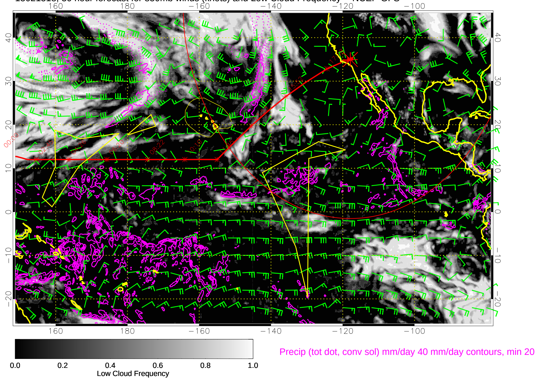
15021518, 30 hour forecast for 850mb winds (knots) and Low Cloud Frequency -- NCEP GFS
