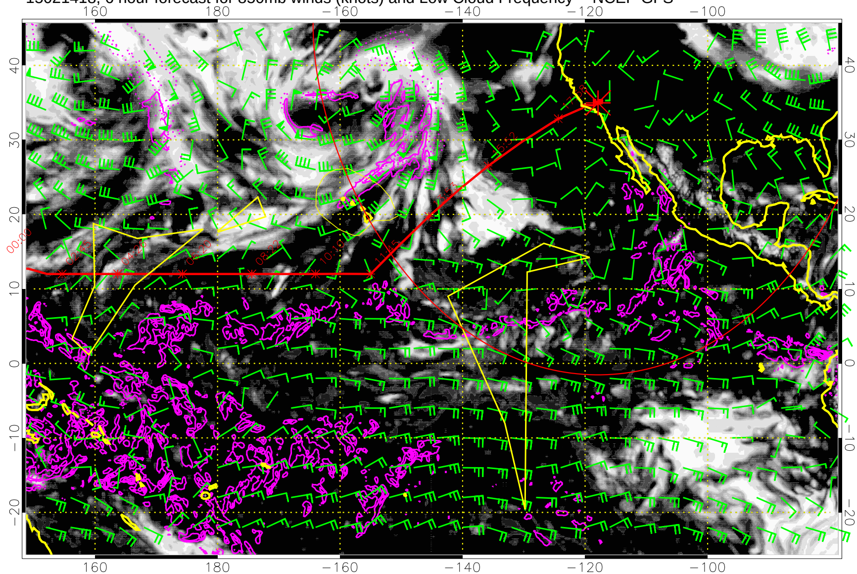
15021418, 6 hour forecast for 850mb winds (knots) and Low Cloud Frequency -- NCEP GFS
