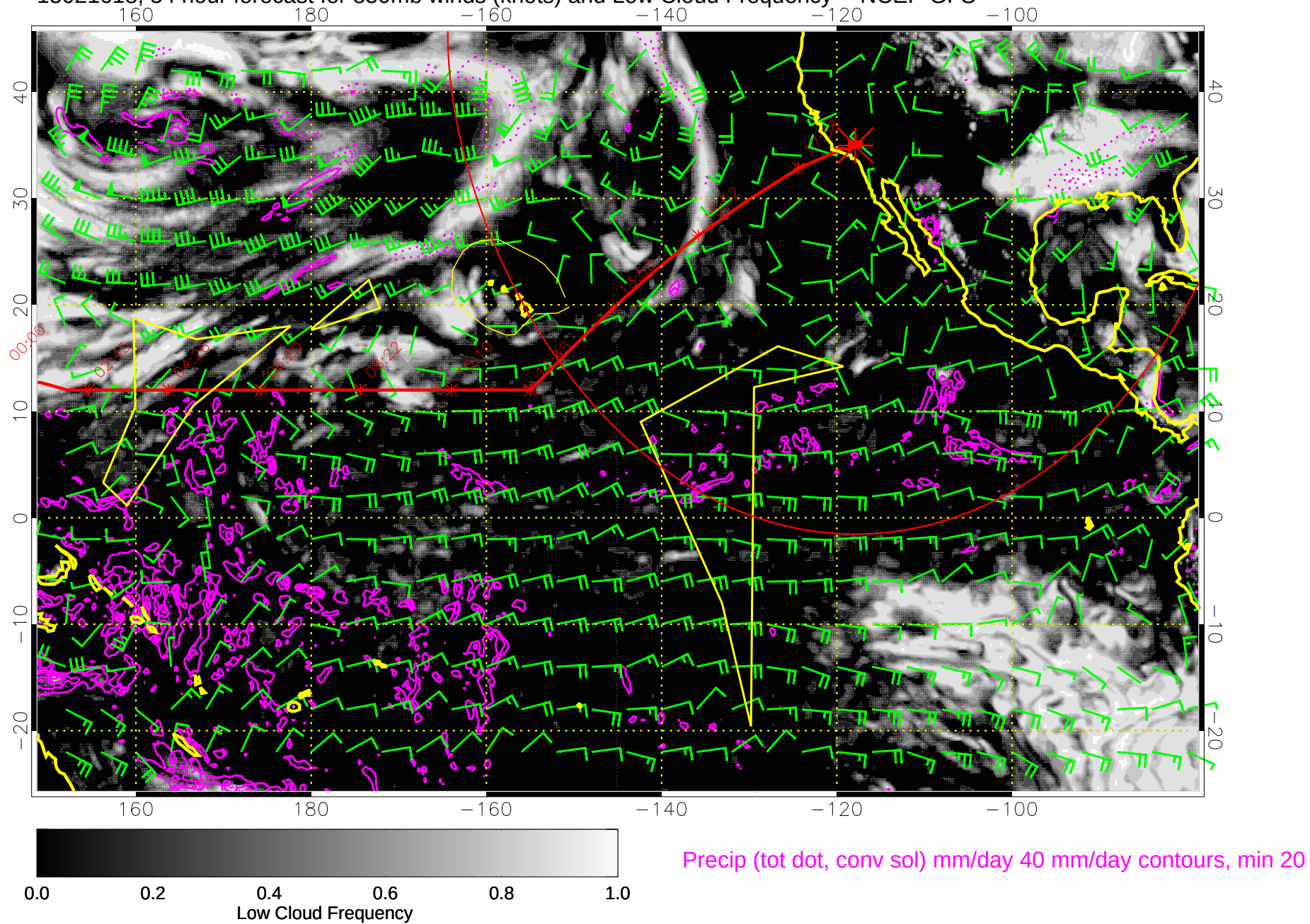
15021618, 54 hour forecast for 850mb winds (knots) and Low Cloud Frequency -- NCEP GFS
