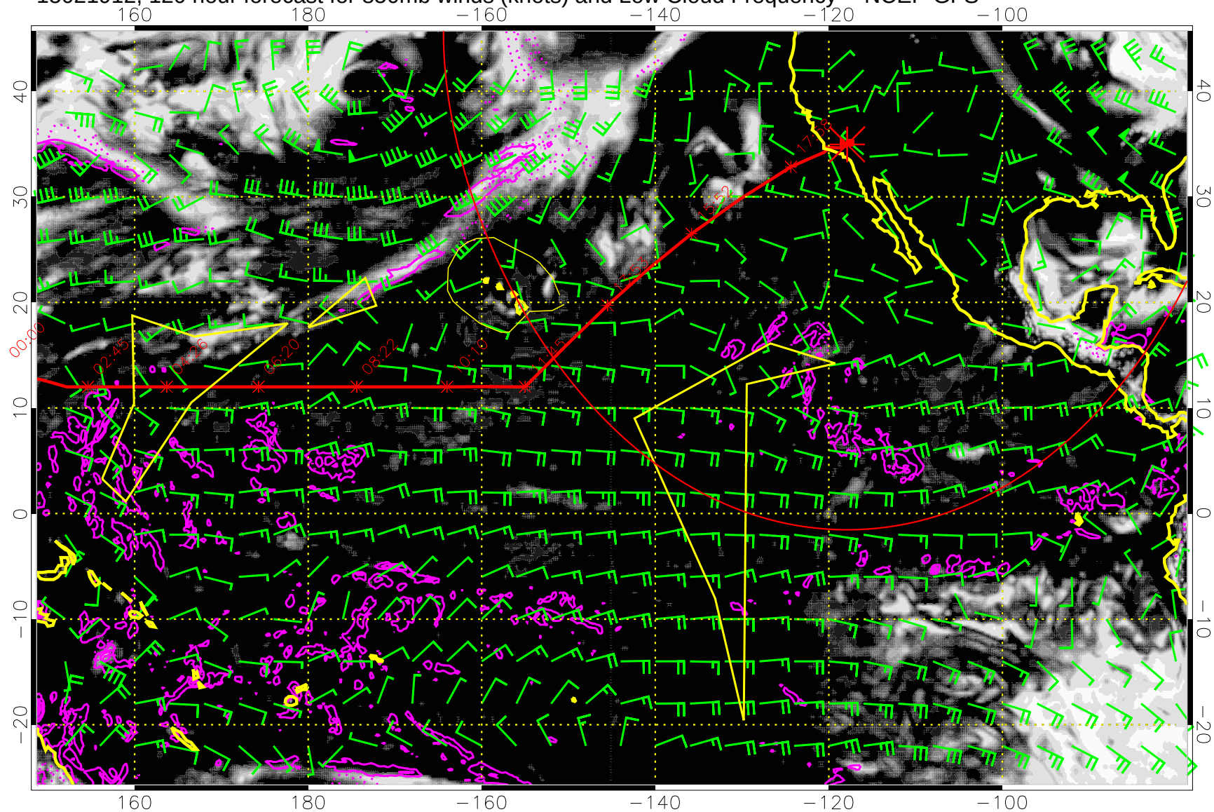
15021912, 120 hour forecast for 850mb winds (knots) and Low Cloud Frequency -- NCEP GFS
