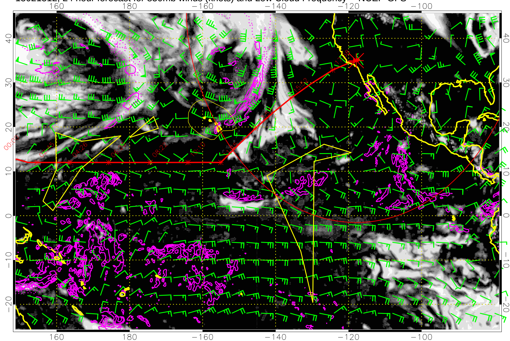
15021512, 24 hour forecast for 850mb winds (knots) and Low Cloud Frequency -- NCEP GFS
