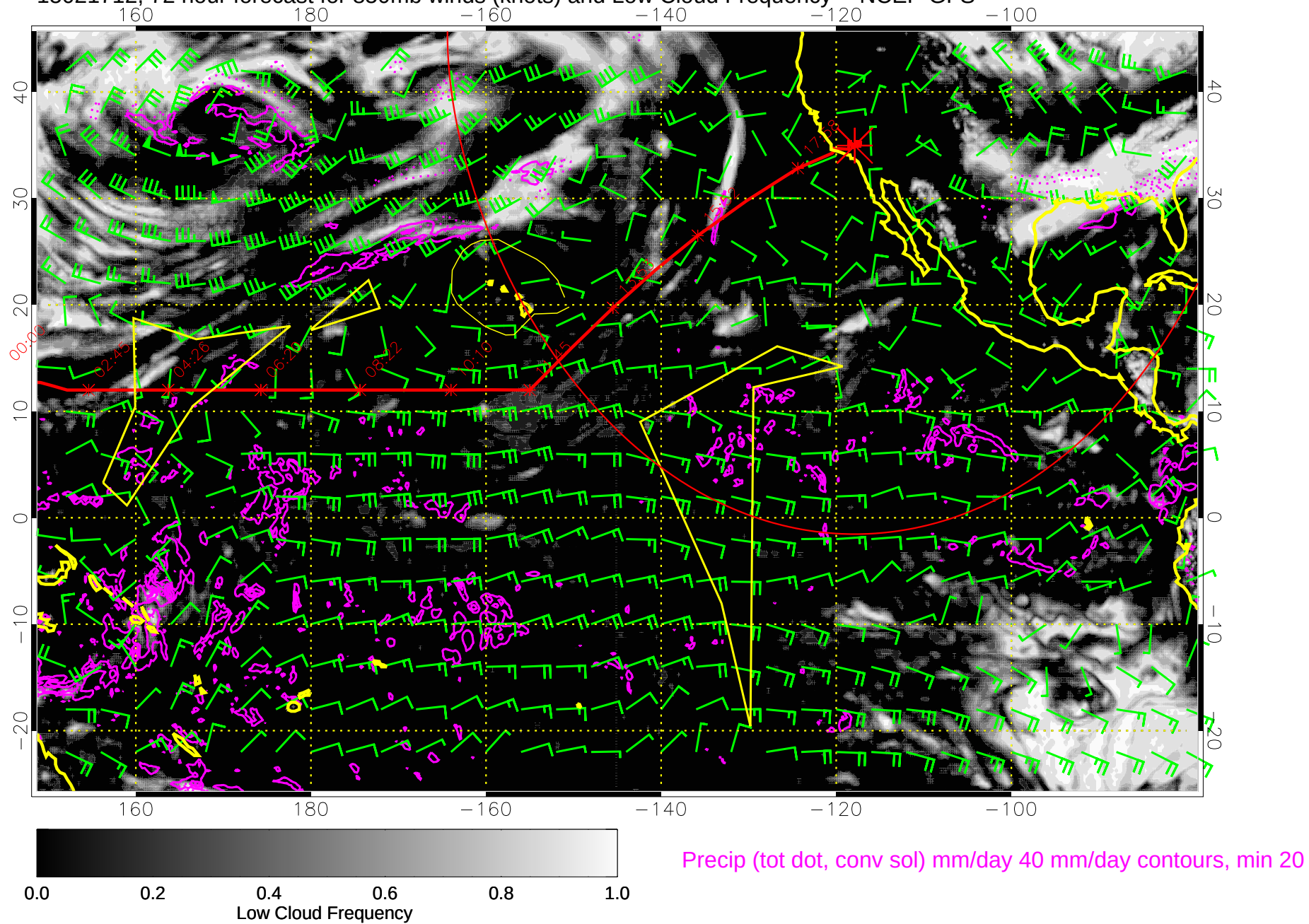
15021712, 72 hour forecast for 850mb winds (knots) and Low Cloud Frequency -- NCEP GFS
