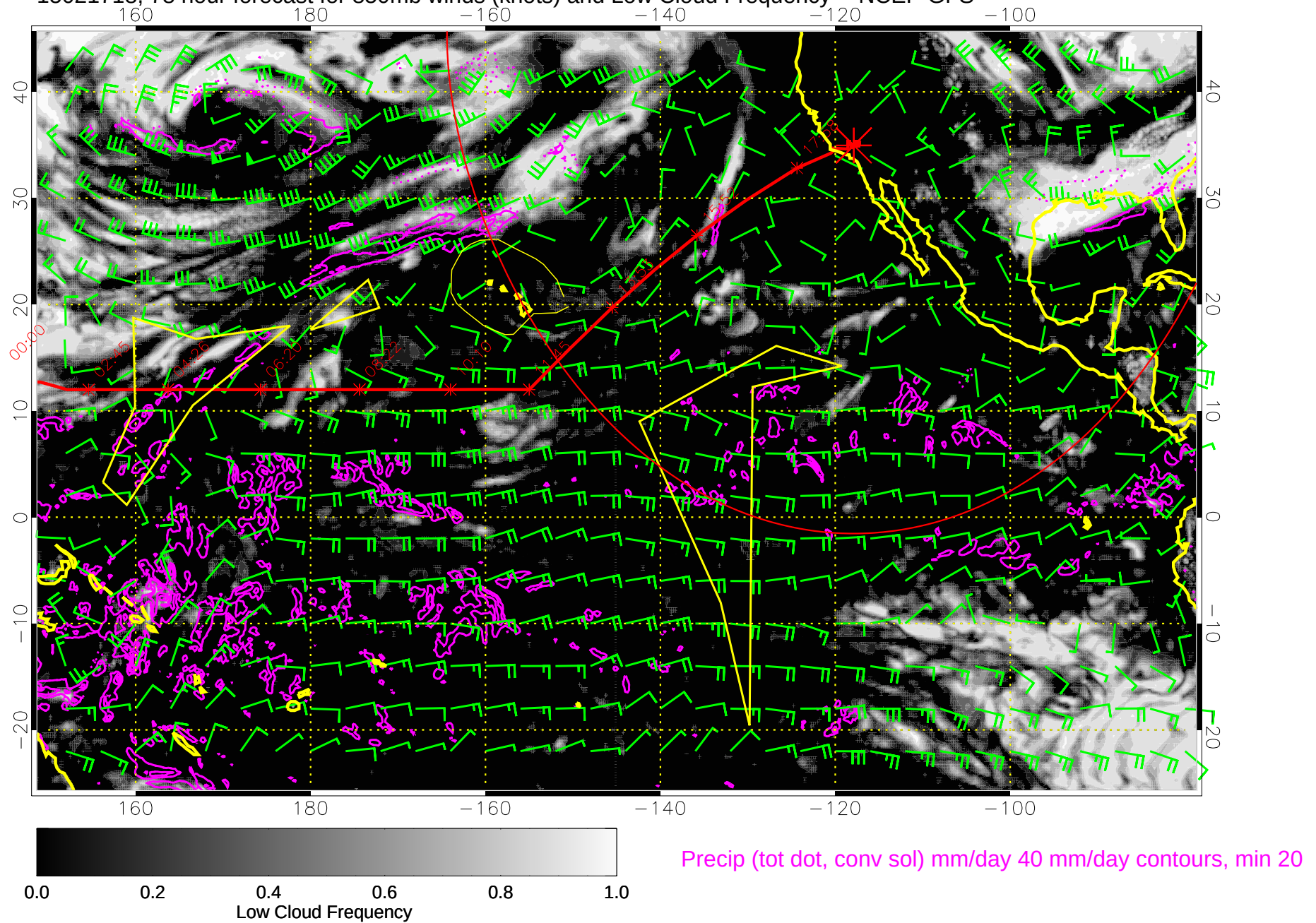
15021718, 78 hour forecast for 850mb winds (knots) and Low Cloud Frequency -- NCEP GFS
