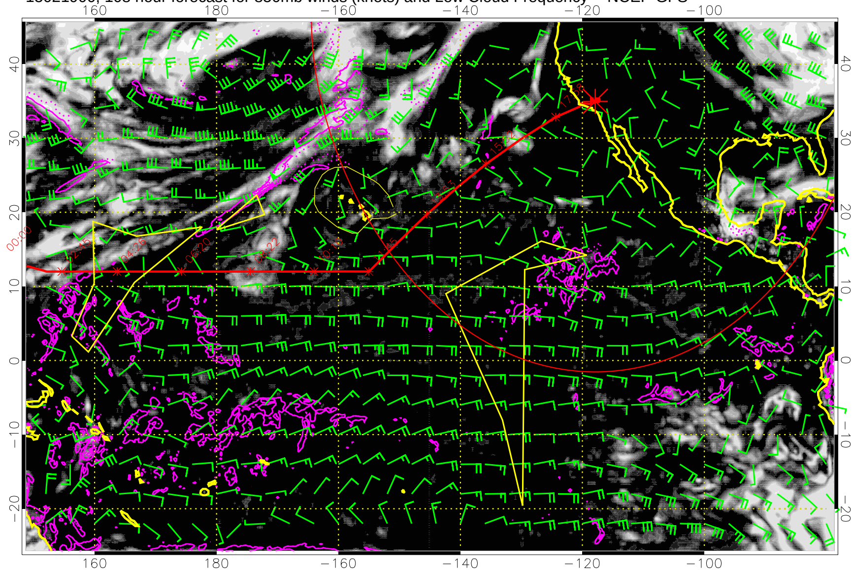
15021900, 108 hour forecast for 850mb winds (knots) and Low Cloud Frequency -- NCEP GFS
