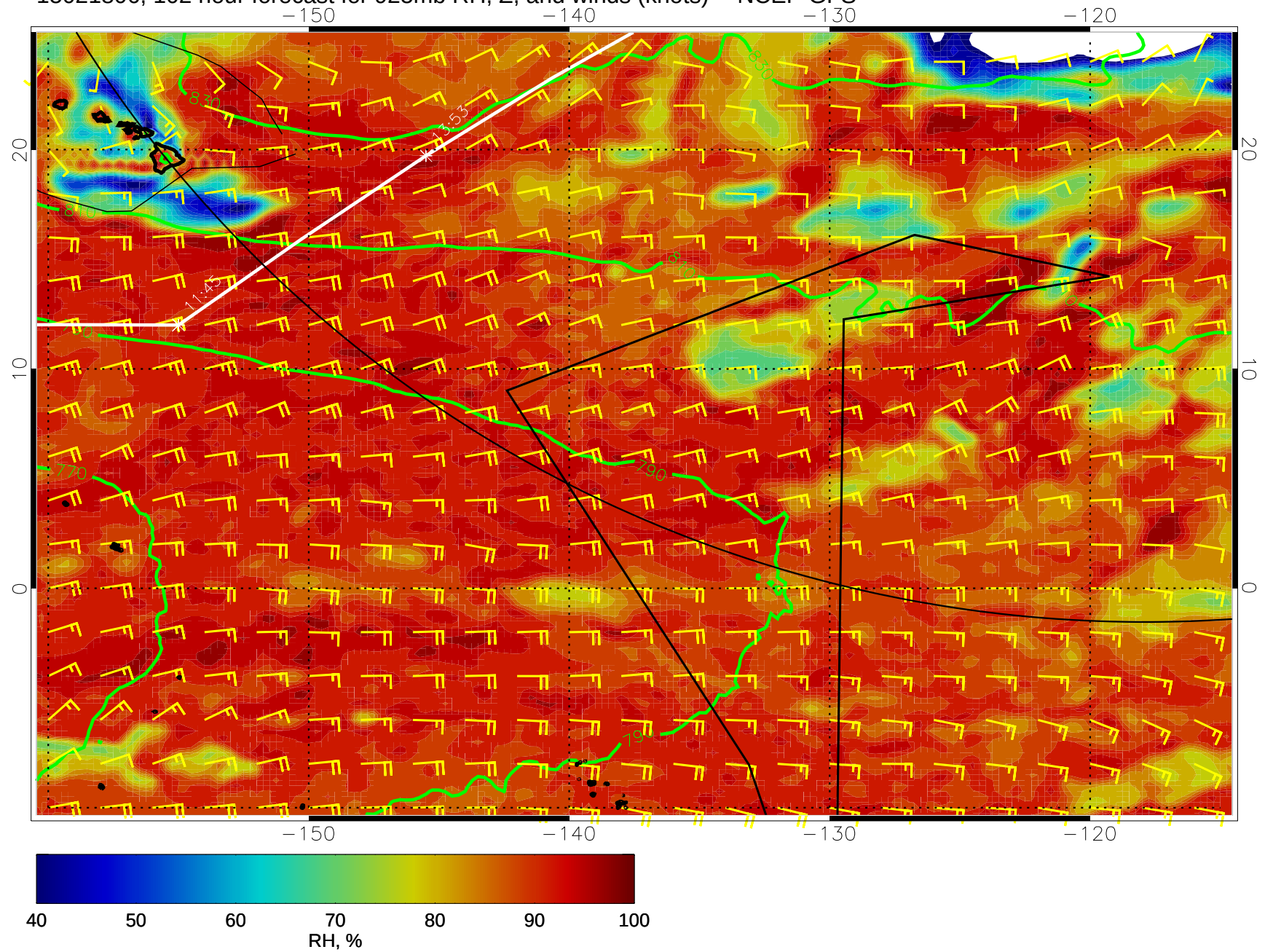
15021806, 102 hour forecast for 925mb RH, Z, and winds (knots) -- NCEP GFS
