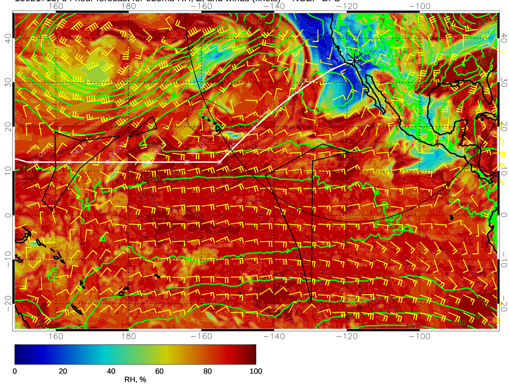
15021712, 84 hour forecast for 925mb RH, Z, and winds (knots) -- NCEP GFS
