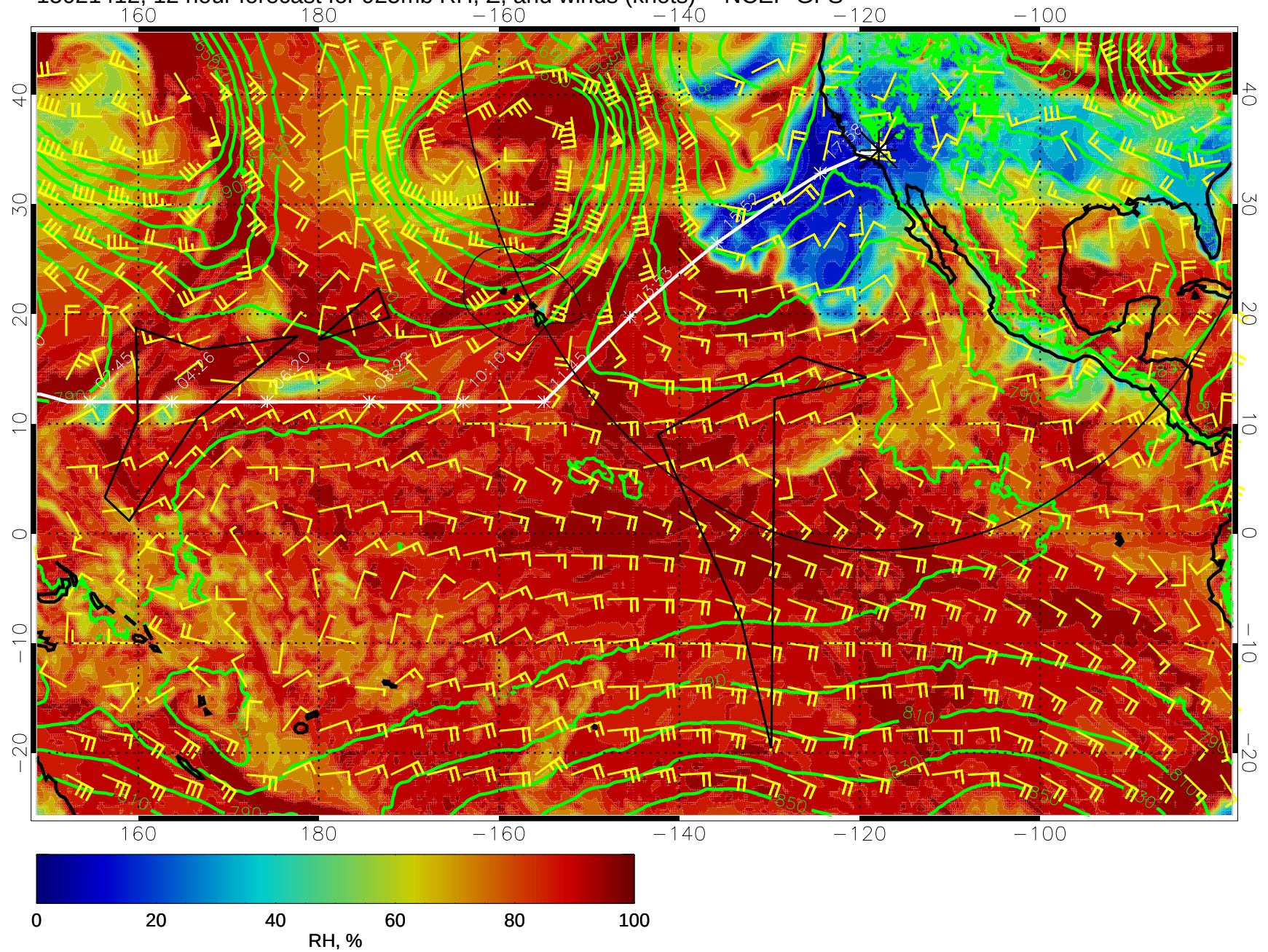
15021412, 12 hour forecast for 925mb RH, Z, and winds (knots) -- NCEP GFS
