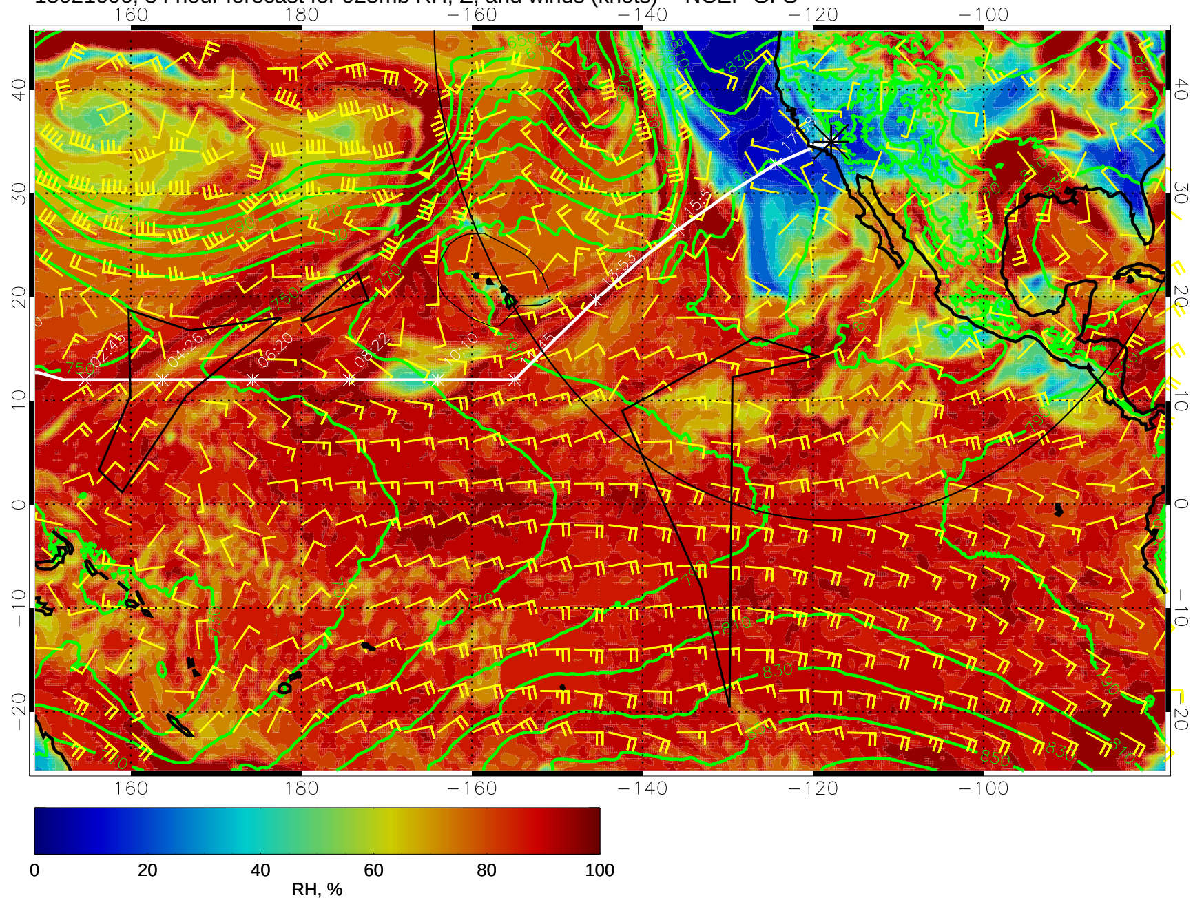
15021606, 54 hour forecast for 925mb RH, Z, and winds (knots) -- NCEP GFS
