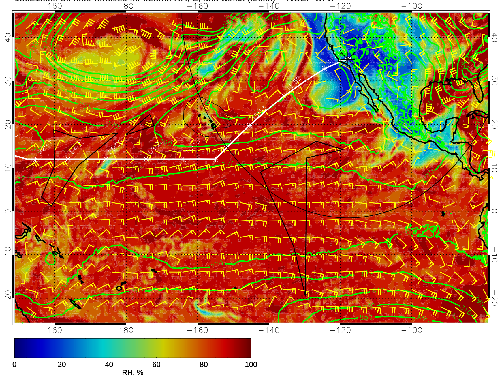
15021800, 96 hour forecast for 925mb RH, Z, and winds (knots) -- NCEP GFS
