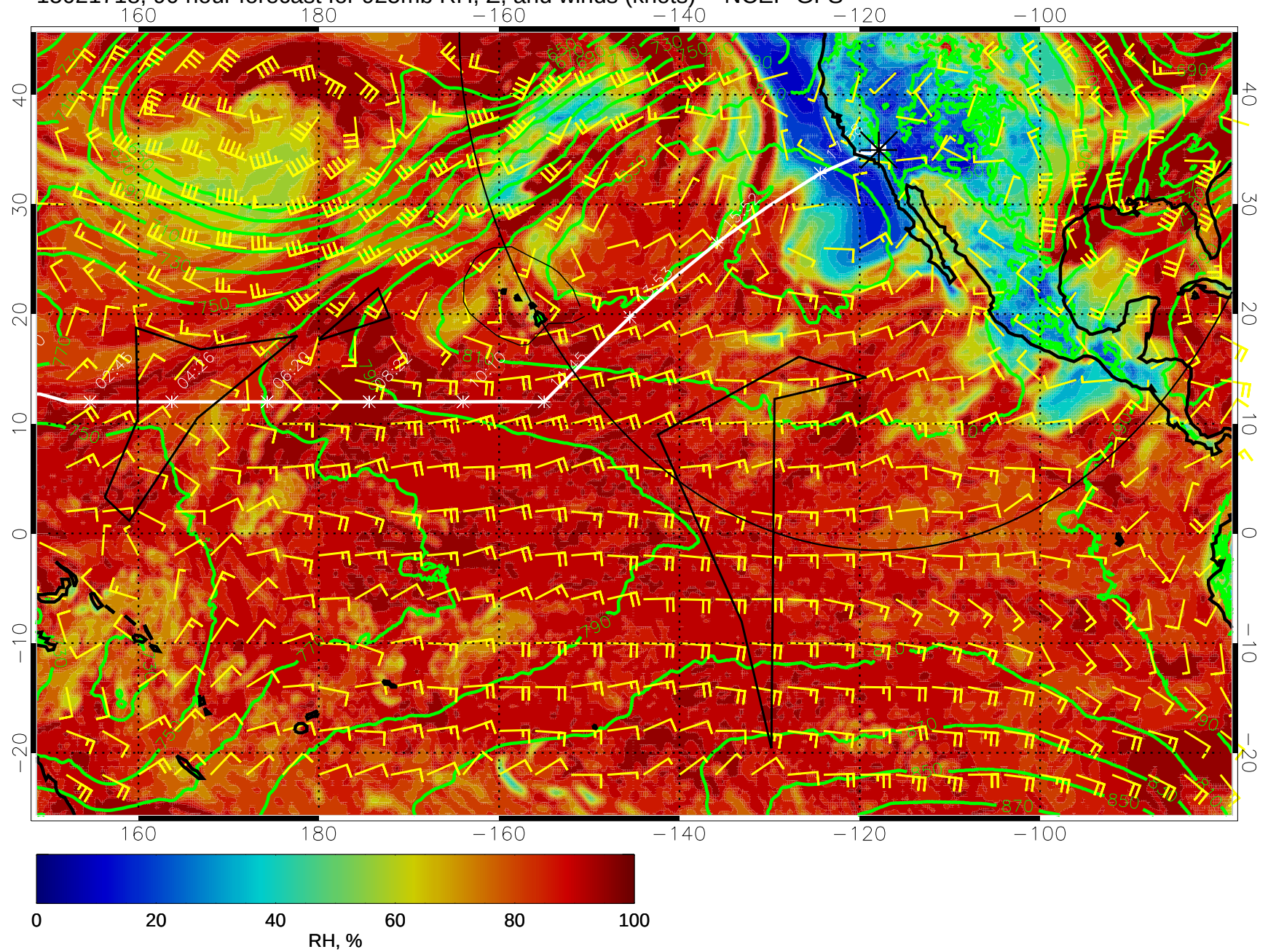
15021718, 90 hour forecast for 925mb RH, Z, and winds (knots) -- NCEP GFS
