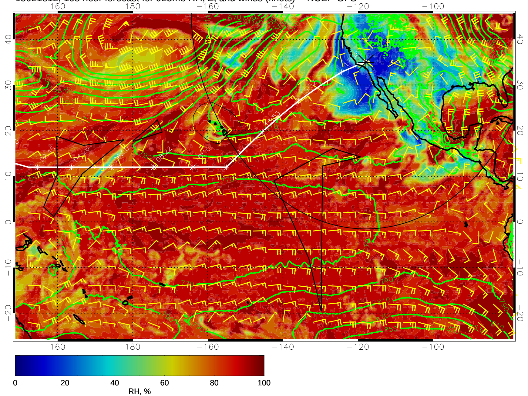
15021812, 108 hour forecast for 925mb RH, Z, and winds (knots) -- NCEP GFS
