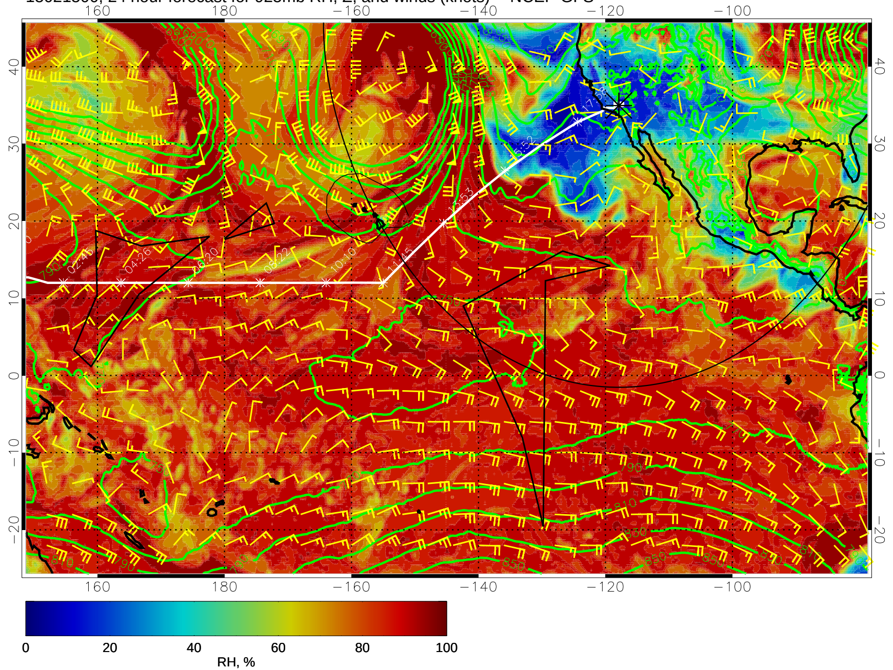
15021500, 24 hour forecast for 925mb RH, Z, and winds (knots) -- NCEP GFS
