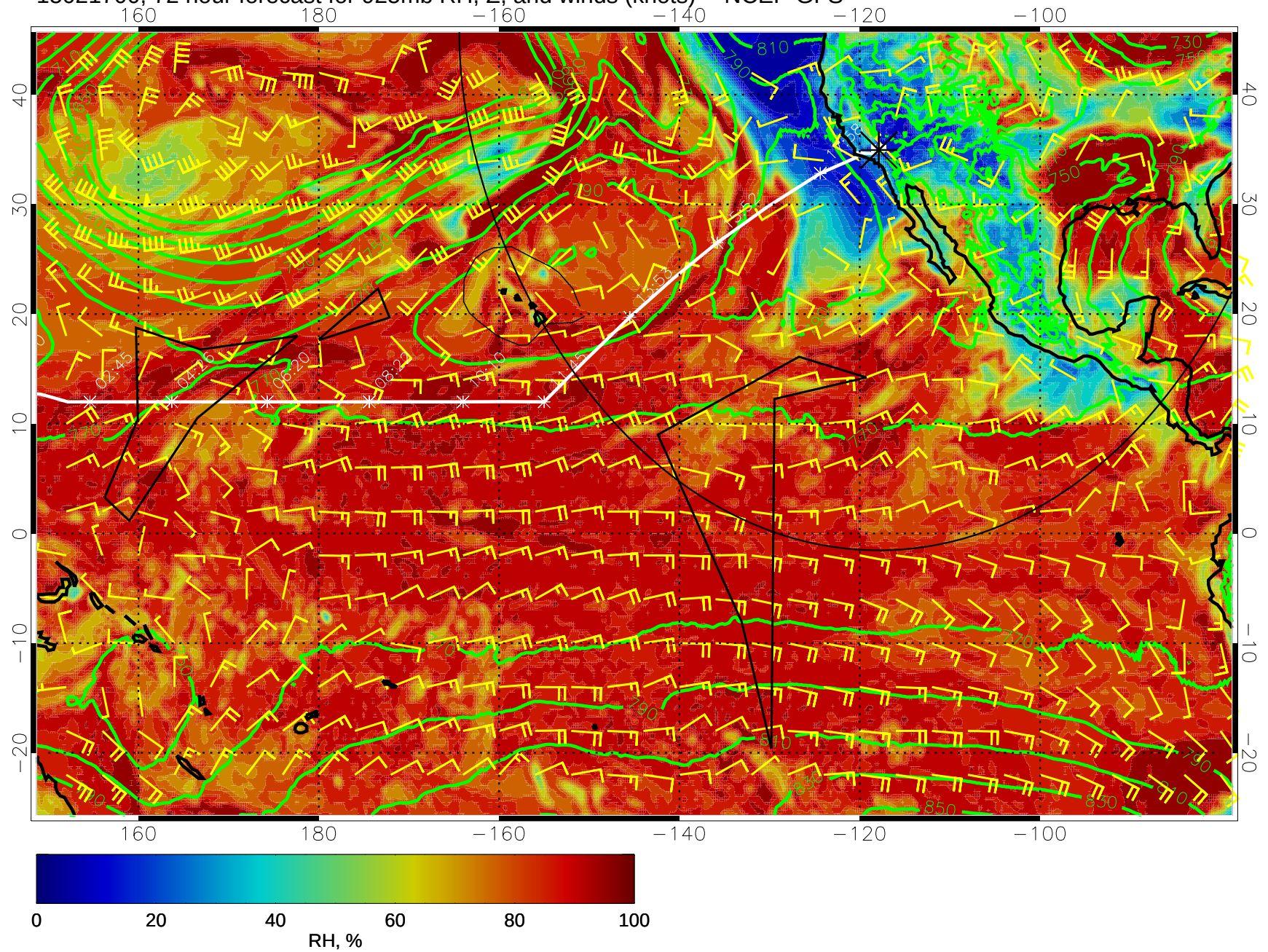
15021700, 72 hour forecast for 925mb RH, Z, and winds (knots) -- NCEP GFS
