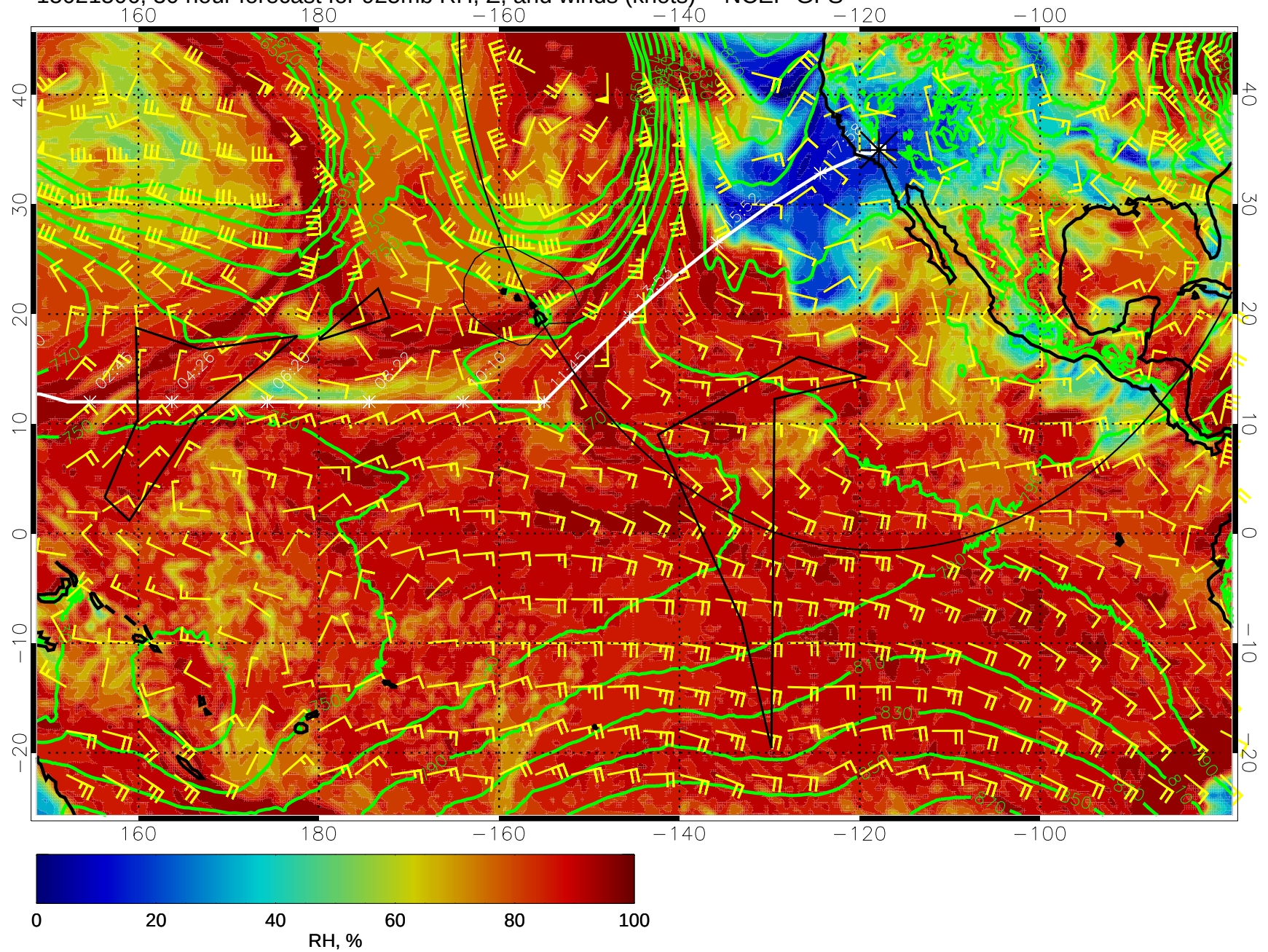
15021506, 30 hour forecast for 925mb RH, Z, and winds (knots) -- NCEP GFS
