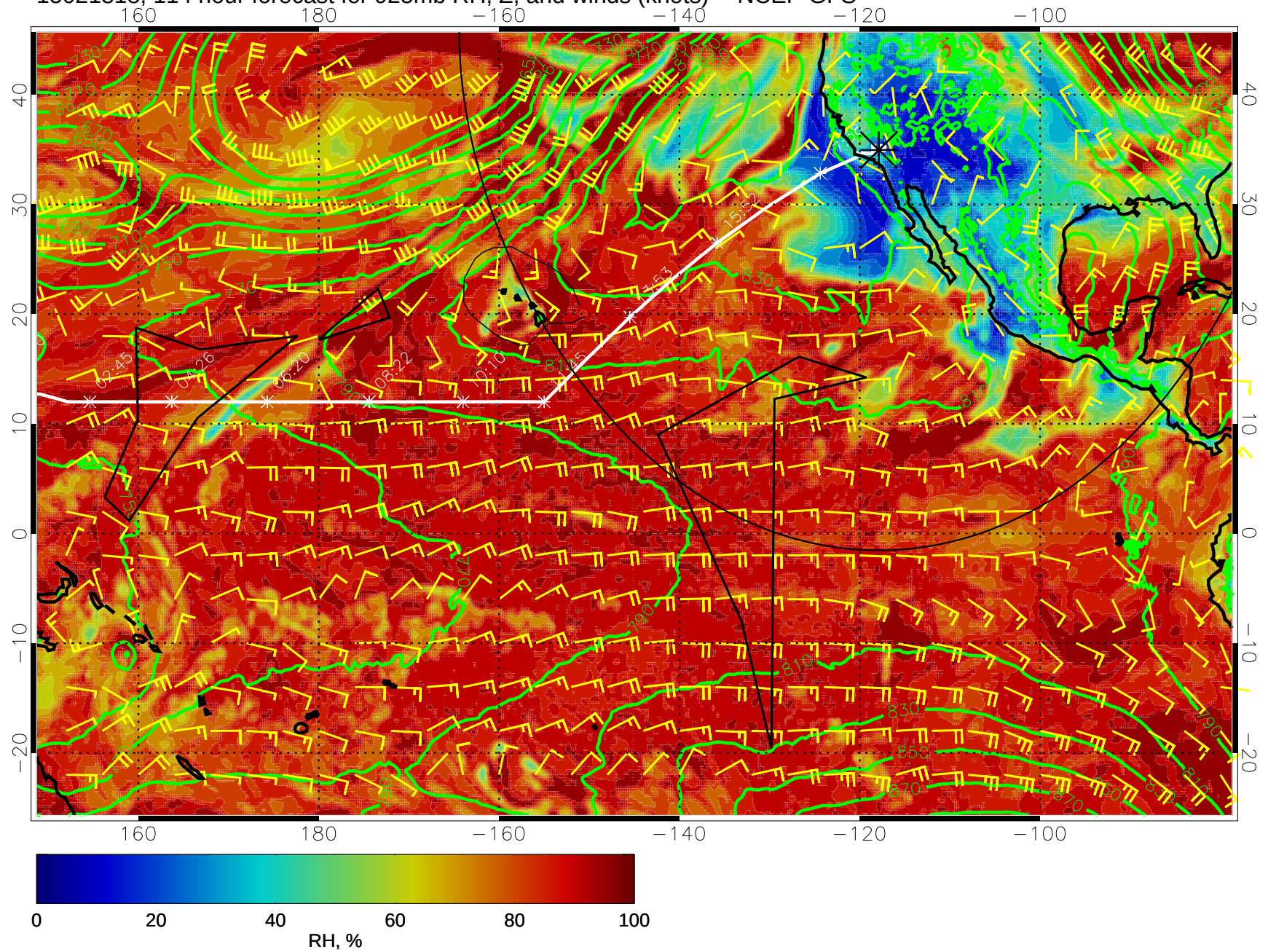
15021818, 114 hour forecast for 925mb RH, Z, and winds (knots) -- NCEP GFS
