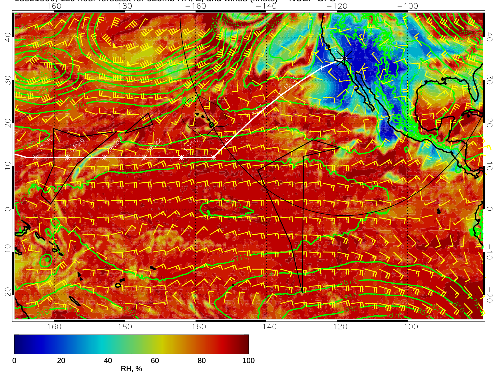
15021900, 120 hour forecast for 925mb RH, Z, and winds (knots) -- NCEP GFS
