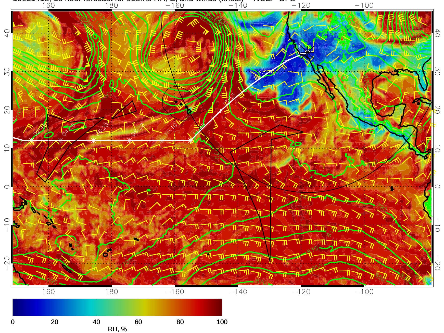
15021418, 18 hour forecast for 925mb RH, Z, and winds (knots) -- NCEP GFS
