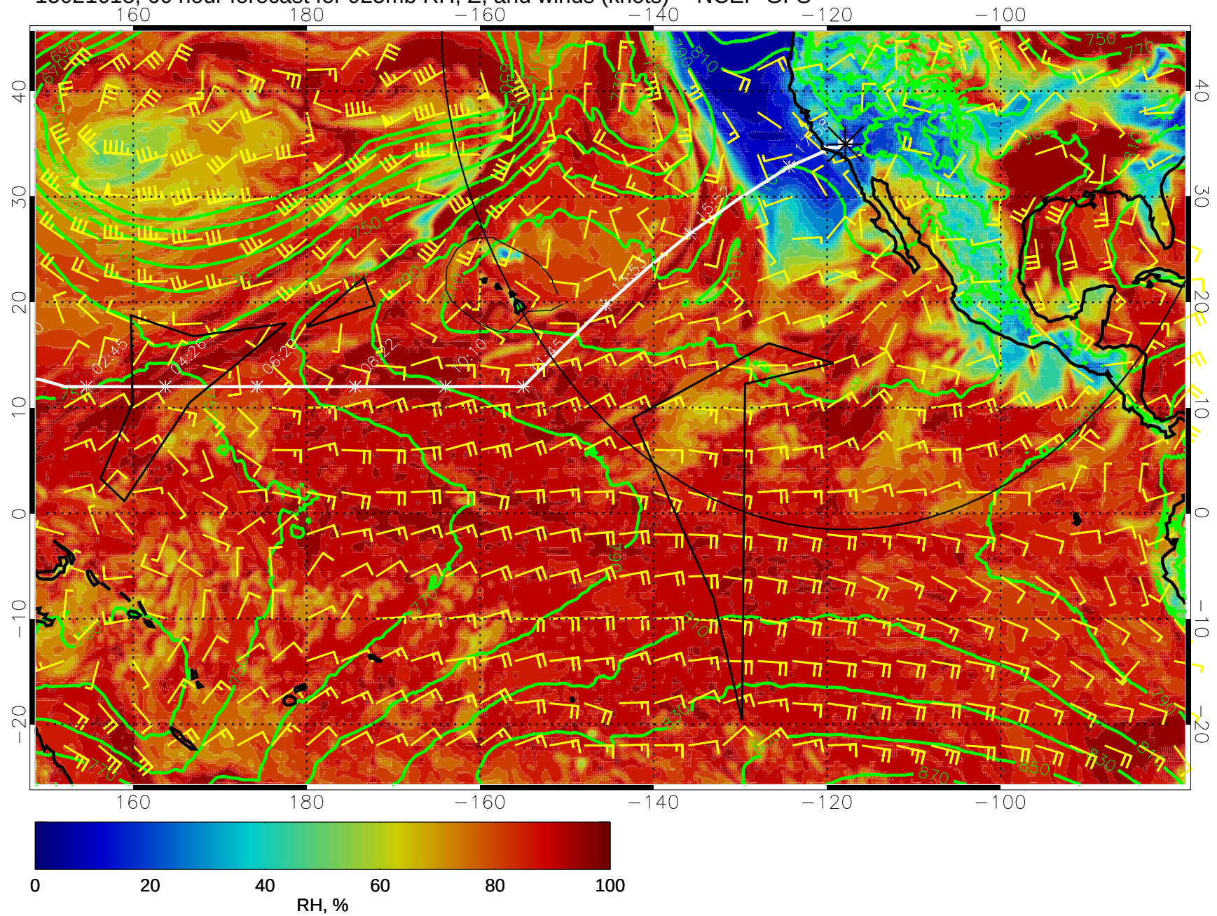
15021618, 66 hour forecast for 925mb RH, Z, and winds (knots) -- NCEP GFS
