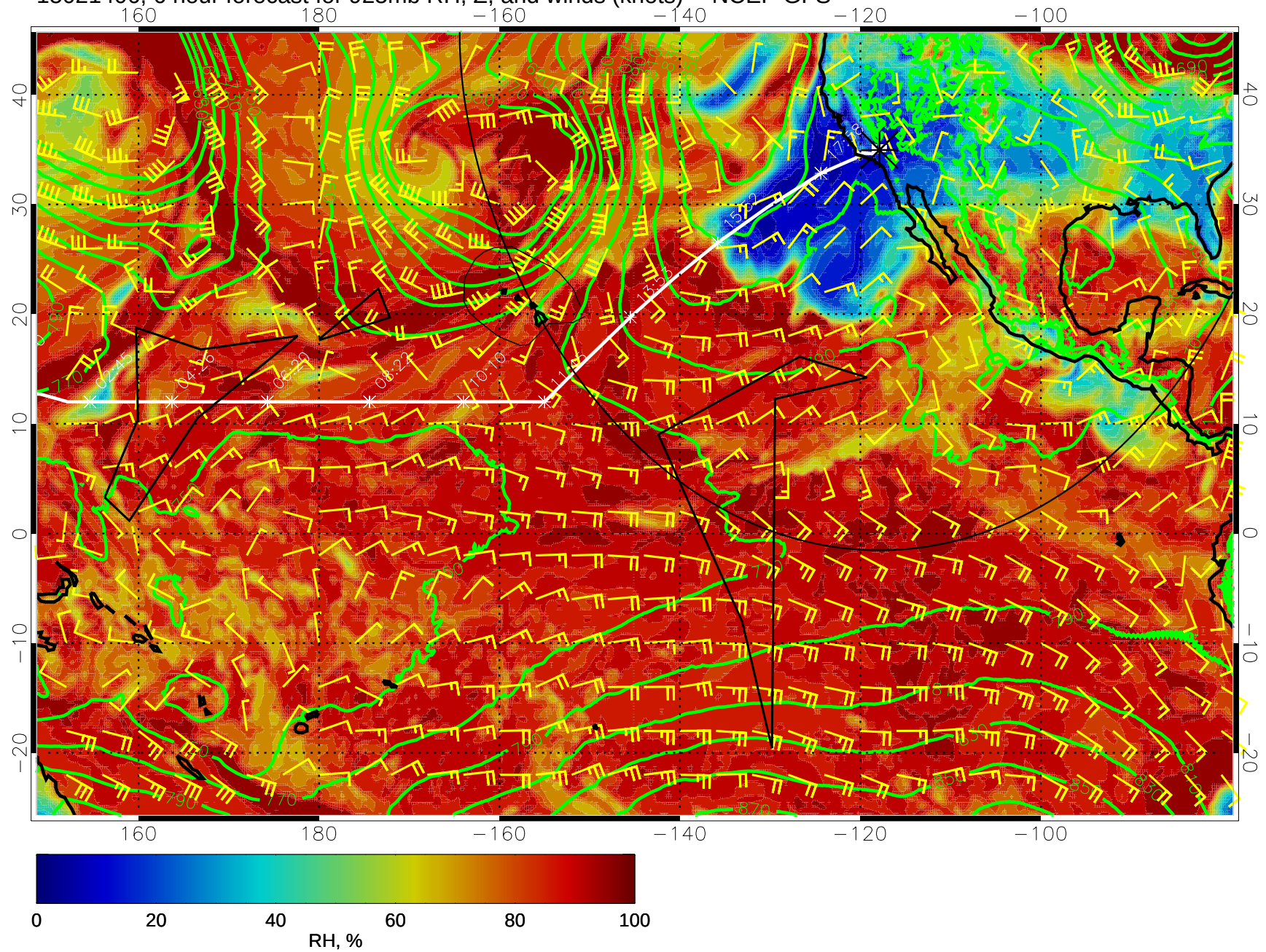
15021406, 6 hour forecast for 925mb RH, Z, and winds (knots) -- NCEP GFS
