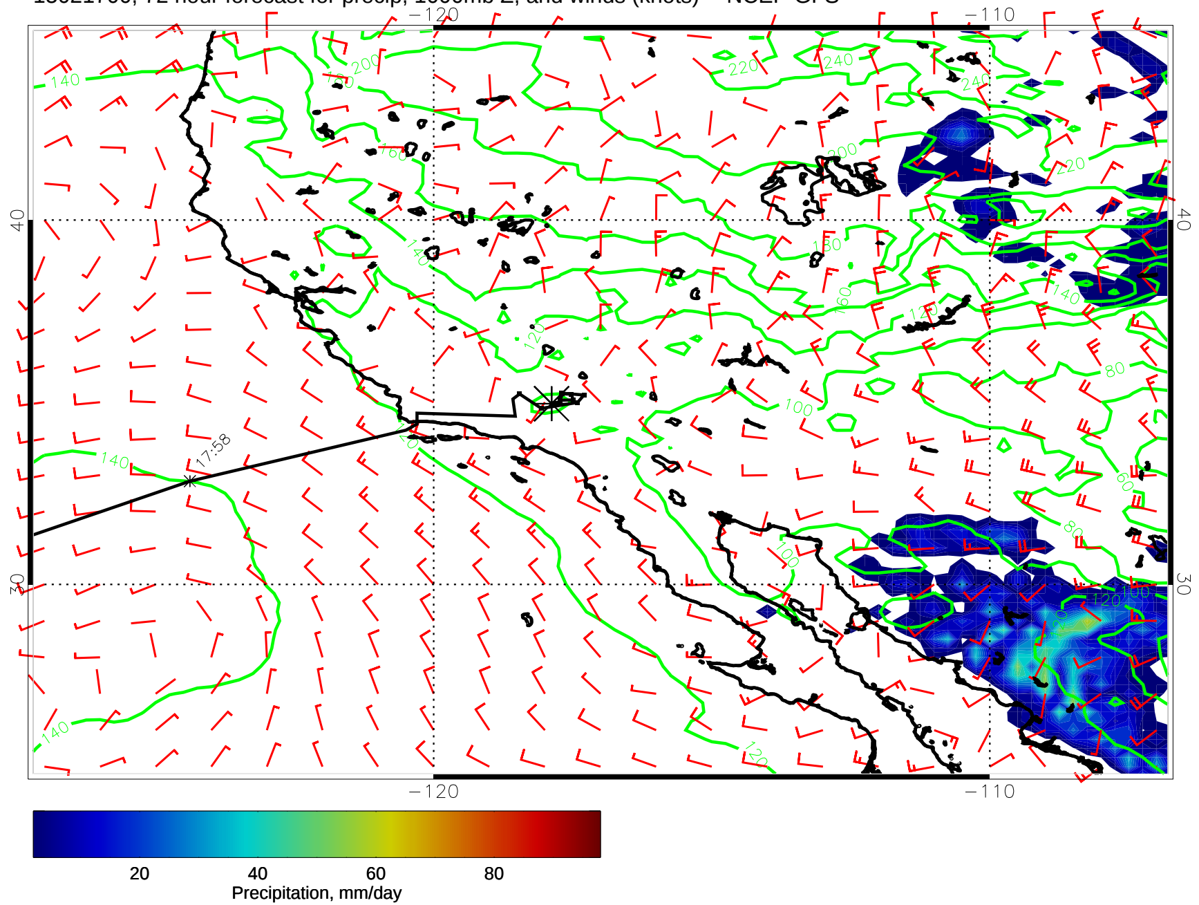
15021700, 72 hour forecast for precip, 1000mb Z, and winds (knots) -- NCEP GFS
