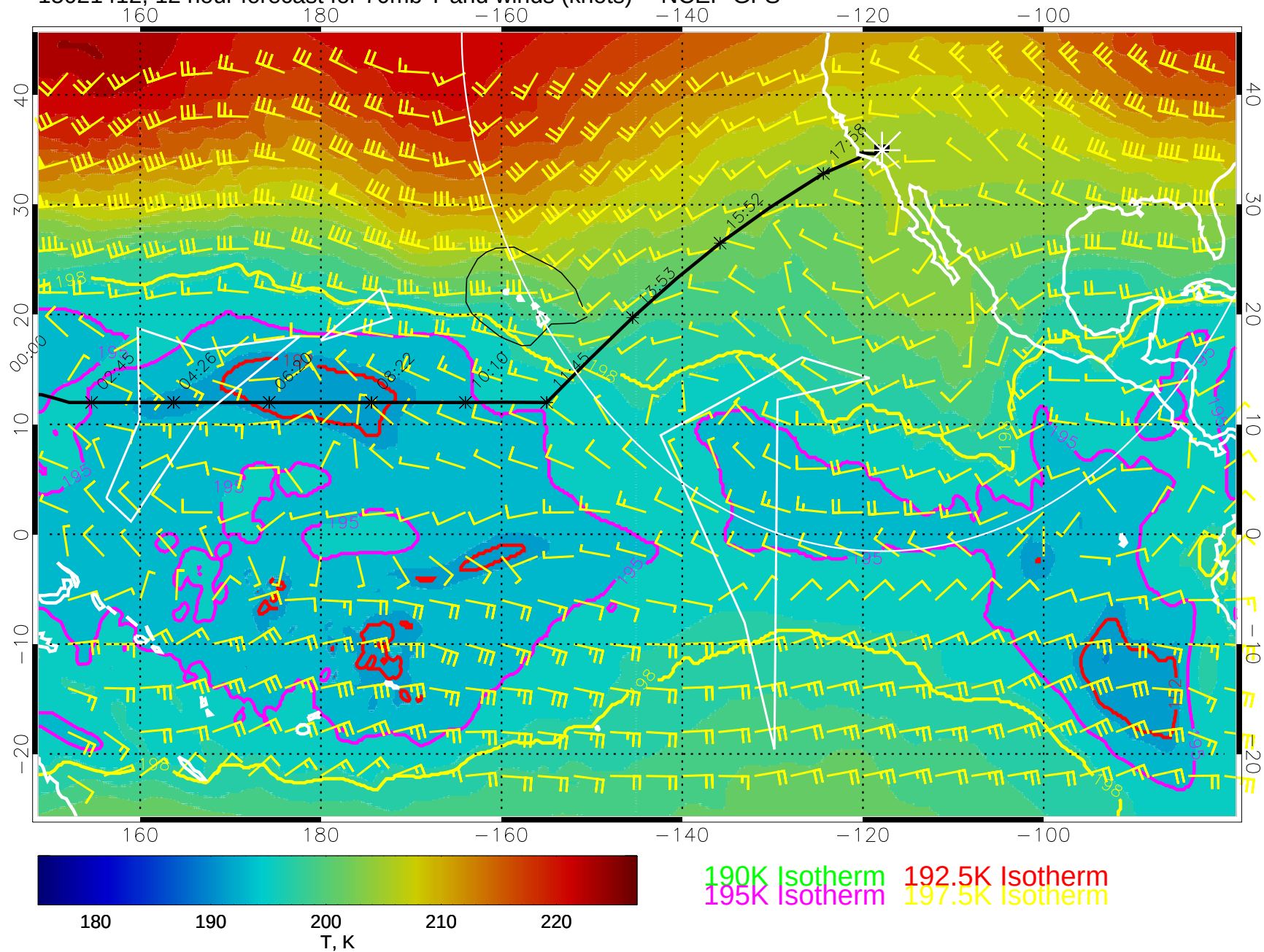
15021412, 12 hour forecast for 70mb T and winds (knots) -- NCEP GFS
