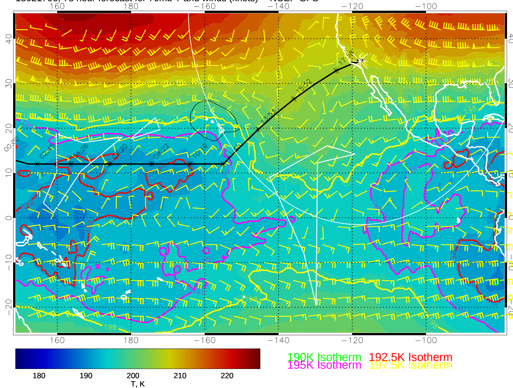
15021706, 78 hour forecast for 70mb T and winds (knots) -- NCEP GFS
