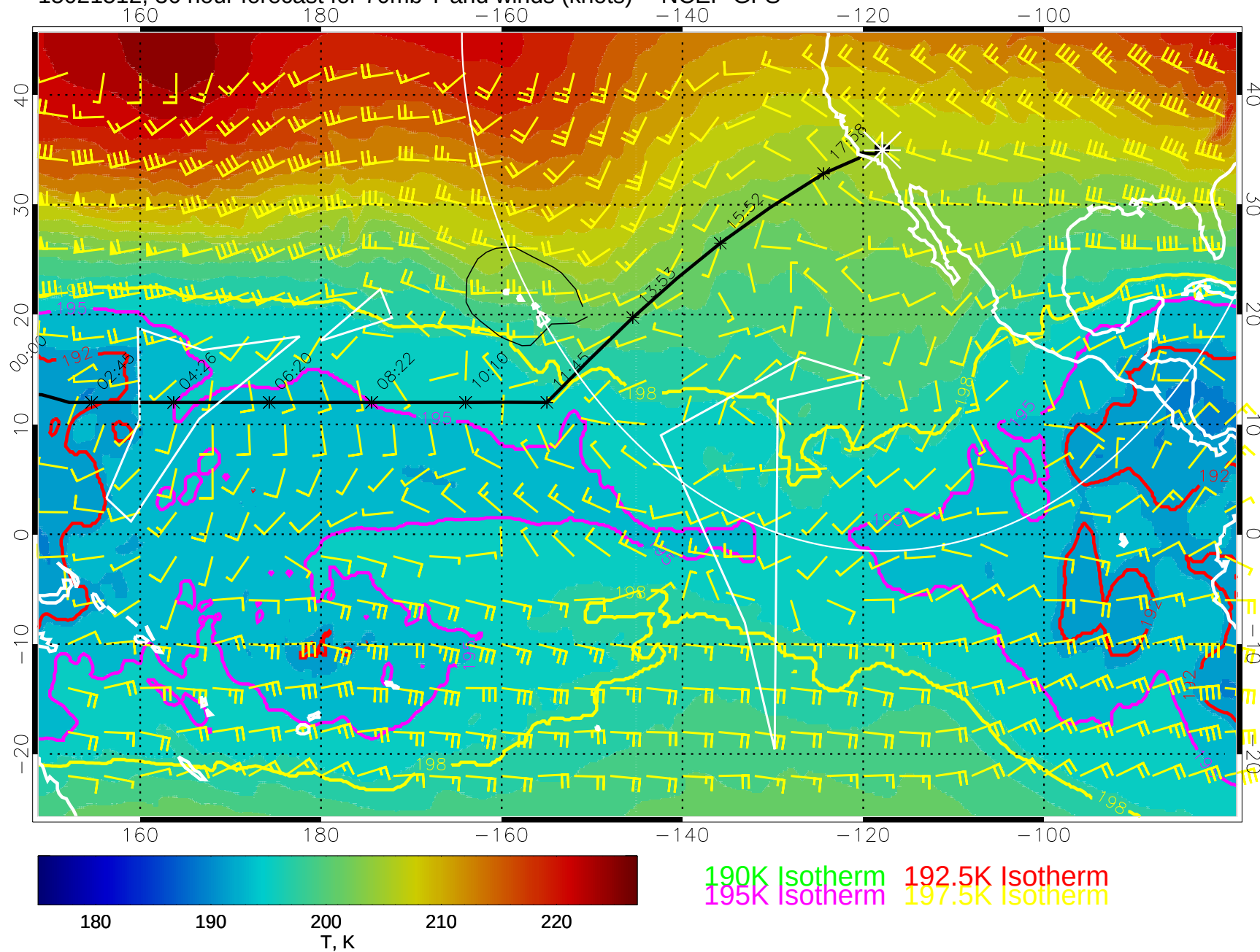
15021512, 36 hour forecast for 70mb T and winds (knots) -- NCEP GFS
