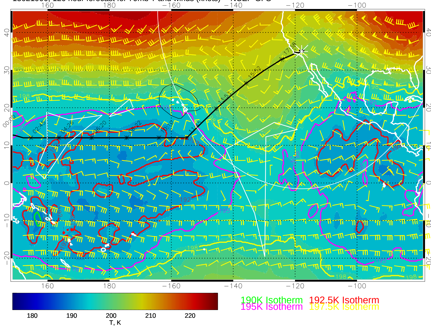
15021900, 120 hour forecast for 70mb T and winds (knots) -- NCEP GFS
