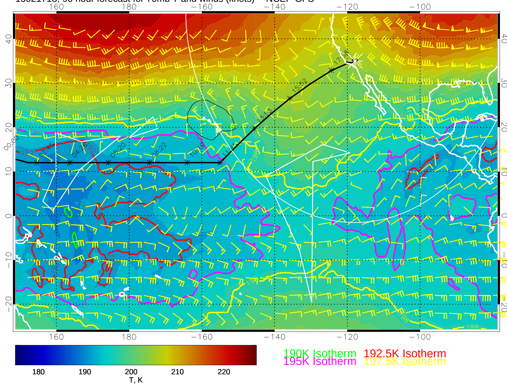
15021718, 90 hour forecast for 70mb T and winds (knots) -- NCEP GFS
