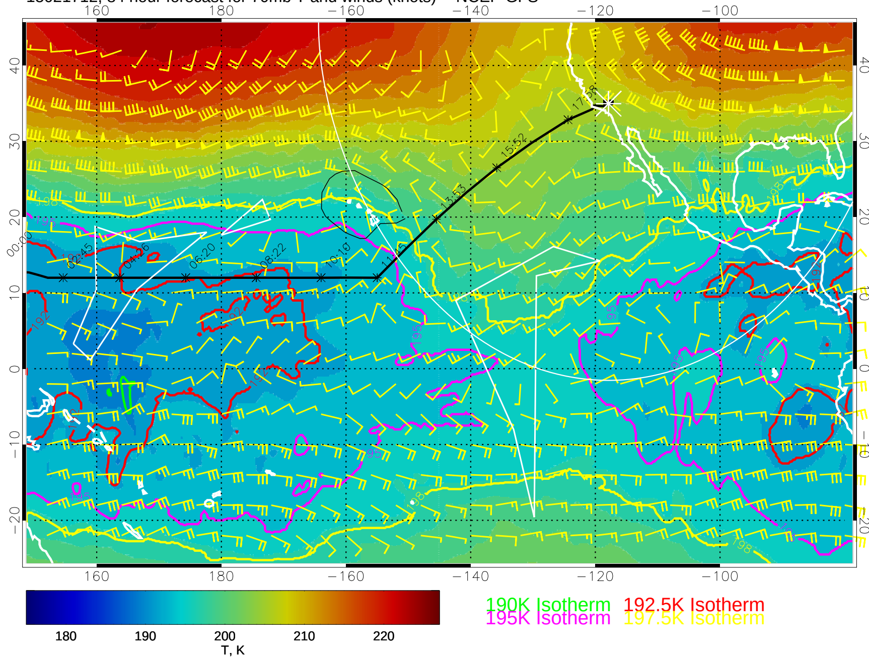
15021712, 84 hour forecast for 70mb T and winds (knots) -- NCEP GFS
