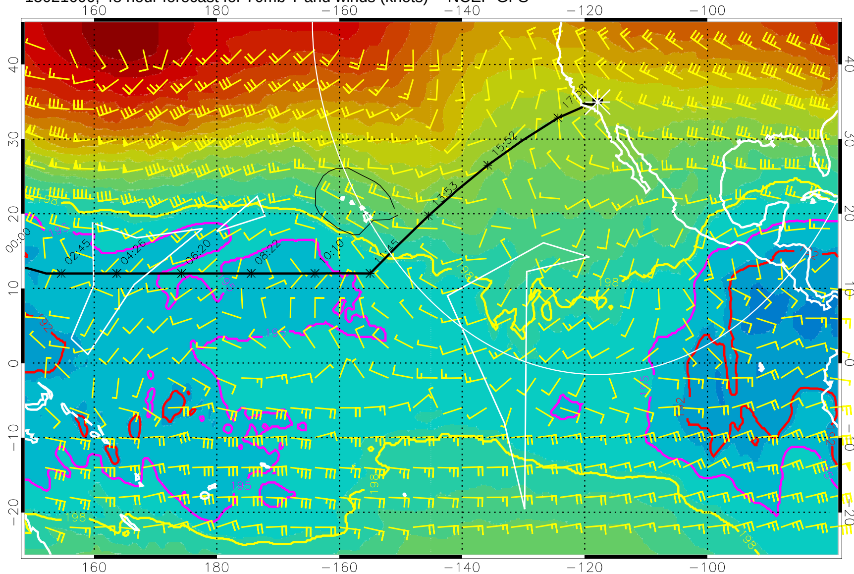
15021600, 48 hour forecast for 70mb T and winds (knots) -- NCEP GFS
