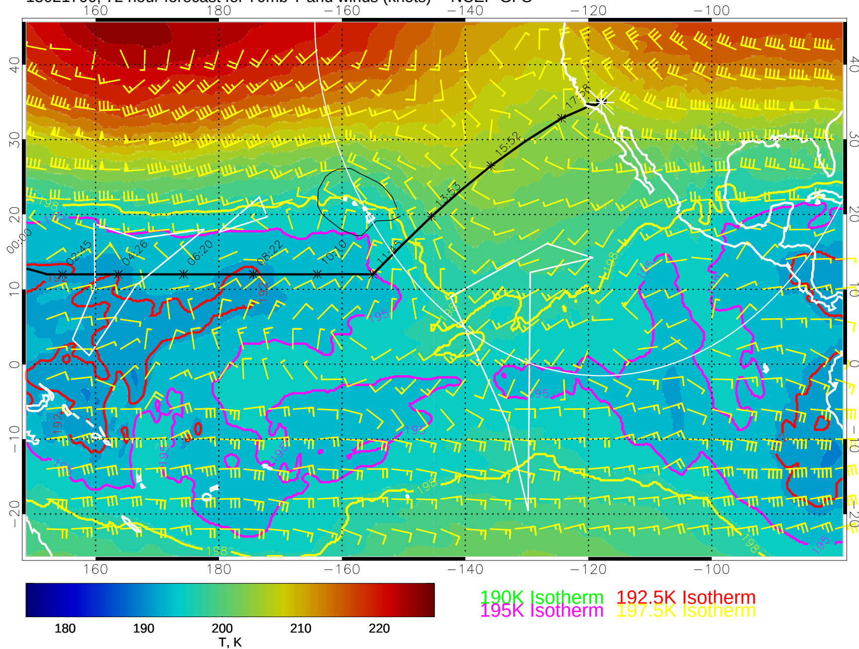
15021700, 72 hour forecast for 70mb T and winds (knots) -- NCEP GFS
