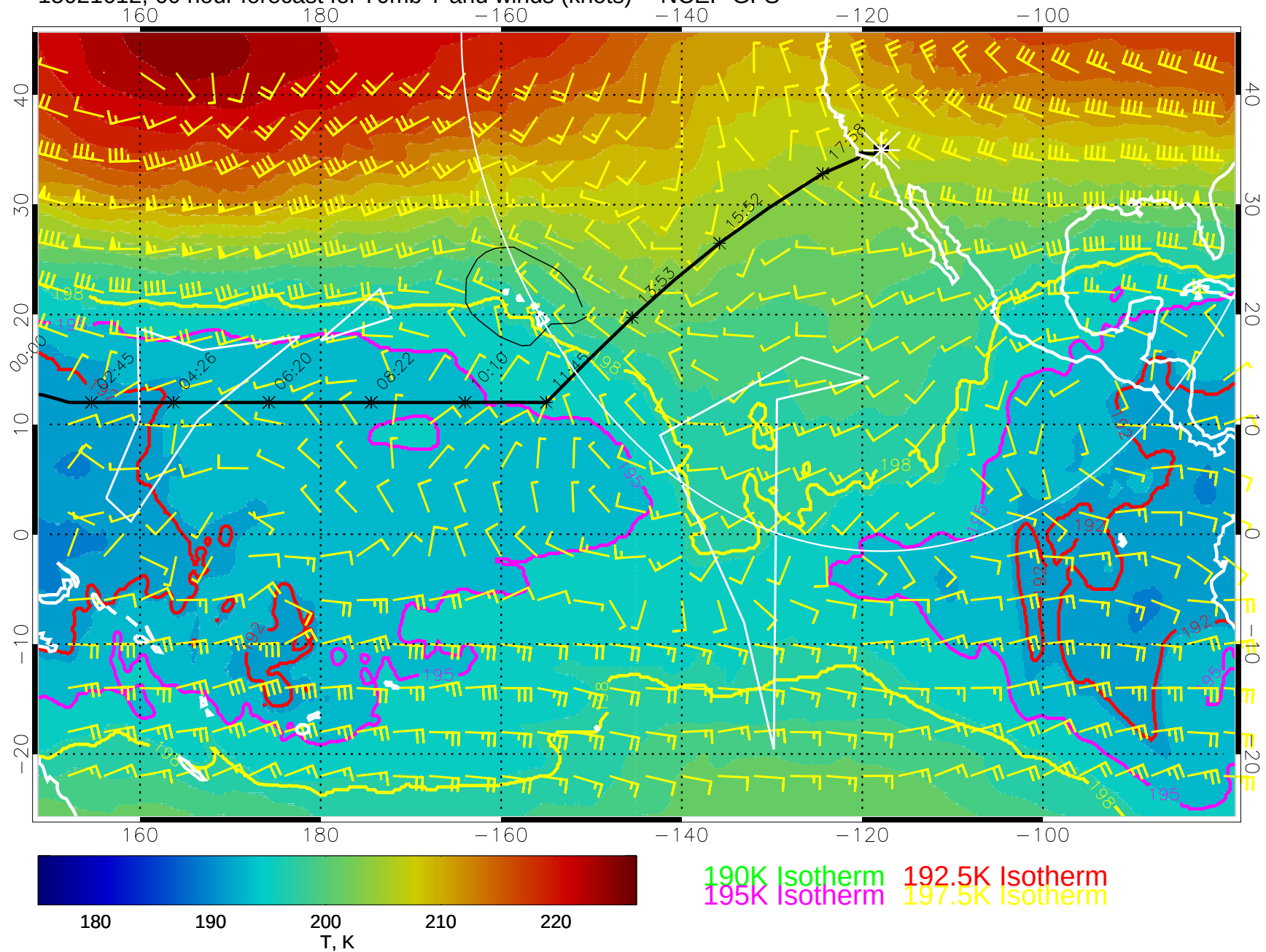
15021612, 60 hour forecast for 70mb T and winds (knots) -- NCEP GFS
