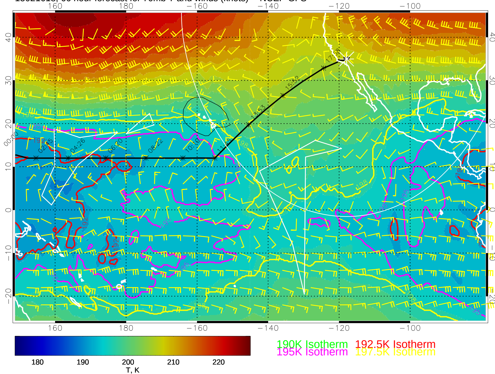
15021618, 66 hour forecast for 70mb T and winds (knots) -- NCEP GFS
