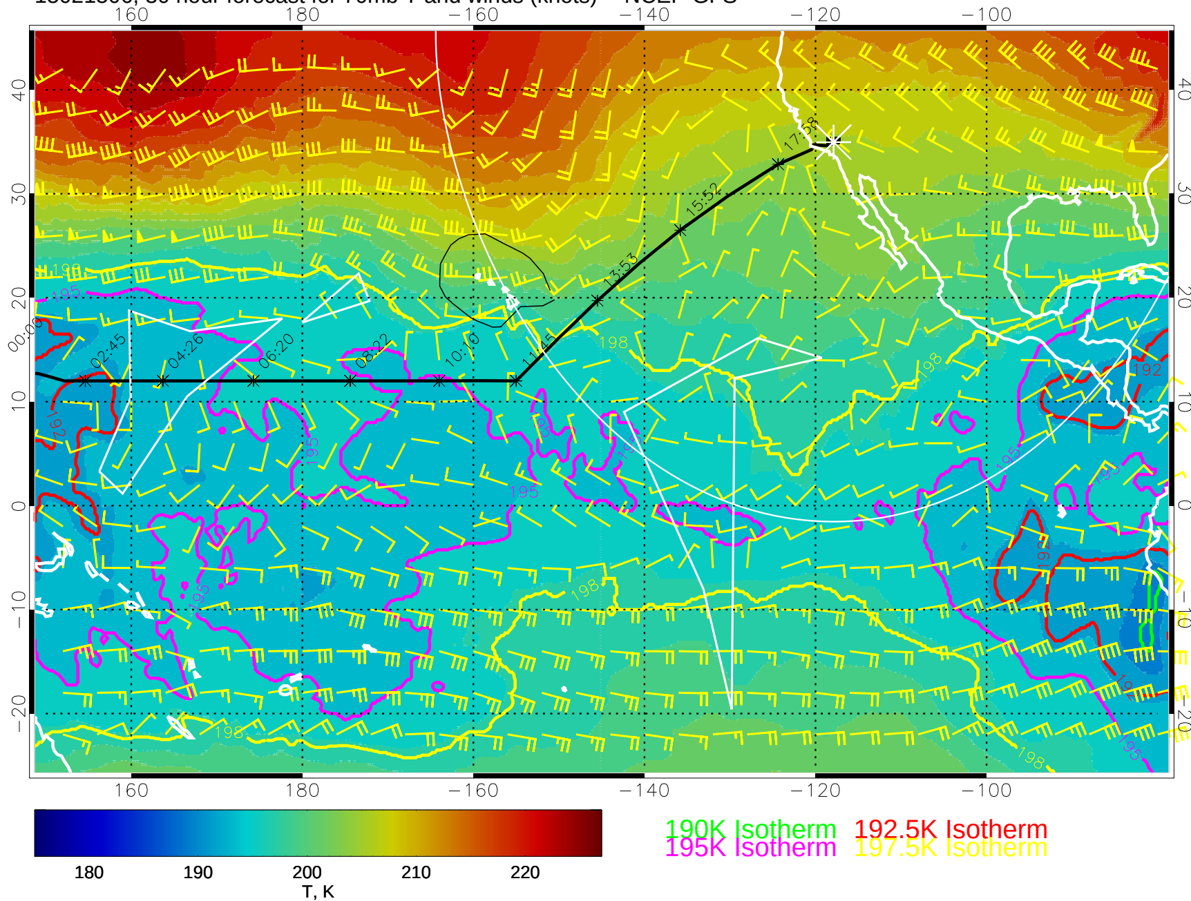
15021506, 30 hour forecast for 70mb T and winds (knots) -- NCEP GFS
