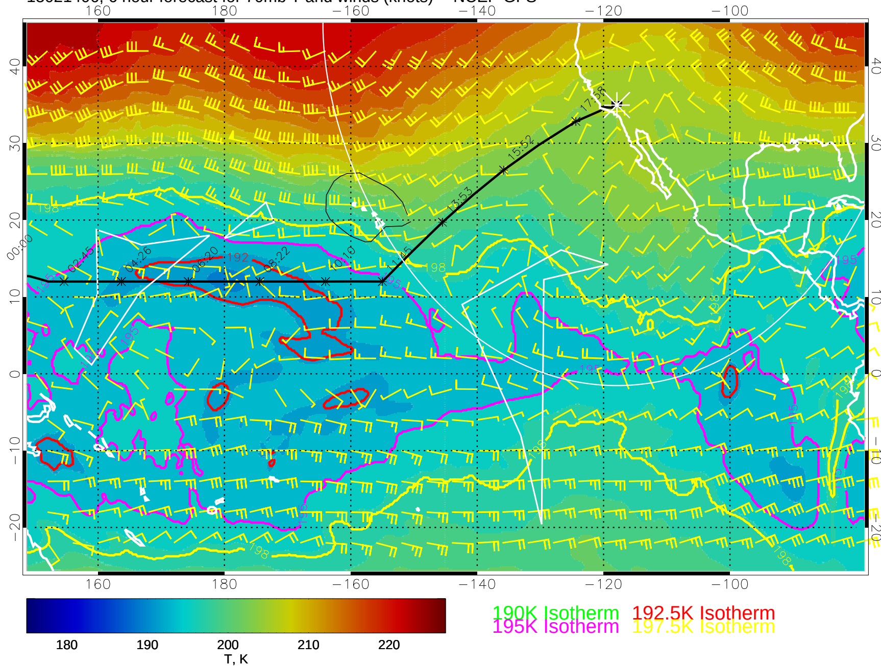
15021406, 6 hour forecast for 70mb T and winds (knots) -- NCEP GFS
