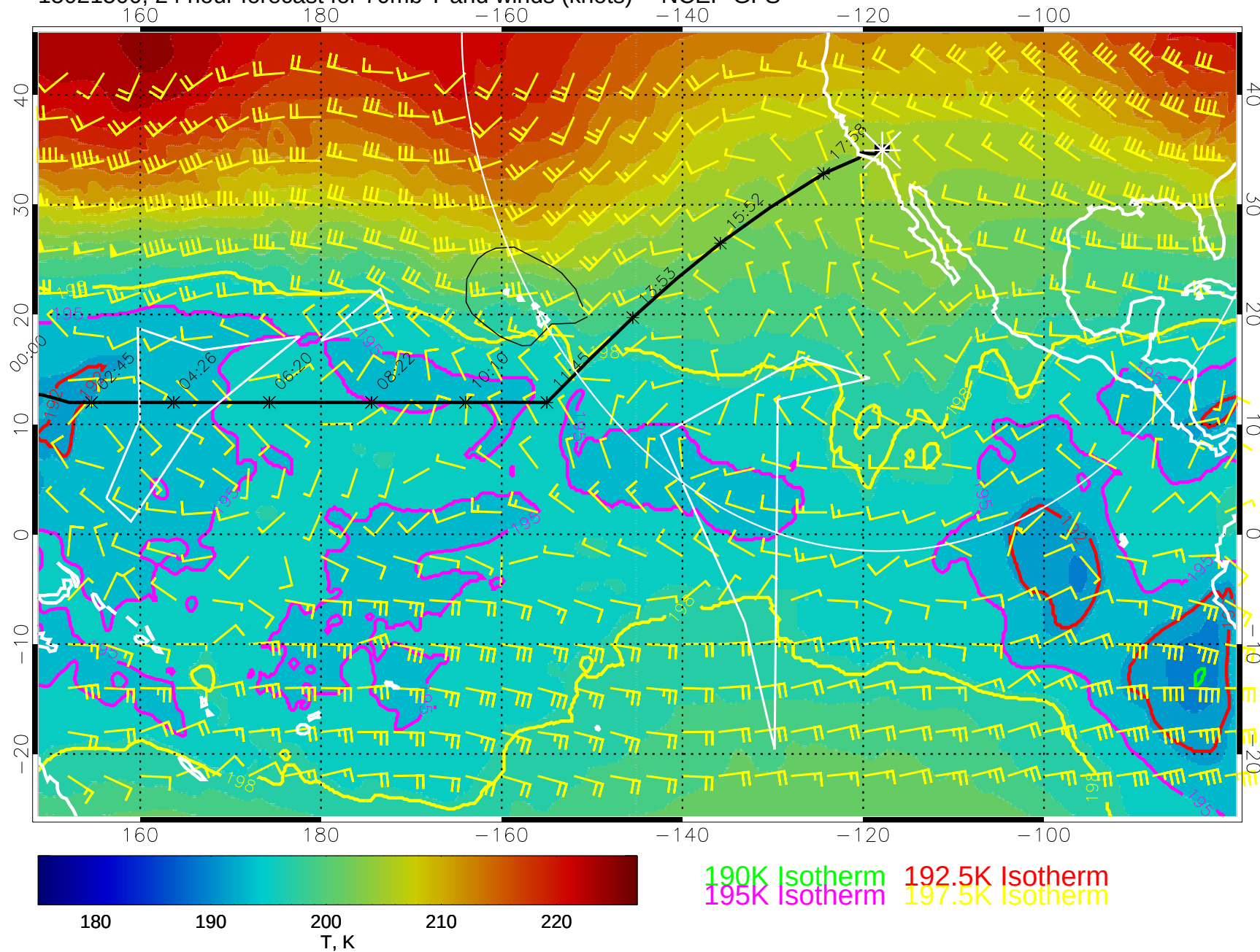
15021500, 24 hour forecast for 70mb T and winds (knots) -- NCEP GFS
