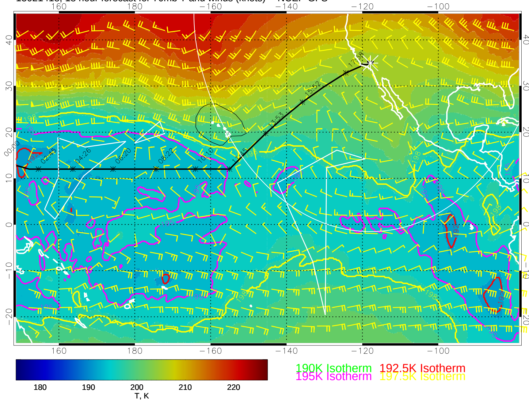
15021418, 18 hour forecast for 70mb T and winds (knots) -- NCEP GFS
