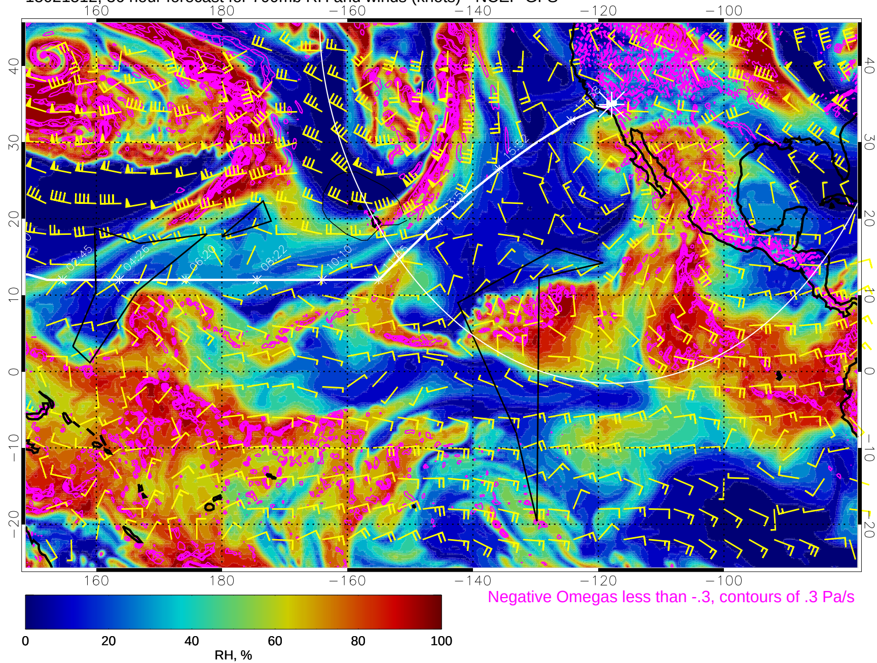
15021512, 36 hour forecast for 700mb RH and winds (knots) - NCEP GFS
