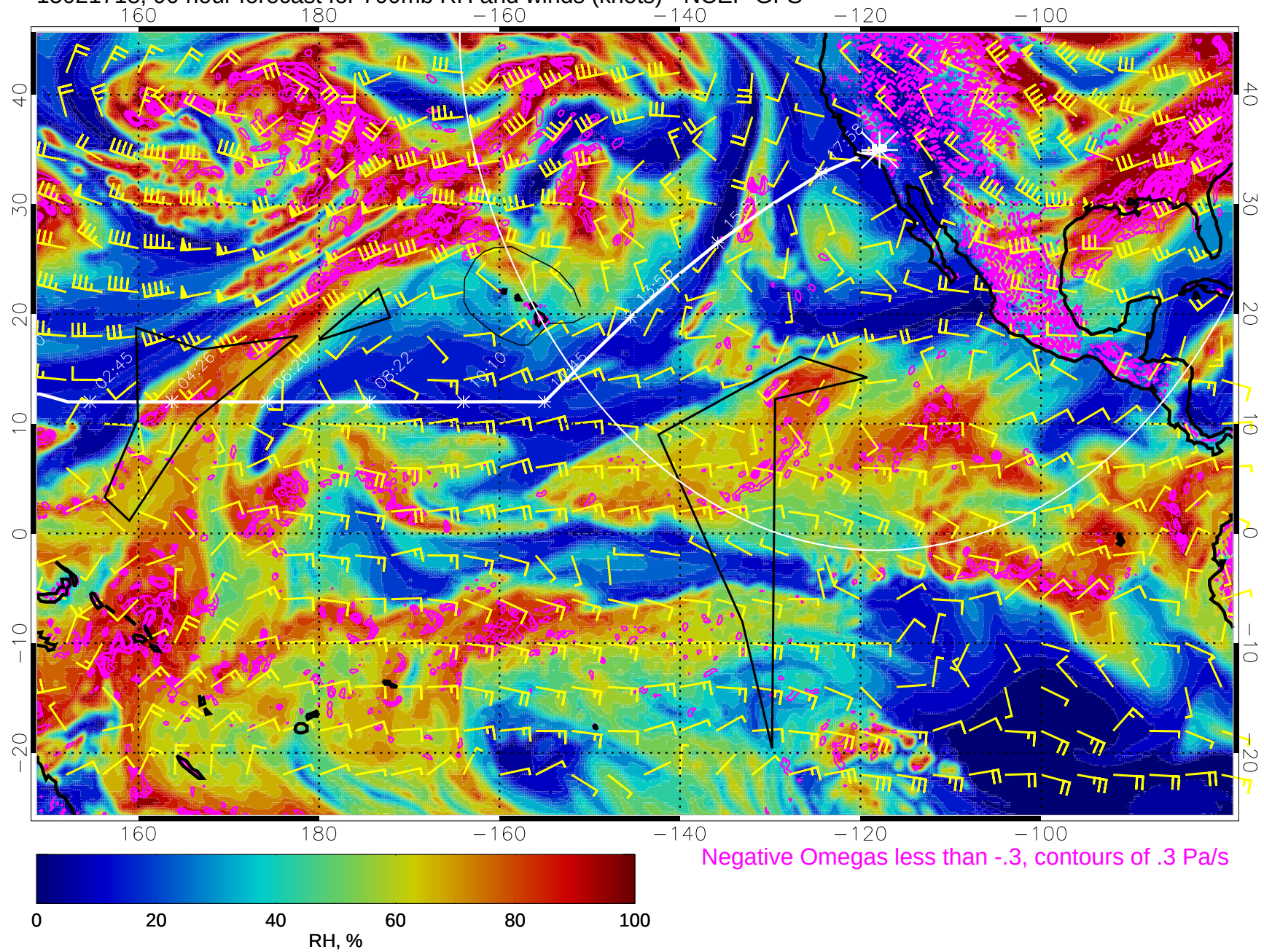
15021718, 90 hour forecast for 700mb RH and winds (knots) - NCEP GFS
