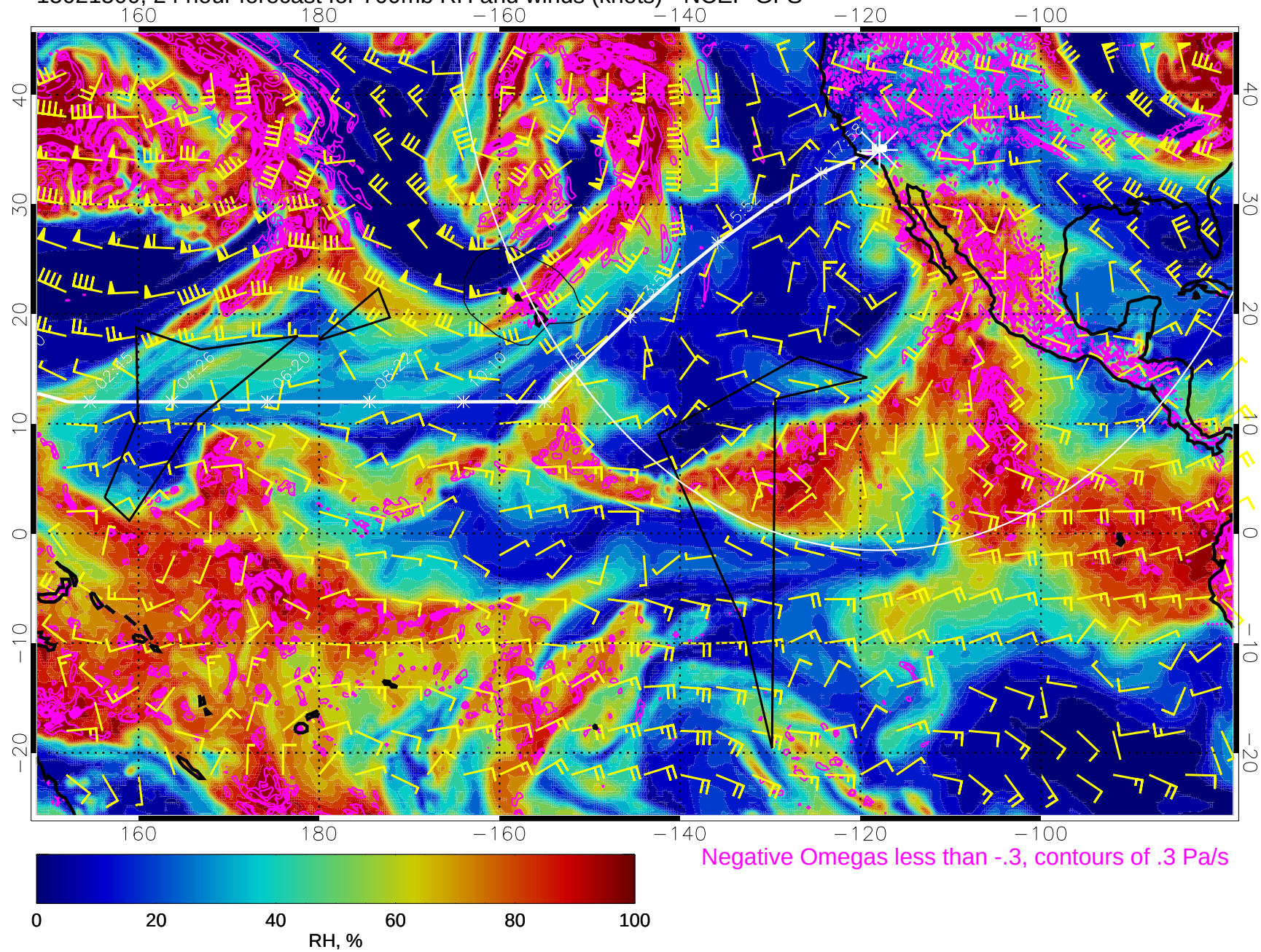
15021500, 24 hour forecast for 700mb RH and winds (knots) - NCEP GFS
