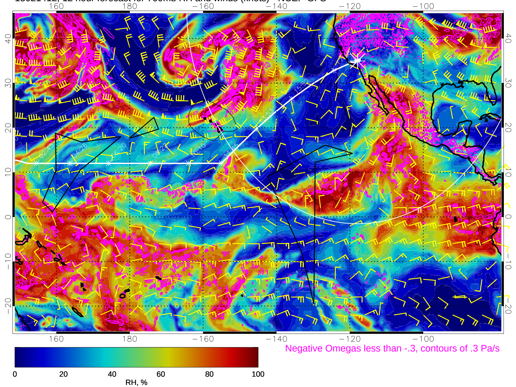
15021412, 12 hour forecast for 700mb RH and winds (knots) - NCEP GFS
