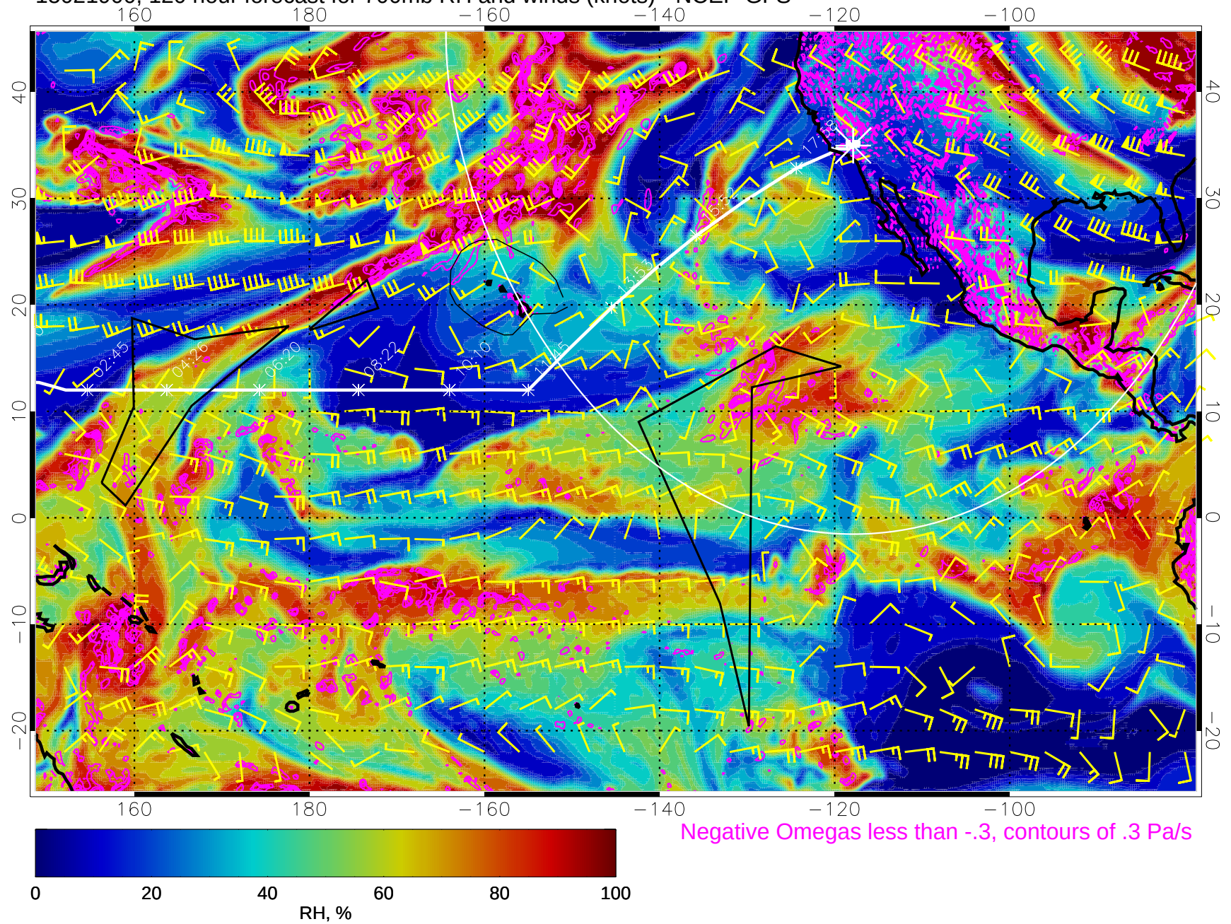
15021900, 120 hour forecast for 700mb RH and winds (knots) - NCEP GFS
