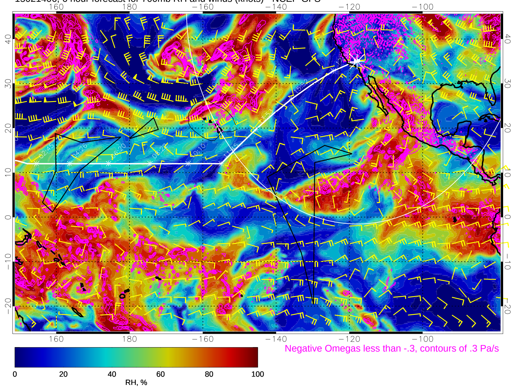
15021406, 6 hour forecast for 700mb RH and winds (knots) - NCEP GFS
