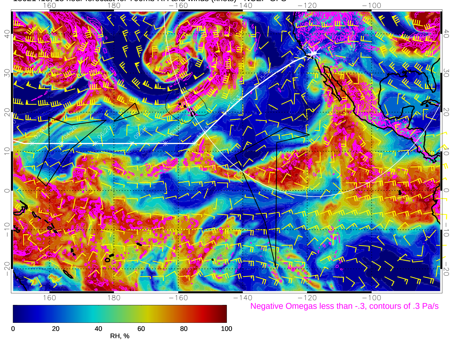
15021418, 18 hour forecast for 700mb RH and winds (knots) - NCEP GFS
