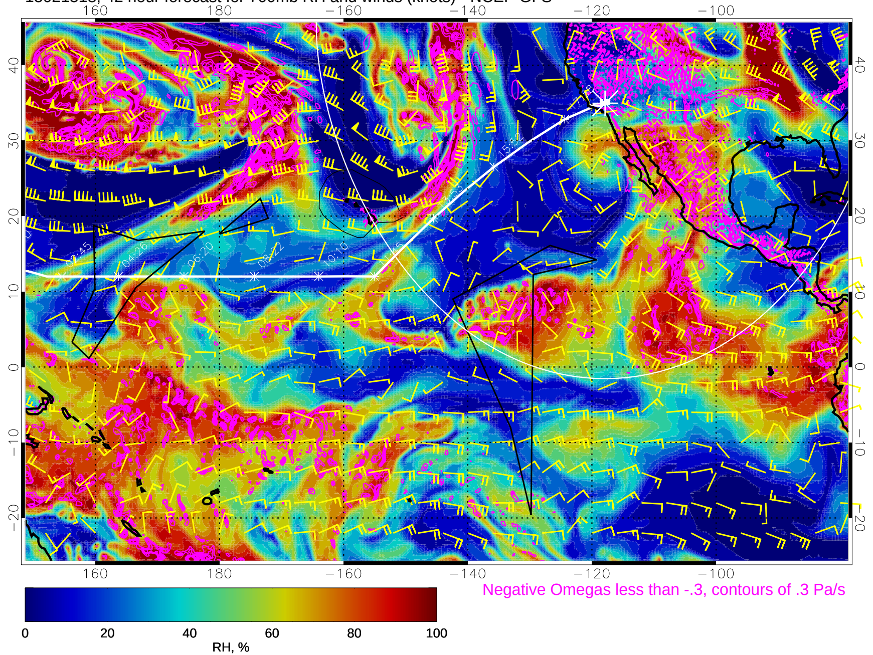
15021518, 42 hour forecast for 700mb RH and winds (knots) - NCEP GFS
