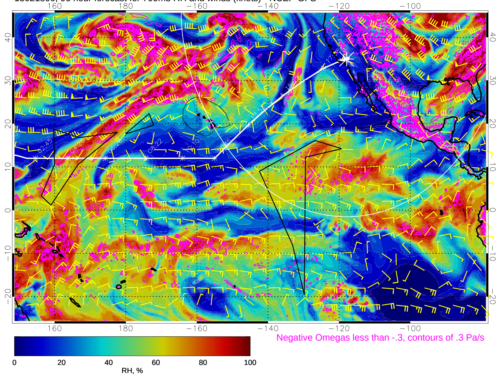
15021800, 96 hour forecast for 700mb RH and winds (knots) - NCEP GFS
