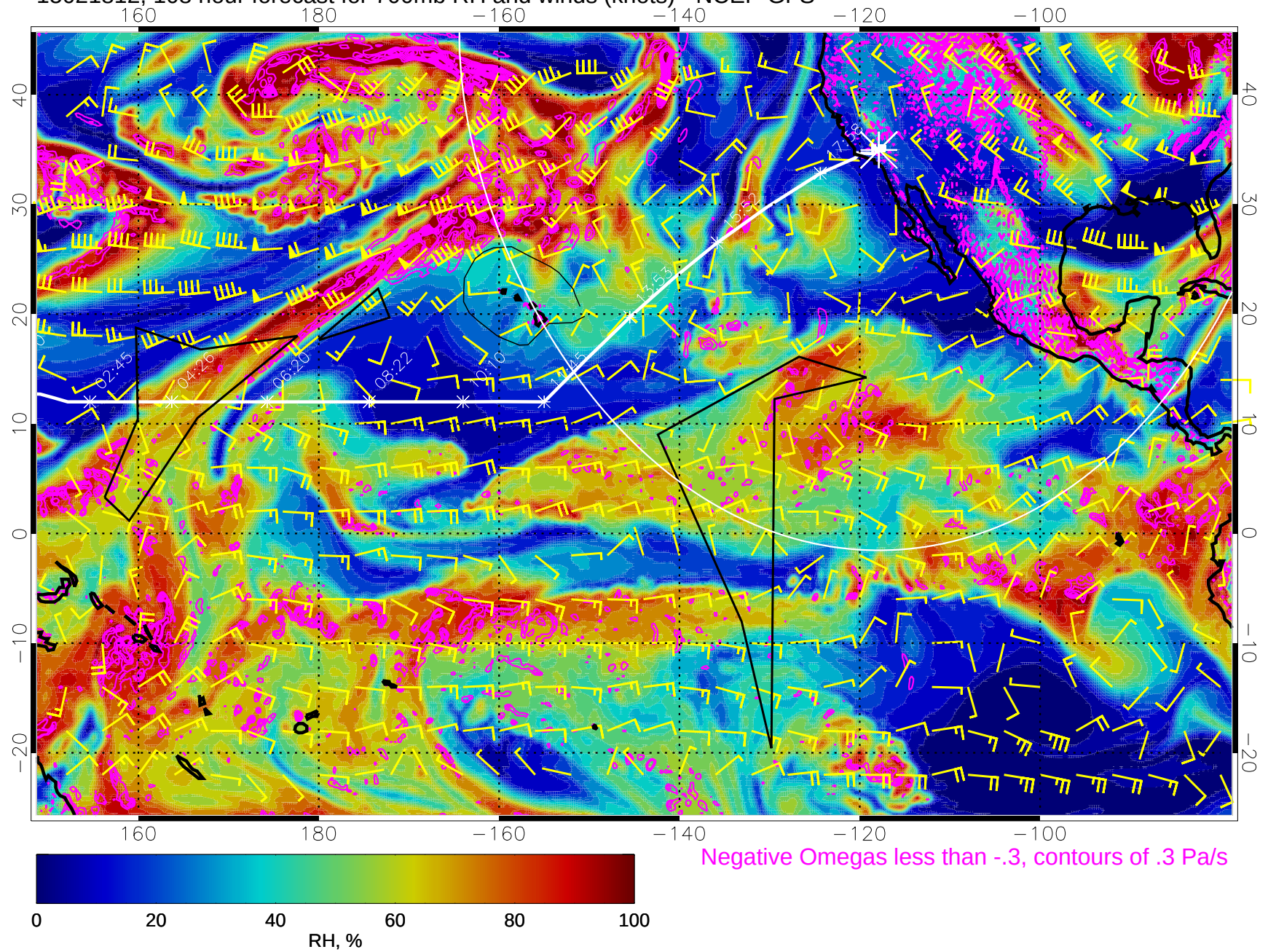
15021812, 108 hour forecast for 700mb RH and winds (knots) - NCEP GFS
