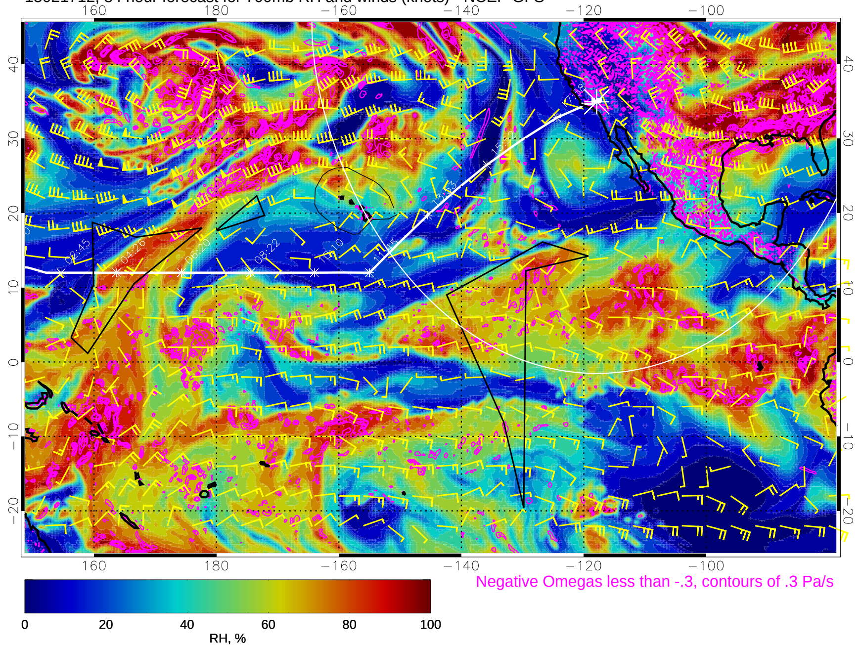
15021712, 84 hour forecast for 700mb RH and winds (knots) - NCEP GFS
