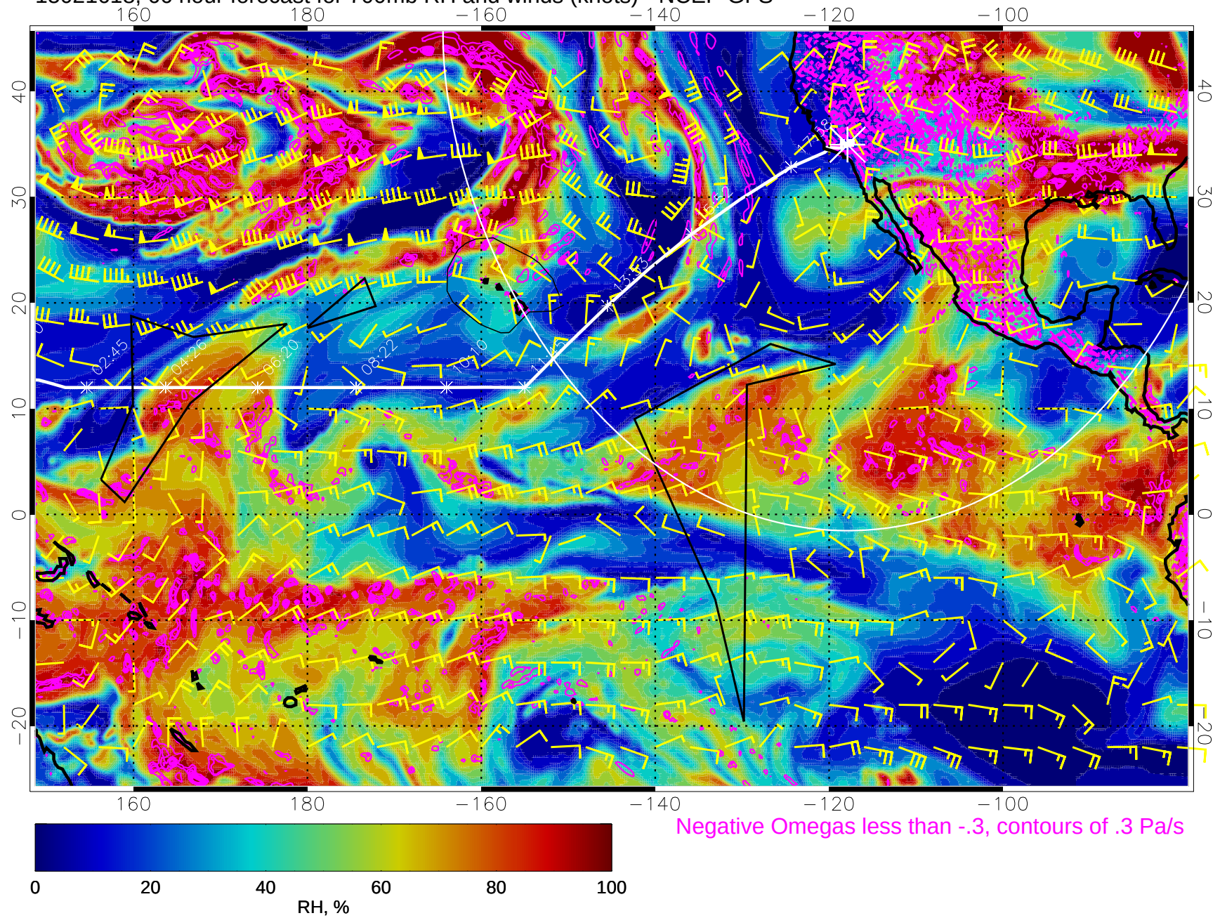
15021618, 66 hour forecast for 700mb RH and winds (knots) - NCEP GFS
