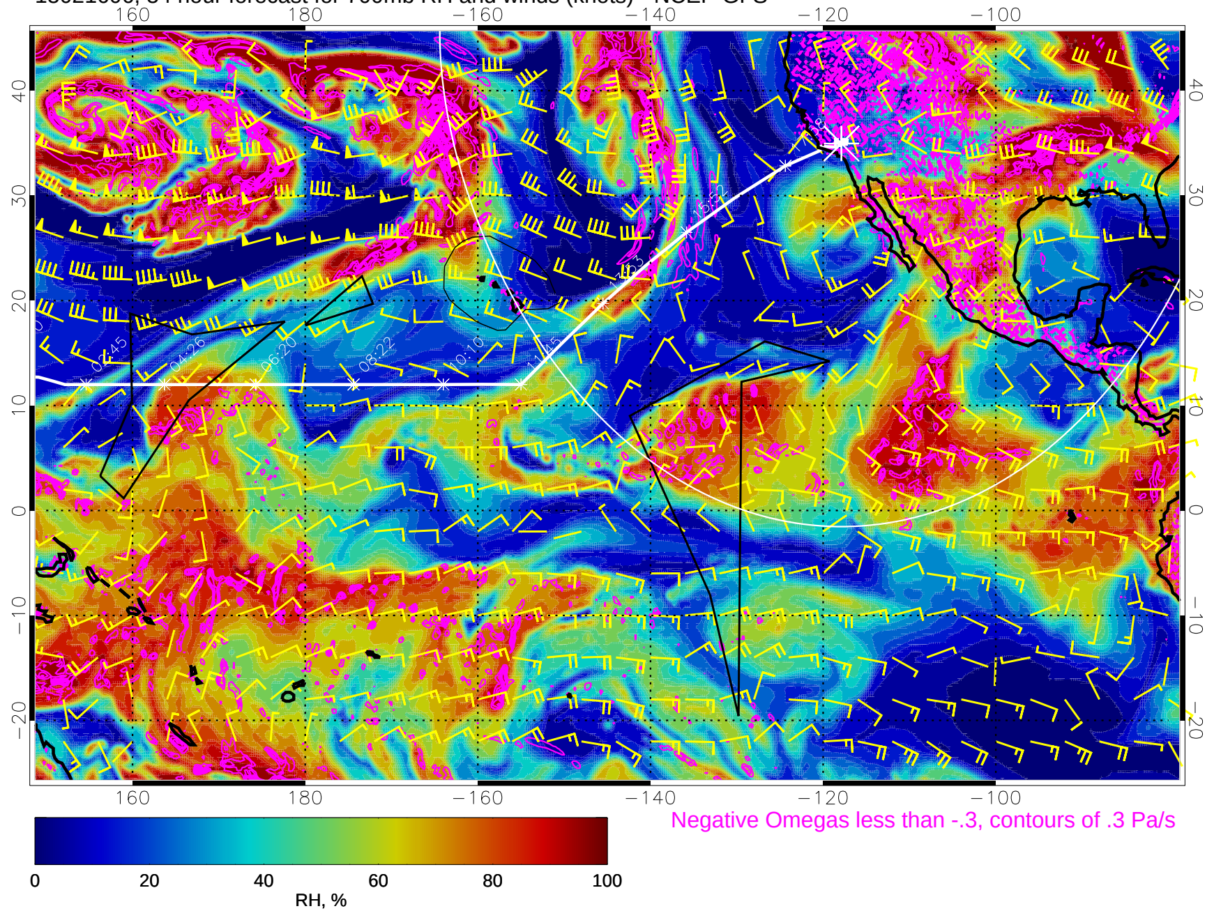
15021606, 54 hour forecast for 700mb RH and winds (knots) - NCEP GFS
