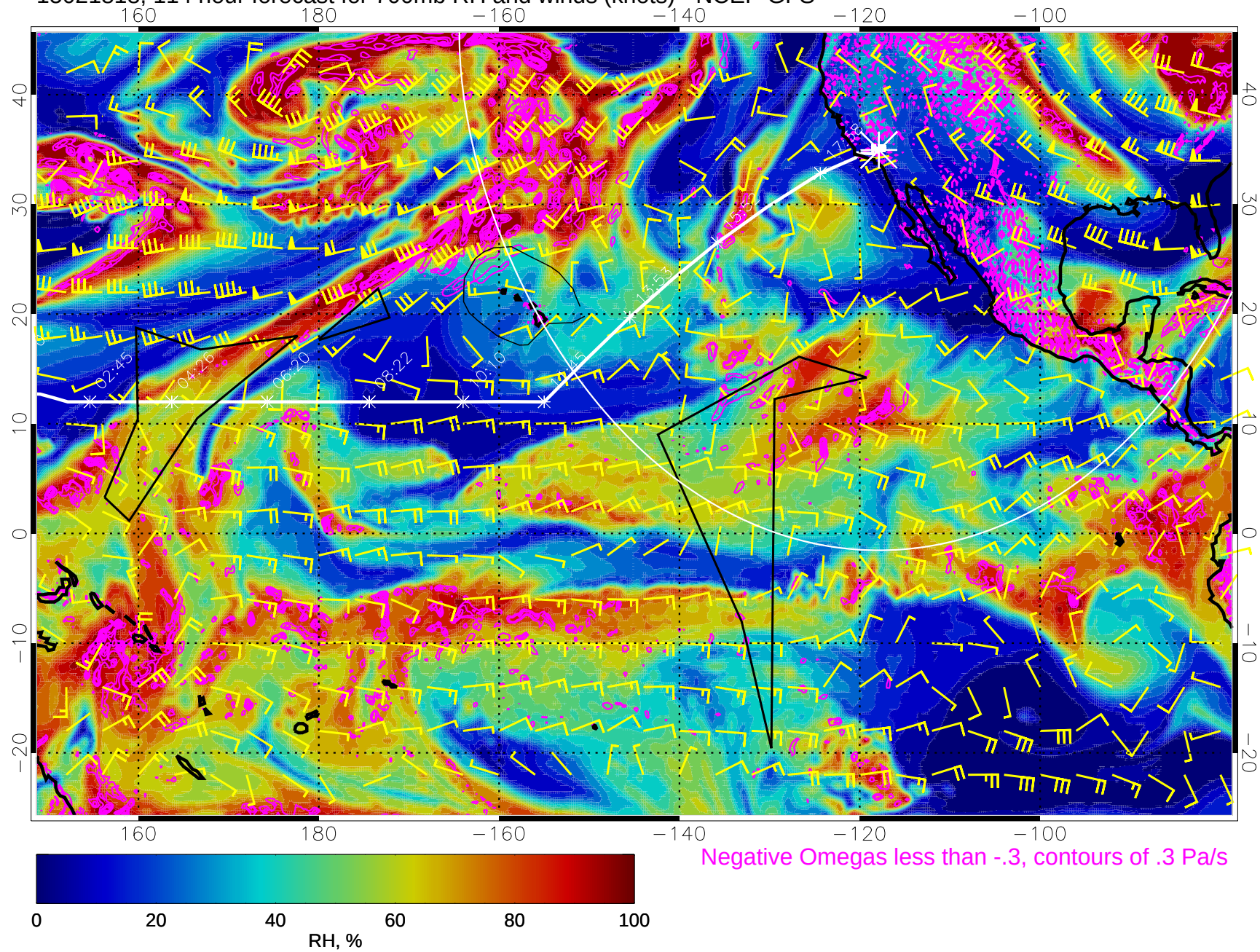
15021818, 114 hour forecast for 700mb RH and winds (knots) - NCEP GFS
