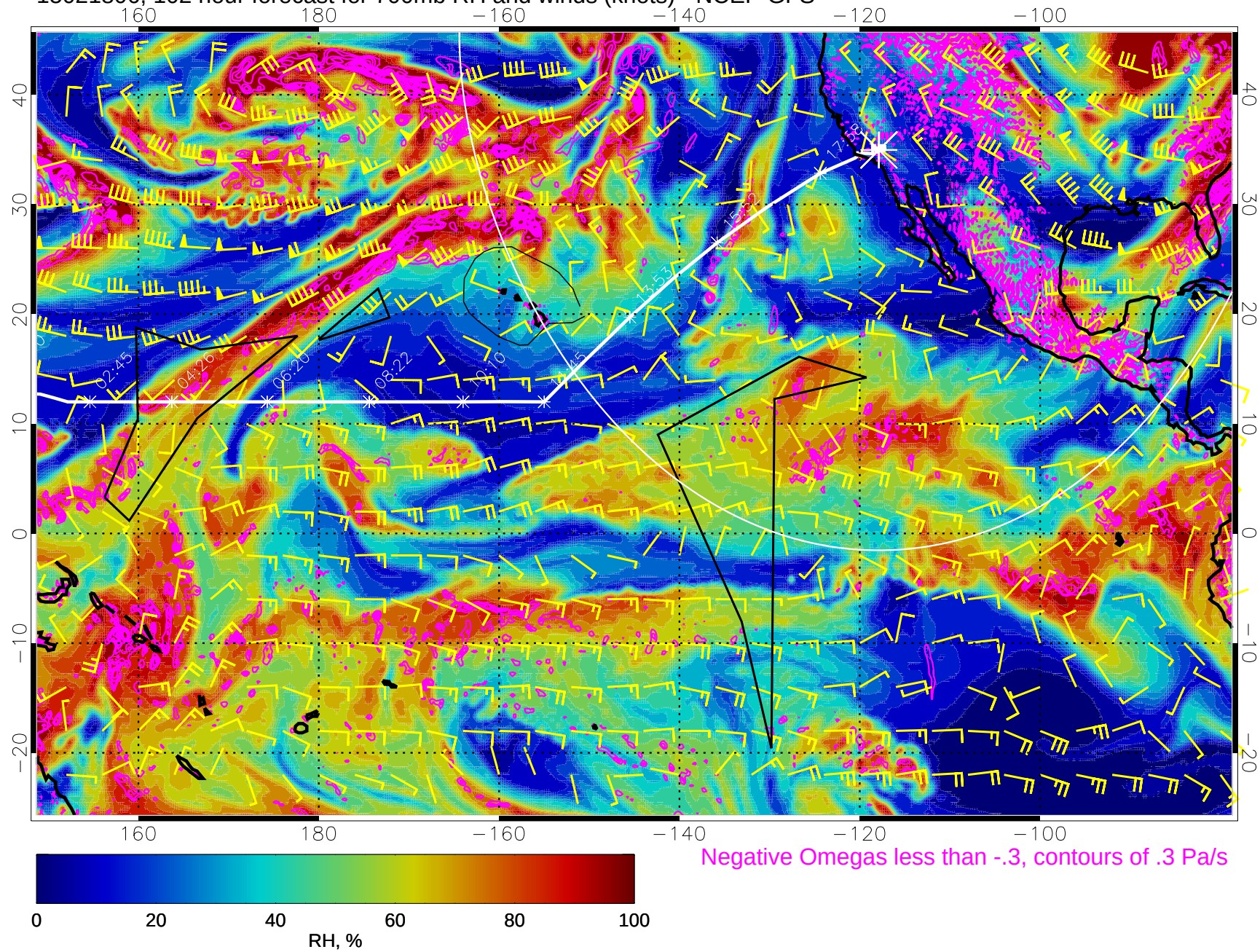
15021806, 102 hour forecast for 700mb RH and winds (knots) - NCEP GFS
