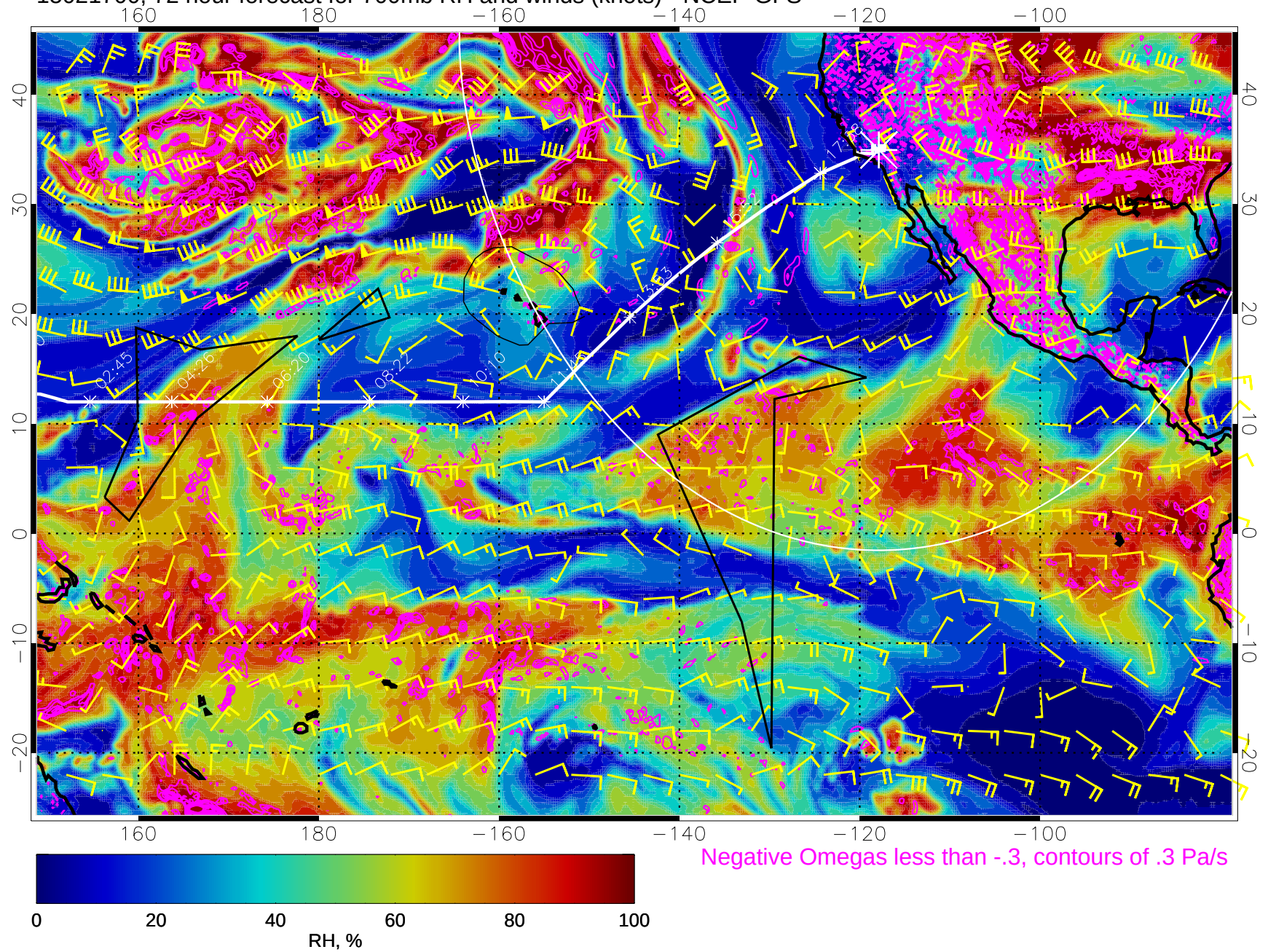
15021700, 72 hour forecast for 700mb RH and winds (knots) - NCEP GFS
