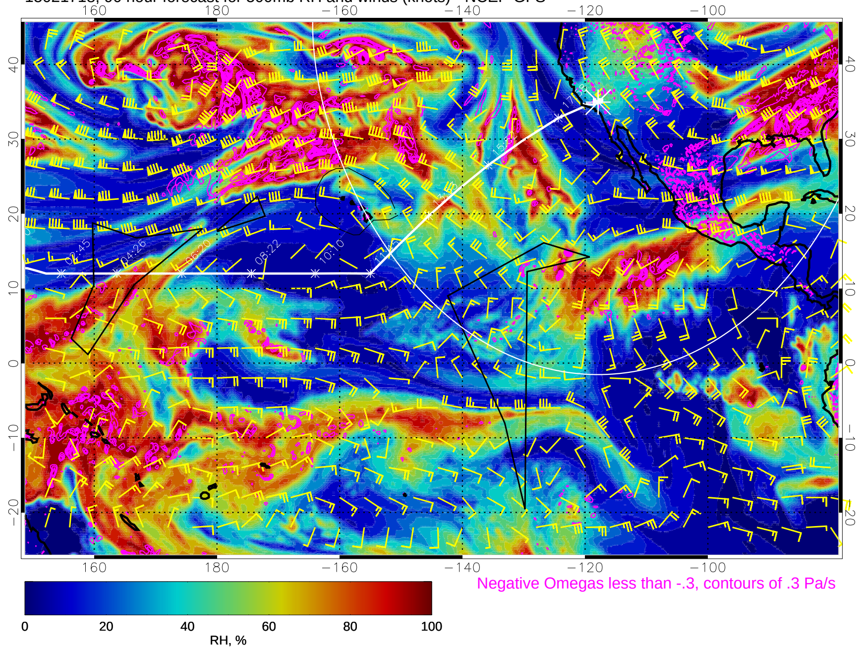
15021718, 90 hour forecast for 500mb RH and winds (knots) - NCEP GFS
