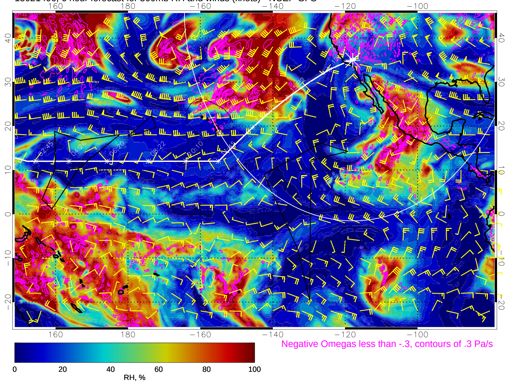
15021406, 6 hour forecast for 500mb RH and winds (knots) - NCEP GFS
