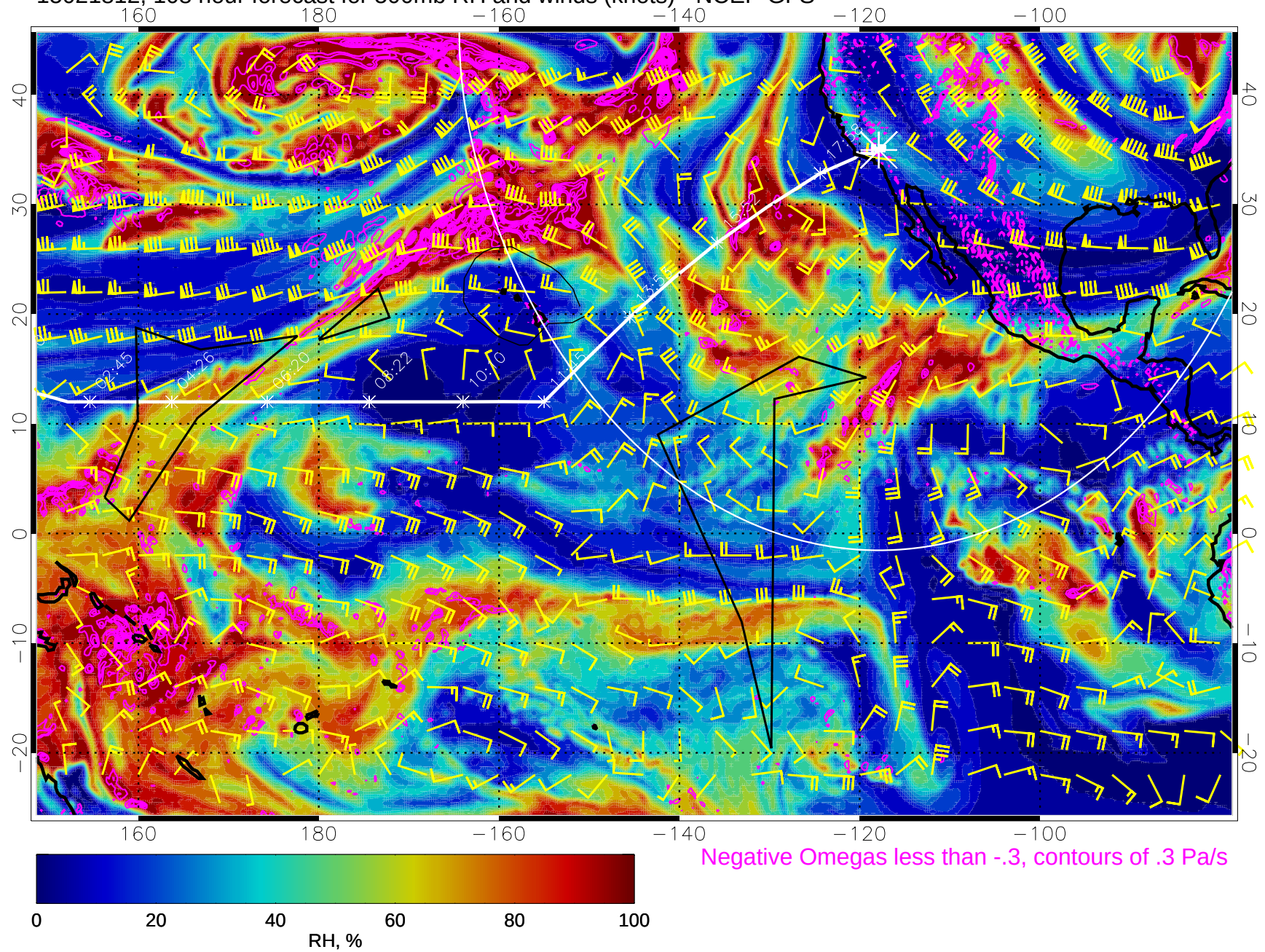
15021812, 108 hour forecast for 500mb RH and winds (knots) - NCEP GFS
