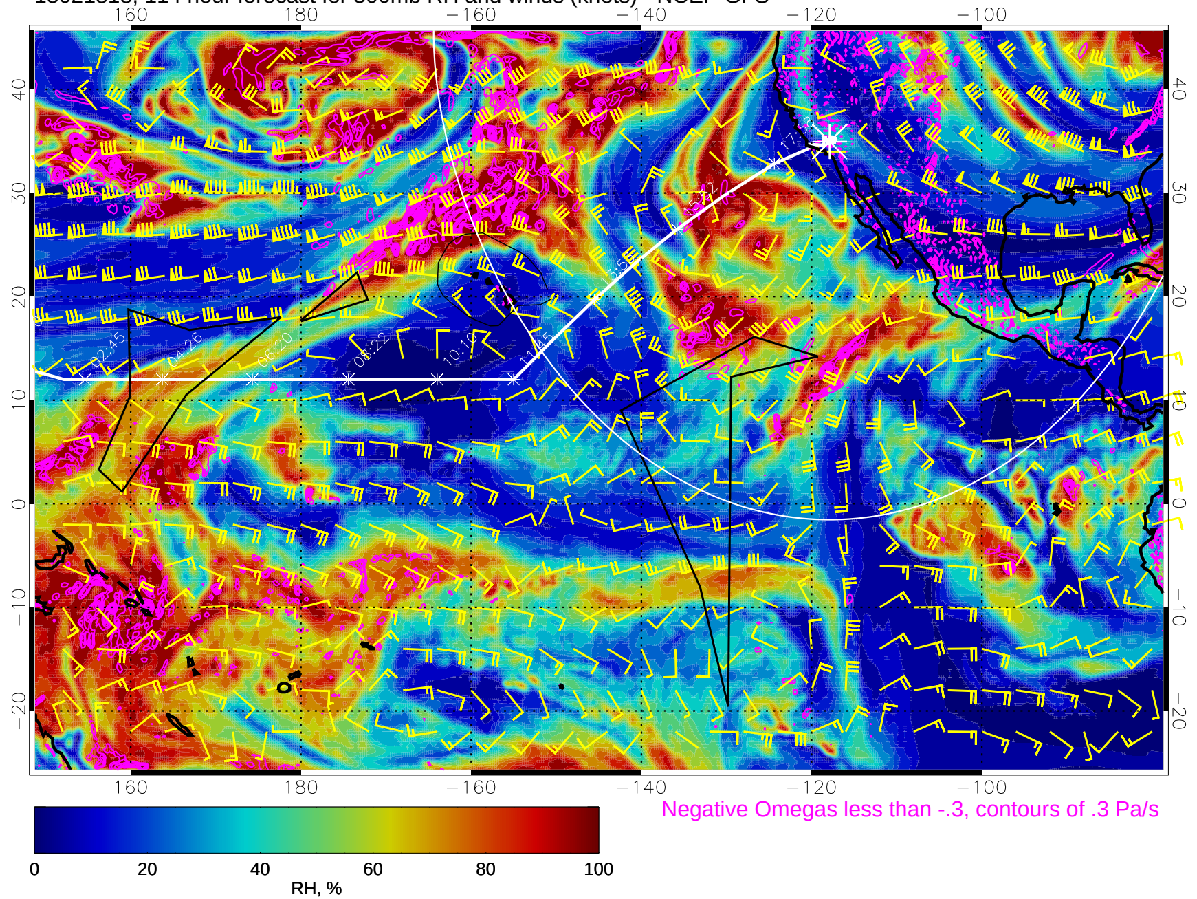
15021818, 114 hour forecast for 500mb RH and winds (knots) - NCEP GFS
