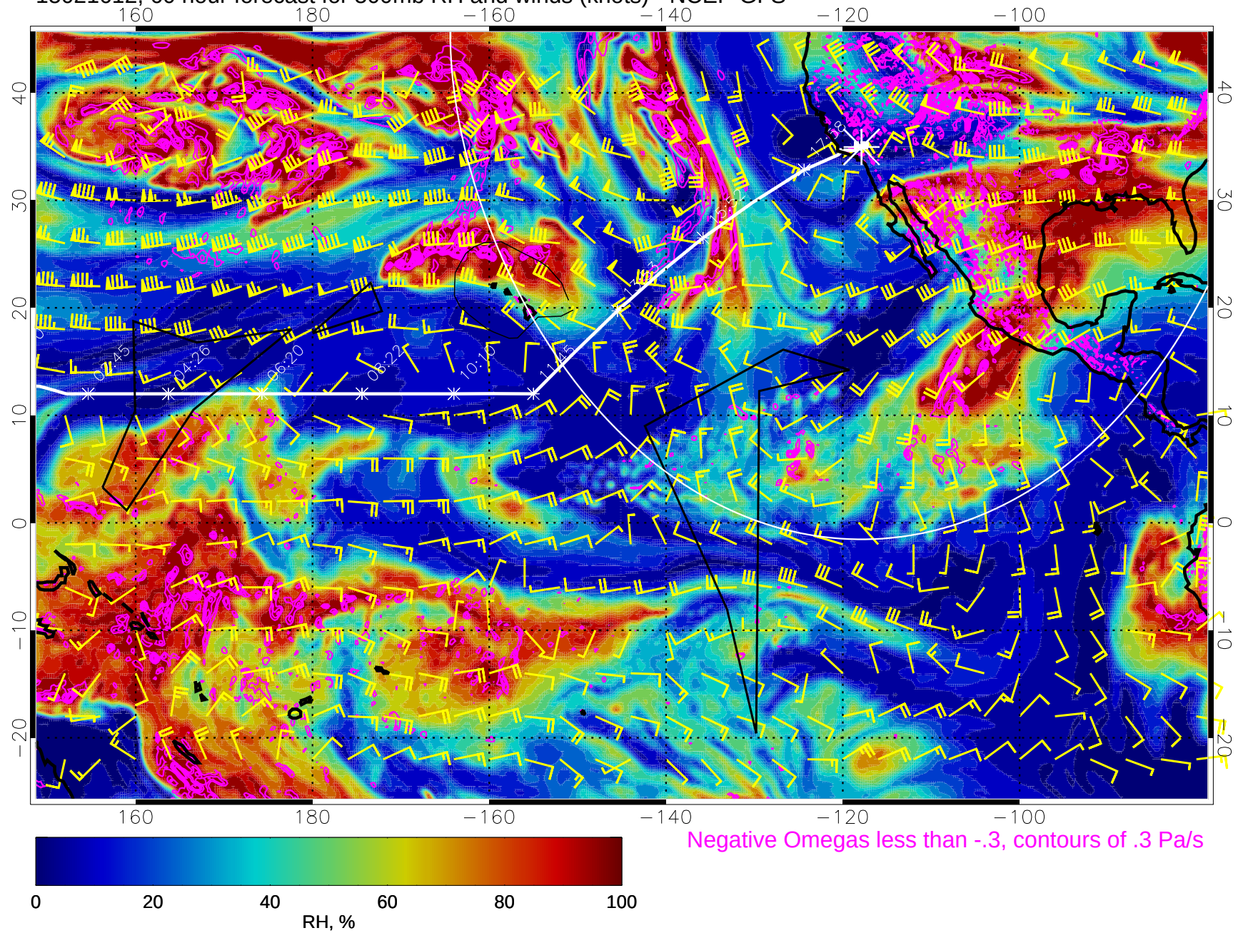
15021612, 60 hour forecast for 500mb RH and winds (knots) - NCEP GFS
