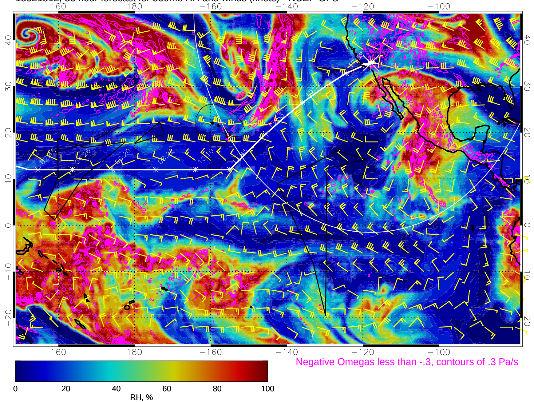
15021512, 36 hour forecast for 500mb RH and winds (knots) - NCEP GFS
