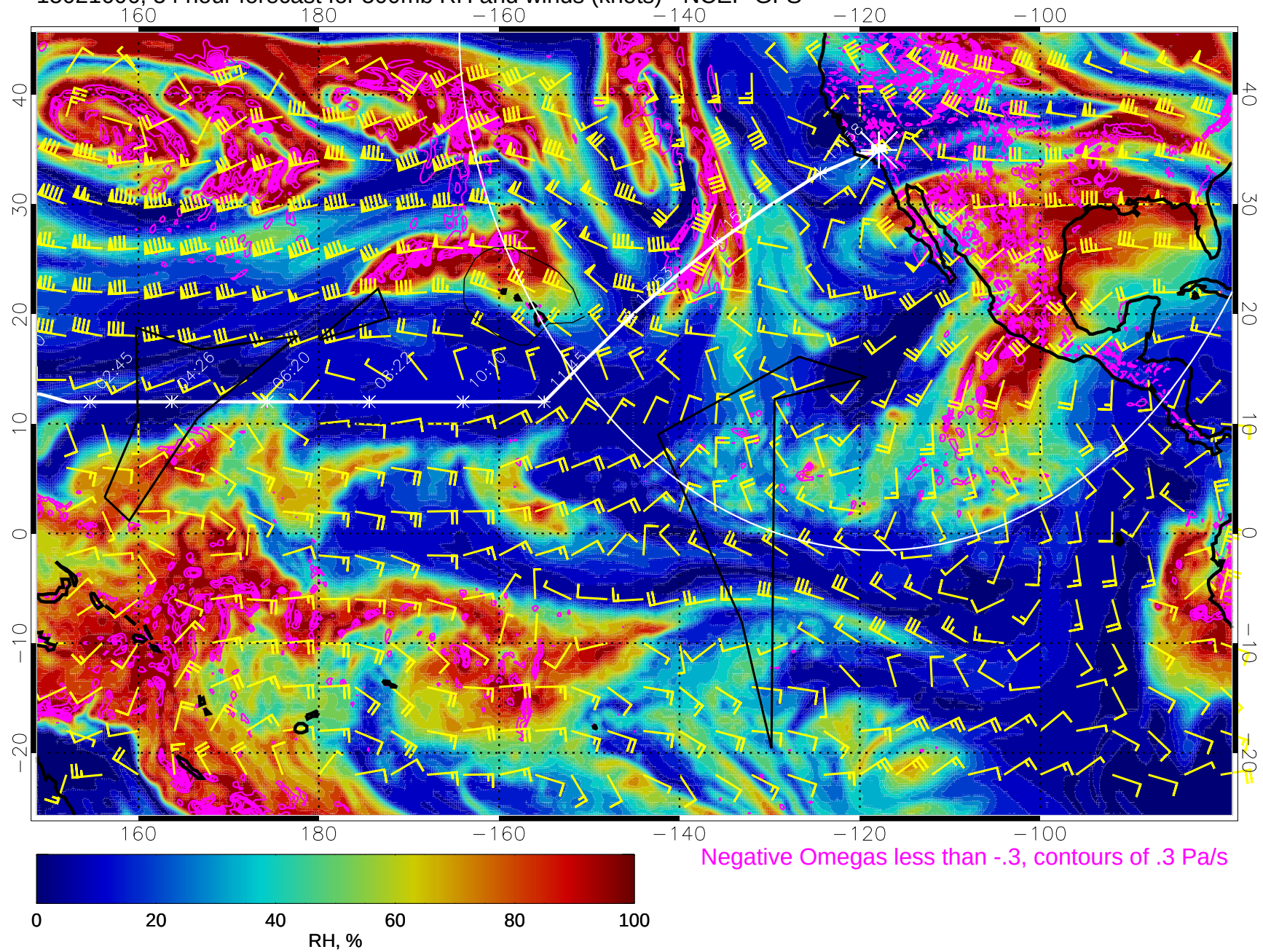
15021606, 54 hour forecast for 500mb RH and winds (knots) - NCEP GFS
