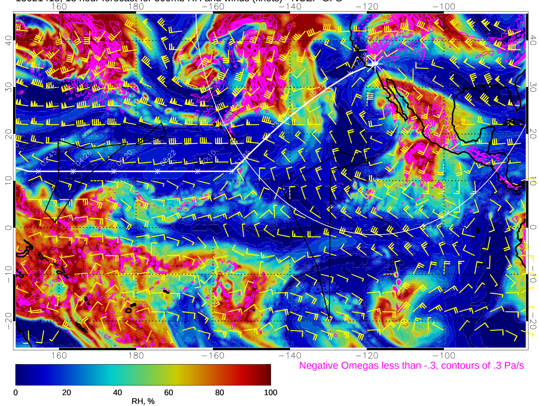
15021418, 18 hour forecast for 500mb RH and winds (knots) - NCEP GFS
