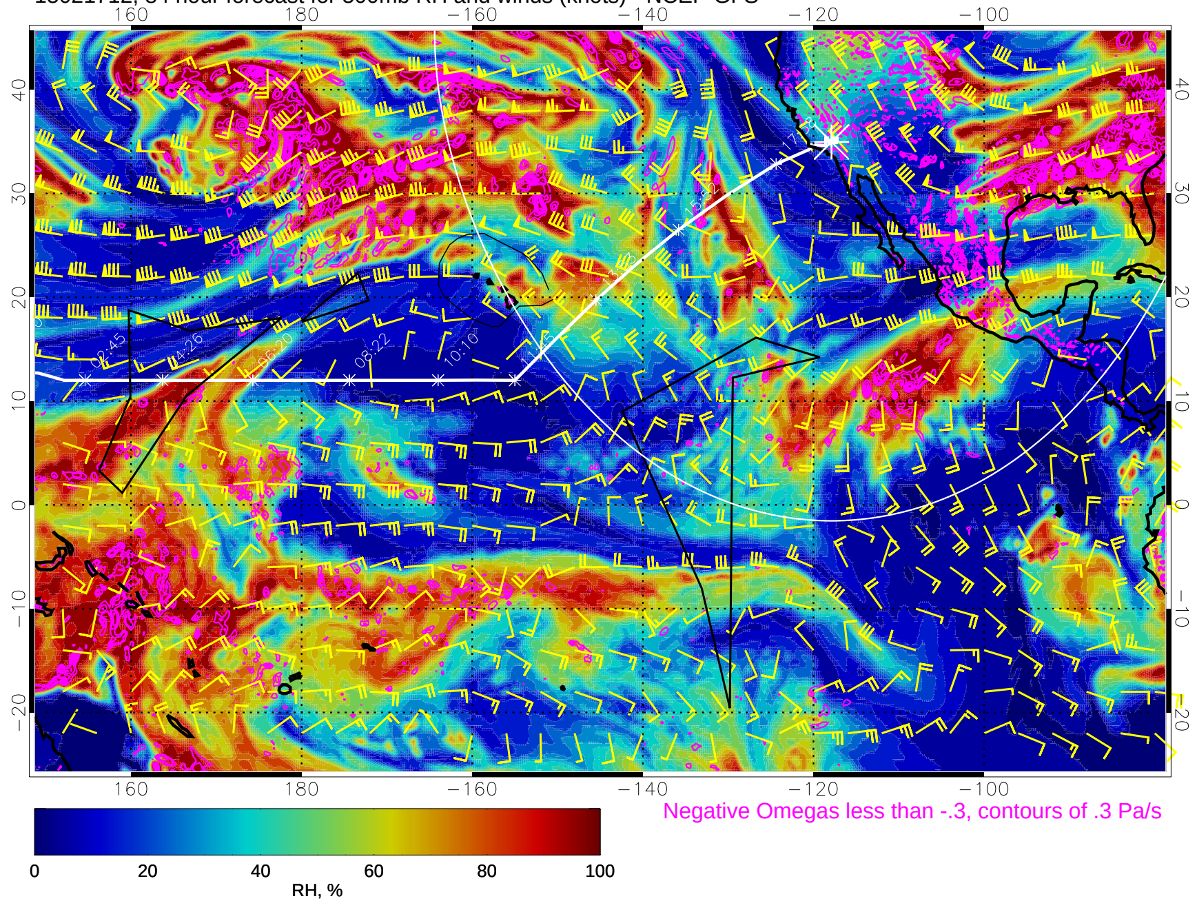
15021712, 84 hour forecast for 500mb RH and winds (knots) - NCEP GFS
