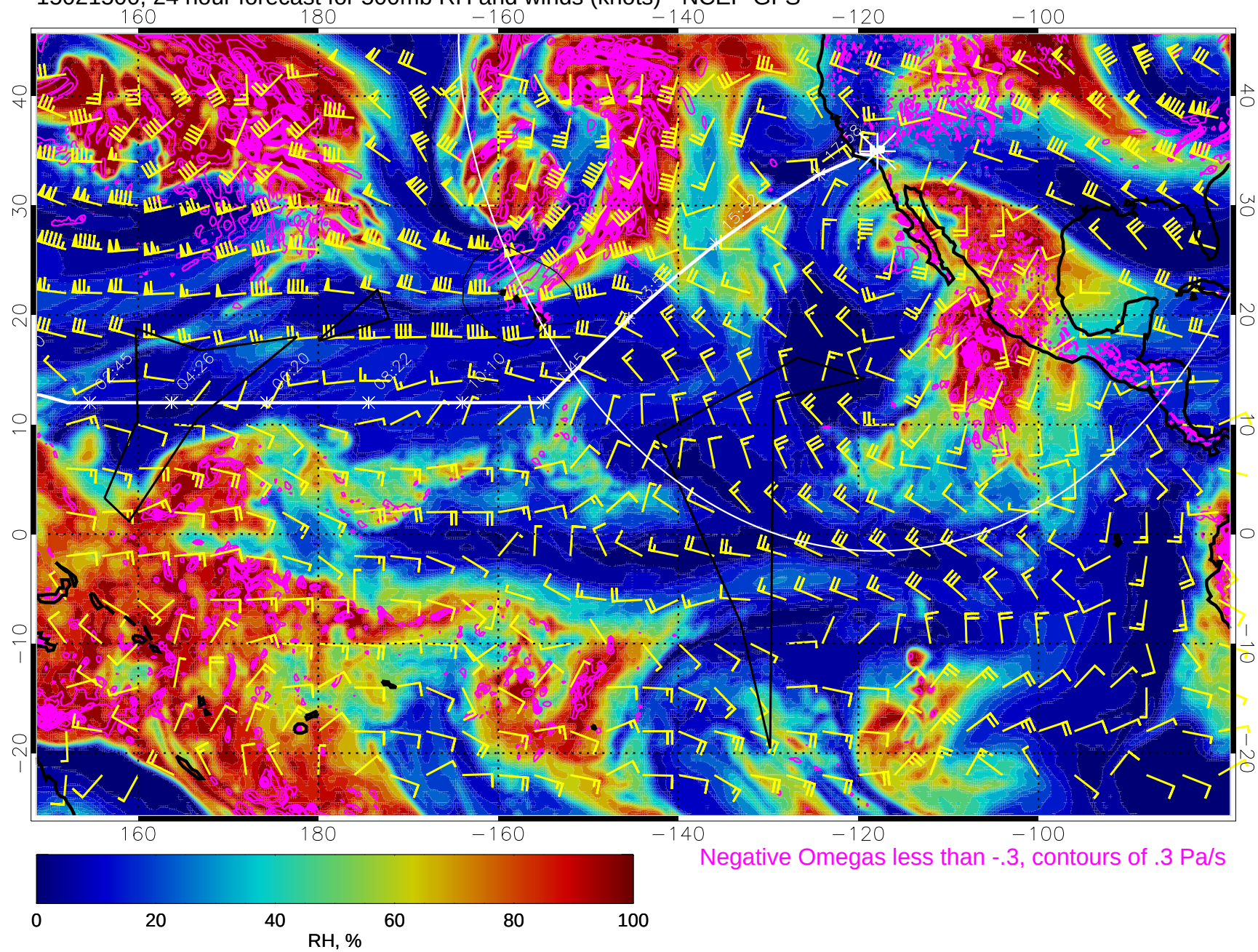
15021500, 24 hour forecast for 500mb RH and winds (knots) - NCEP GFS
