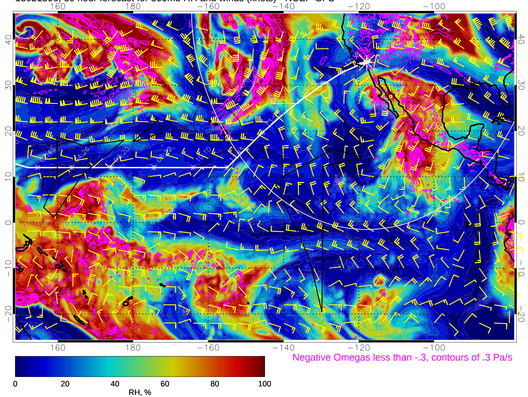
15021506, 30 hour forecast for 500mb RH and winds (knots) - NCEP GFS
