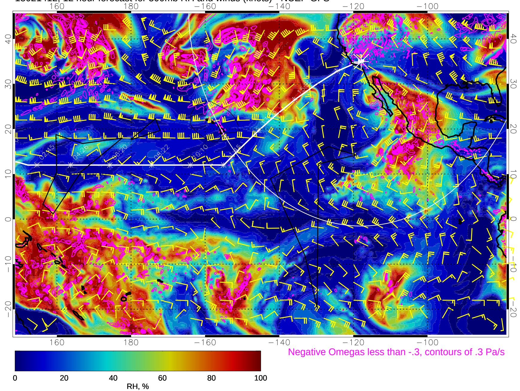
15021412, 12 hour forecast for 500mb RH and winds (knots) - NCEP GFS
