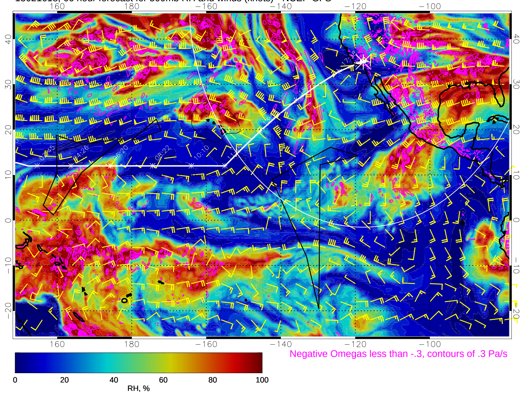
15021618, 66 hour forecast for 500mb RH and winds (knots) - NCEP GFS
