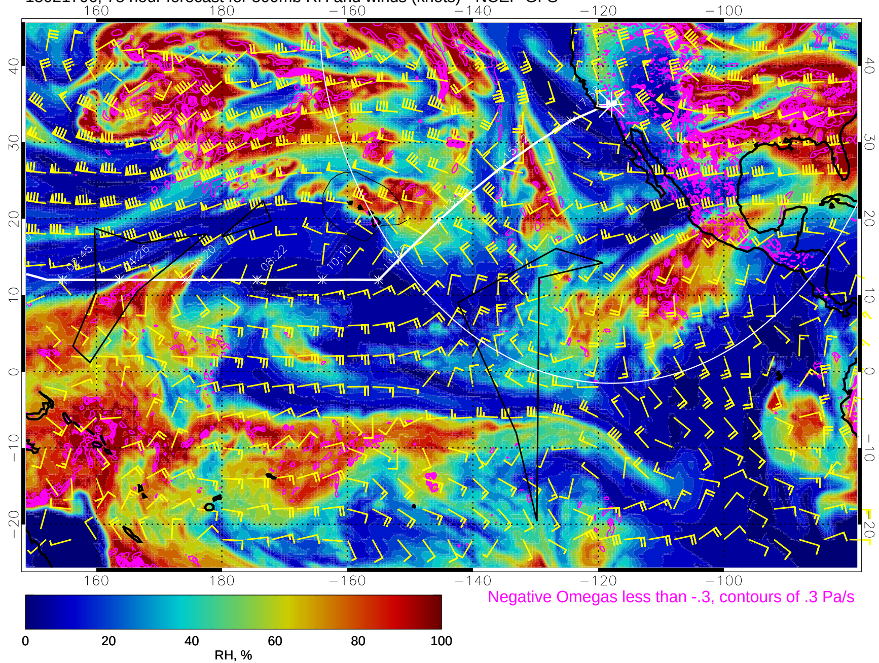
15021706, 78 hour forecast for 500mb RH and winds (knots) - NCEP GFS
