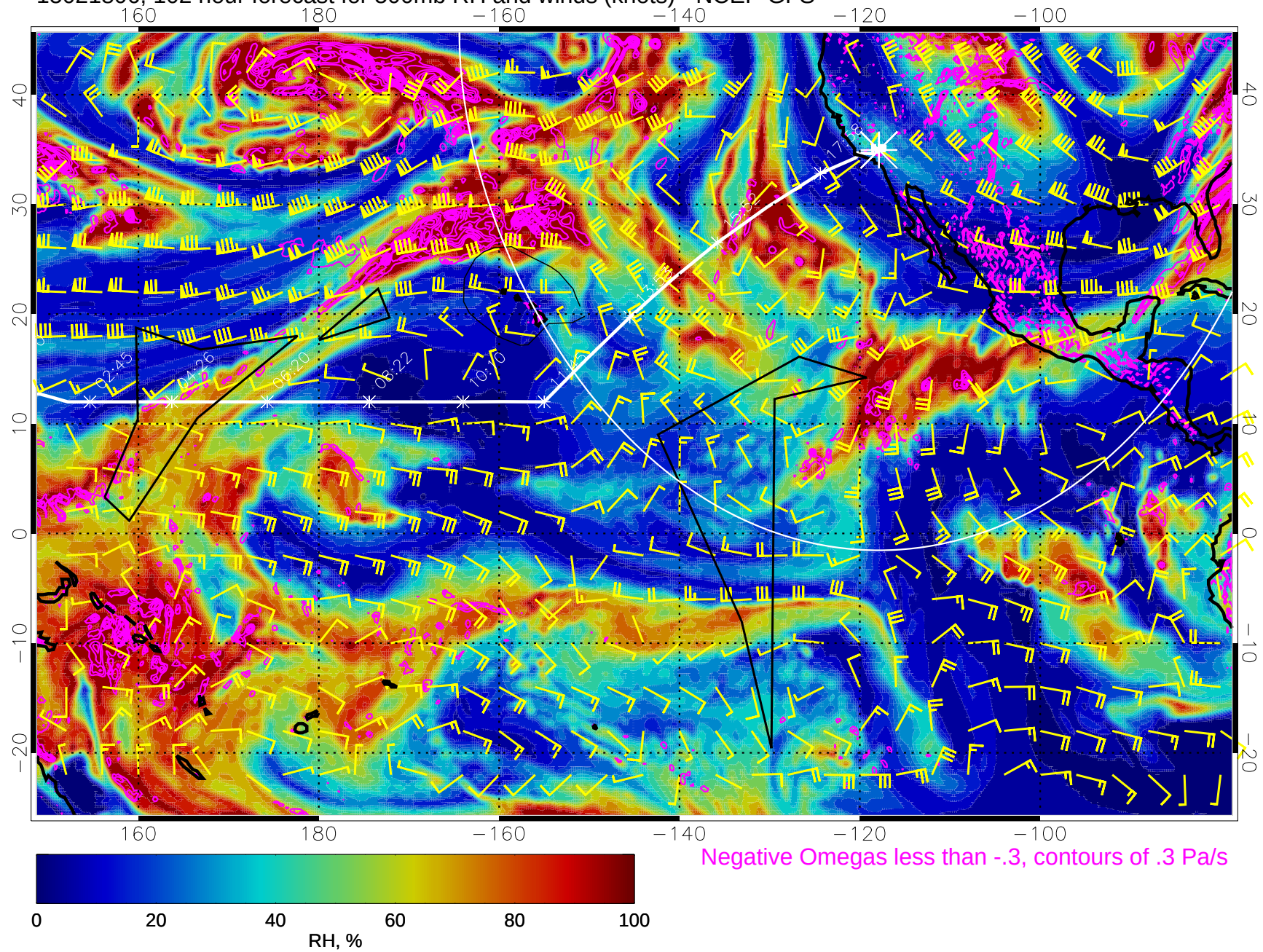
15021806, 102 hour forecast for 500mb RH and winds (knots) - NCEP GFS
