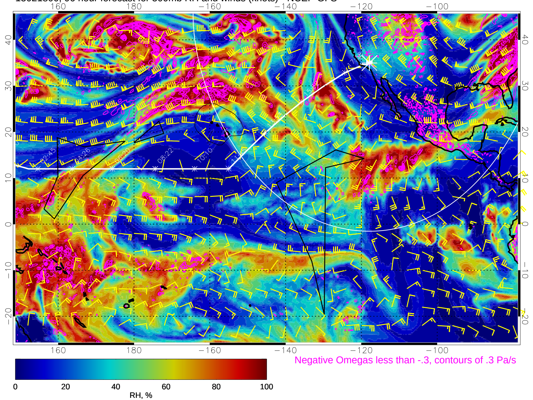
15021800, 96 hour forecast for 500mb RH and winds (knots) - NCEP GFS
