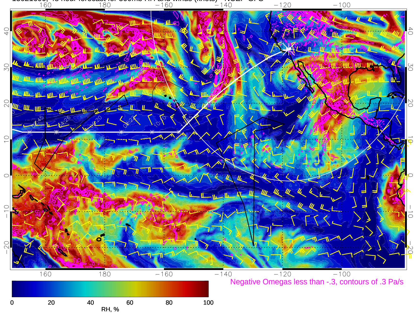
15021600, 48 hour forecast for 500mb RH and winds (knots) - NCEP GFS
