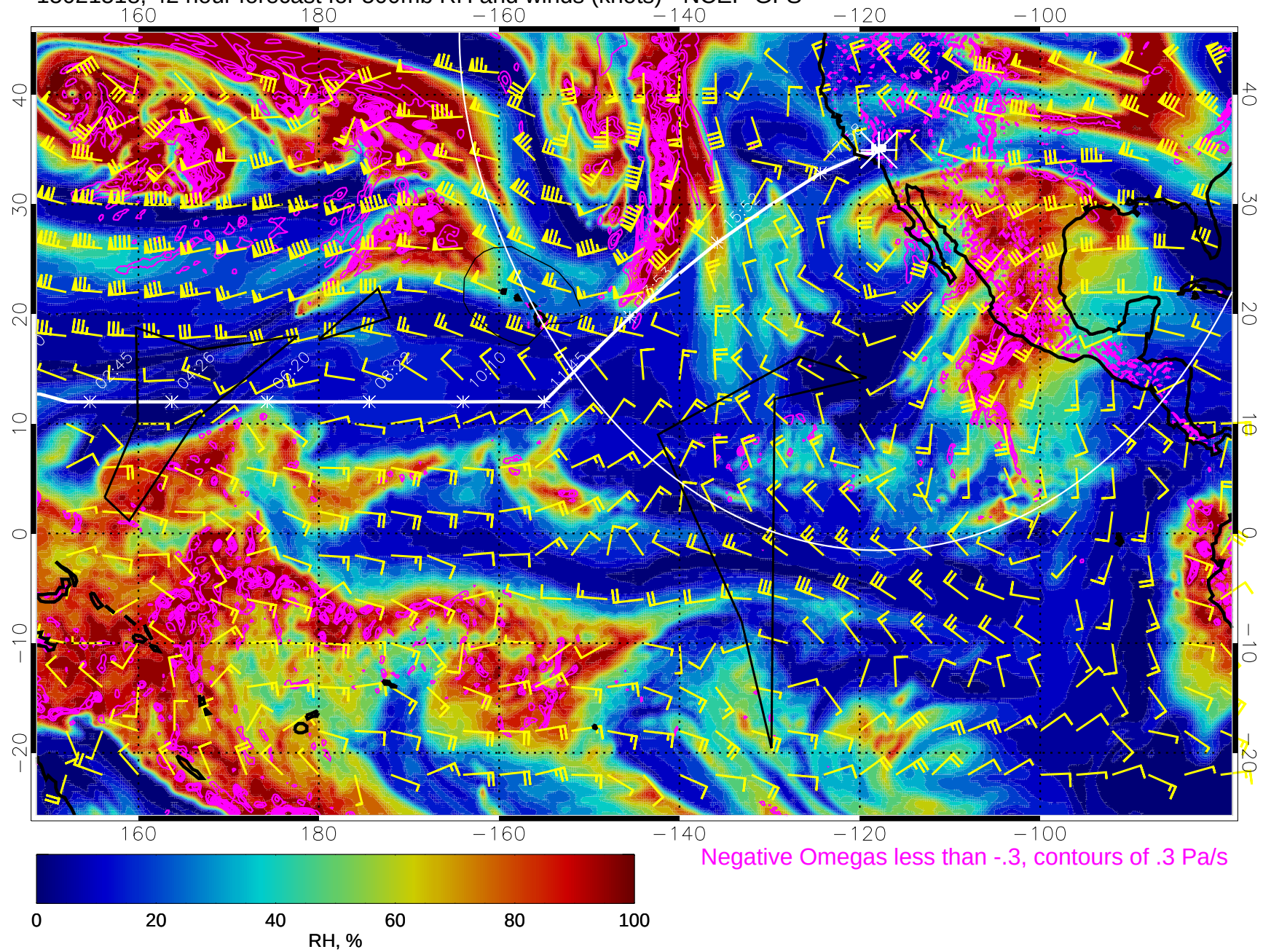
15021518, 42 hour forecast for 500mb RH and winds (knots) - NCEP GFS
