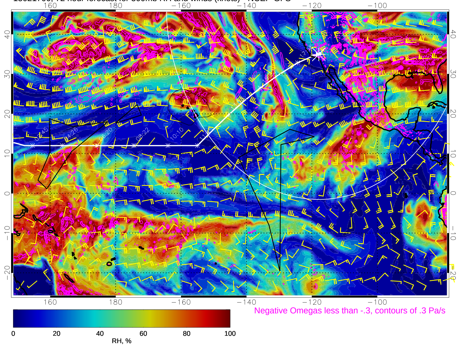
15021700, 72 hour forecast for 500mb RH and winds (knots) - NCEP GFS
