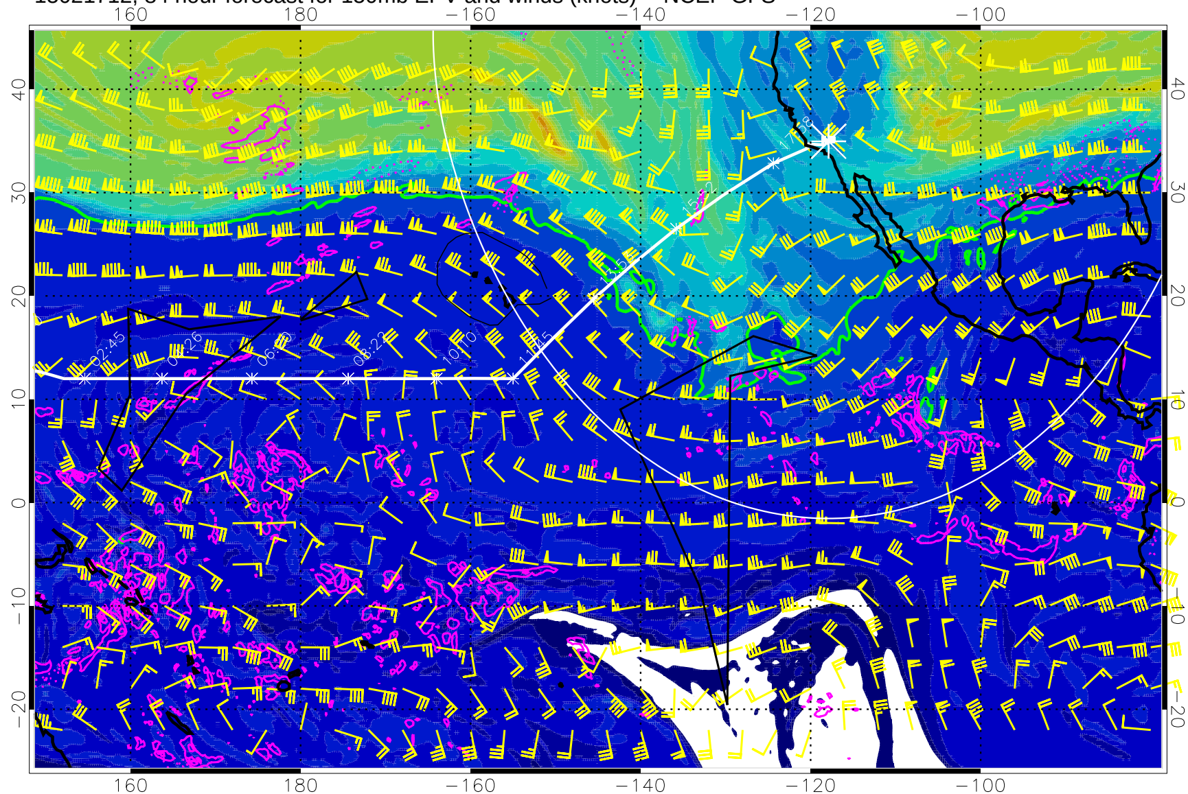
15021712, 84 hour forecast for 150mb EPV and winds (knots) -- NCEP GFS
