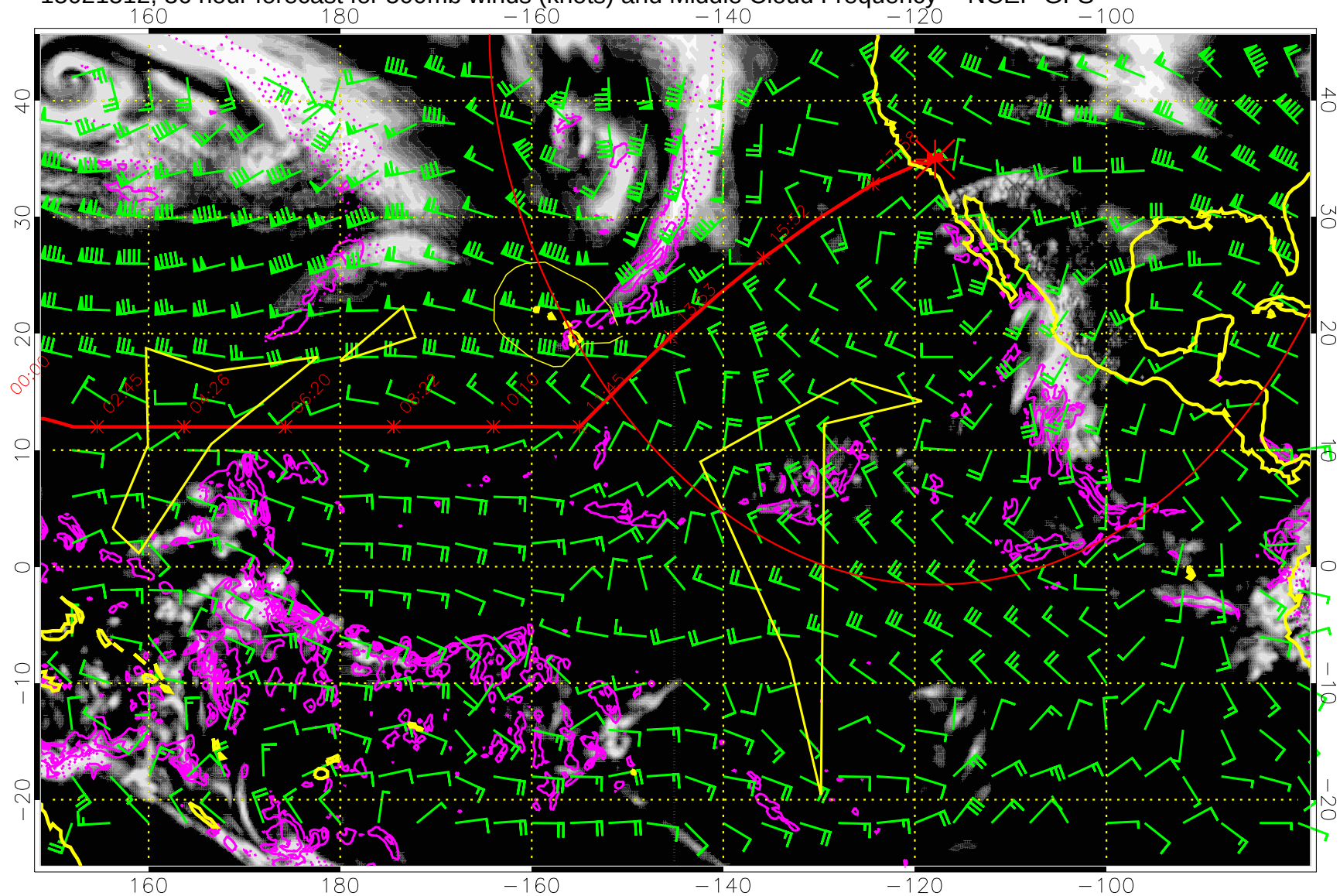
15021512, 36 hour forecast for 500mb winds (knots) and Middle Cloud Frequency -- NCEP GFS
