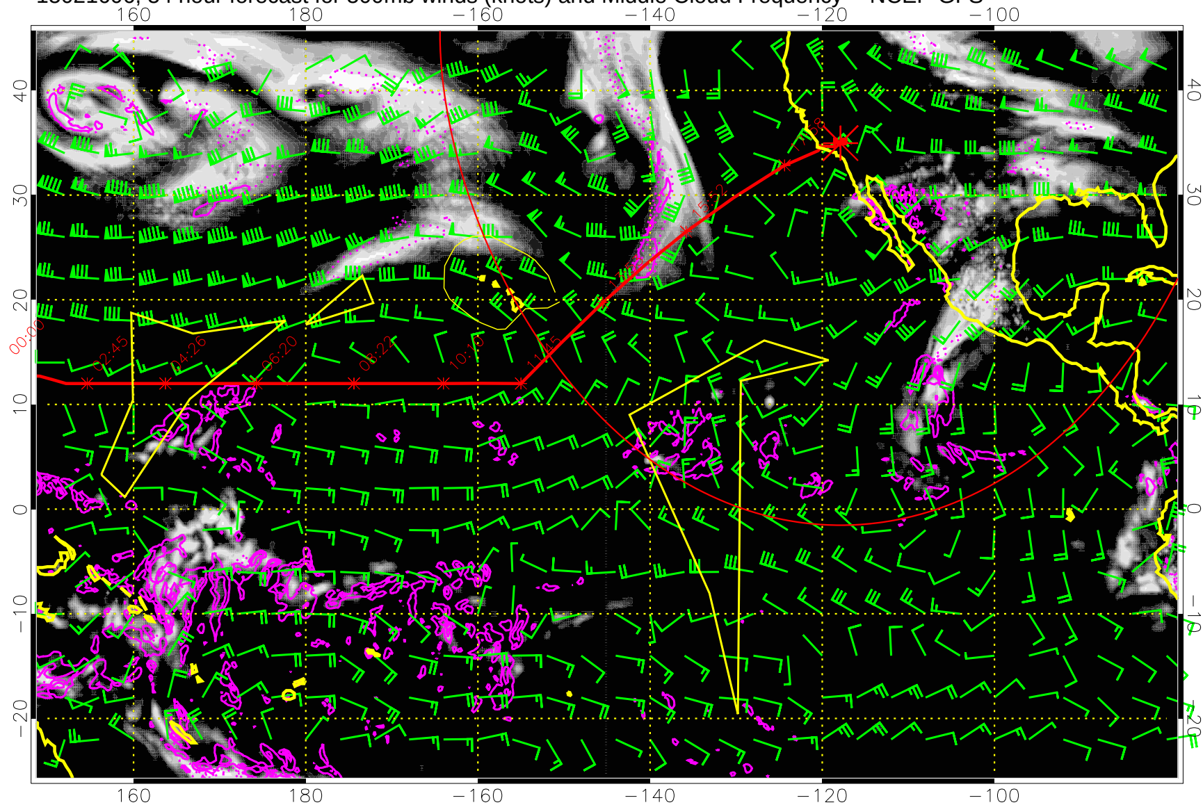
15021606, 54 hour forecast for 500mb winds (knots) and Middle Cloud Frequency -- NCEP GFS
