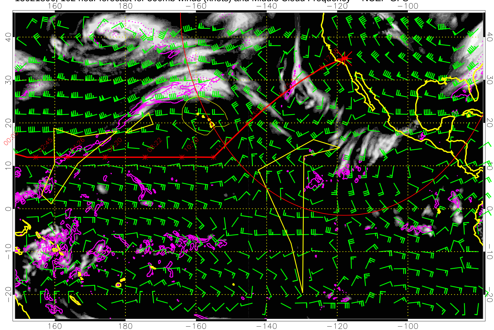
15021806, 102 hour forecast for 500mb winds (knots) and Middle Cloud Frequency -- NCEP GFS
