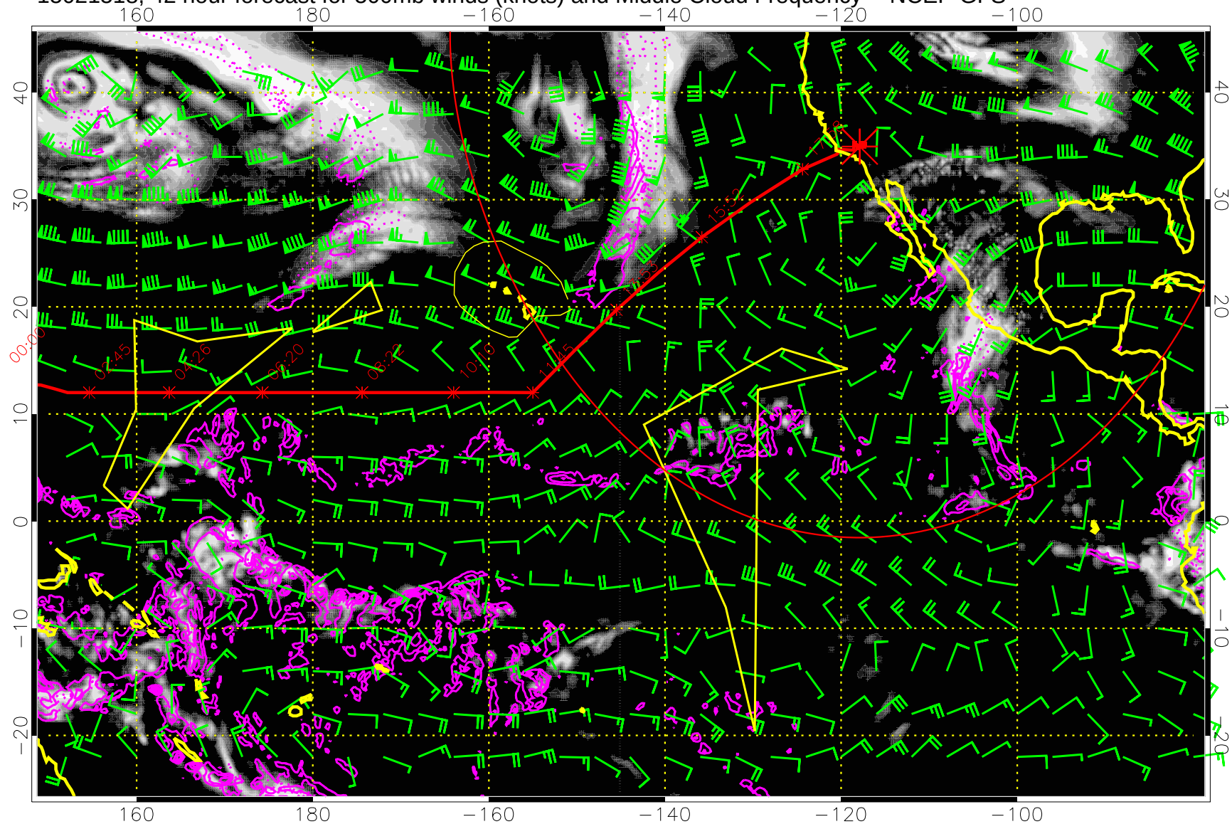
15021518, 42 hour forecast for 500mb winds (knots) and Middle Cloud Frequency -- NCEP GFS
