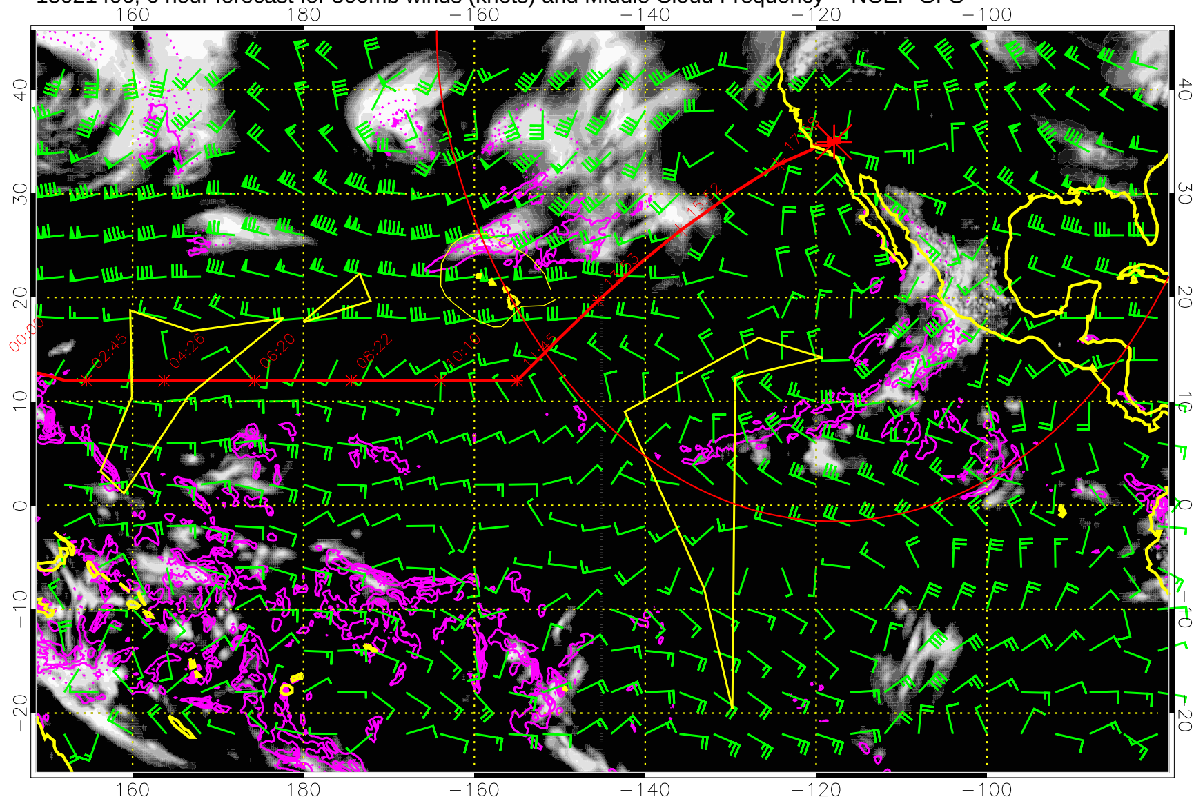
15021406, 6 hour forecast for 500mb winds (knots) and Middle Cloud Frequency -- NCEP GFS
