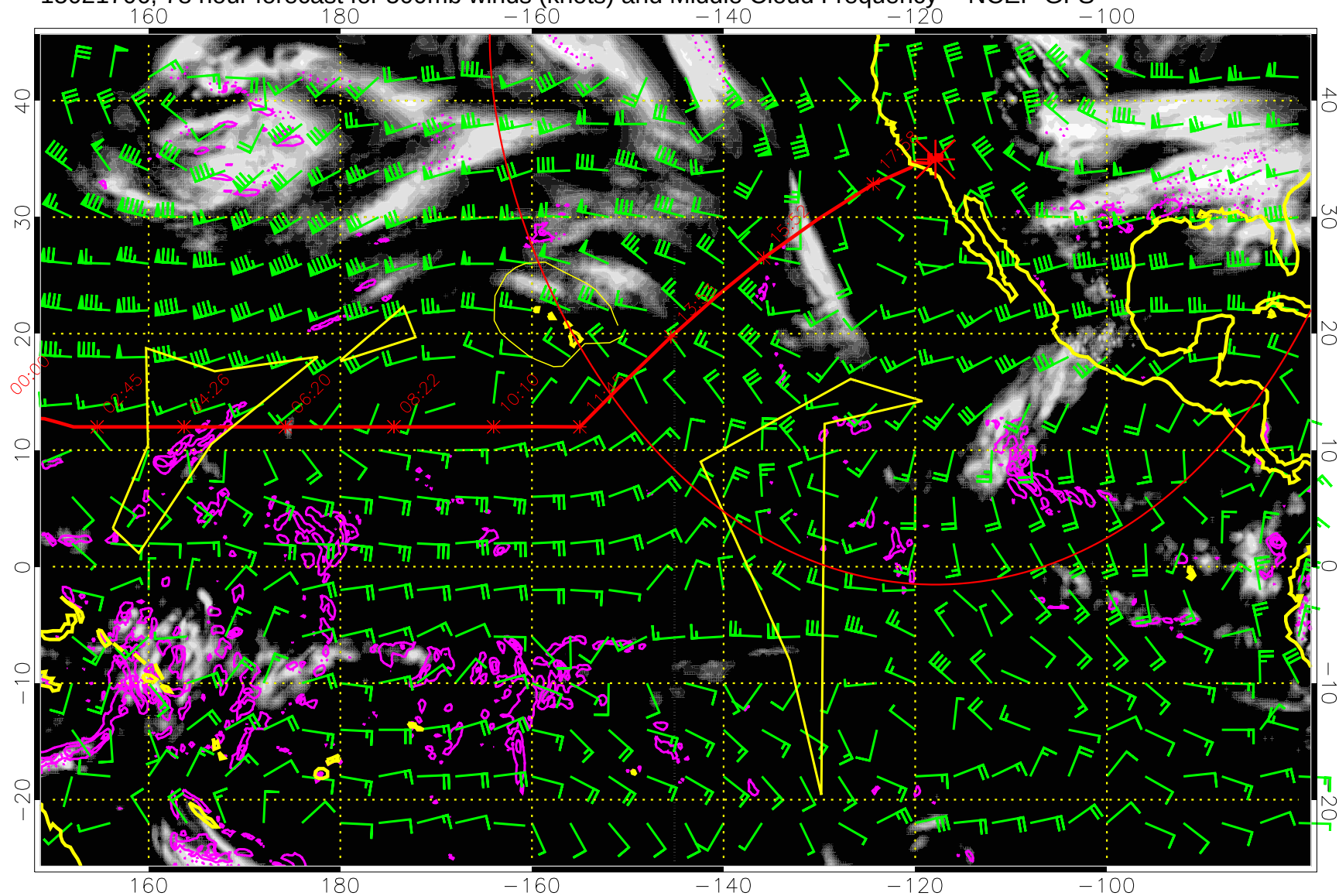
15021706, 78 hour forecast for 500mb winds (knots) and Middle Cloud Frequency -- NCEP GFS
