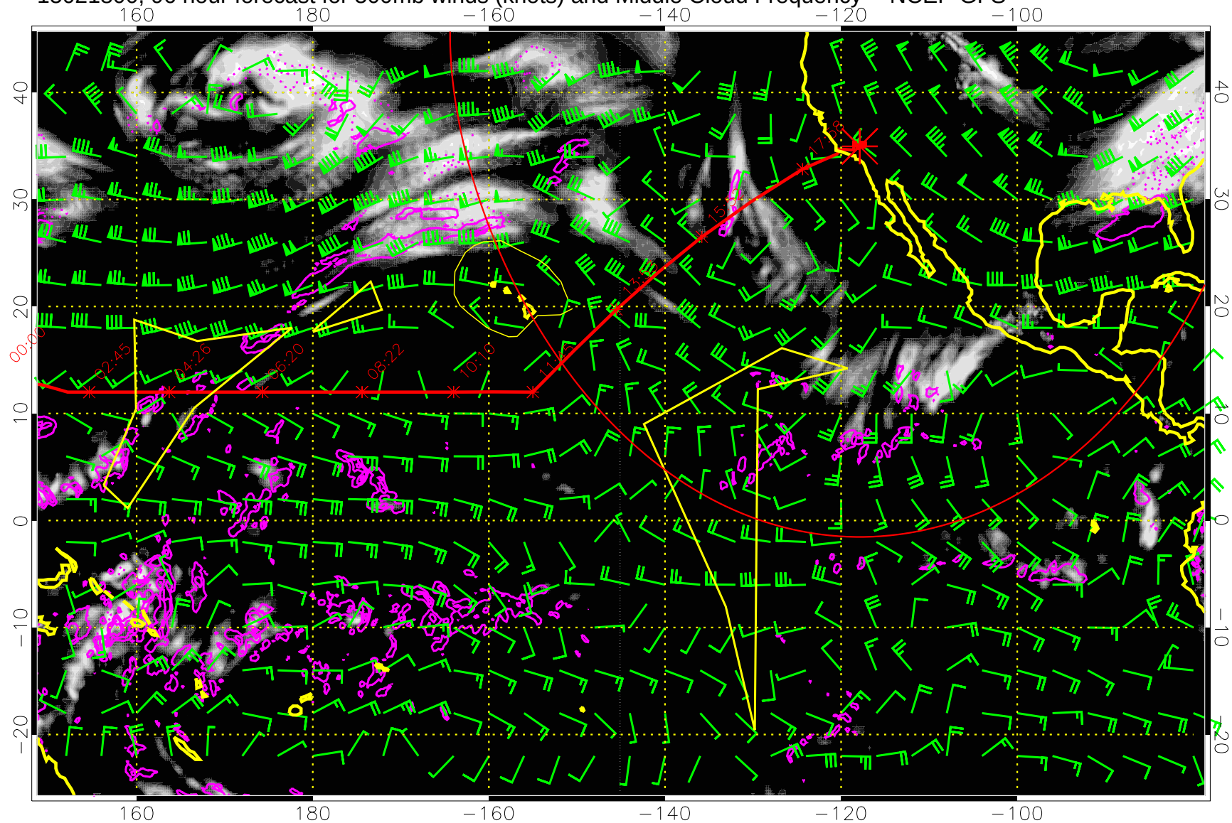
15021800, 96 hour forecast for 500mb winds (knots) and Middle Cloud Frequency -- NCEP GFS
