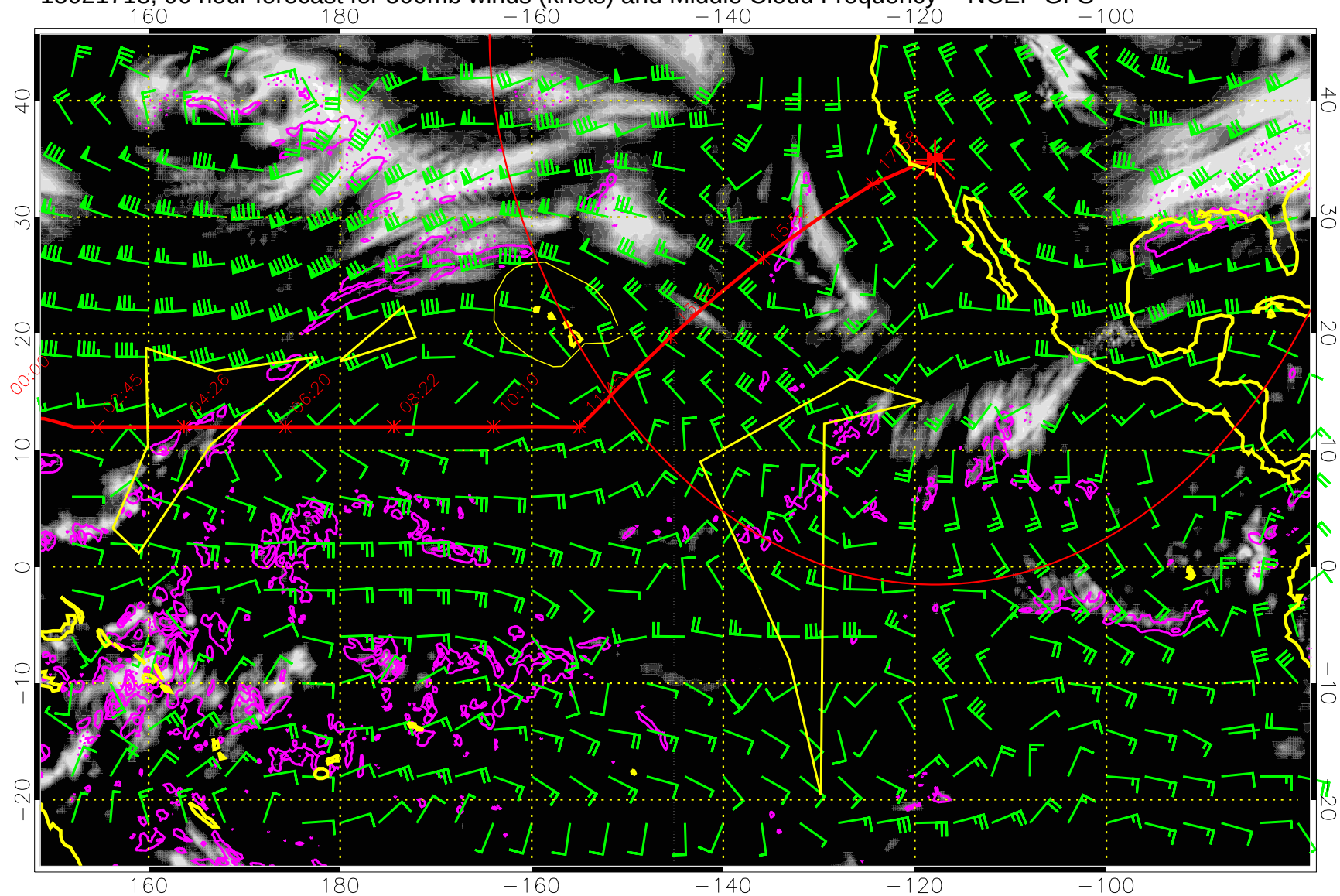
15021718, 90 hour forecast for 500mb winds (knots) and Middle Cloud Frequency -- NCEP GFS
