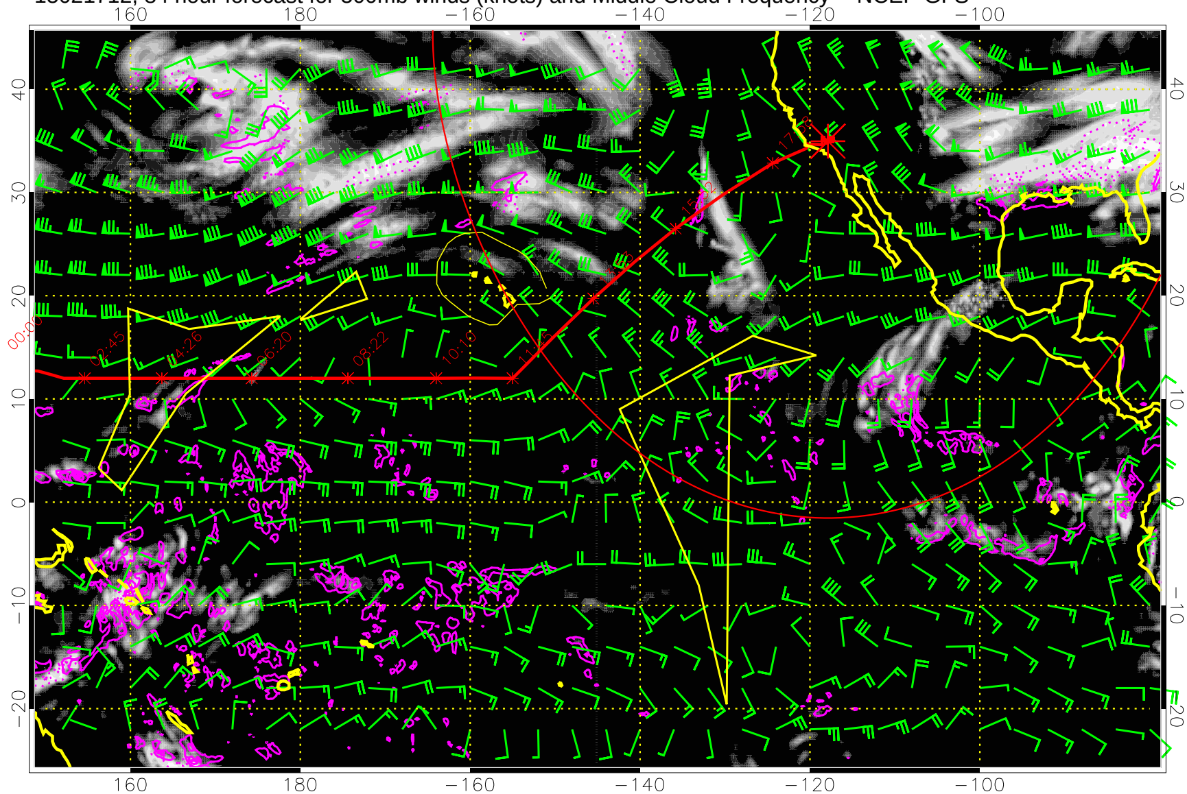
15021712, 84 hour forecast for 500mb winds (knots) and Middle Cloud Frequency -- NCEP GFS
