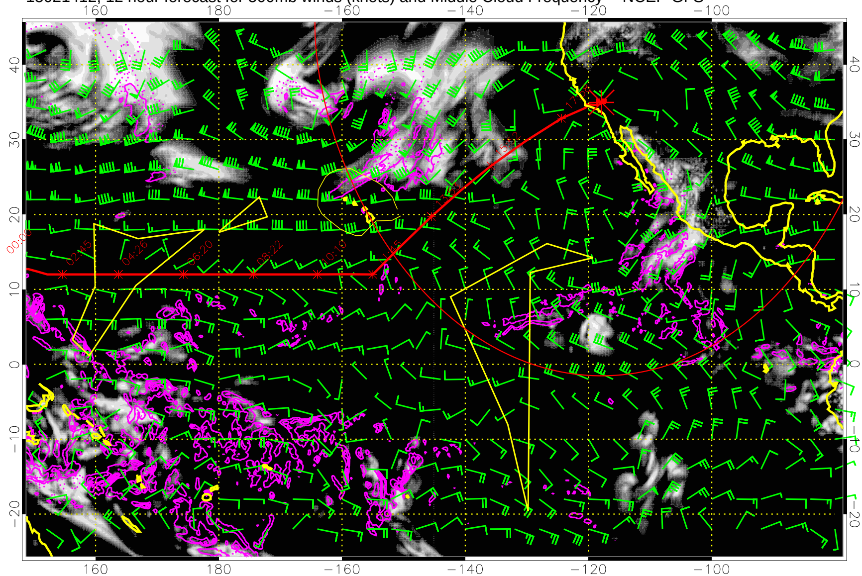
15021412, 12 hour forecast for 500mb winds (knots) and Middle Cloud Frequency -- NCEP GFS
