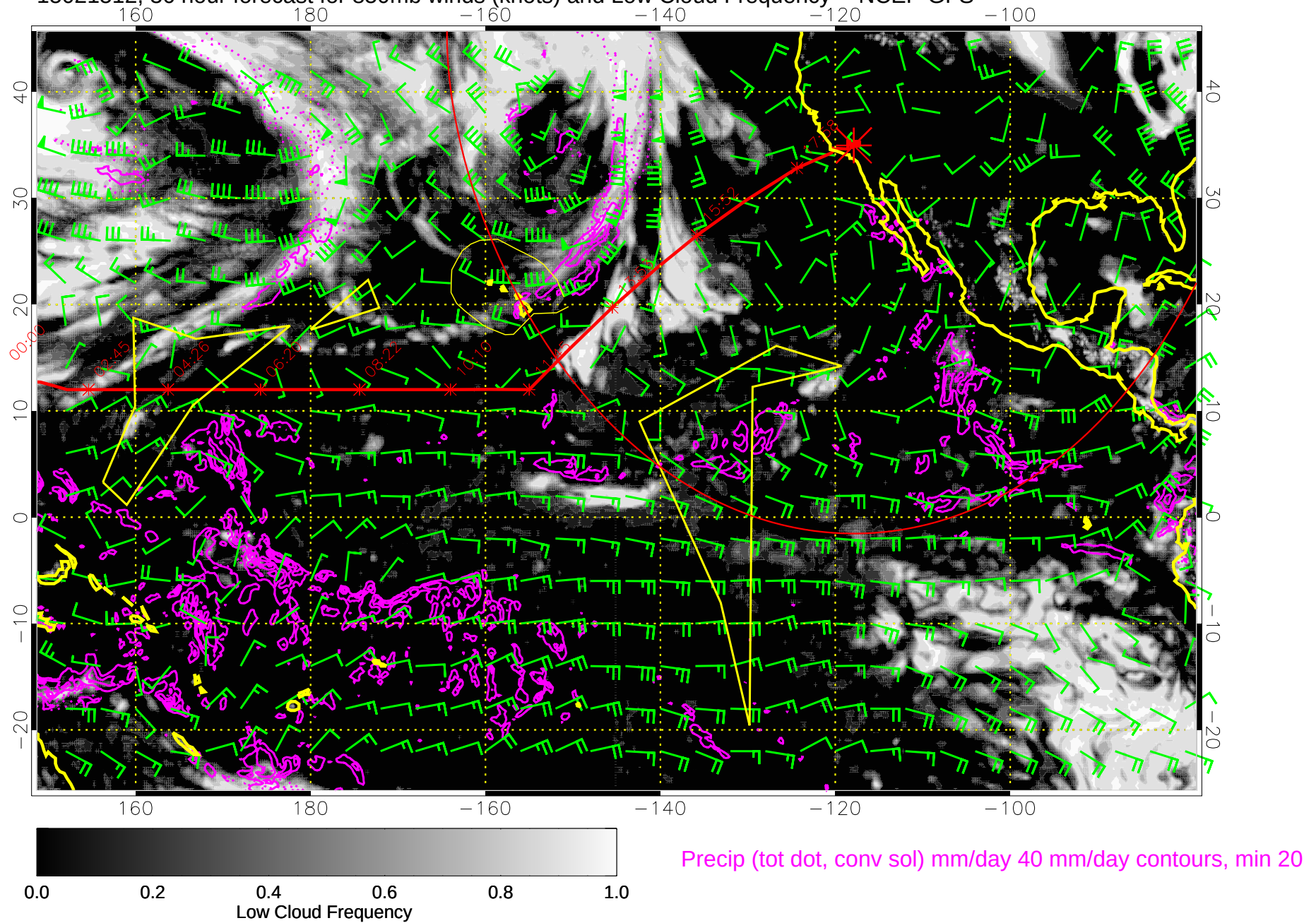
15021512, 36 hour forecast for 850mb winds (knots) and Low Cloud Frequency -- NCEP GFS
