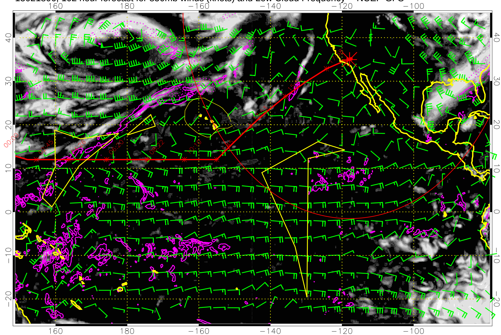
15021806, 102 hour forecast for 850mb winds (knots) and Low Cloud Frequency -- NCEP GFS
