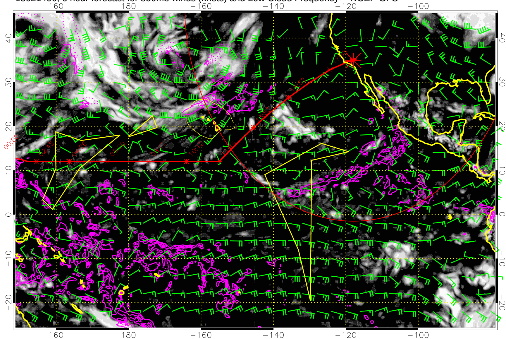
15021406, 6 hour forecast for 850mb winds (knots) and Low Cloud Frequency -- NCEP GFS
