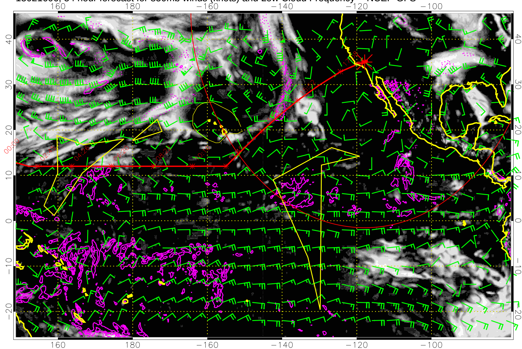
15021606, 54 hour forecast for 850mb winds (knots) and Low Cloud Frequency -- NCEP GFS
