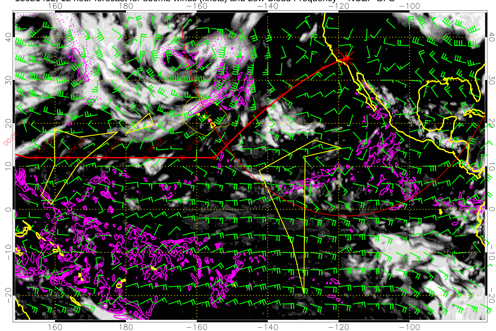
15021412, 12 hour forecast for 850mb winds (knots) and Low Cloud Frequency -- NCEP GFS
