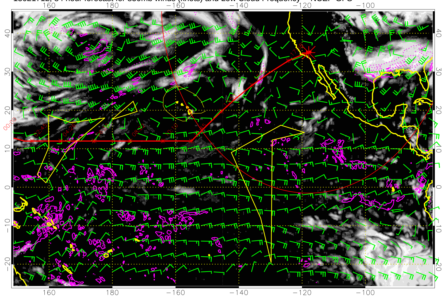
15021712, 84 hour forecast for 850mb winds (knots) and Low Cloud Frequency -- NCEP GFS
