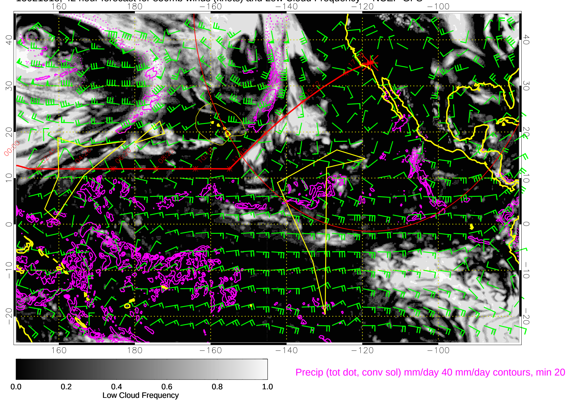
15021518, 42 hour forecast for 850mb winds (knots) and Low Cloud Frequency -- NCEP GFS
