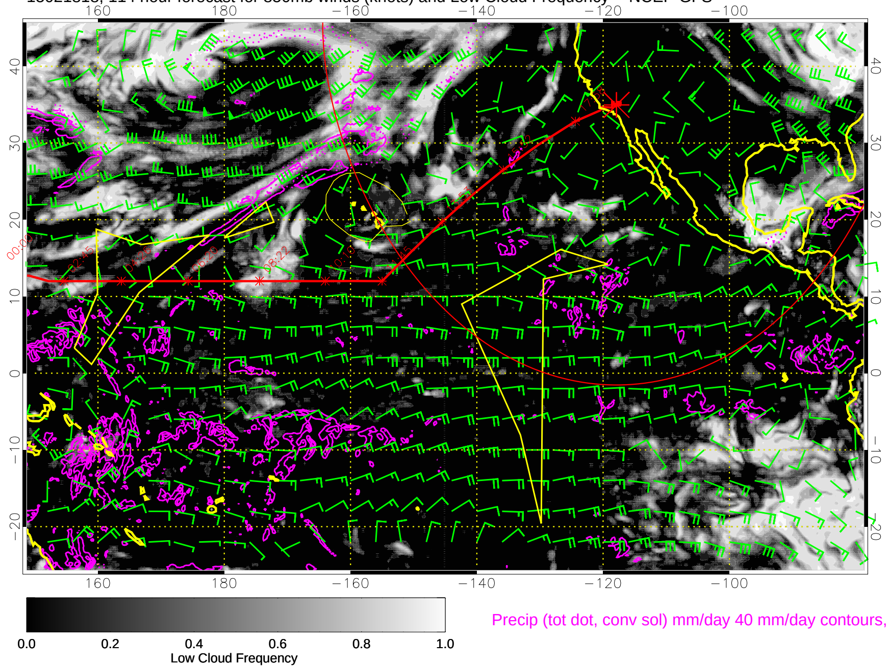
15021818, 114 hour forecast for 850mb winds (knots) and Low Cloud Frequency -- NCEP GFS
