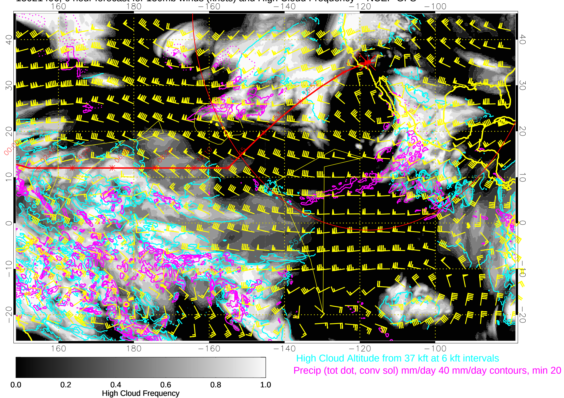
15021406, 6 hour forecast for 150mb winds (knots) and High Cloud Frequency -- NCEP GFS
