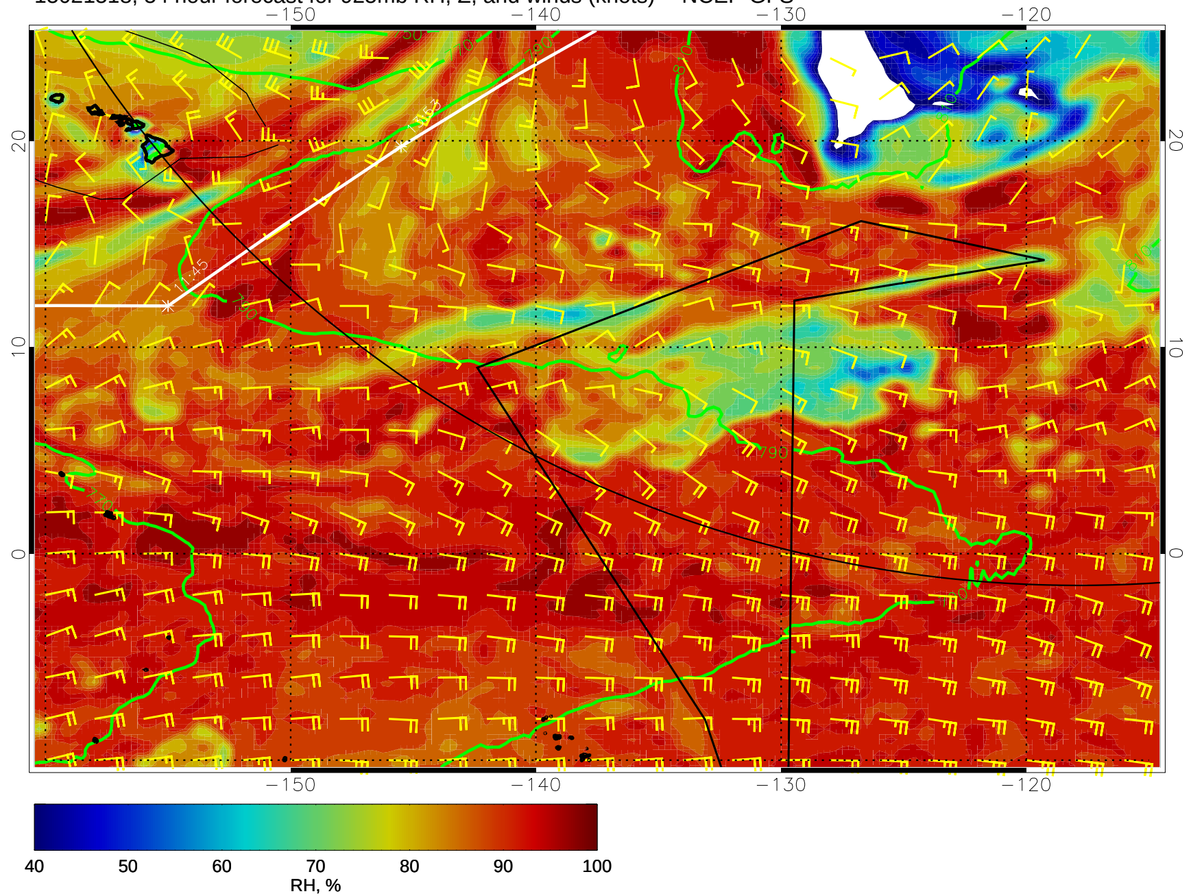
15021518, 54 hour forecast for 925mb RH, Z, and winds (knots) -- NCEP GFS
