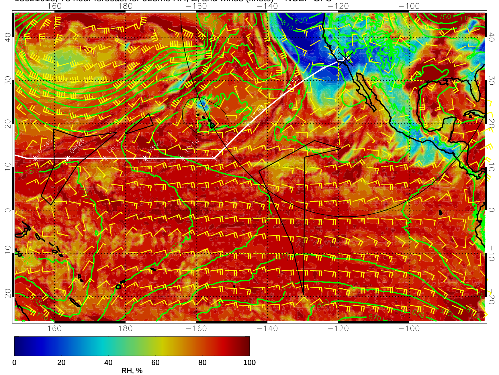
15021618, 78 hour forecast for 925mb RH, Z, and winds (knots) -- NCEP GFS
