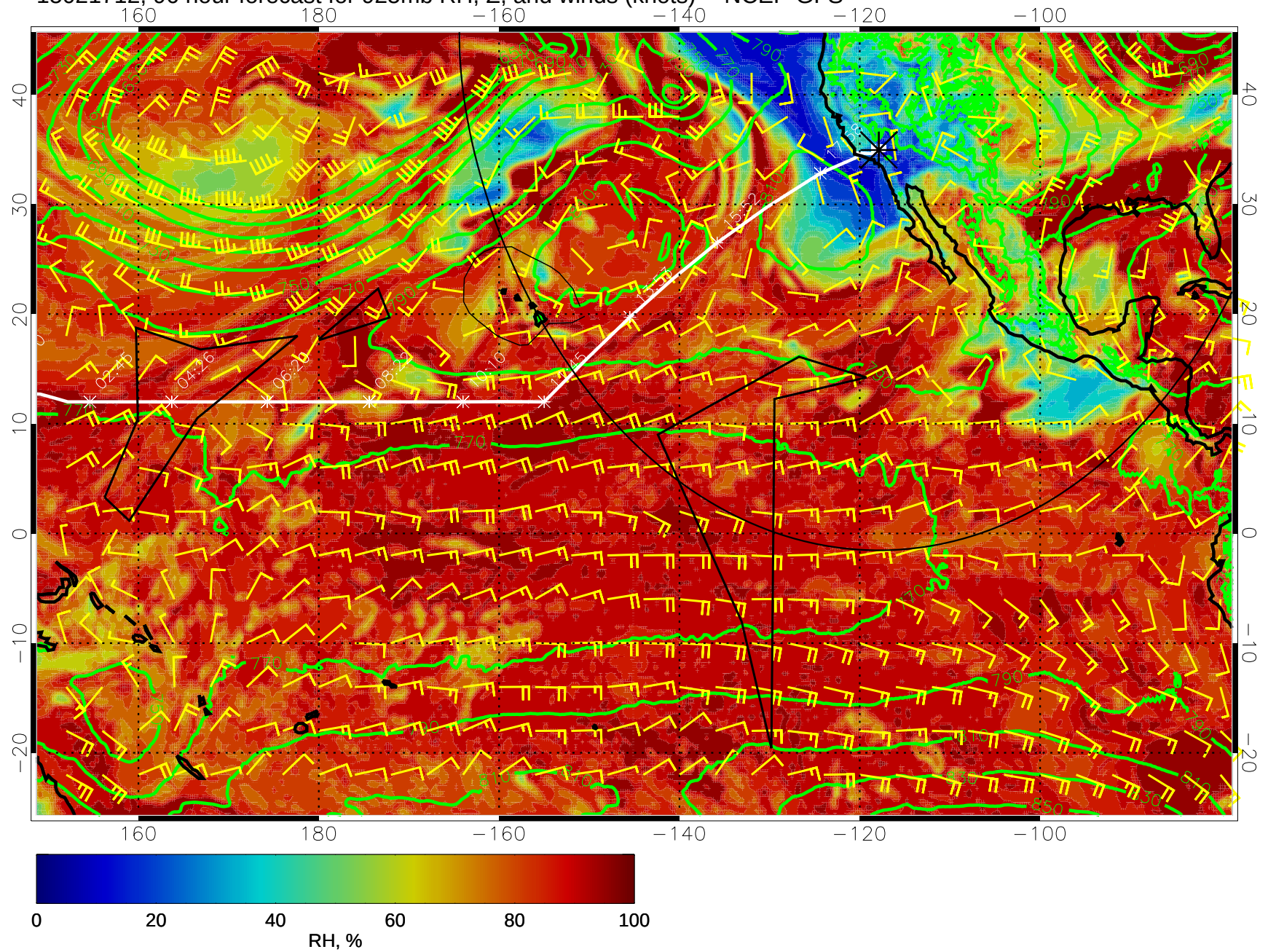
15021712, 96 hour forecast for 925mb RH, Z, and winds (knots) -- NCEP GFS
