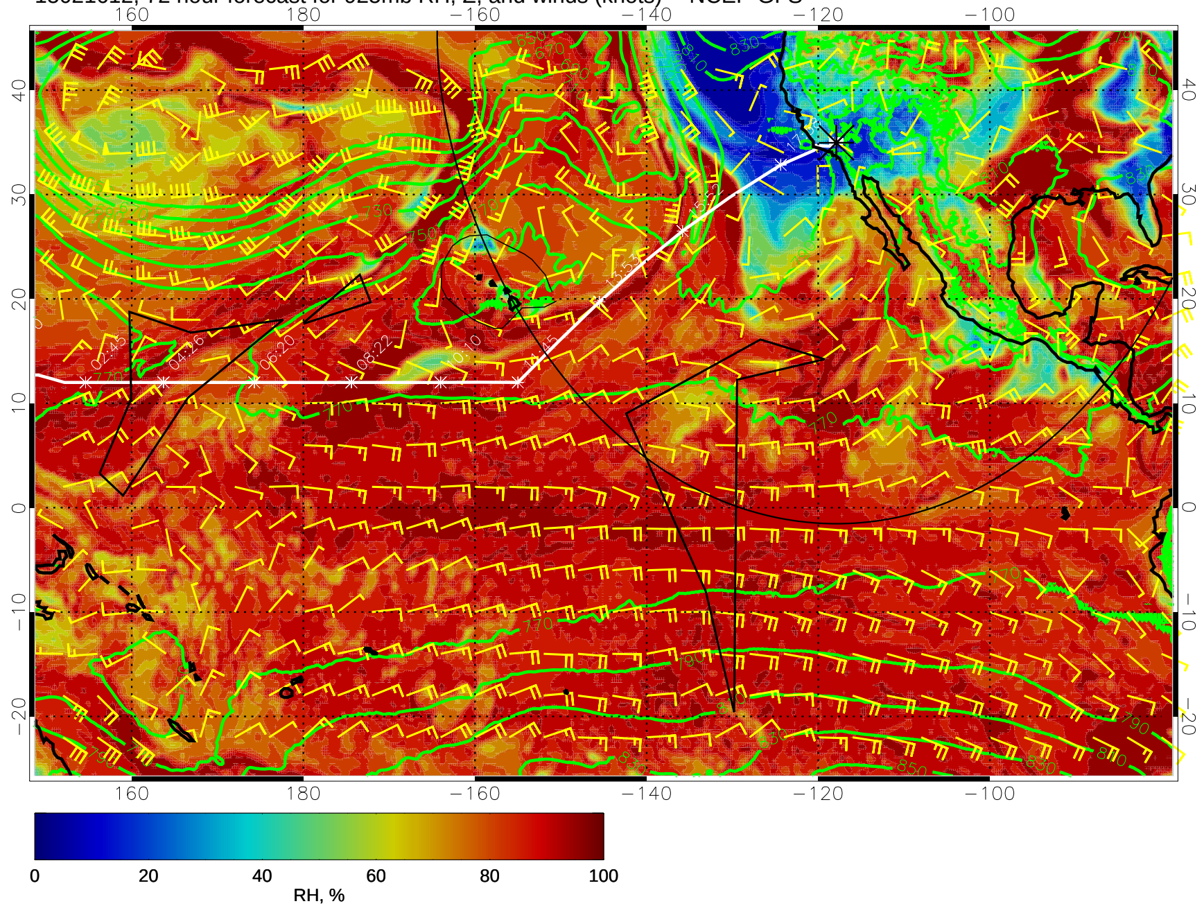
15021612, 72 hour forecast for 925mb RH, Z, and winds (knots) -- NCEP GFS
