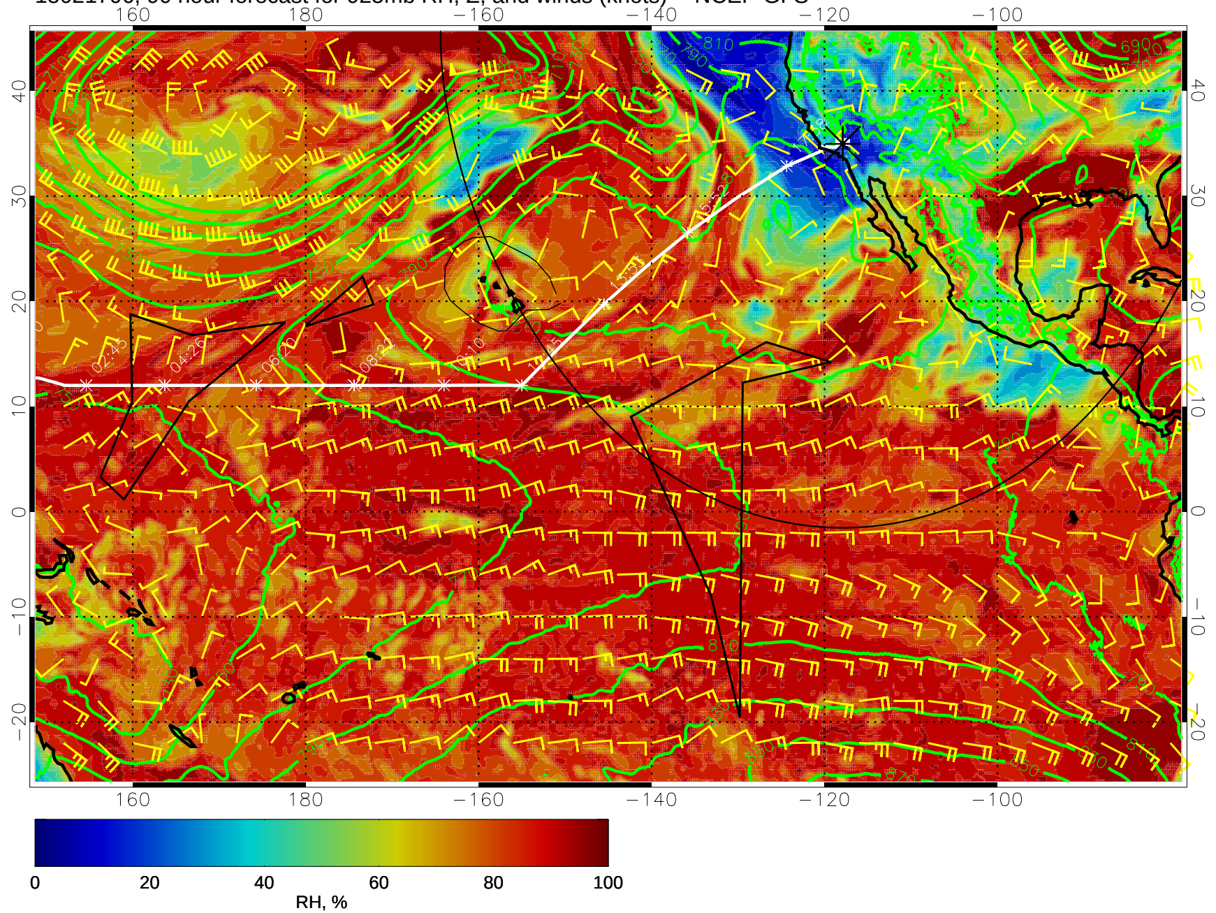
15021706, 90 hour forecast for 925mb RH, Z, and winds (knots) -- NCEP GFS
