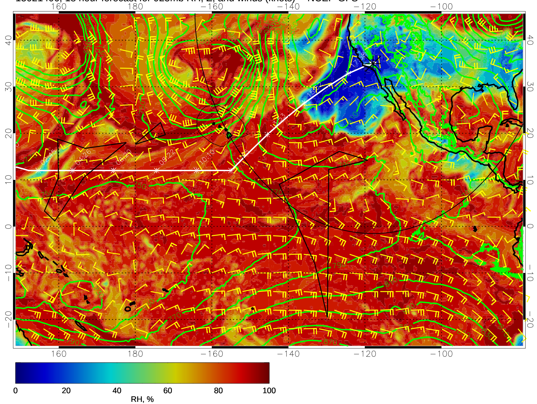
15021406, 18 hour forecast for 925mb RH, Z, and winds (knots) -- NCEP GFS
