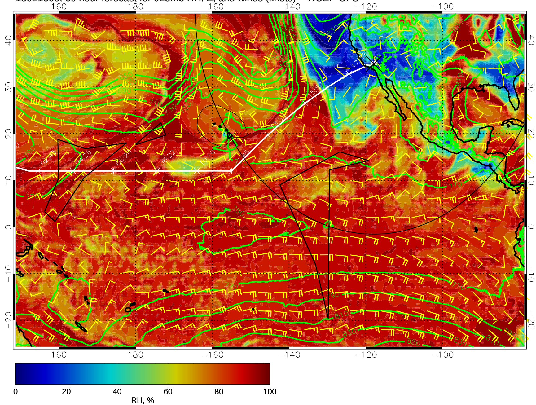
15021600, 60 hour forecast for 925mb RH, Z, and winds (knots) -- NCEP GFS
