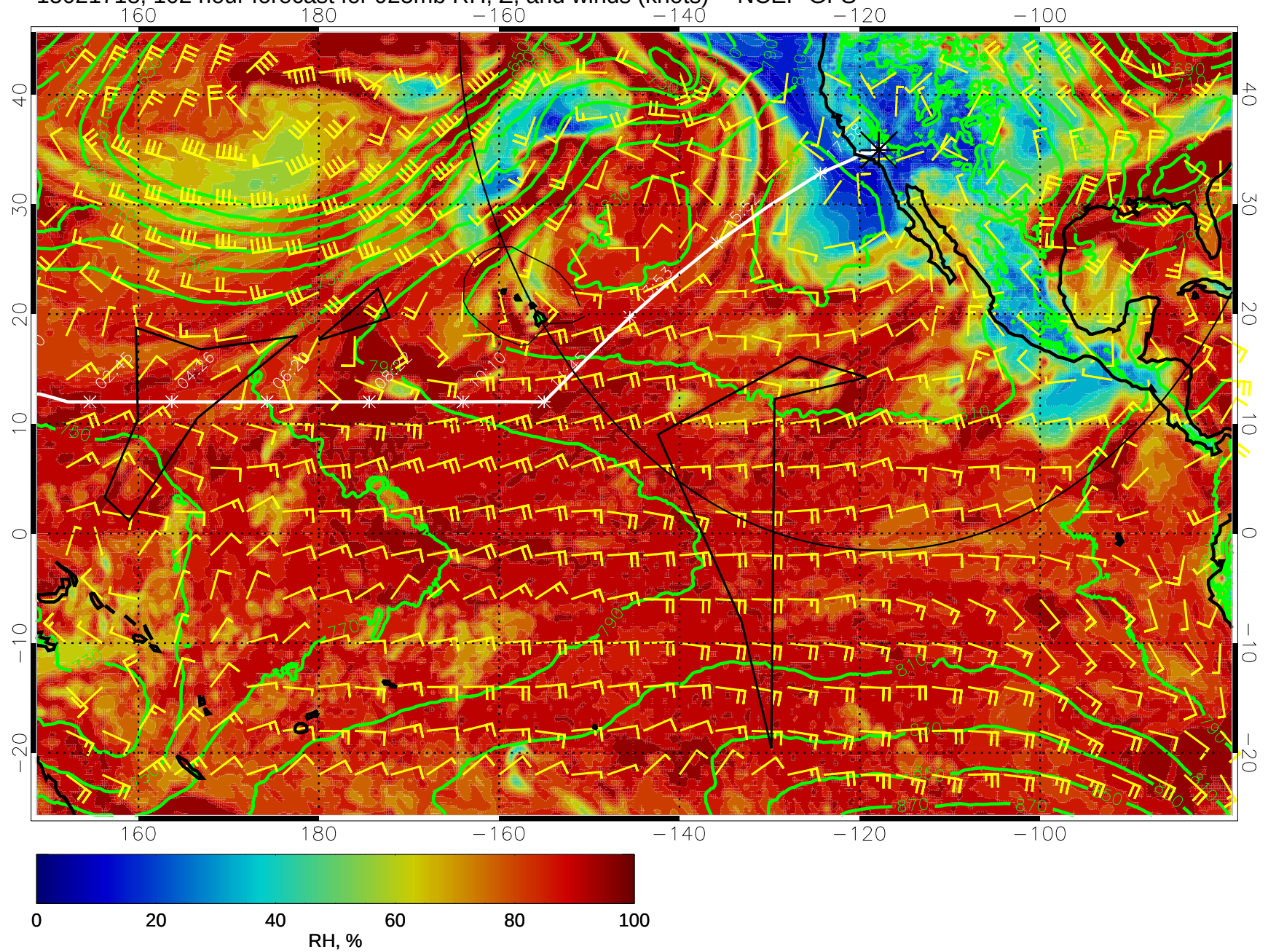
15021718, 102 hour forecast for 925mb RH, Z, and winds (knots) -- NCEP GFS
