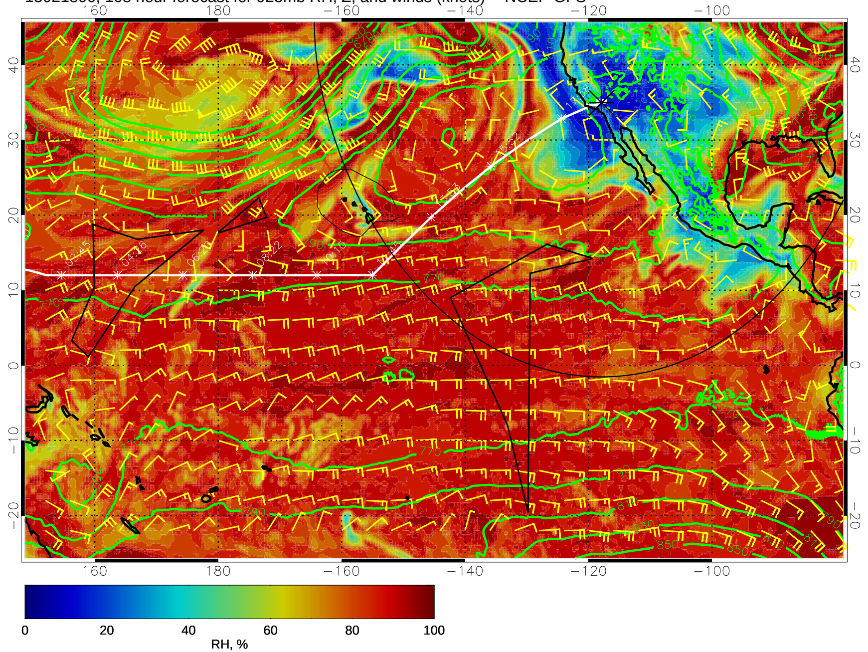
15021800, 108 hour forecast for 925mb RH, Z, and winds (knots) -- NCEP GFS
