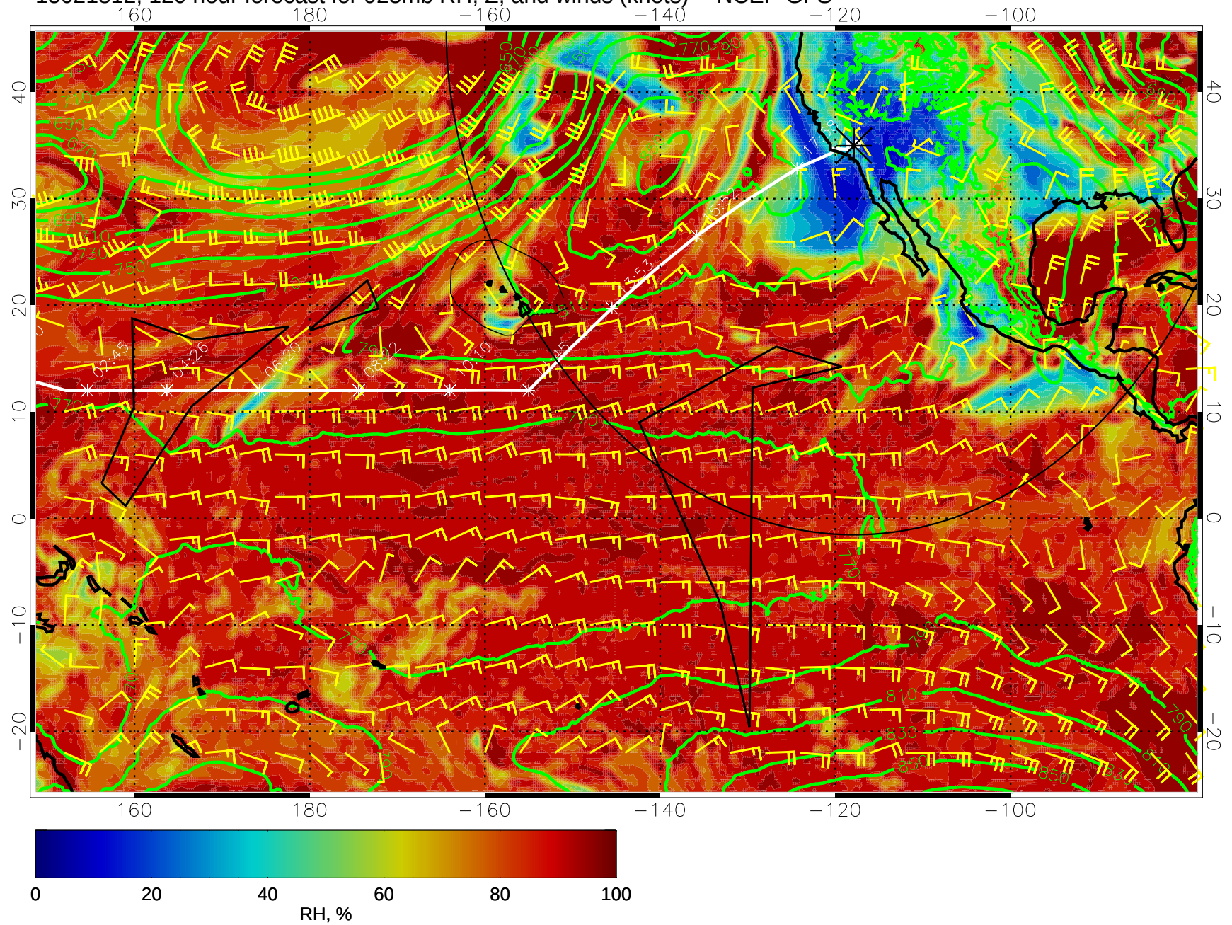
15021812, 120 hour forecast for 925mb RH, Z, and winds (knots) -- NCEP GFS
