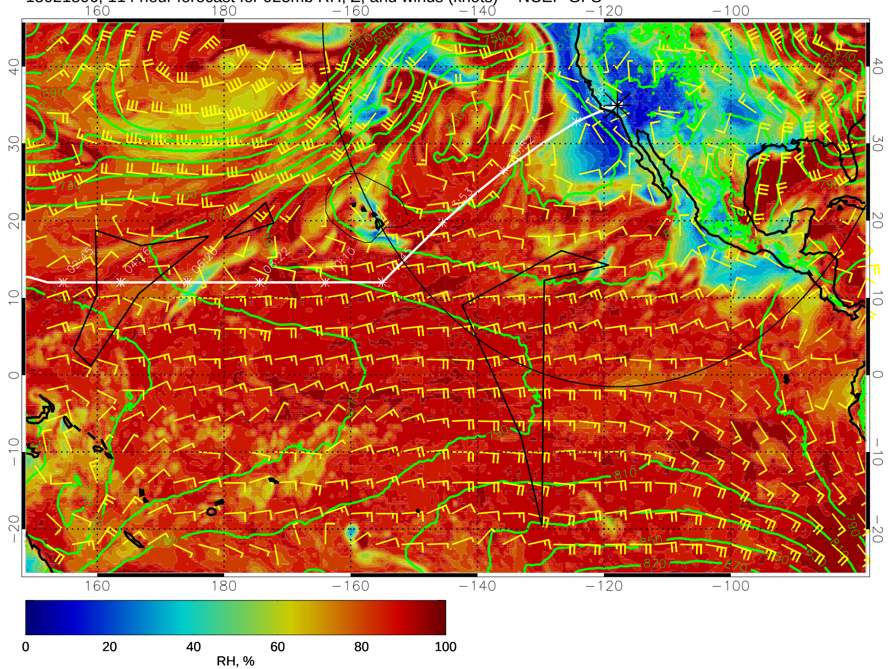
15021806, 114 hour forecast for 925mb RH, Z, and winds (knots) -- NCEP GFS
