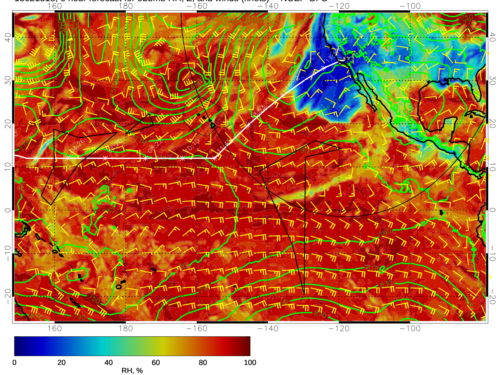
15021318, 6 hour forecast for 925mb RH, Z, and winds (knots) -- NCEP GFS
