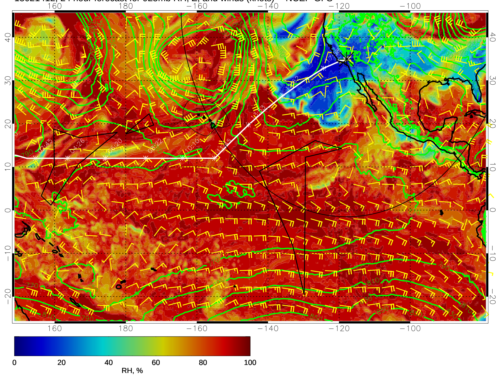
15021412, 24 hour forecast for 925mb RH, Z, and winds (knots) -- NCEP GFS
