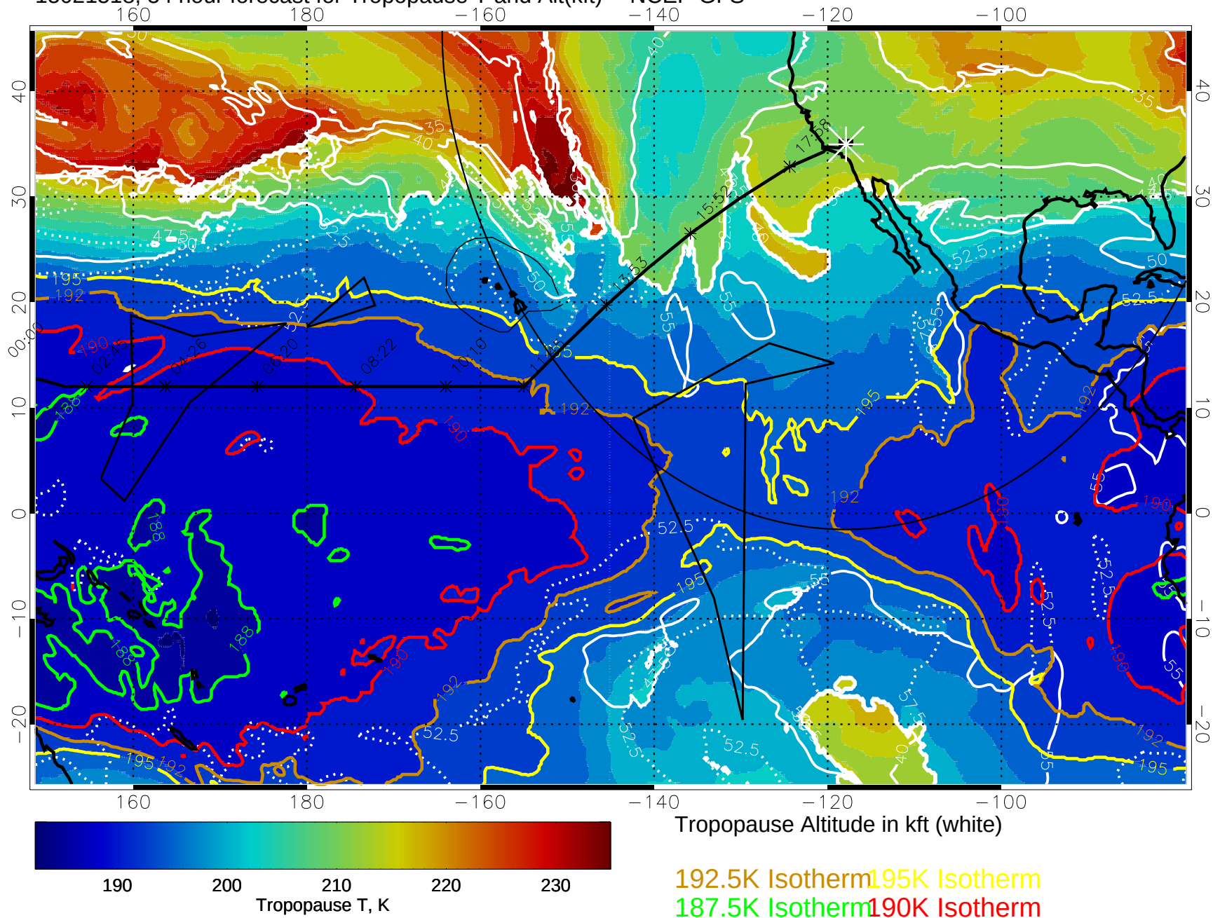
15021518, 54 hour forecast for Tropopause T and Alt(kft) -- NCEP GFS
