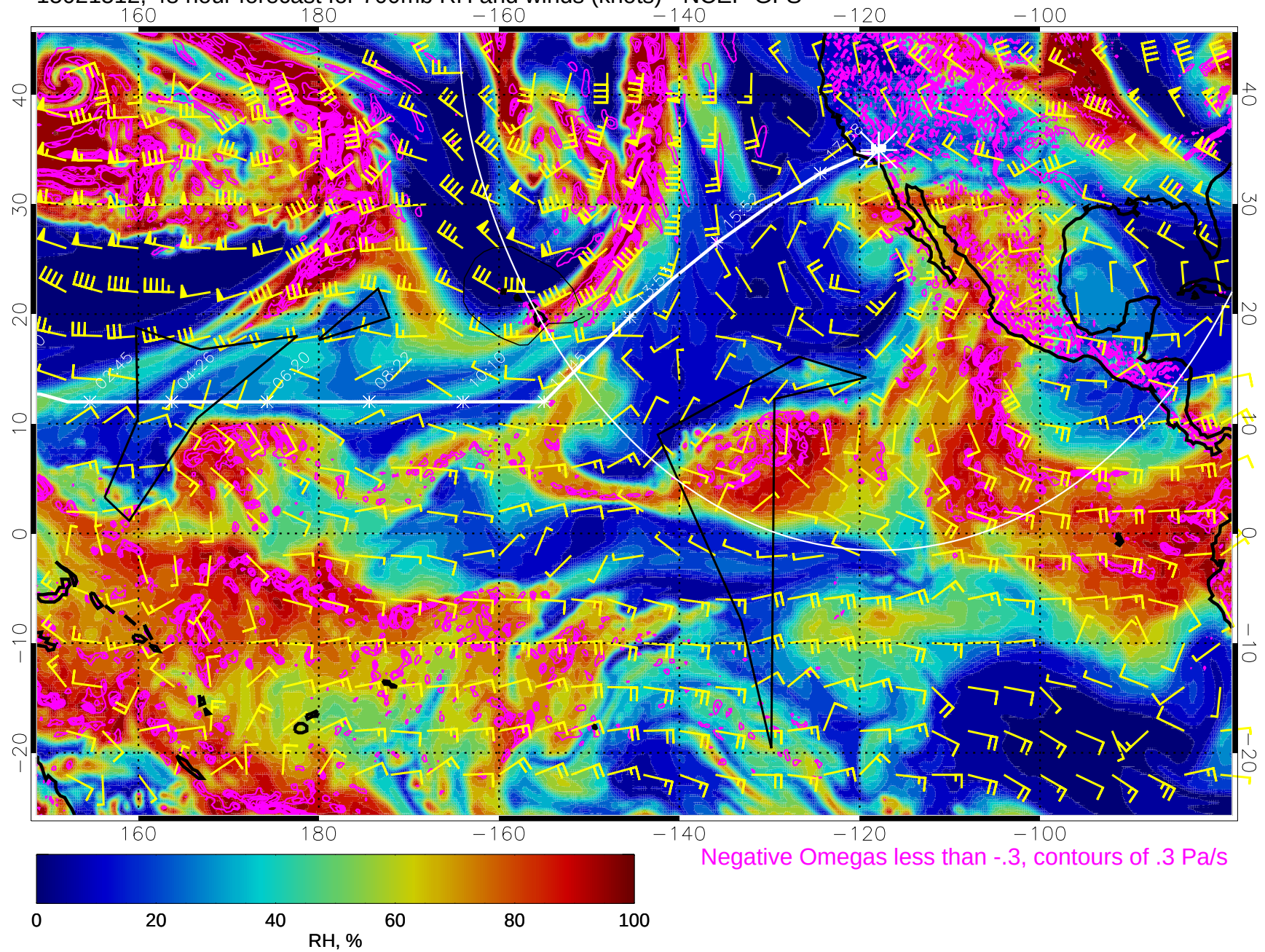
15021512, 48 hour forecast for 700mb RH and winds (knots) - NCEP GFS
