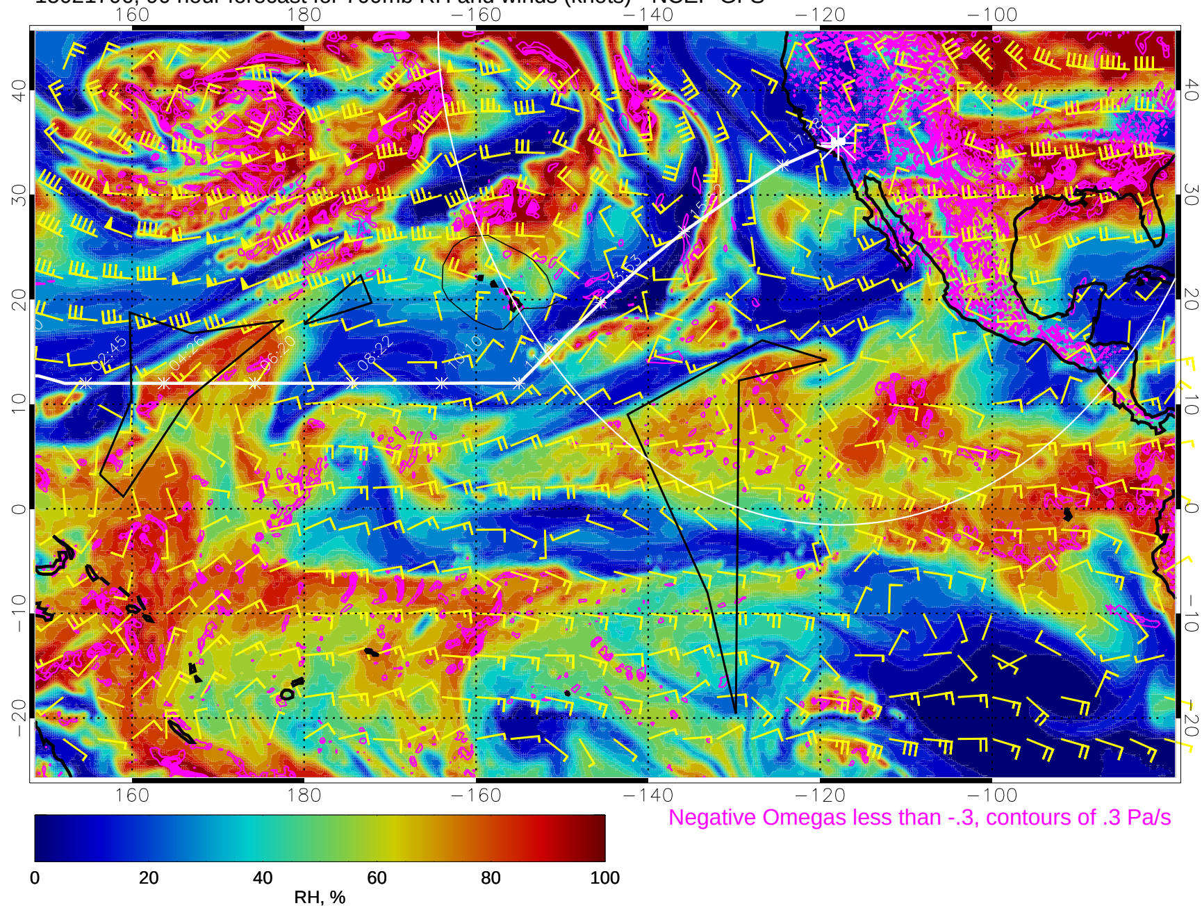
15021706, 90 hour forecast for 700mb RH and winds (knots) - NCEP GFS
