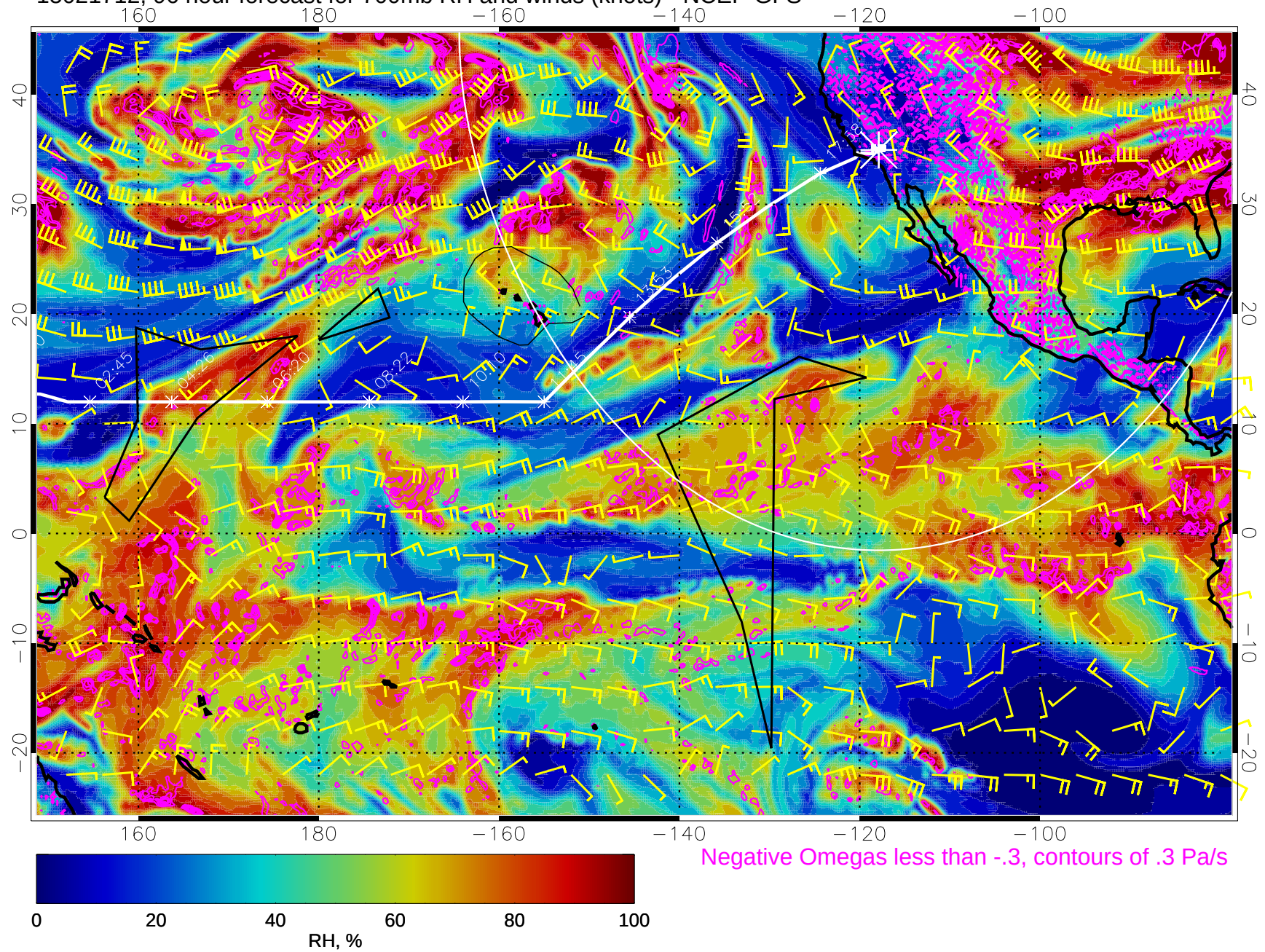
15021712, 96 hour forecast for 700mb RH and winds (knots) - NCEP GFS
