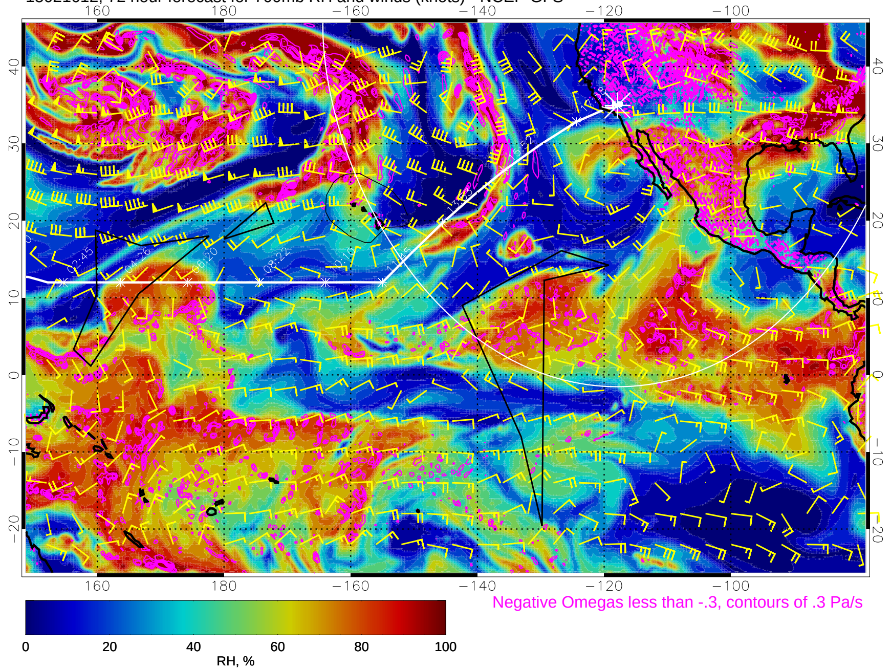
15021612, 72 hour forecast for 700mb RH and winds (knots) - NCEP GFS
