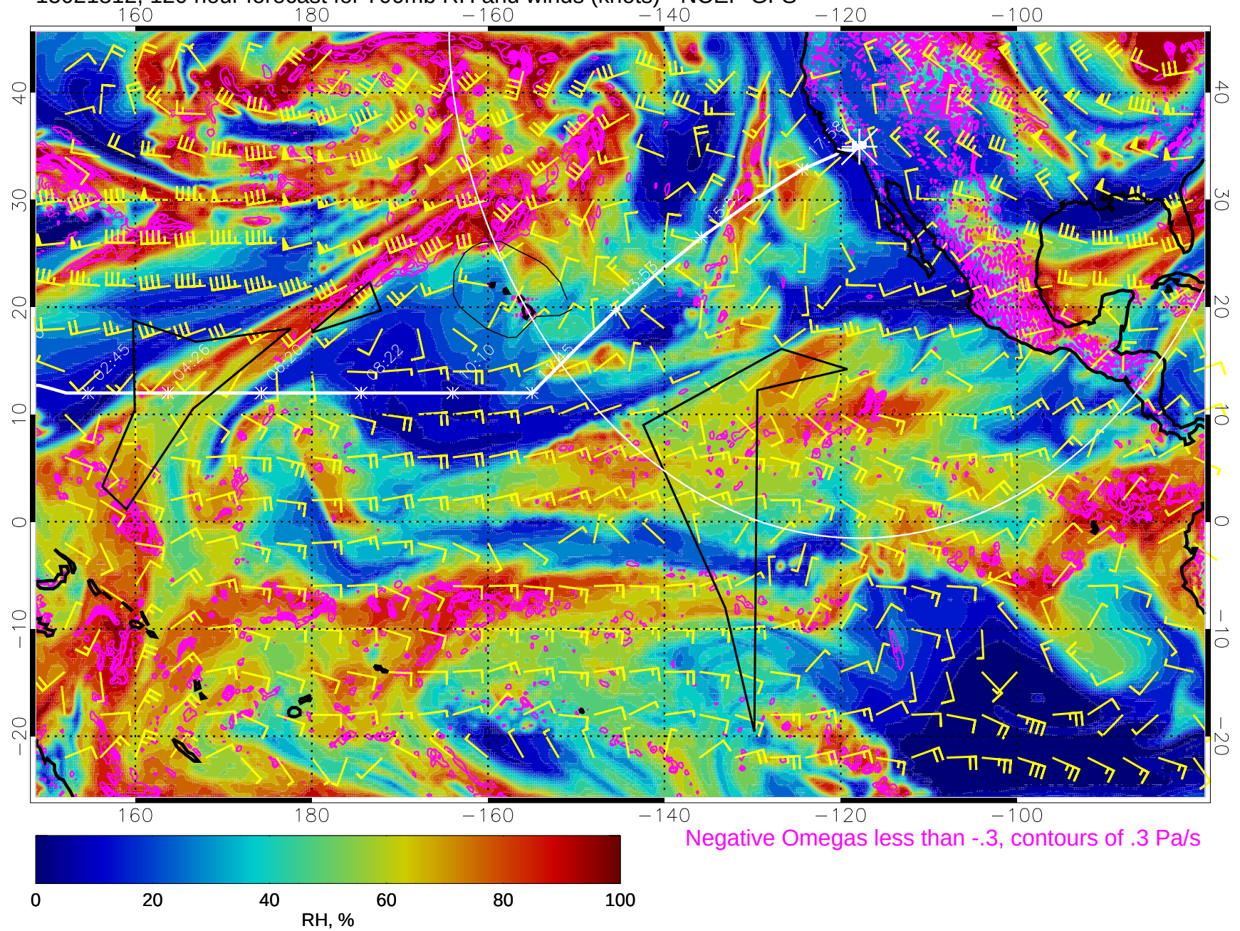
15021812, 120 hour forecast for 700mb RH and winds (knots) - NCEP GFS
