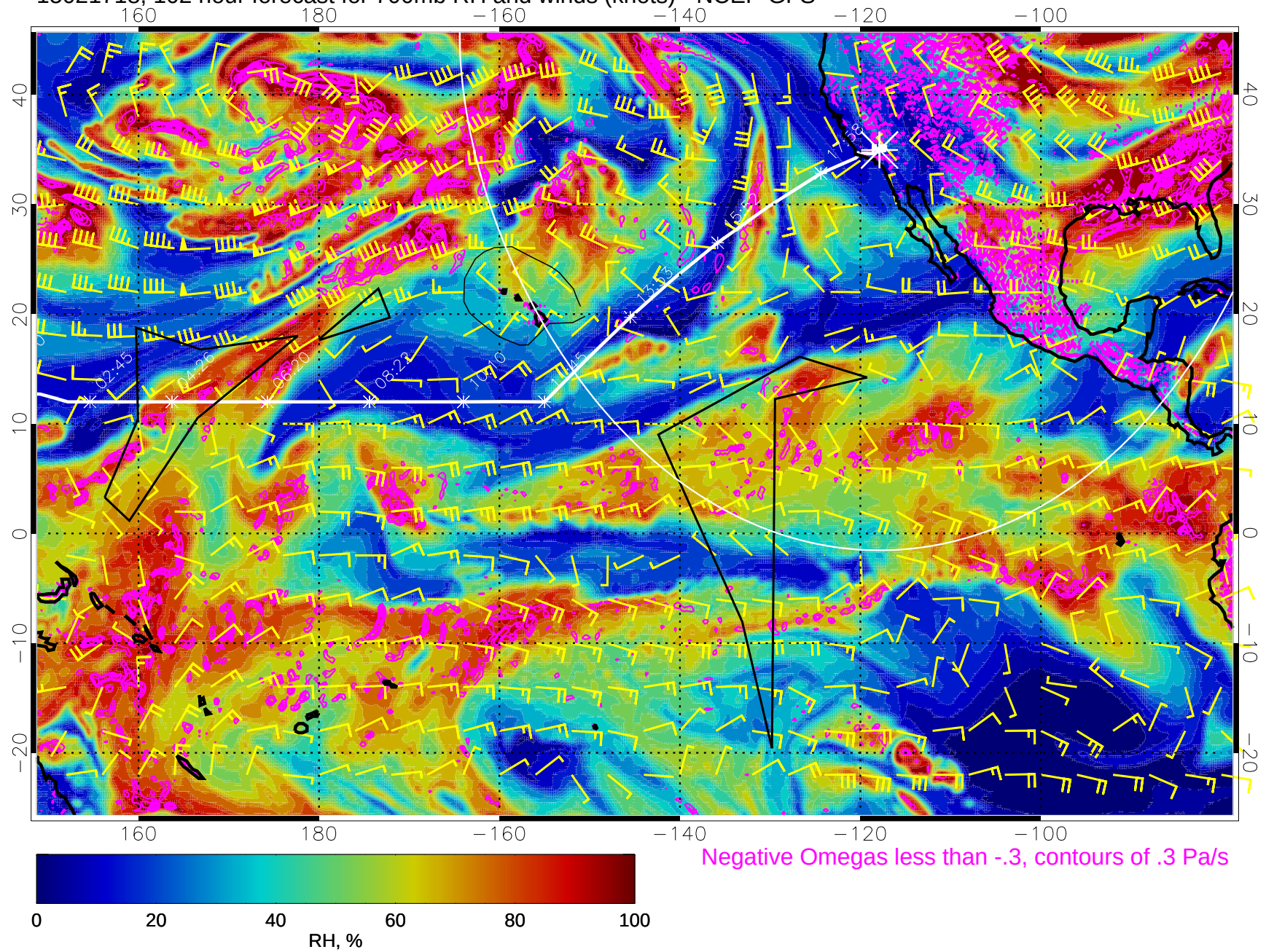
15021718, 102 hour forecast for 700mb RH and winds (knots) - NCEP GFS
