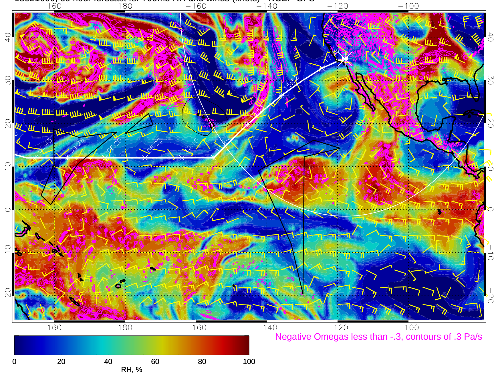
15021600, 60 hour forecast for 700mb RH and winds (knots) - NCEP GFS
