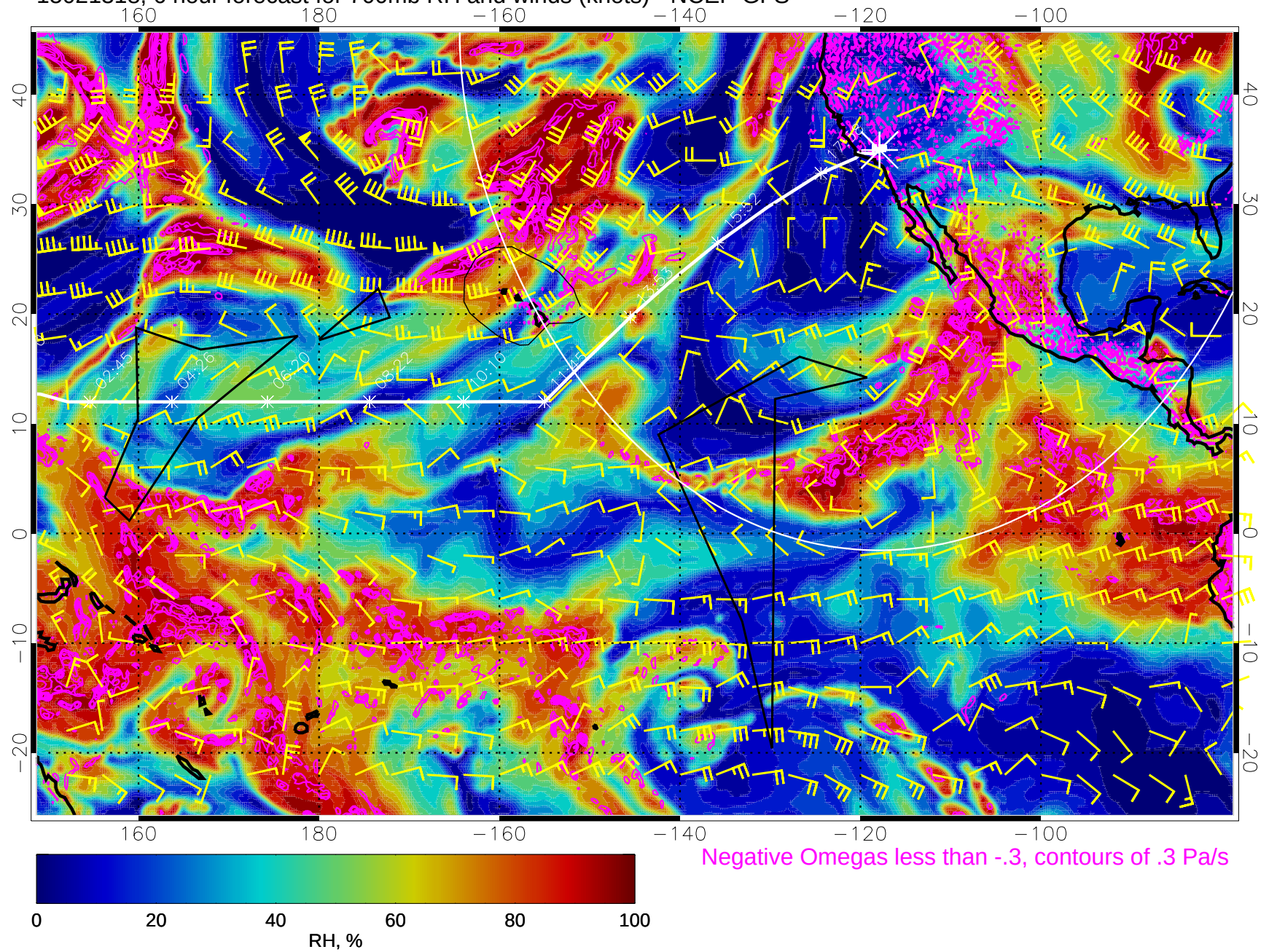
15021318, 6 hour forecast for 700mb RH and winds (knots) - NCEP GFS
