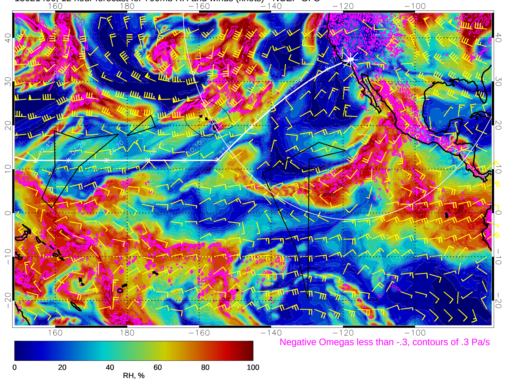
15021400, 12 hour forecast for 700mb RH and winds (knots) - NCEP GFS
