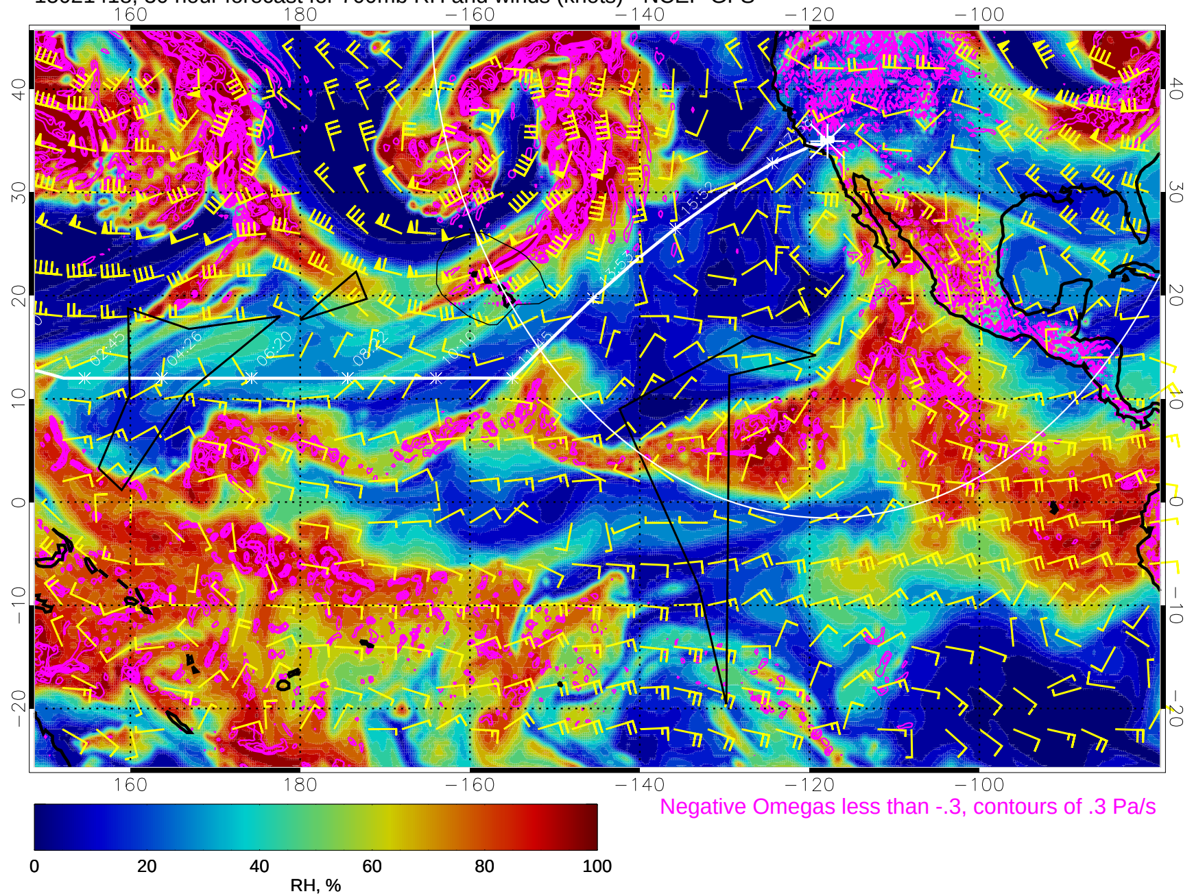
15021418, 30 hour forecast for 700mb RH and winds (knots) - NCEP GFS
