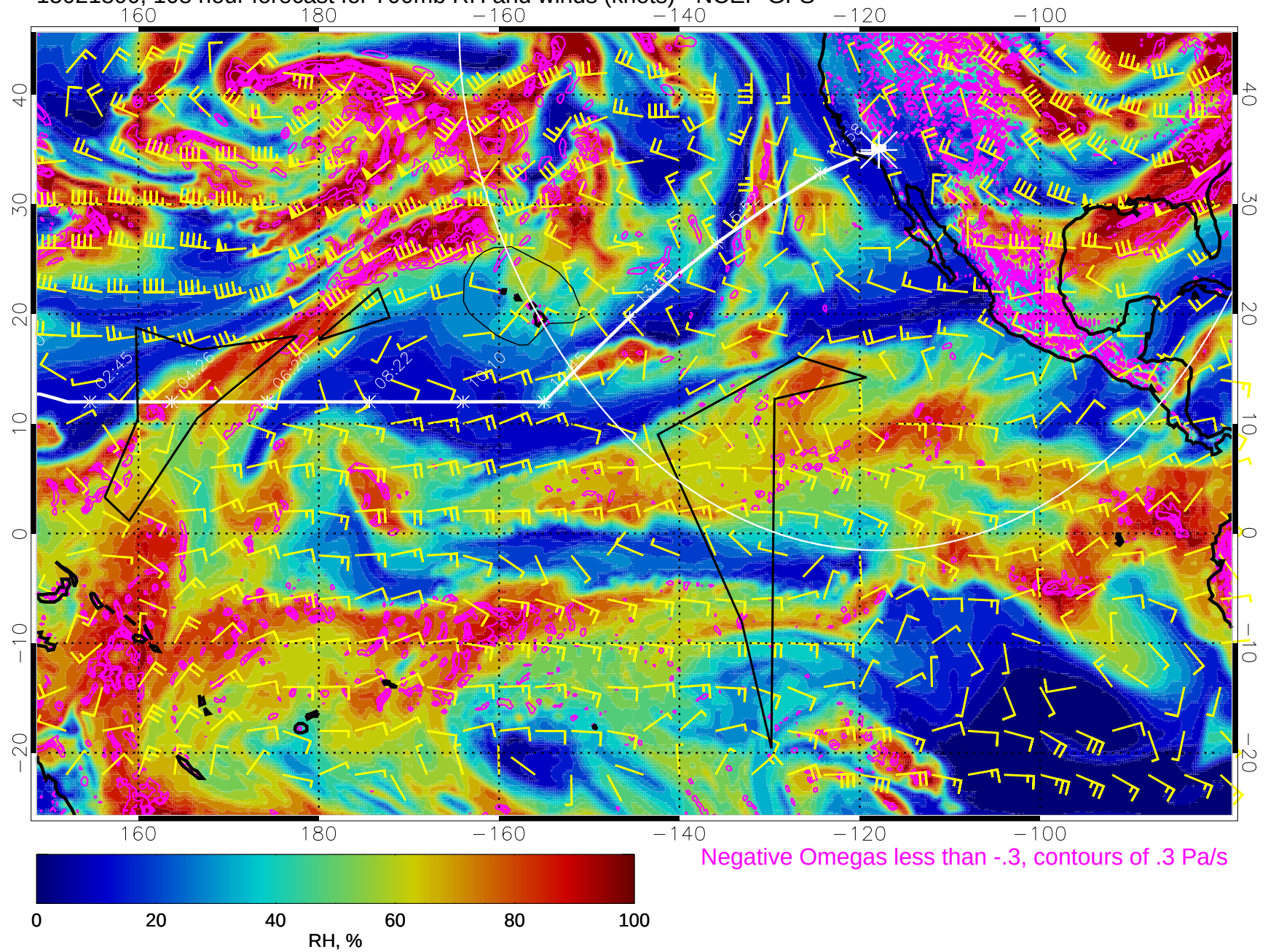
15021800, 108 hour forecast for 700mb RH and winds (knots) - NCEP GFS
