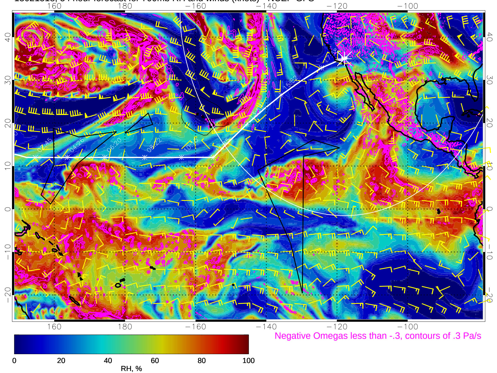
15021518, 54 hour forecast for 700mb RH and winds (knots) - NCEP GFS
