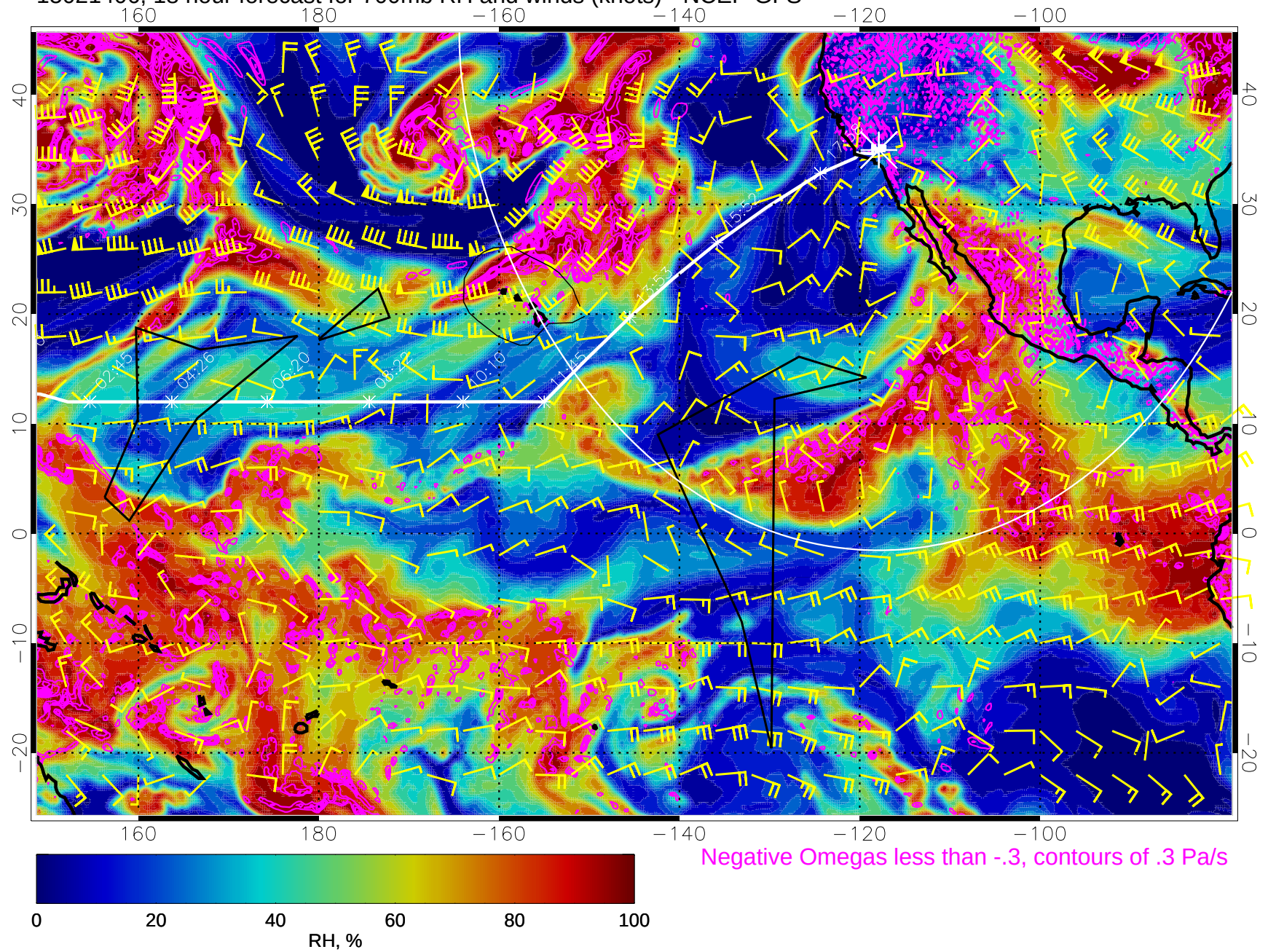
15021406, 18 hour forecast for 700mb RH and winds (knots) - NCEP GFS
