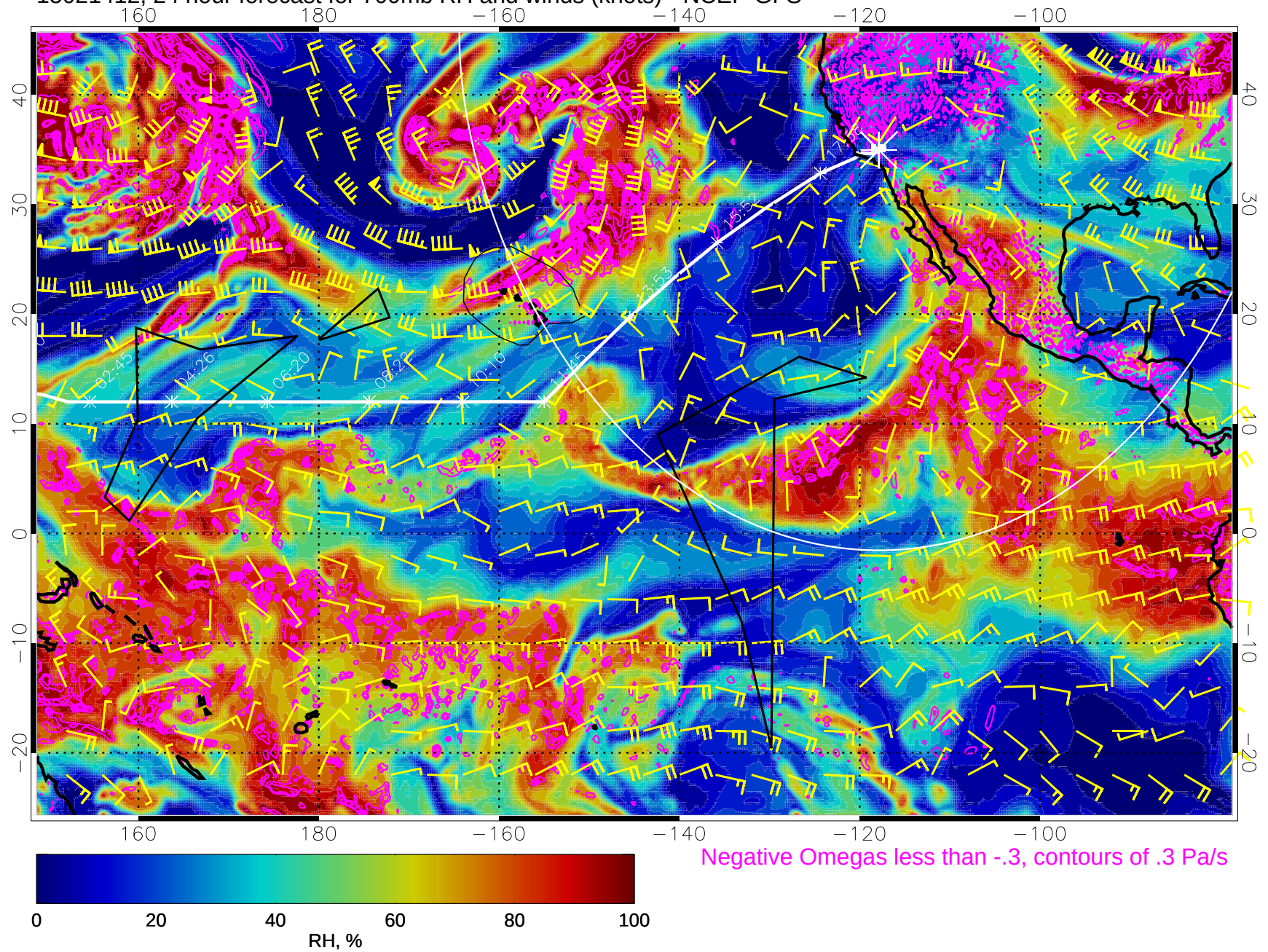
15021412, 24 hour forecast for 700mb RH and winds (knots) - NCEP GFS
