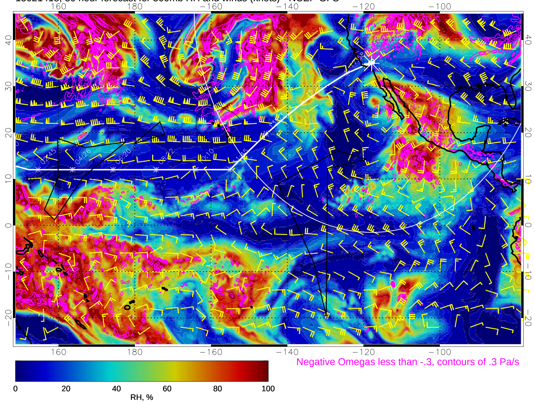
15021418, 30 hour forecast for 500mb RH and winds (knots) - NCEP GFS
