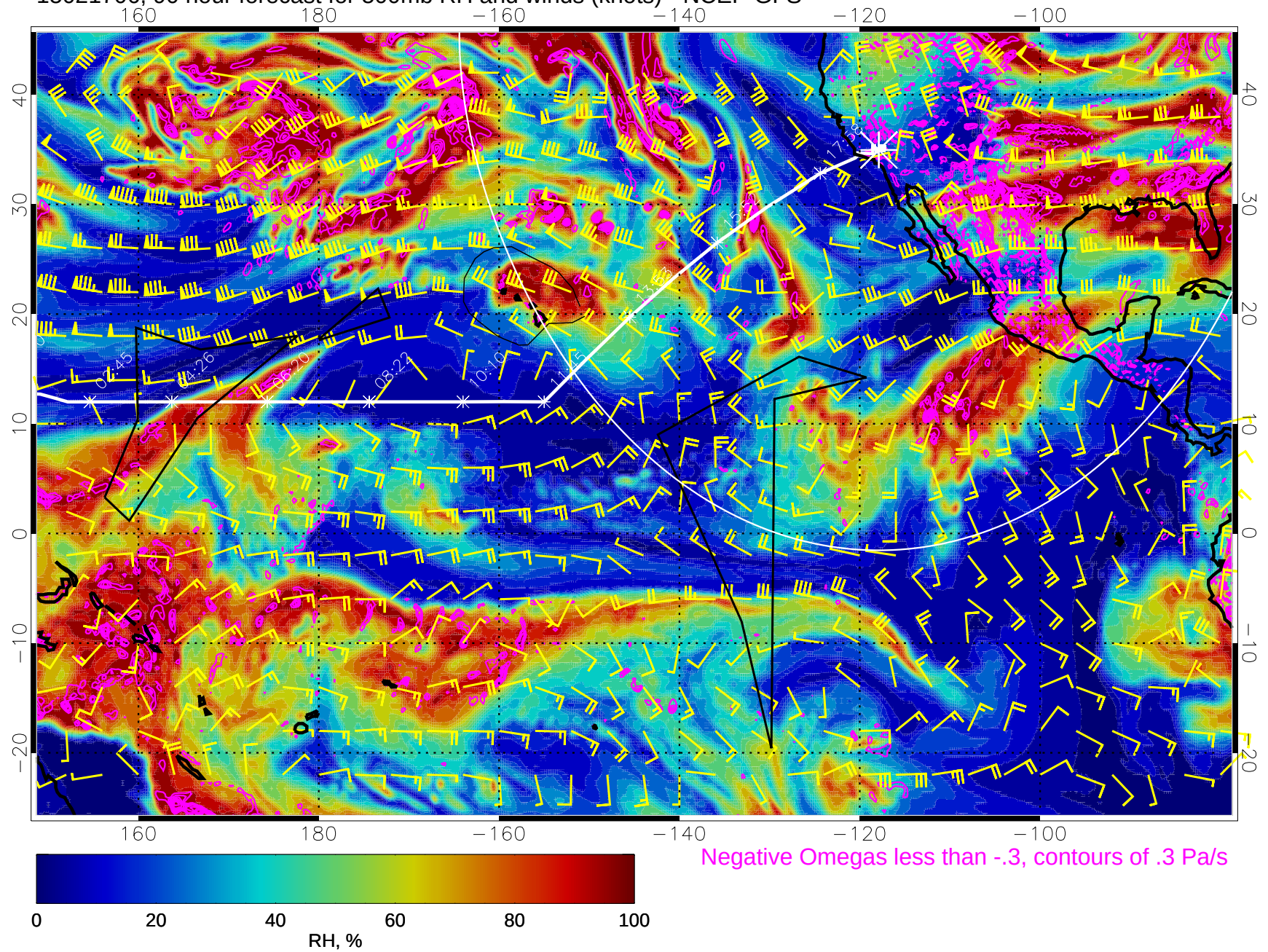
15021706, 90 hour forecast for 500mb RH and winds (knots) - NCEP GFS
