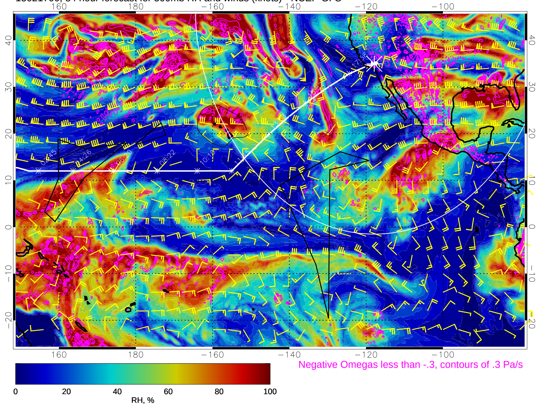
15021700, 84 hour forecast for 500mb RH and winds (knots) - NCEP GFS
