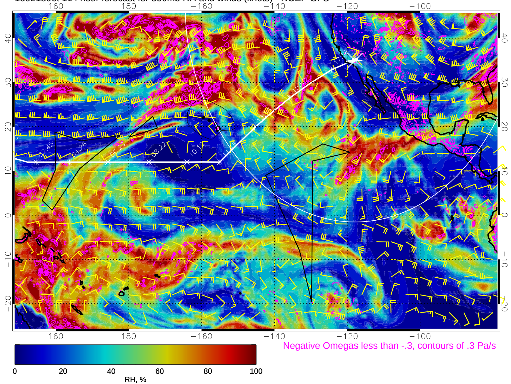
15021806, 114 hour forecast for 500mb RH and winds (knots) - NCEP GFS
