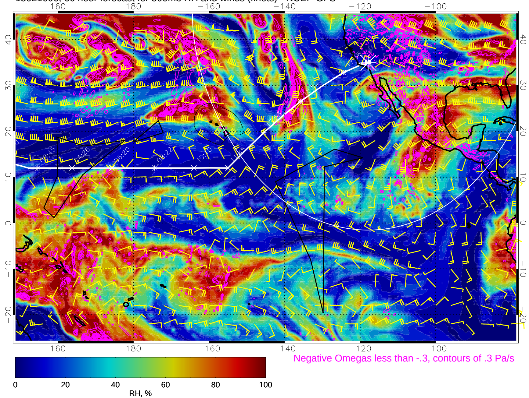
15021606, 66 hour forecast for 500mb RH and winds (knots) - NCEP GFS
