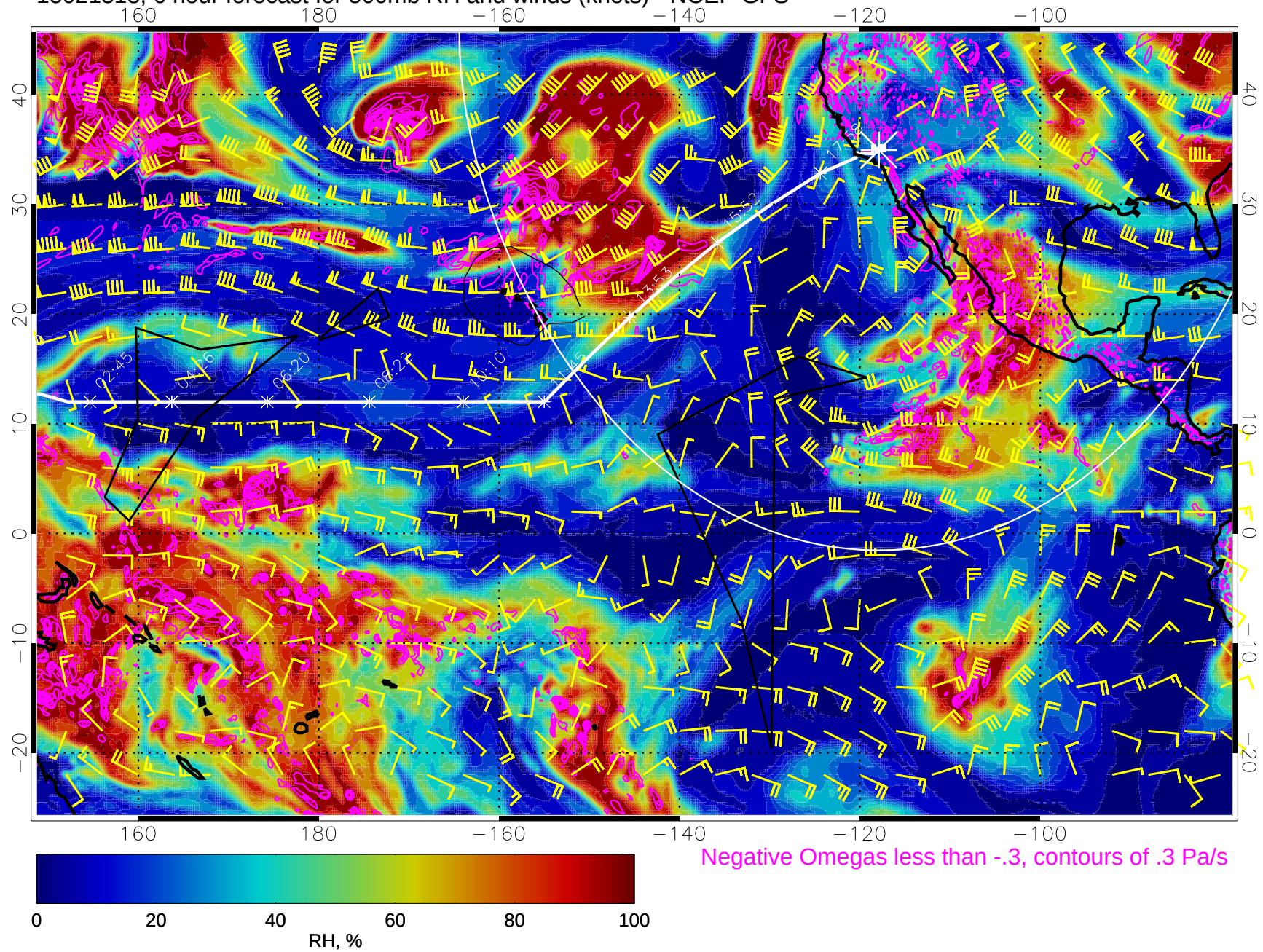
15021318, 6 hour forecast for 500mb RH and winds (knots) - NCEP GFS
