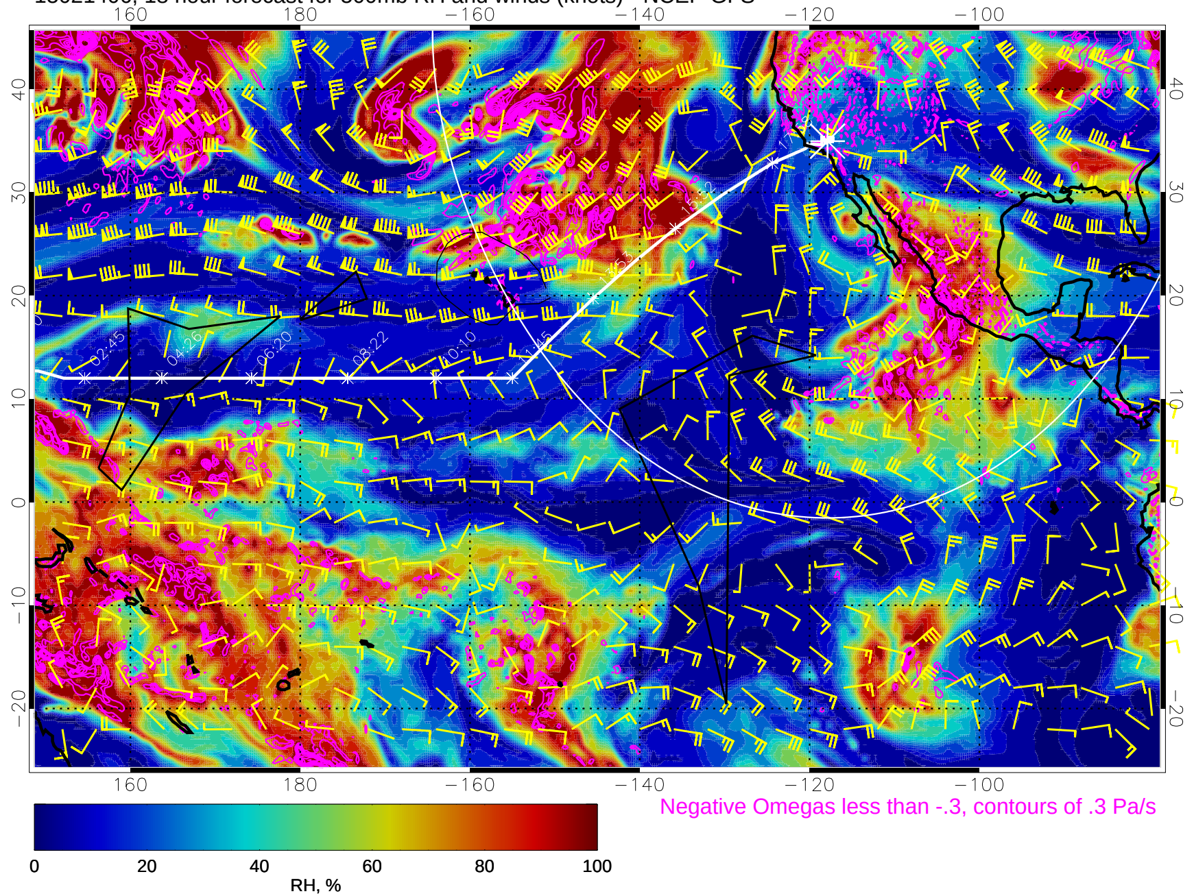
15021406, 18 hour forecast for 500mb RH and winds (knots) - NCEP GFS
