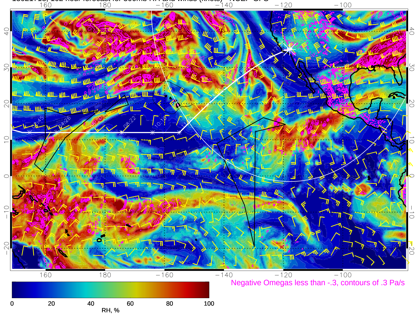
15021718, 102 hour forecast for 500mb RH and winds (knots) - NCEP GFS
