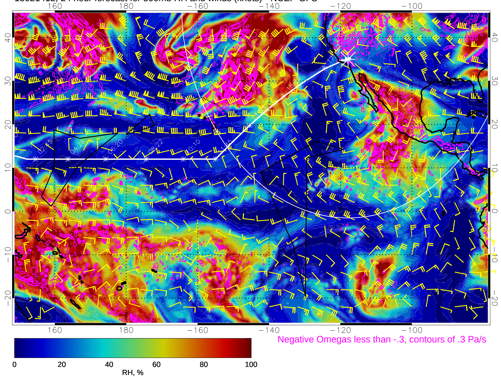
15021412, 24 hour forecast for 500mb RH and winds (knots) - NCEP GFS
