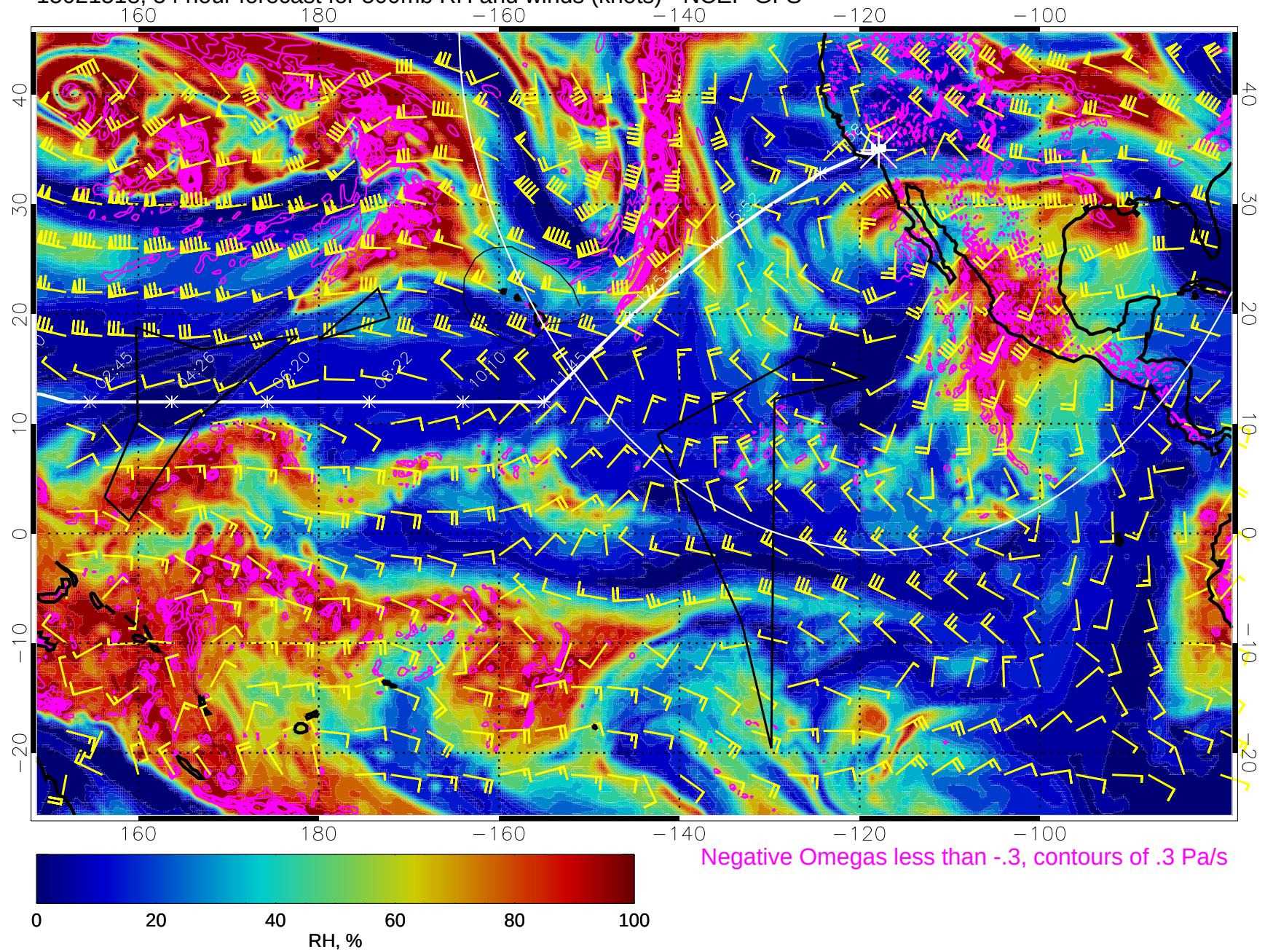
15021518, 54 hour forecast for 500mb RH and winds (knots) - NCEP GFS
