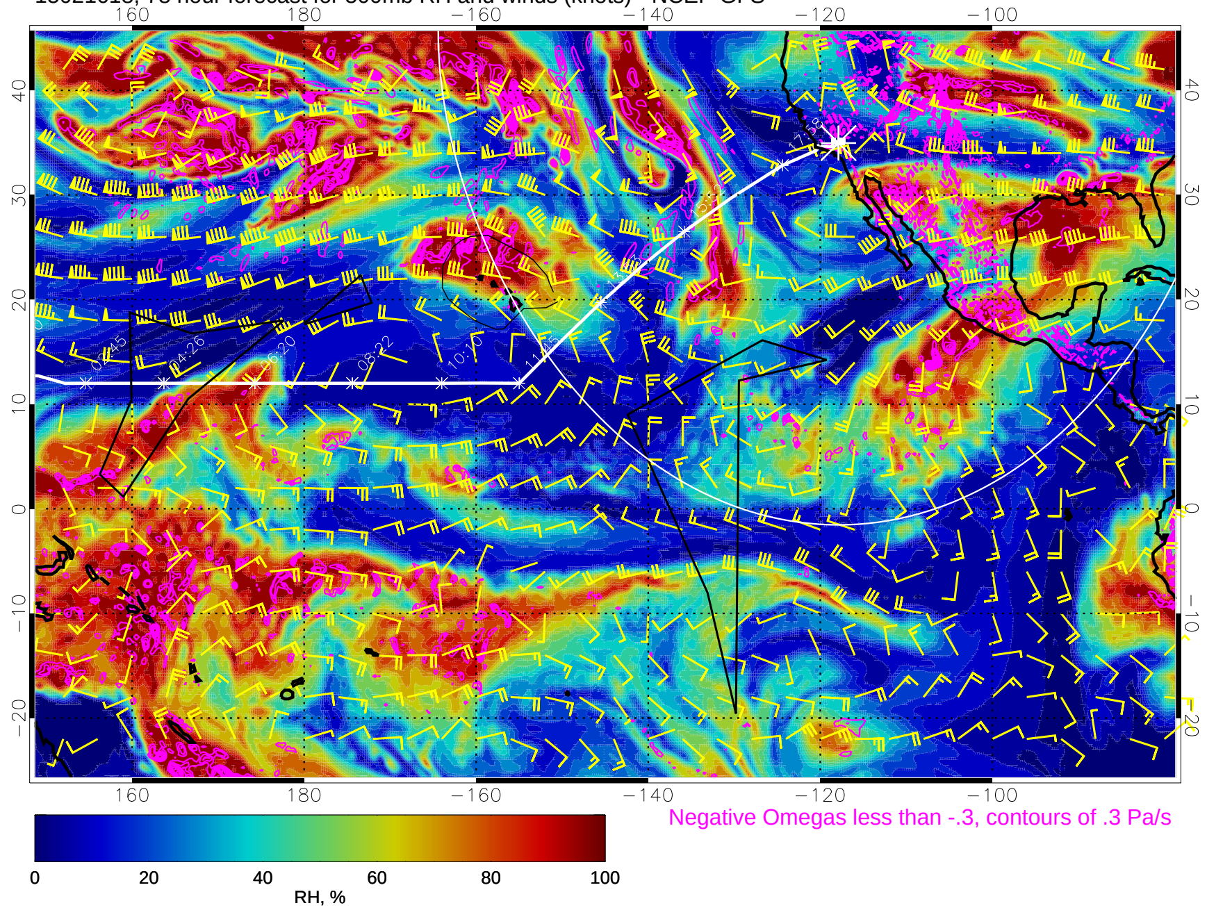
15021618, 78 hour forecast for 500mb RH and winds (knots) - NCEP GFS
