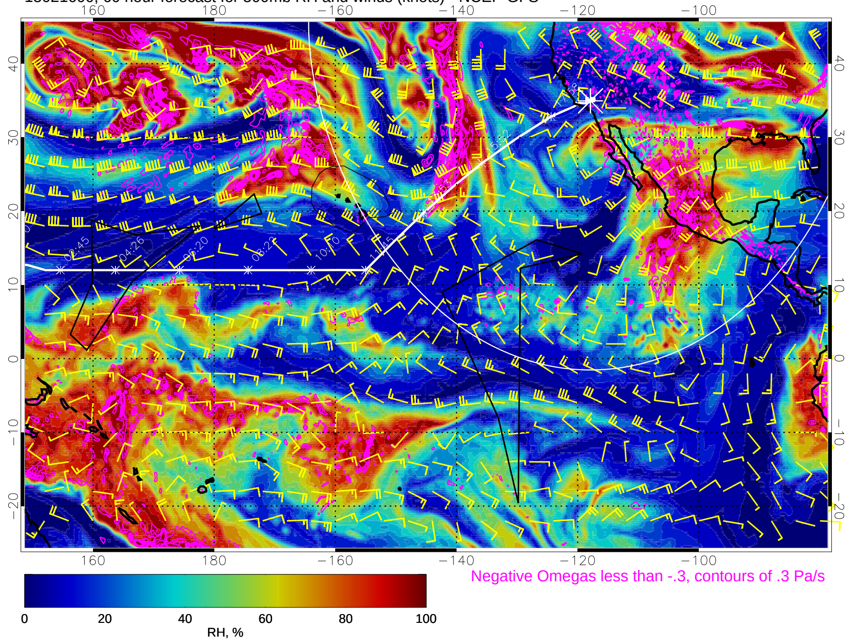
15021600, 60 hour forecast for 500mb RH and winds (knots) - NCEP GFS
