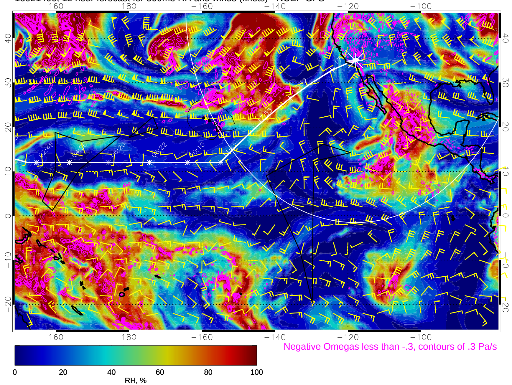
15021400, 12 hour forecast for 500mb RH and winds (knots) - NCEP GFS
