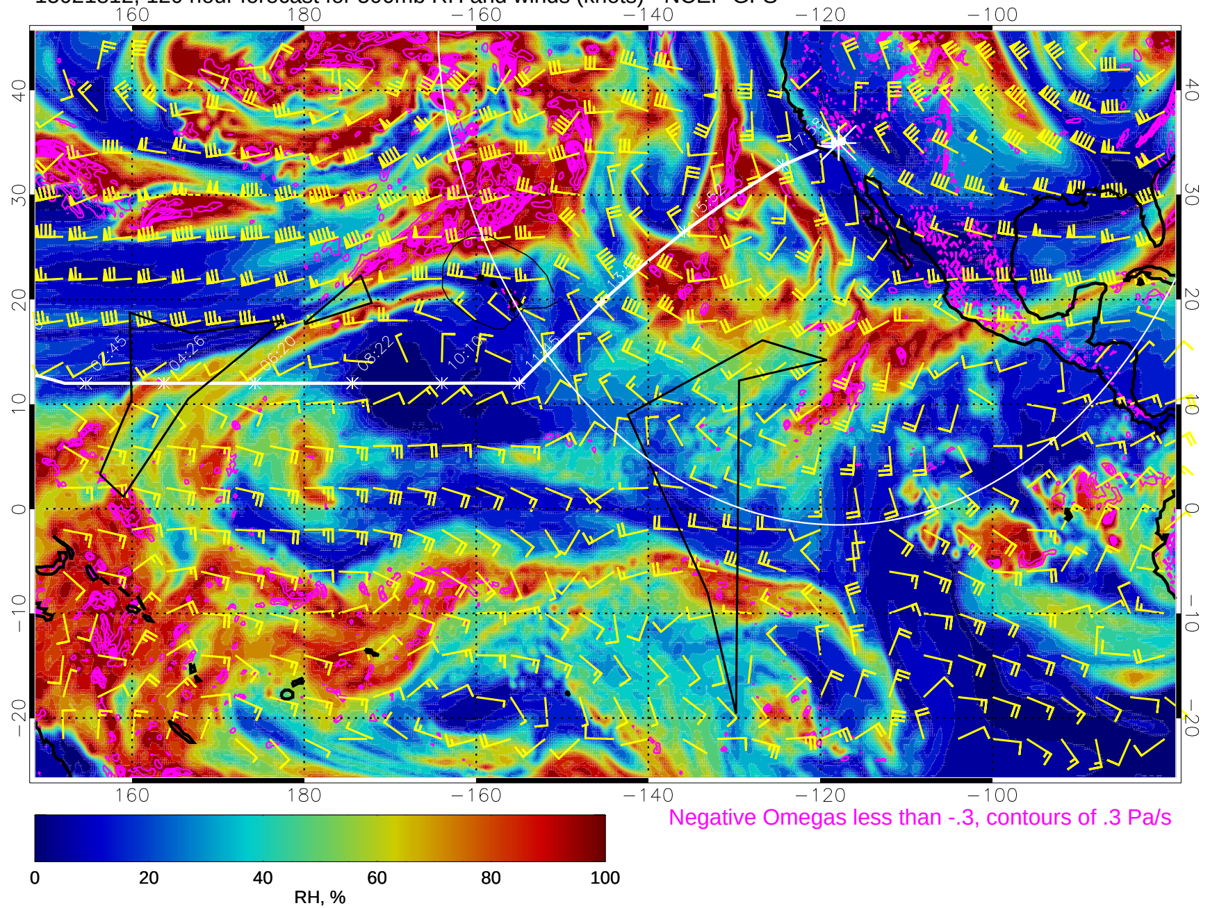
15021812, 120 hour forecast for 500mb RH and winds (knots) - NCEP GFS
