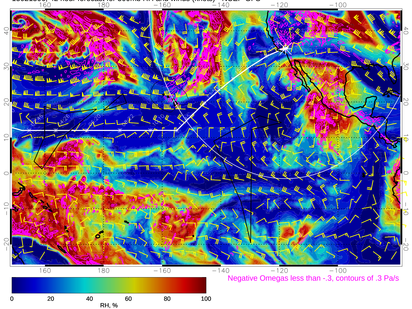
15021506, 42 hour forecast for 500mb RH and winds (knots) - NCEP GFS
