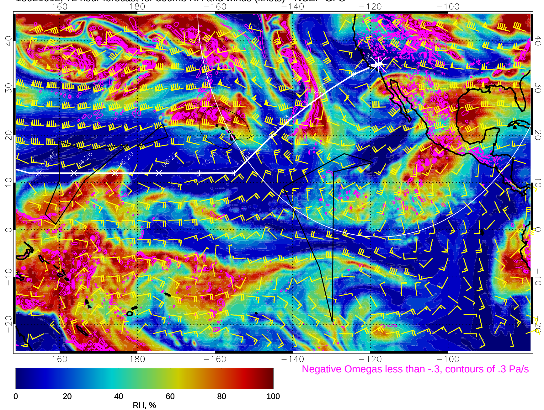
15021612, 72 hour forecast for 500mb RH and winds (knots) - NCEP GFS
