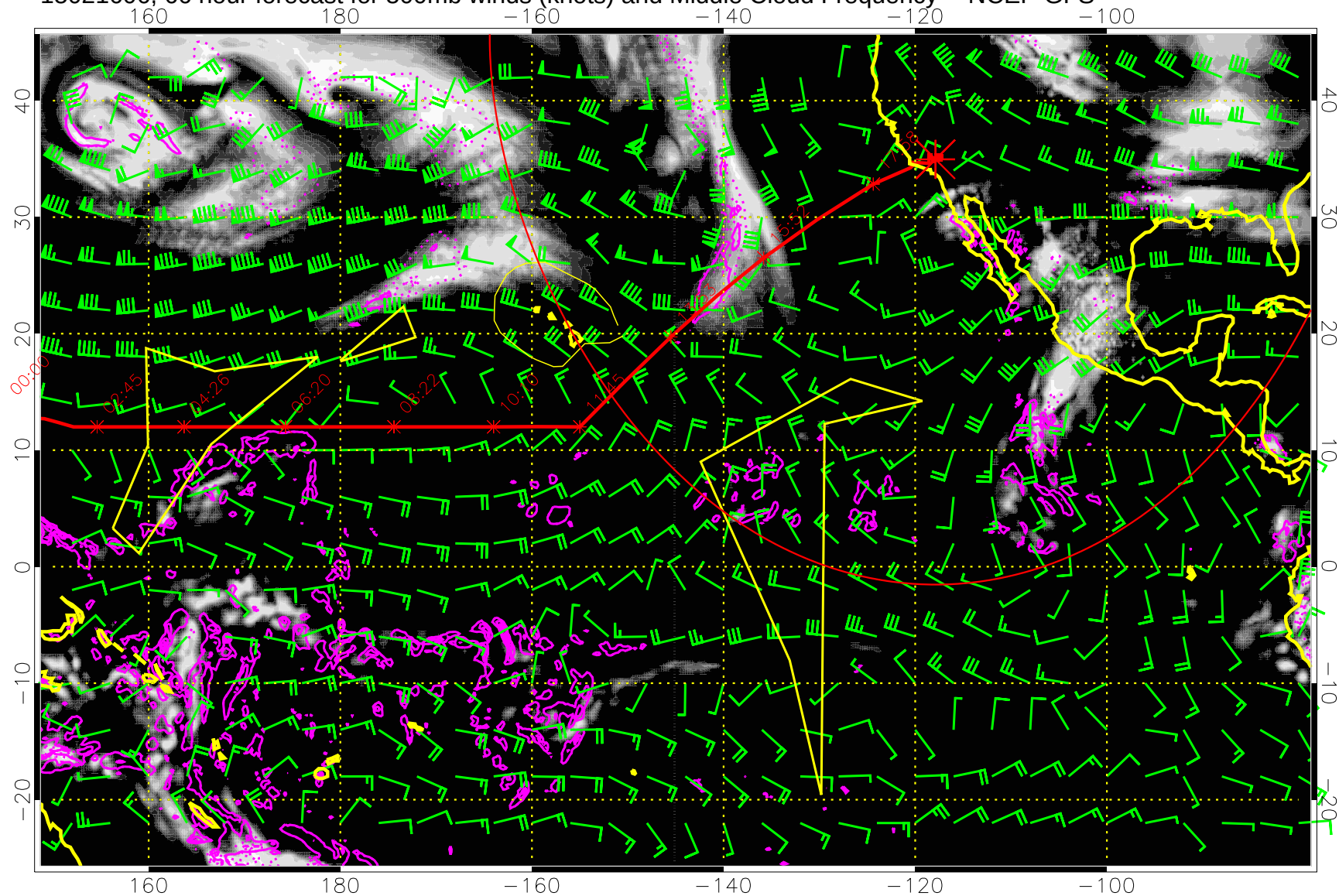
15021606, 66 hour forecast for 500mb winds (knots) and Middle Cloud Frequency -- NCEP GFS
