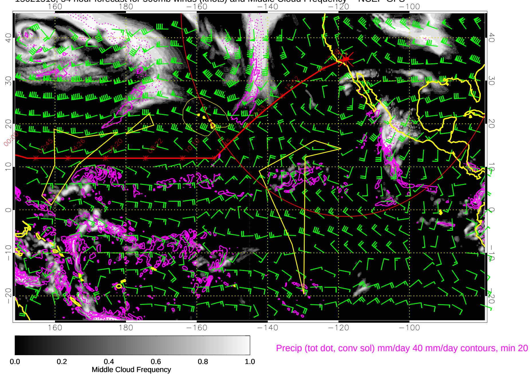
15021518, 54 hour forecast for 500mb winds (knots) and Middle Cloud Frequency -- NCEP GFS
