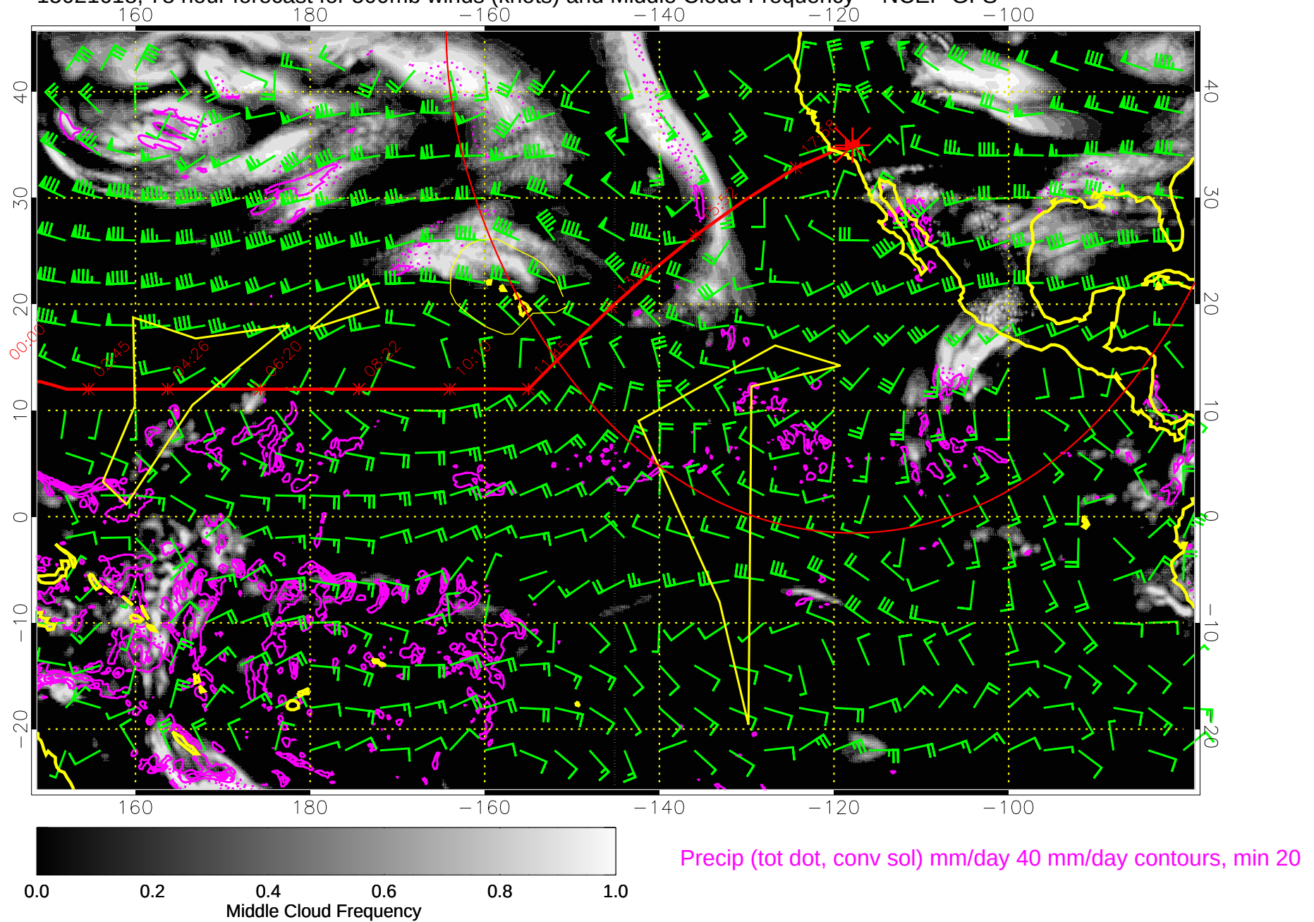
15021618, 78 hour forecast for 500mb winds (knots) and Middle Cloud Frequency -- NCEP GFS
