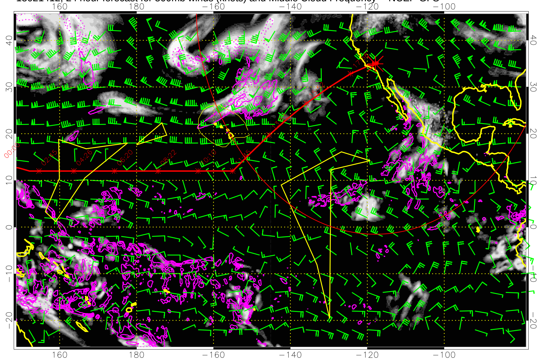
15021412, 24 hour forecast for 500mb winds (knots) and Middle Cloud Frequency -- NCEP GFS
