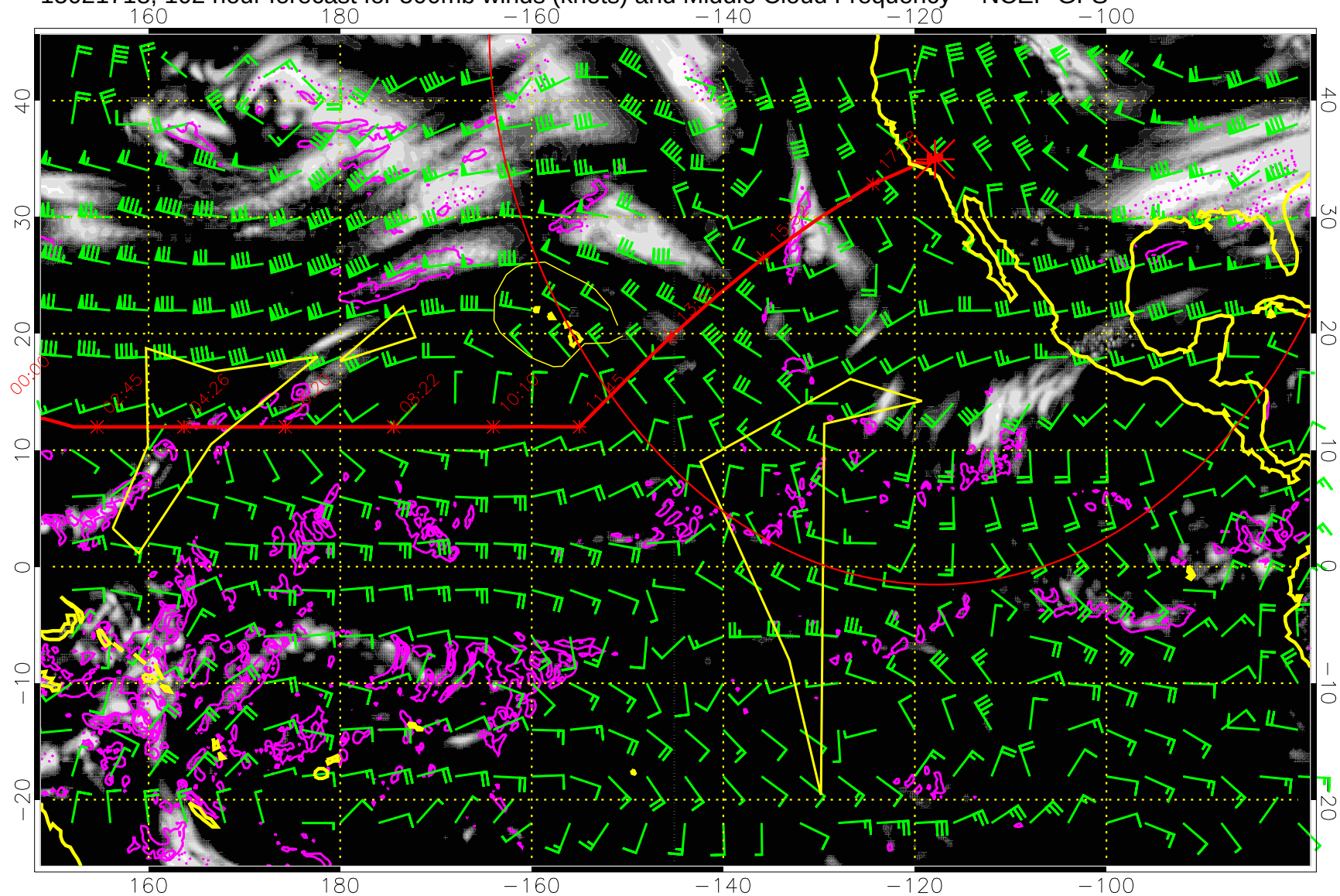
15021718, 102 hour forecast for 500mb winds (knots) and Middle Cloud Frequency -- NCEP GFS
