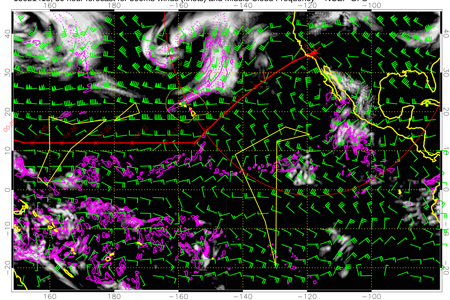
15021418, 30 hour forecast for 500mb winds (knots) and Middle Cloud Frequency -- NCEP GFS
