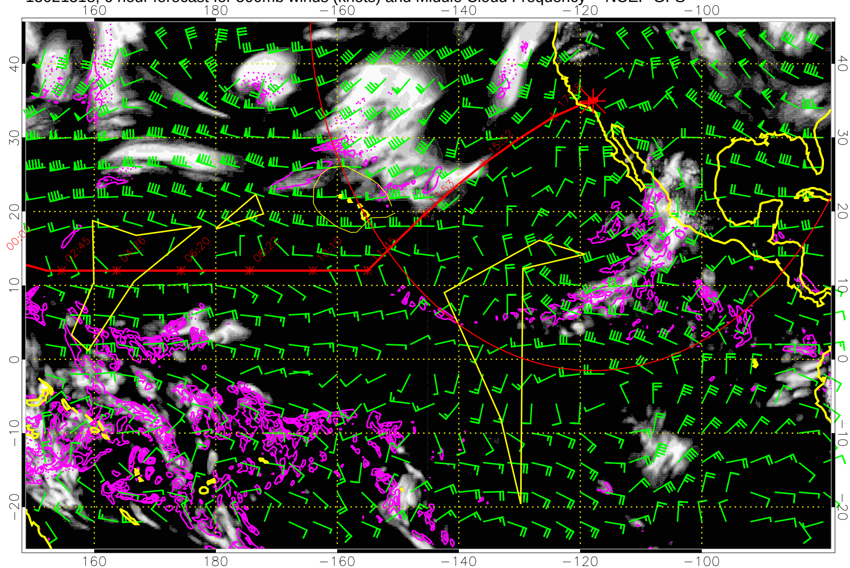
15021318, 6 hour forecast for 500mb winds (knots) and Middle Cloud Frequency -- NCEP GFS
