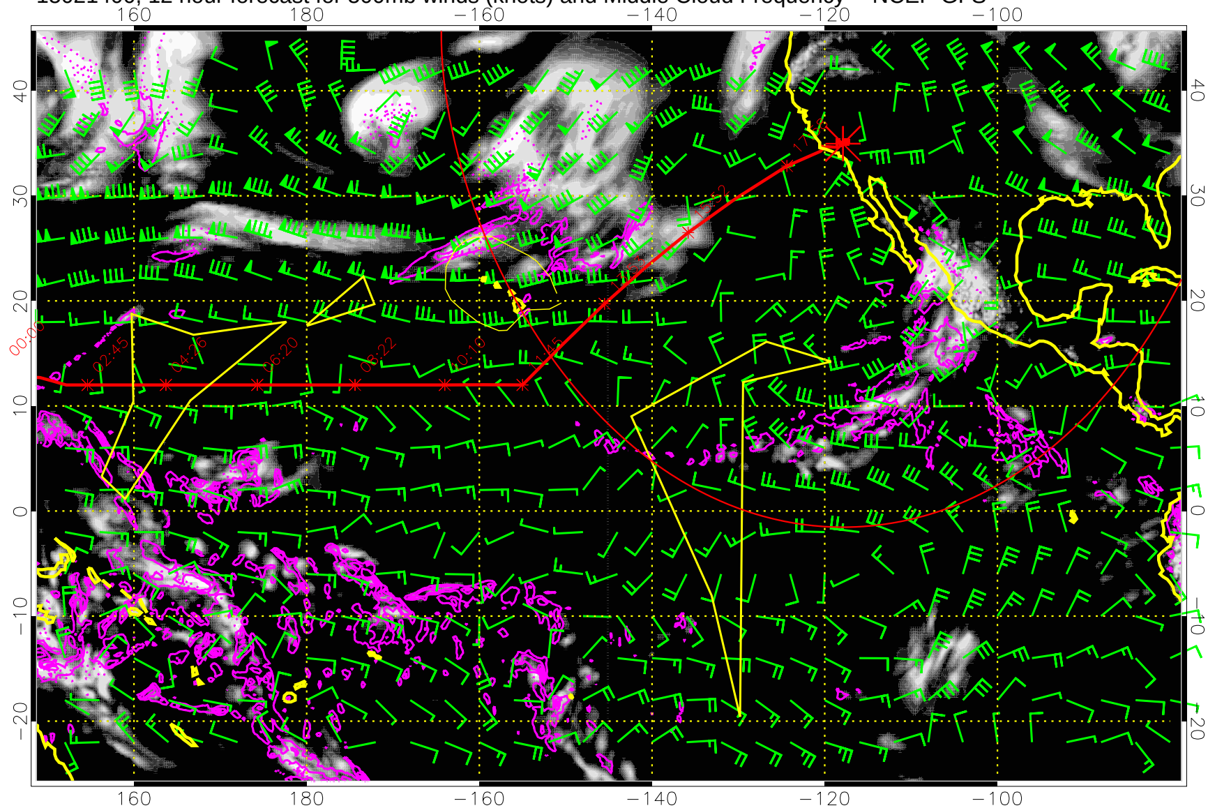
15021400, 12 hour forecast for 500mb winds (knots) and Middle Cloud Frequency -- NCEP GFS
