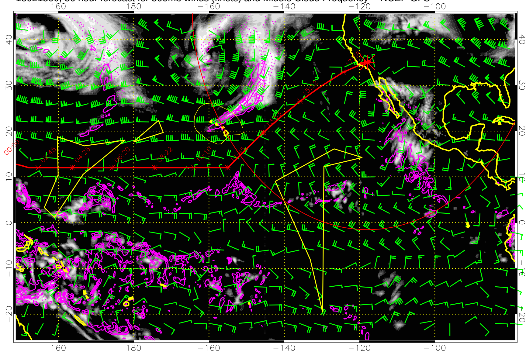
15021500, 36 hour forecast for 500mb winds (knots) and Middle Cloud Frequency -- NCEP GFS
