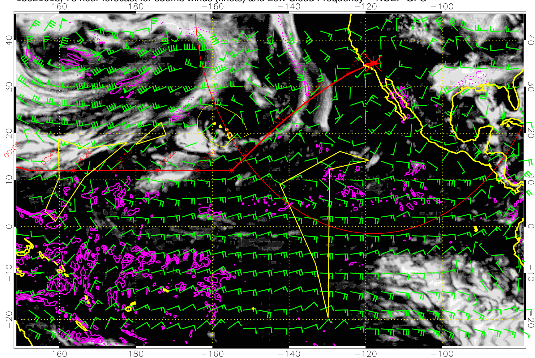
15021618, 78 hour forecast for 850mb winds (knots) and Low Cloud Frequency -- NCEP GFS
