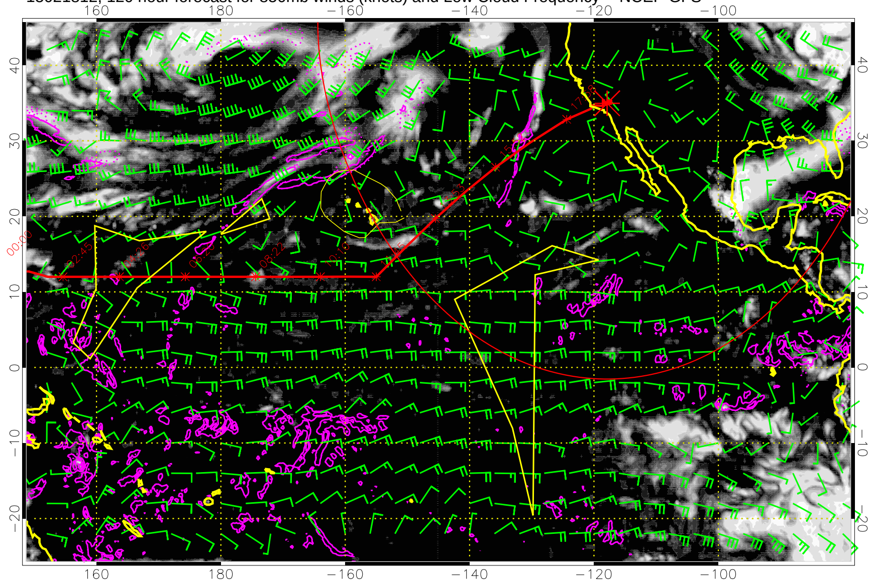
15021812, 120 hour forecast for 850mb winds (knots) and Low Cloud Frequency -- NCEP GFS
