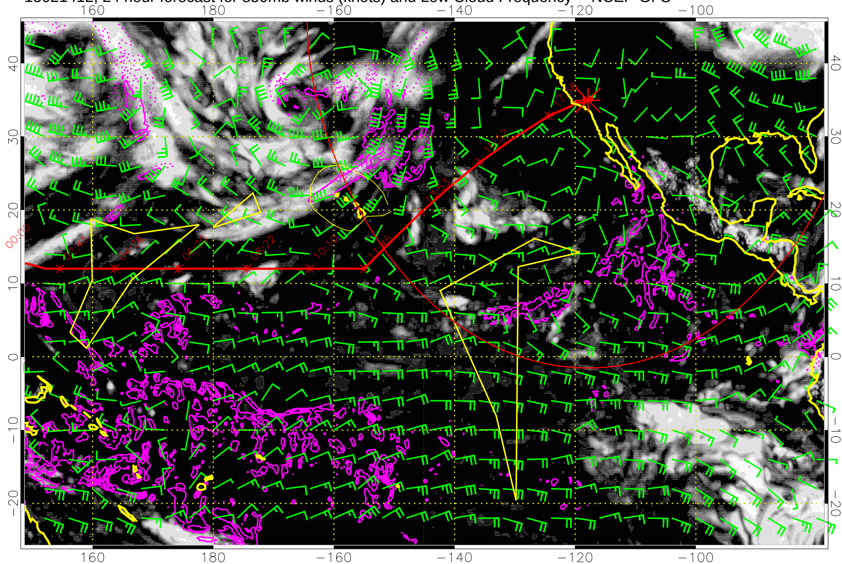
15021412, 24 hour forecast for 850mb winds (knots) and Low Cloud Frequency -- NCEP GFS
