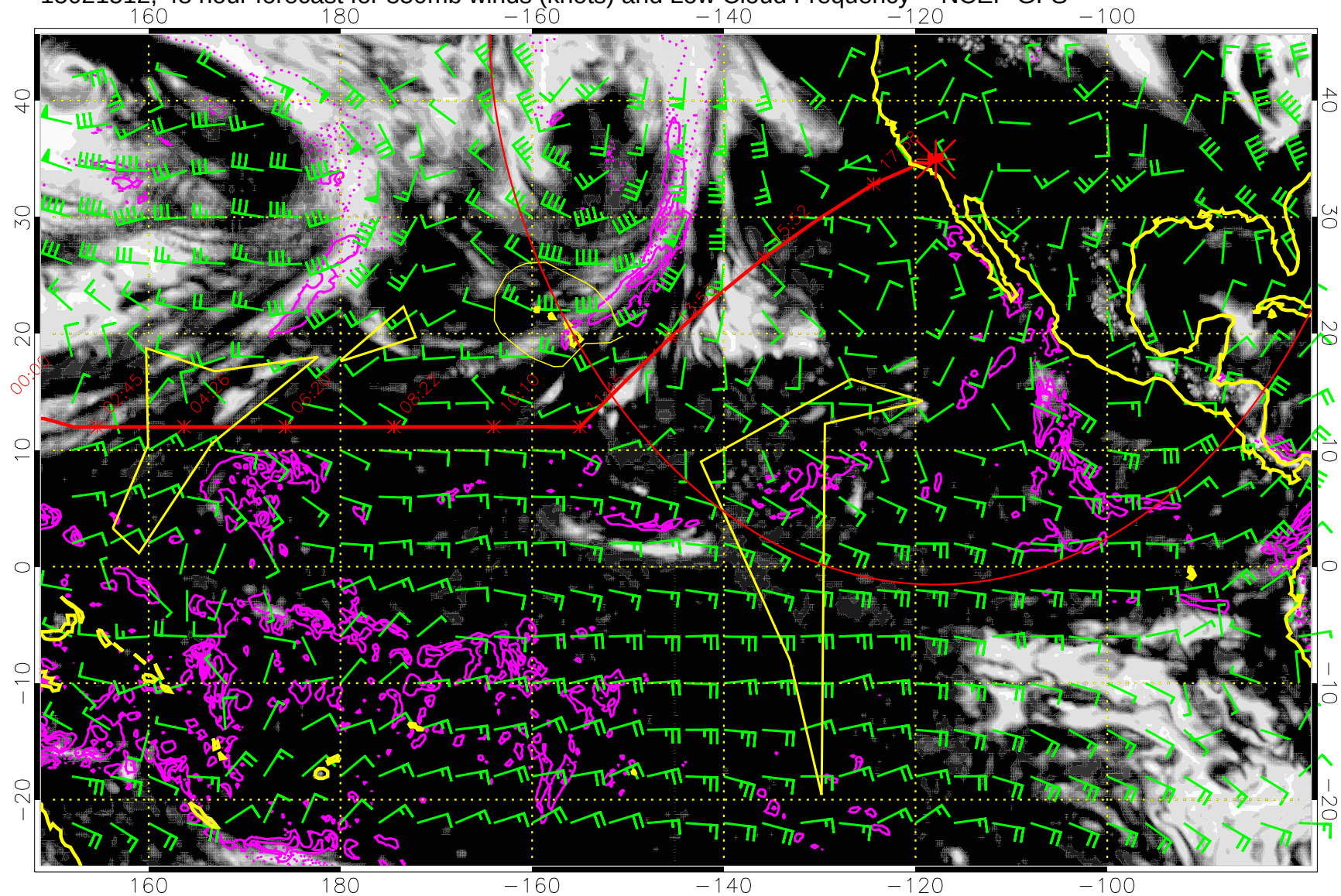
15021512, 48 hour forecast for 850mb winds (knots) and Low Cloud Frequency -- NCEP GFS
