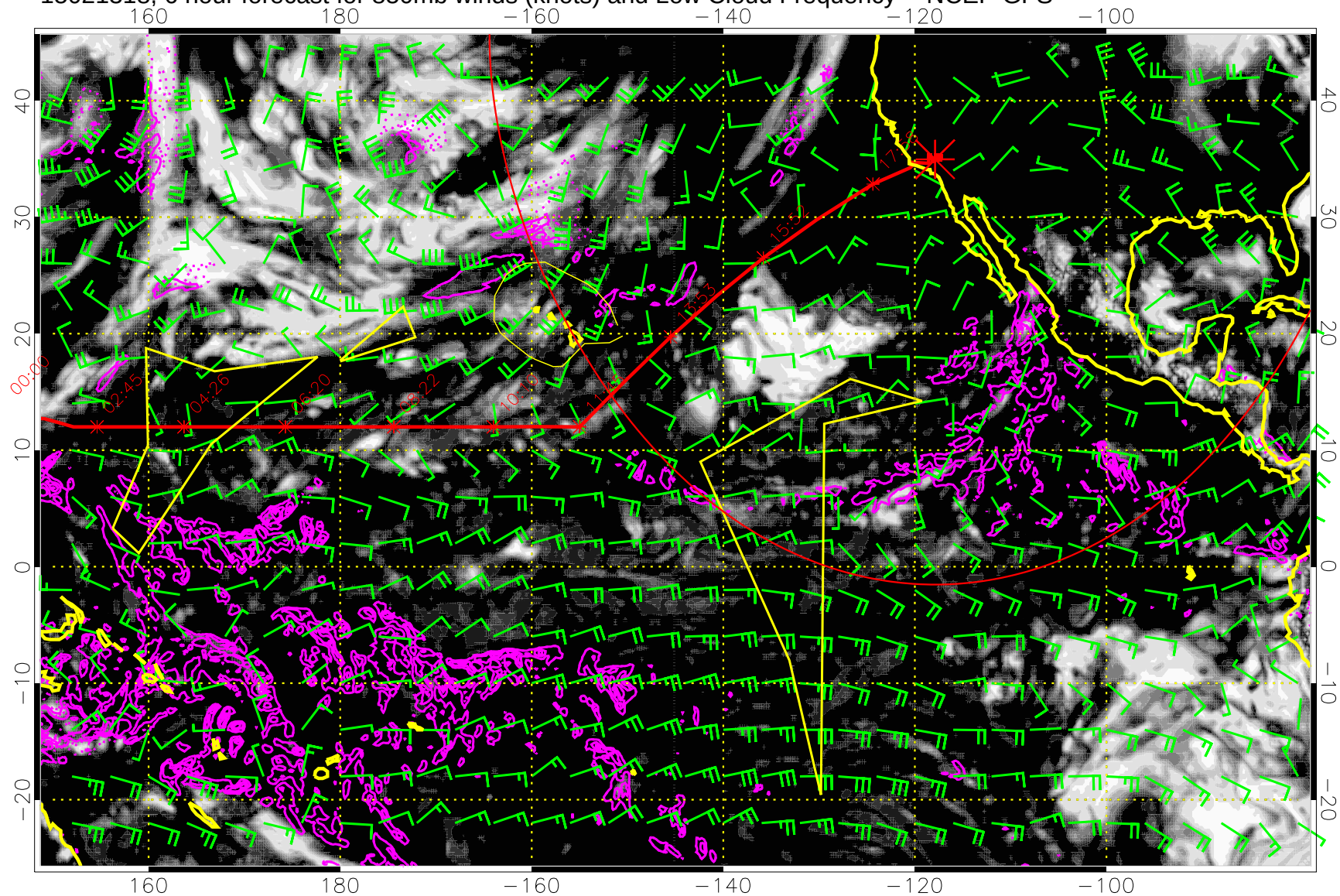
15021318, 6 hour forecast for 850mb winds (knots) and Low Cloud Frequency -- NCEP GFS
