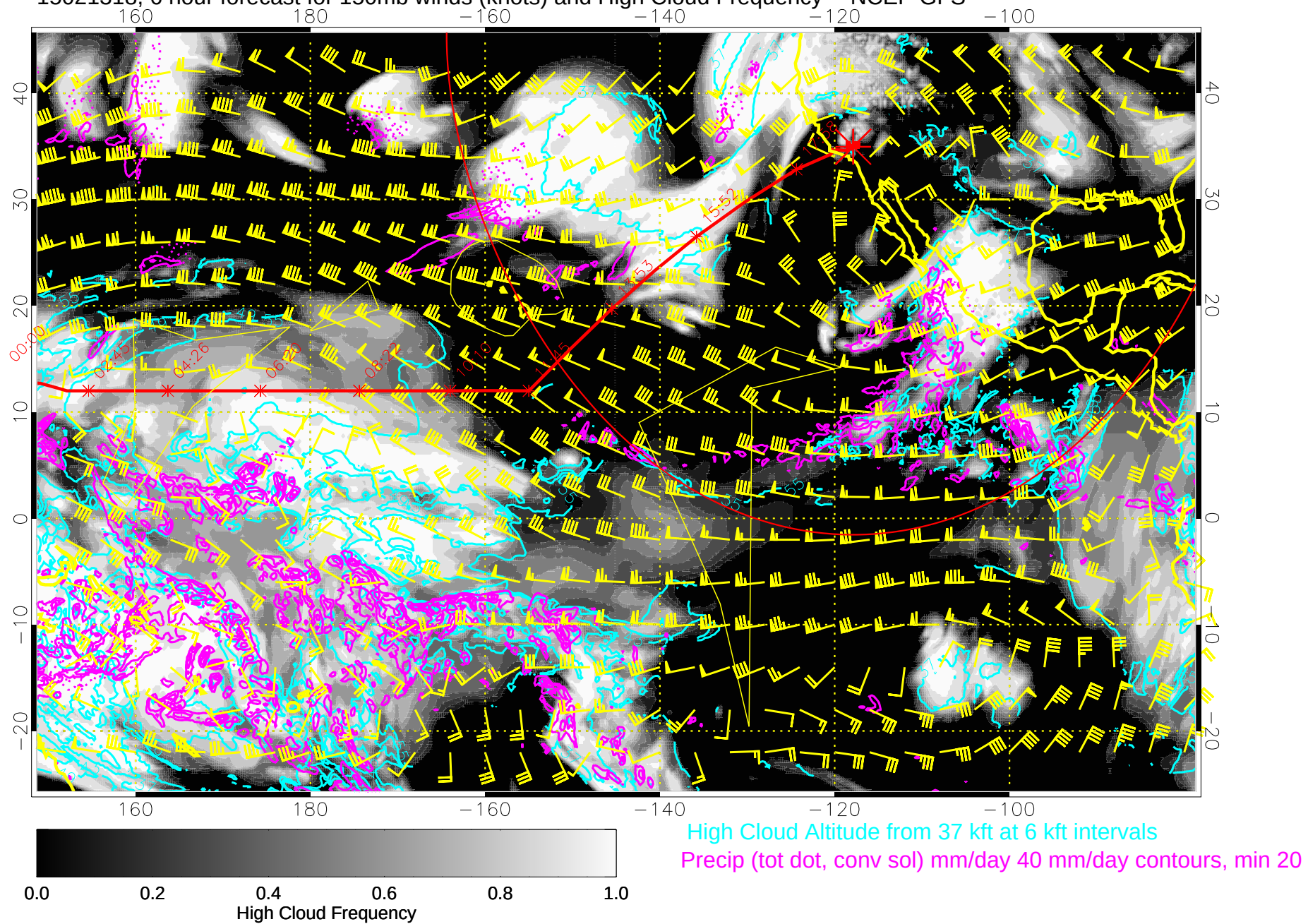
15021318, 6 hour forecast for 150mb winds (knots) and High Cloud Frequency -- NCEP GFS
