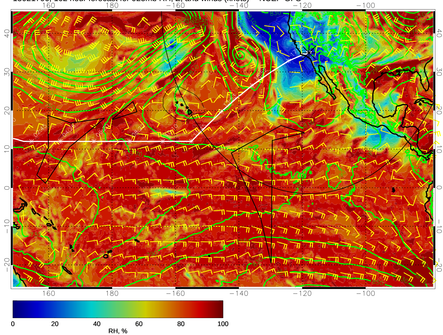
15021706, 102 hour forecast for 925mb RH, Z, and winds (knots) -- NCEP GFS
