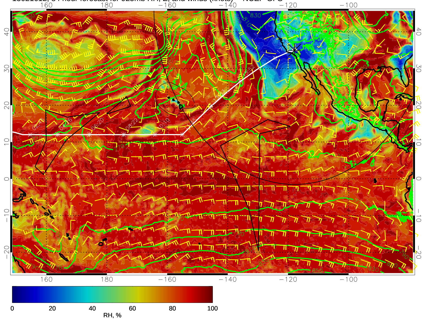
15021612, 84 hour forecast for 925mb RH, Z, and winds (knots) -- NCEP GFS
