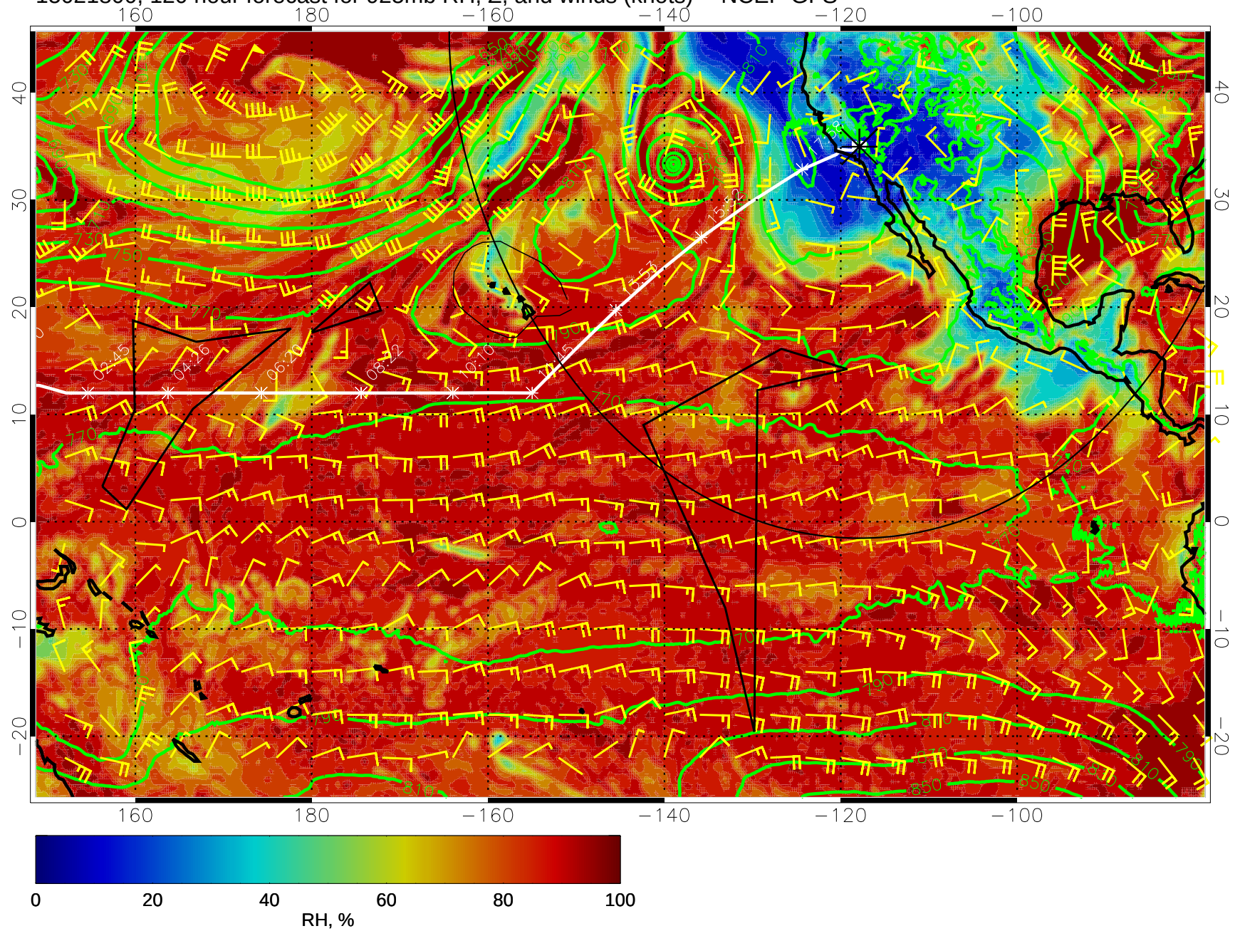
15021800, 120 hour forecast for 925mb RH, Z, and winds (knots) -- NCEP GFS
