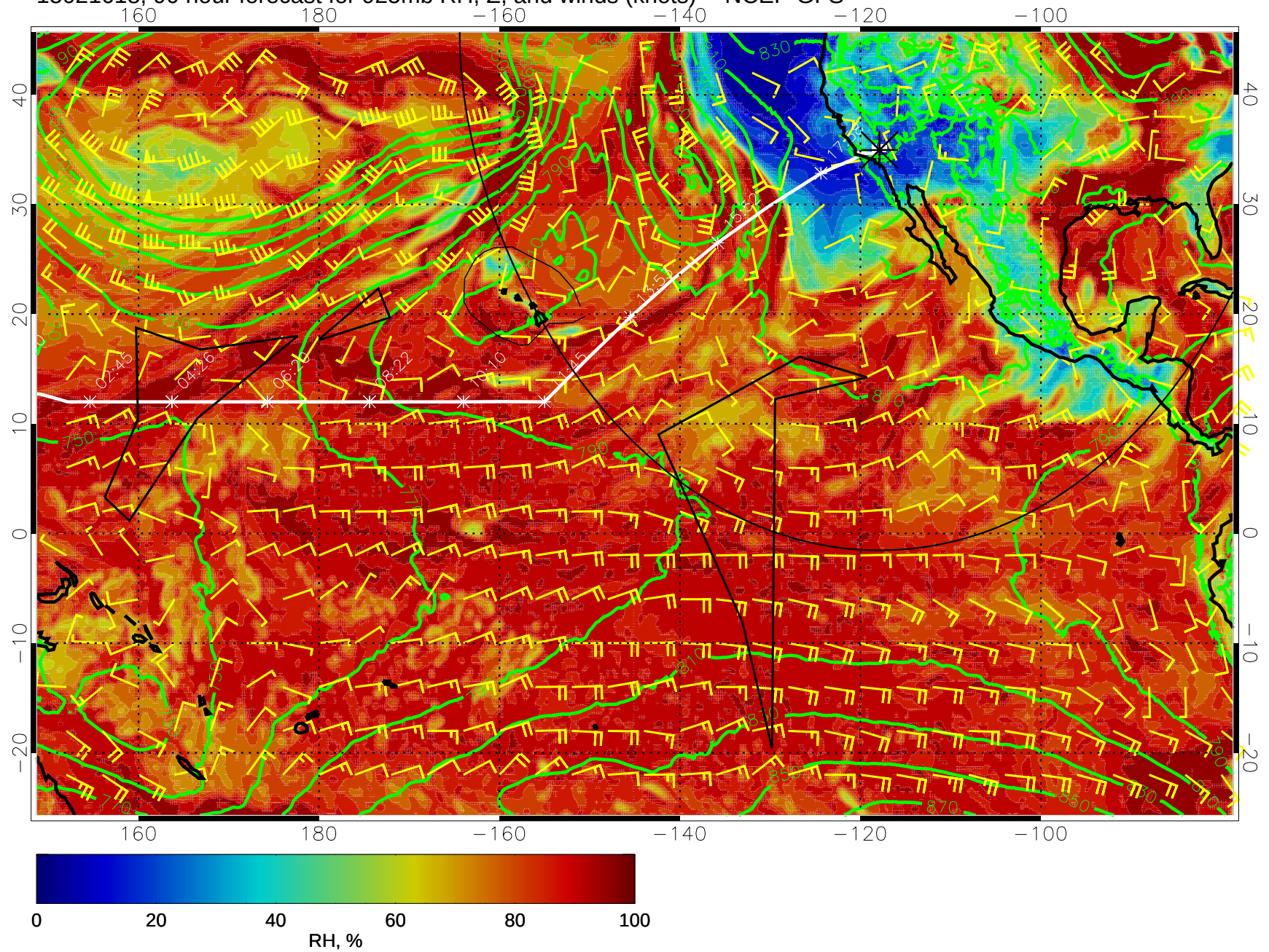
15021618, 90 hour forecast for 925mb RH, Z, and winds (knots) -- NCEP GFS
