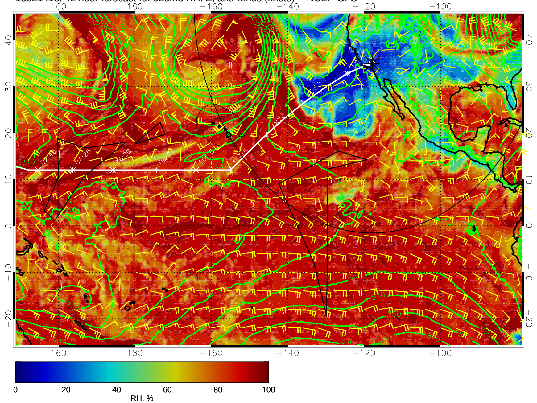
15021418, 42 hour forecast for 925mb RH, Z, and winds (knots) -- NCEP GFS
