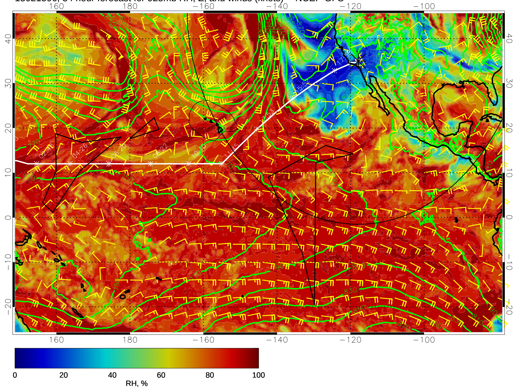
15021506, 54 hour forecast for 925mb RH, Z, and winds (knots) -- NCEP GFS
