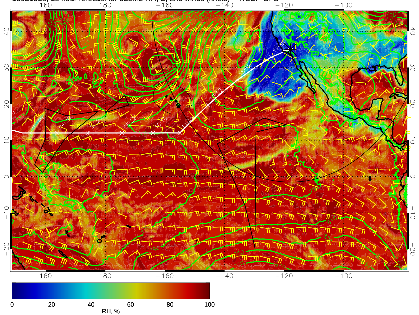
15021318, 18 hour forecast for 925mb RH, Z, and winds (knots) -- NCEP GFS
