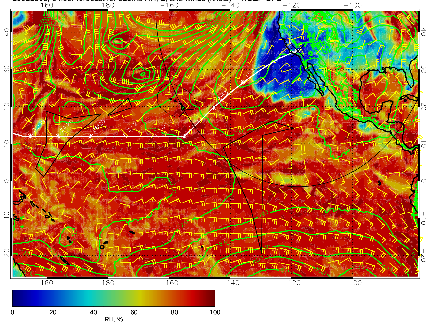
15021306, 6 hour forecast for 925mb RH, Z, and winds (knots) -- NCEP GFS
