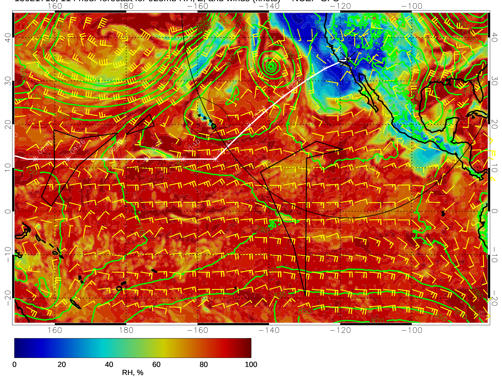
15021718, 114 hour forecast for 925mb RH, Z, and winds (knots) -- NCEP GFS
