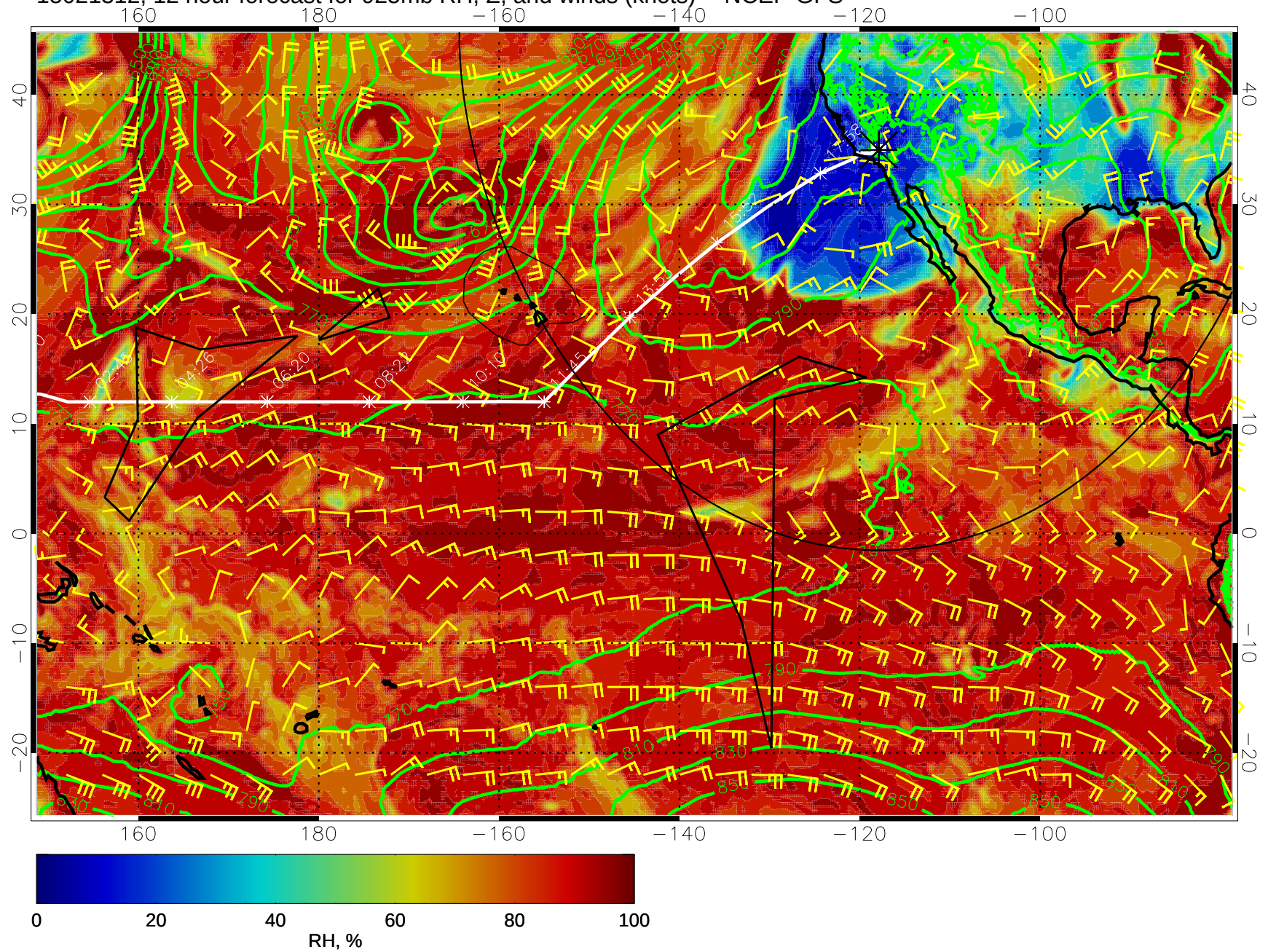
15021312, 12 hour forecast for 925mb RH, Z, and winds (knots) -- NCEP GFS
