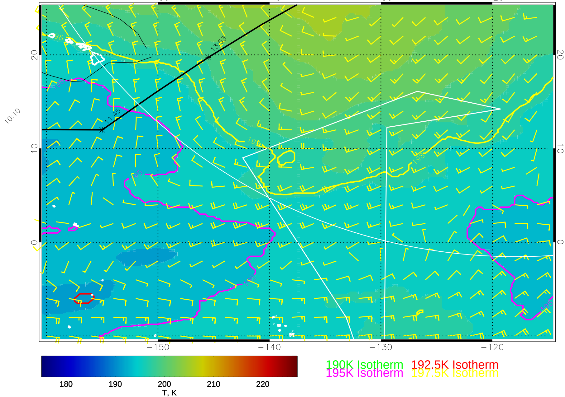
15021800, 120 hour forecast for 70mb T and winds (knots) -- NCEP GFS
