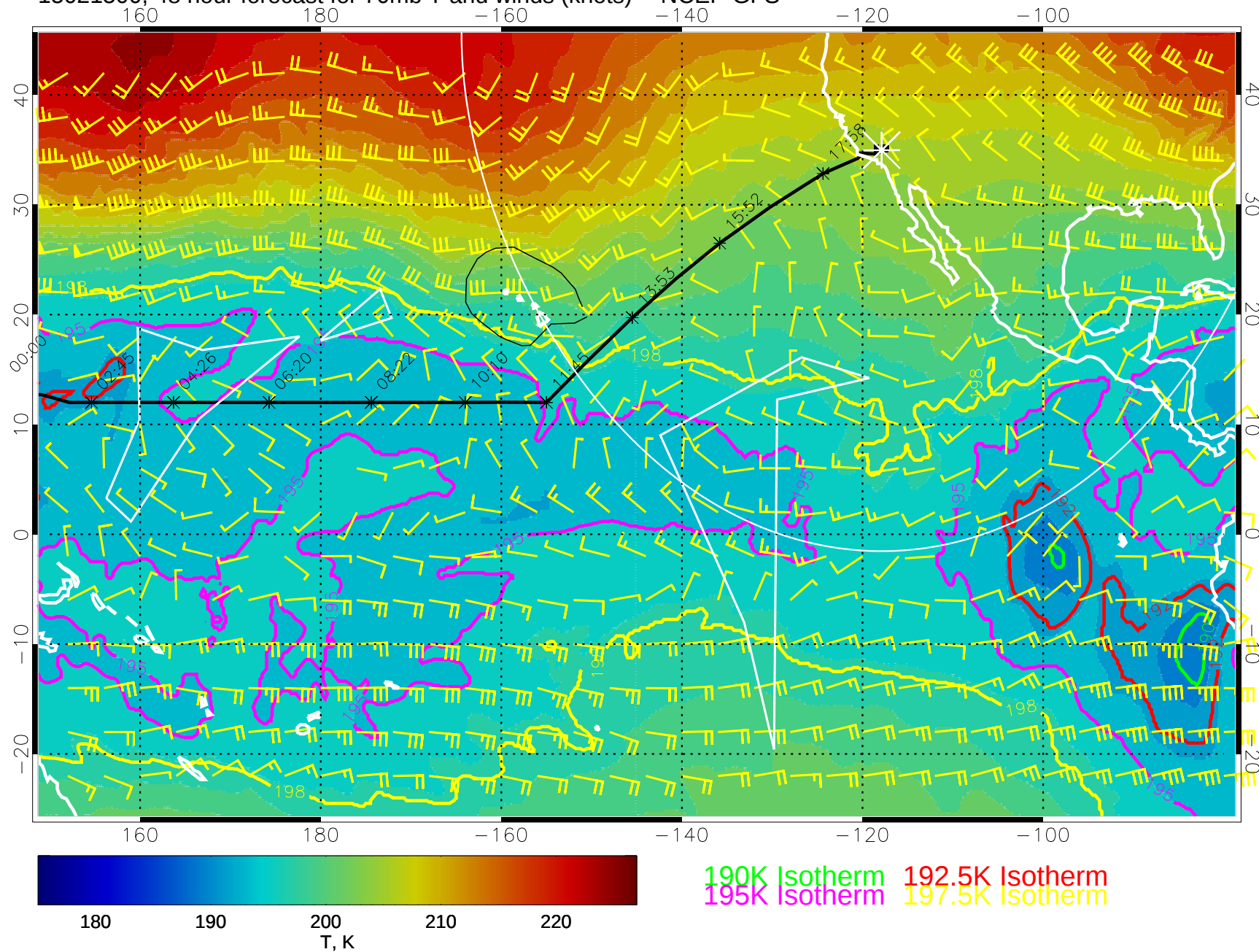
15021500, 48 hour forecast for 70mb T and winds (knots) -- NCEP GFS
