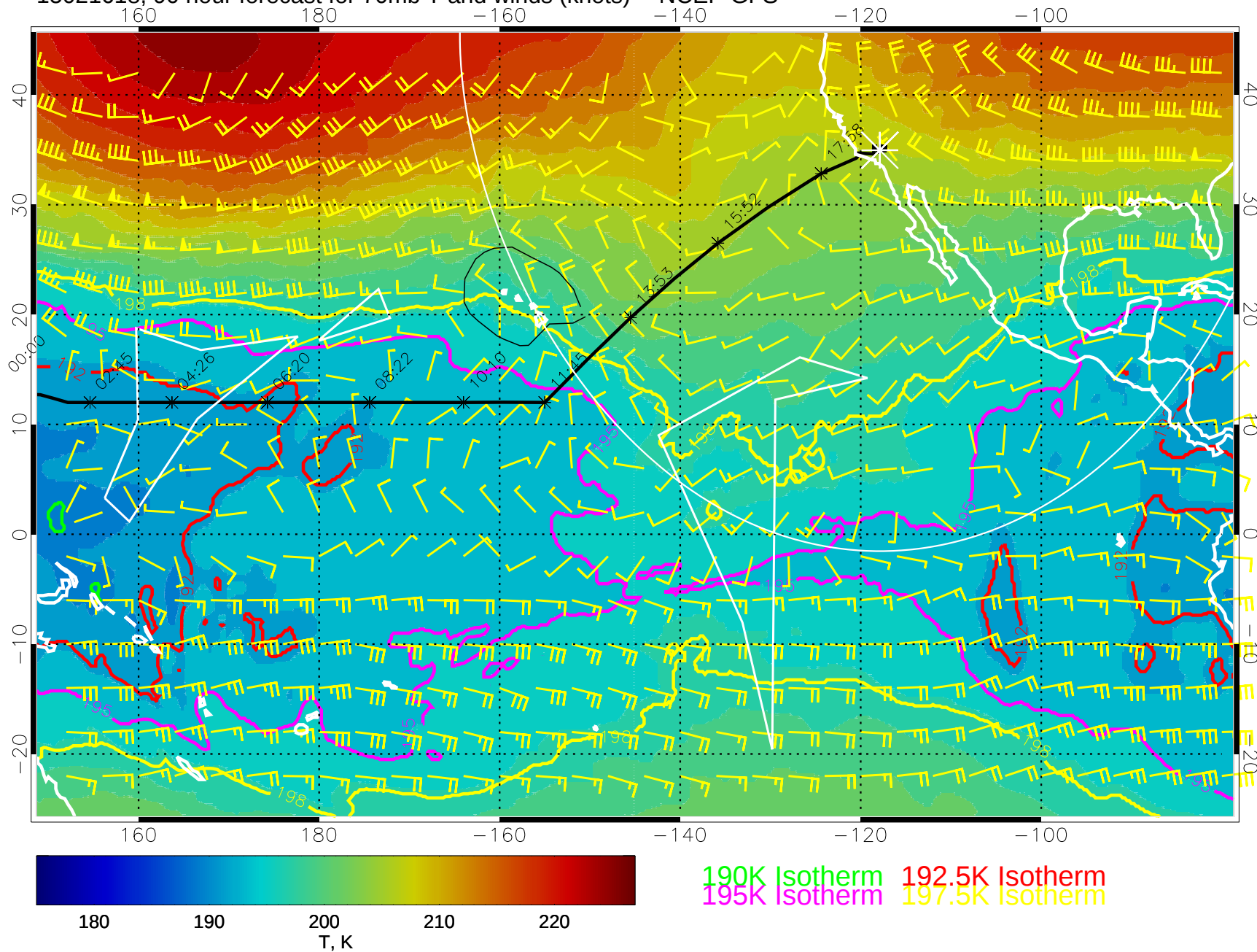
15021618, 90 hour forecast for 70mb T and winds (knots) -- NCEP GFS
