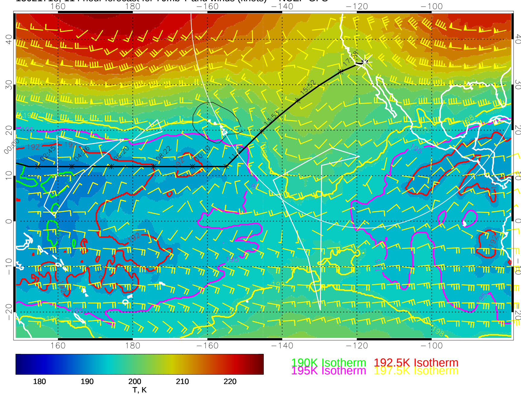
15021718, 114 hour forecast for 70mb T and winds (knots) -- NCEP GFS
