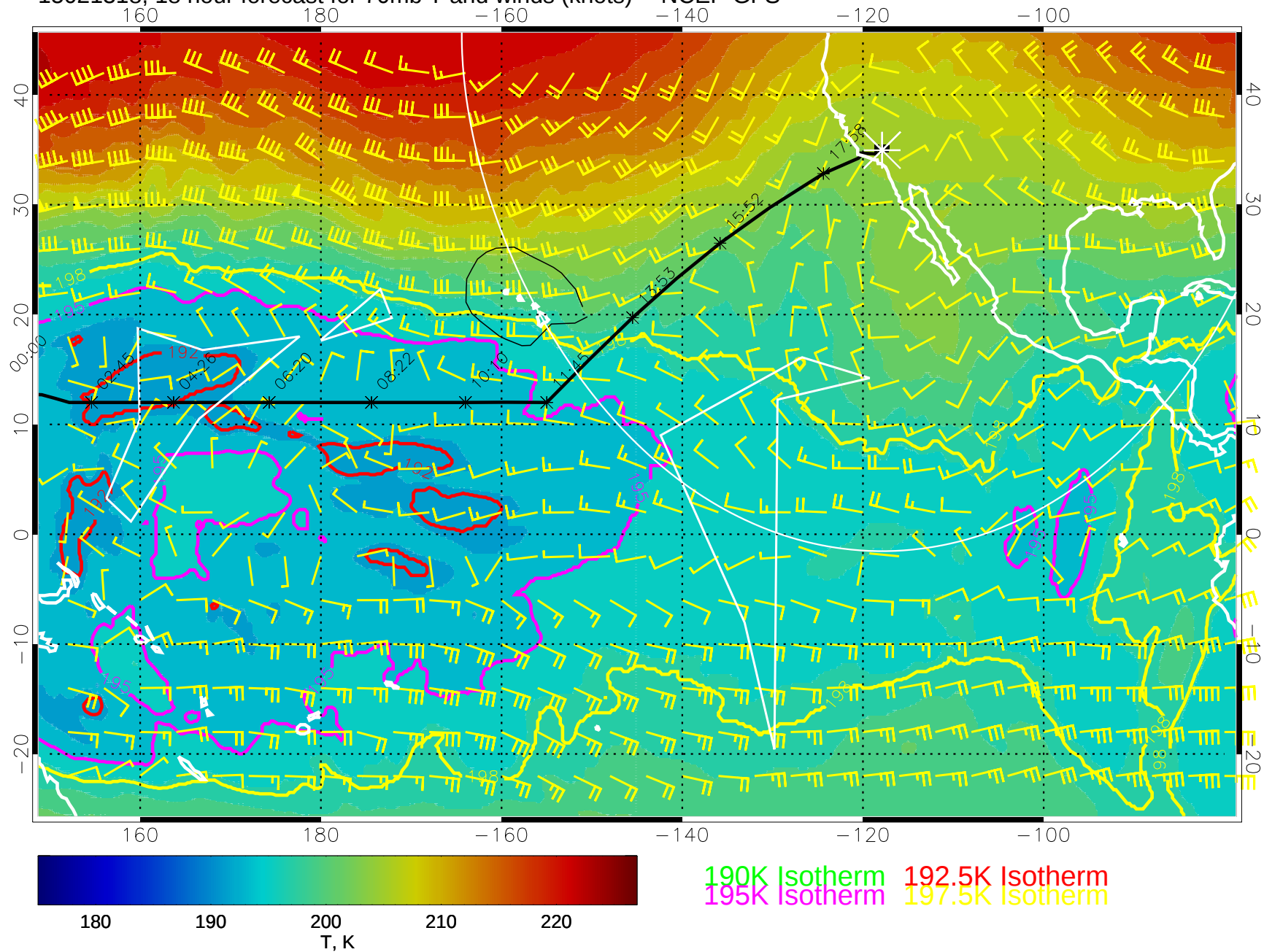
15021318, 18 hour forecast for 70mb T and winds (knots) -- NCEP GFS
