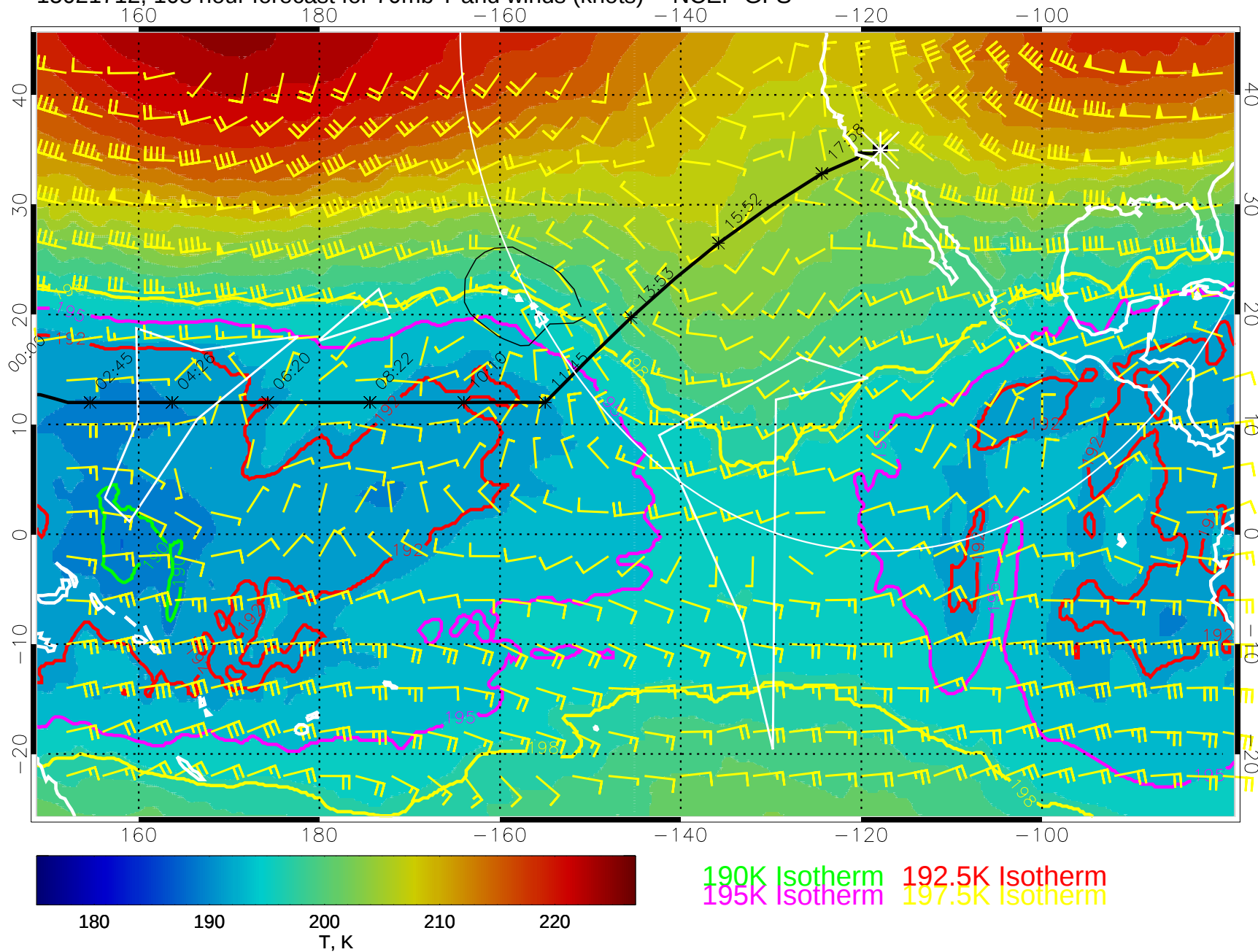
15021712, 108 hour forecast for 70mb T and winds (knots) -- NCEP GFS
