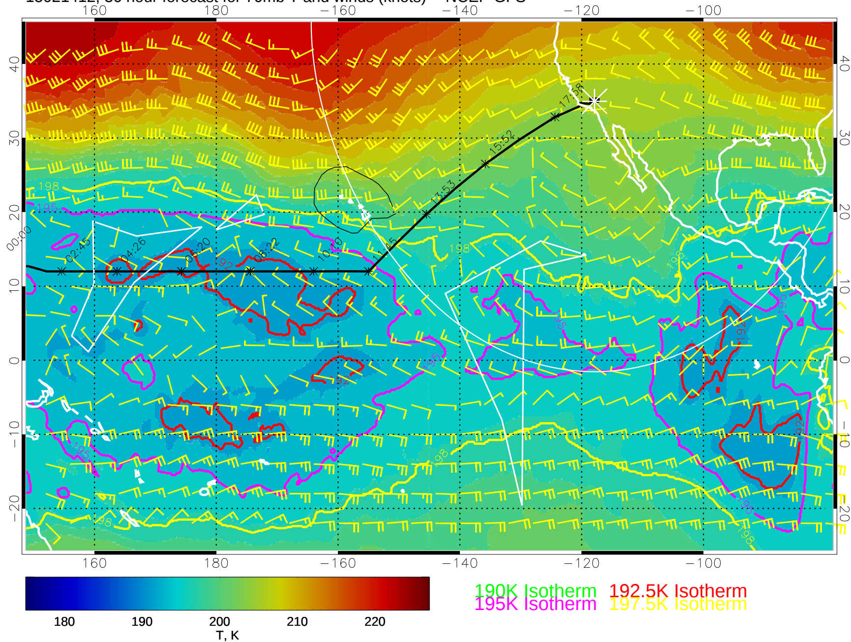
15021412, 36 hour forecast for 70mb T and winds (knots) -- NCEP GFS
