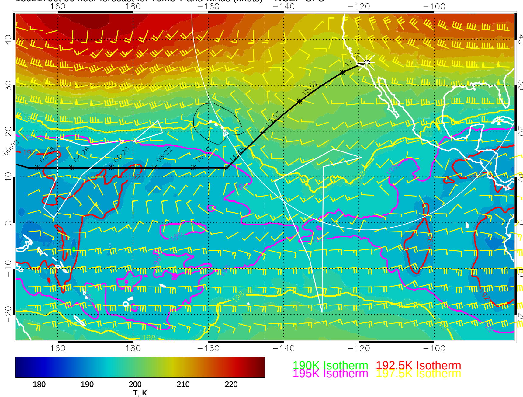
15021700, 96 hour forecast for 70mb T and winds (knots) -- NCEP GFS
