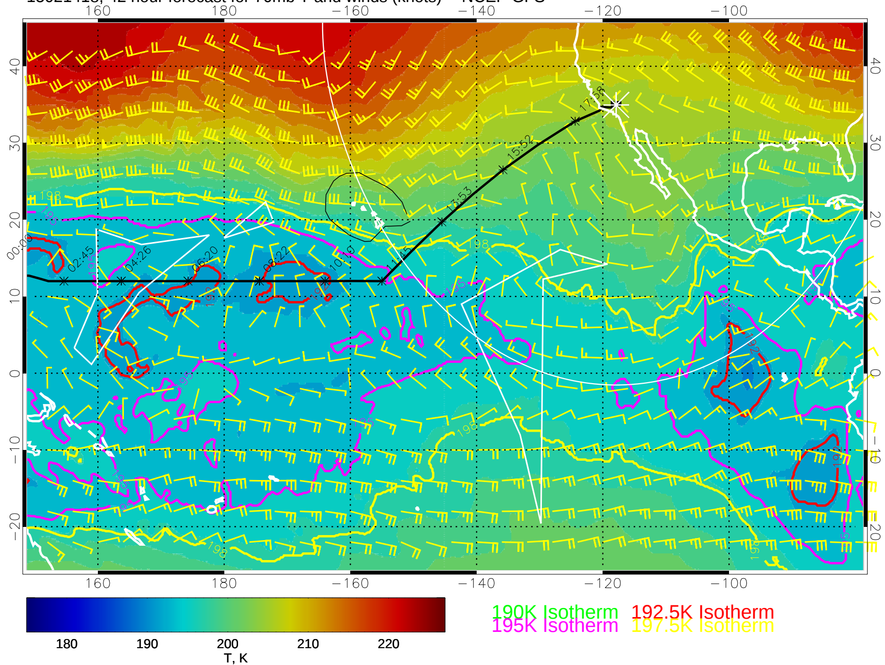
15021418, 42 hour forecast for 70mb T and winds (knots) -- NCEP GFS
