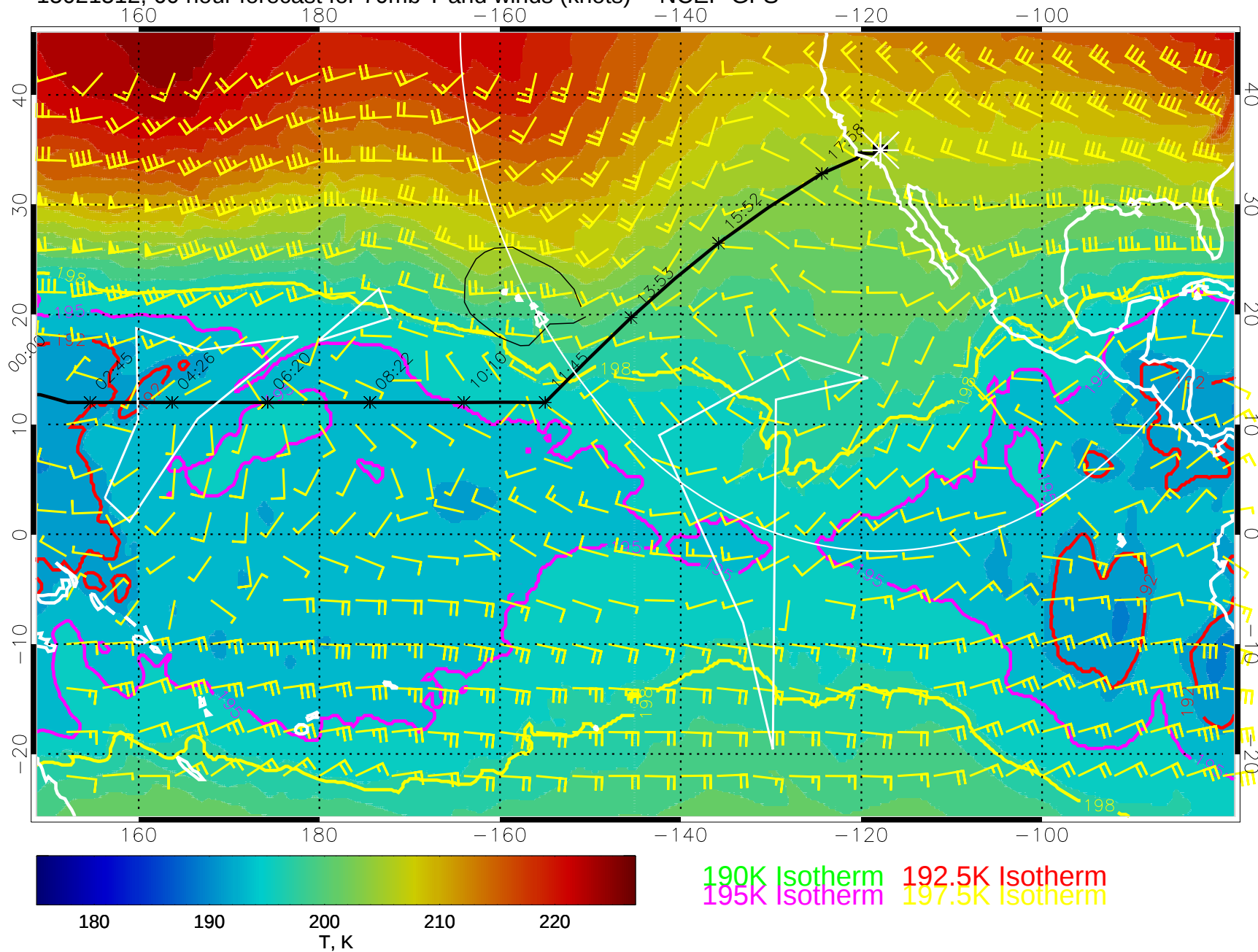
15021512, 60 hour forecast for 70mb T and winds (knots) -- NCEP GFS
