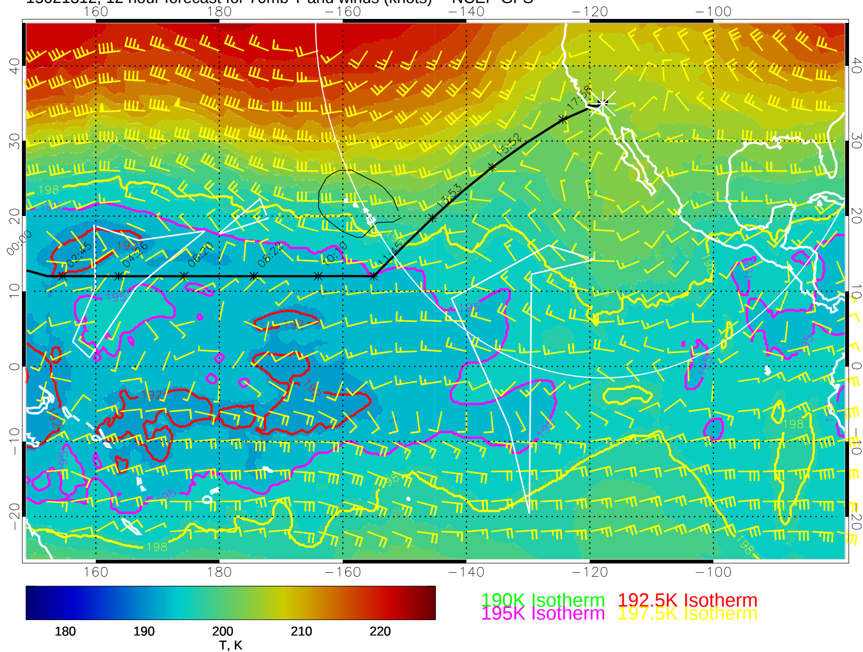
15021312, 12 hour forecast for 70mb T and winds (knots) -- NCEP GFS
