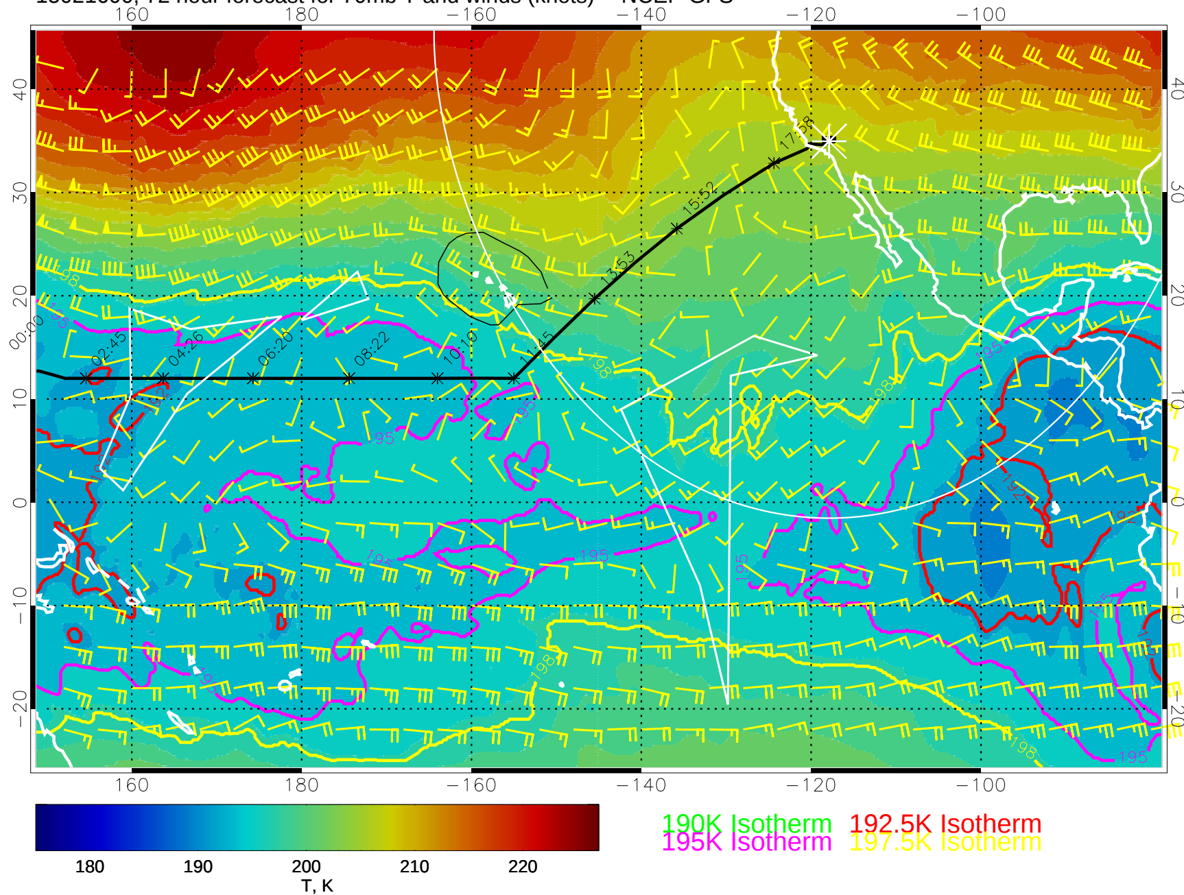
15021600, 72 hour forecast for 70mb T and winds (knots) -- NCEP GFS
