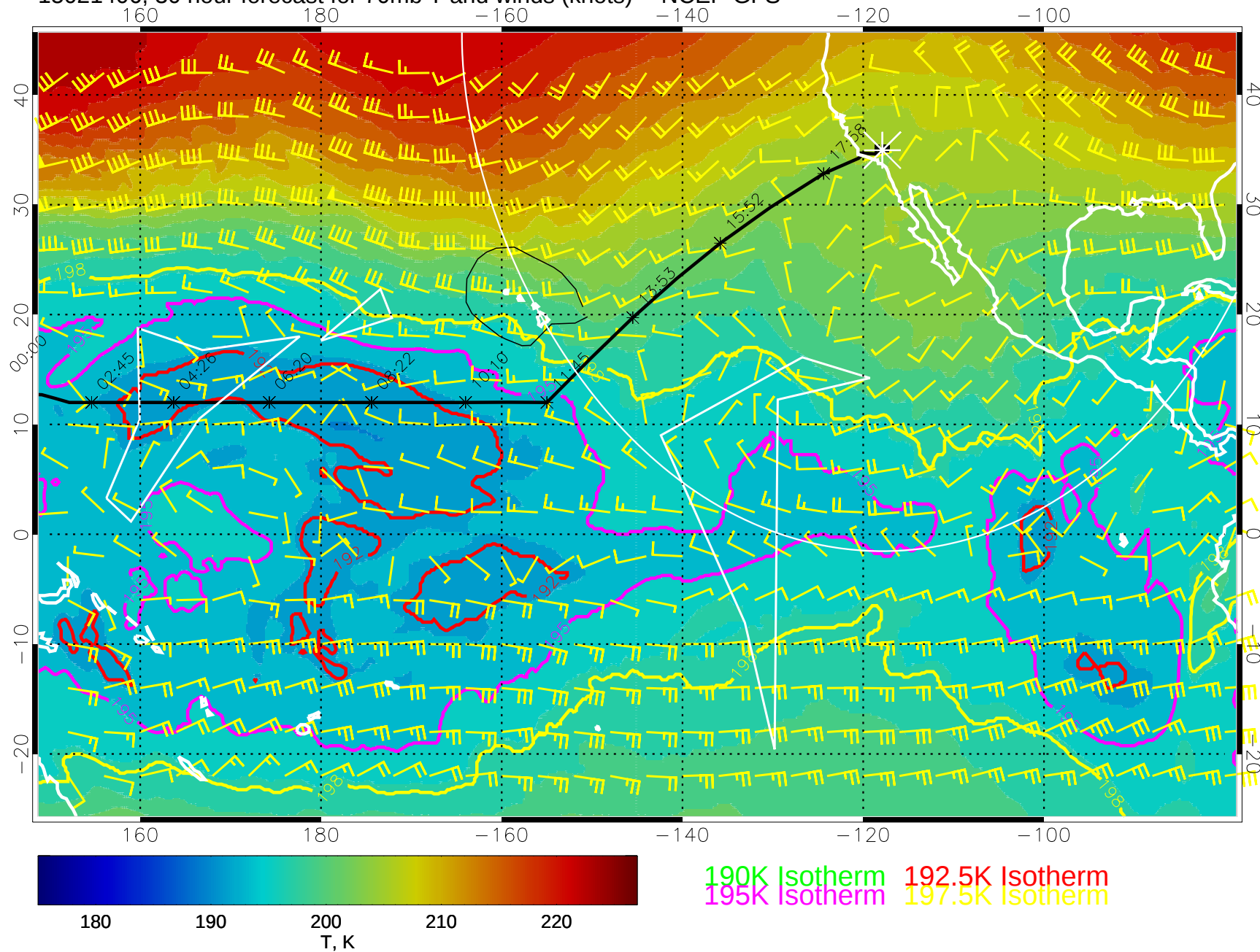
15021406, 30 hour forecast for 70mb T and winds (knots) -- NCEP GFS
