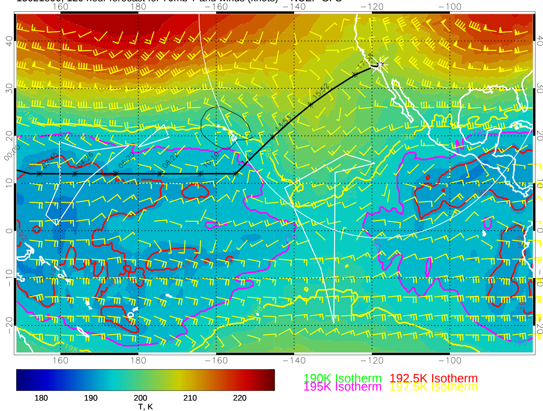
15021800, 120 hour forecast for 70mb T and winds (knots) -- NCEP GFS
