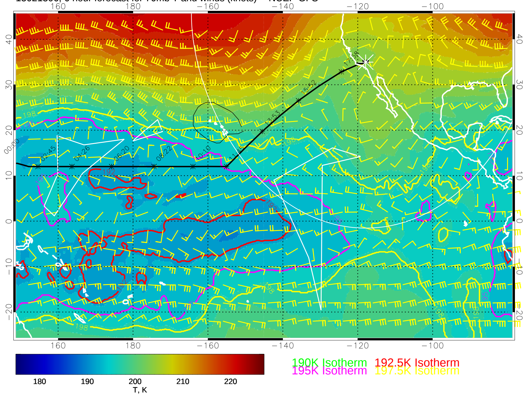
15021306, 6 hour forecast for 70mb T and winds (knots) -- NCEP GFS
