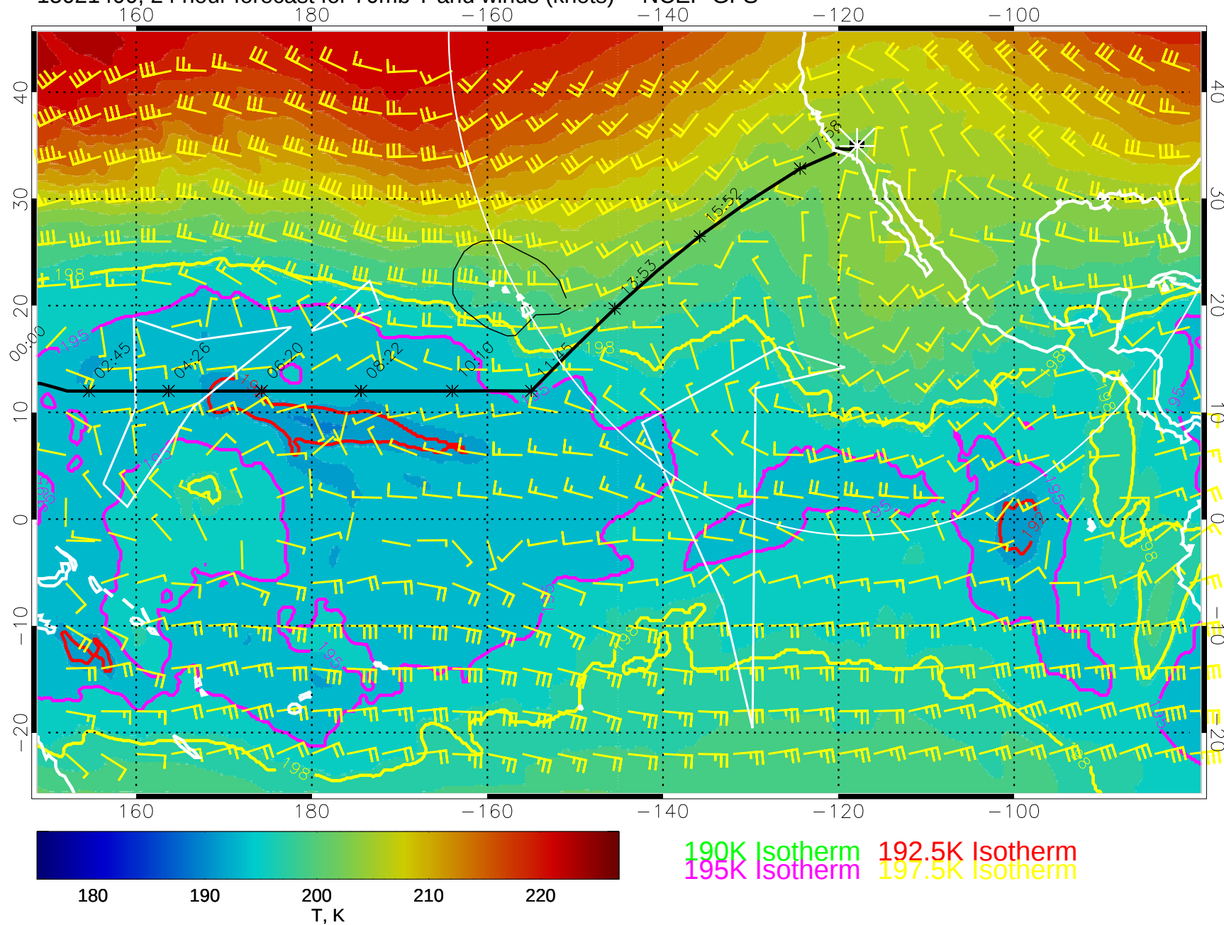
15021400, 24 hour forecast for 70mb T and winds (knots) -- NCEP GFS
