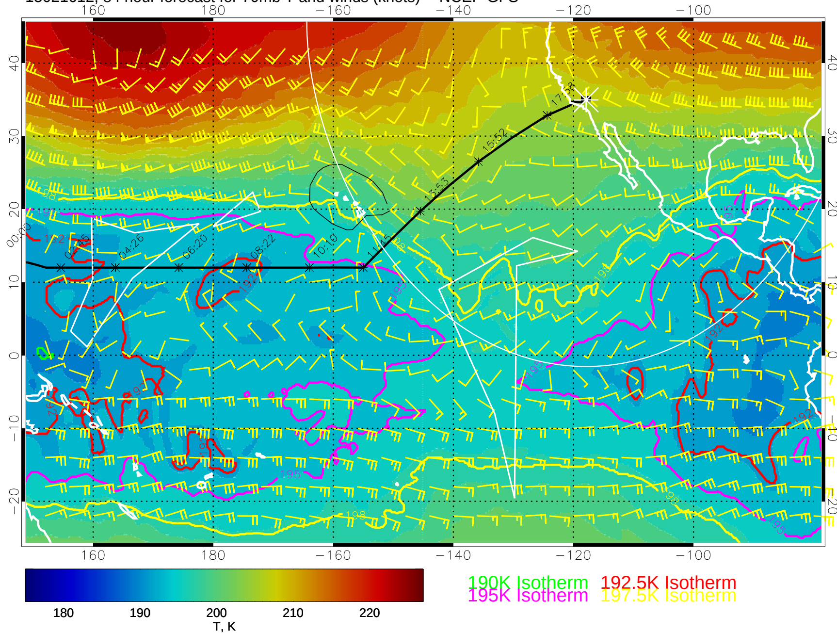
15021612, 84 hour forecast for 70mb T and winds (knots) -- NCEP GFS
