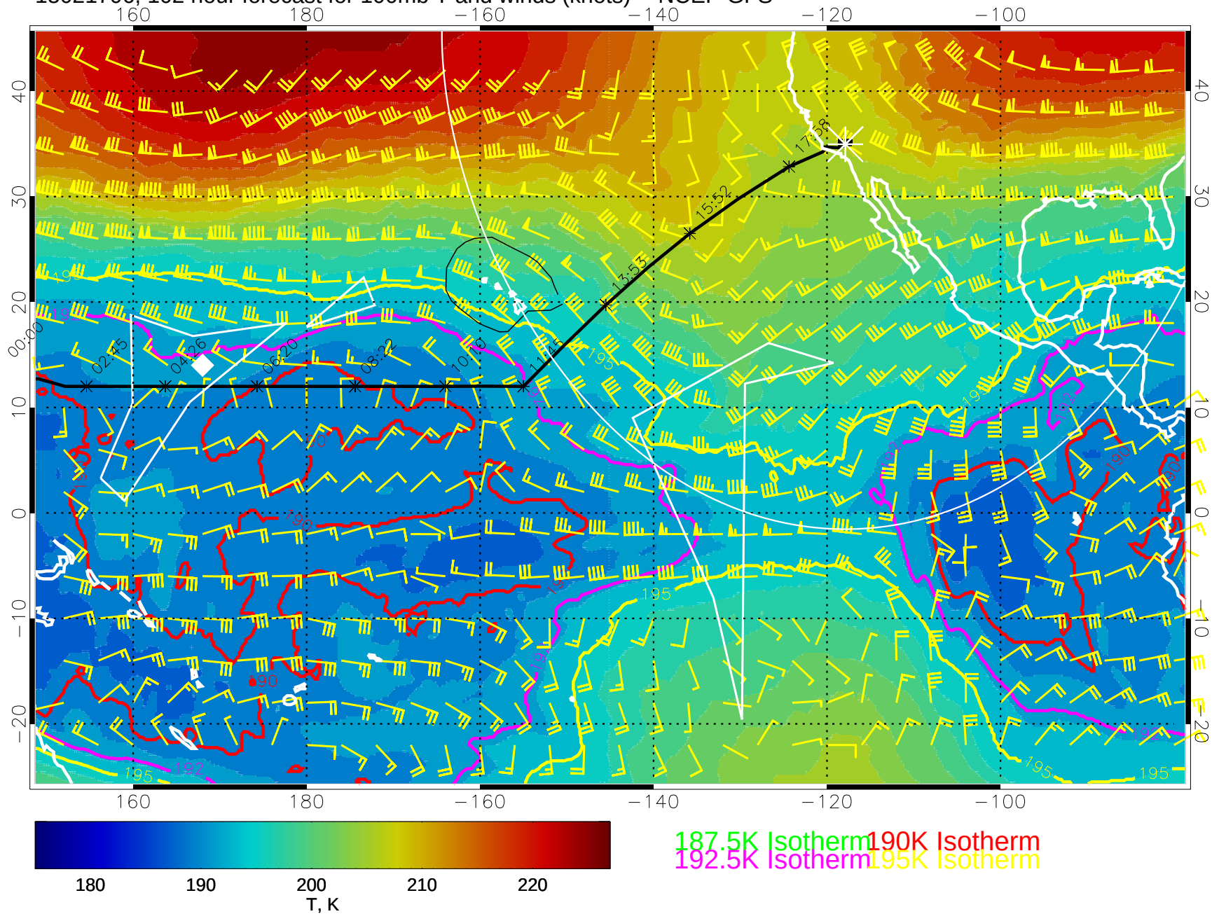
15021706, 102 hour forecast for 100mb T and winds (knots) -- NCEP GFS
