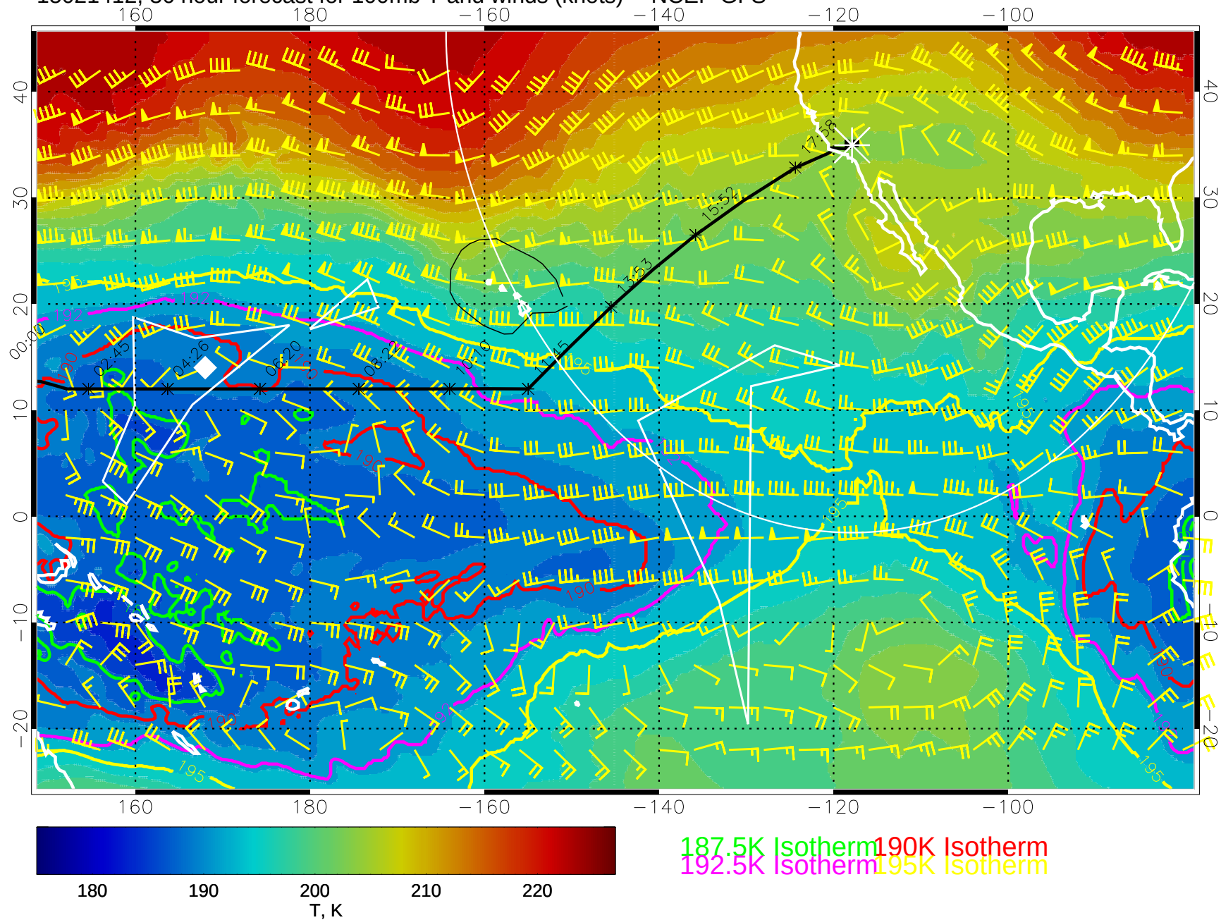
15021412, 36 hour forecast for 100mb T and winds (knots) -- NCEP GFS
